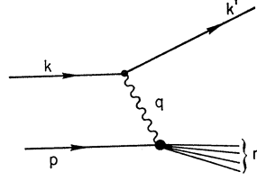
FIG. 1. The kinematics of inelastic electron-nucleon scattering.
