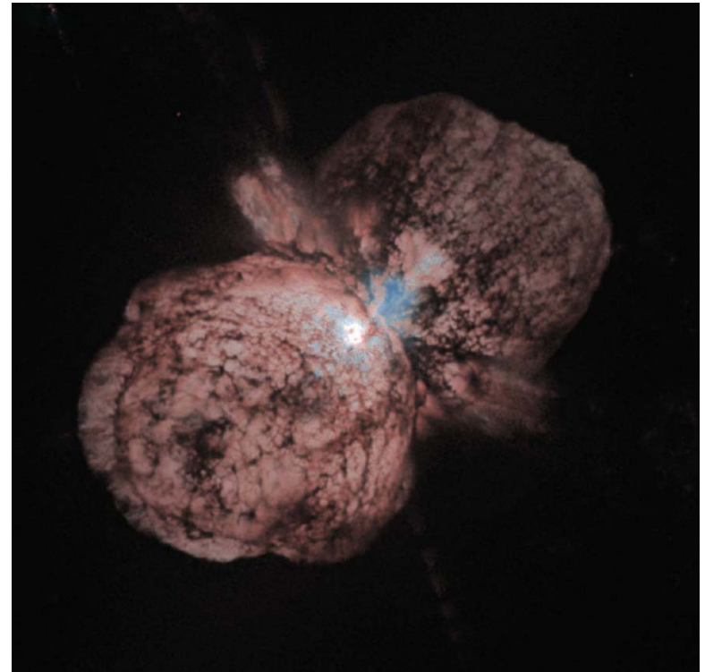
\eta Carinae, surrounded by the expanding debris from its outburst of 1820-1840 ( HST image by Jon Morse and Kris Davidson).
