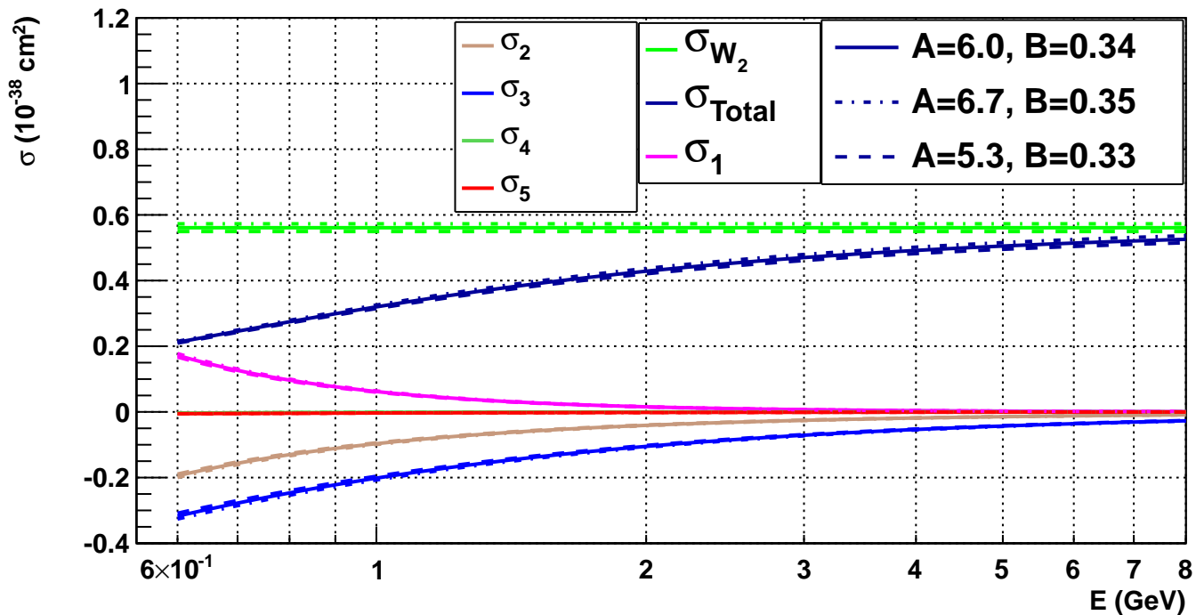
Contributions to Quasi-elastic \sigma_{\text{Total}} for Antineutrino ( \nu < 0.25 )
