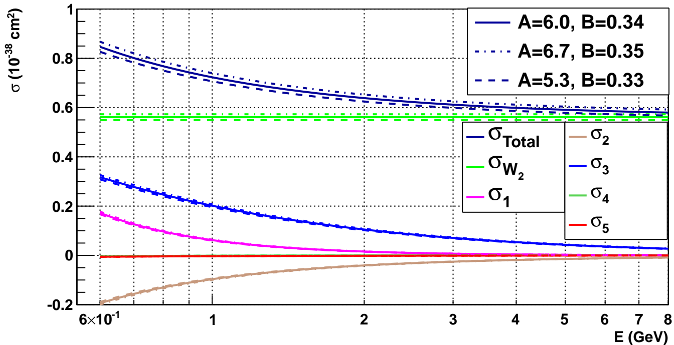
Contributions to Quasi-elastic \sigma_{\text{Total}} for Neutrino ( \nu < 0.25 )
