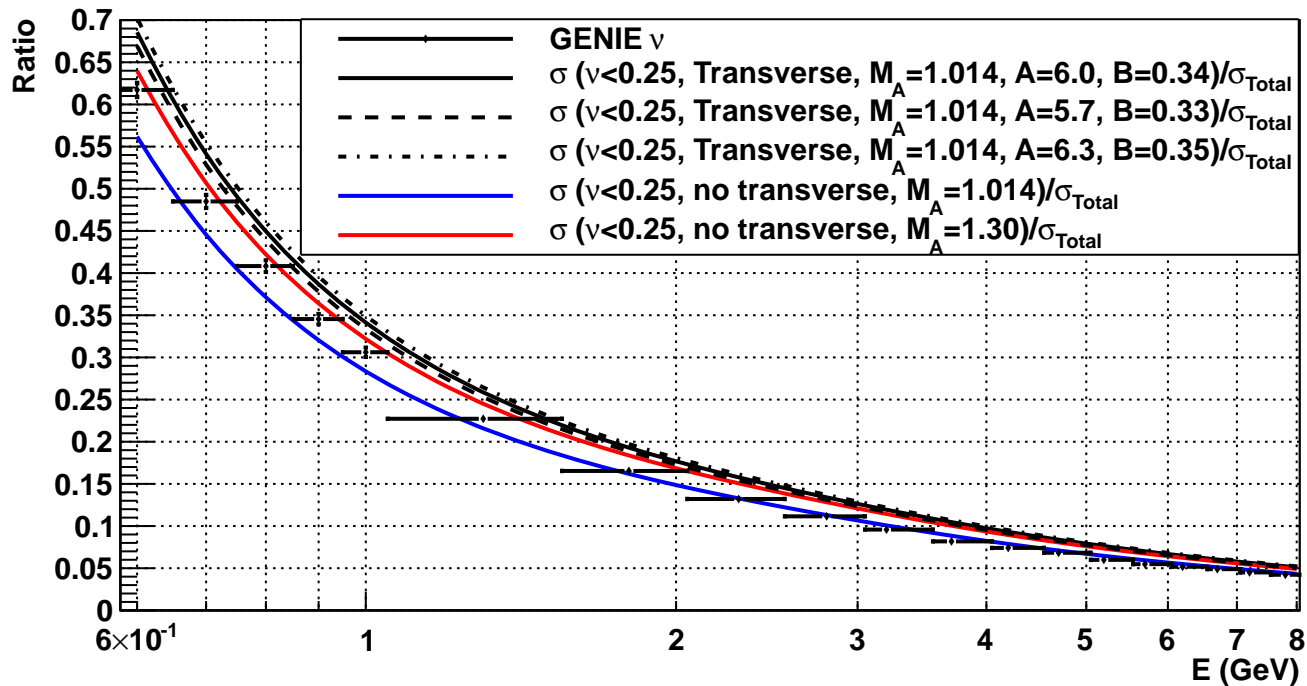
Fraction of \nu < 0.25 Cross Section to Total Cross Section for Neutrino
