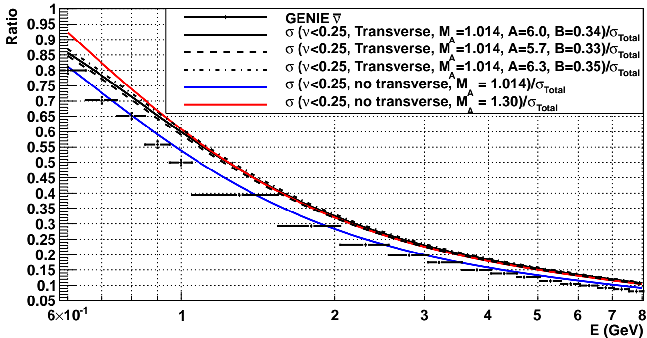
Fraction of \nu < 0.25 Cross Section to Total Cross Section for Antineutrino
