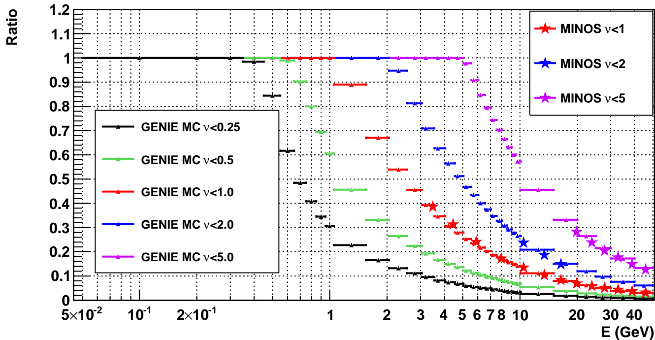
Fraction of Events with \nu Cut for Neutrino on Carbon
