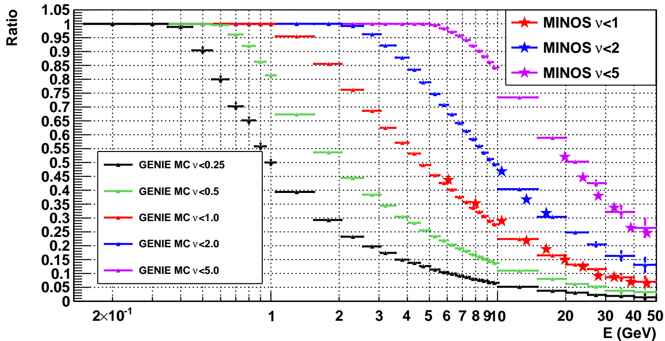
Fraction of Events with \nu Cut for Antineutrino on Carbon
