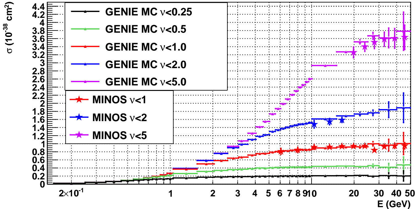
Cross Sections per Nucleon for Antineutrino on Carbon with \nu Cut
