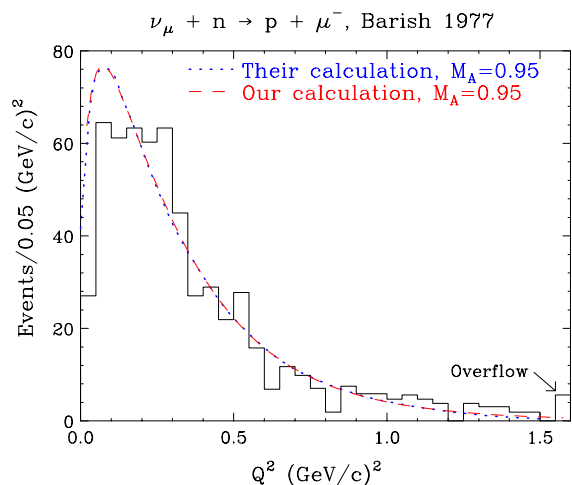
Figure 10. Q^2 distribution from Barish et al. [10]. The dotted curve is their calculation taken from their Q^2 distribution histogram. The dashed curve is our calculation using their assumptions.
