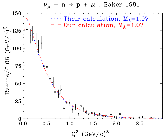
Figure 9. Q^2 distribution from Baker et al. [9]. The dotted curve is their calculation taken from their Q^2 distribution histogram. The dashed curve is our calculation using their assumptions.
