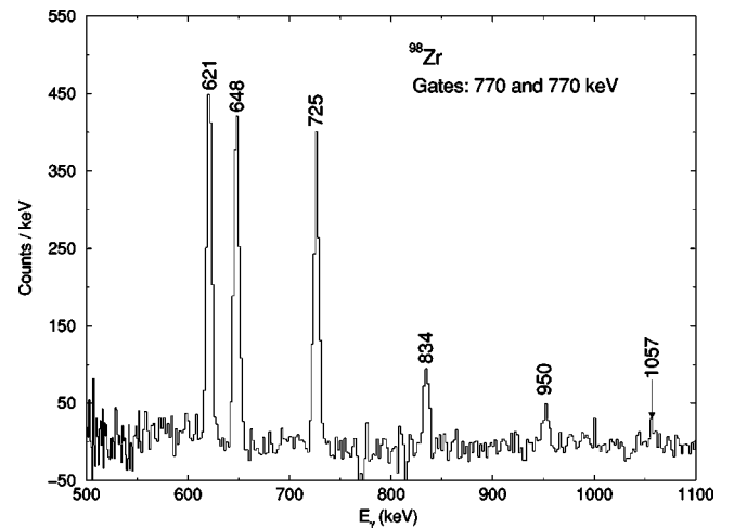
FIG. 4. Doppler-shift corrected prompt \gamma -ray spectrum derived from a double gate placed on the same prompt \gamma -ray energy, 770 keV, in ^{98}\text{Zr} .
