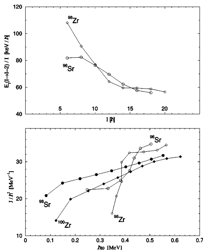
FIG. 5. Kinematic moment of inertia as a function of rotational frequency for the yrast states with spin above 4^+ in ^{96}\text{Sr} and ^{98}\text{Zr} and for the ground-state bands in ^{98}\text{Sr} and ^{100}\text{Zr} (bottom). The 911.3, 1010.3, and 1104.6 keV \gamma rays were assigned, for the first time, to the 14^+ \rightarrow 12^+ , 16^+ \rightarrow 14^+ , and 18^+ \rightarrow 16^+ transitions, respectively, in ^{98}\text{Sr} from the present work. E-GOS plots for the yrast states in ^{96}\text{Sr} and ^{98}\text{Zr} (top).
