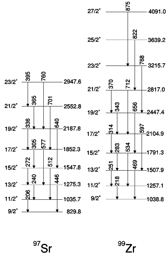
FIG. 12. Level schemes of rotational bands built on the 9/2^+[404] neutron configuration in ^{97}\text{Sr} and ^{99}\text{Zr} . Energies are in keV and the uncertainty on the transition energies is \approx 1 keV.
