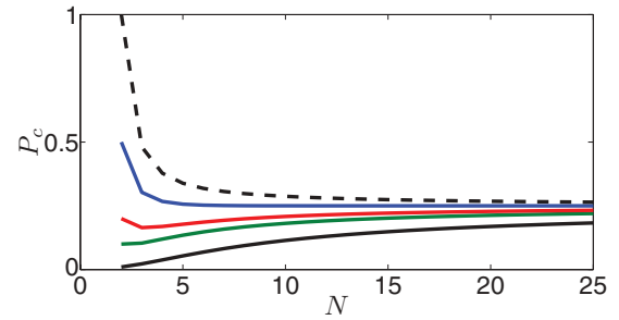
FIG. 2. (Color online) P_c vs number of qubits for different initial states |\Phi_N^{(0)}, \alpha\rangle . From bottom up \tan \alpha = 0.01, 0.1, 0.2, 0.5 , and 1 respectively.
