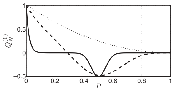
FIG. 1. The Q_N^{(0)} vs P for different numbers of qubits for the initial state |\Phi_N^{(0)}, \frac{\pi}{4}\rangle . N = 2 is the dotted line, N = 10 is the dashed line, and N = 100 is the solid line.
