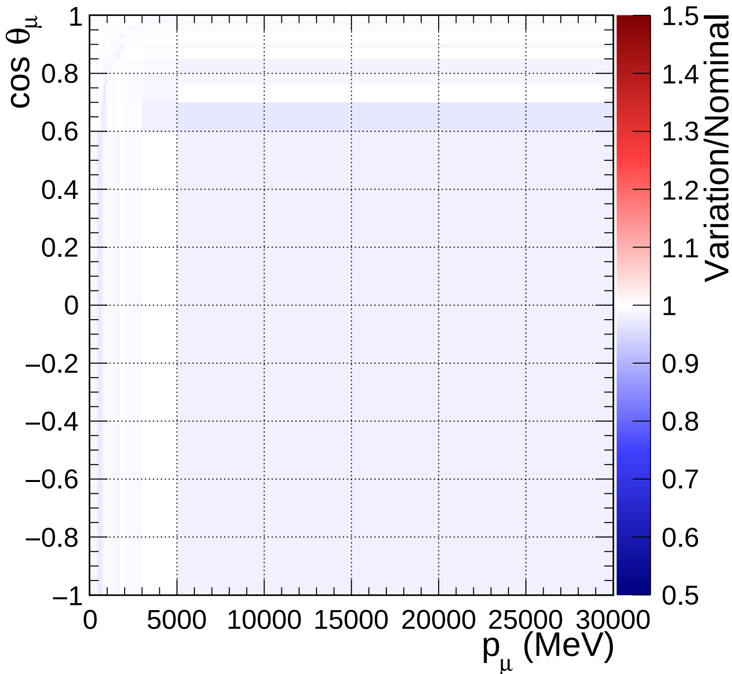
FGD2_numuCC_other_Q2_norm_6_0.46
