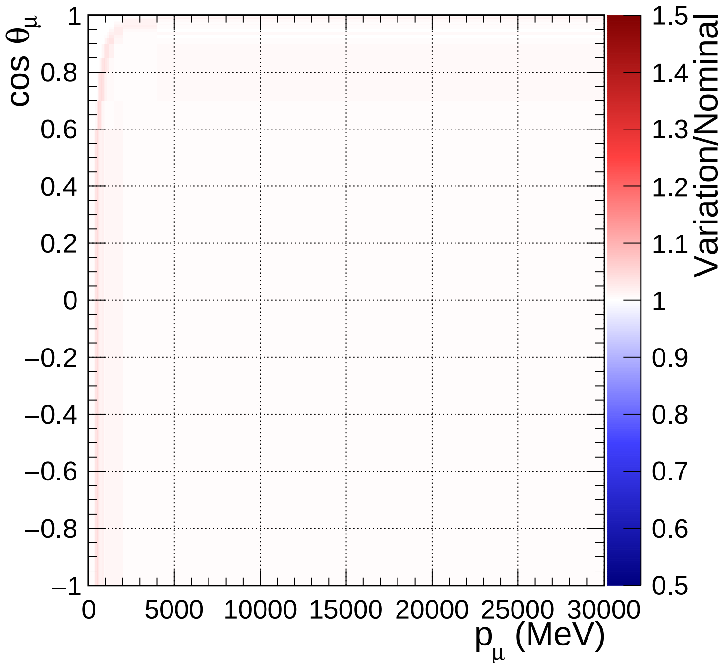
FGD1_anti-numuCC_0pi_Q2_norm_5_1.11
