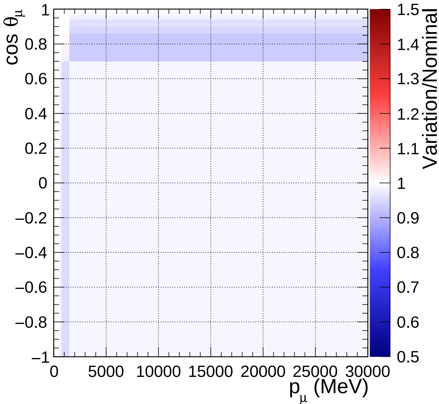
FGD2_NuMuBkg_CC1pi_in_AntiNu_Mode_Q2_norm_7_-0.2
