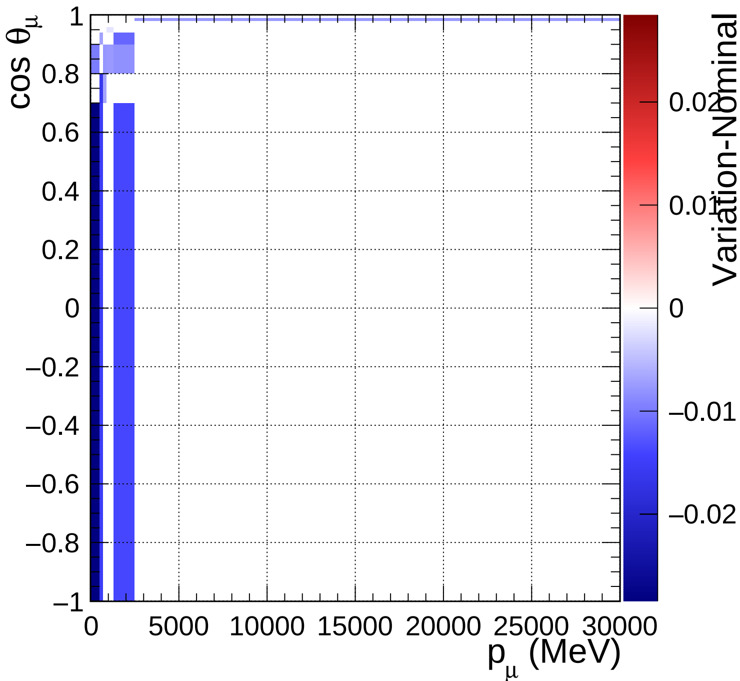
FGD1_anti-numuCC_1pi_Q2_norm_5_0.89
