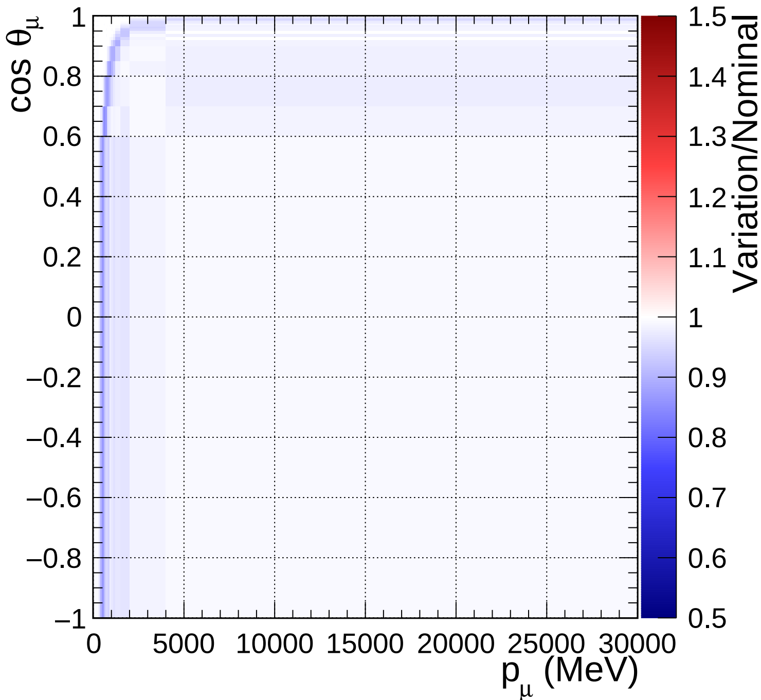
FGD1_anti-numuCC_0pi_Q2_norm_5_0.67
