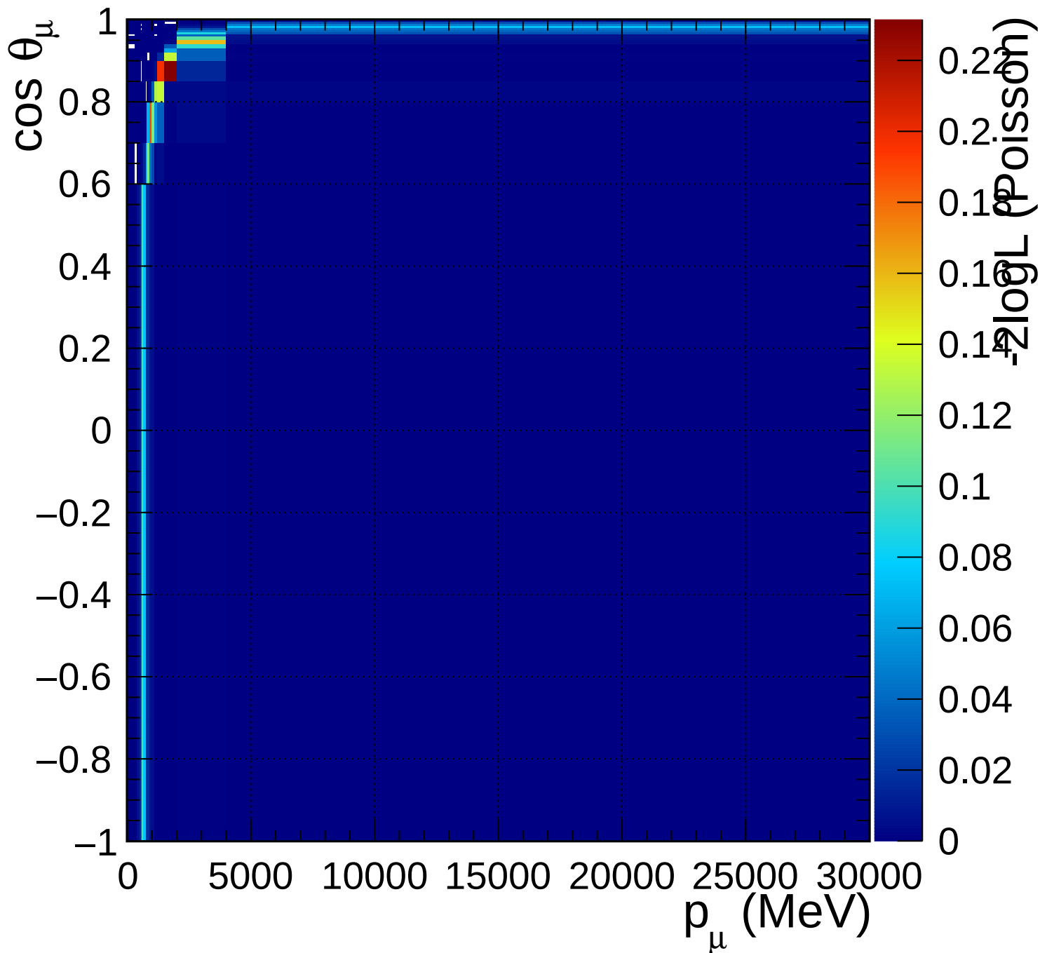
FGD1_anti-numuCC_0pi_Q2_norm_6_0.46
