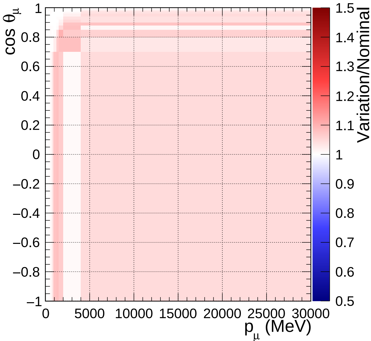
FGD2_NuMuBkg_CC0pi_in_AntiNu_Mode_Q2_norm_7_1.4
