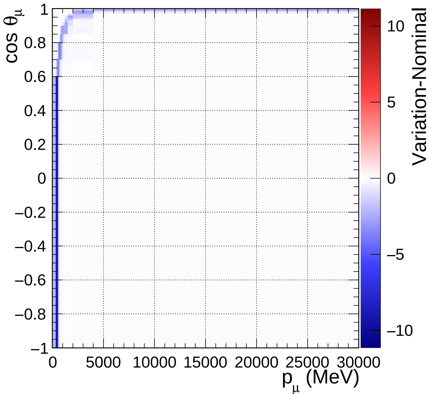
FGD2_anti-numuCC_0pi_Q2_norm_5_0.67
