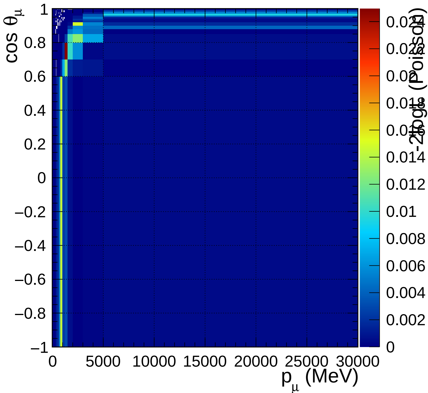
FGD2_numuCC_1pi_Q2_norm_7_0.6
