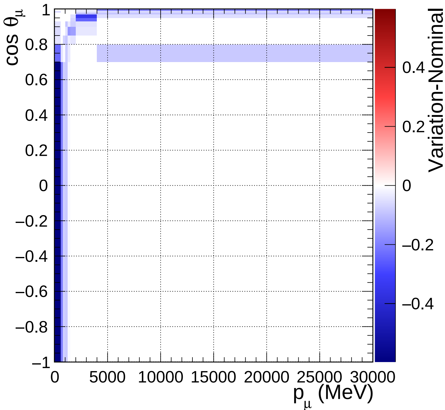
FGD2_anti-numuCC_other_Q2_norm_6_0.46
