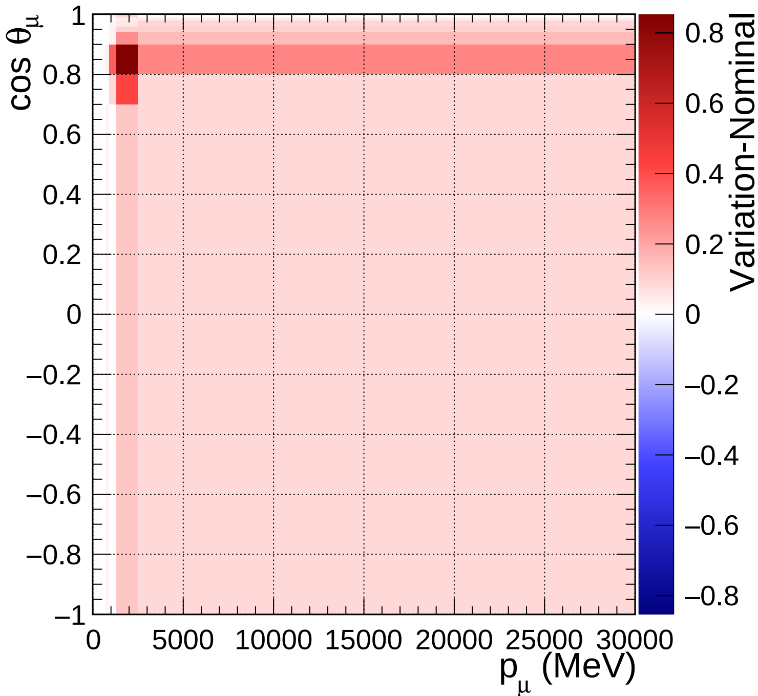
FGD2_anti-numuCC_1pi_Q2_norm_7_1.4
