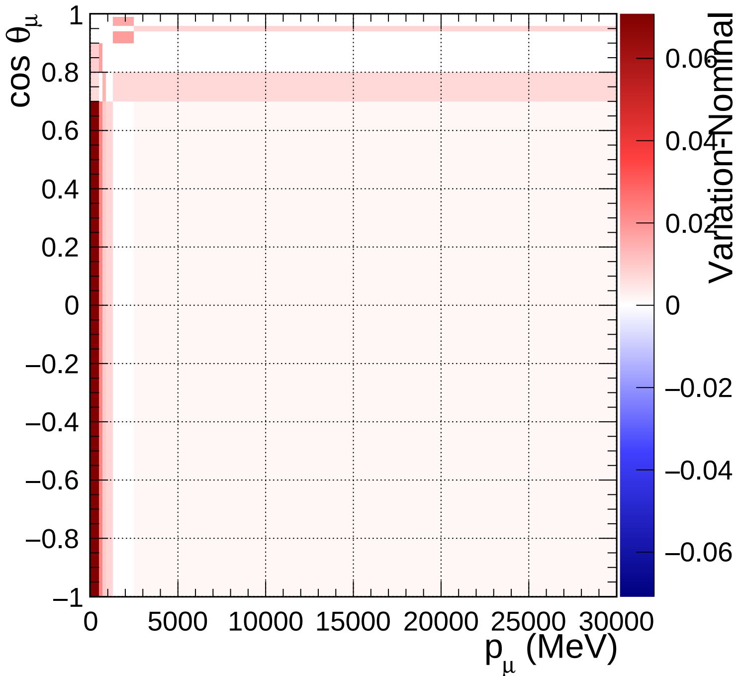
FGD2_anti-numuCC_1pi_Q2_norm_5_1.11
