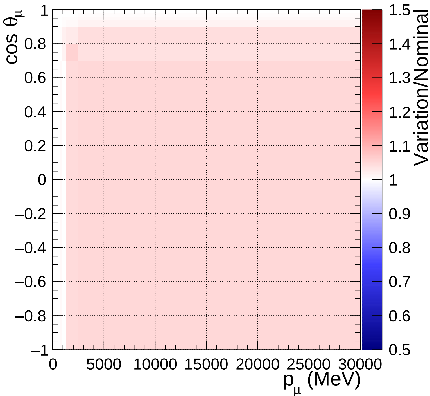
FGD2_anti-numuCC_1pi_Q2_norm_7_1.4
