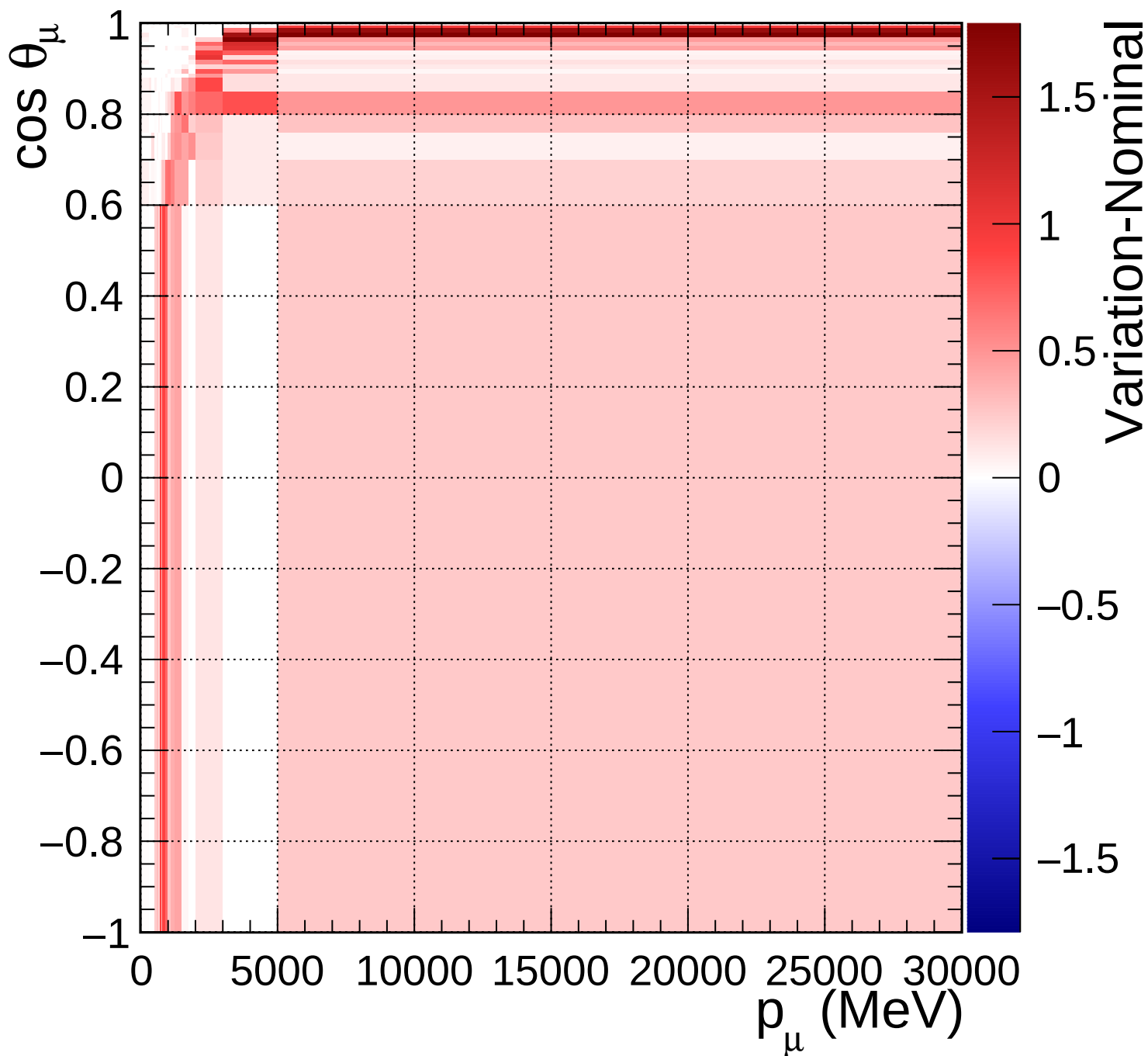
FGD1_numuCC_other_Q2_norm_7_2.2
