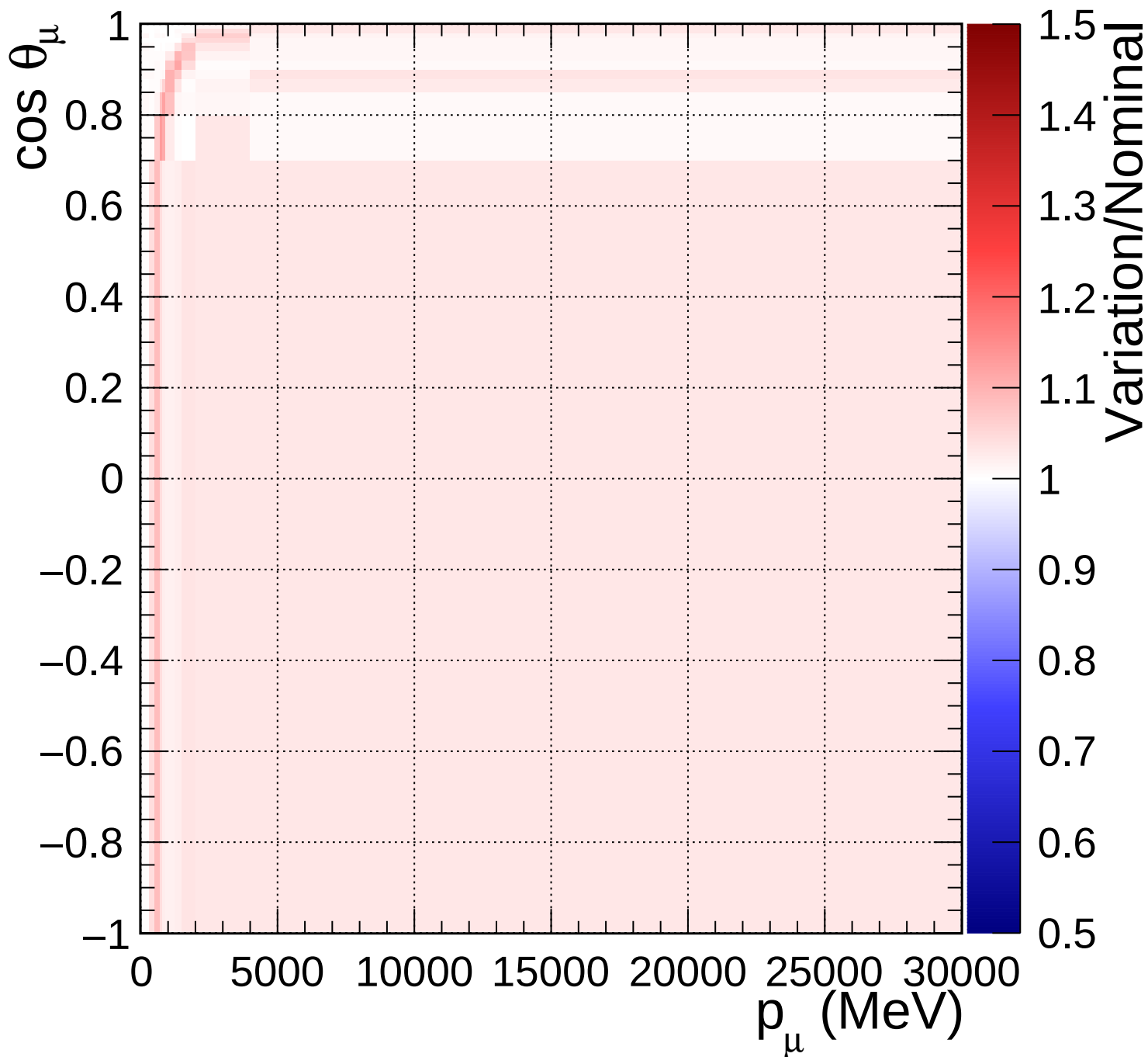
FGD1_NuMuBkg_CC0pi_in_AntiNu_Mode_Q2_norm_5_1.33
