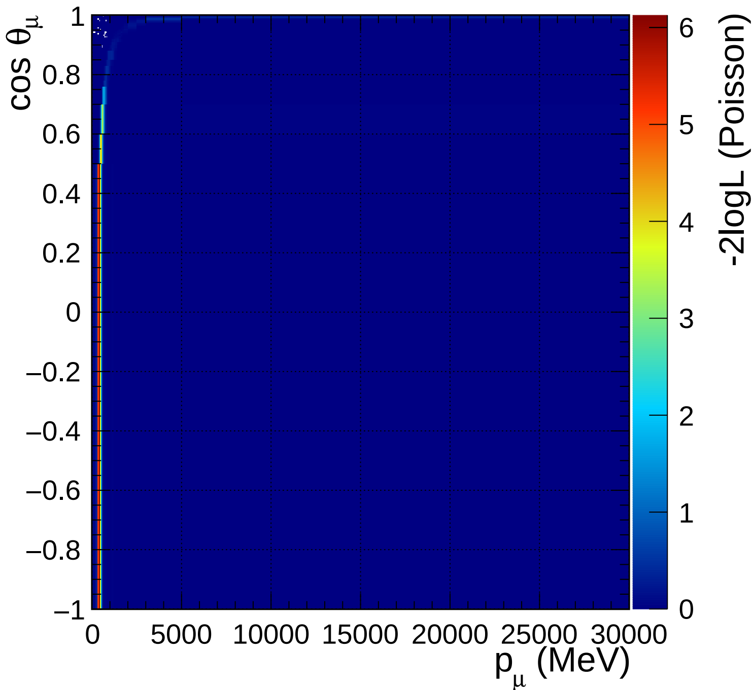
FGD1_numuCC_0pi_Q2_norm_5_0.67
