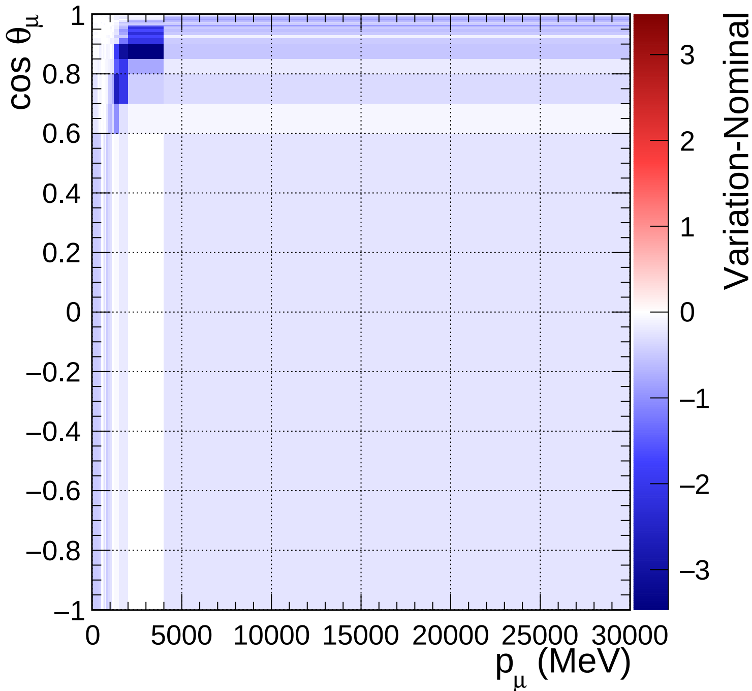
FGD2_anti-numuCC_0pi_Q2_norm_7_-0.2
