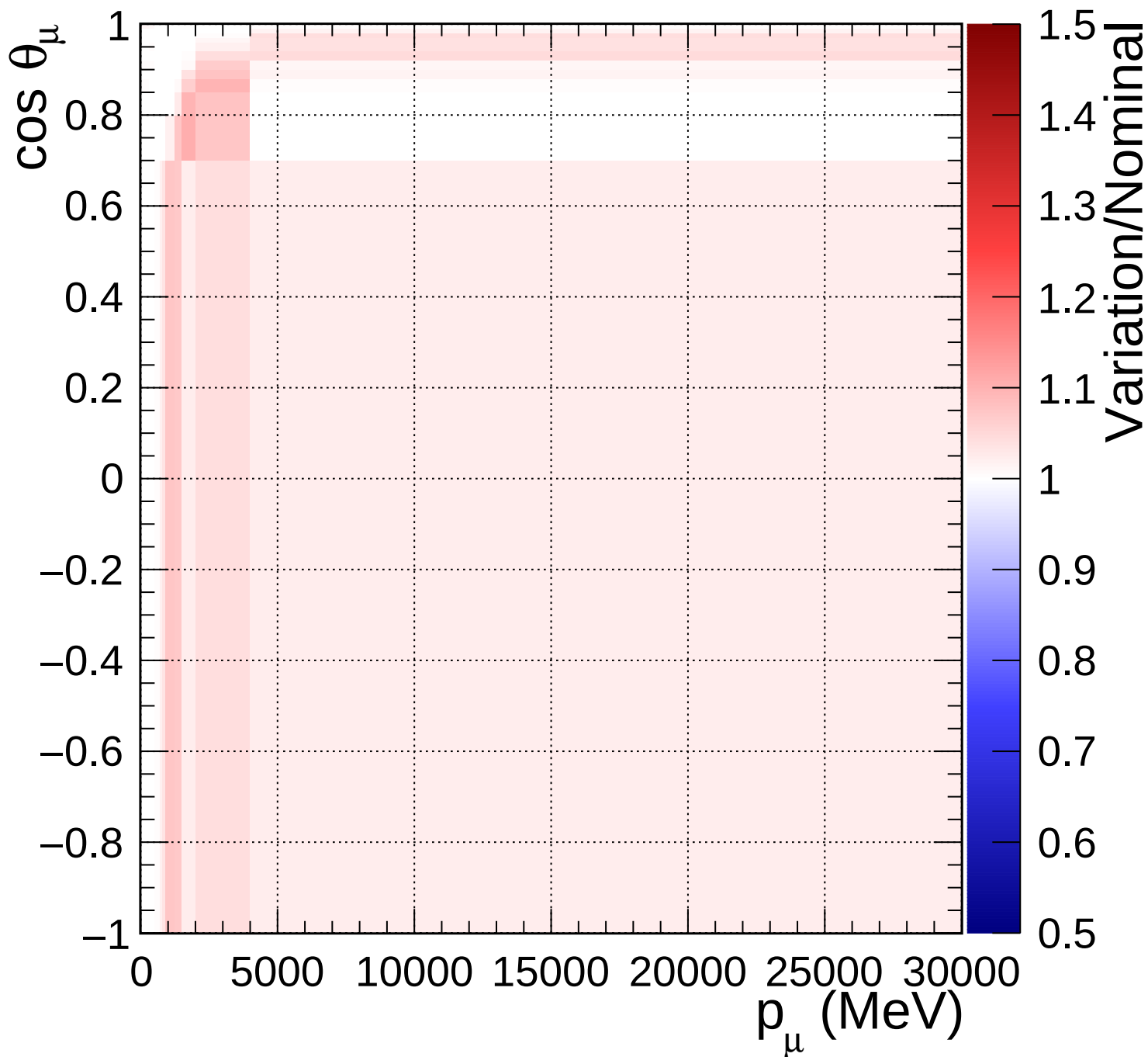
FGD1_NuMuBkg_CC0pi_in_AntiNu_Mode_Q2_norm_7_1.4
