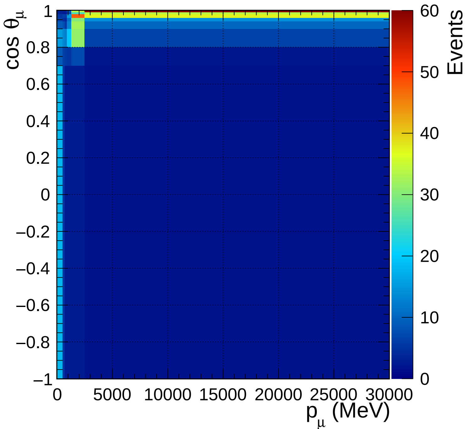
FGD2_anti-numuCC_1pi_Q2_norm_5_1
