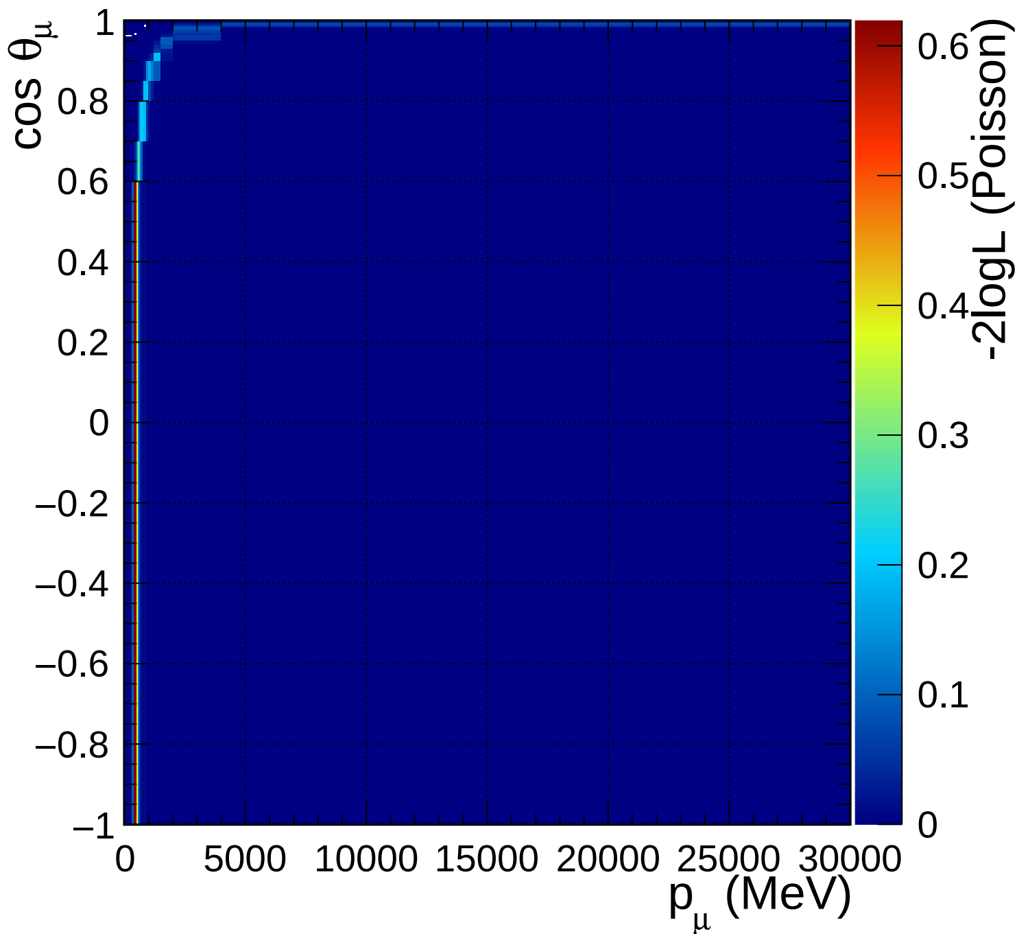
FGD1_anti-numuCC_0pi_Q2_norm_5_1.33
