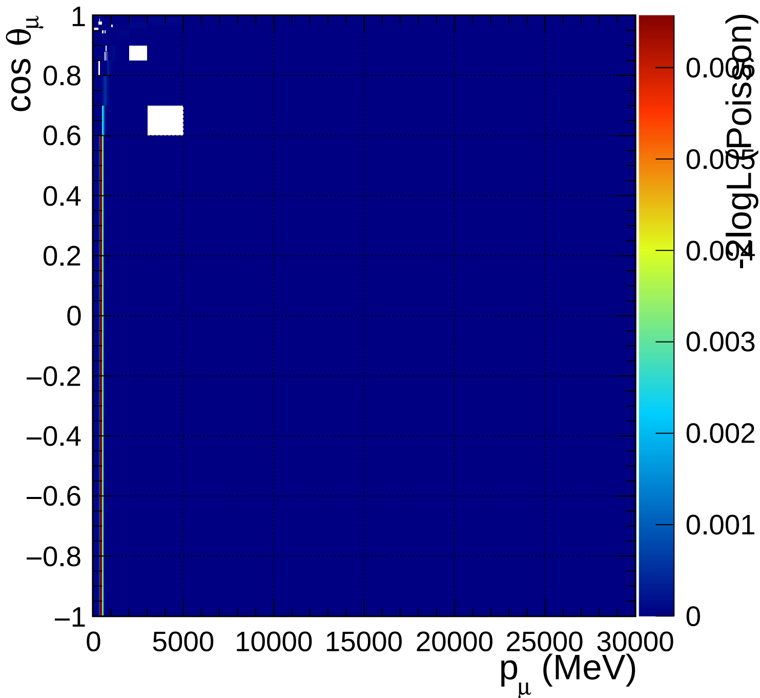
FGD1_numuCC_1pi_Q2_norm_5_1.11
