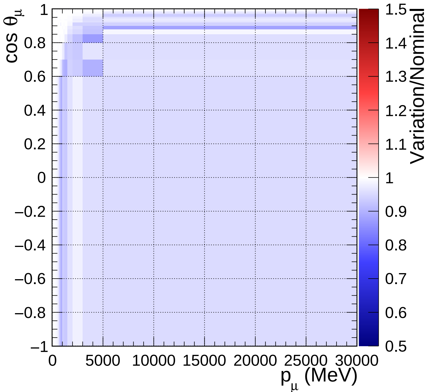
FGD2_numuCC_1pi_Q2_norm_7_-0.2
