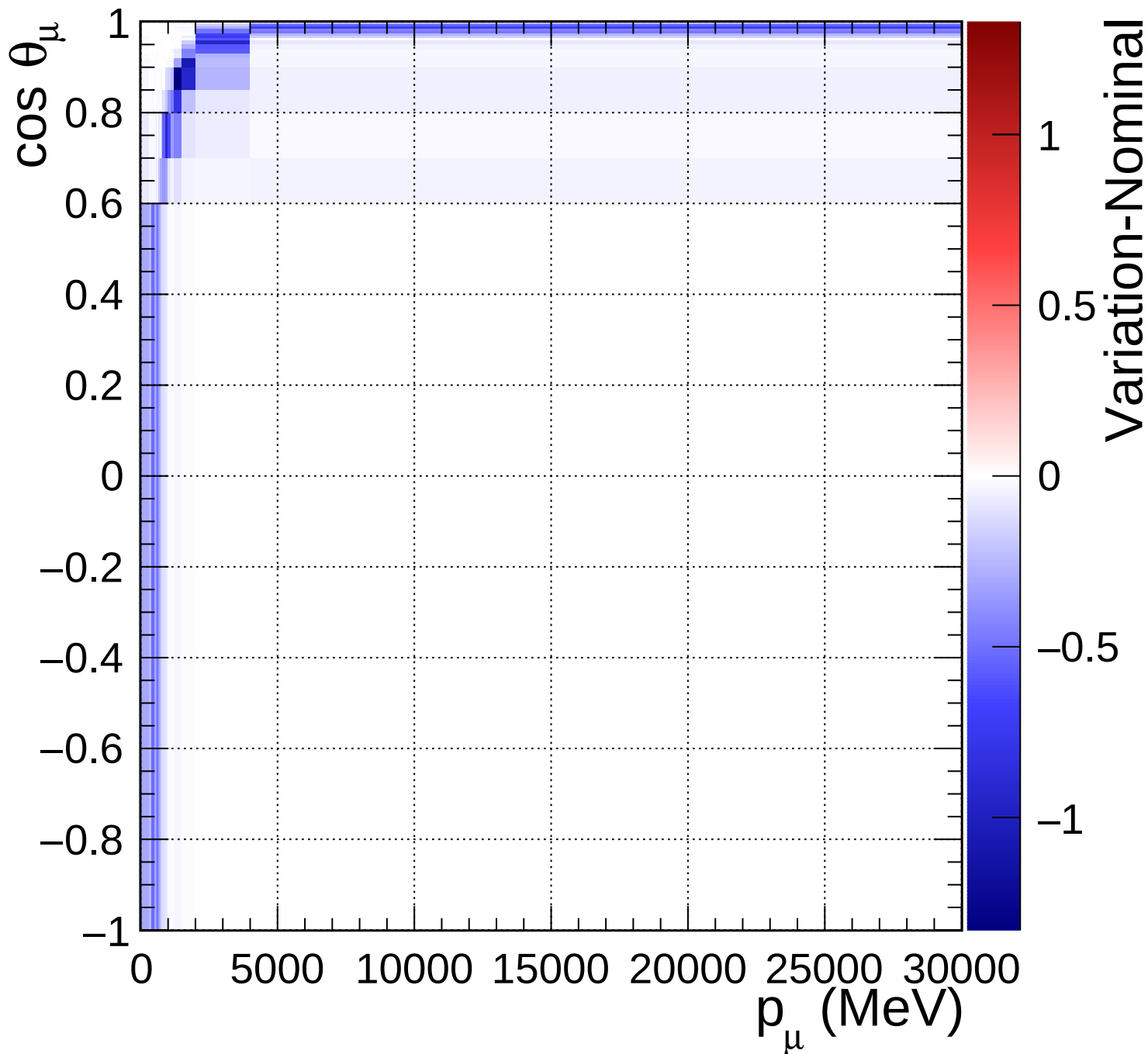
FGD2_anti-numuCC_0pi_Q2_norm_6_0.82
