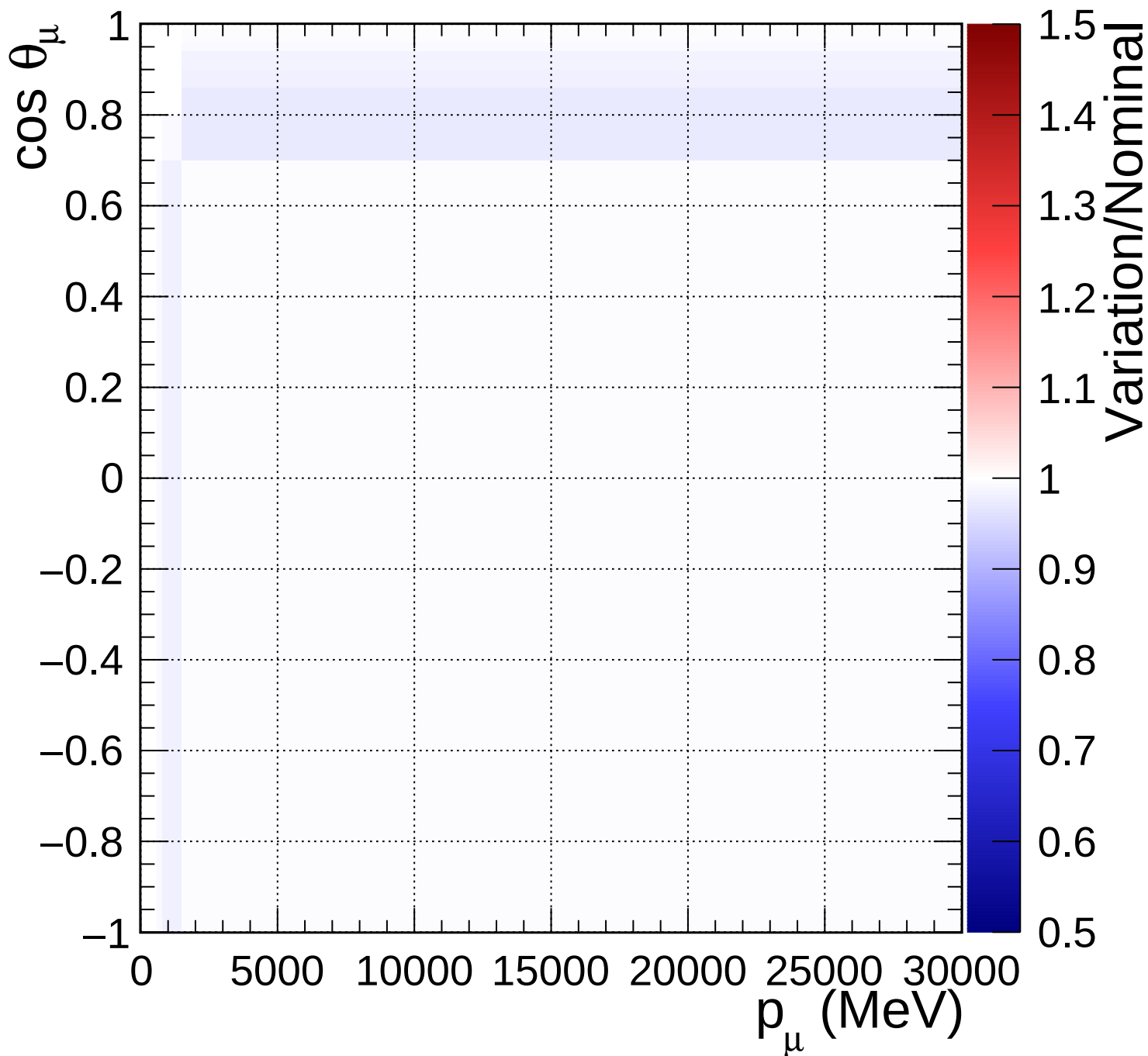
FGD2_NuMuBkg_CC1pi_in_AntiNu_Mode_Q2_norm_7_0.6
