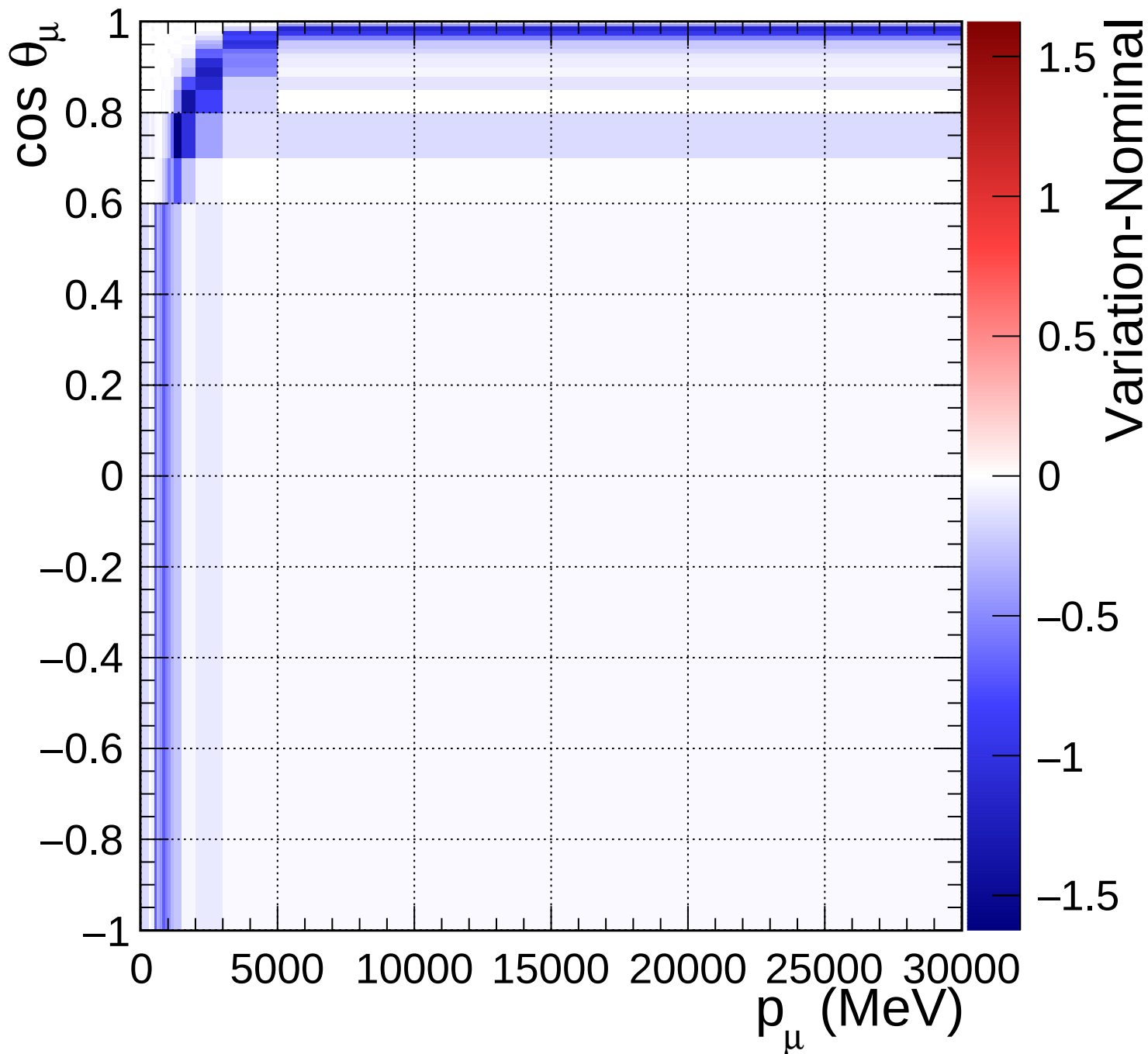
FGD1_numuCC_1pi_Q2_norm_7_0.6
