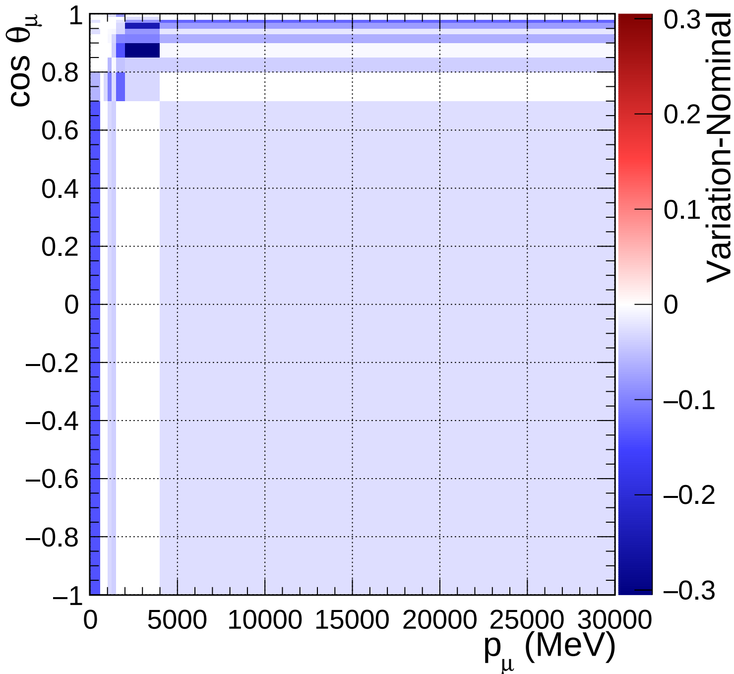
FGD2_anti-numuCC_other_Q2_norm_7_0.6
