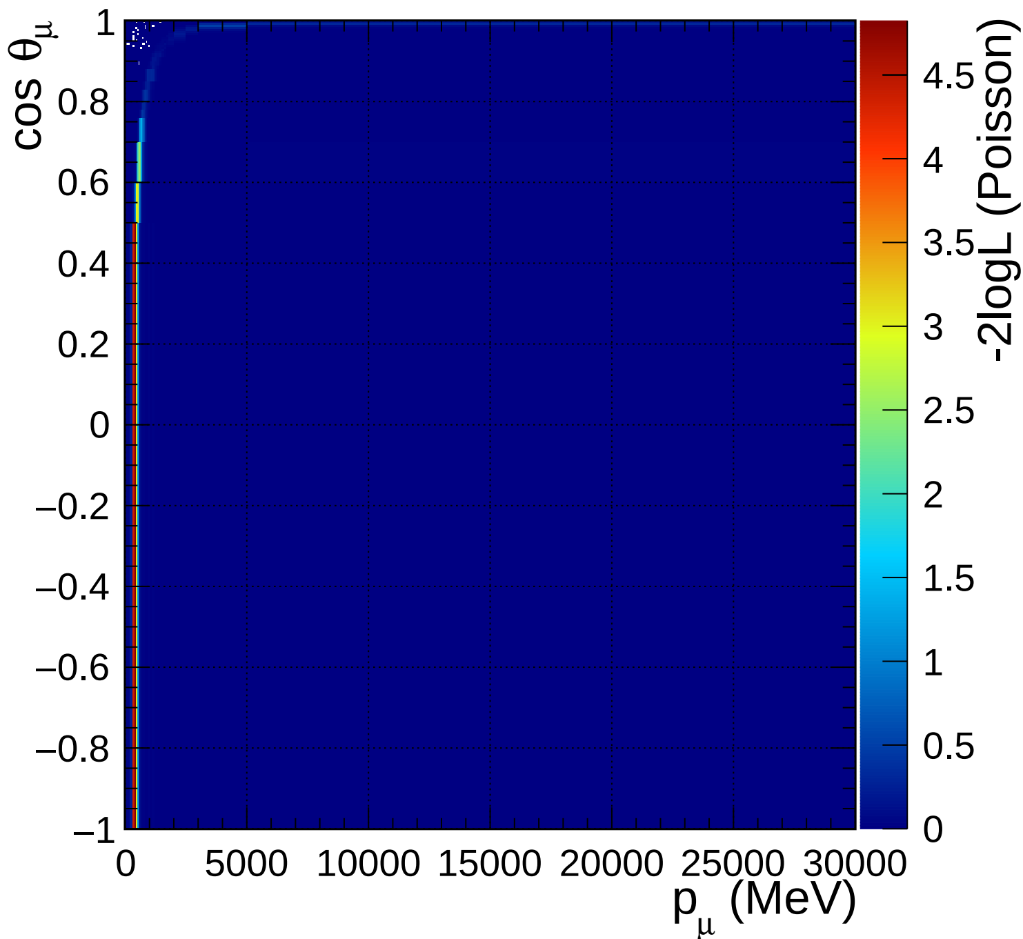
FGD1_numuCC_0pi_Q2_norm_5_1.33
