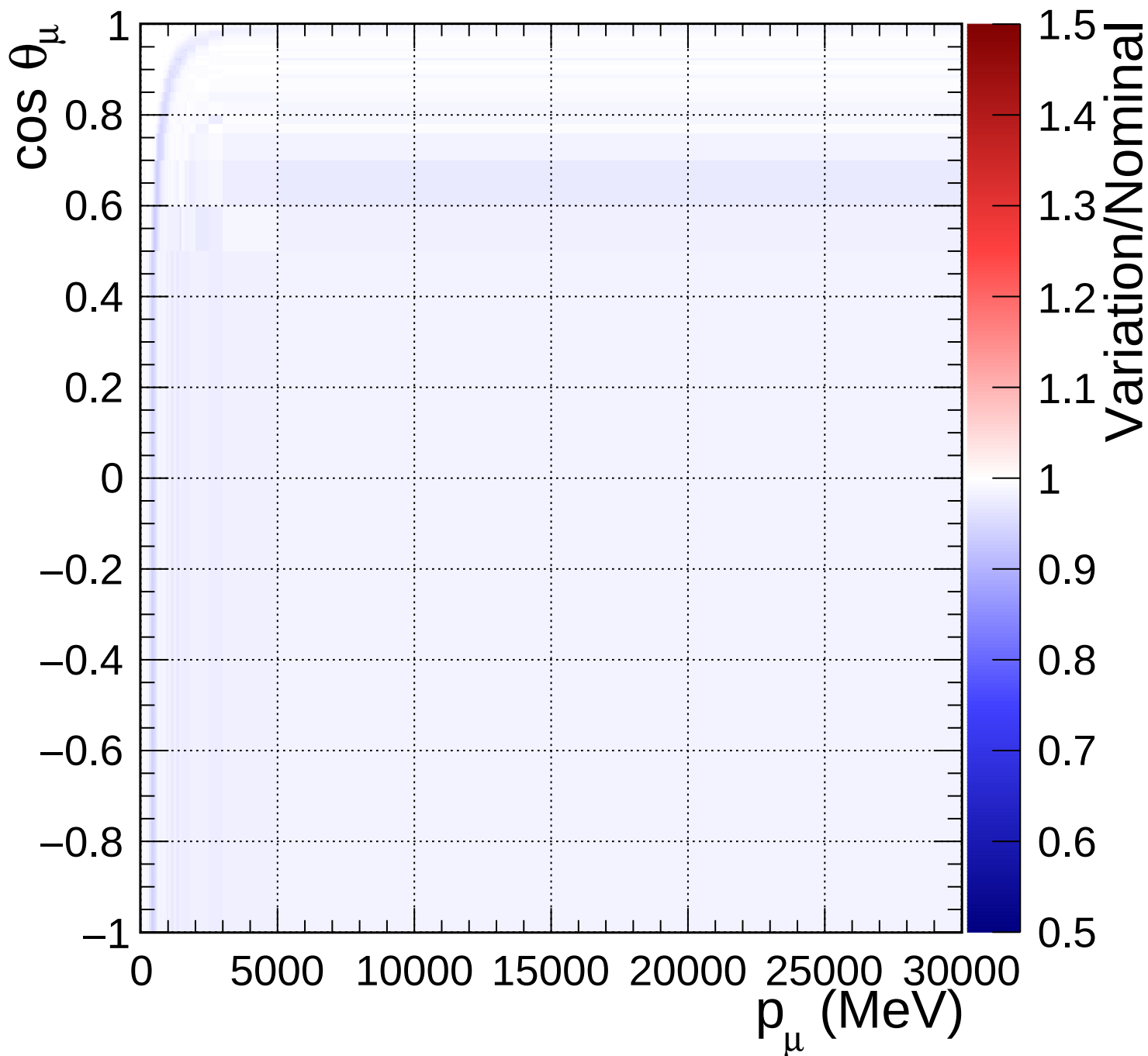
FGD1_numuCC_0pi_Q2_norm_5_0.89
