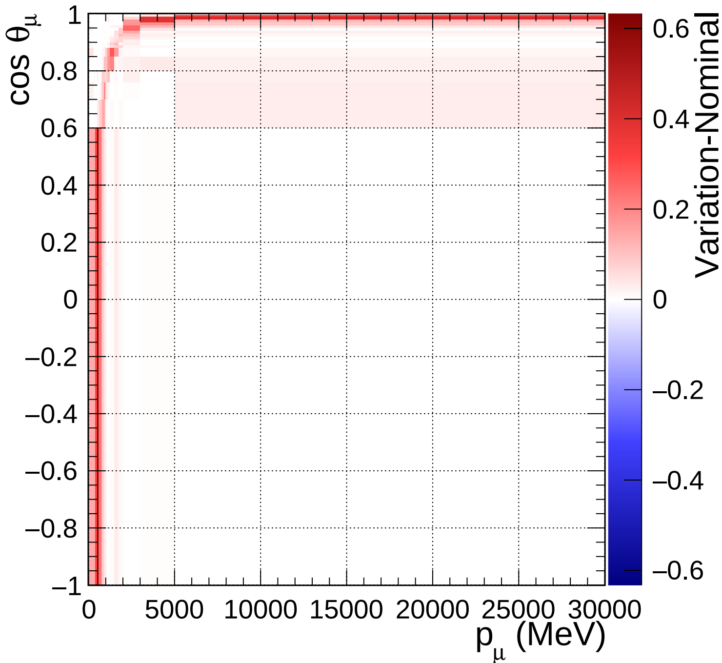
FGD1_numuCC_other_Q2_norm_6_1.18
