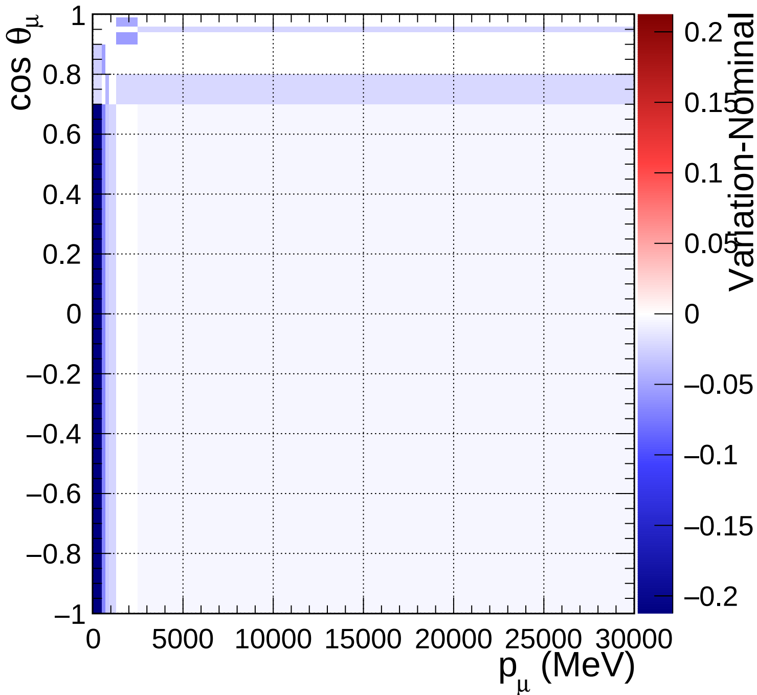
FGD2_anti-numuCC_1pi_Q2_norm_5_0.67
