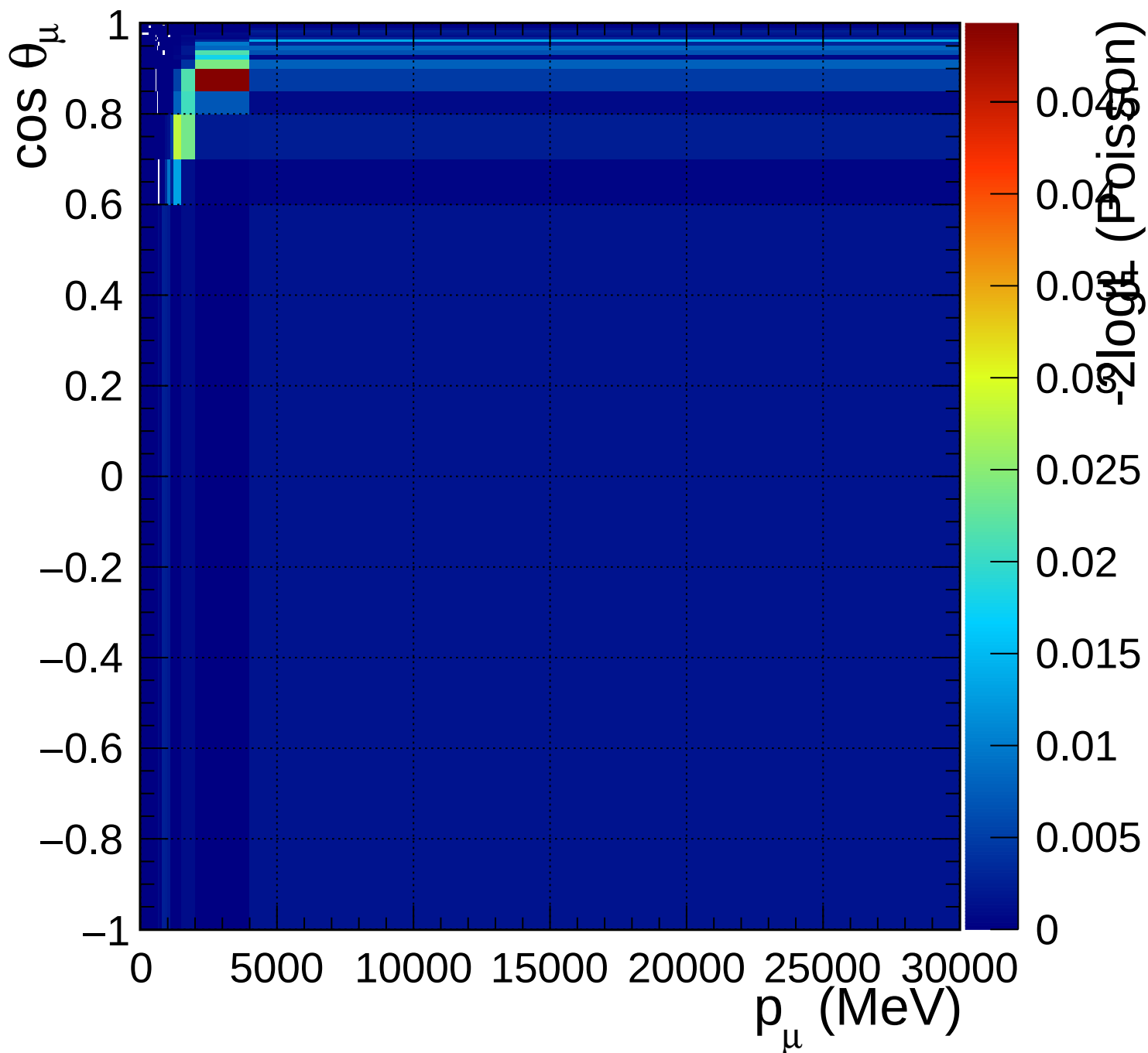
FGD2_anti-numuCC_0pi_Q2_norm_7_0.6
