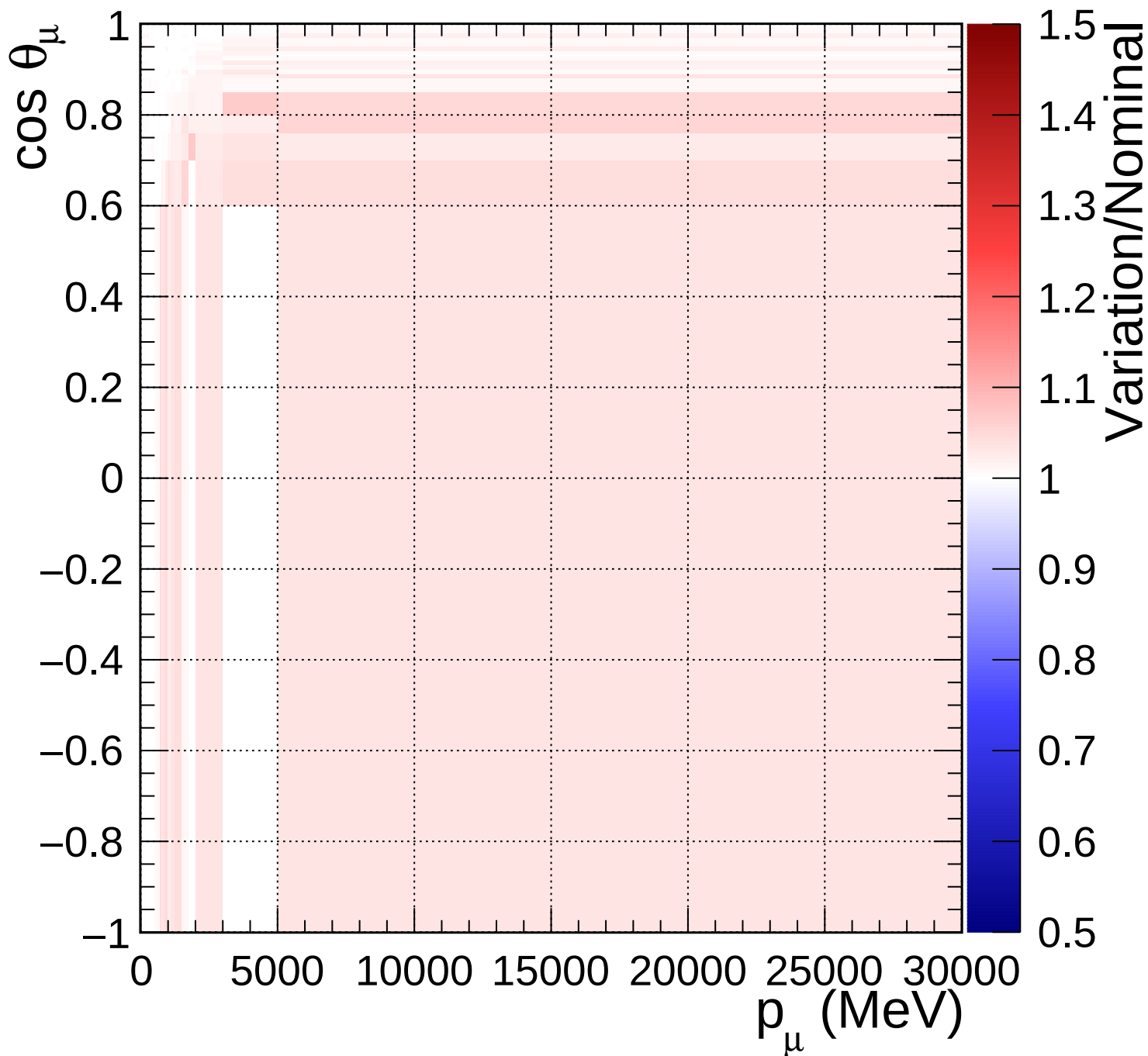
FGD1_numuCC_other_Q2_norm_7_2.2
