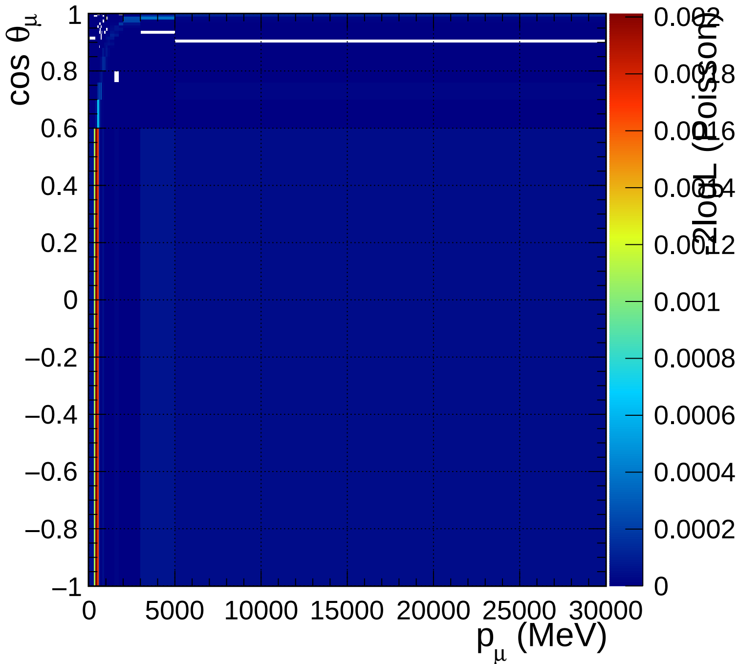
FGD1_numuCC_other_Q2_norm_5_1.11
