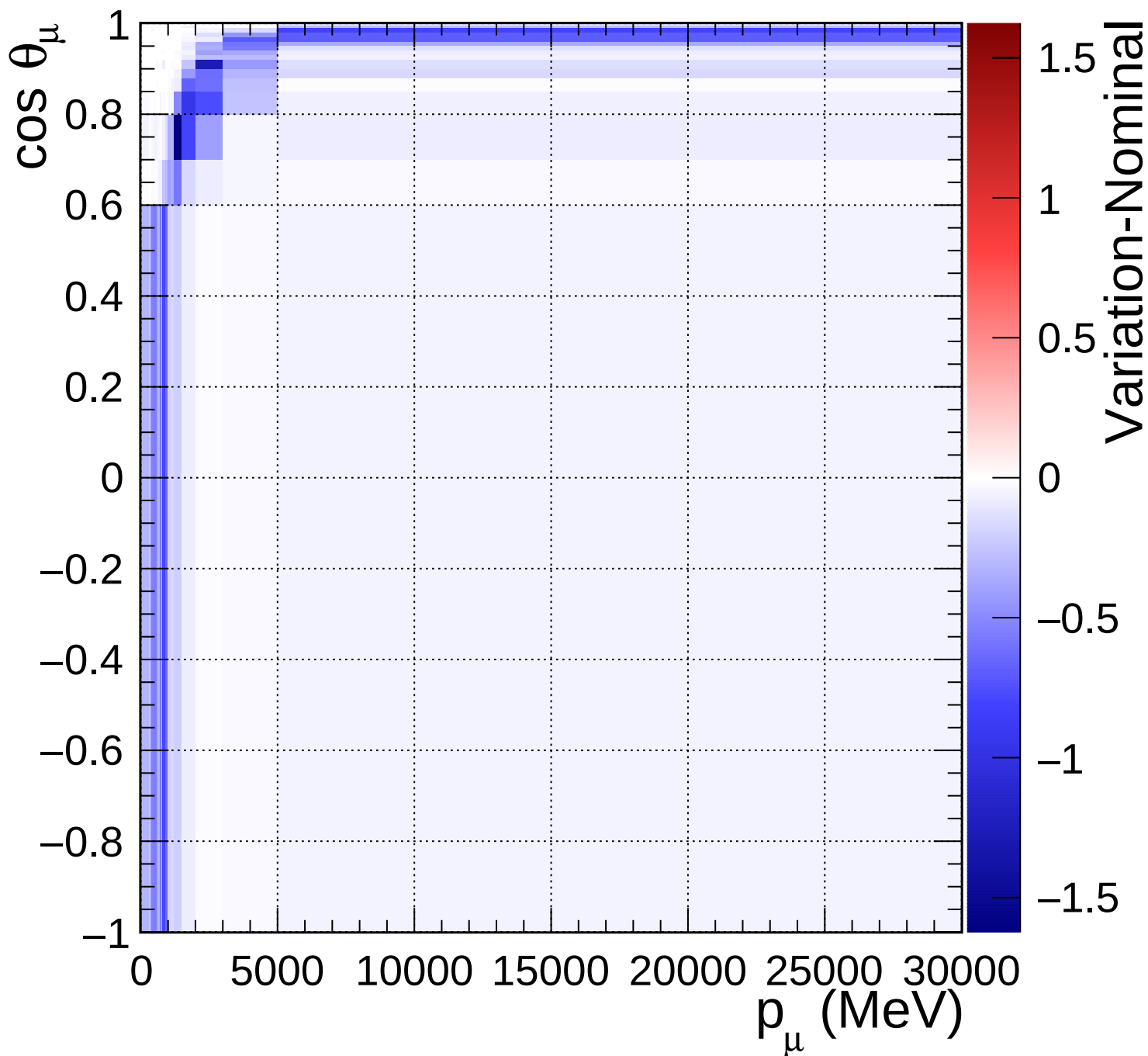
FGD2_numuCC_1pi_Q2_norm_7_0.6
