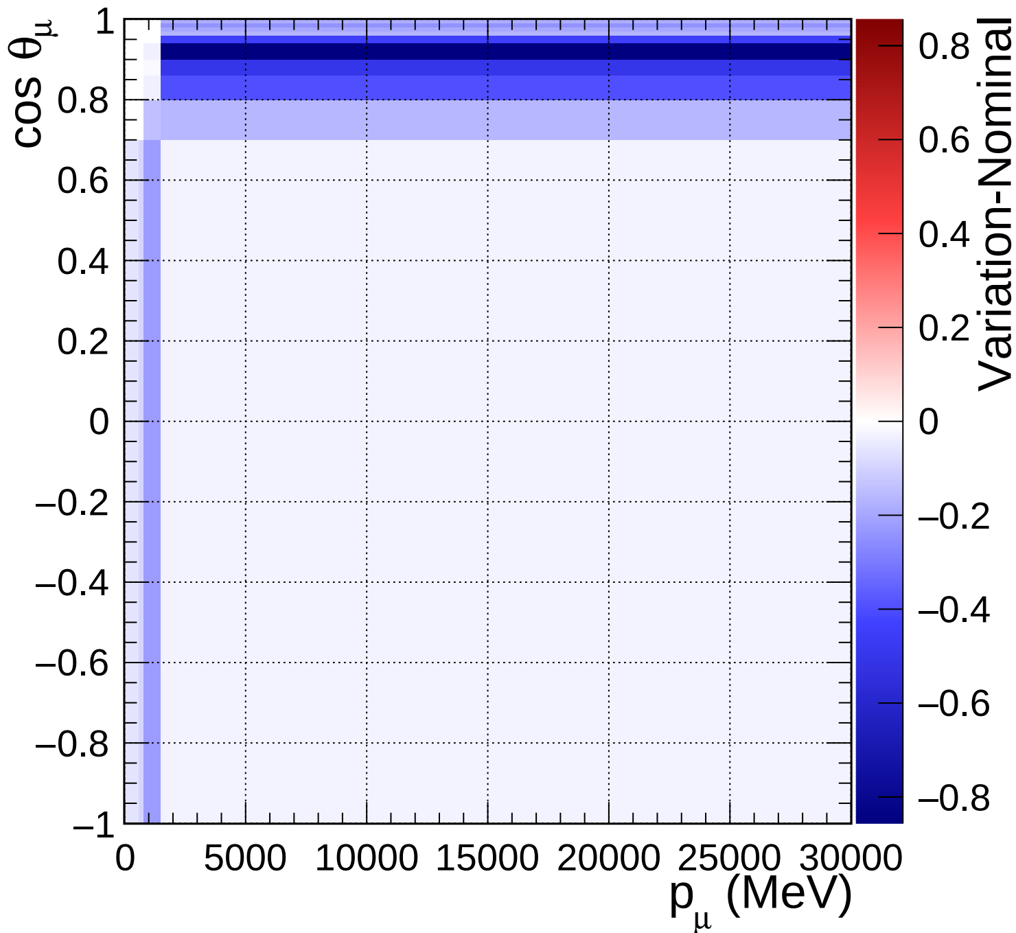
FGD2_NuMuBkg_CC1pi_in_AntiNu_Mode_Q2_norm_7_0.6
