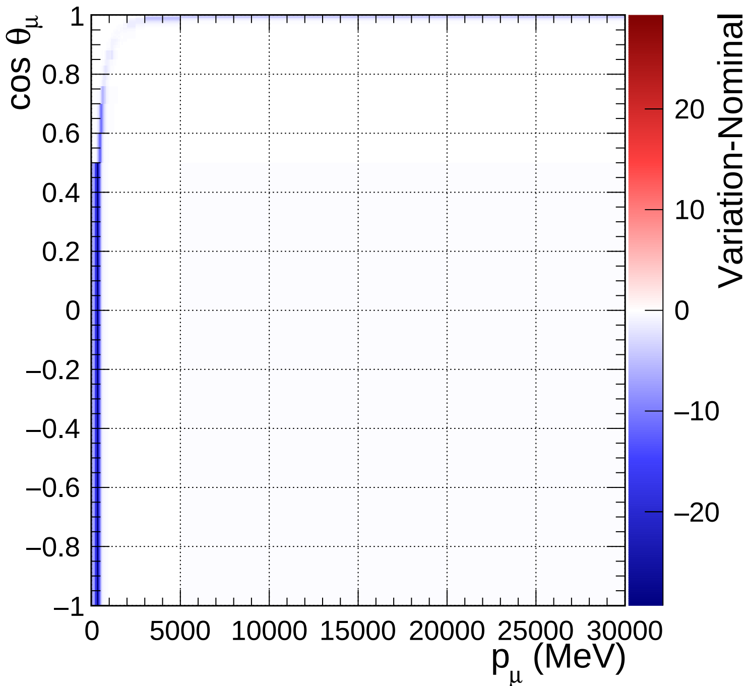
FGD2_numuCC_0pi_Q2_norm_5_0.89
