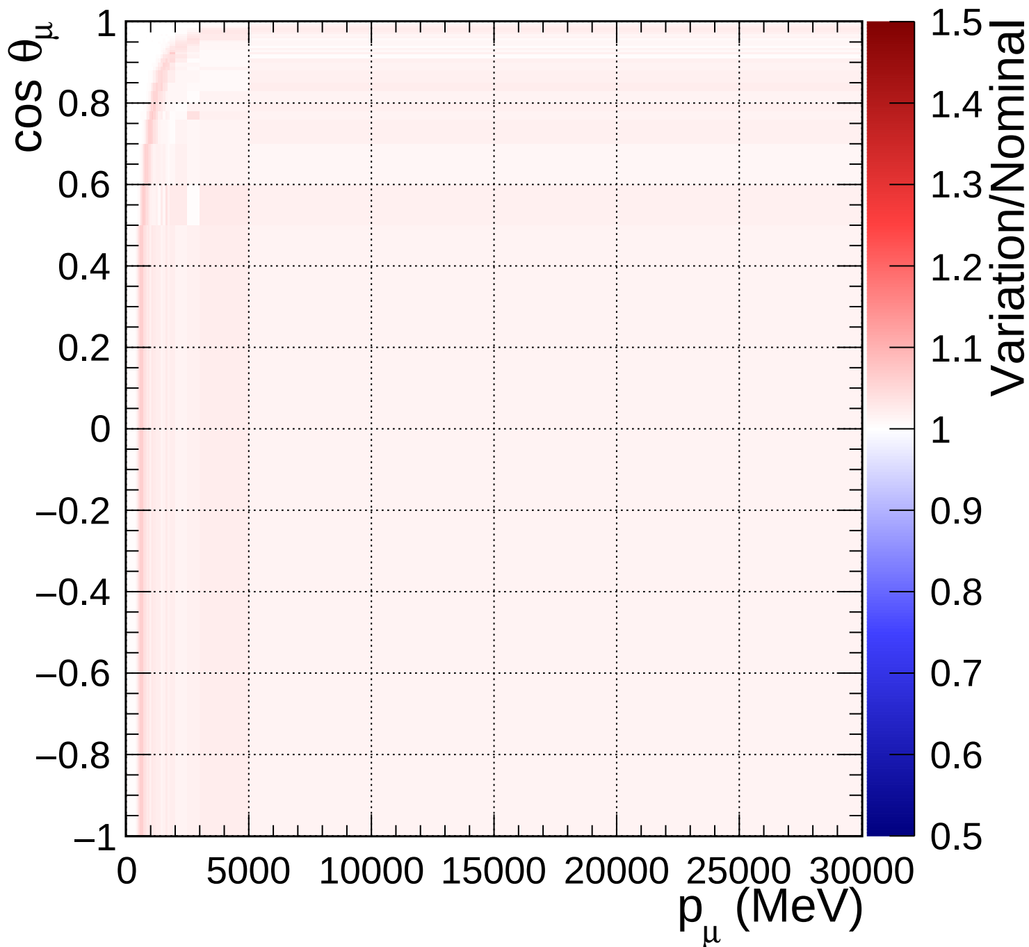
FGD1_numuCC_0pi_Q2_norm_6_1.18
