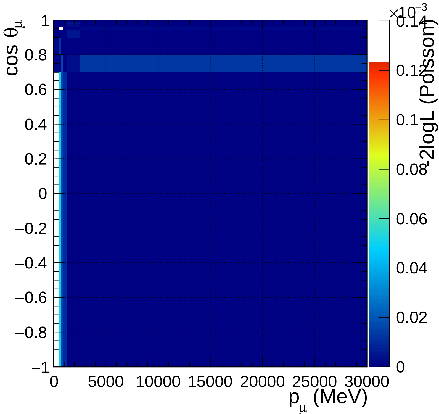
FGD2_anti-numuCC_1pi_Q2_norm_5_0.89
