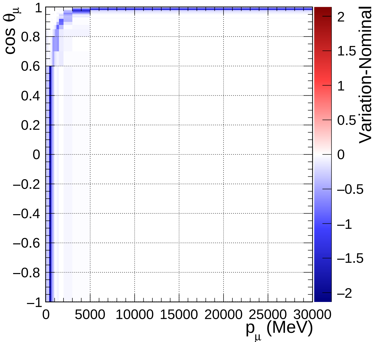
FGD1_numuCC_1pi_Q2_norm_6_0.46
