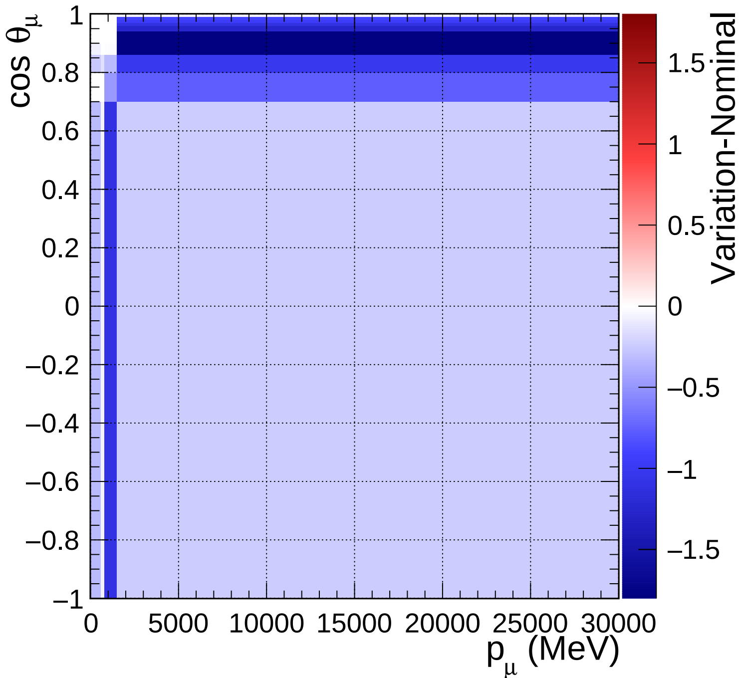
FGD1_NuMuBkg_CC1pi_in_AntiNu_Mode_Q2_norm_7_-0.2
