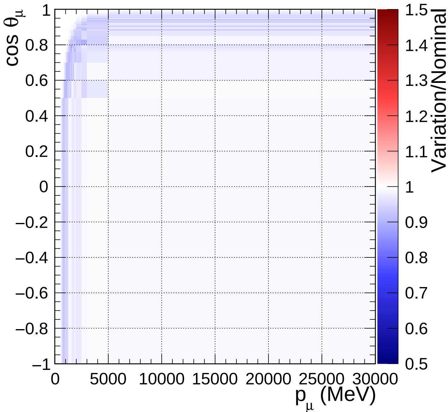
FGD2_numuCC_0pi_Q2_norm_7_0.6
