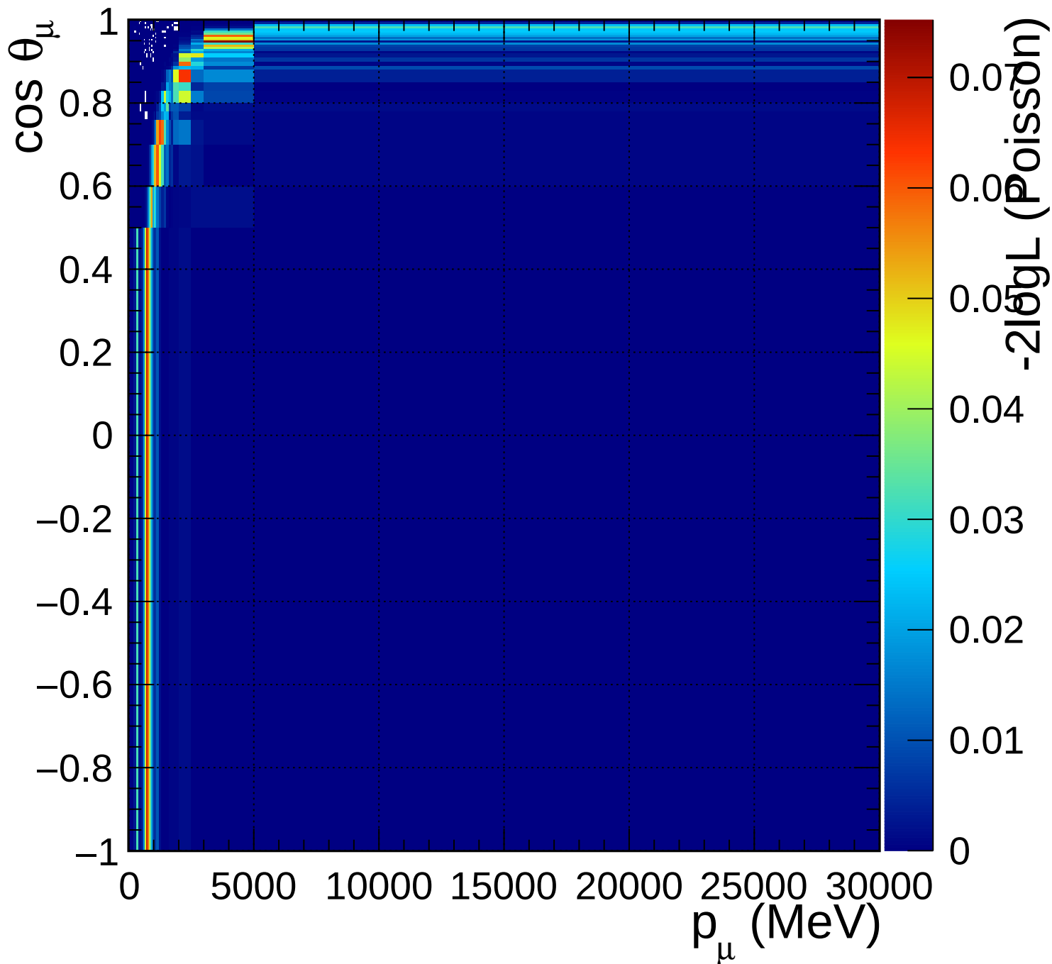
FGD2_numuCC_0pi_Q2_norm_7_1.4
