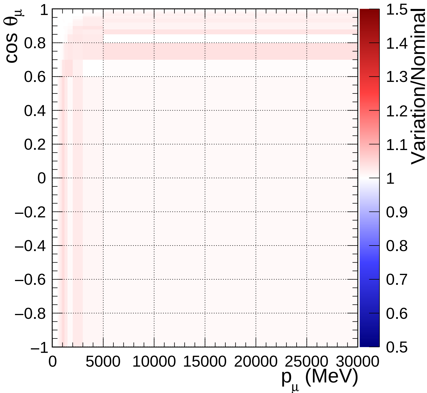
FGD1_numuCC_1pi_Q2_norm_7_1.4
