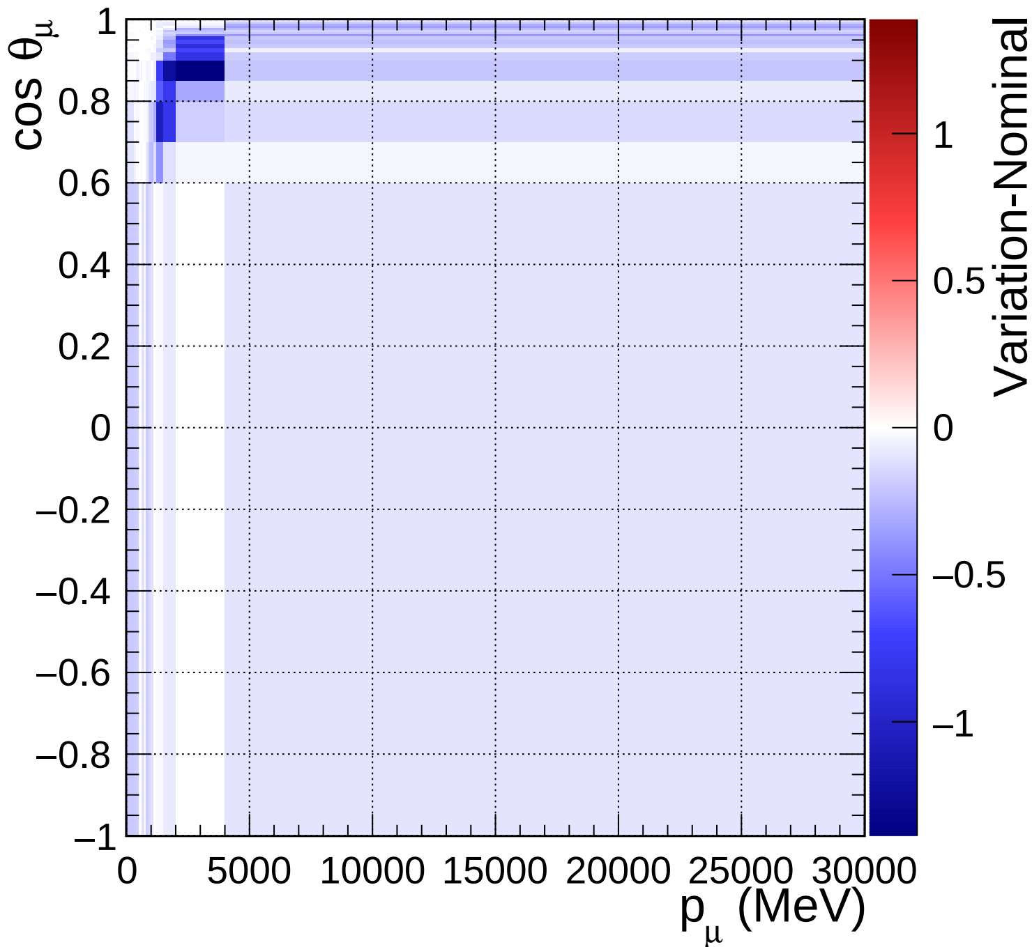
FGD2_anti-numuCC_0pi_Q2_norm_7_0.6
