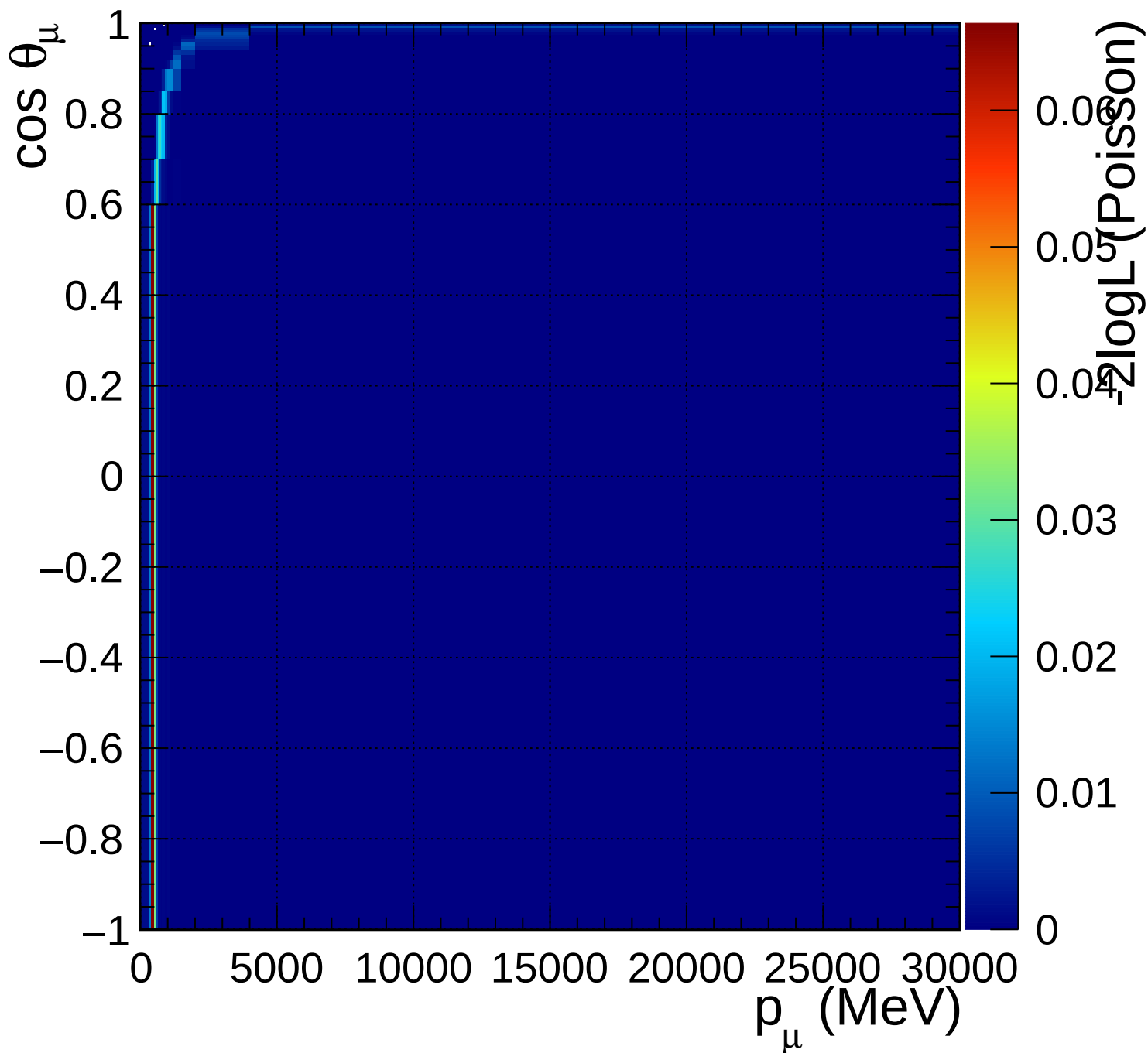
FGD2_anti-numuCC_0pi_Q2_norm_5_0.89
