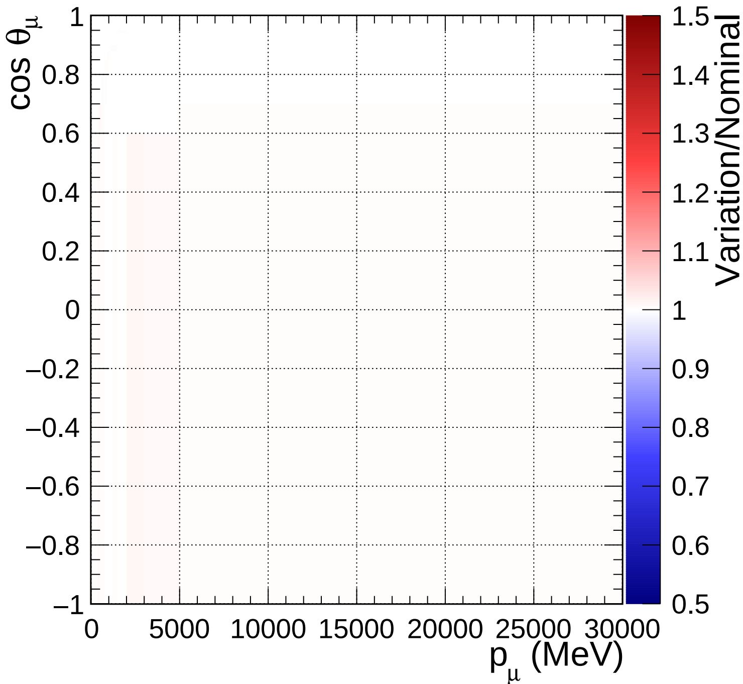
FGD2_numuCC_1pi_Q2_norm_5_1.11
