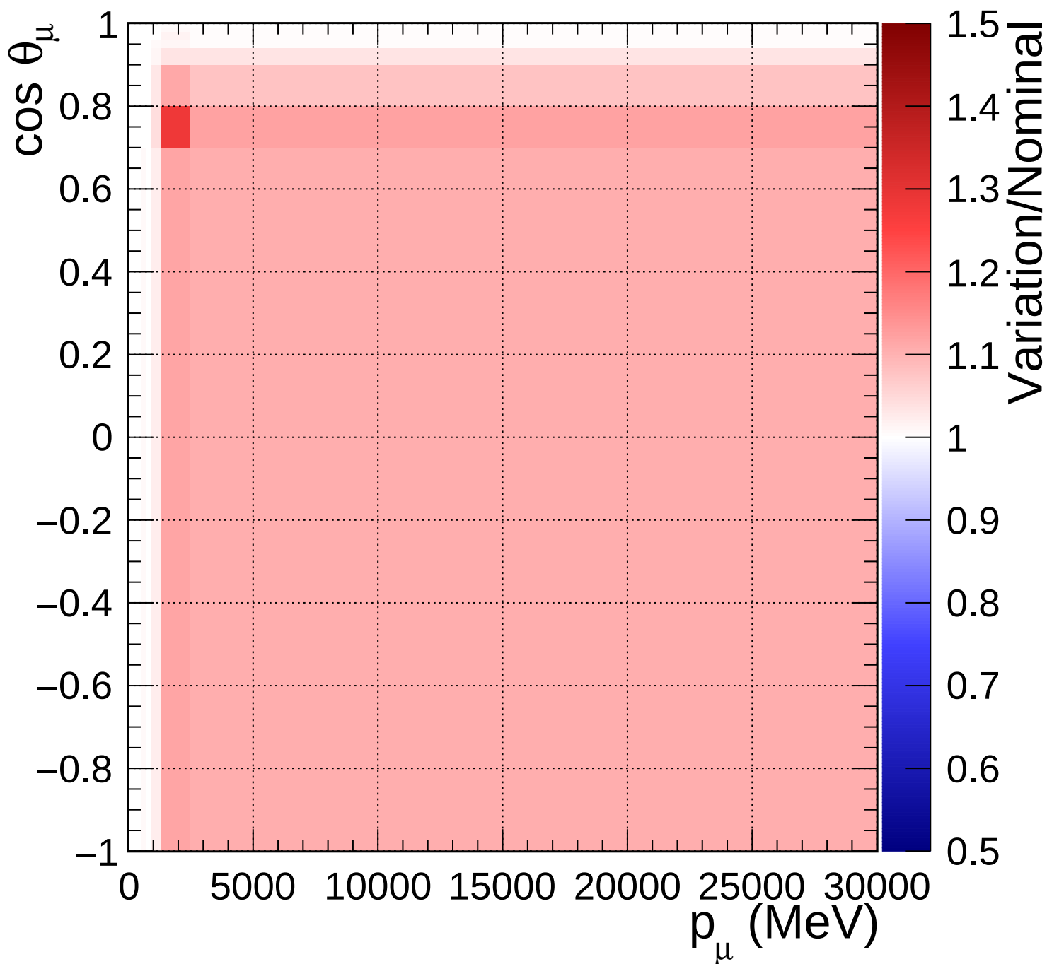
FGD1_anti-numuCC_1pi_Q2_norm_7_2.2
