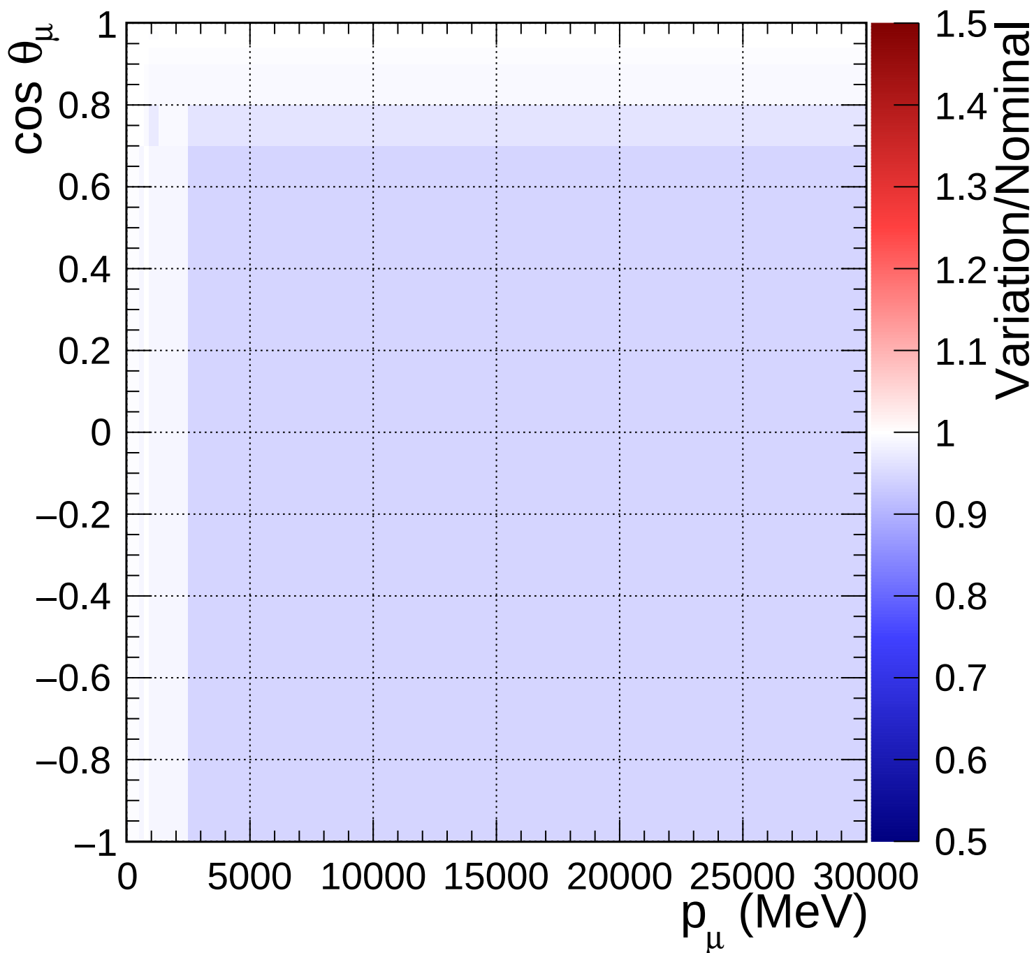
FGD1_anti-numuCC_1pi_Q2_norm_6_0.46
