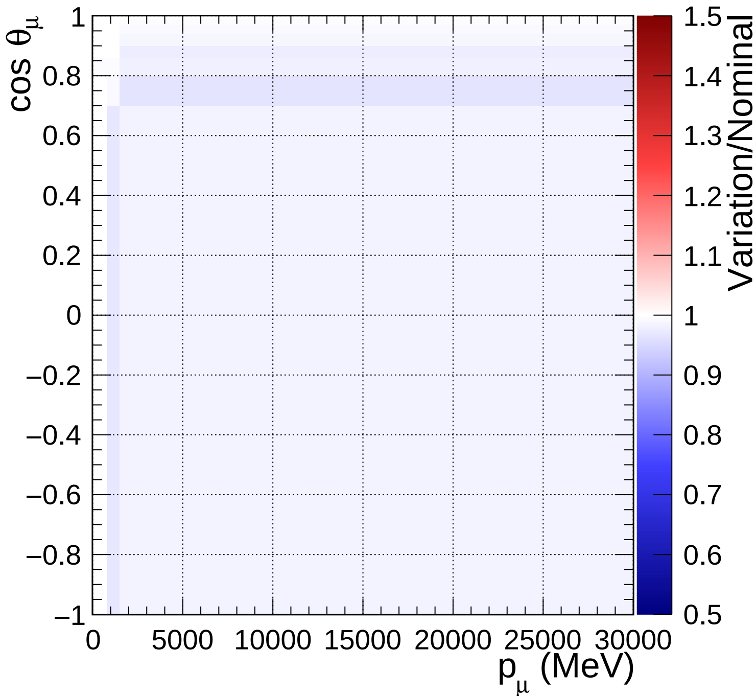
FGD1_NuMuBkg_CC1pi_in_AntiNu_Mode_Q2_norm_7_0.6
