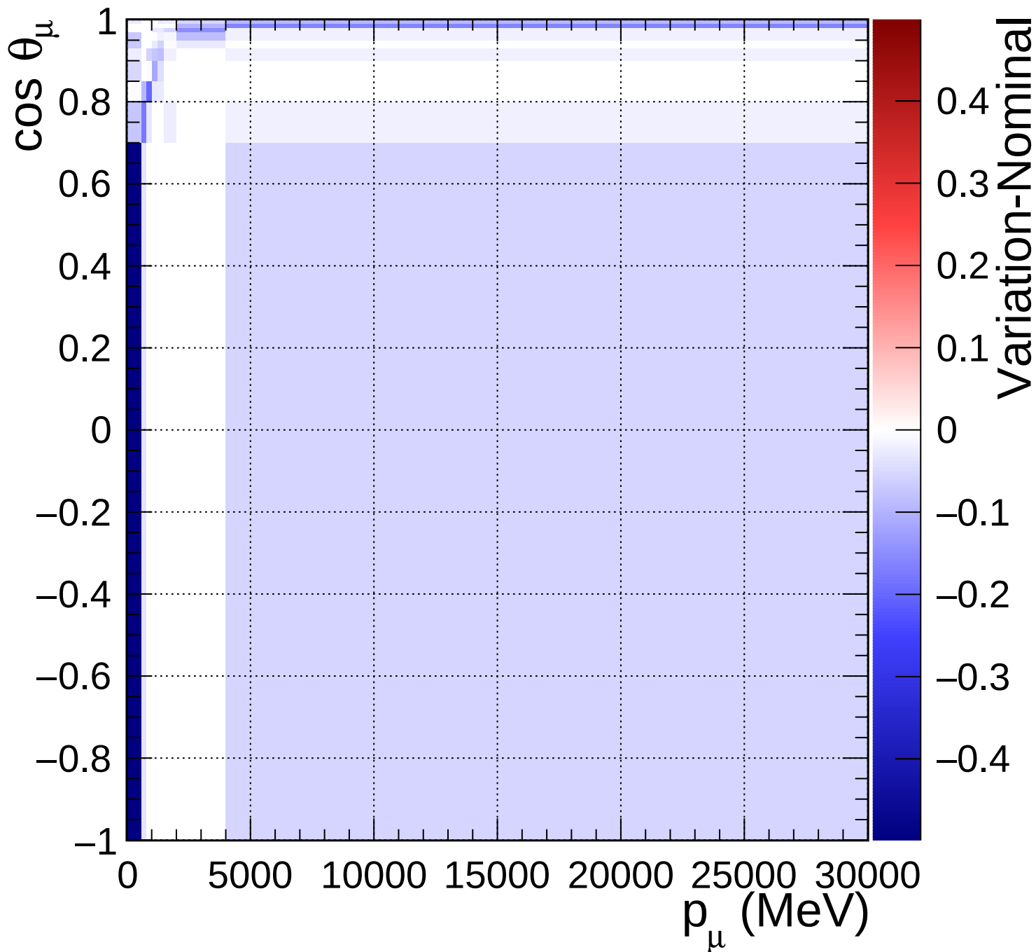
FGD2_anti-numuCC_other_Q2_norm_5_0.67
