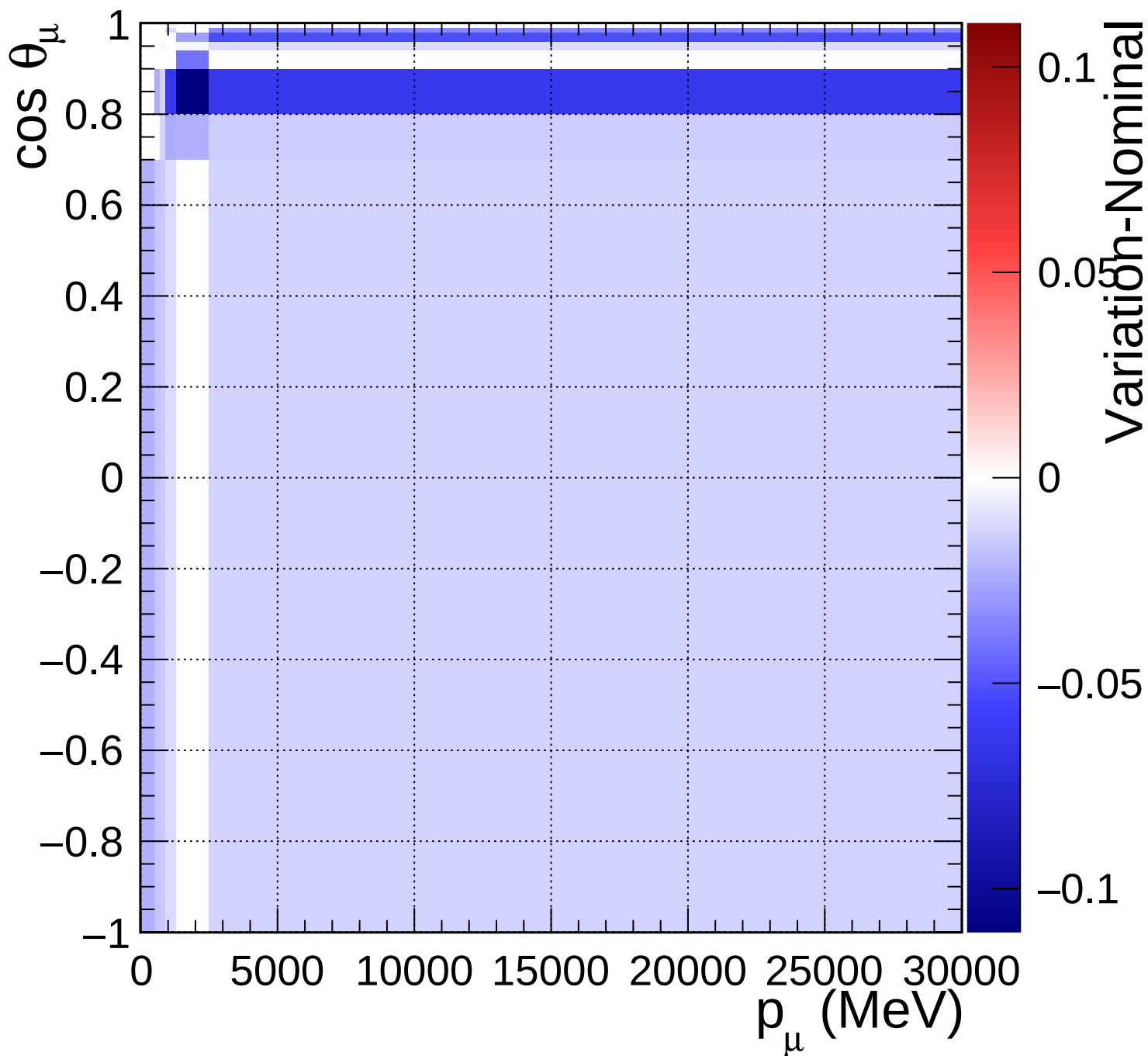
FGD2_anti-numuCC_1pi_Q2_norm_6_0.82
