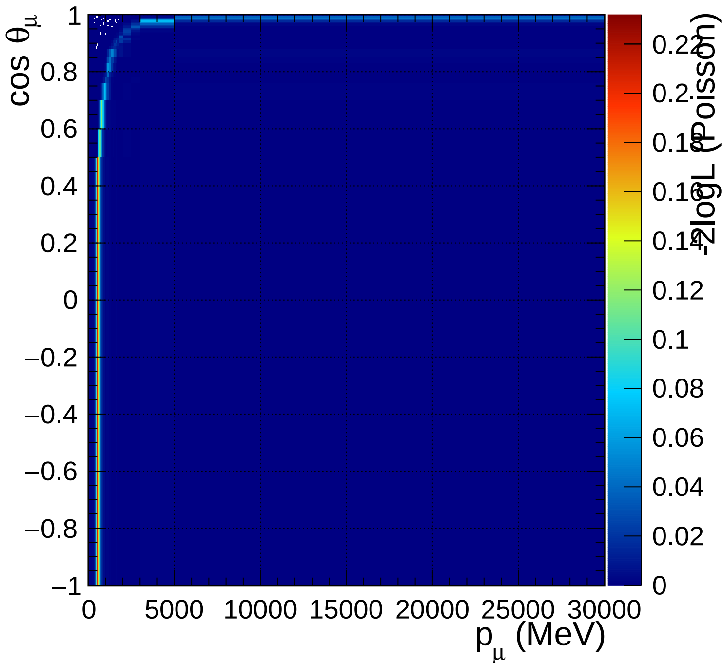
FGD1_numuCC_0pi_Q2_norm_6_0.82
