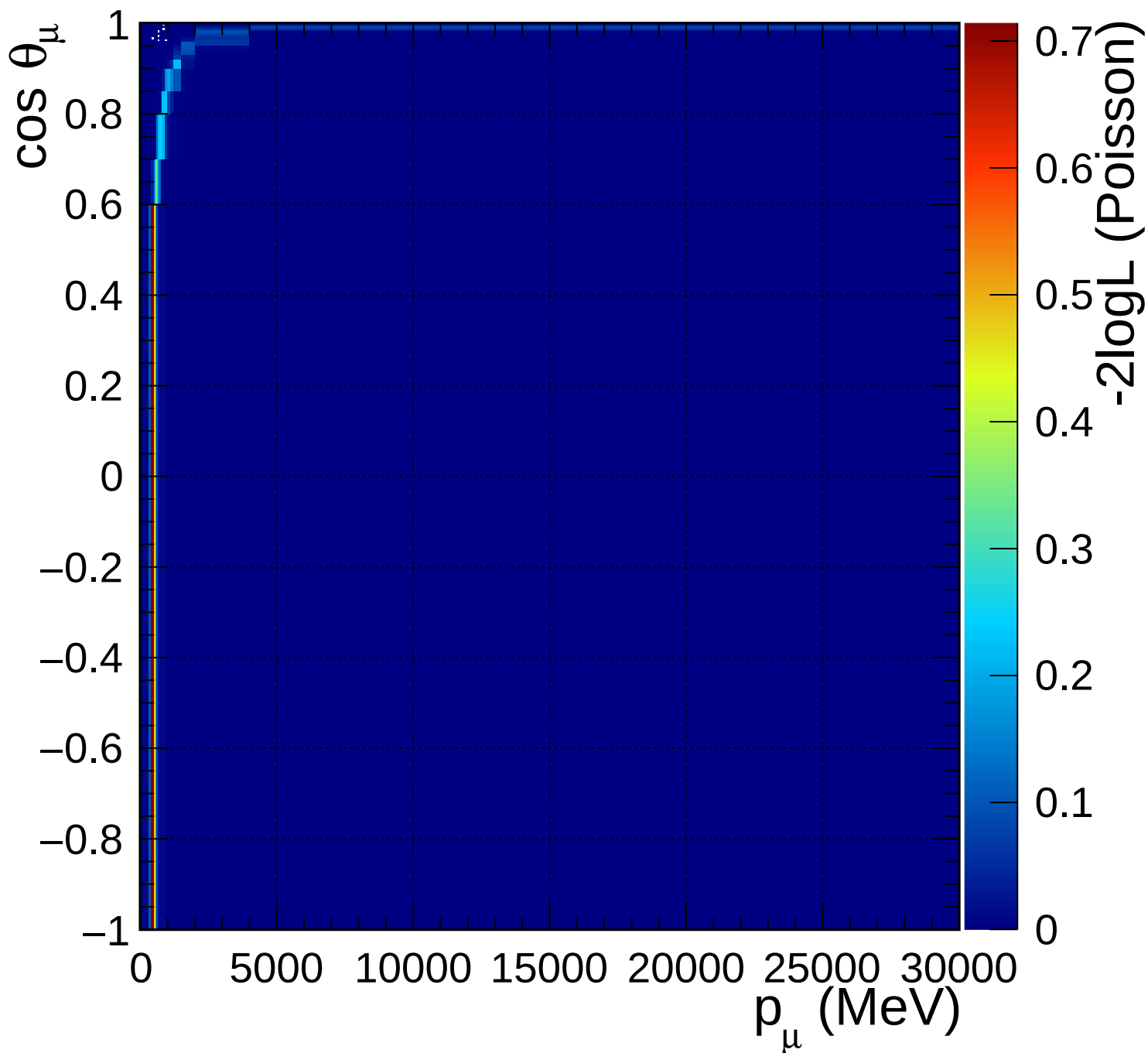
FGD1_anti-numuCC_0pi_Q2_norm_5_0.67
