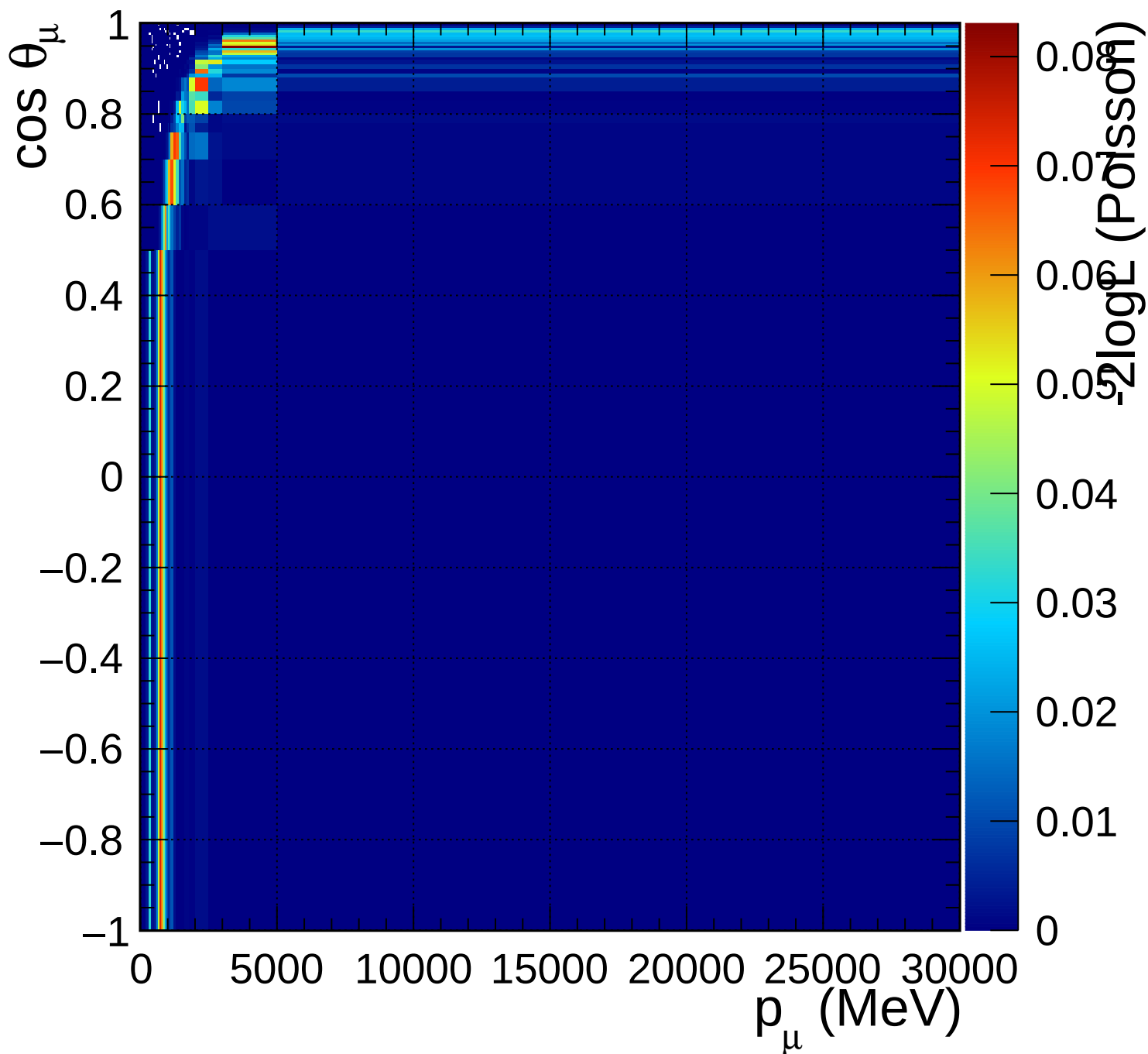
FGD2_numuCC_0pi_Q2_norm_7_0.6
