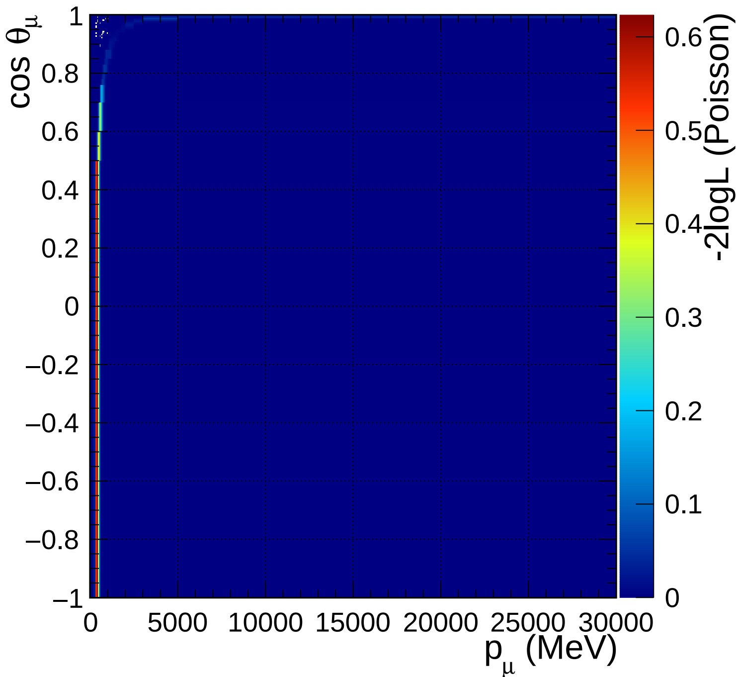
FGD1_numuCC_0pi_Q2_norm_5_0.89
