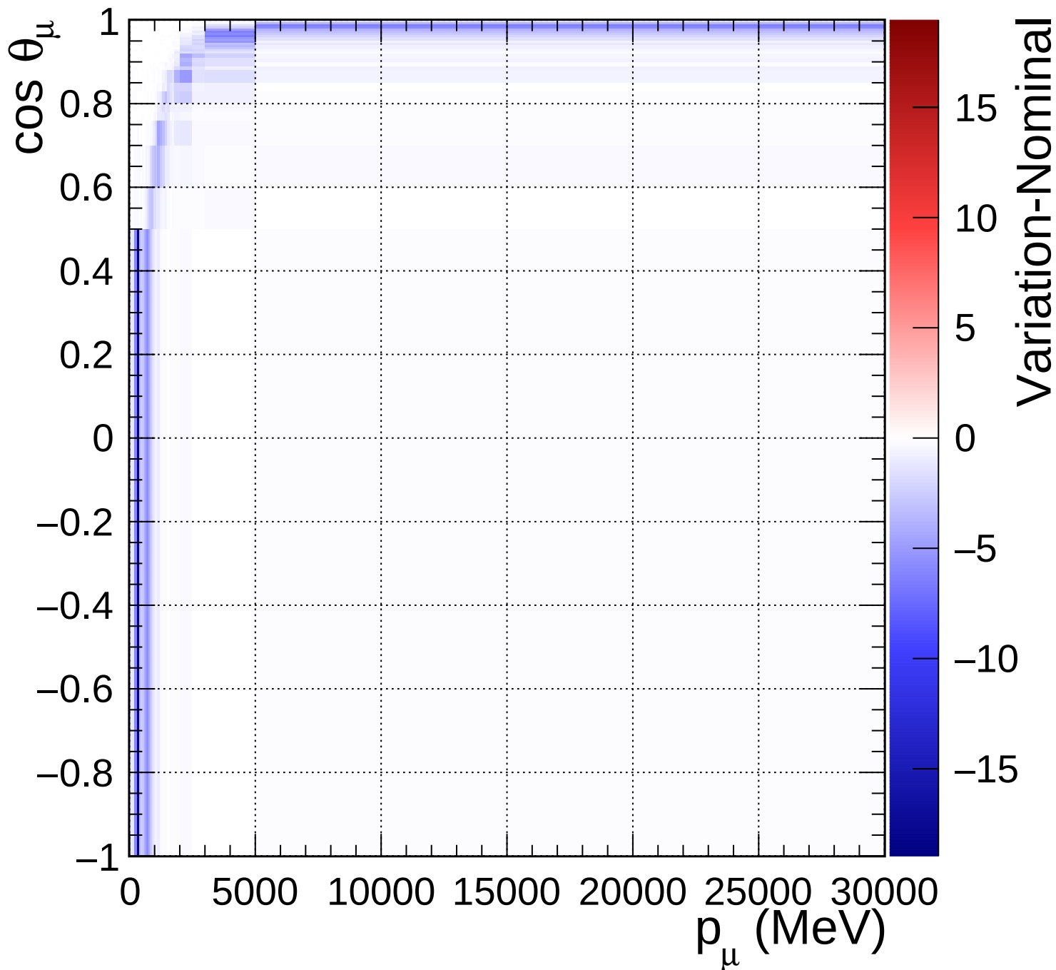
FGD2_numuCC_0pi_Q2_norm_7_-0.2
