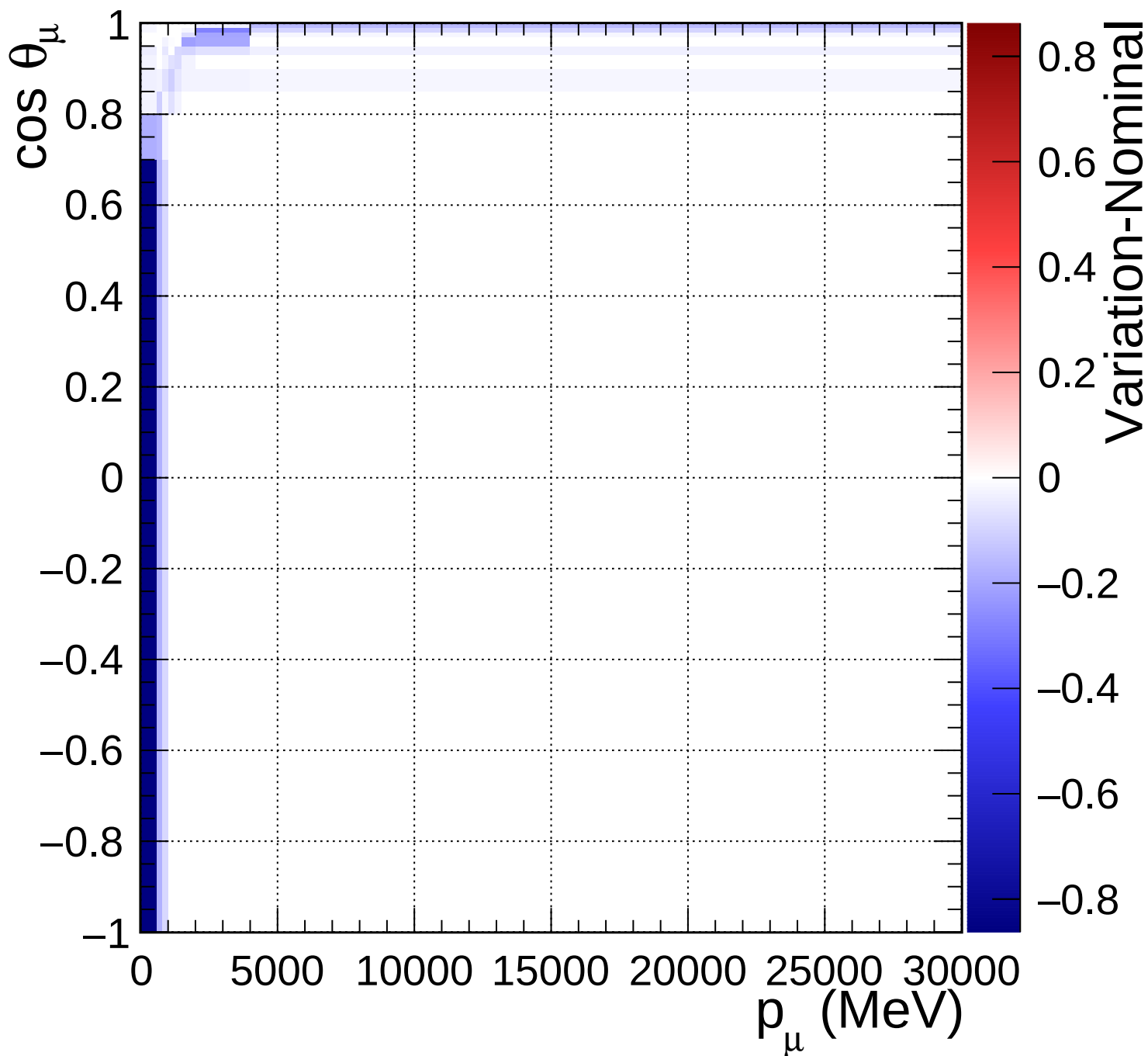
FGD1_anti-numuCC_other_Q2_norm_5_0.67
