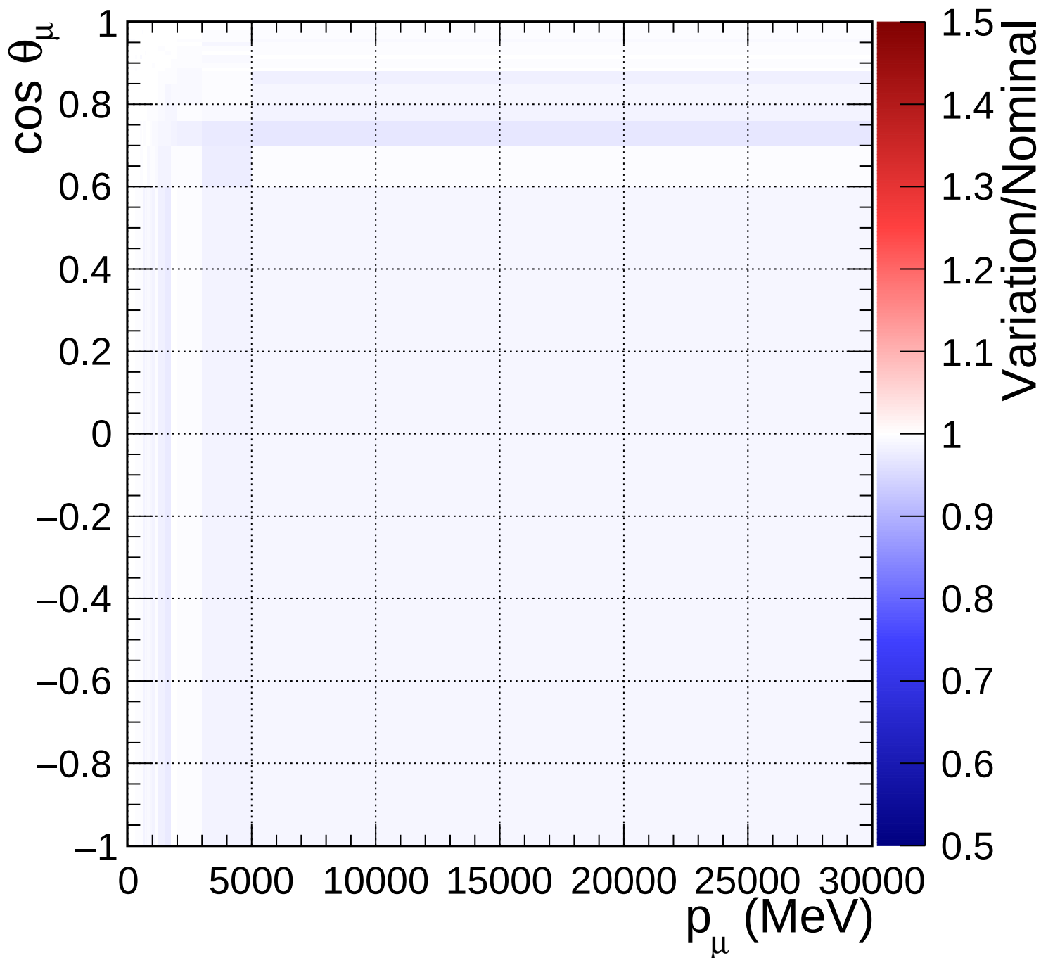
FGD2_numuCC_other_Q2_norm_7_0.6
