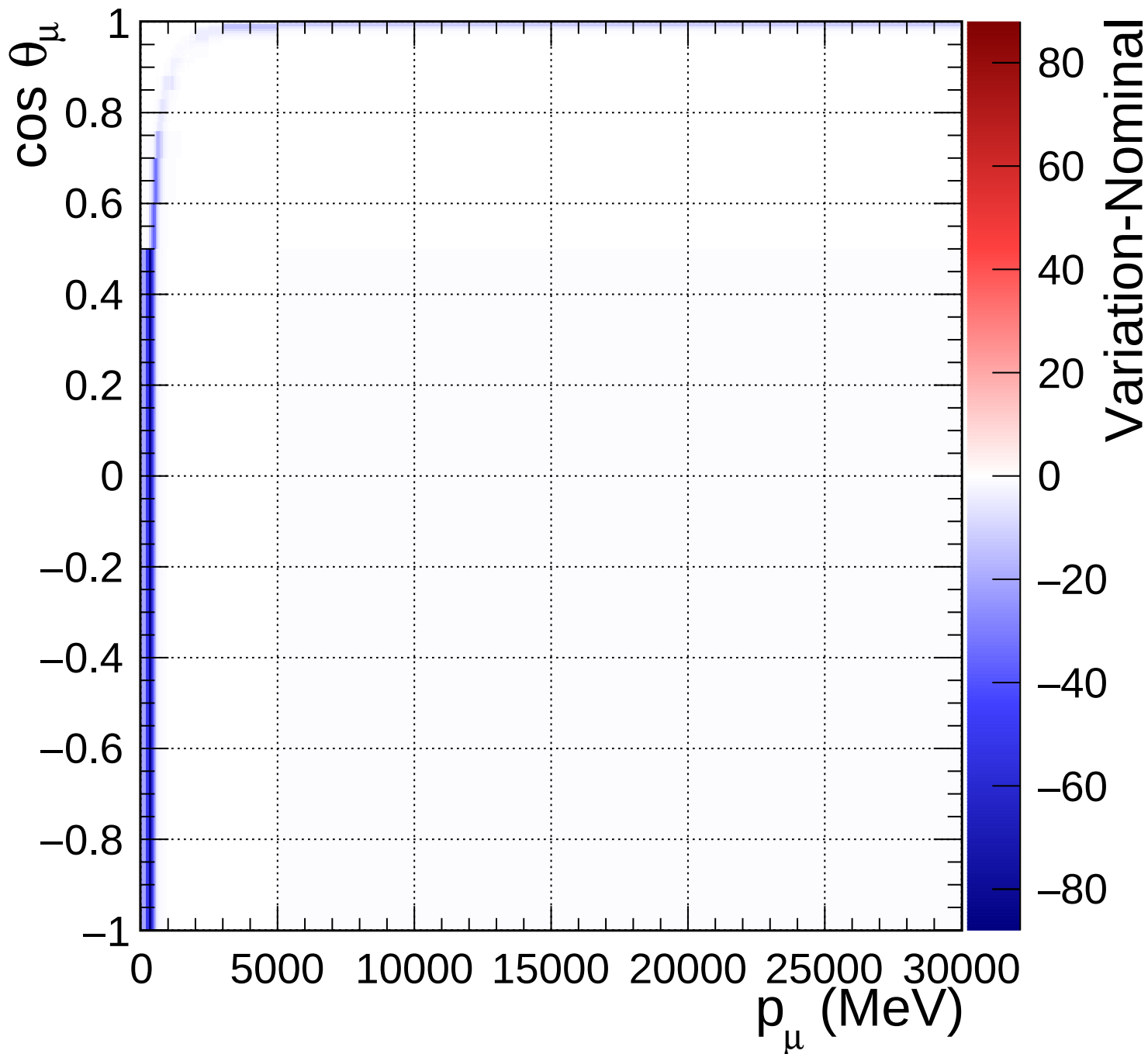
FGD2_numuCC_0pi_Q2_norm_5_0.67
