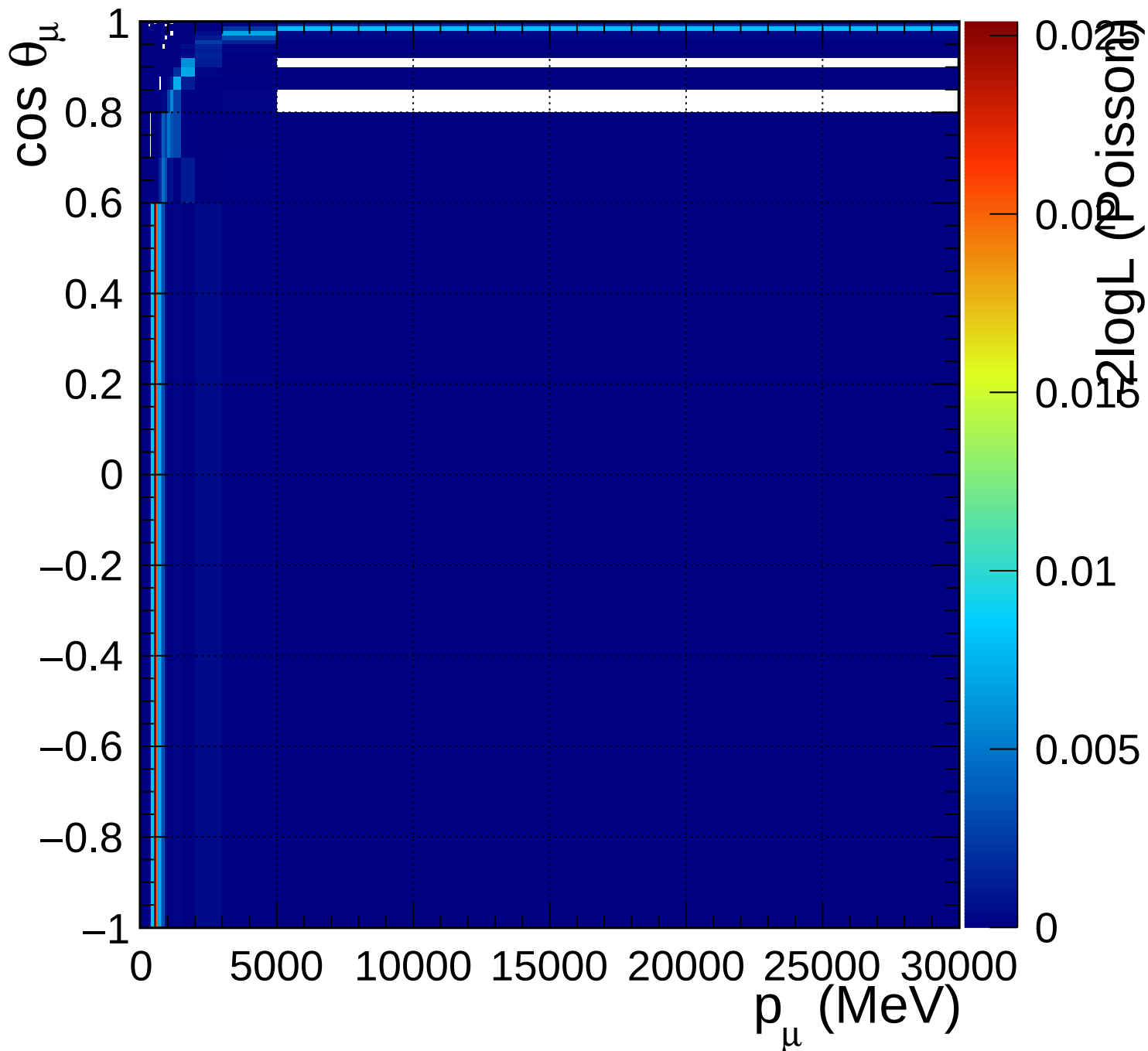
FGD1_numuCC_1pi_Q2_norm_6_0.46
