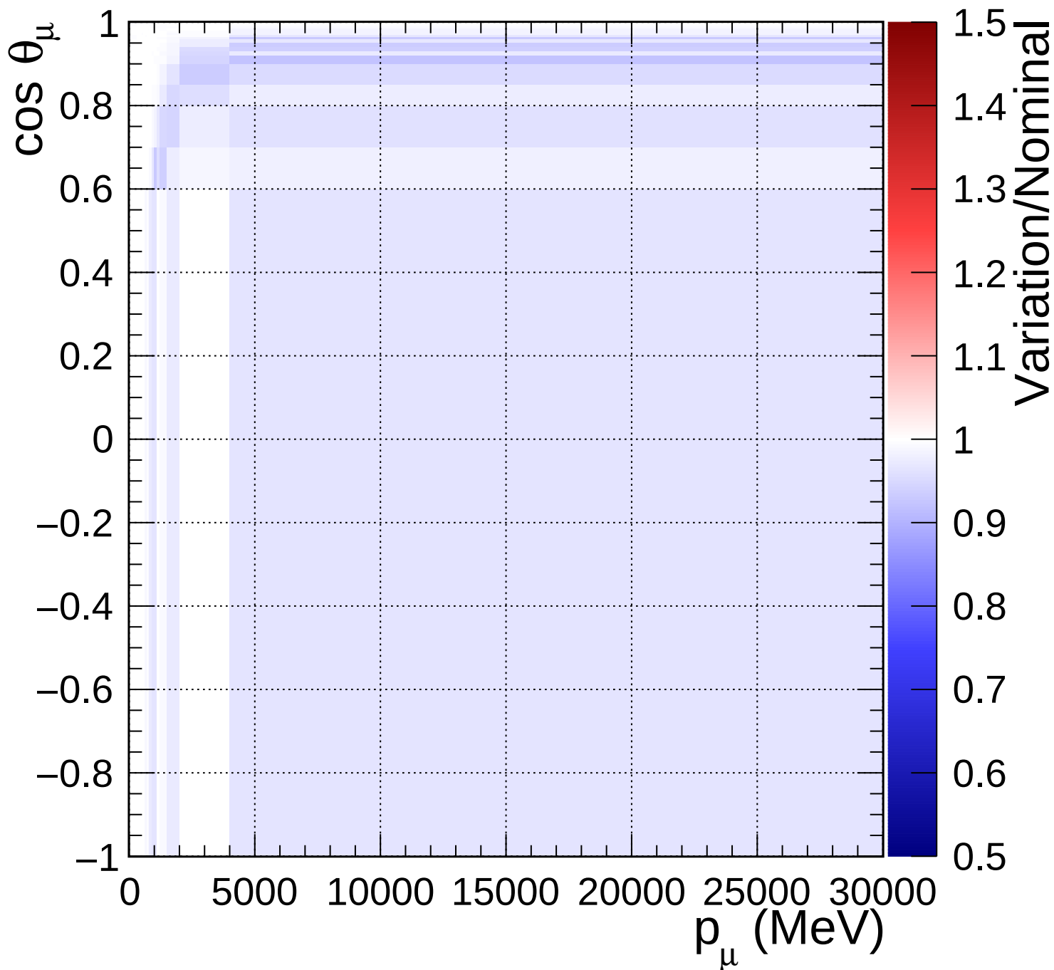
FGD2_anti-numuCC_0pi_Q2_norm_7_0.6
