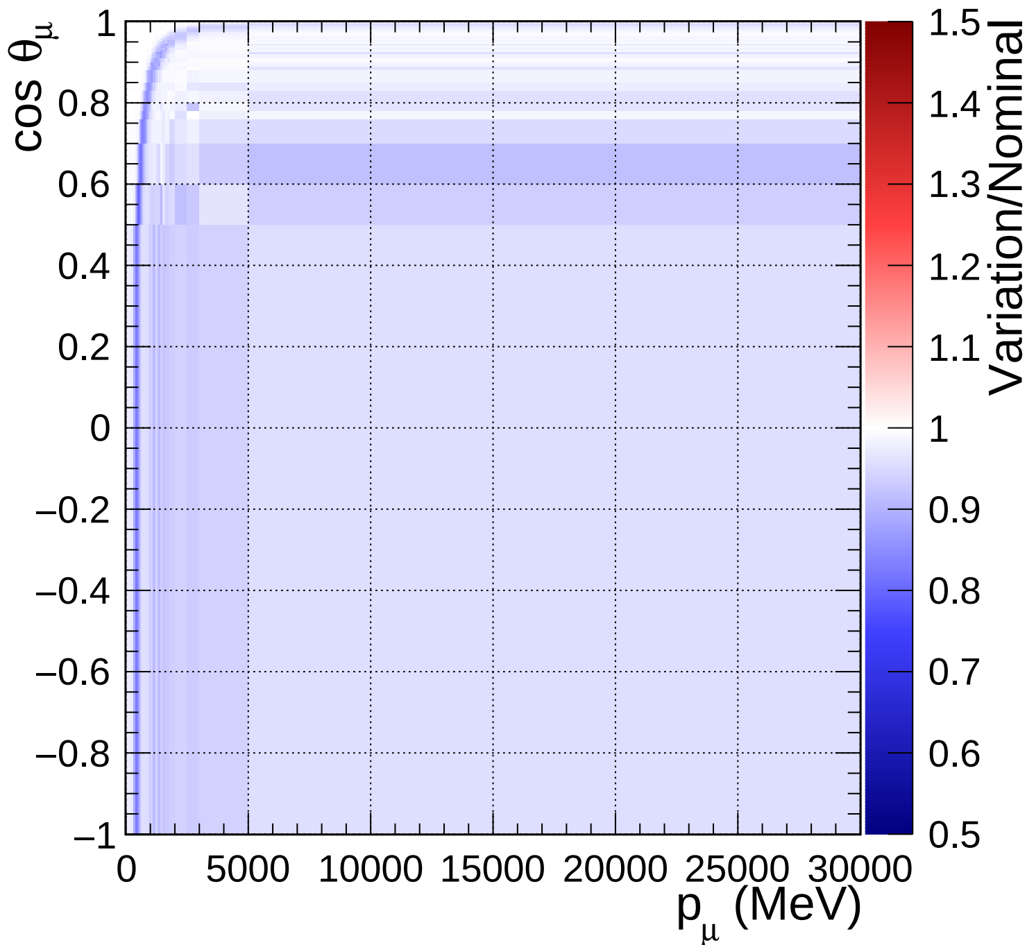
FGD1_numuCC_0pi_Q2_norm_5_0.67
