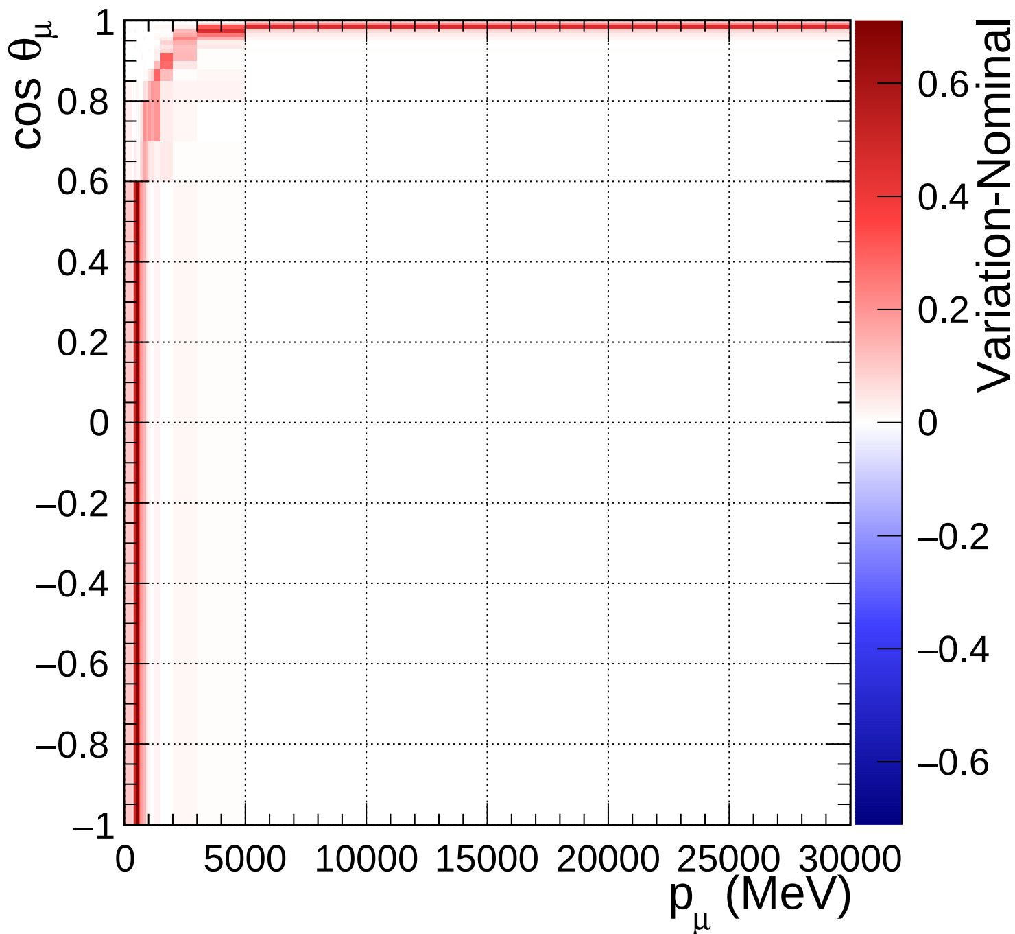
FGD1_numuCC_1pi_Q2_norm_6_1.18
