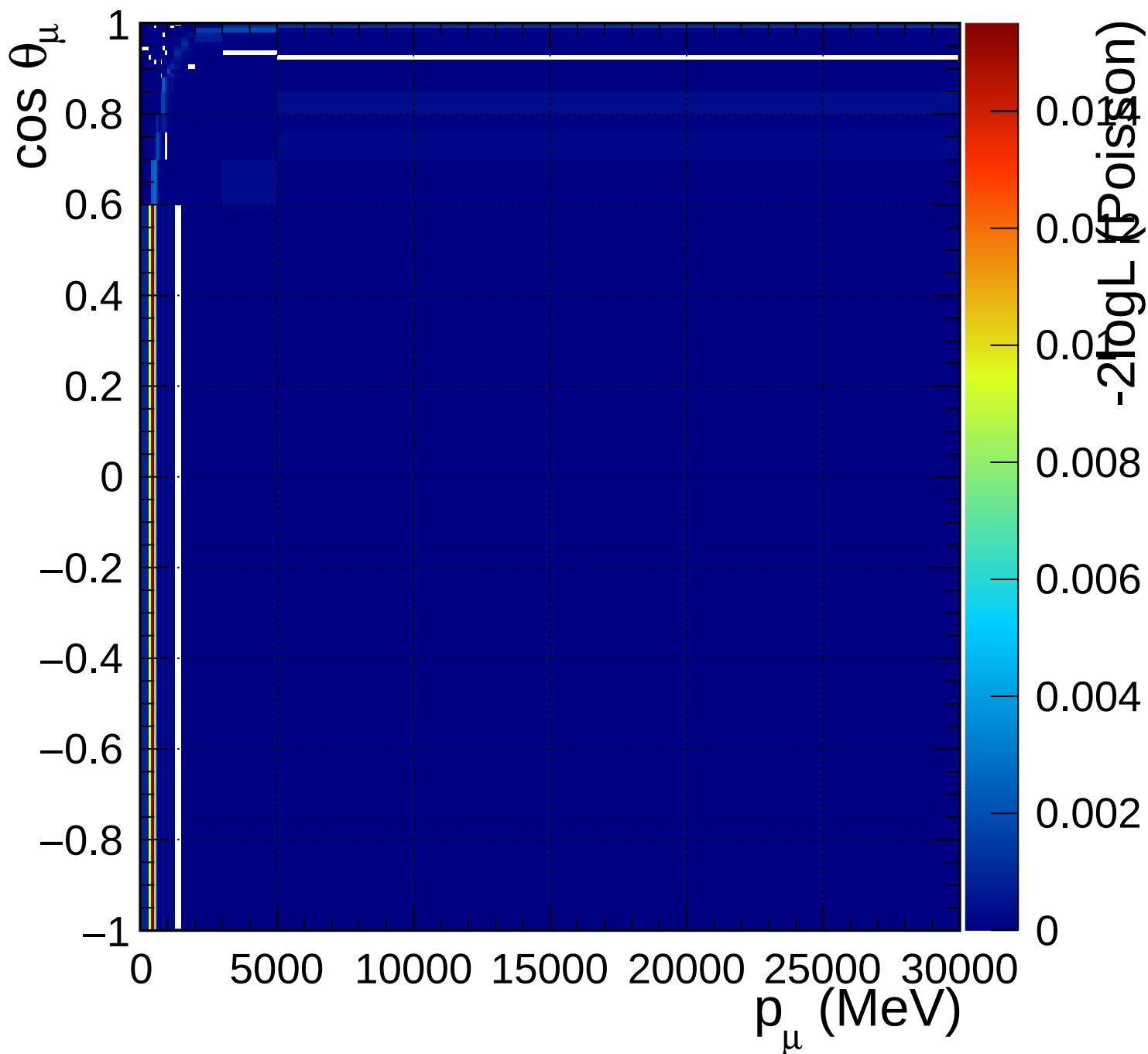
FGD2_numuCC_other_Q2_norm_5_0.67
