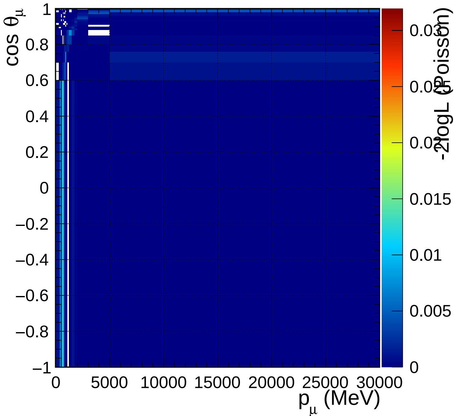
FGD1_numuCC_other_Q2_norm_6_0.46
