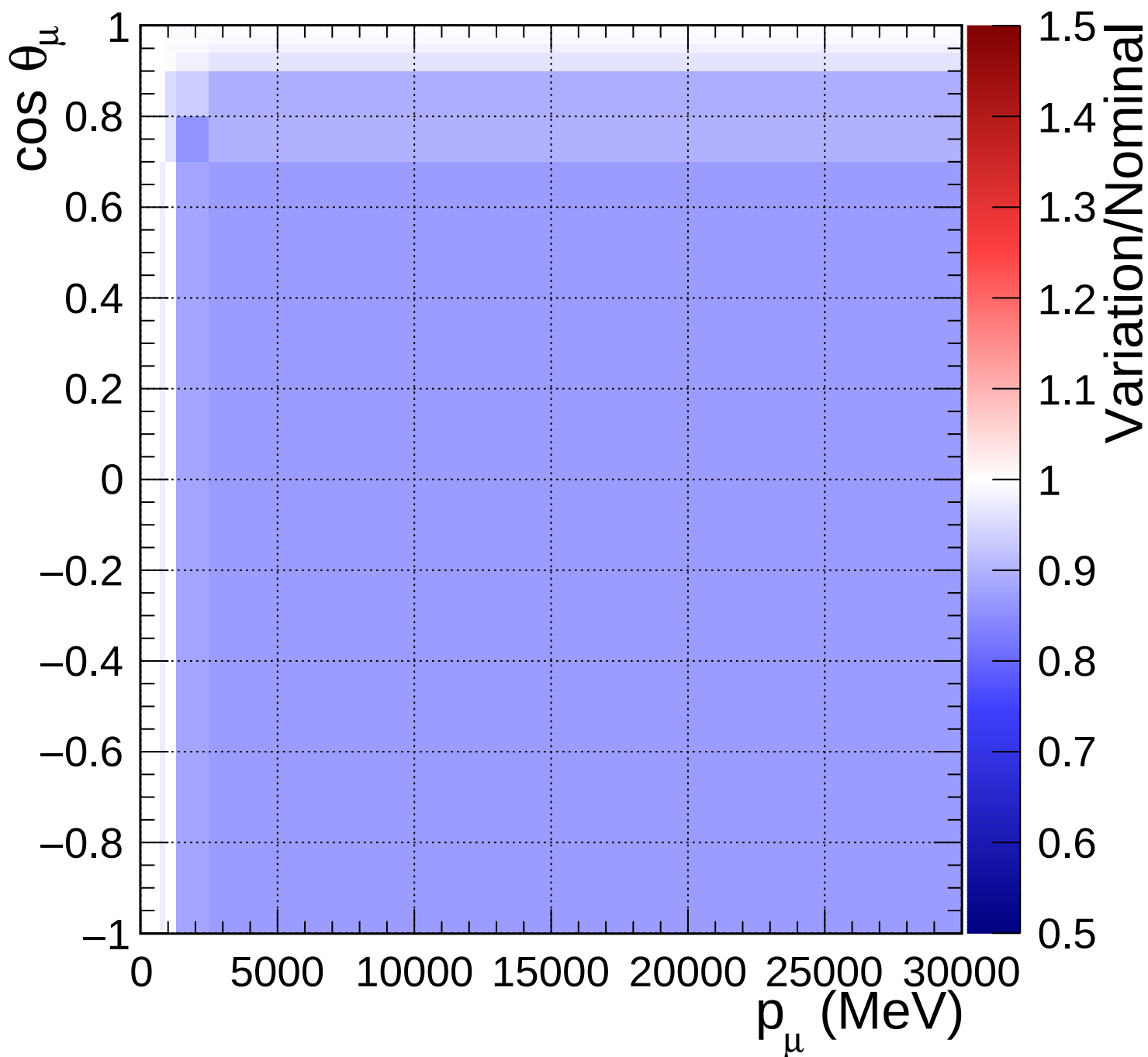
FGD2_anti-numuCC_1pi_Q2_norm_7_-0.2
