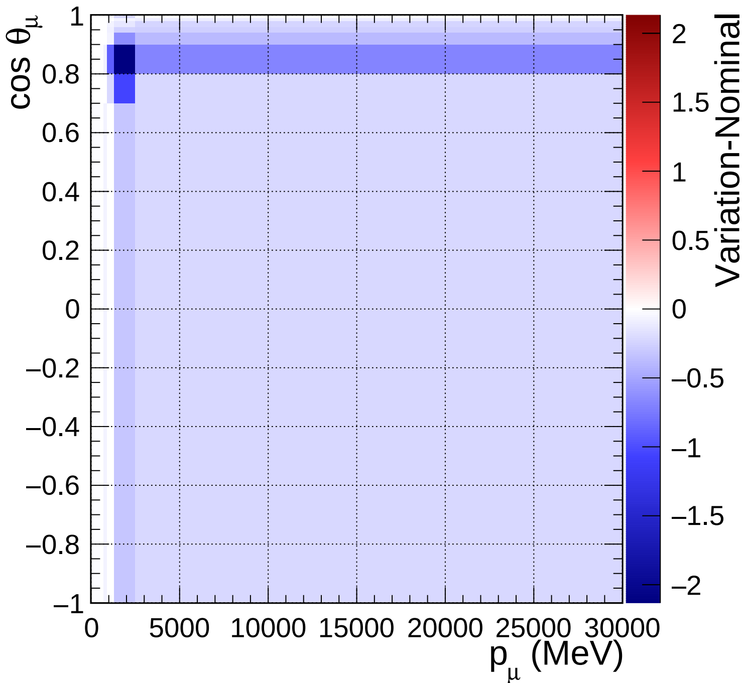
FGD2_anti-numuCC_1pi_Q2_norm_7_-0.2
