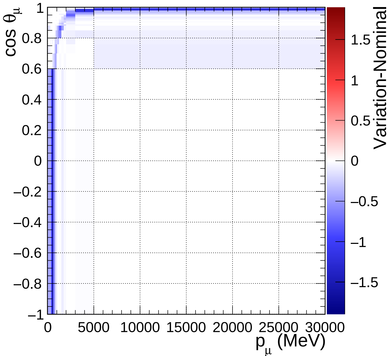
FGD1_numuCC_other_Q2_norm_6_0.46
