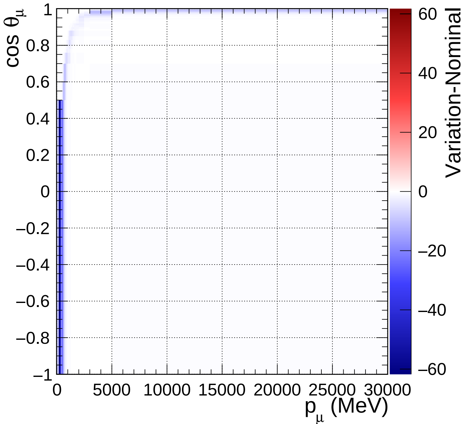
FGD2_numuCC_0pi_Q2_norm_6_0.46
