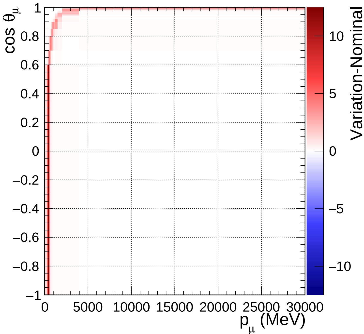
FGD1_anti-numuCC_0pi_Q2_norm_5_1.33
