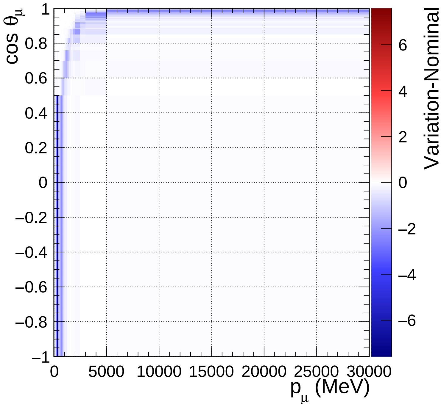
FGD2_numuCC_0pi_Q2_norm_7_0.6
