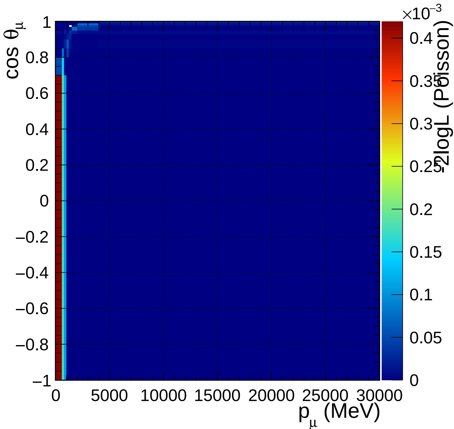
FGD1_anti-numuCC_other_Q2_norm_5_0.89
