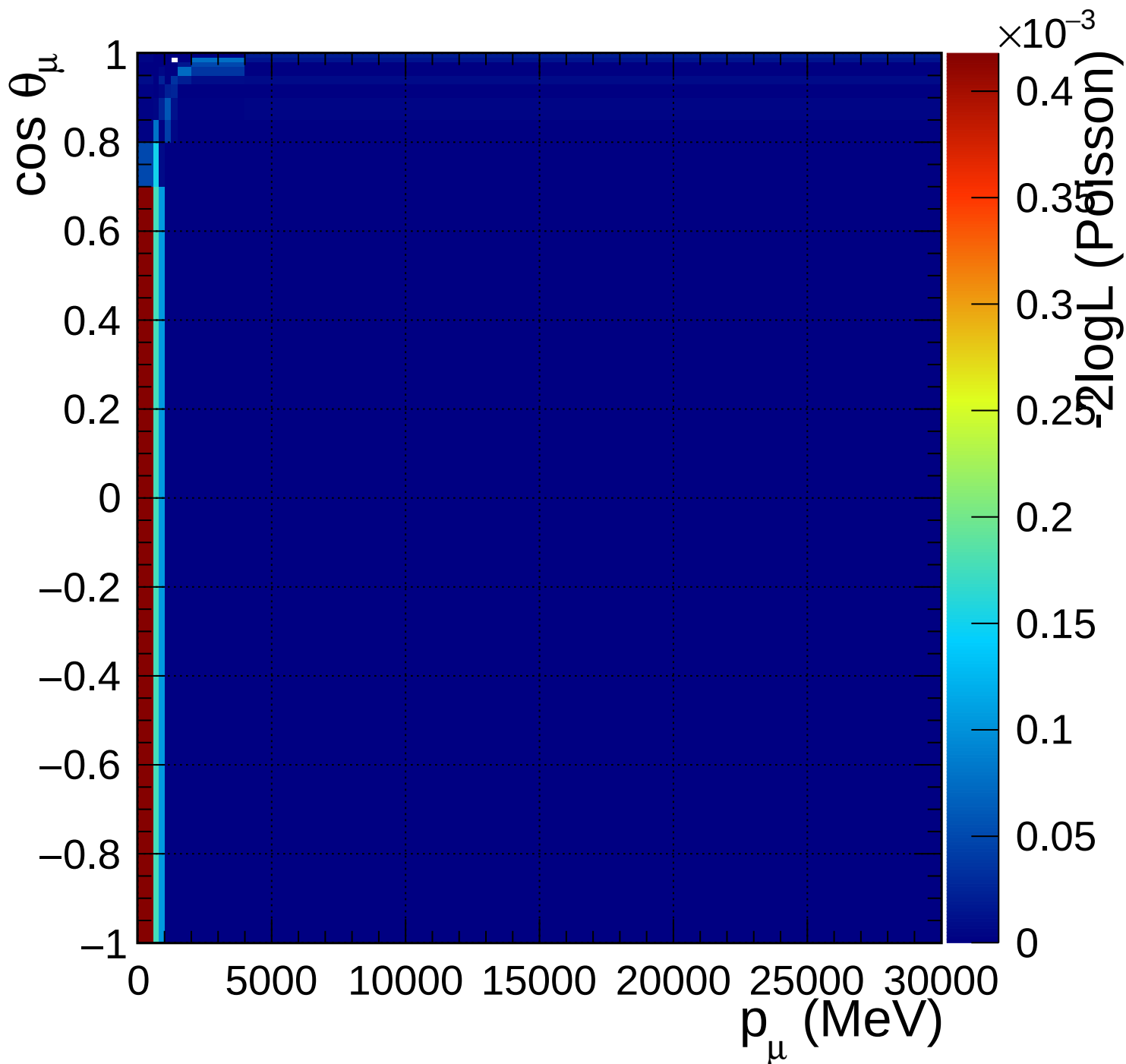
FGD1_anti-numuCC_other_Q2_norm_5_1.11
