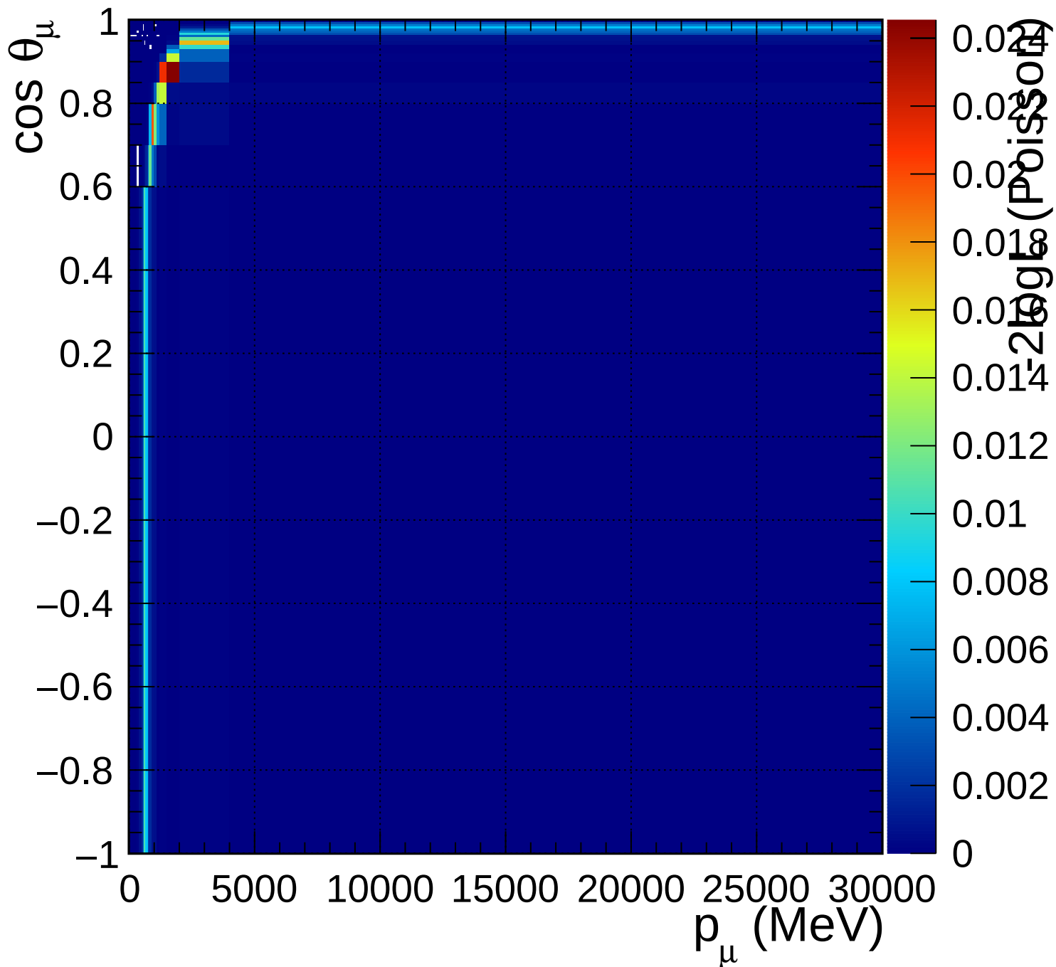
FGD1_anti-numuCC_0pi_Q2_norm_6_0.82
