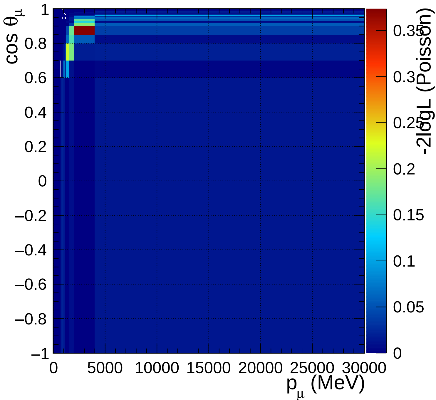
FGD2_anti-numuCC_0pi_Q2_norm_7_2.2
