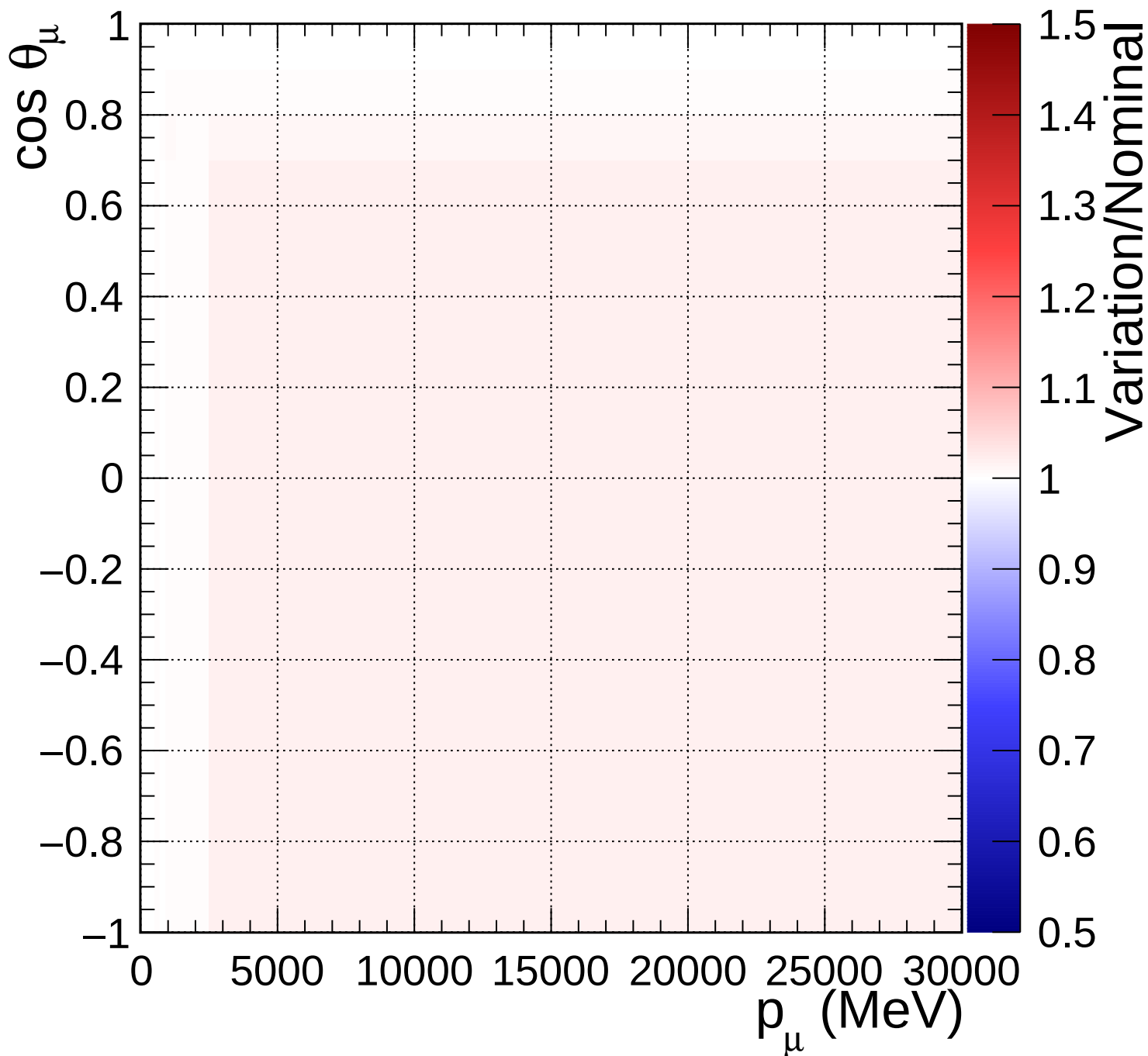
FGD1_anti-numuCC_1pi_Q2_norm_6_1.18
