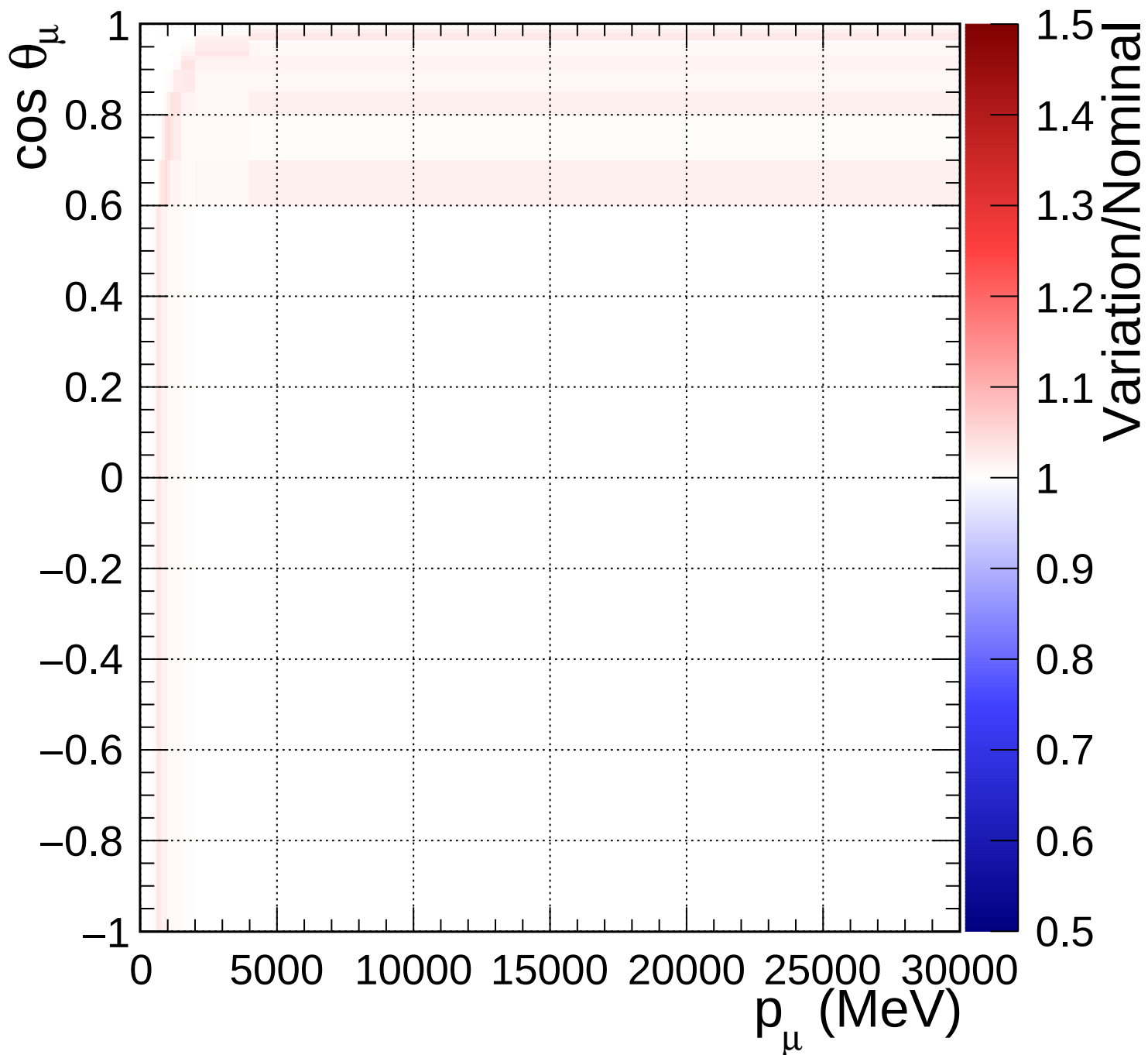
FGD2_anti-numuCC_0pi_Q2_norm_6_1.18
