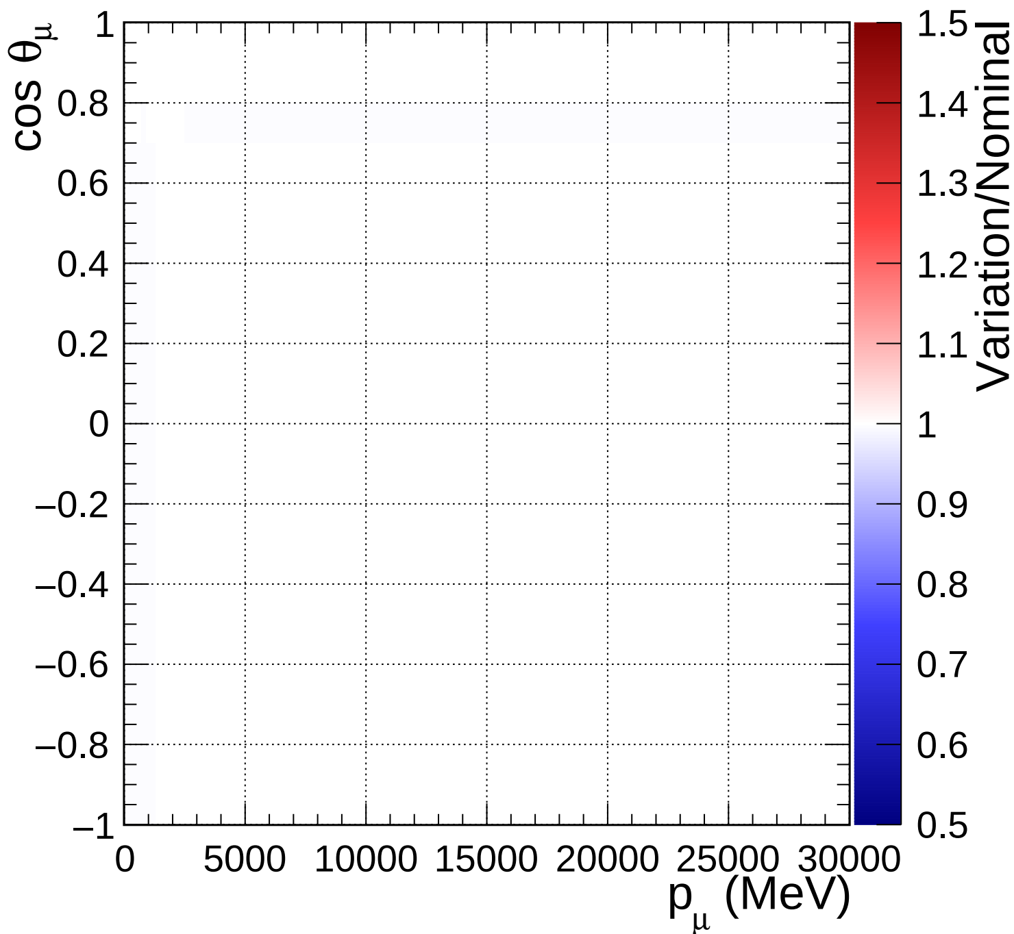
FGD2_anti-numuCC_1pi_Q2_norm_5_0.89
