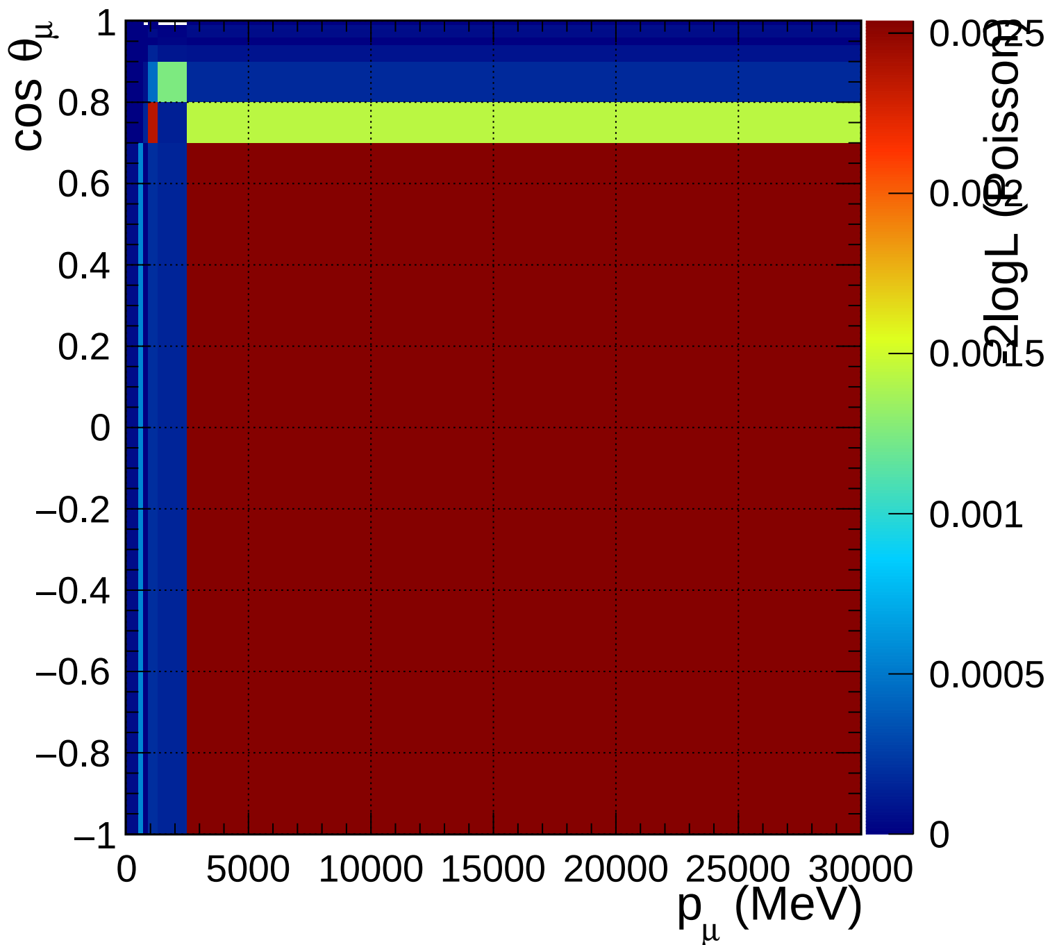
FGD1_anti-numuCC_1pi_Q2_norm_6_0.46
