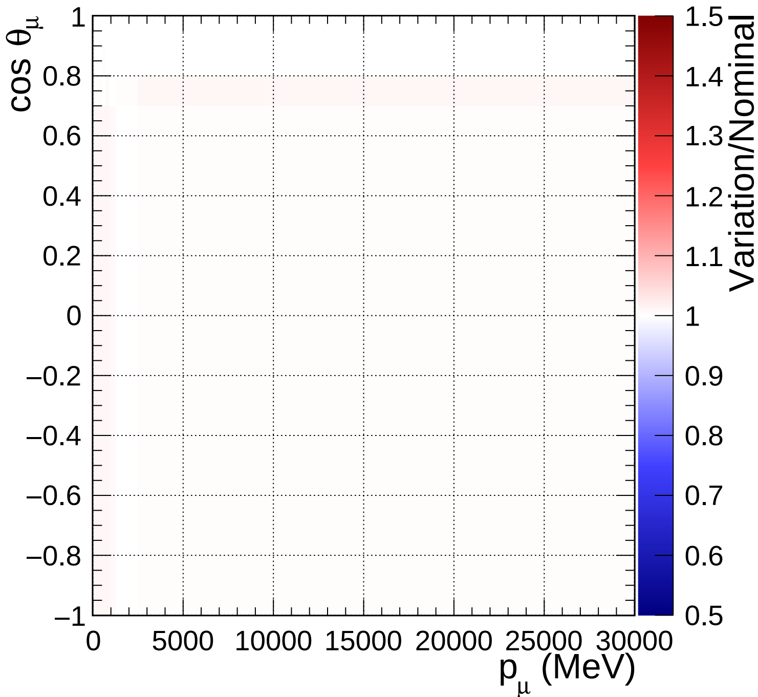
FGD2_anti-numuCC_1pi_Q2_norm_5_1.33
