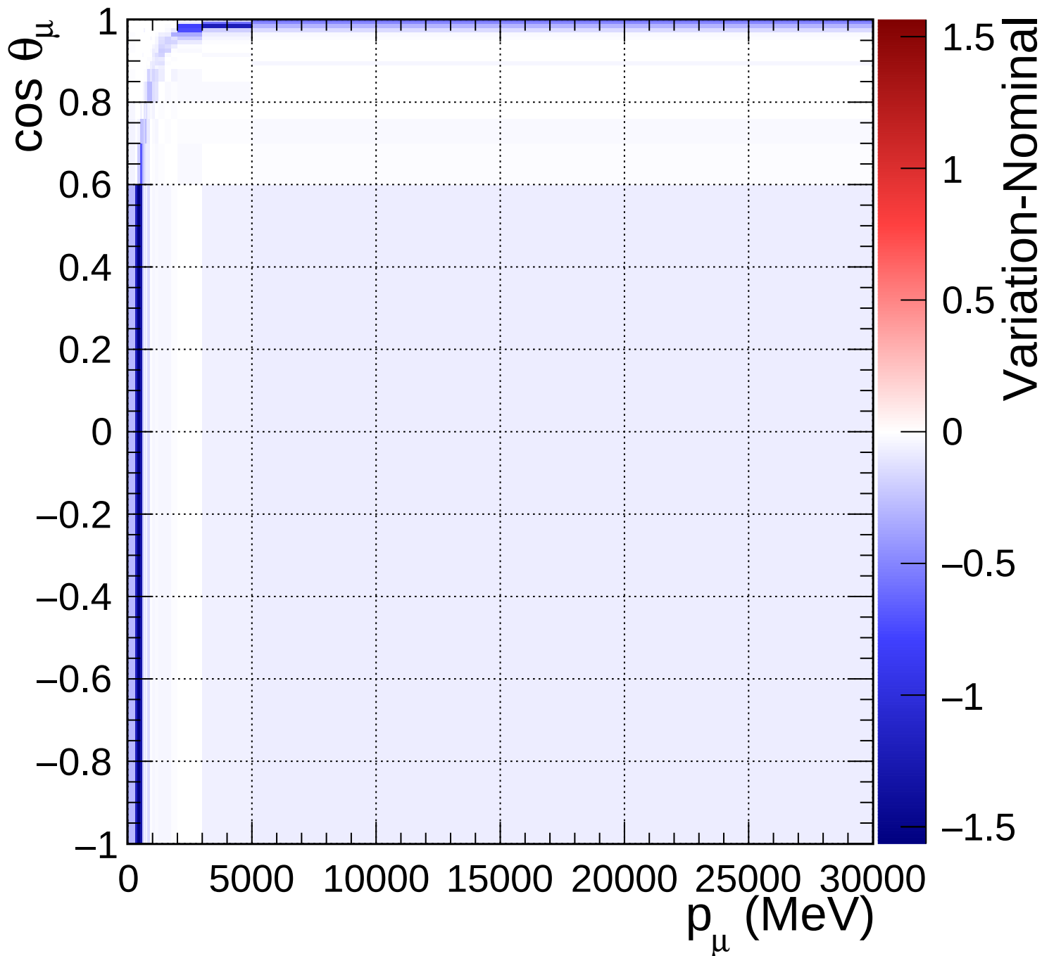
FGD1_numuCC_other_Q2_norm_5_0.67
