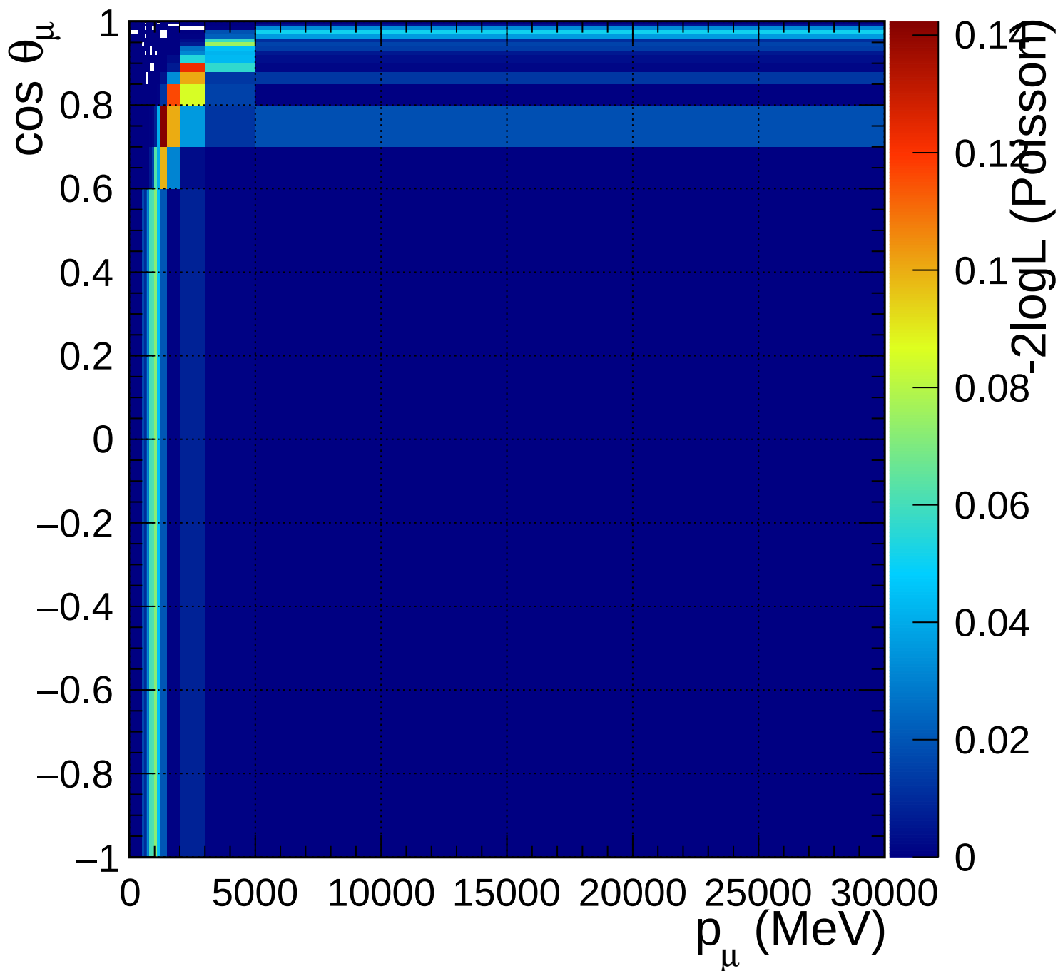
FGD1_numuCC_1pi_Q2_norm_7_-0.2
