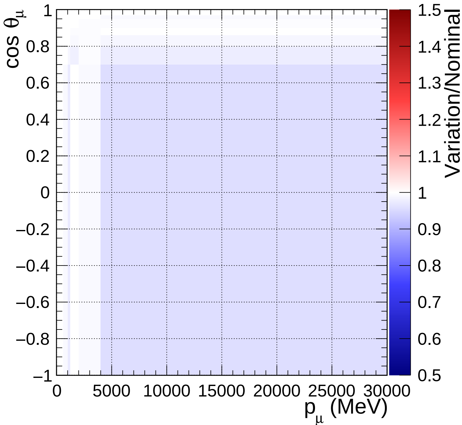
FGD1_NuMuBkg_CCoTher_in_AntiNu_Mode_Q2_norm_7_0.6
