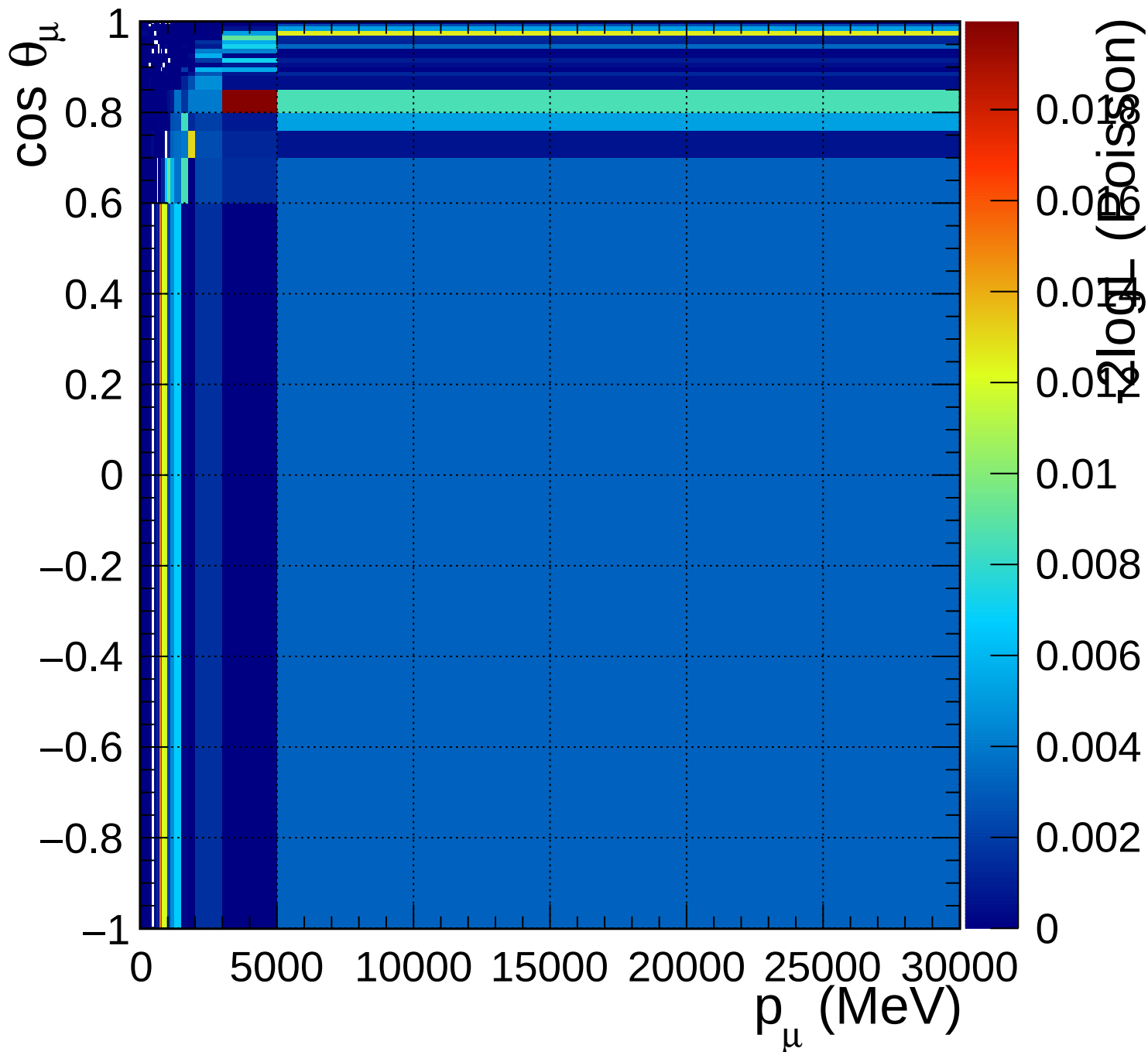
FGD1_numuCC_other_Q2_norm_7_-0.2
