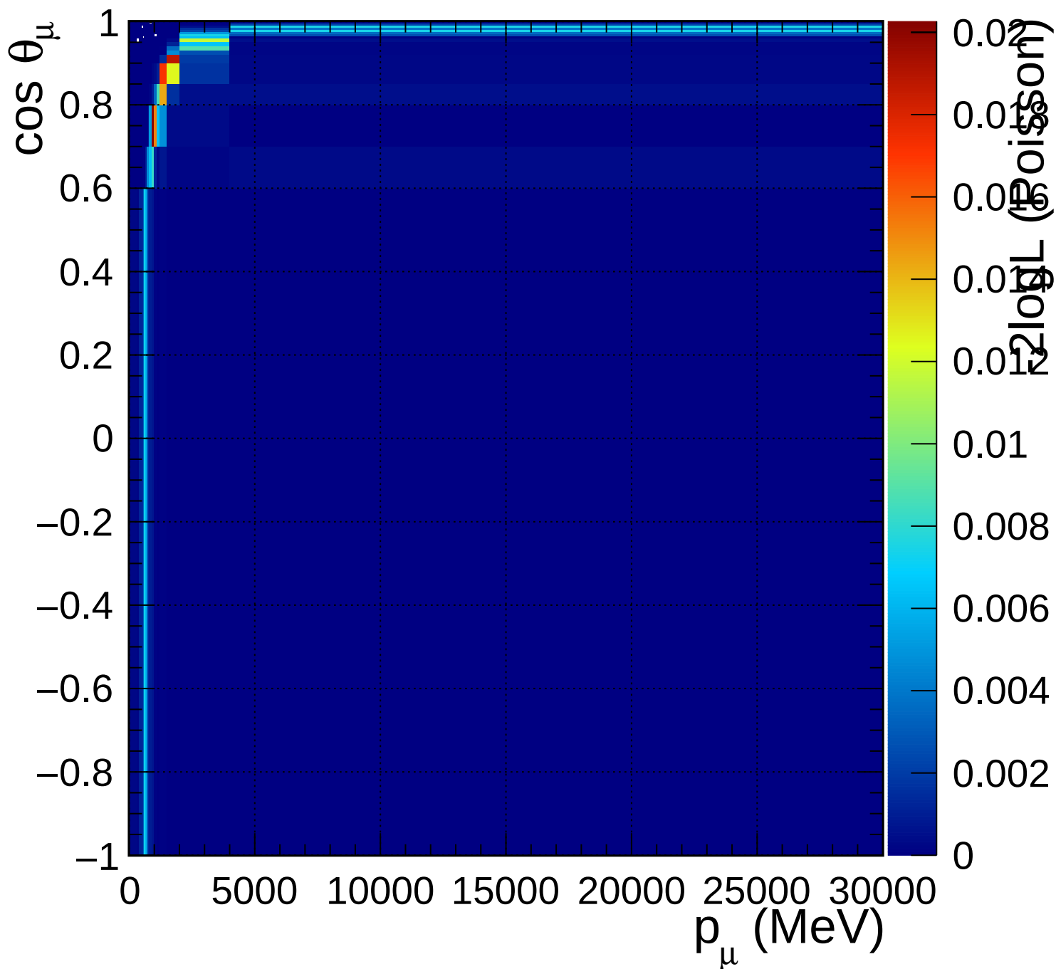
FGD2_anti-numuCC_0pi_Q2_norm_6_0.82
