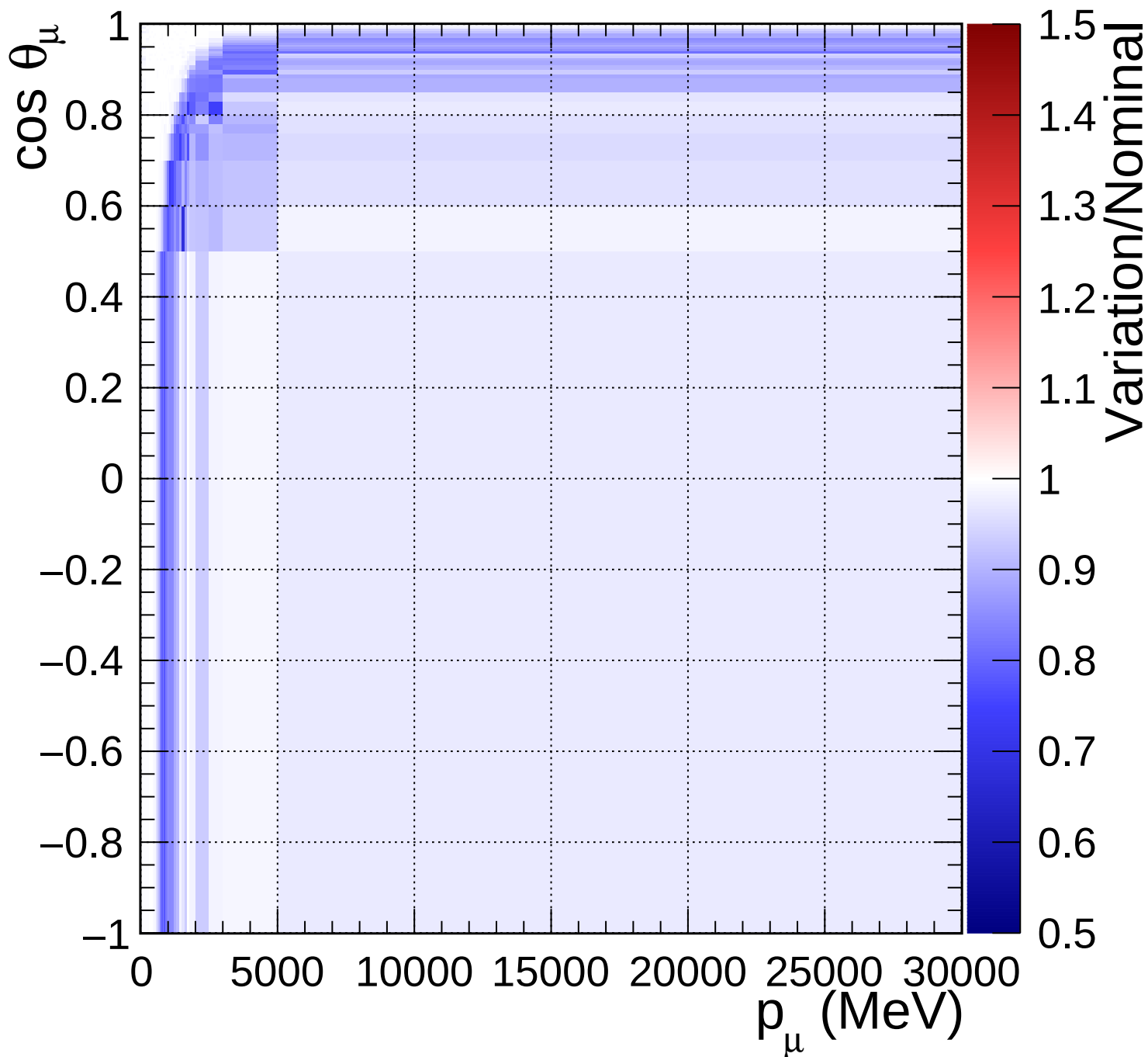
FGD1_numuCC_0pi_Q2_norm_7_-0.2
