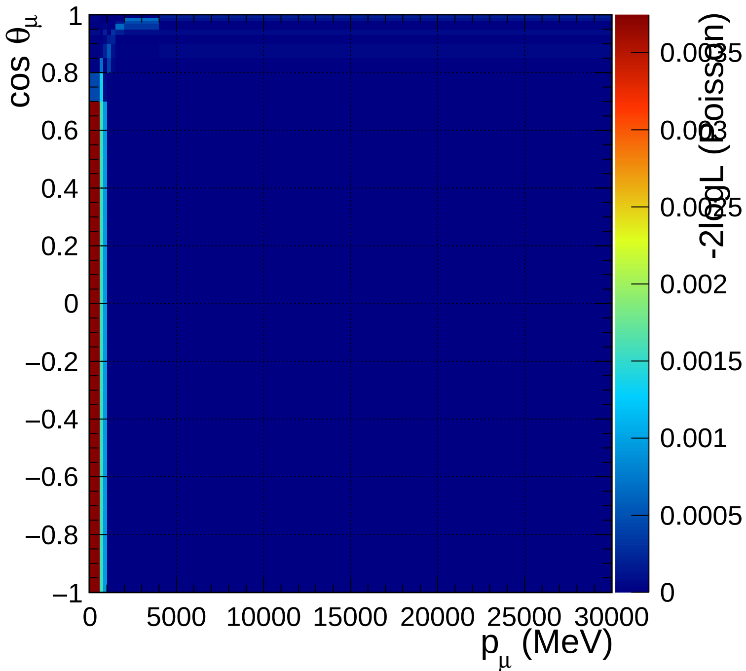
FGD1_anti-numuCC_other_Q2_norm_5_1.33
