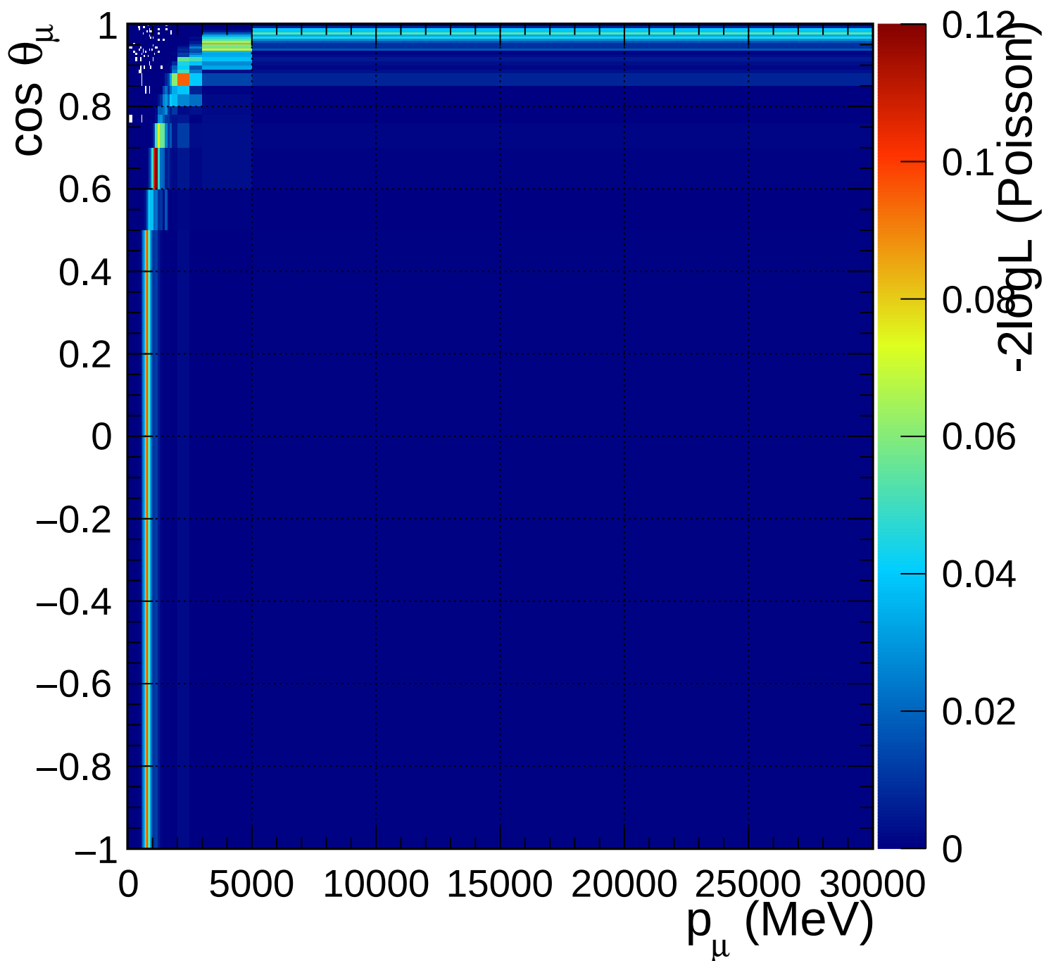
FGD1_numuCC_0pi_Q2_norm_7_0.6
