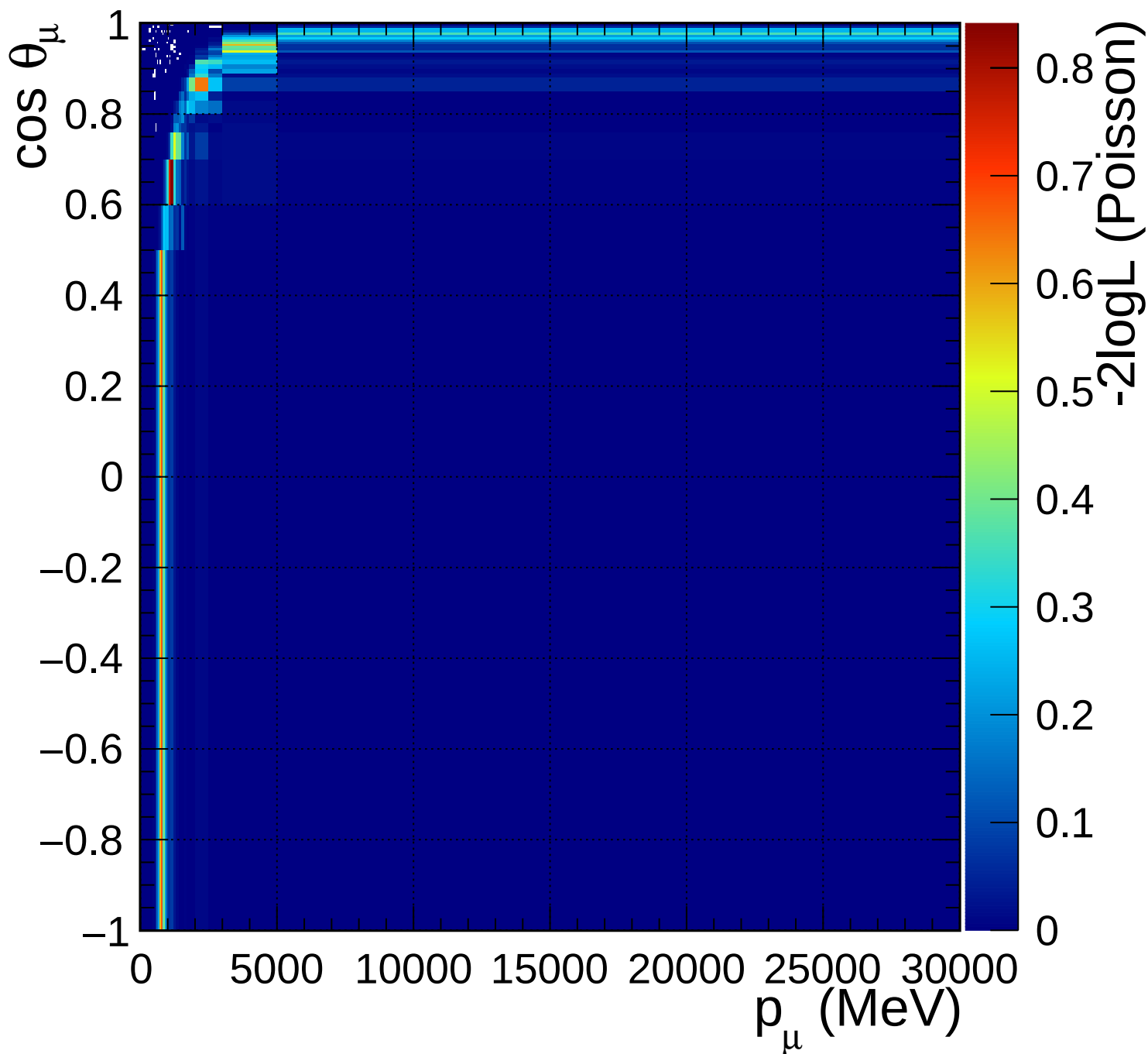
FGD1_numuCC_0pi_Q2_norm_7_-0.2
