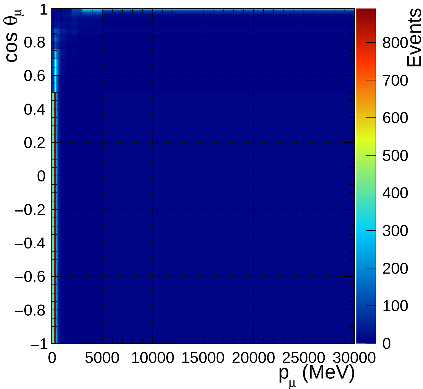
FGD2_numuCC_0pi_Q2_norm_6_1
