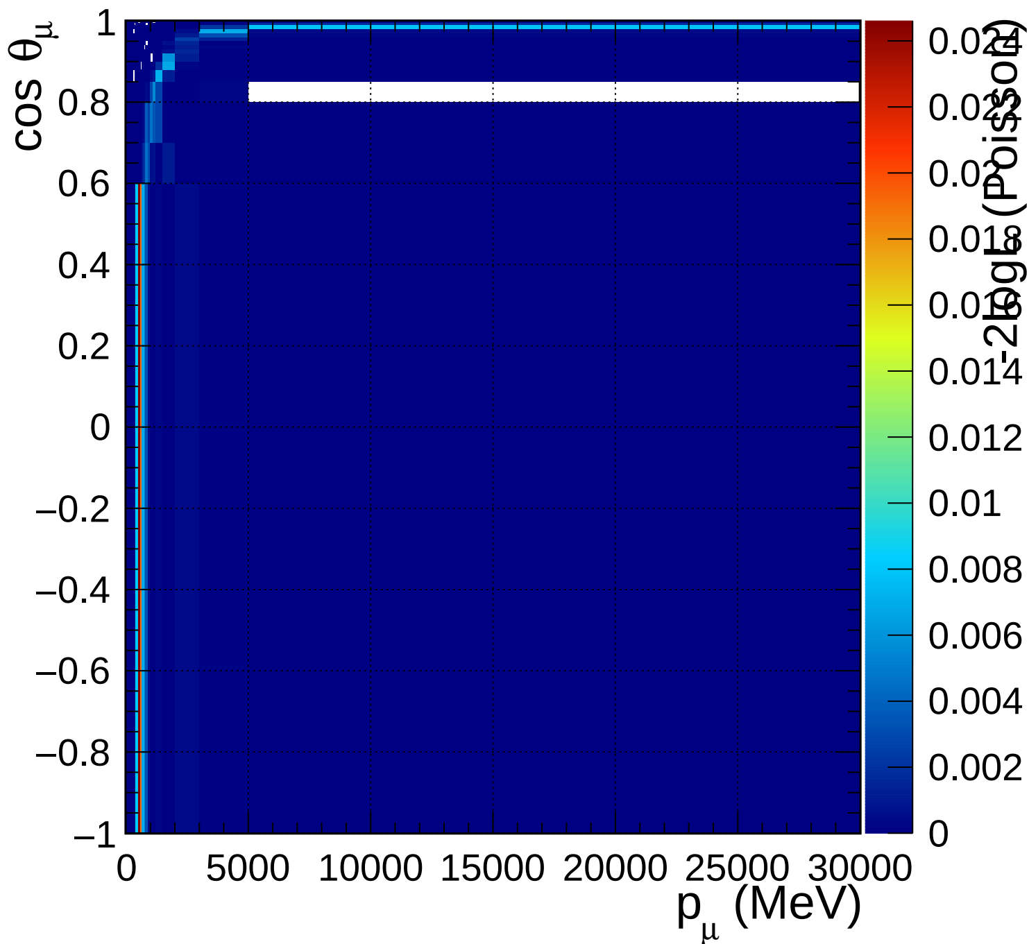
FGD1_numuCC_1pi_Q2_norm_6_1.54
