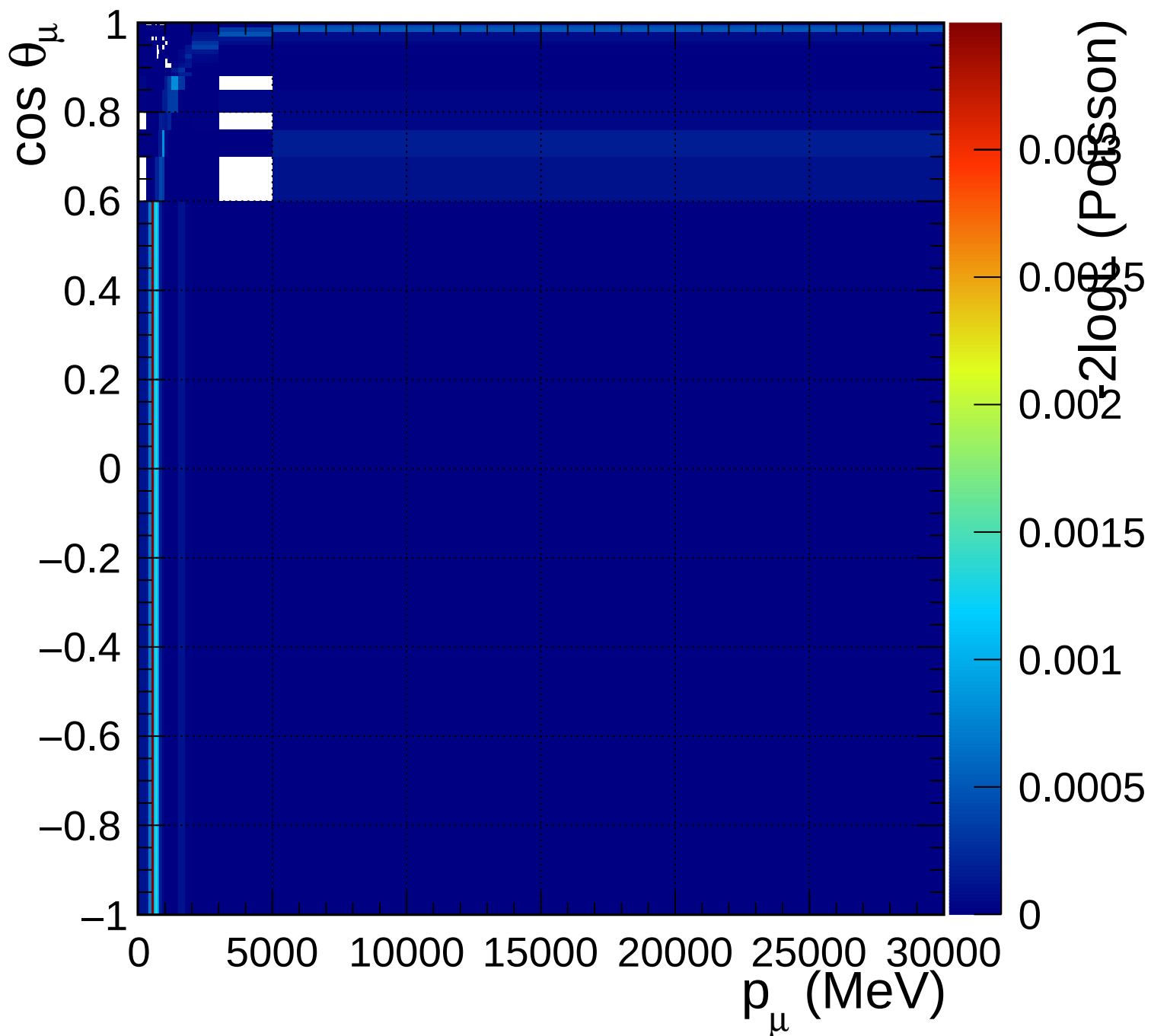
FGD1_numuCC_other_Q2_norm_6_0.82
