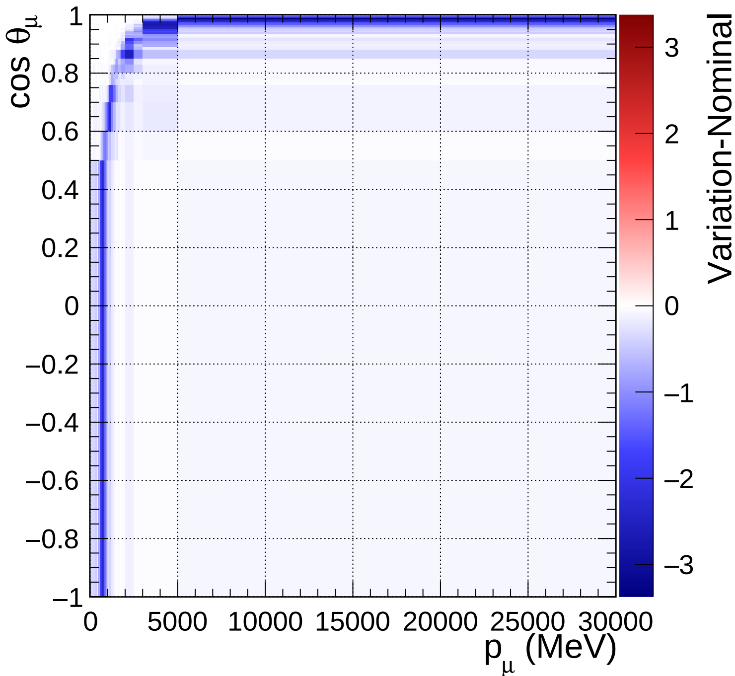
FGD1_numuCC_0pi_Q2_norm_7_0.6
