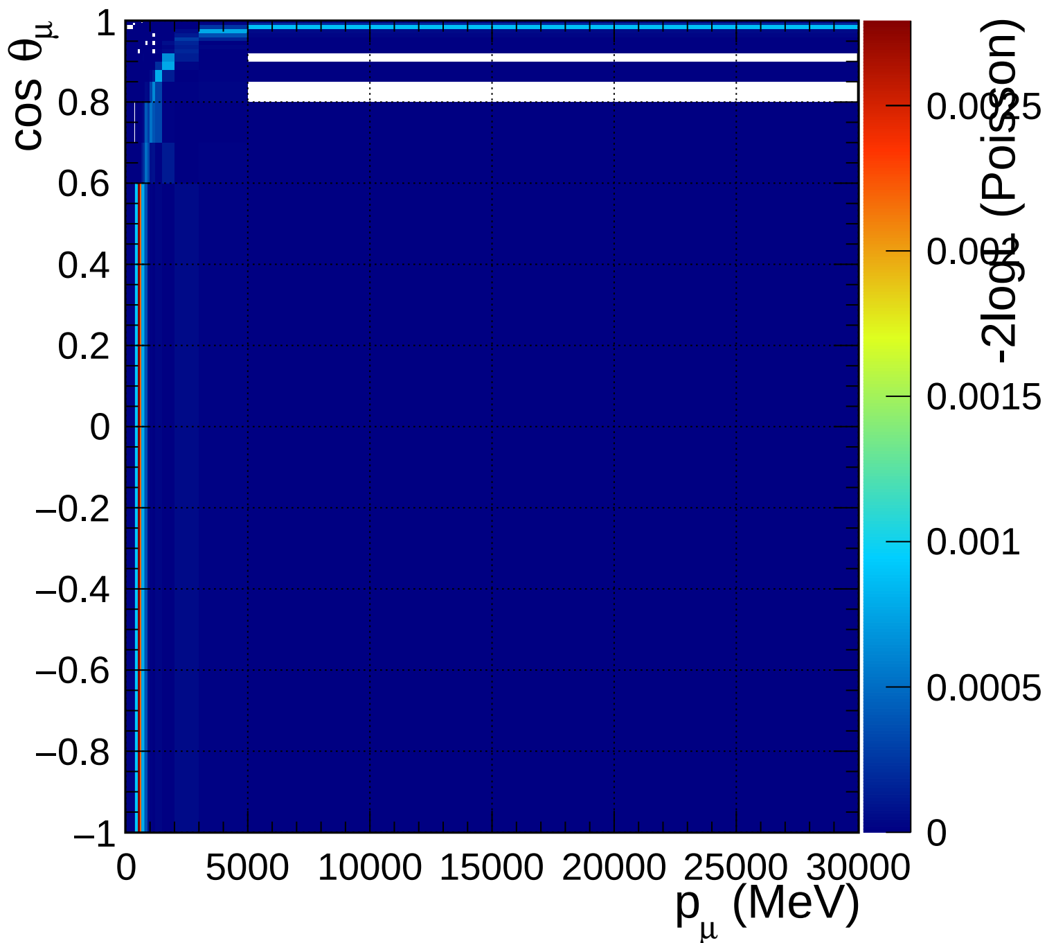
FGD1_numuCC_1pi_Q2_norm_6_0.82
