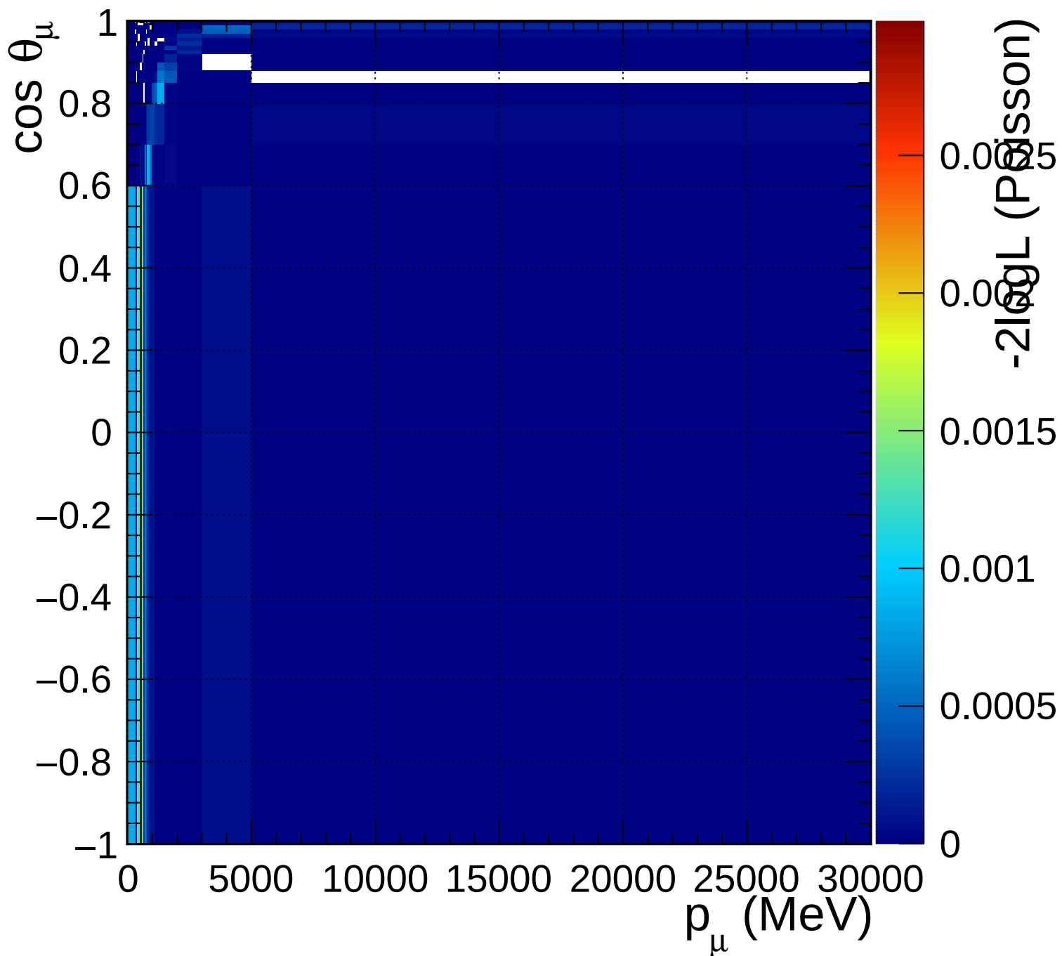
FGD2_numuCC_1pi_Q2_norm_6_0.82
