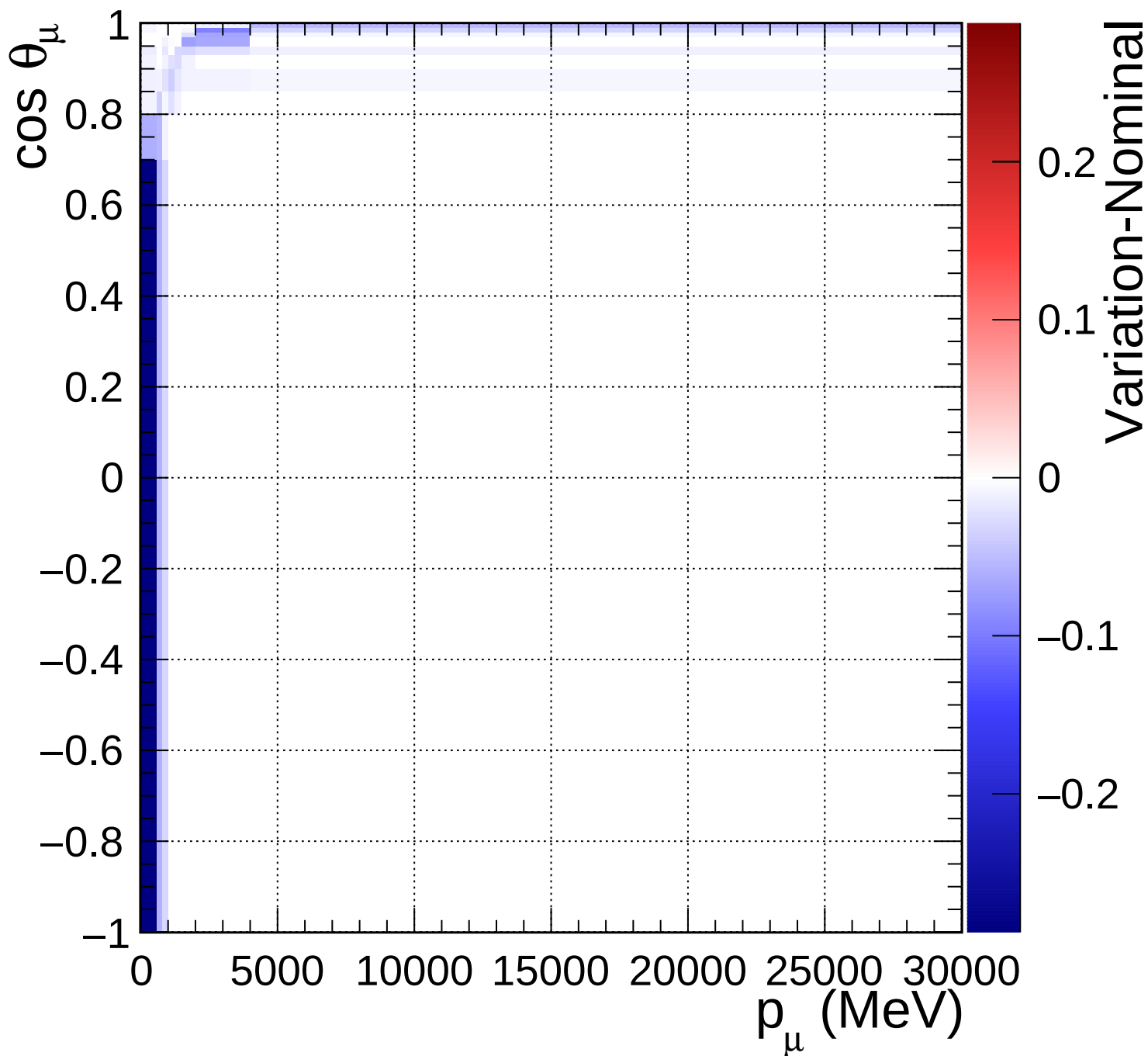
FGD1_anti-numuCC_other_Q2_norm_5_0.89
