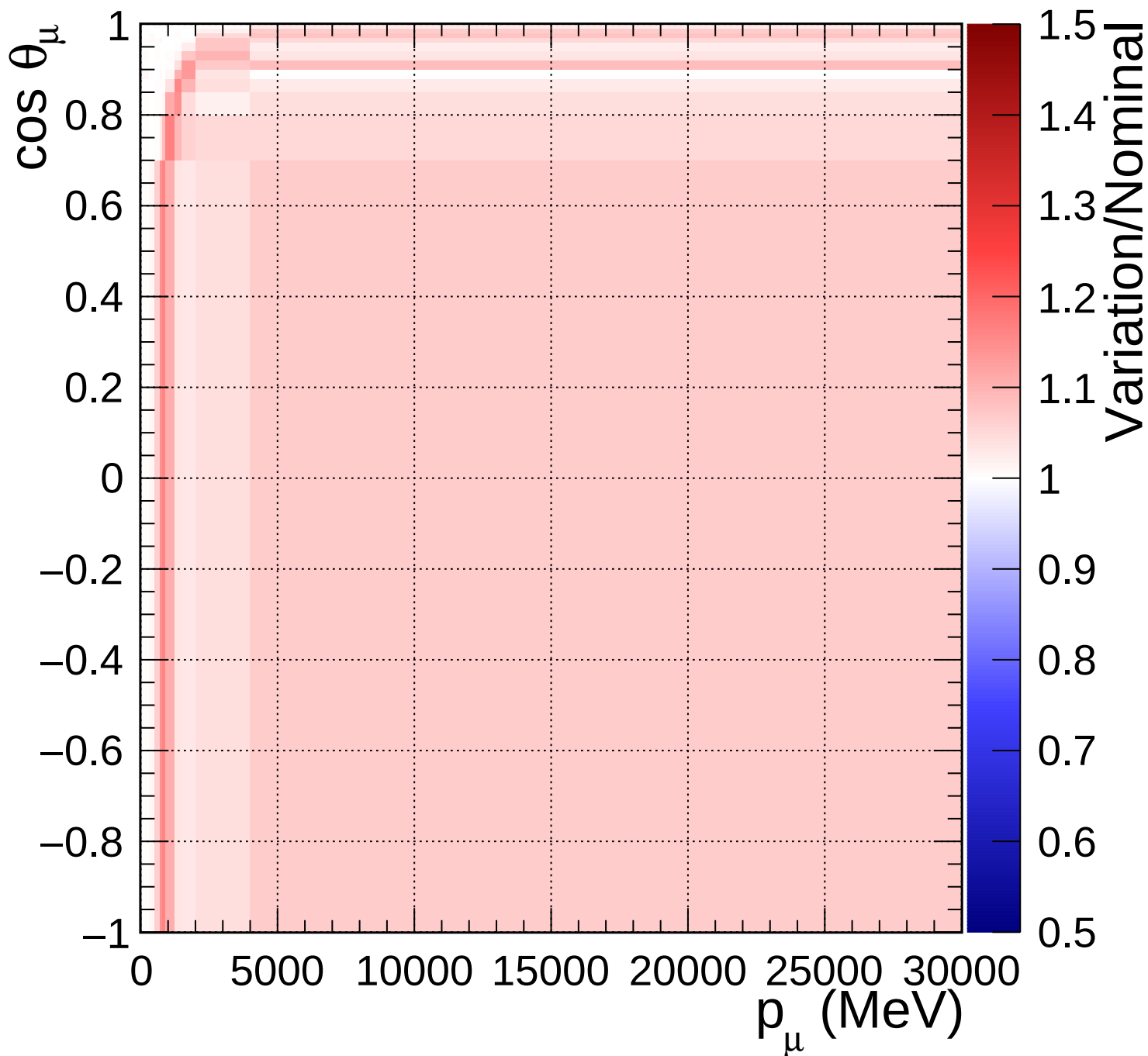
FGD1_NuMuBkg_CC0pi_in_AntiNu_Mode_Q2_norm_6_1.54
