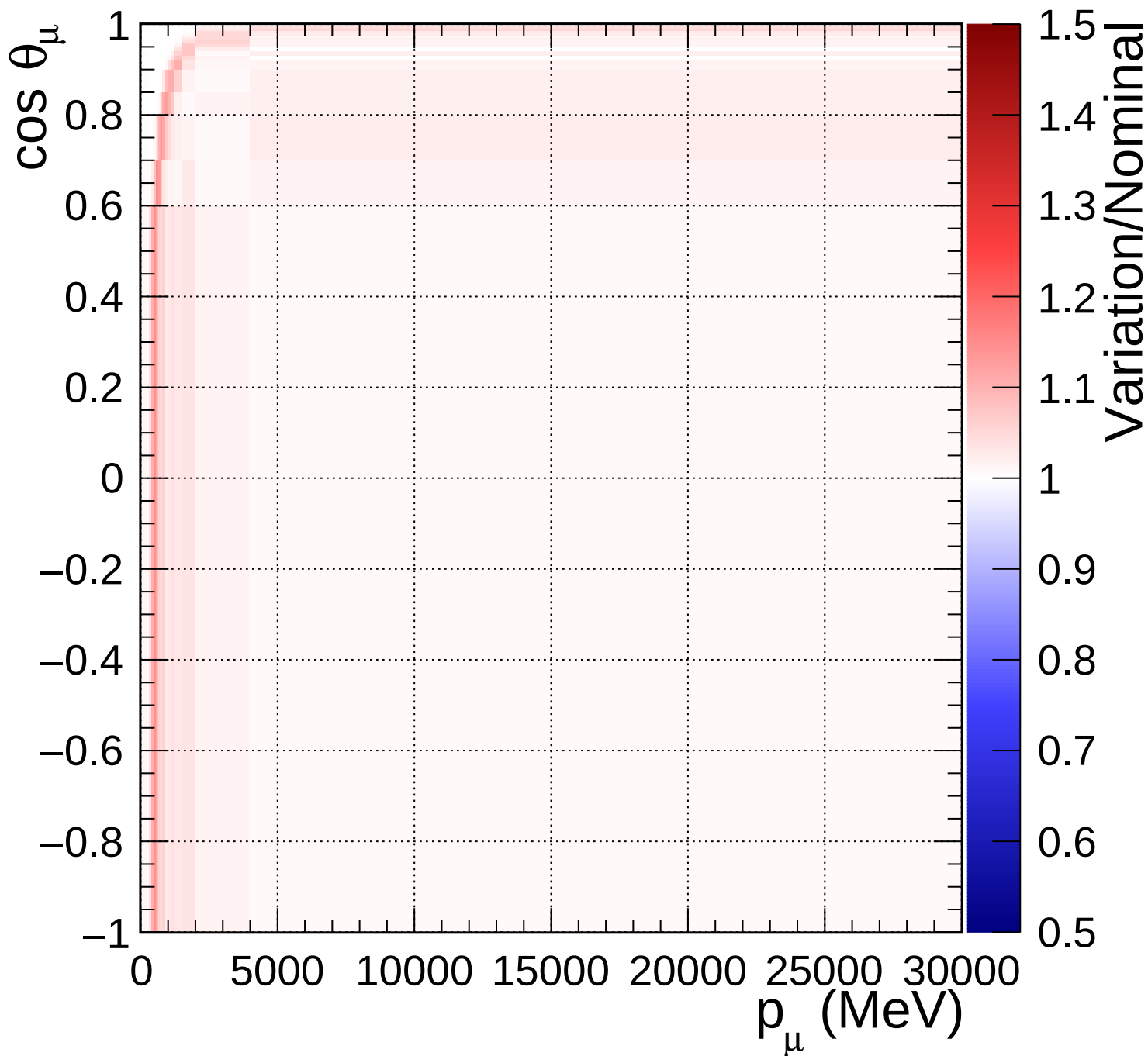
FGD1_anti-numuCC_0pi_Q2_norm_5_1.33
