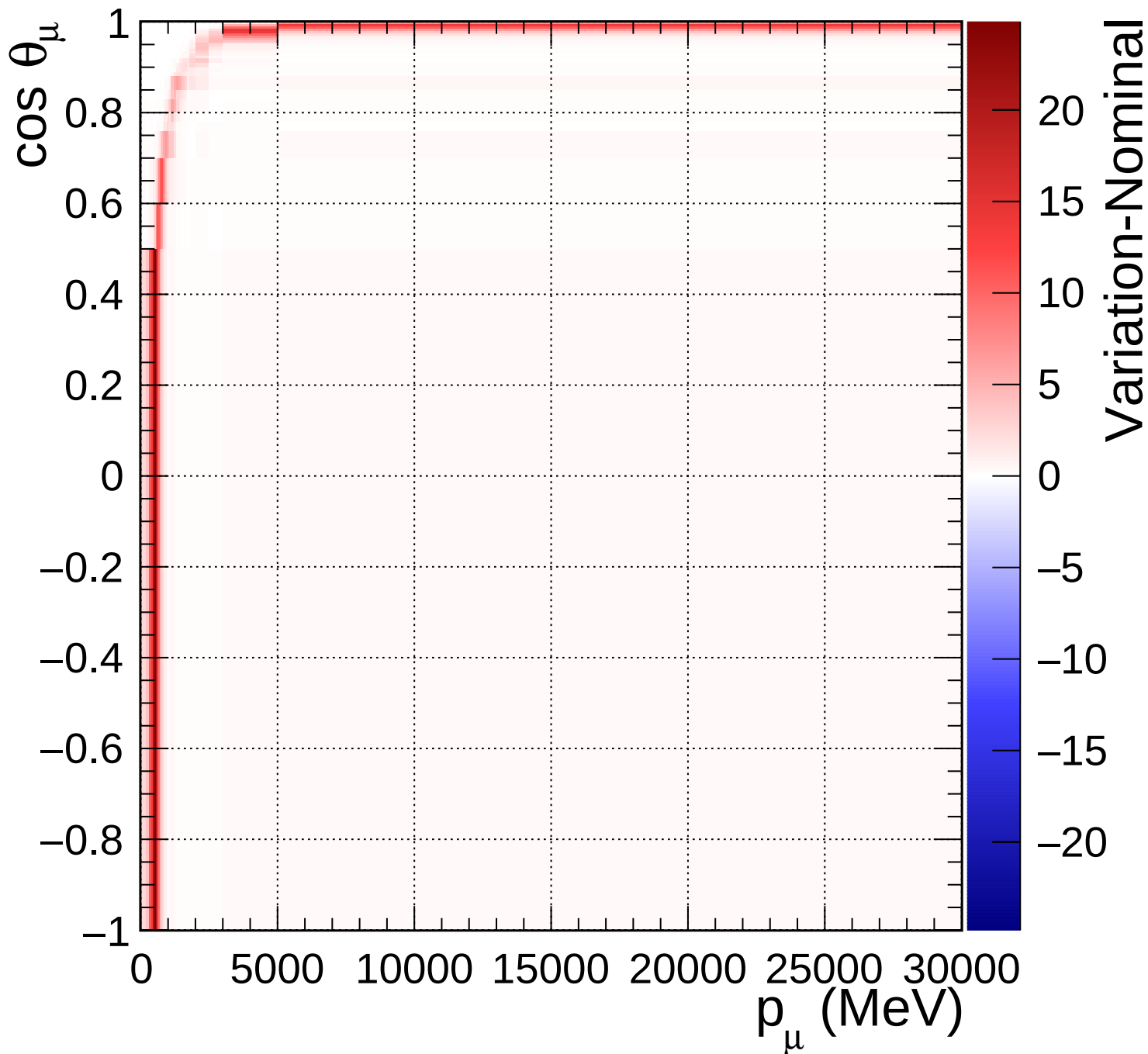
FGD1_numuCC_0pi_Q2_norm_6_1.54
