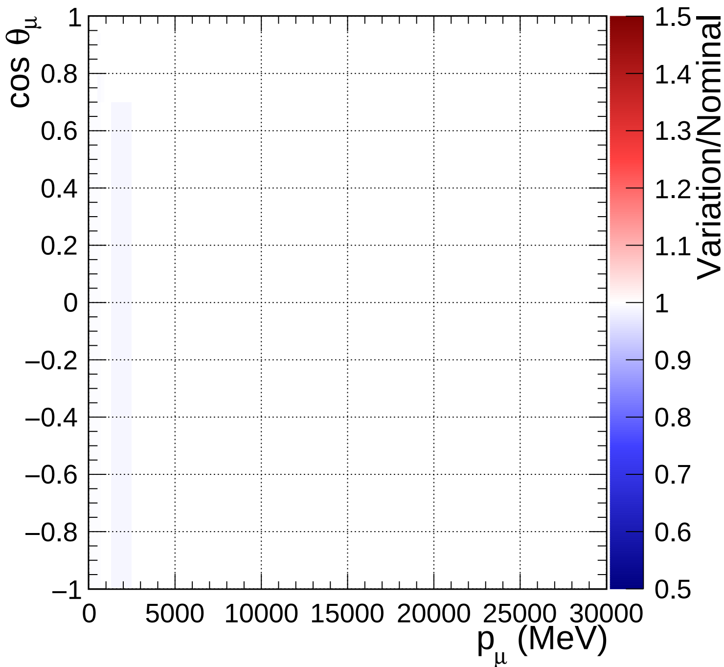
FGD1_anti-numuCC_1pi_Q2_norm_5_0.67
