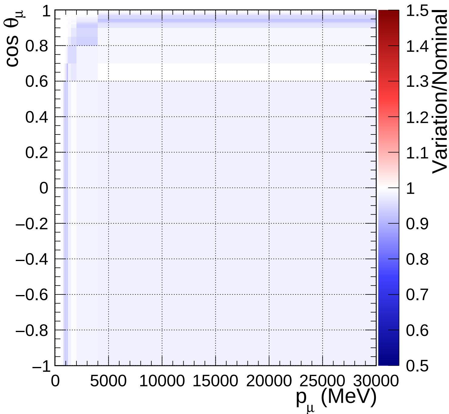
FGD1_anti-numuCC_0pi_Q2_norm_7_0.6
