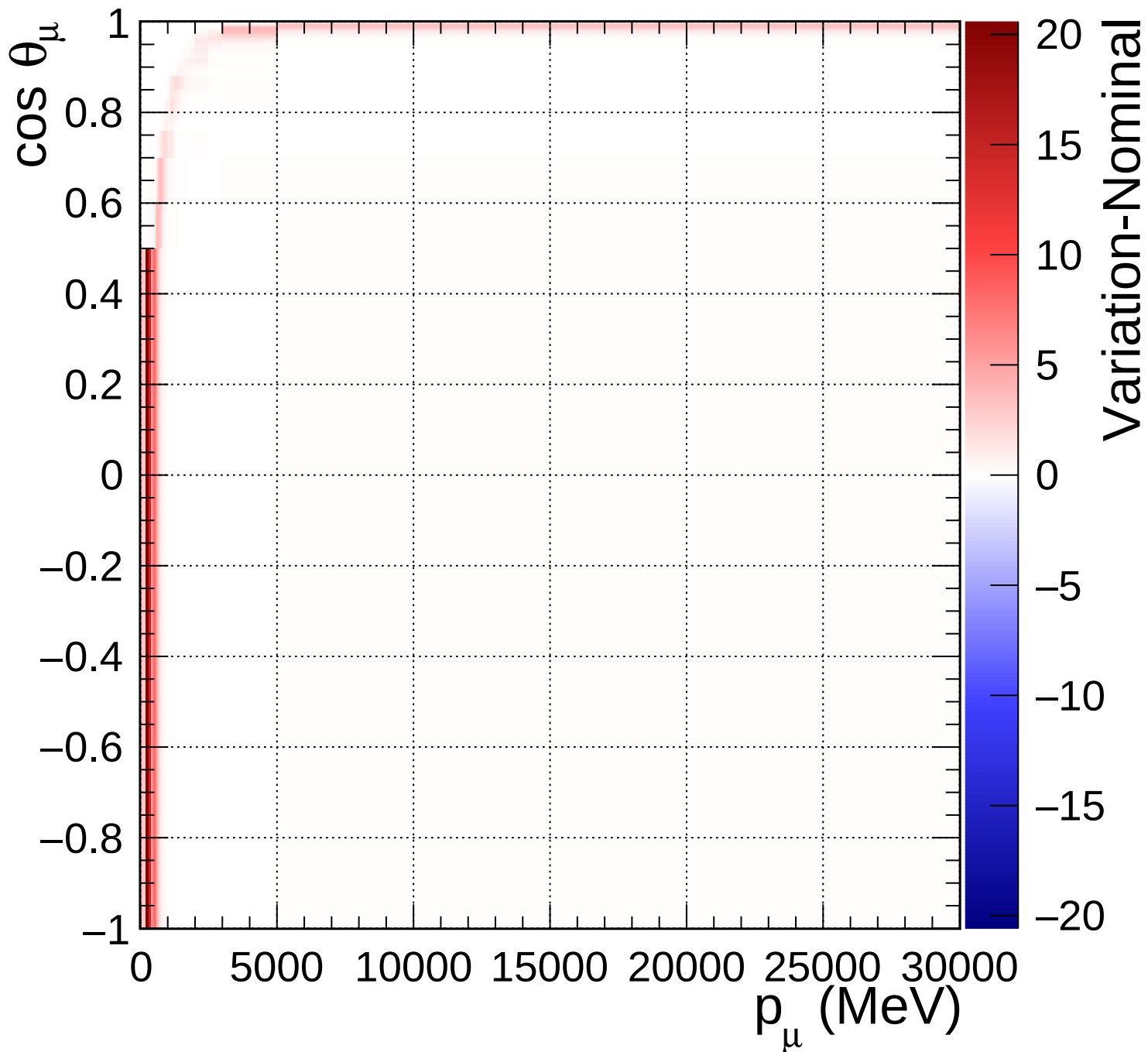
FGD2_numuCC_0pi_Q2_norm_6_1.18
