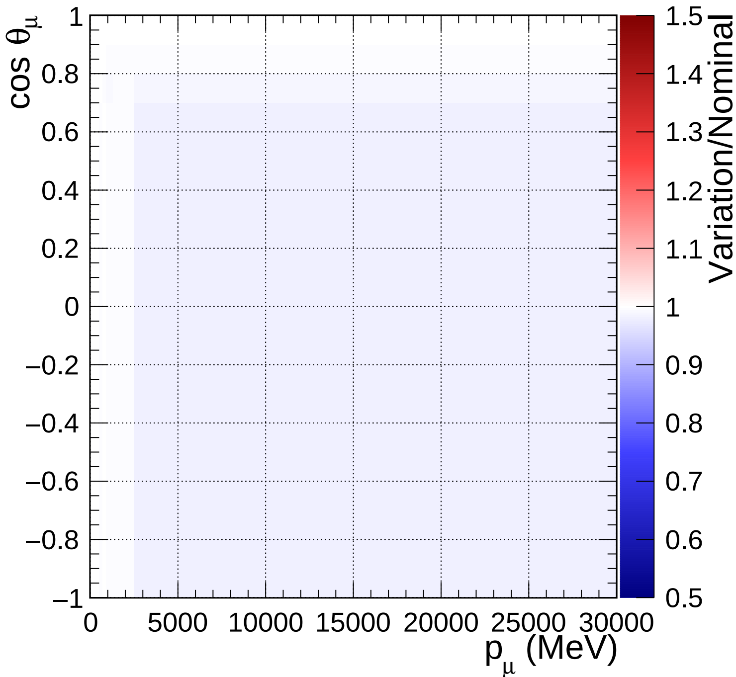
FGD1_anti-numuCC_1pi_Q2_norm_6_0.82
