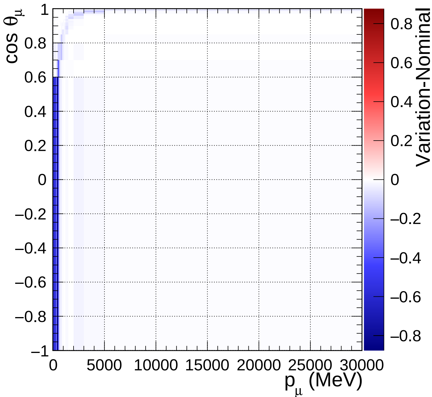
FGD2_numuCC_1pi_Q2_norm_5_0.89
