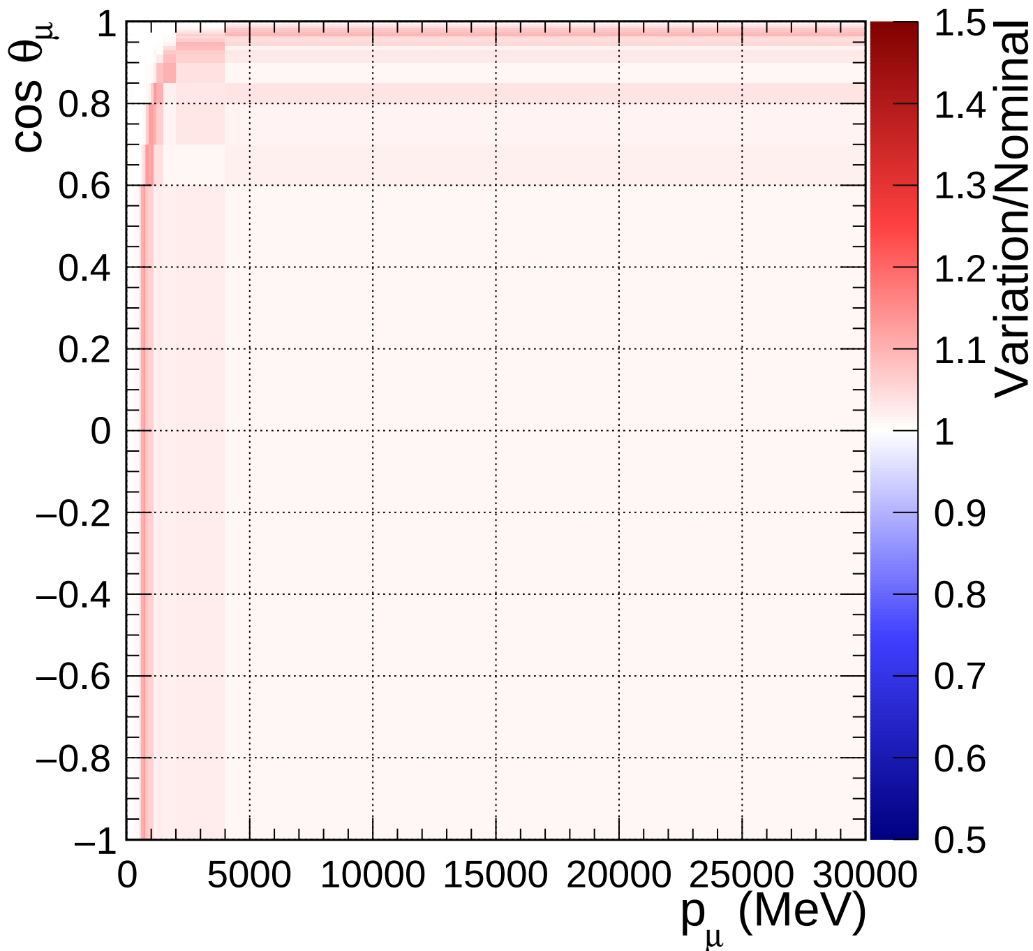
FGD1_anti-numuCC_0pi_Q2_norm_6_1.54
