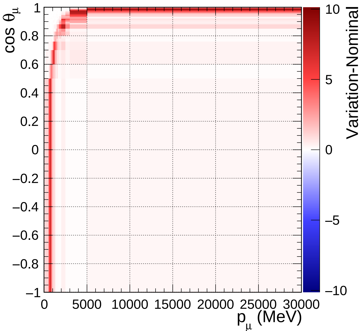
FGD1_numuCC_0pi_Q2_norm_7_2.2
