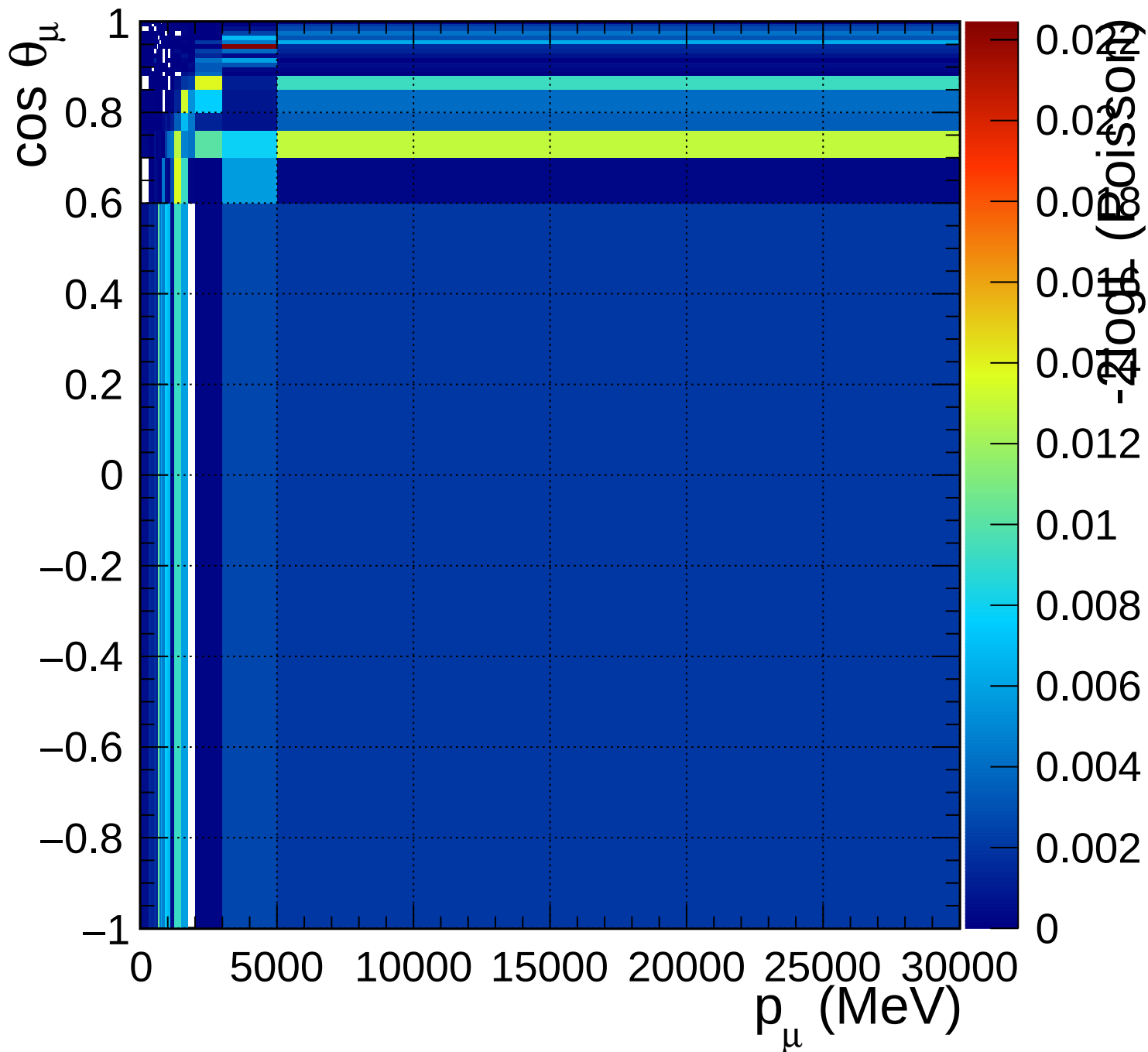
FGD2_numuCC_other_Q2_norm_7_-0.2
