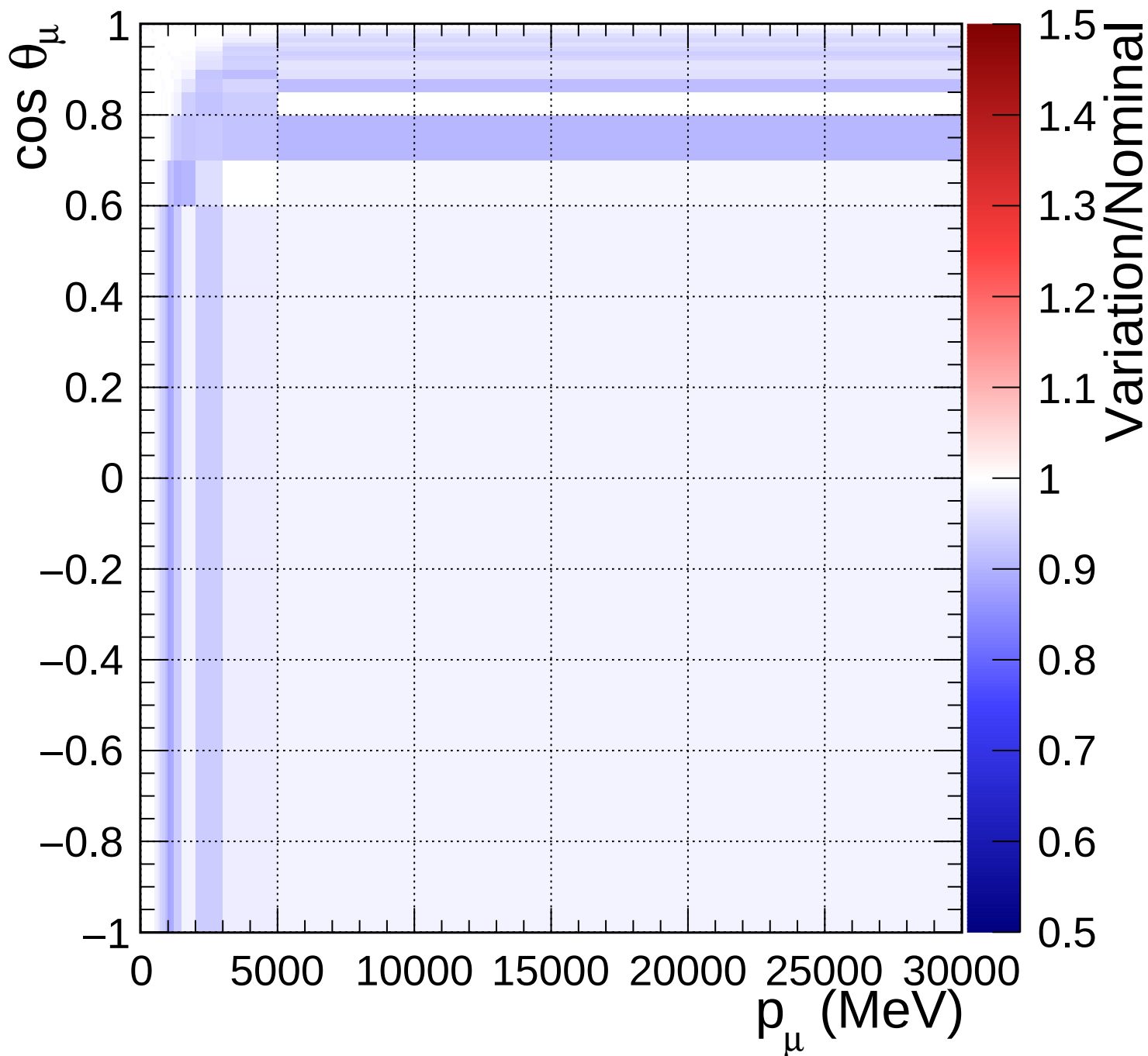
FGD1_numuCC_1pi_Q2_norm_7_-0.2
