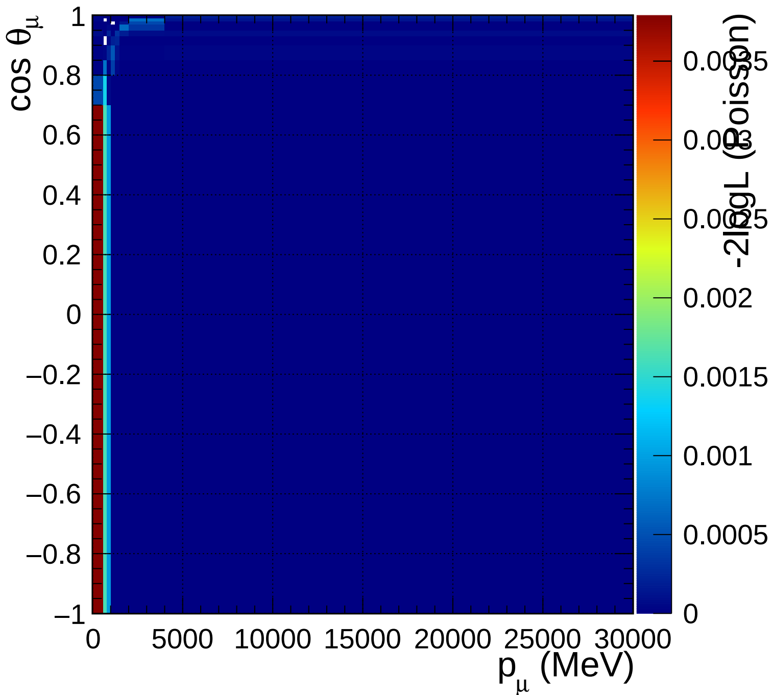
FGD1_anti-numuCC_other_Q2_norm_5_0.67
