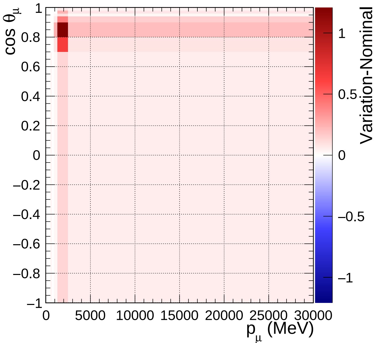
FGD1_anti-numuCC_1pi_Q2_norm_7_1.4
