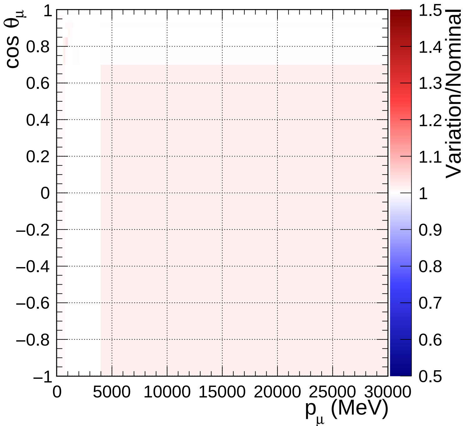
FGD2_anti-numuCC_other_Q2_norm_5_1.33
