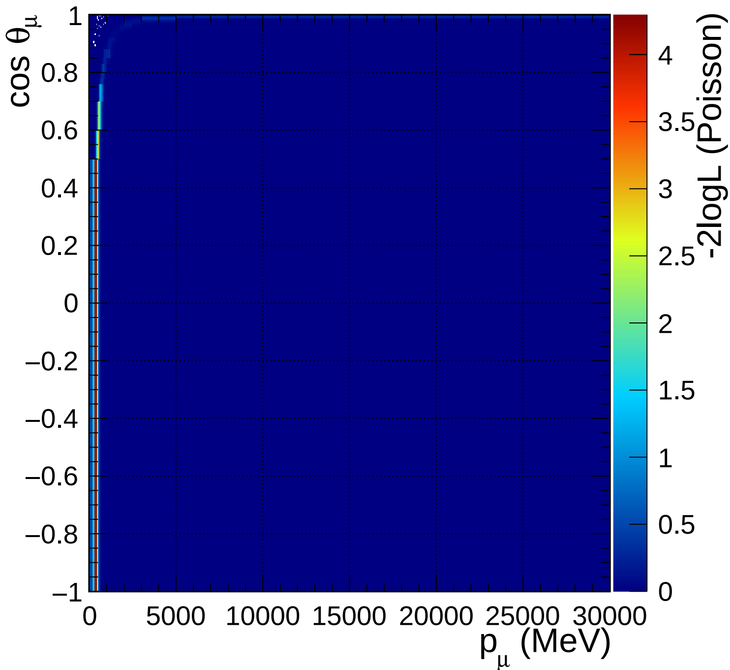
FGD2_numuCC_0pi_Q2_norm_5_1.33
