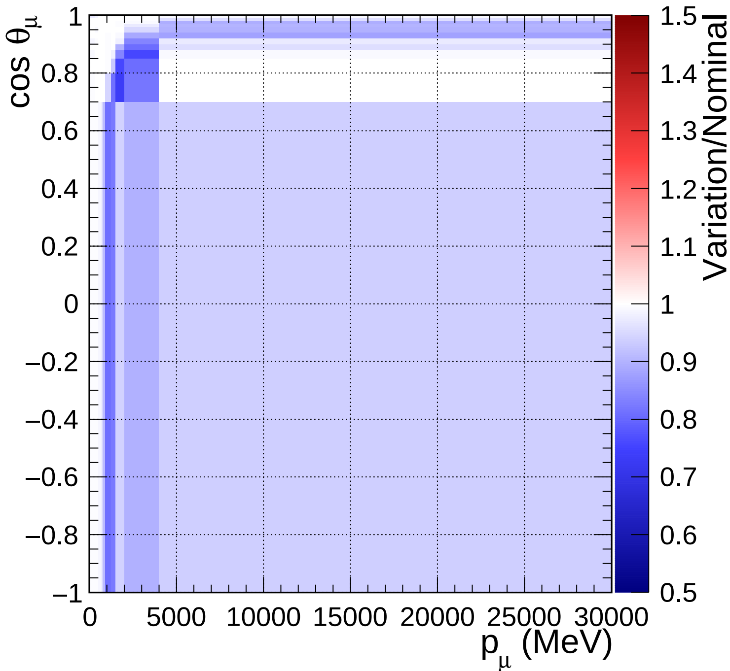
FGD1_NuMuBkg_CC0pi_in_AntiNu_Mode_Q2_norm_7_-0.2
