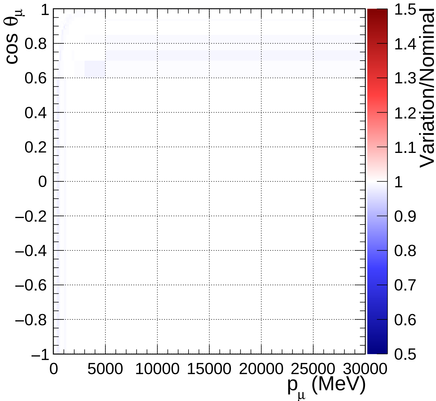
FGD2_numuCC_other_Q2_norm_5_0.67
