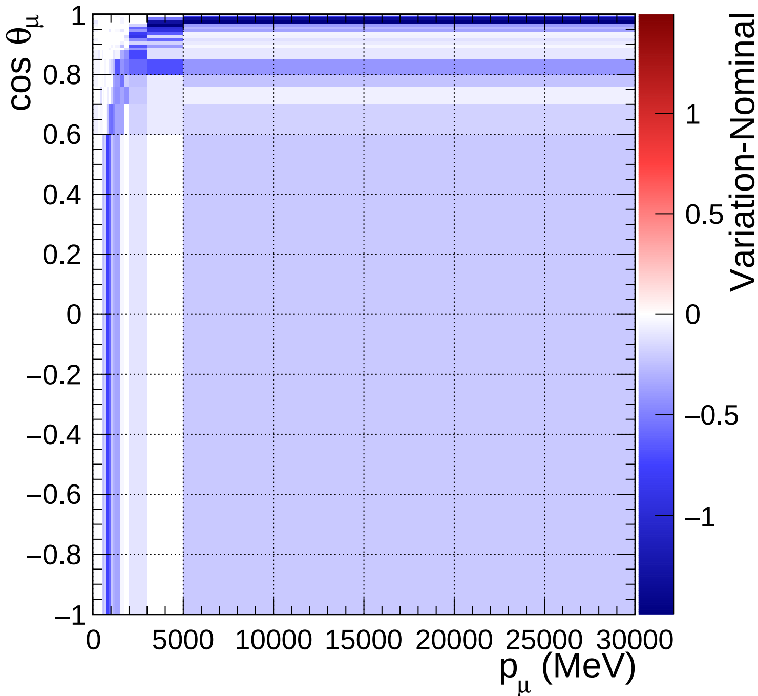
FGD1_numuCC_other_Q2_norm_7_-0.2
