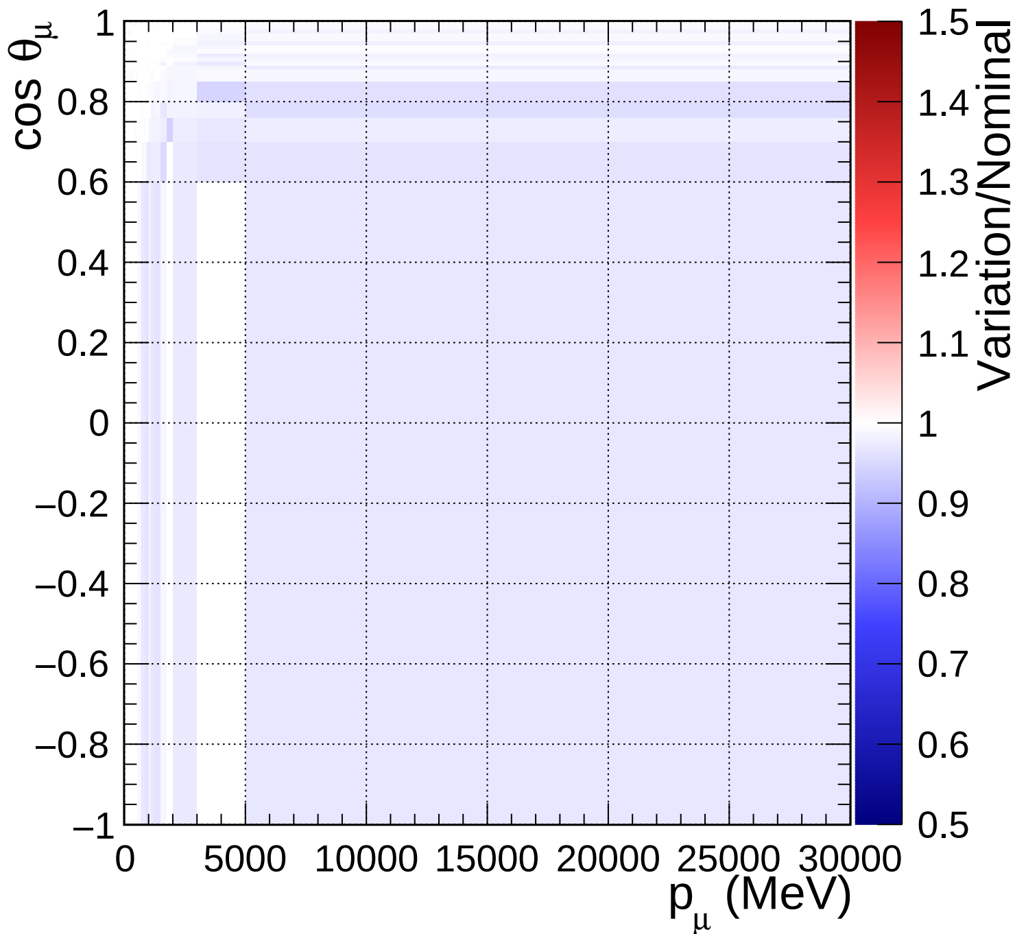
FGD1_numuCC_other_Q2_norm_7_-0.2
