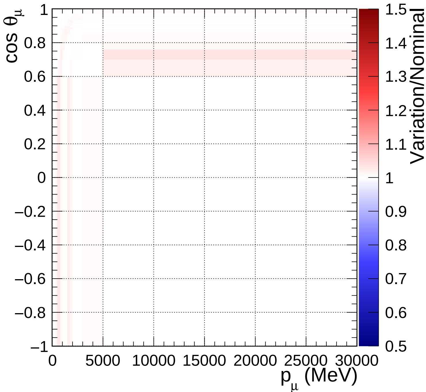
FGD1_numuCC_other_Q2_norm_6_1.54
