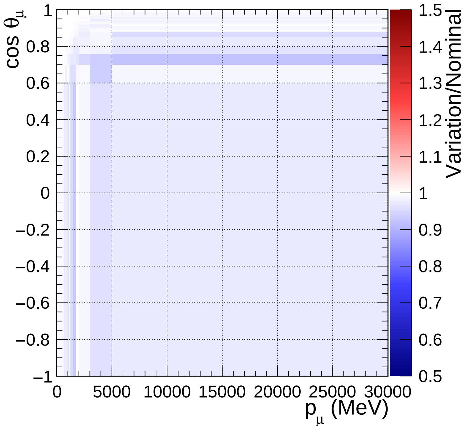
FGD2_numuCC_other_Q2_norm_7_-0.2
