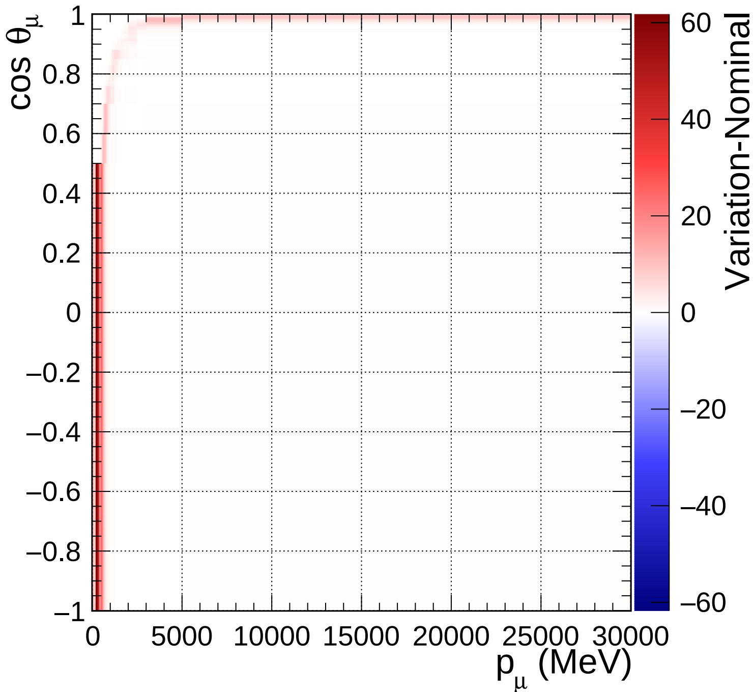
FGD2_numuCC_0pi_Q2_norm_6_1.54
