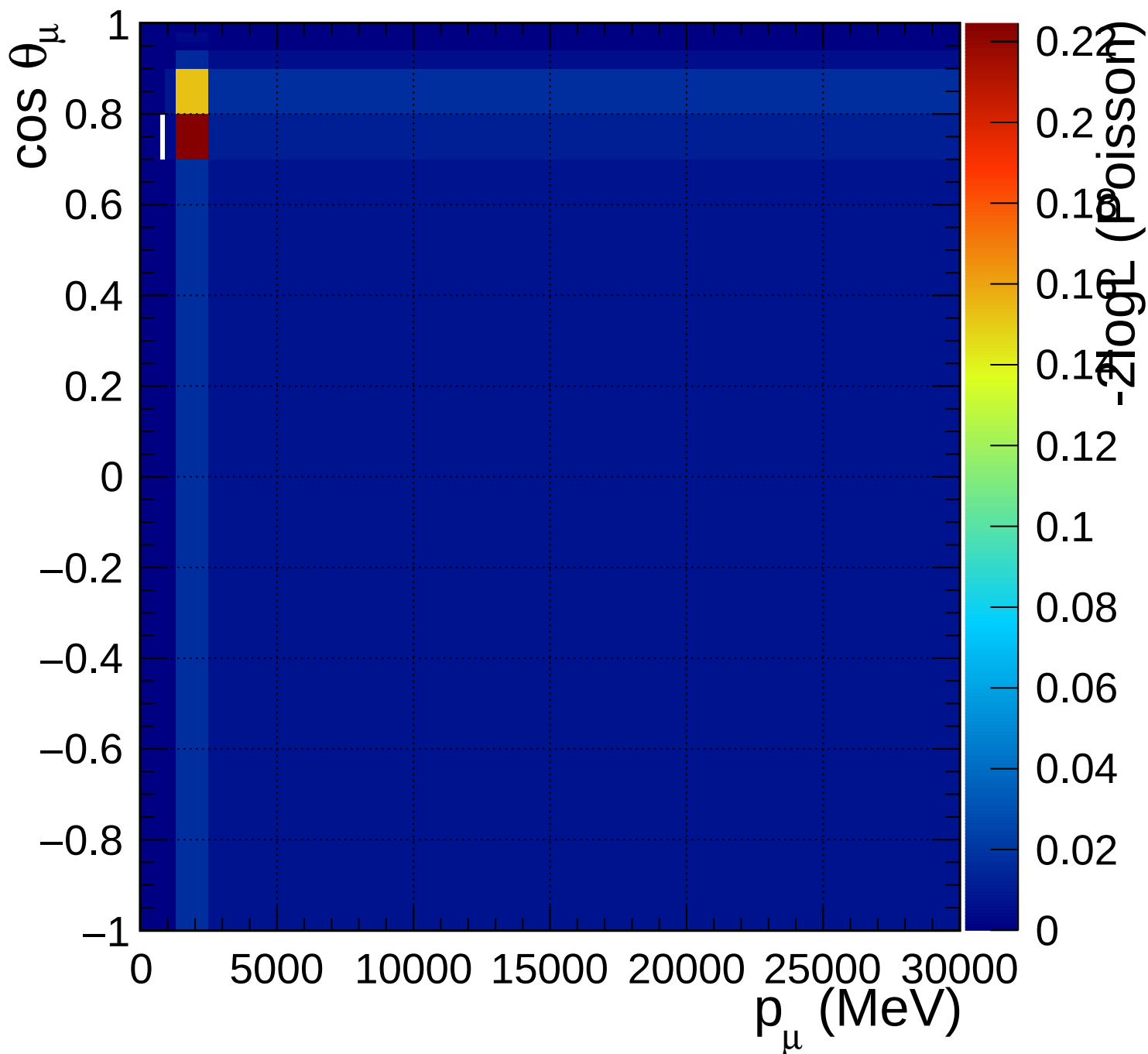
FGD1_anti-numuCC_1pi_Q2_norm_7_-0.2
