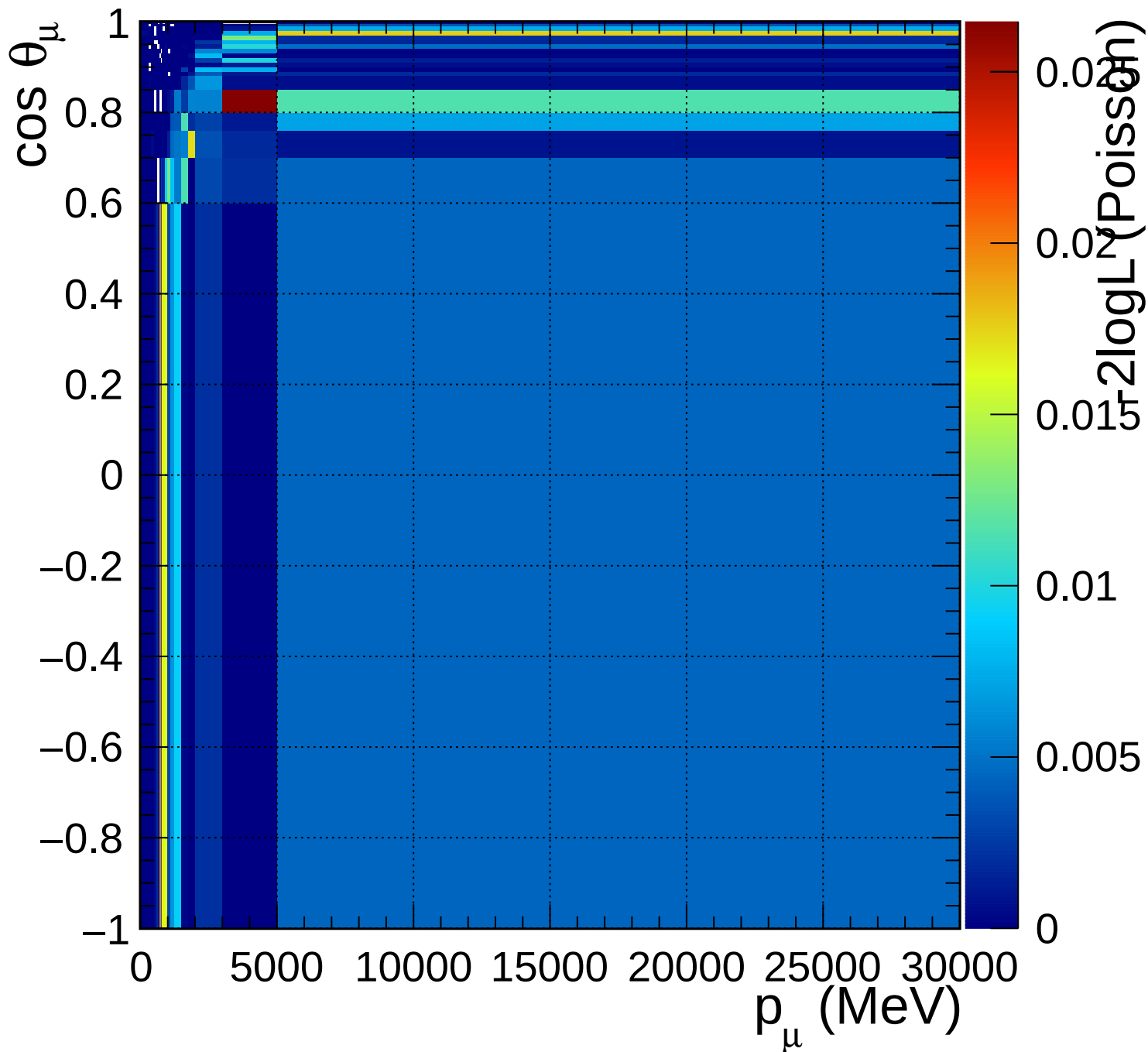
FGD1_numuCC_other_Q2_norm_7_2.2
