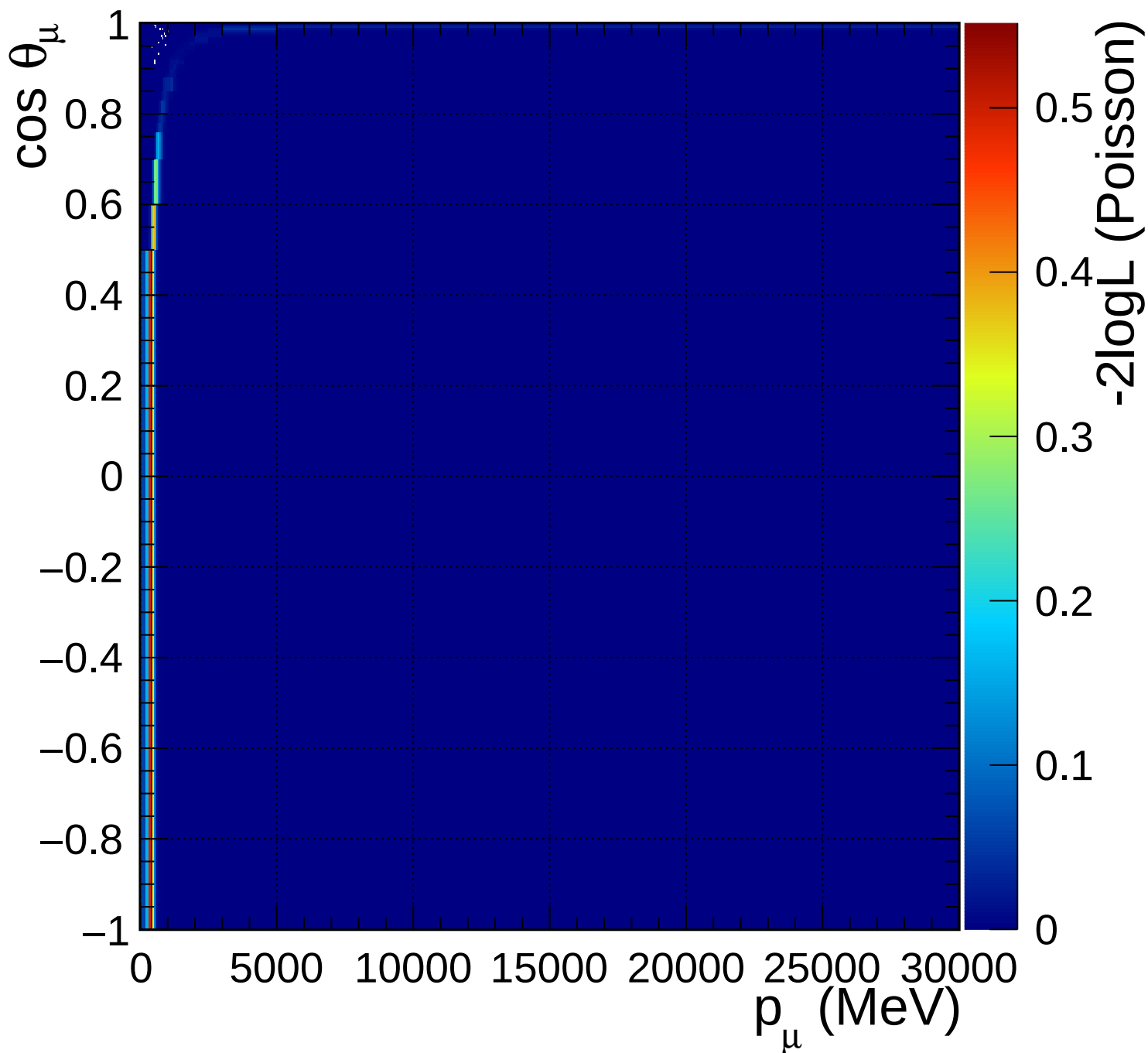
FGD2_numuCC_0pi_Q2_norm_5_0.89
