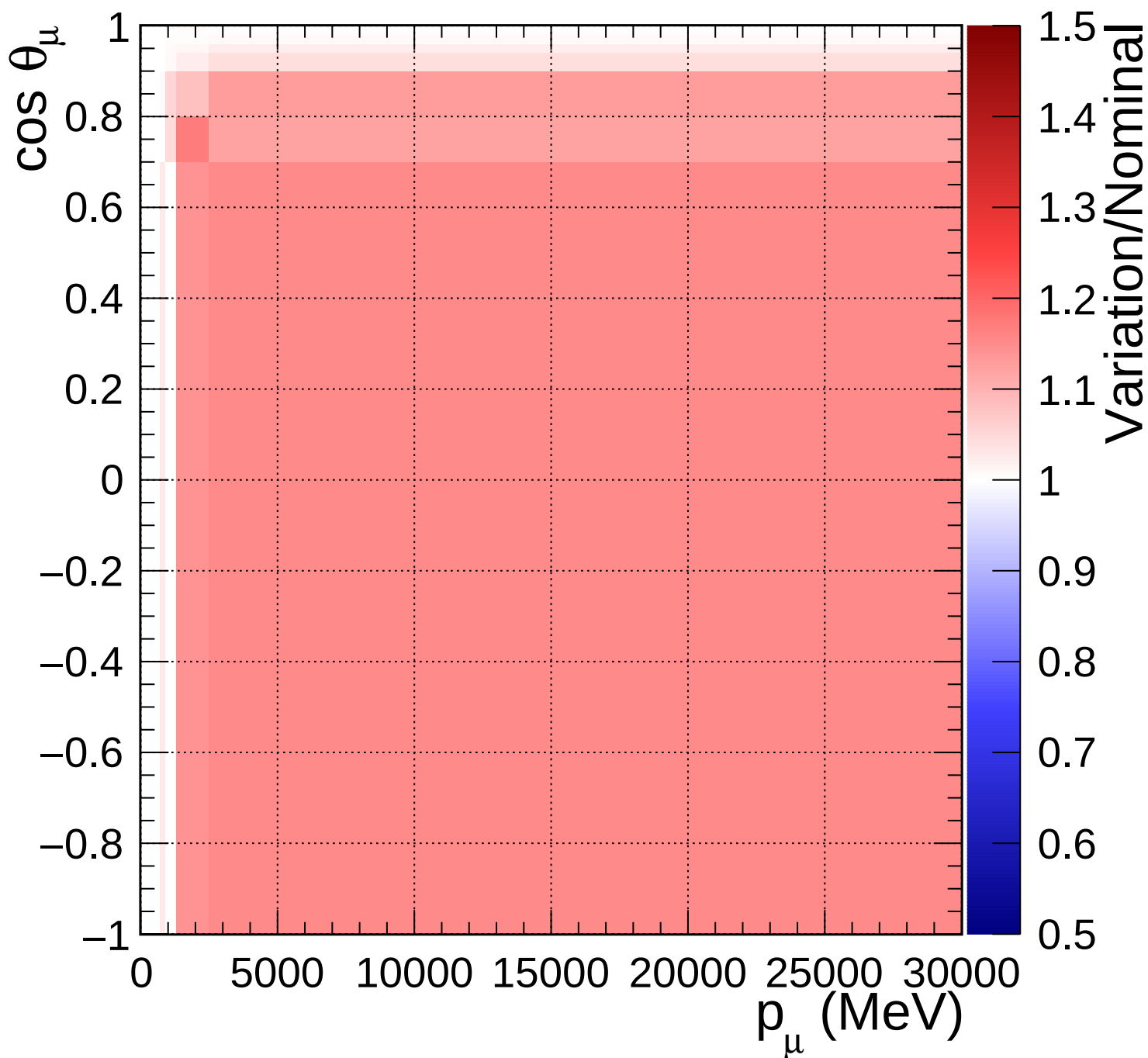
FGD2_anti-numuCC_1pi_Q2_norm_7_2.2
