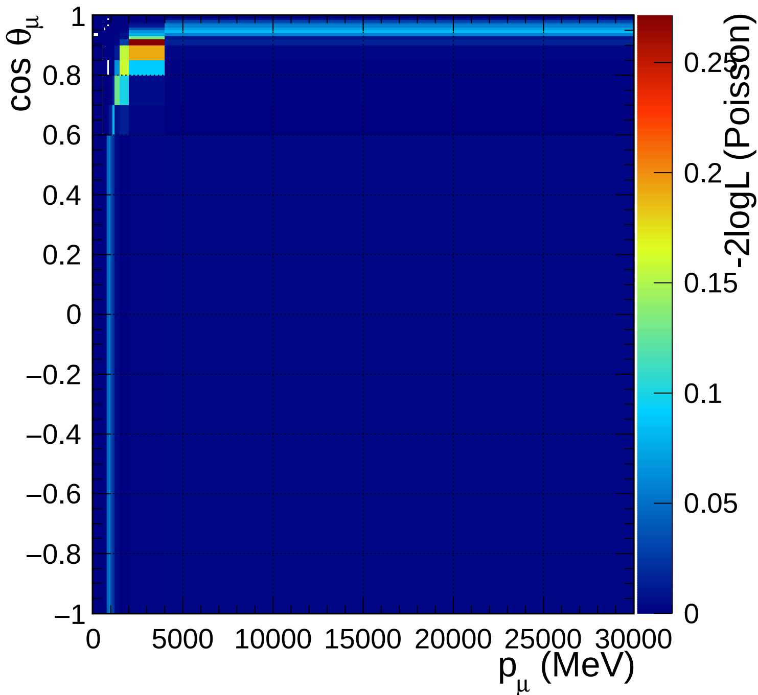
FGD1_anti-numuCC_0pi_Q2_norm_7_-0.2
