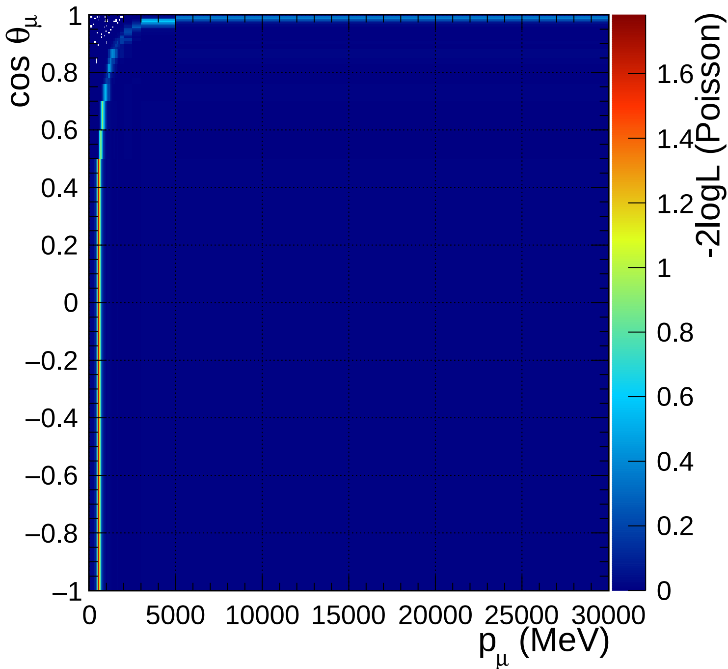
FGD1_numuCC_0pi_Q2_norm_6_1.54
