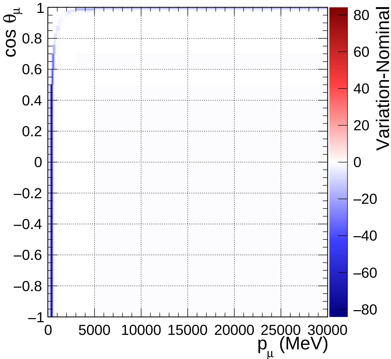
FGD1_numuCC_0pi_Q2_norm_5_0.67
