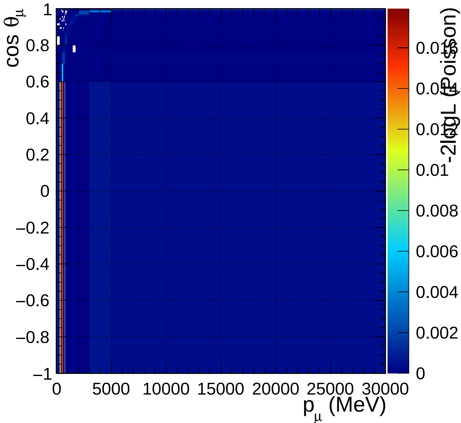
FGD1_numuCC_other_Q2_norm_5_1.33
