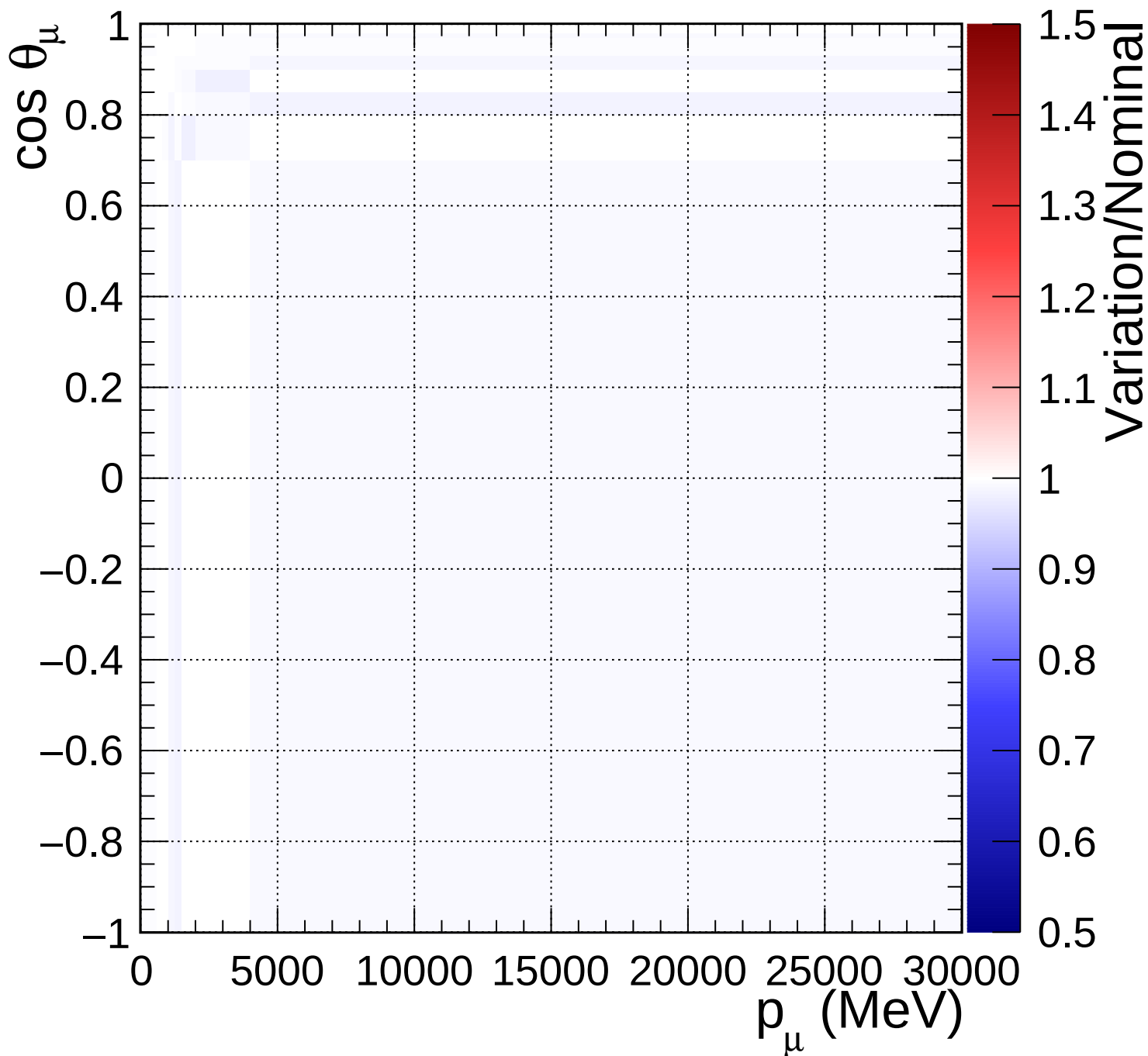
FGD2_anti-numuCC_other_Q2_norm_7_0.6
