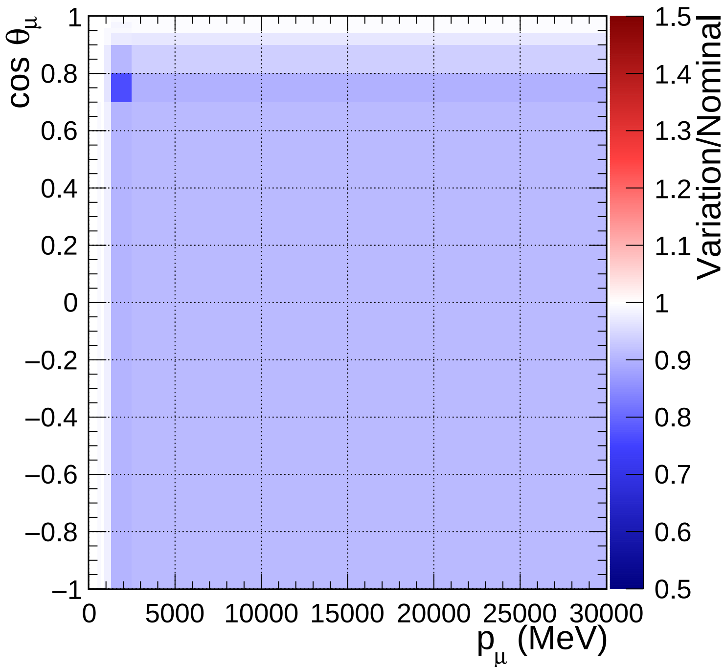
FGD1_anti-numuCC_1pi_Q2_norm_7_-0.2
