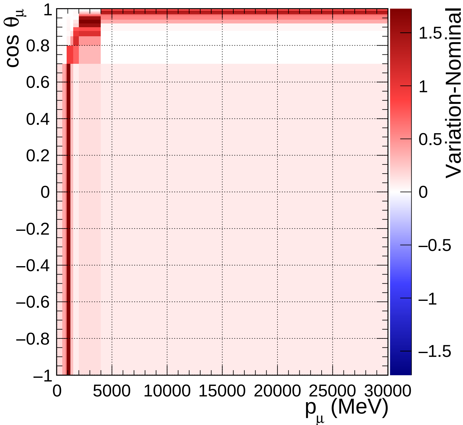
FGD1_NuMuBkg_CC0pi_in_AntiNu_Mode_Q2_norm_7_1.4
