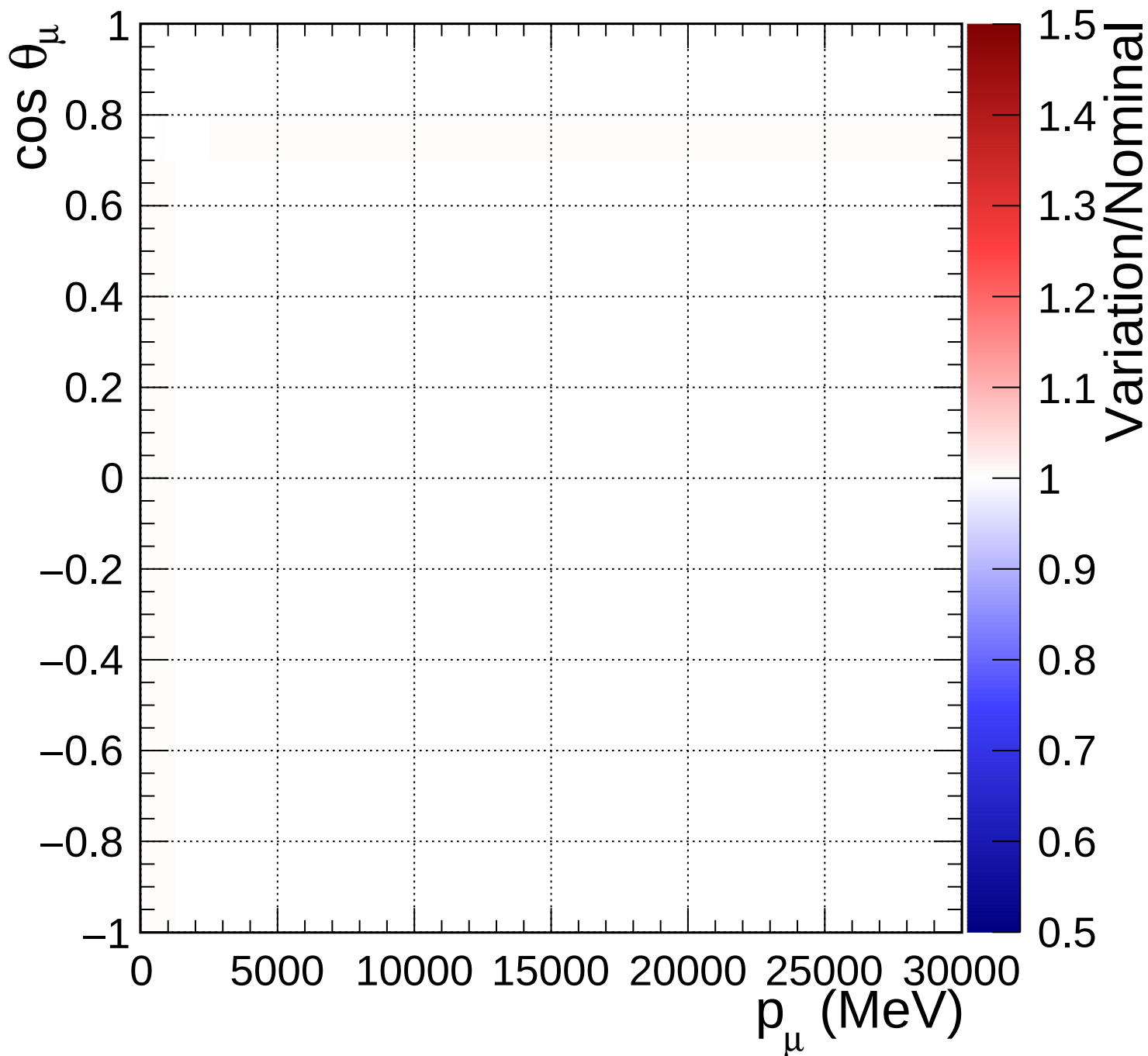
FGD2_anti-numuCC_1pi_Q2_norm_5_1.11
