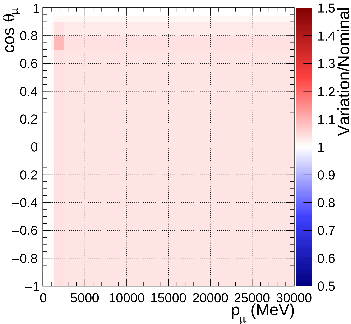
FGD1_anti-numuCC_1pi_Q2_norm_7_1.4
