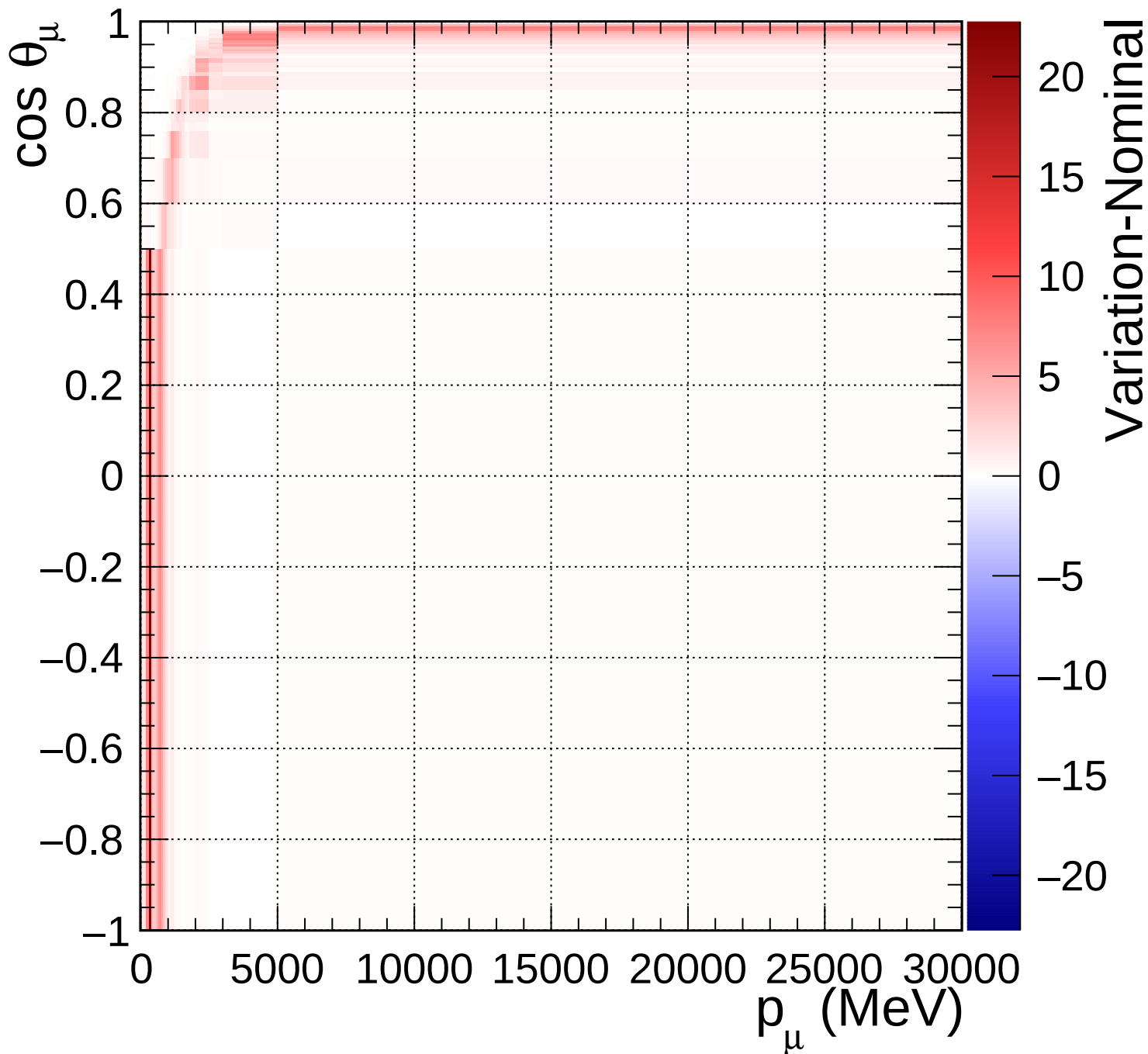
FGD2_numuCC_0pi_Q2_norm_7_2.2
