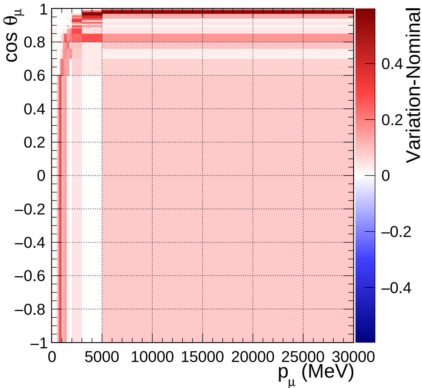
FGD1_numuCC_other_Q2_norm_7_1.4
