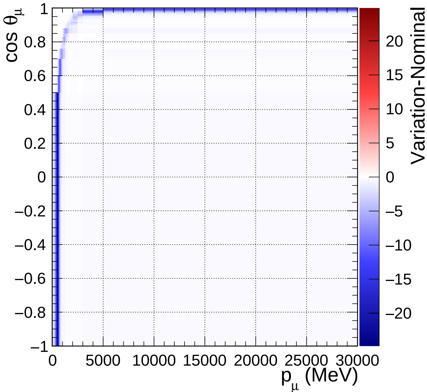
FGD1_numuCC_0pi_Q2_norm_6_0.46
