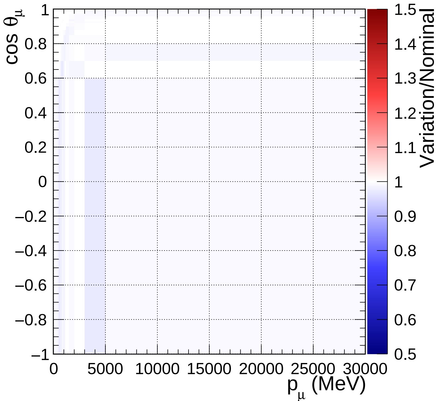
FGD2_numuCC_1pi_Q2_norm_6_0.46
