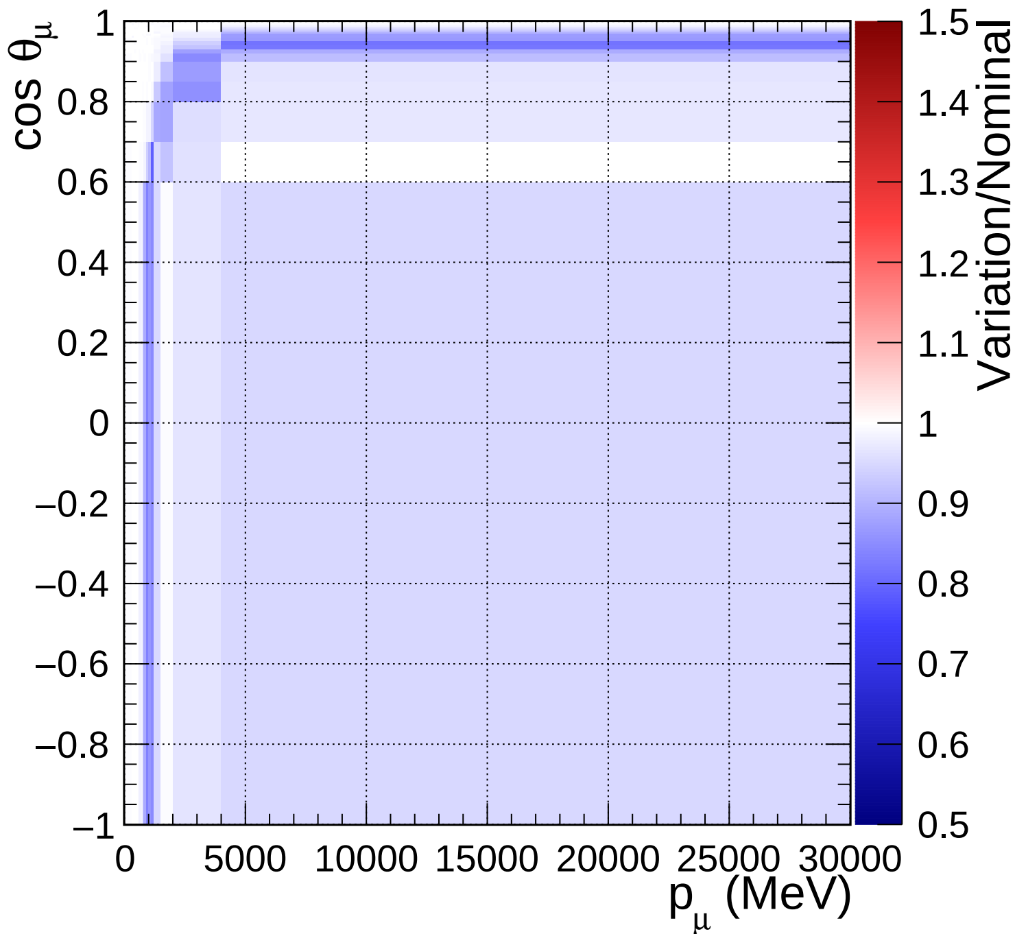
FGD1_anti-numuCC_0pi_Q2_norm_7_-0.2
