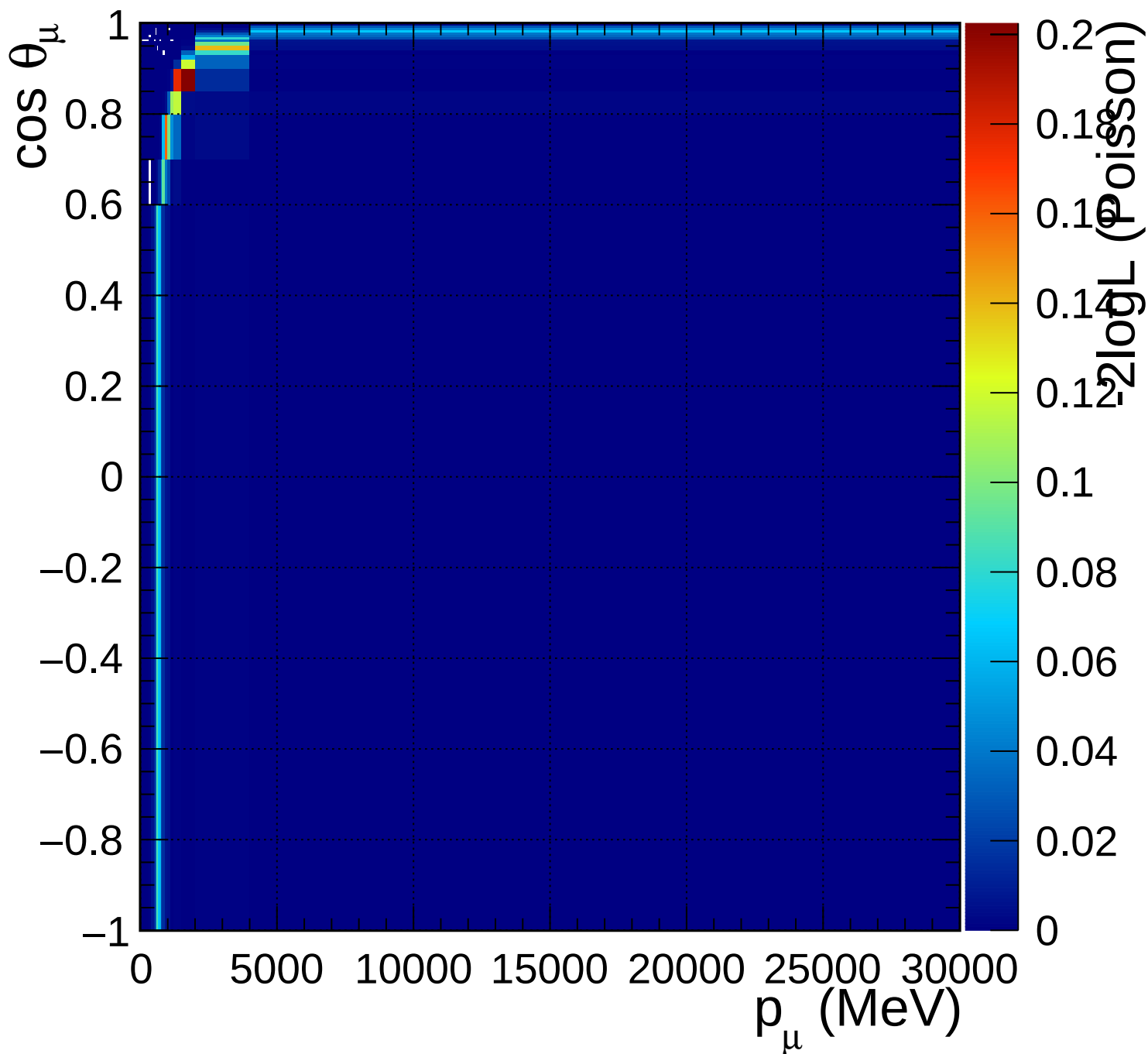
FGD1_anti-numuCC_0pi_Q2_norm_6_1.54
