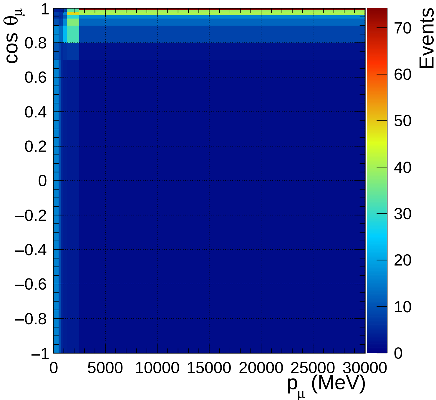
FGD1_anti-numuCC_1pi_Q2_norm_7_1
