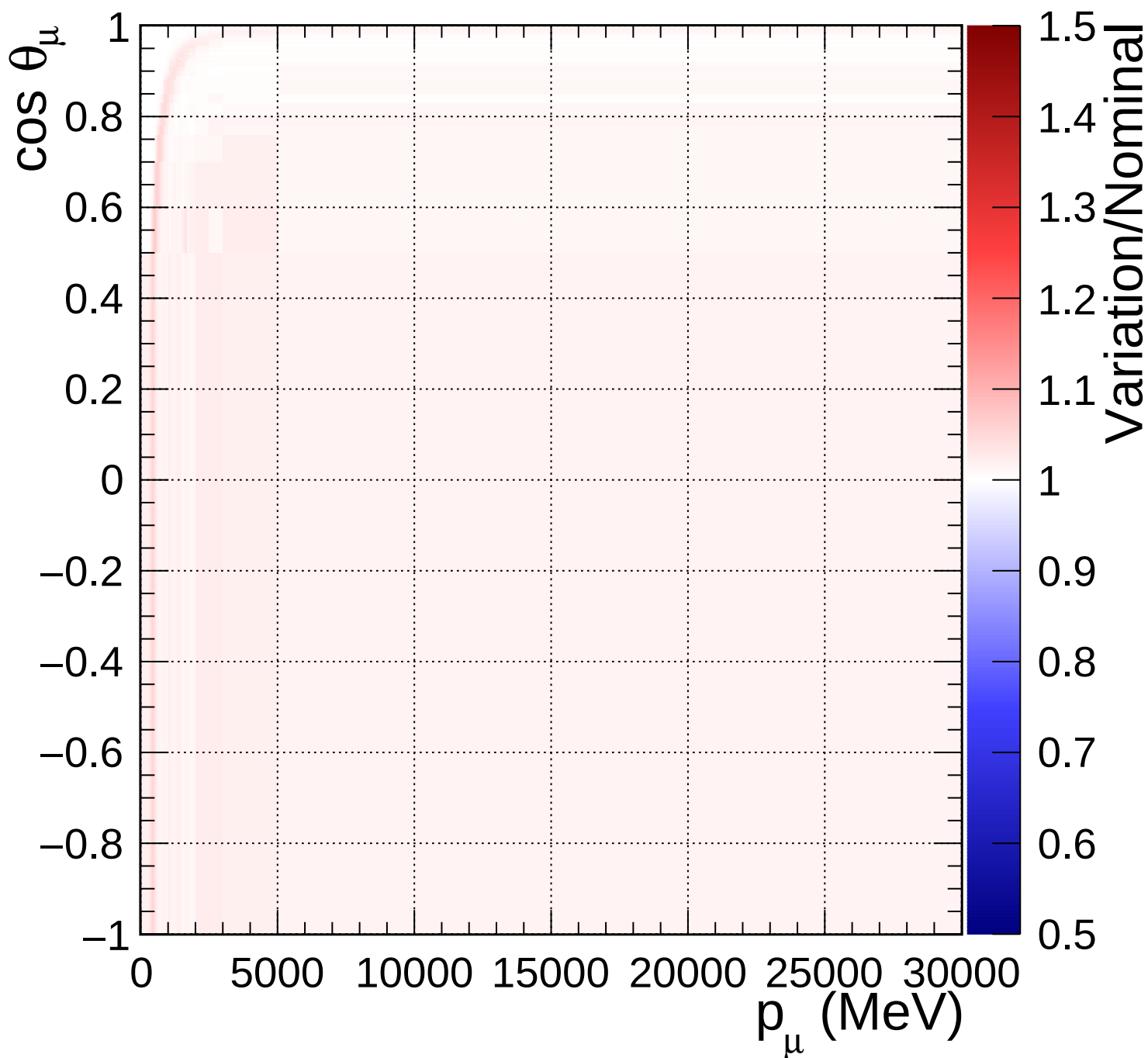
FGD2_numuCC_0pi_Q2_norm_5_1.11
