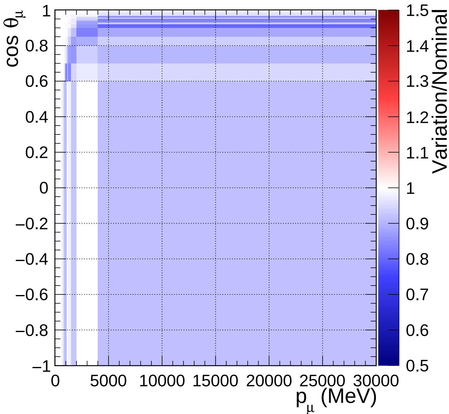
FGD2_anti-numuCC_0pi_Q2_norm_7_-0.2
