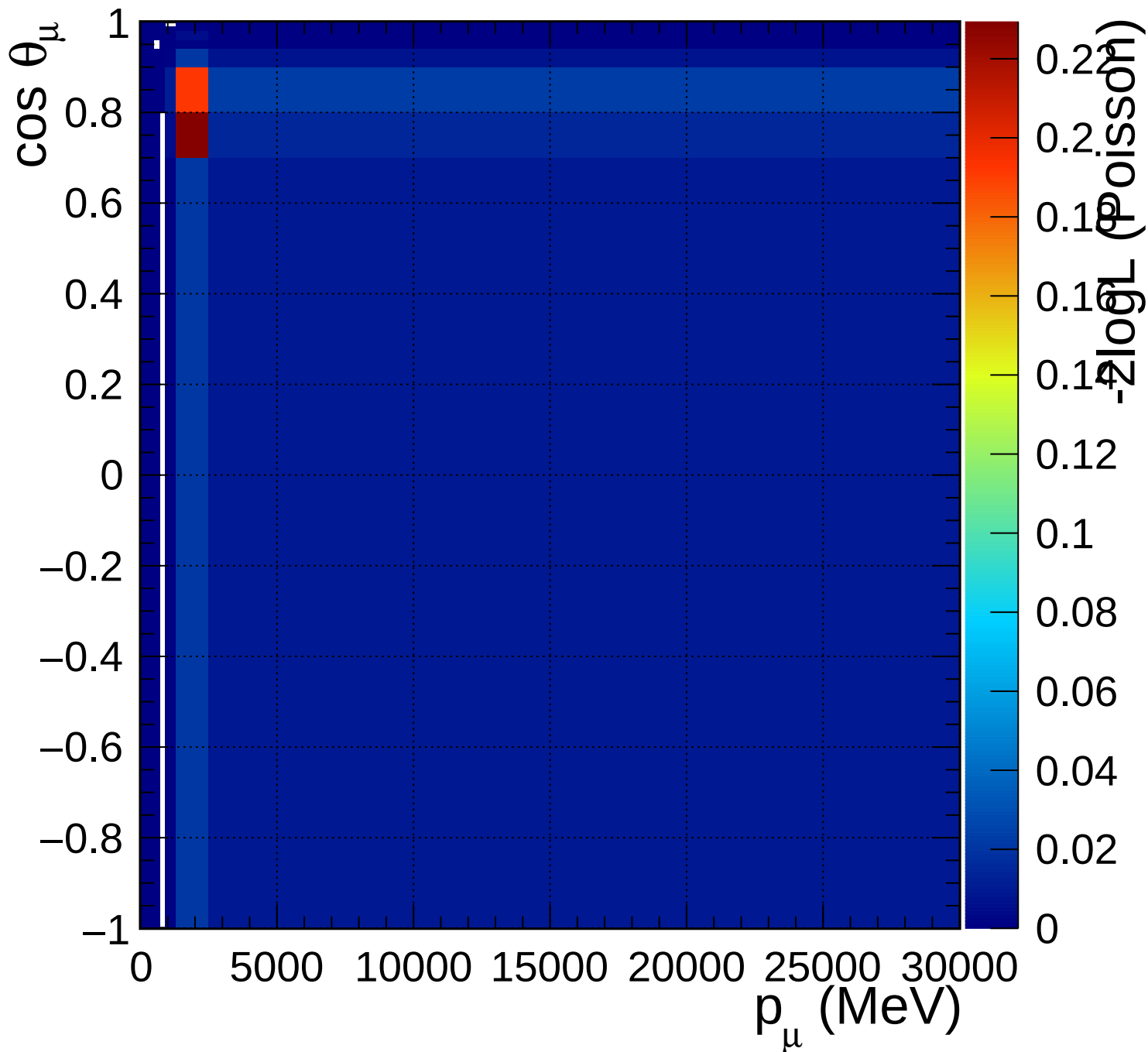
FGD1_anti-numuCC_1pi_Q2_norm_7_2.2
