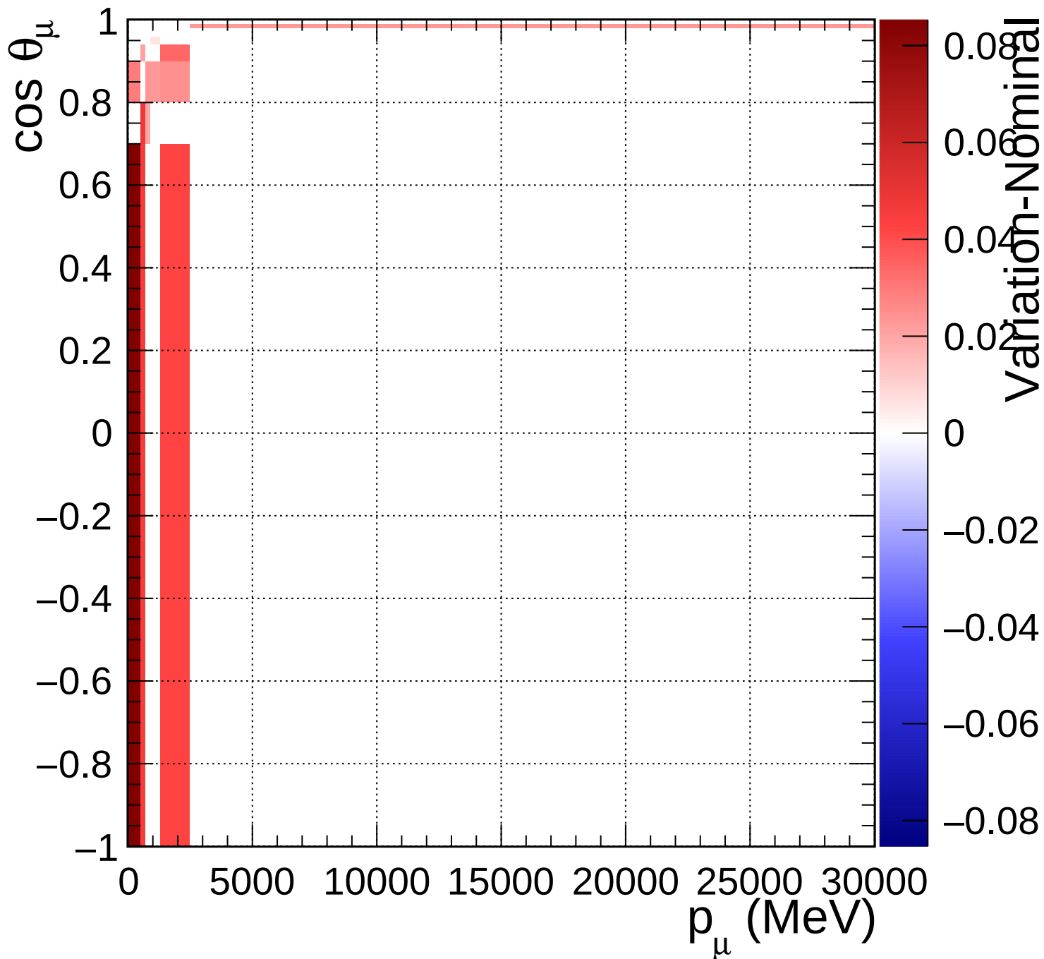
FGD1_anti-numuCC_1pi_Q2_norm_5_1.33
