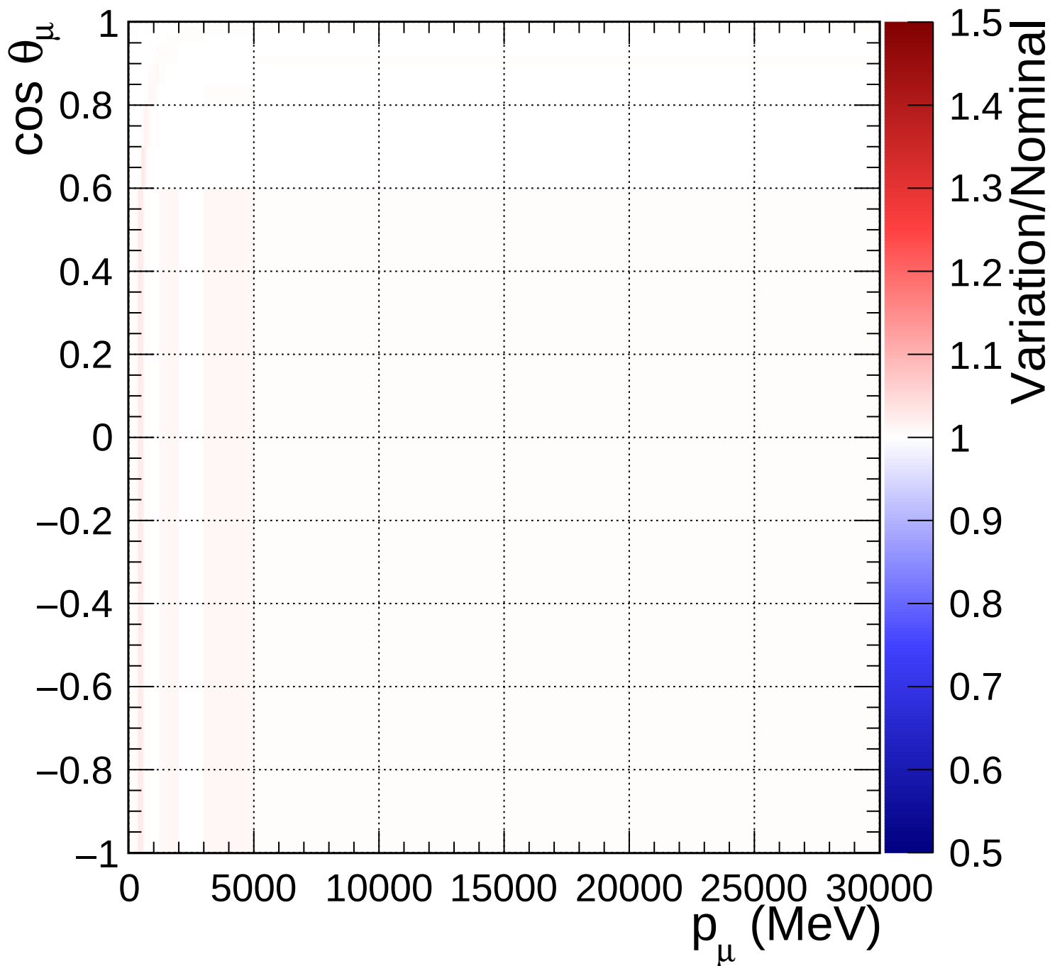
FGD1_numuCC_1pi_Q2_norm_5_1.33
