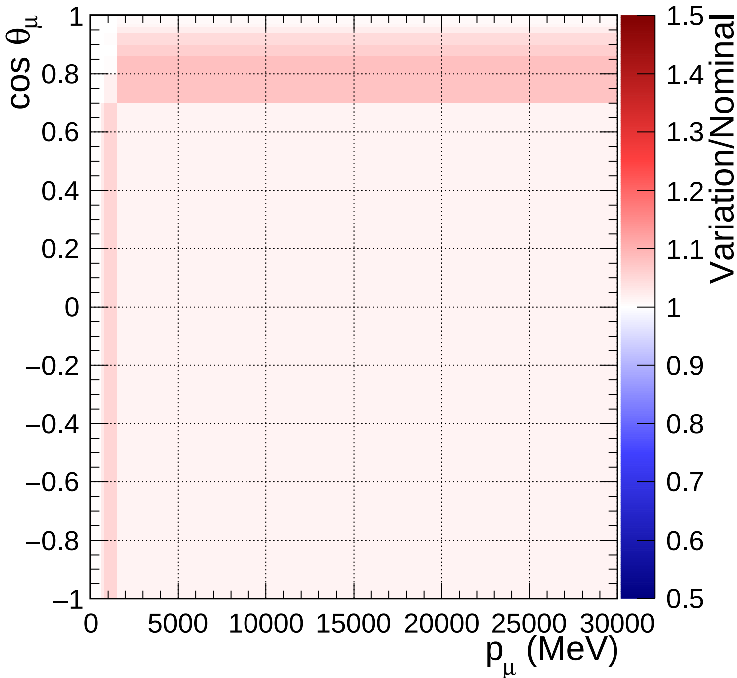
FGD2_NuMuBkg_CC1pi_in_AntiNu_Mode_Q2_norm_7_2.2
