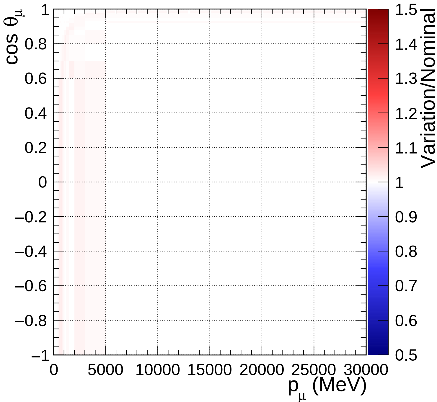
FGD1_numuCC_1pi_Q2_norm_6_1.54
