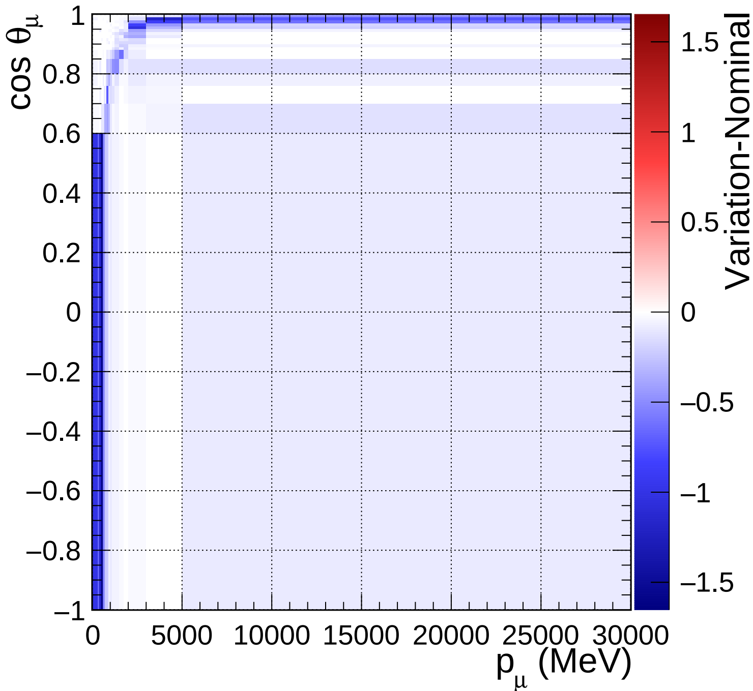
FGD2_numuCC_other_Q2_norm_6_0.46
