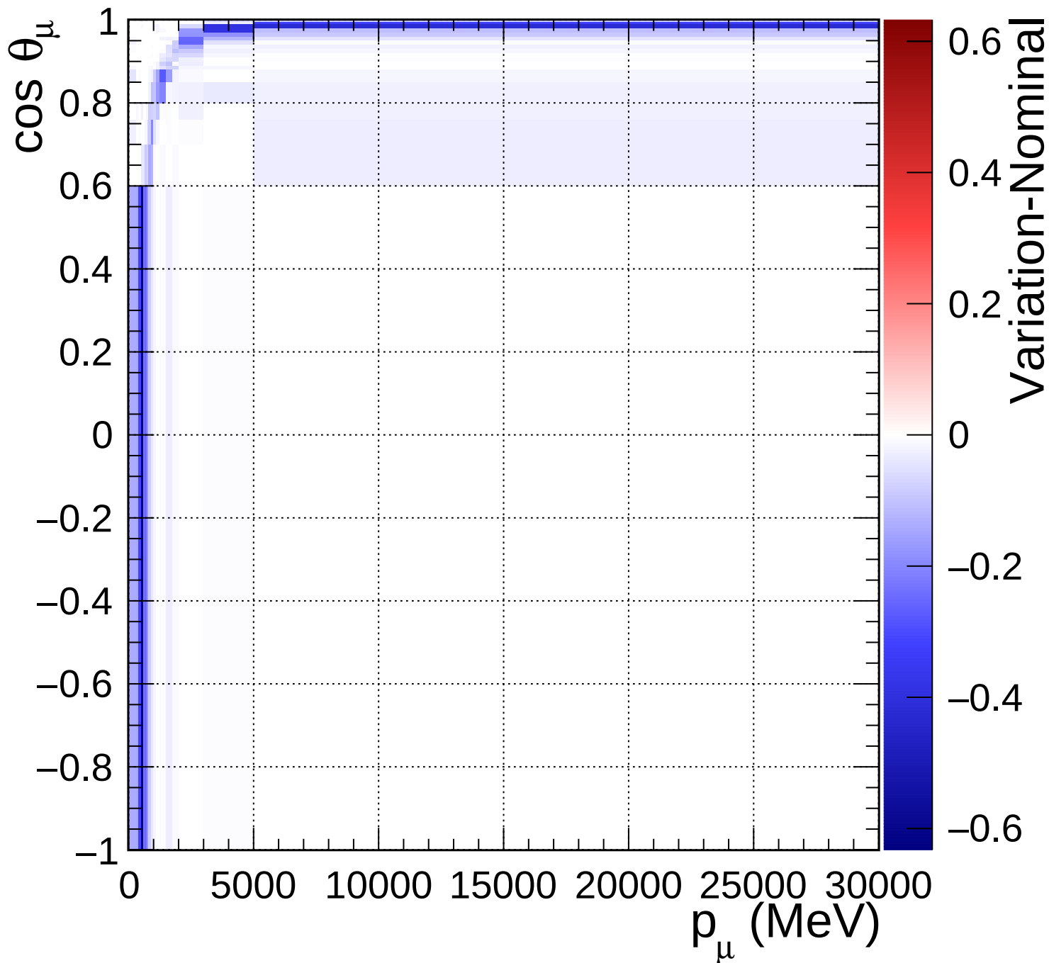
FGD1_numuCC_other_Q2_norm_6_0.82
