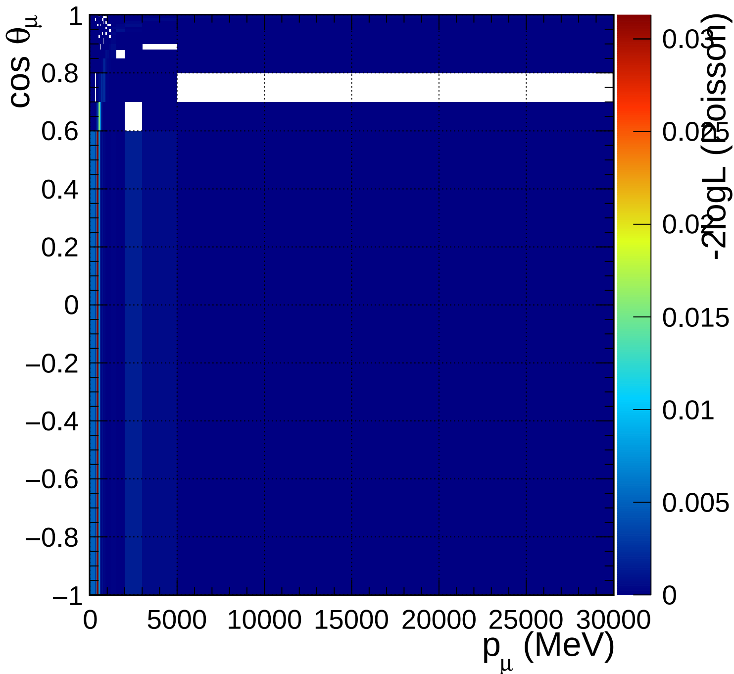
FGD2_numuCC_1pi_Q2_norm_5_1.33
