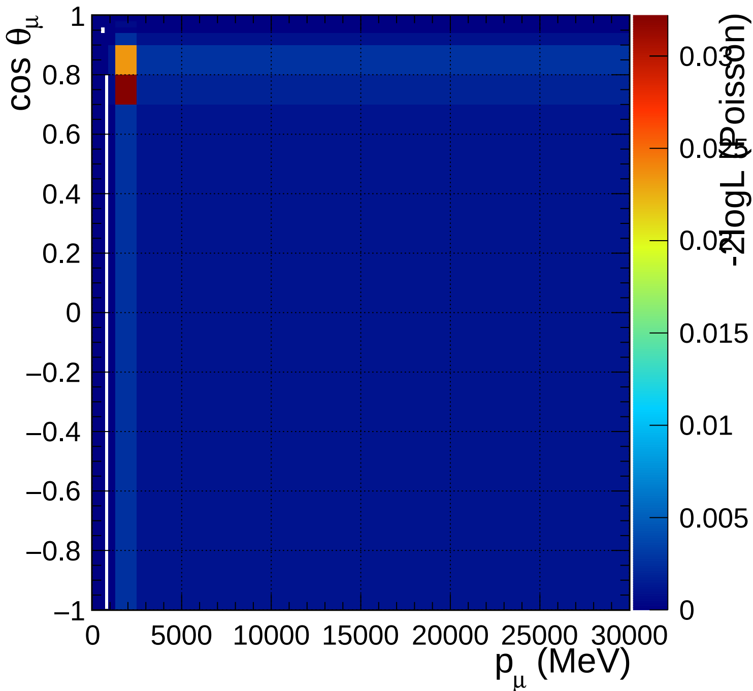
FGD1_anti-numuCC_1pi_Q2_norm_7_0.6
