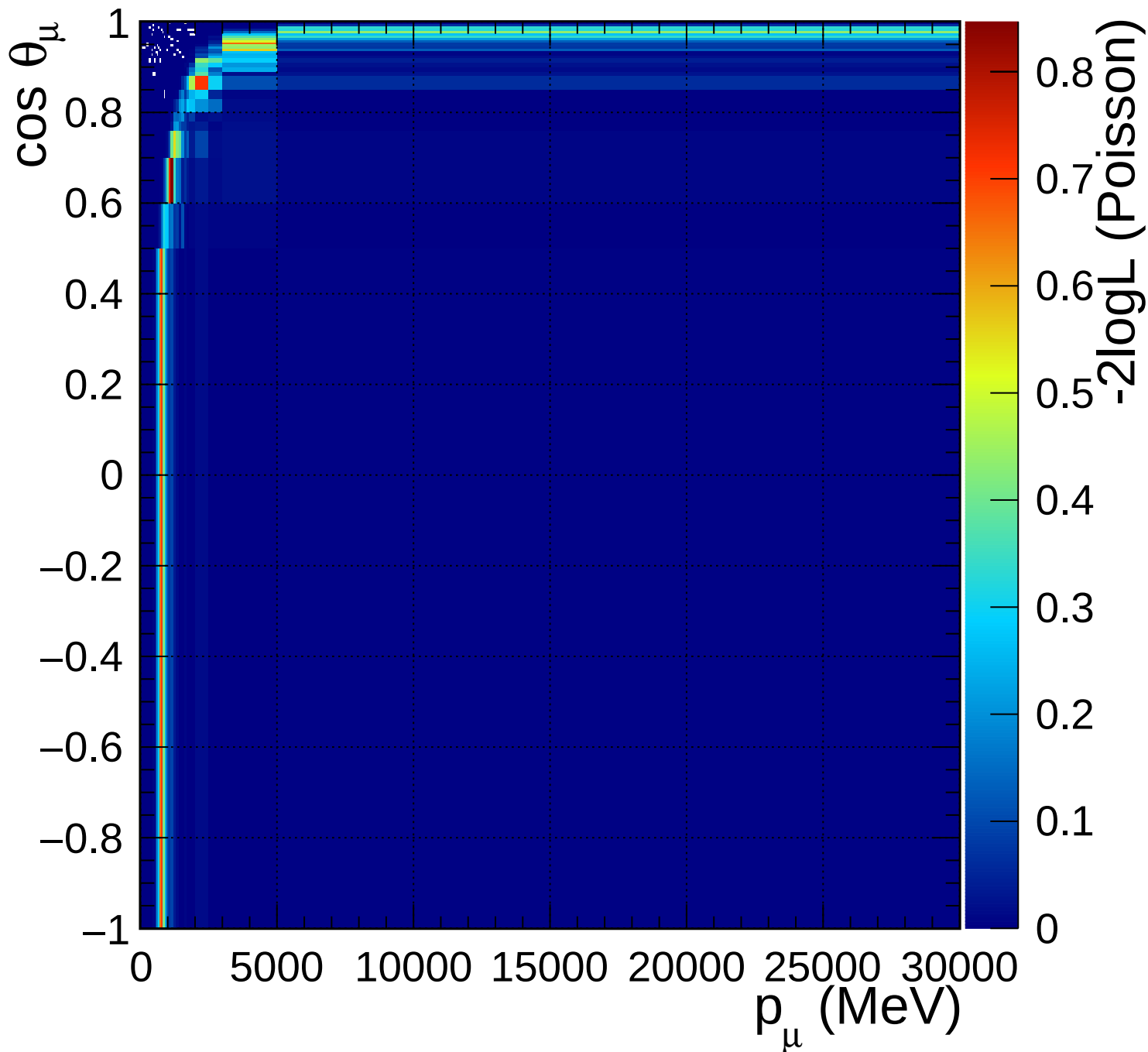
FGD1_numuCC_0pi_Q2_norm_7_2.2
