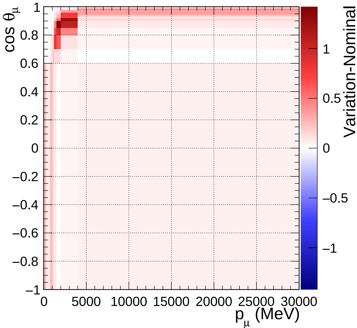
FGD1_anti-numuCC_0pi_Q2_norm_7_1.4
