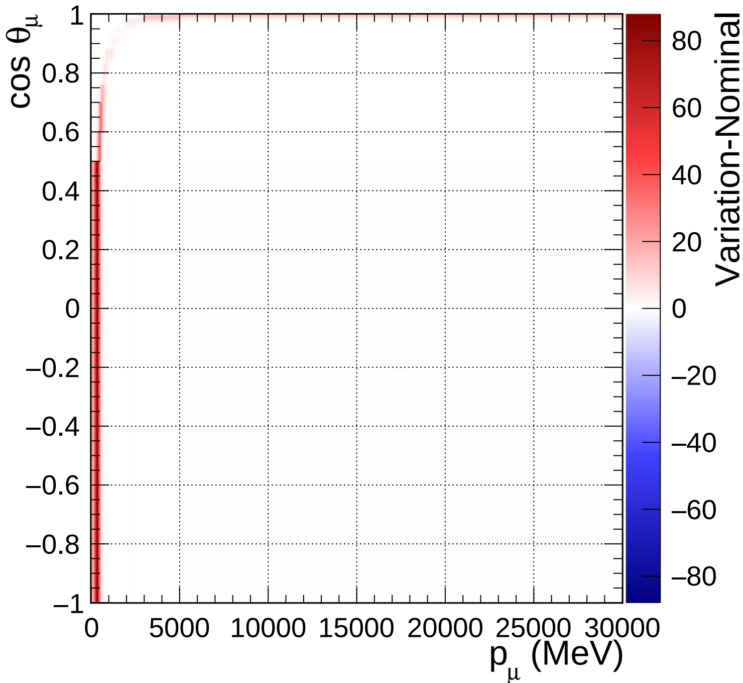
FGD2_numuCC_0pi_Q2_norm_5_1.33
