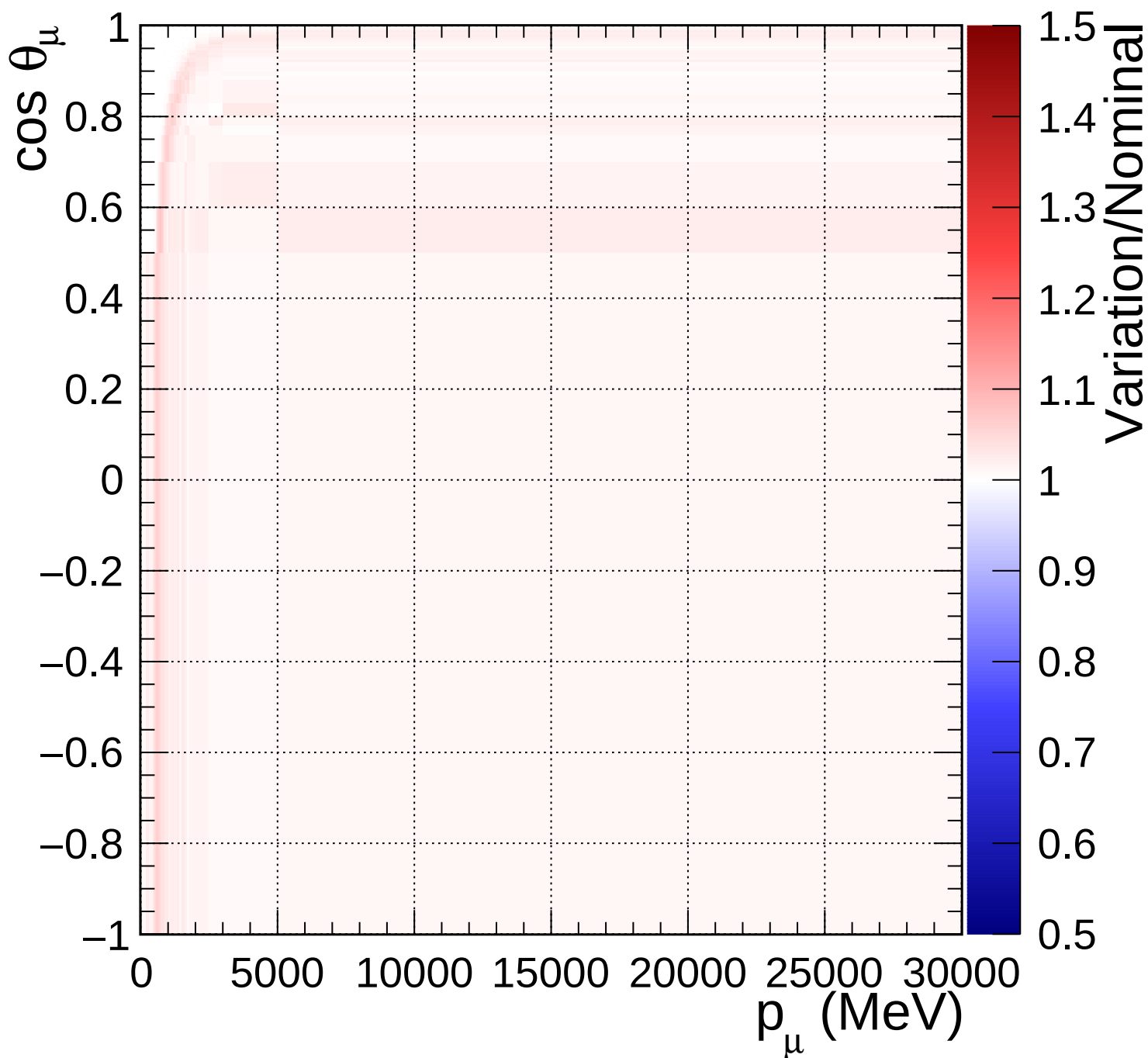
FGD2_numuCC_0pi_Q2_norm_6_1.18
