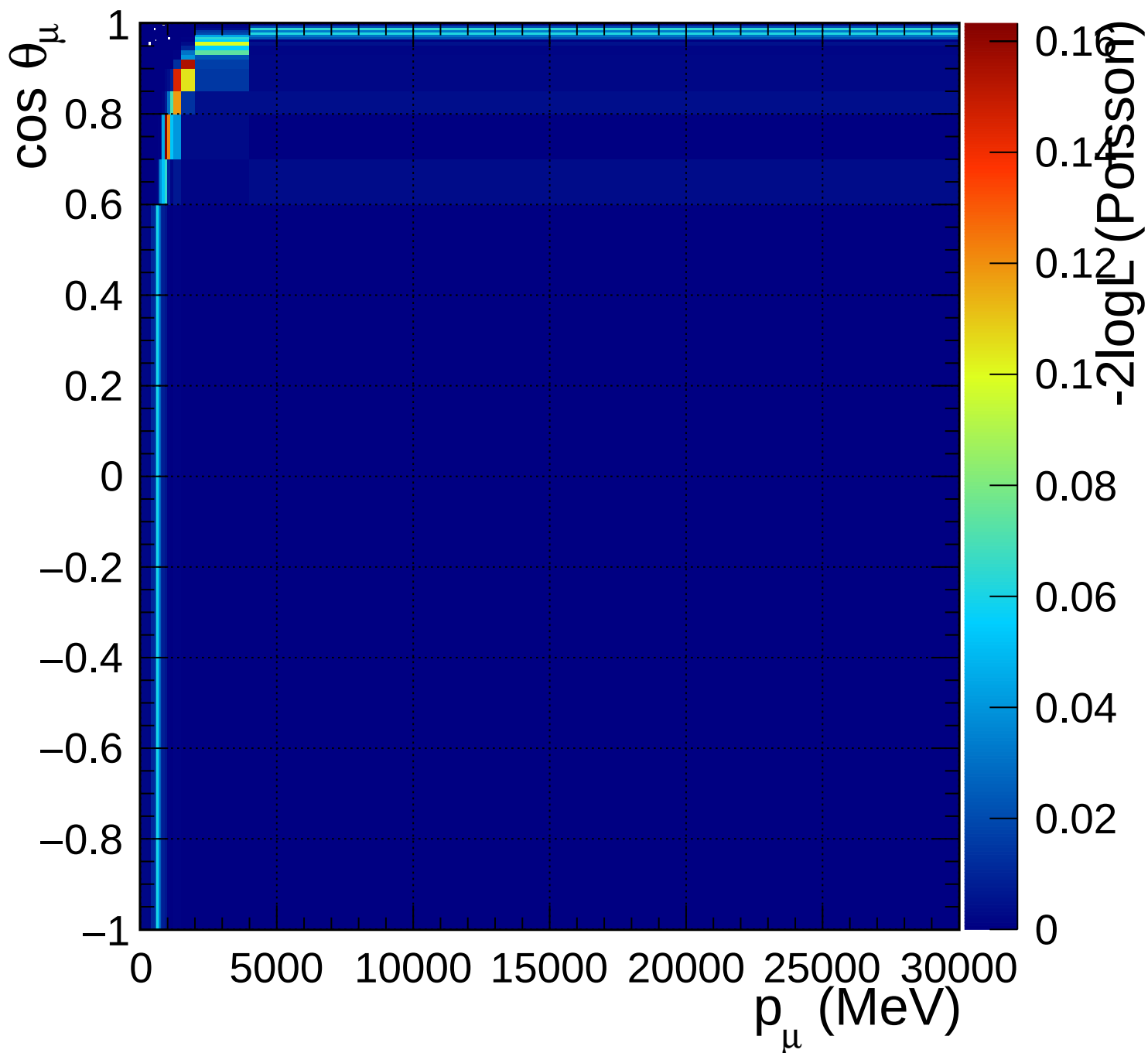
FGD2_anti-numuCC_0pi_Q2_norm_6_1.54
