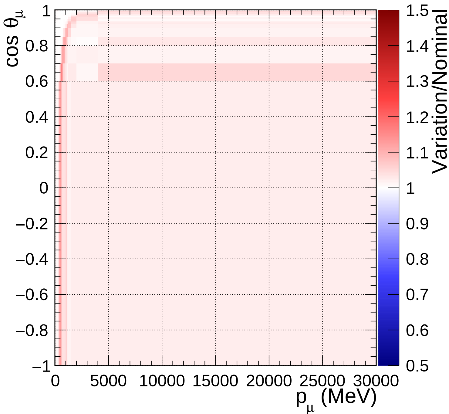
FGD2_anti-numuCC_0pi_Q2_norm_5_1.33
