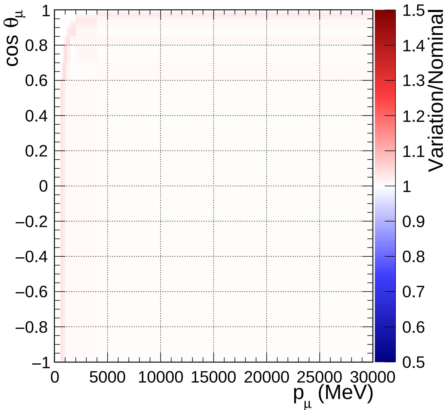
FGD1_anti-numuCC_0pi_Q2_norm_6_1.18
