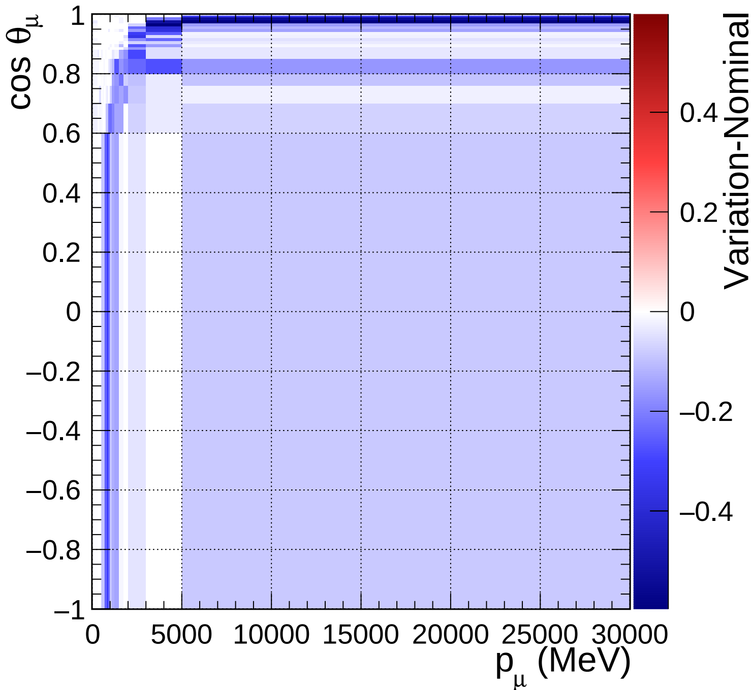
FGD1_numuCC_other_Q2_norm_7_0.6
