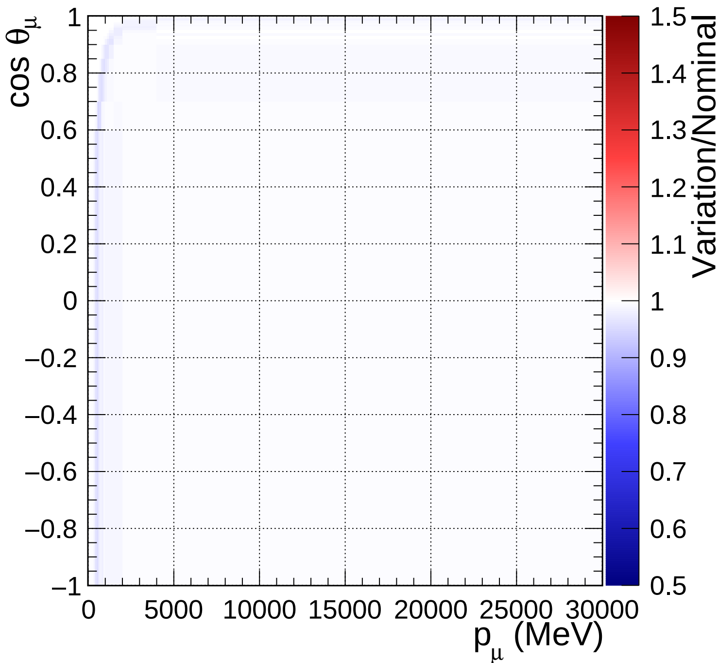
FGD1_anti-numuCC_0pi_Q2_norm_5_0.89
