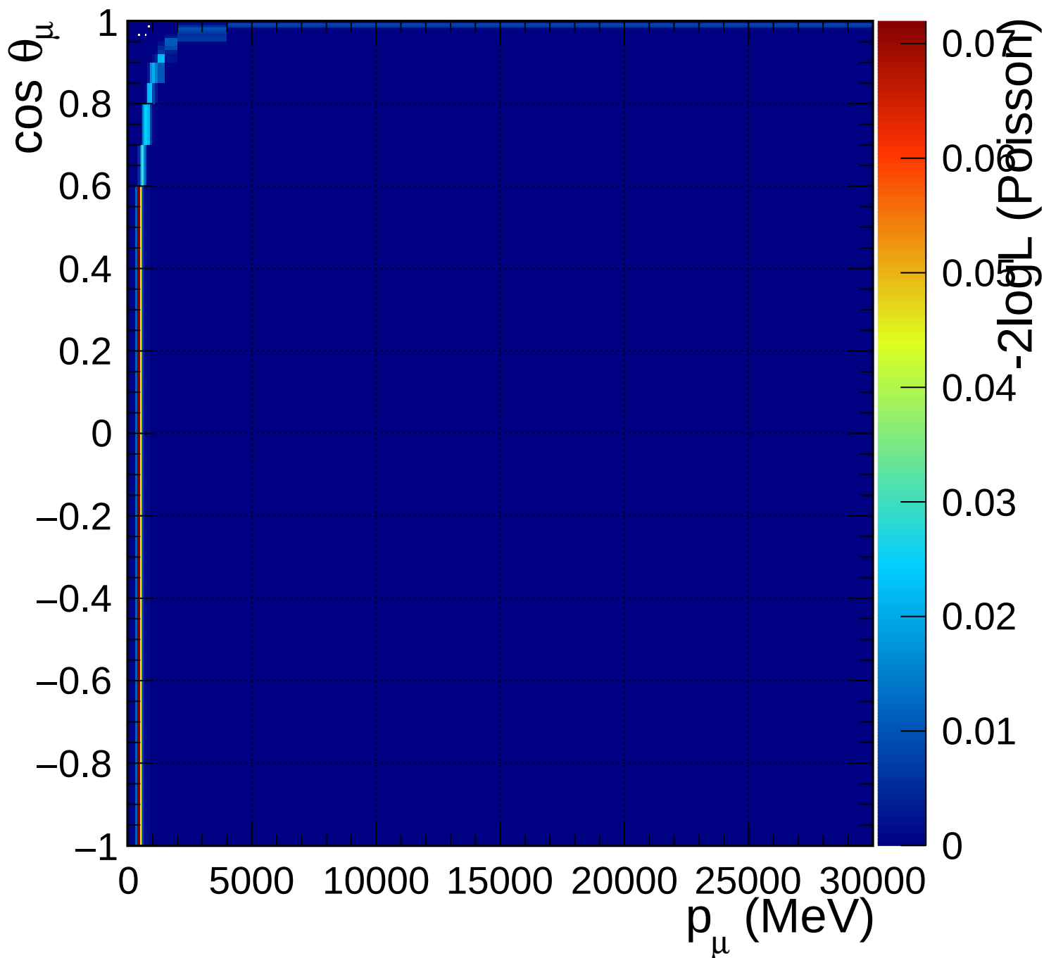
FGD1_anti-numuCC_0pi_Q2_norm_5_1.11
