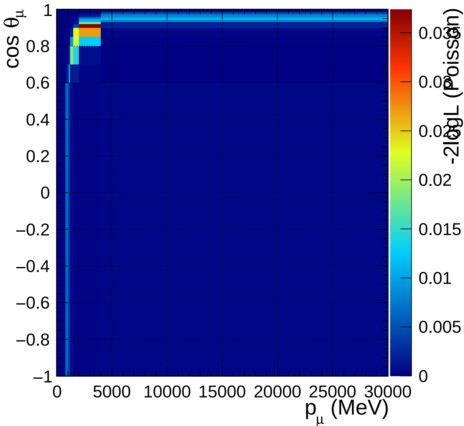
FGD1_anti-numuCC_0pi_Q2_norm_7_1.4
