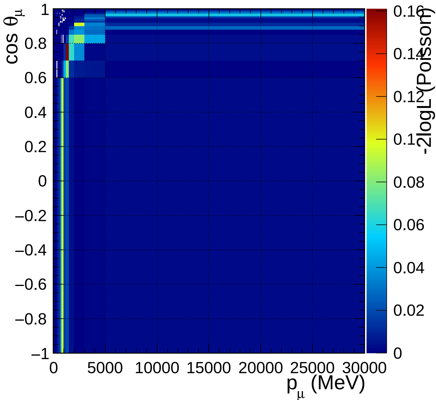
FGD2_numuCC_1pi_Q2_norm_7_-0.2
