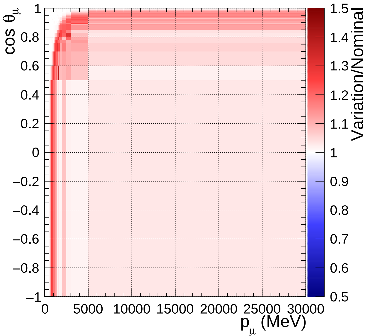
FGD1_numuCC_0pi_Q2_norm_7_2.2
