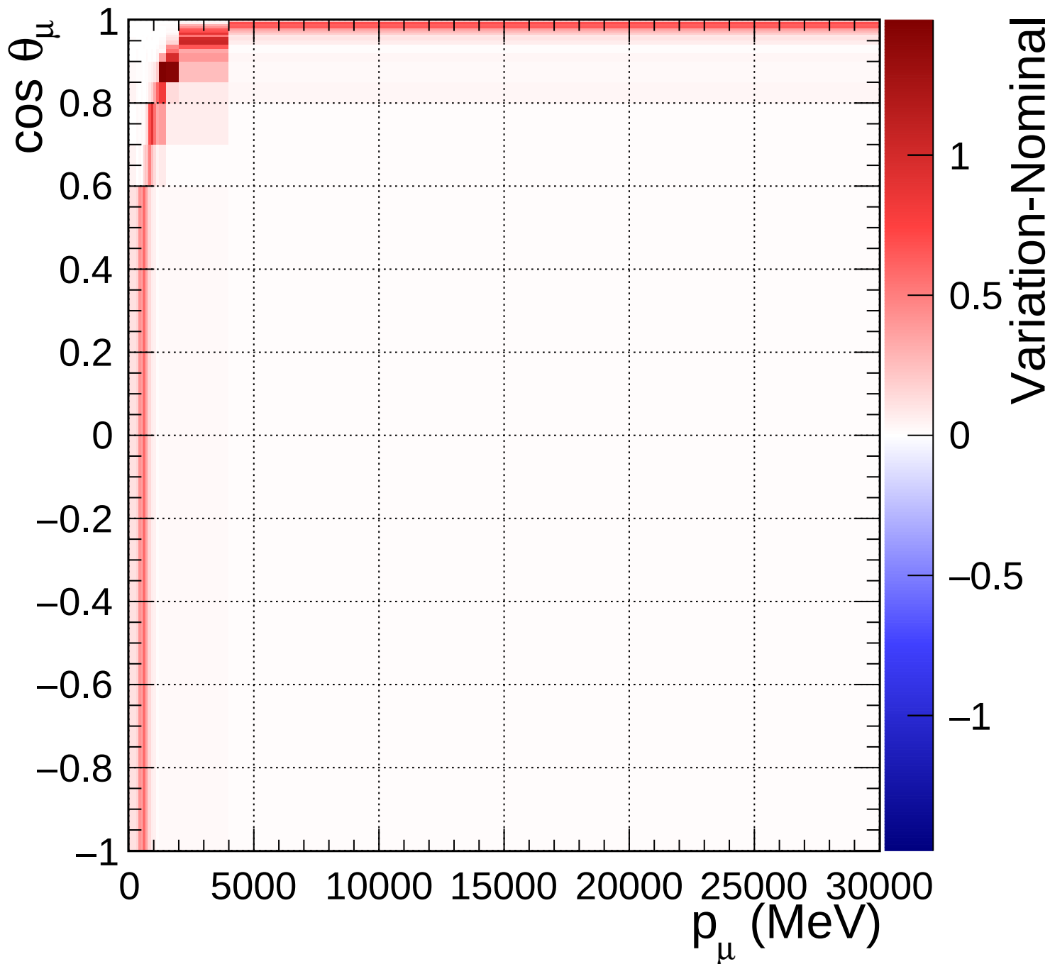
FGD1_anti-numuCC_0pi_Q2_norm_6_1.18
