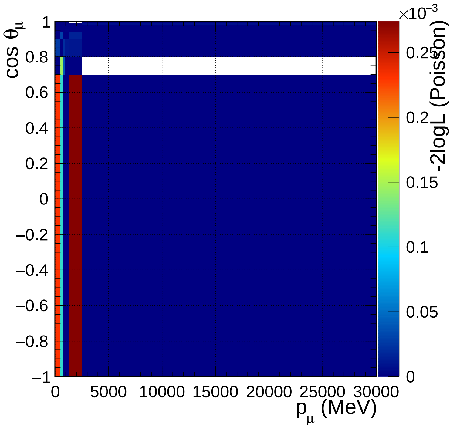
FGD1_anti-numuCC_1pi_Q2_norm_5_0.67
