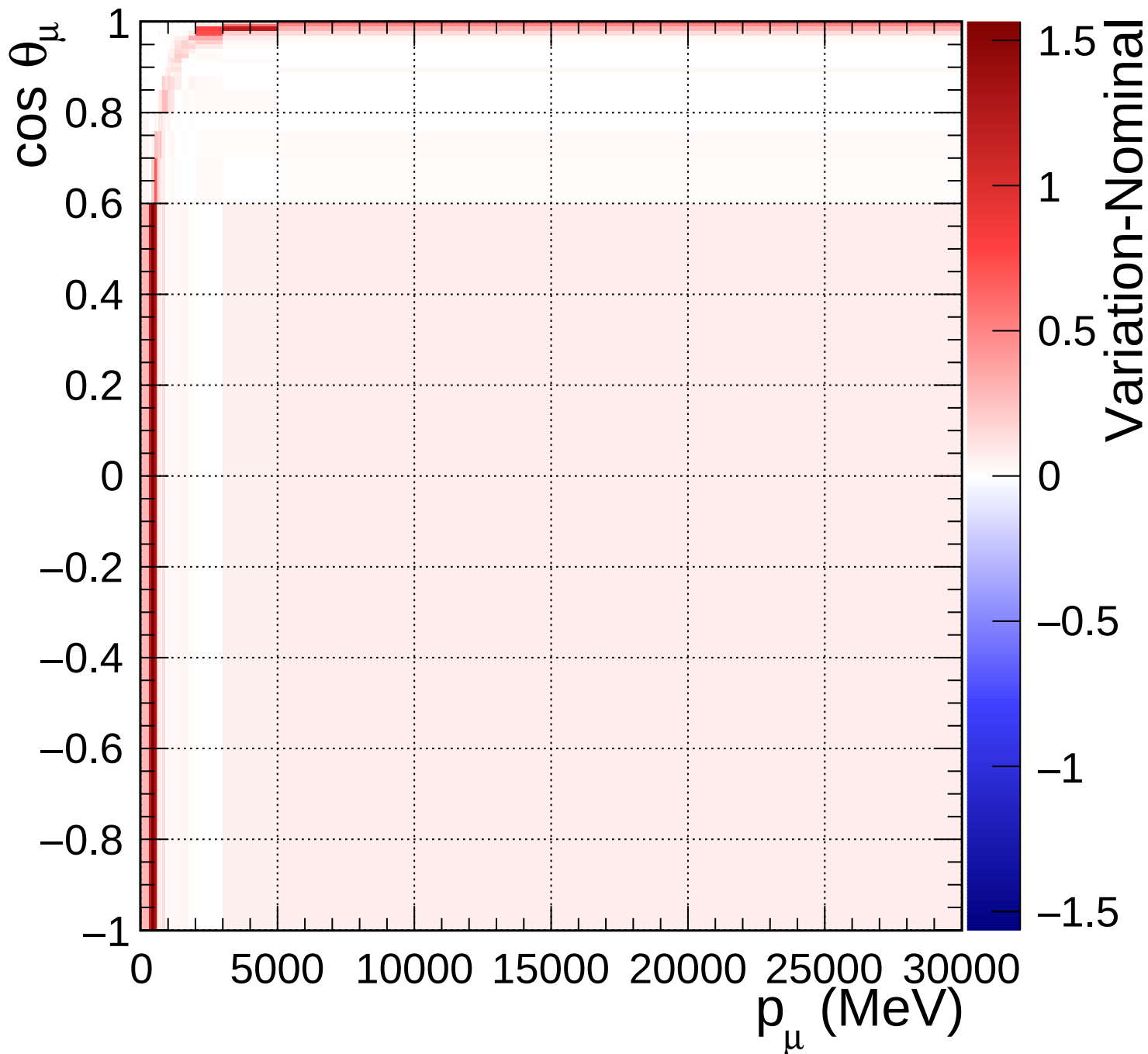
FGD1_numuCC_other_Q2_norm_5_1.33
