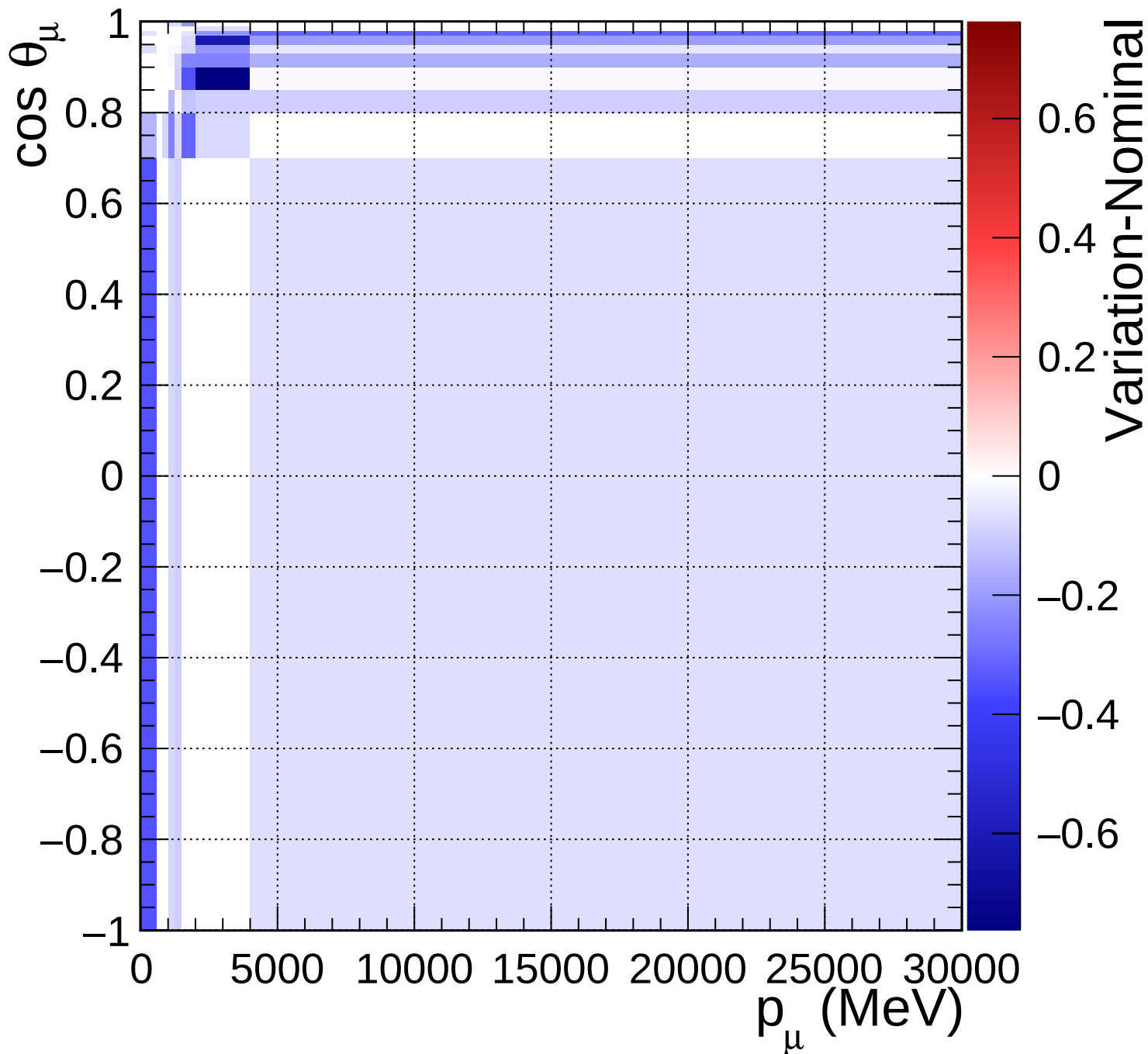
FGD2_anti-numuCC_other_Q2_norm_7_-0.2
