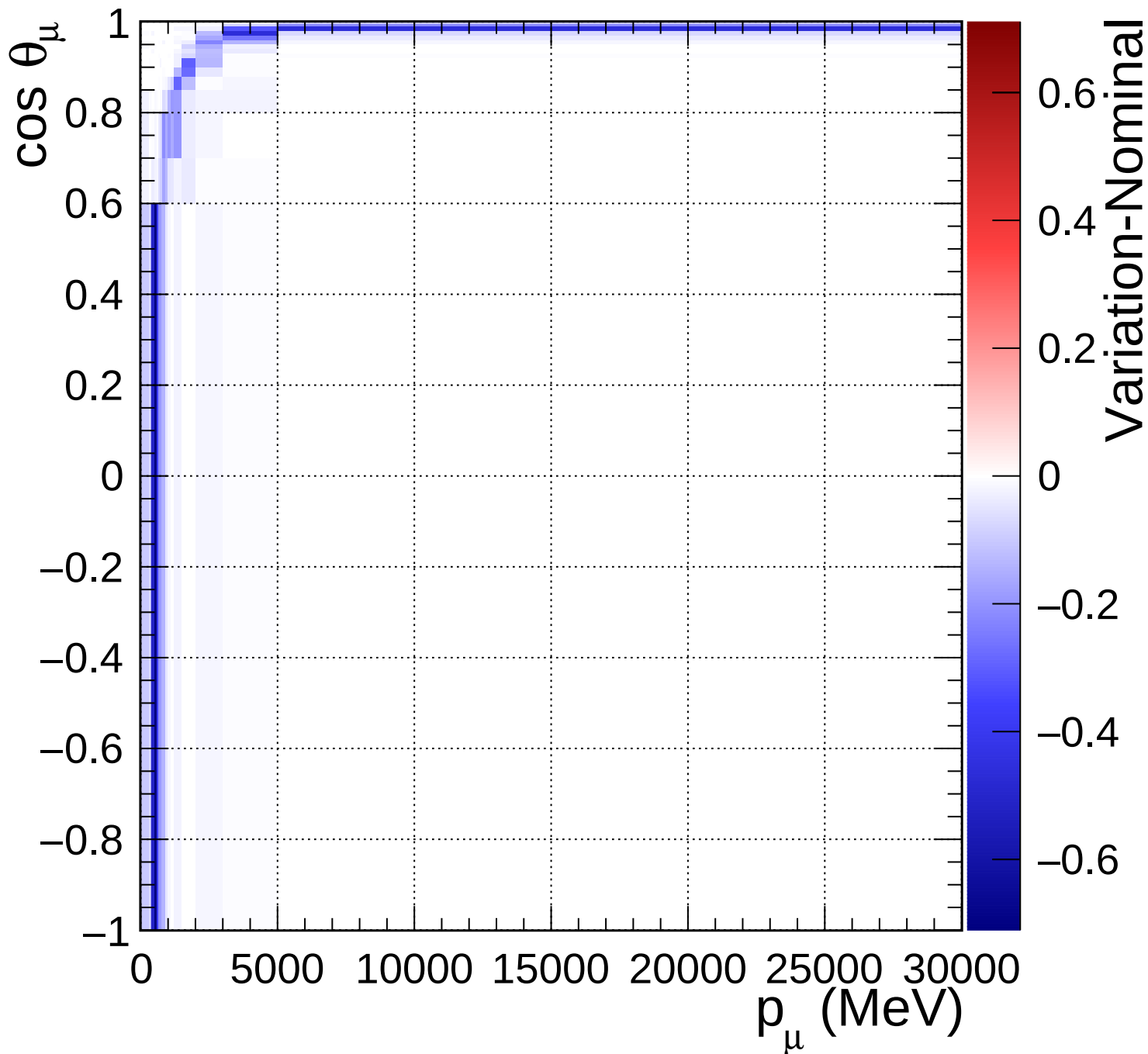
FGD1_numuCC_1pi_Q2_norm_6_0.82
