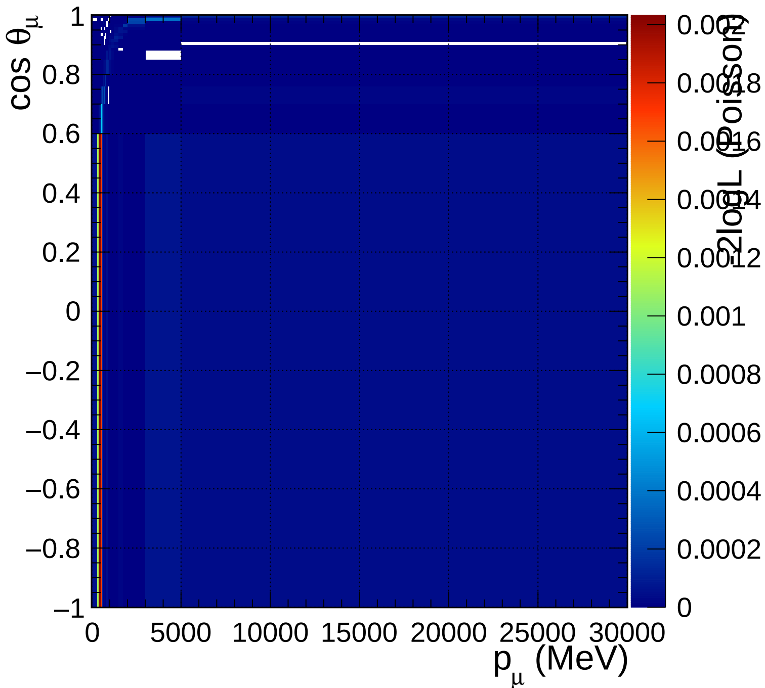
FGD1_numuCC_other_Q2_norm_5_0.89
