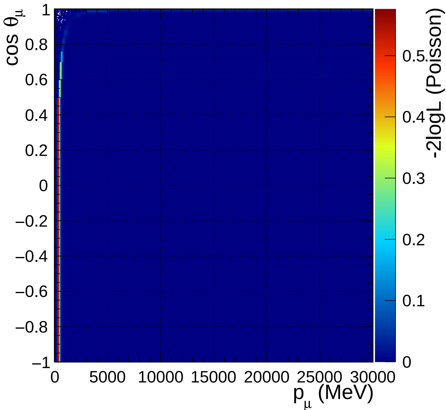
FGD1_numuCC_0pi_Q2_norm_5_1.11
