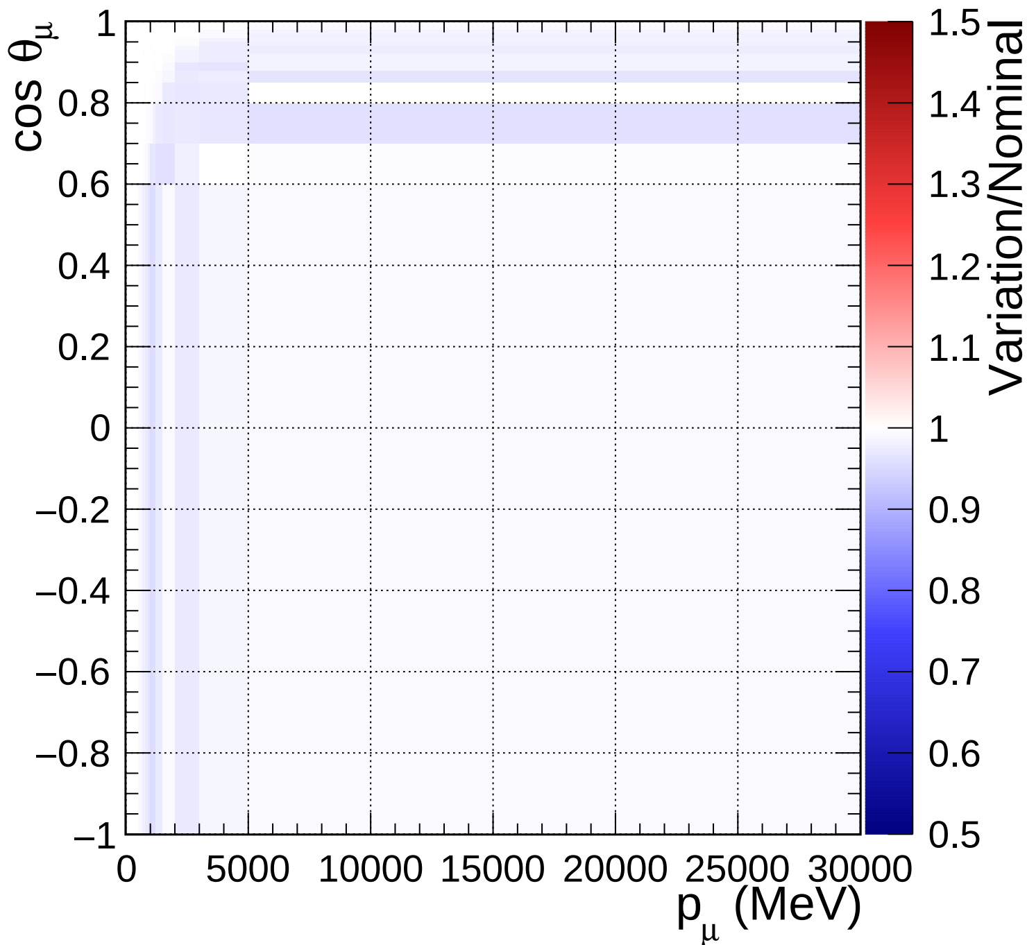
FGD1_numuCC_1pi_Q2_norm_7_0.6
