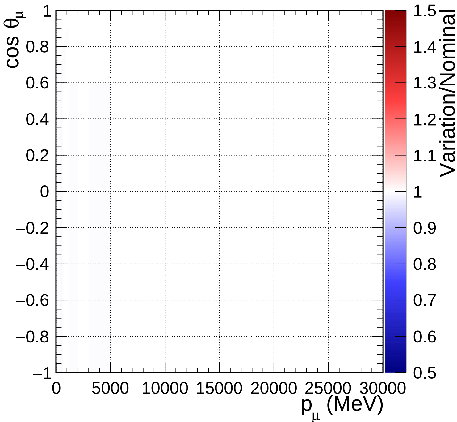
FGD1_numuCC_1pi_Q2_norm_5_0.89
