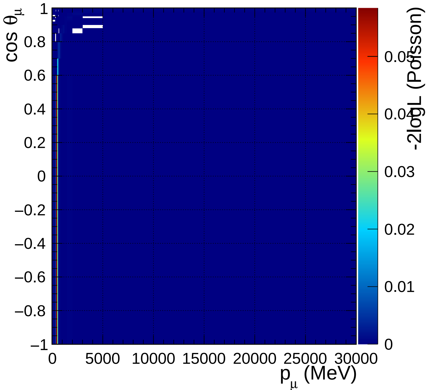
FGD1_numuCC_1pi_Q2_norm_5_1.33
