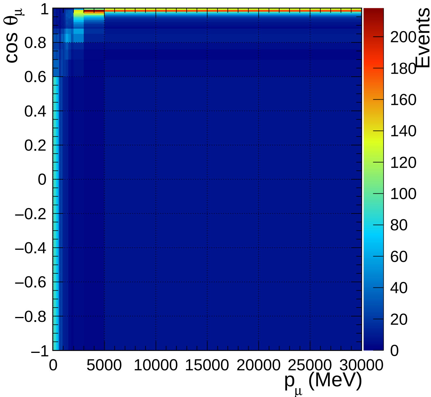
FGD1_numuCC_other_Q2_norm_7_1
