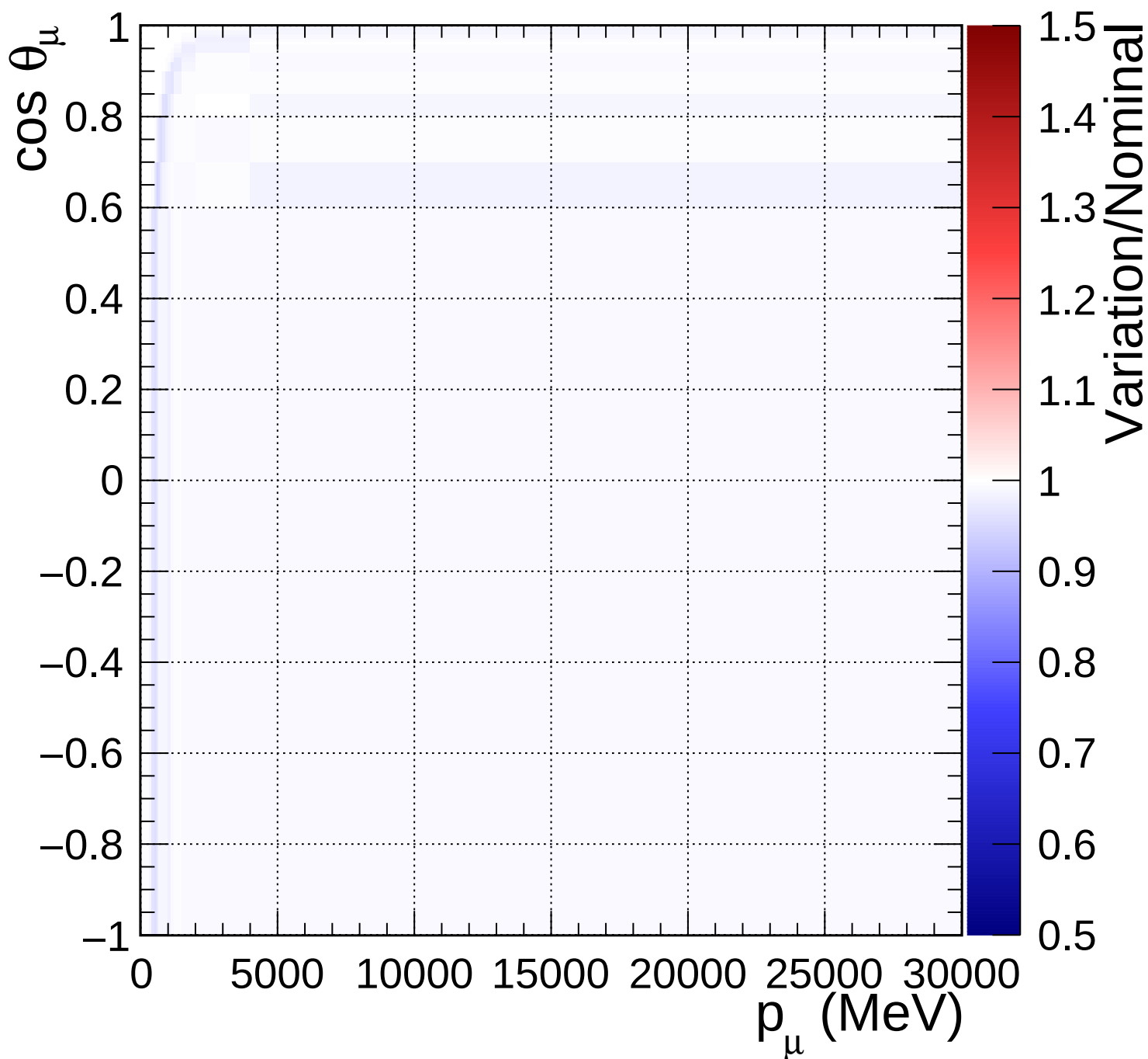
FGD2_anti-numuCC_0pi_Q2_norm_5_0.89
