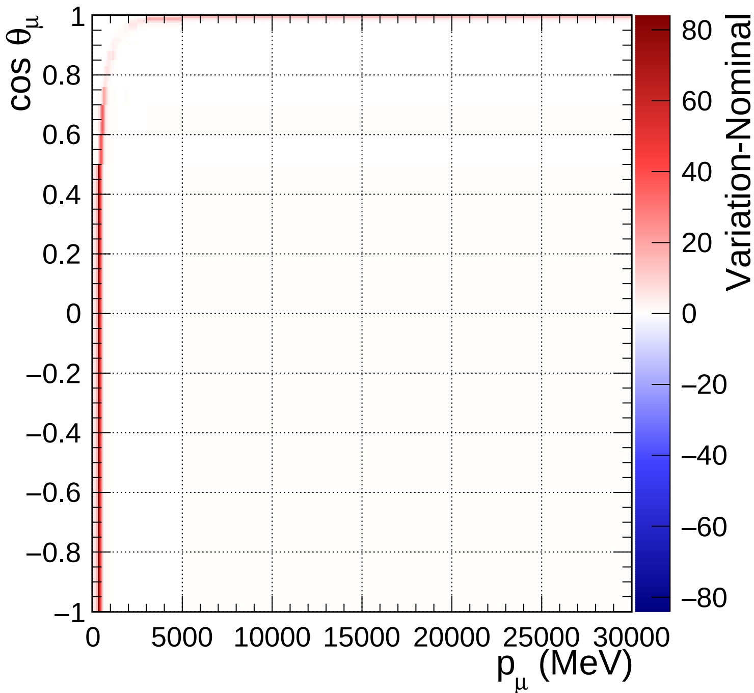
FGD1_numuCC_0pi_Q2_norm_5_1.33
