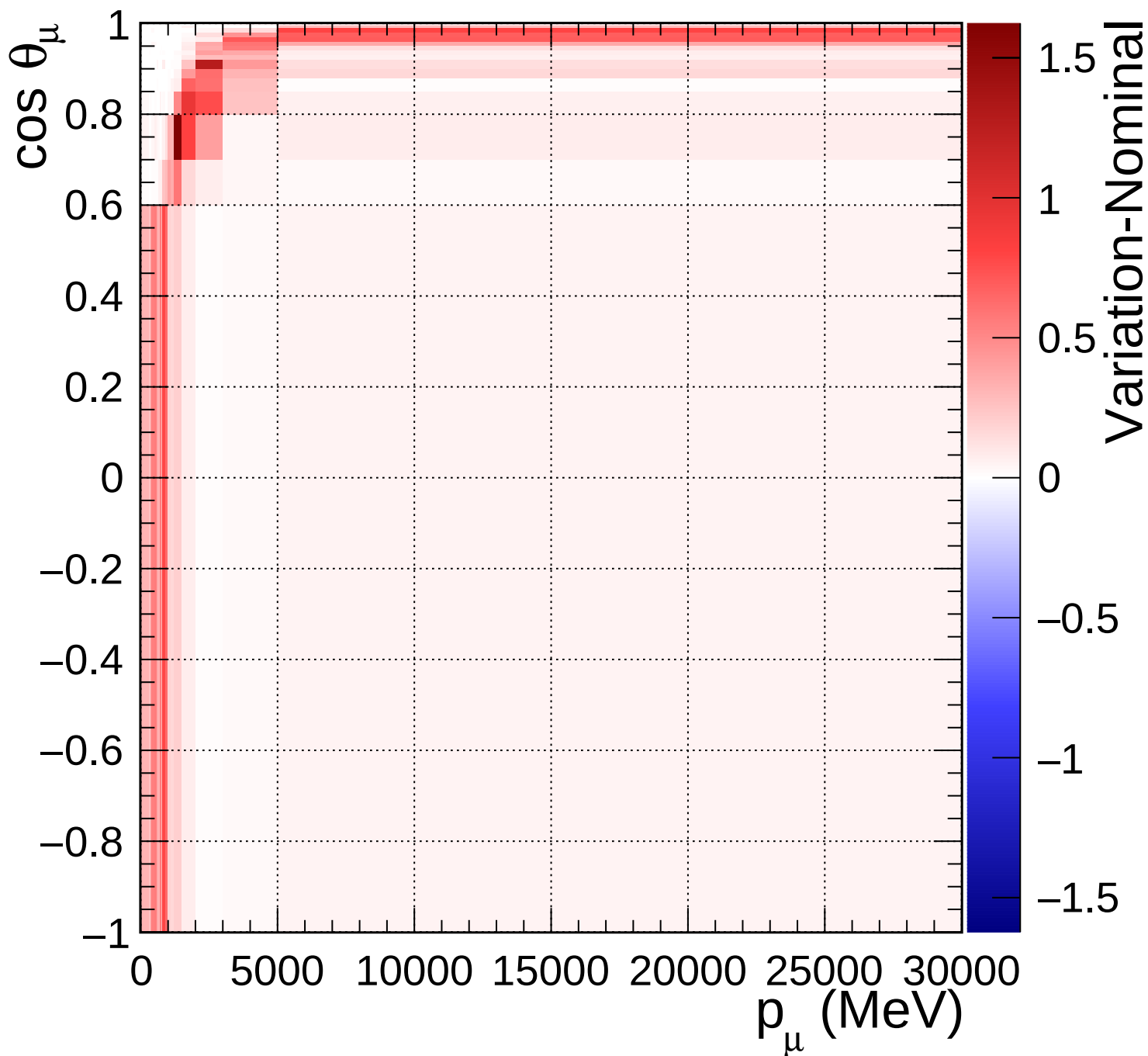
FGD2_numuCC_1pi_Q2_norm_7_1.4
