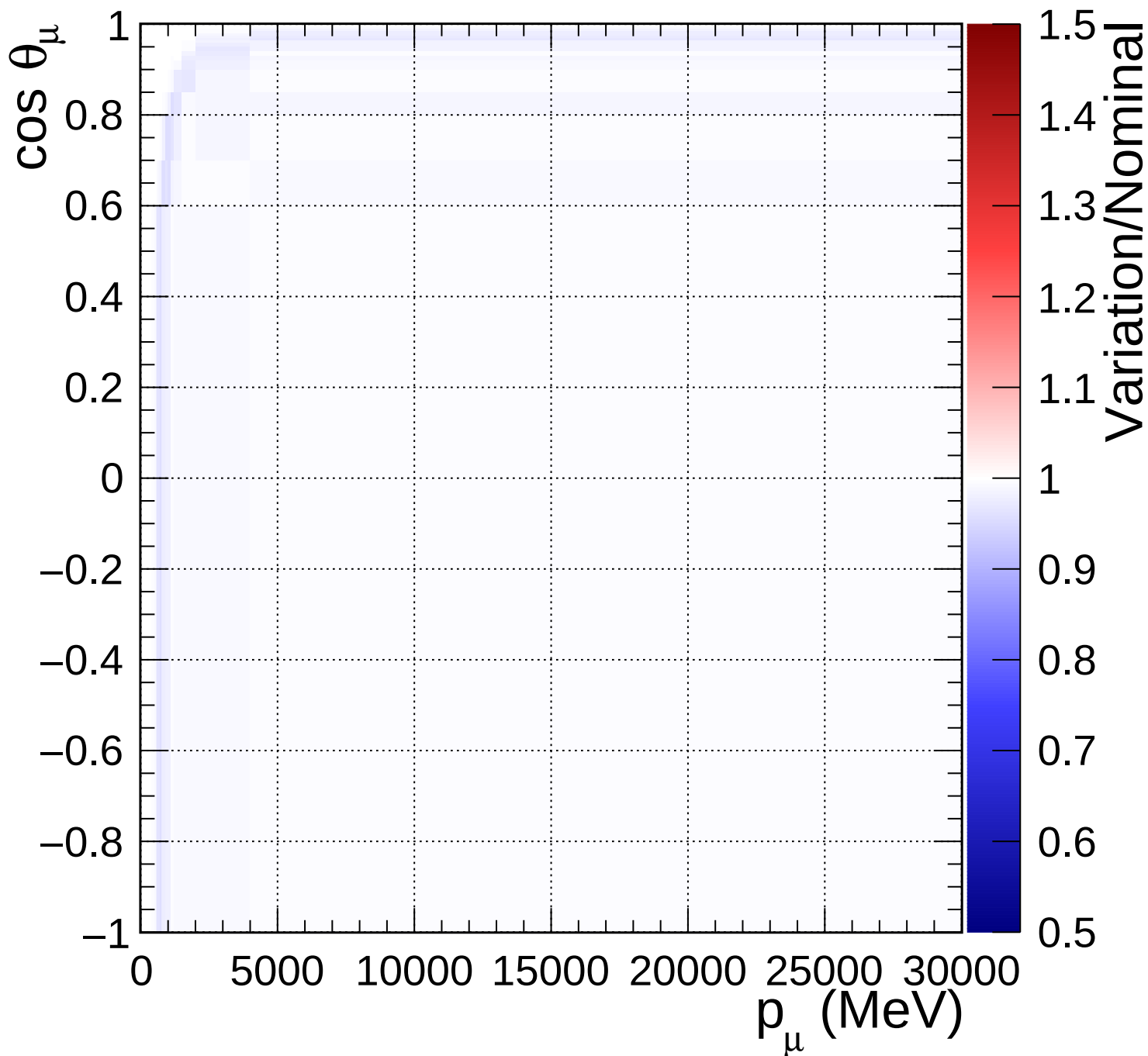
FGD1_anti-numuCC_0pi_Q2_norm_6_0.82
