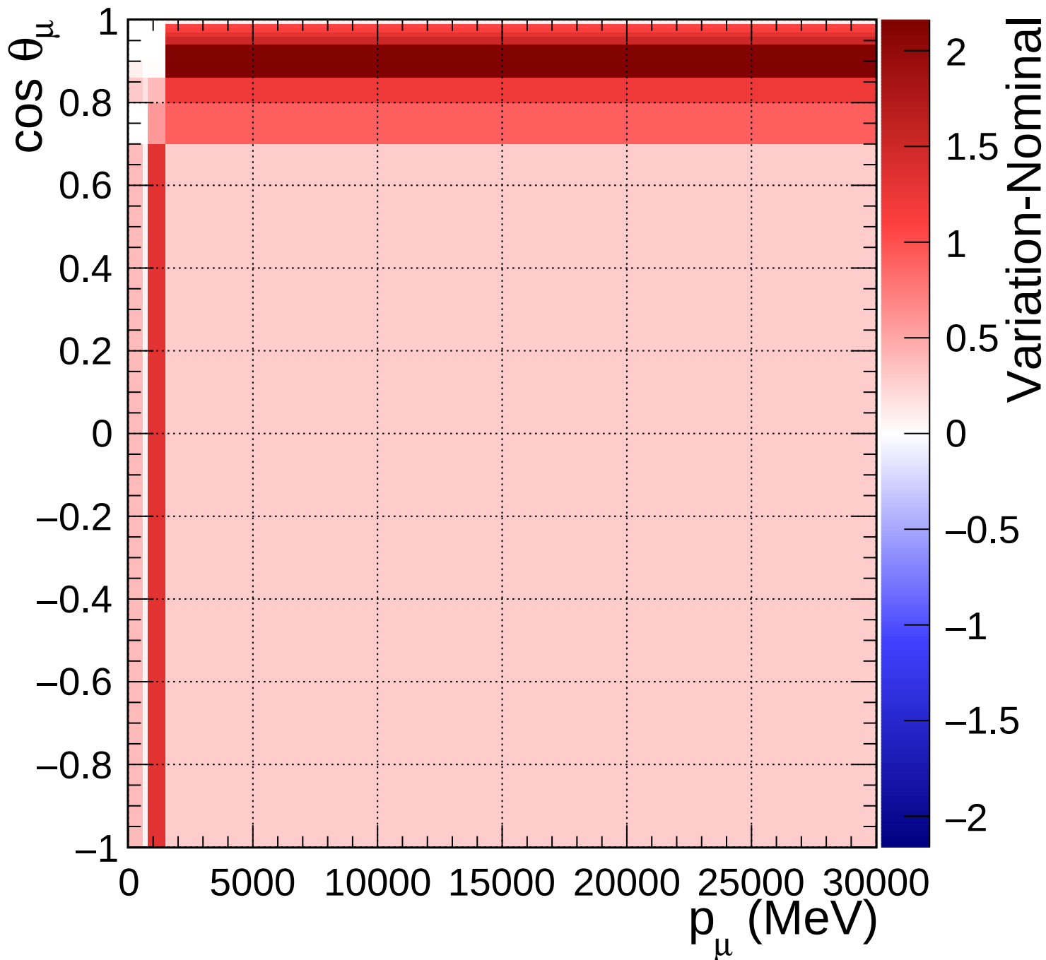
FGD1_NuMuBkg_CC1pi_in_AntiNu_Mode_Q2_norm_7_2.2
