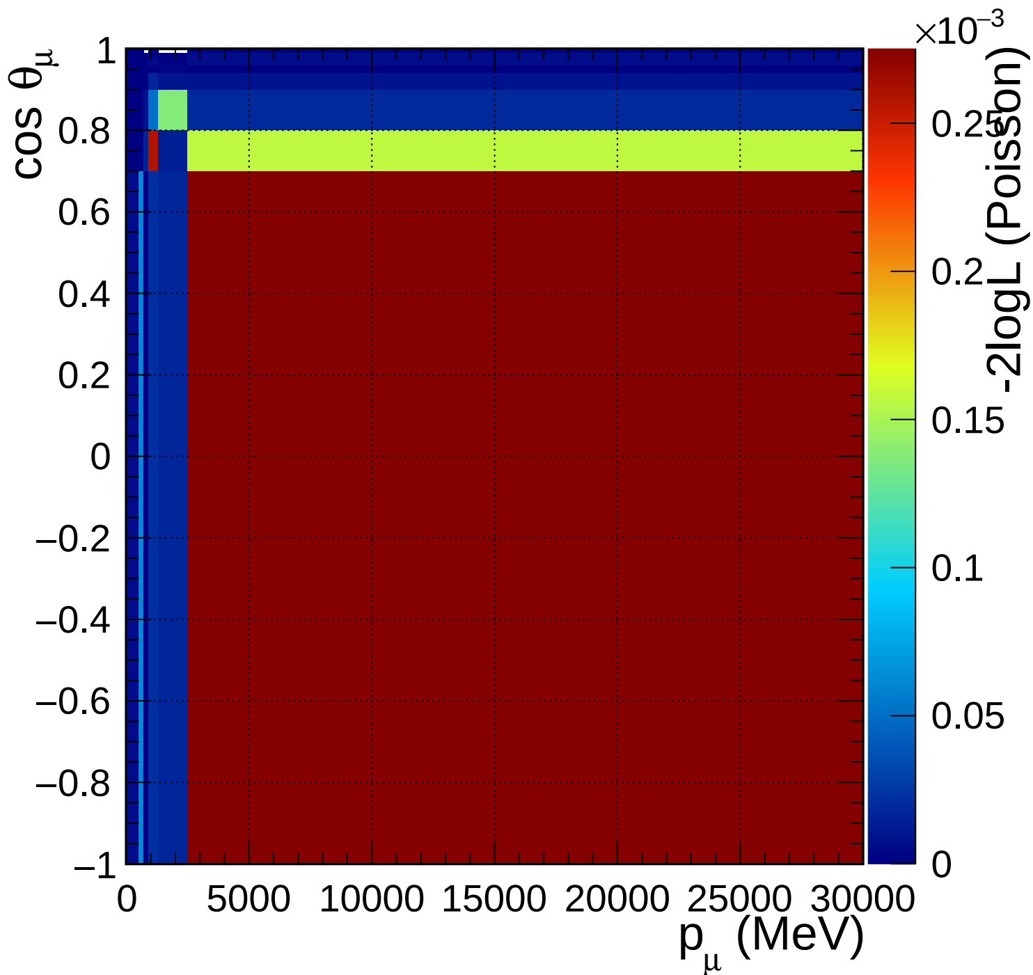
FGD1_anti-numuCC_1pi_Q2_norm_6_0.82
