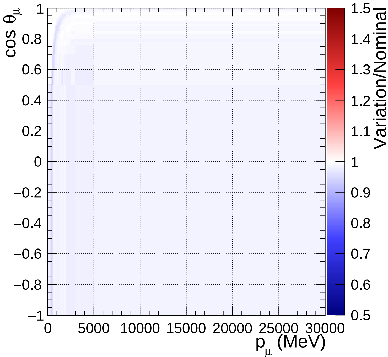
FGD2_numuCC_0pi_Q2_norm_5_0.89
