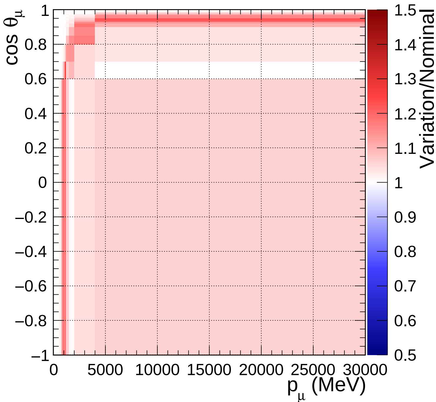
FGD1_anti-numuCC_0pi_Q2_norm_7_2.2
