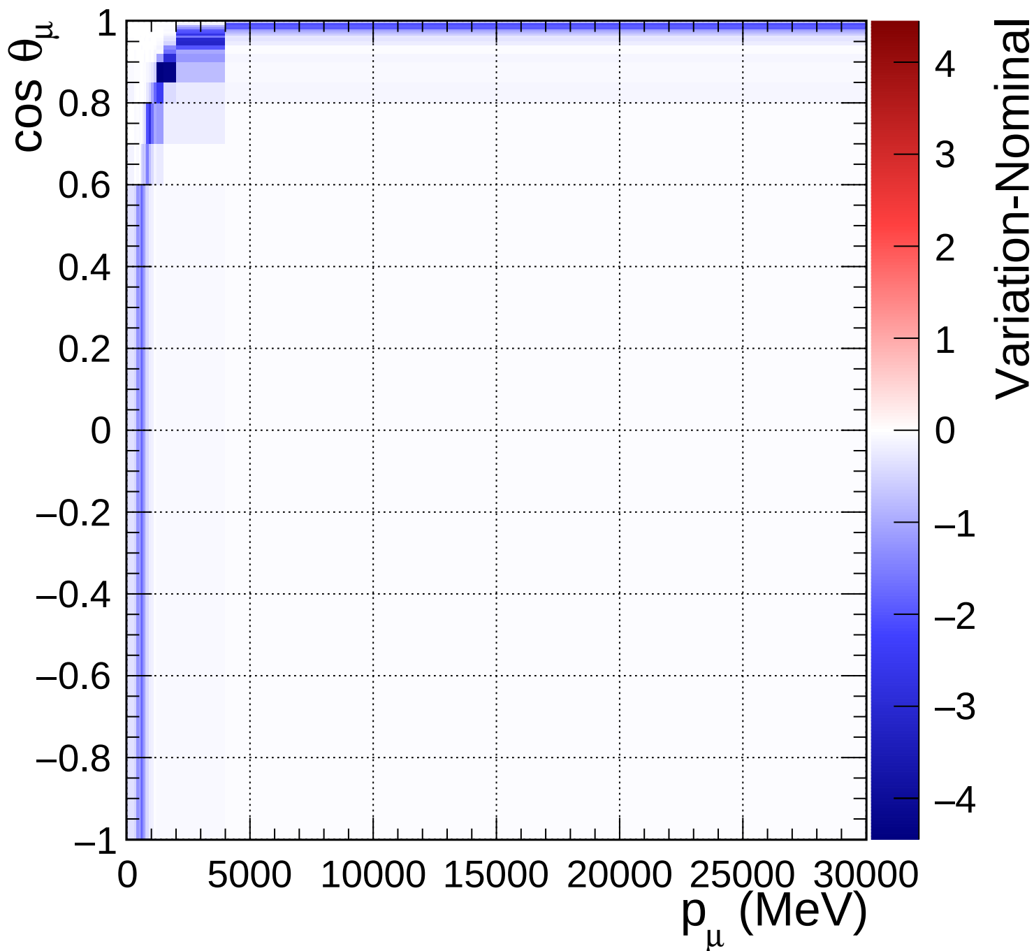
FGD1_anti-numuCC_0pi_Q2_norm_6_0.46
