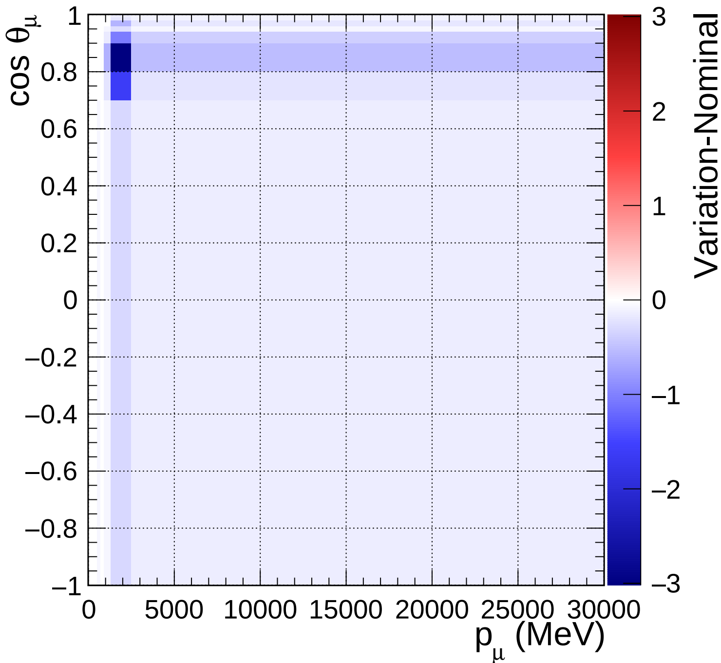
FGD1_anti-numuCC_1pi_Q2_norm_7_-0.2
