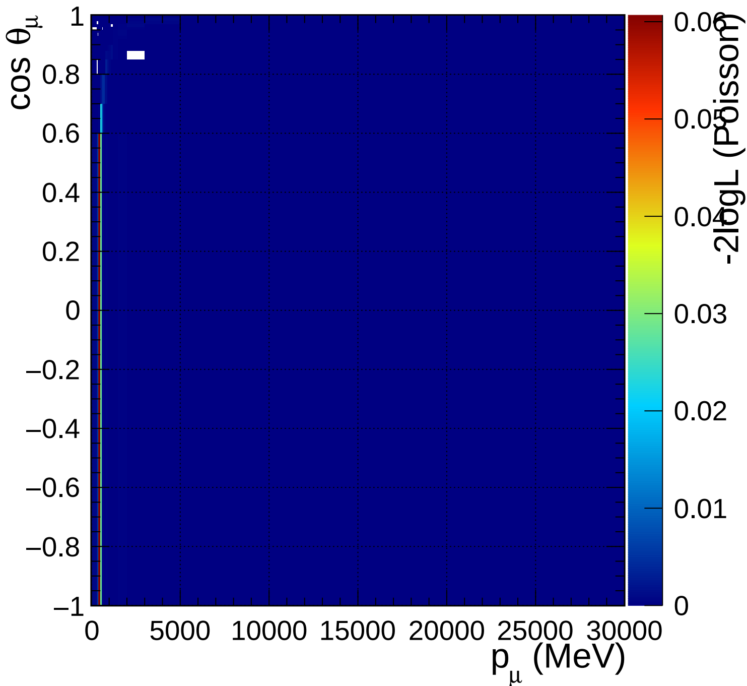
FGD1_numuCC_1pi_Q2_norm_5_0.67
