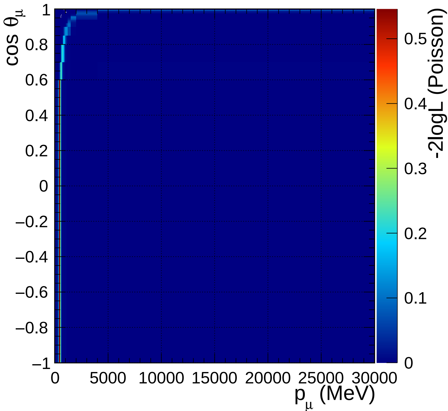
FGD2_anti-numuCC_0pi_Q2_norm_5_1.33
