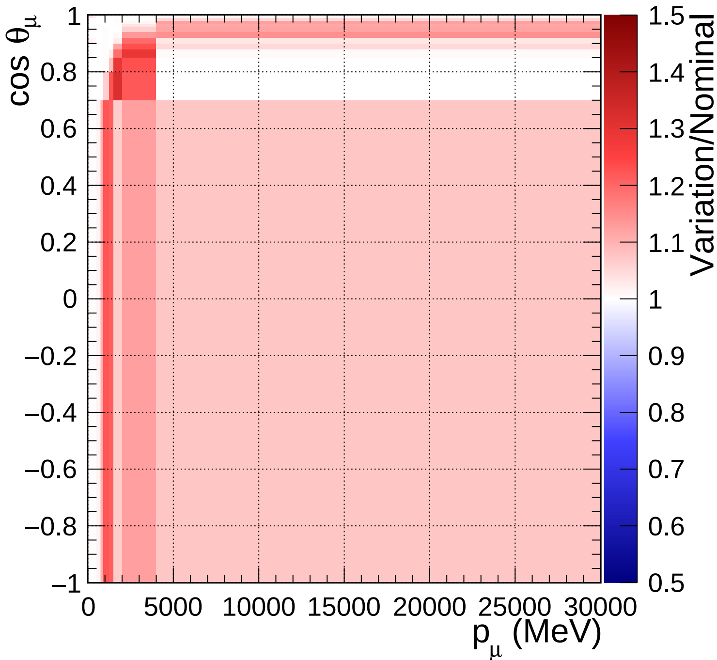
FGD1_NuMuBkg_CC0pi_in_AntiNu_Mode_Q2_norm_7_2.2
