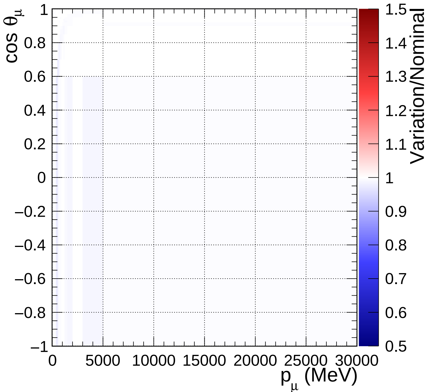
FGD1_numuCC_1pi_Q2_norm_5_0.67
