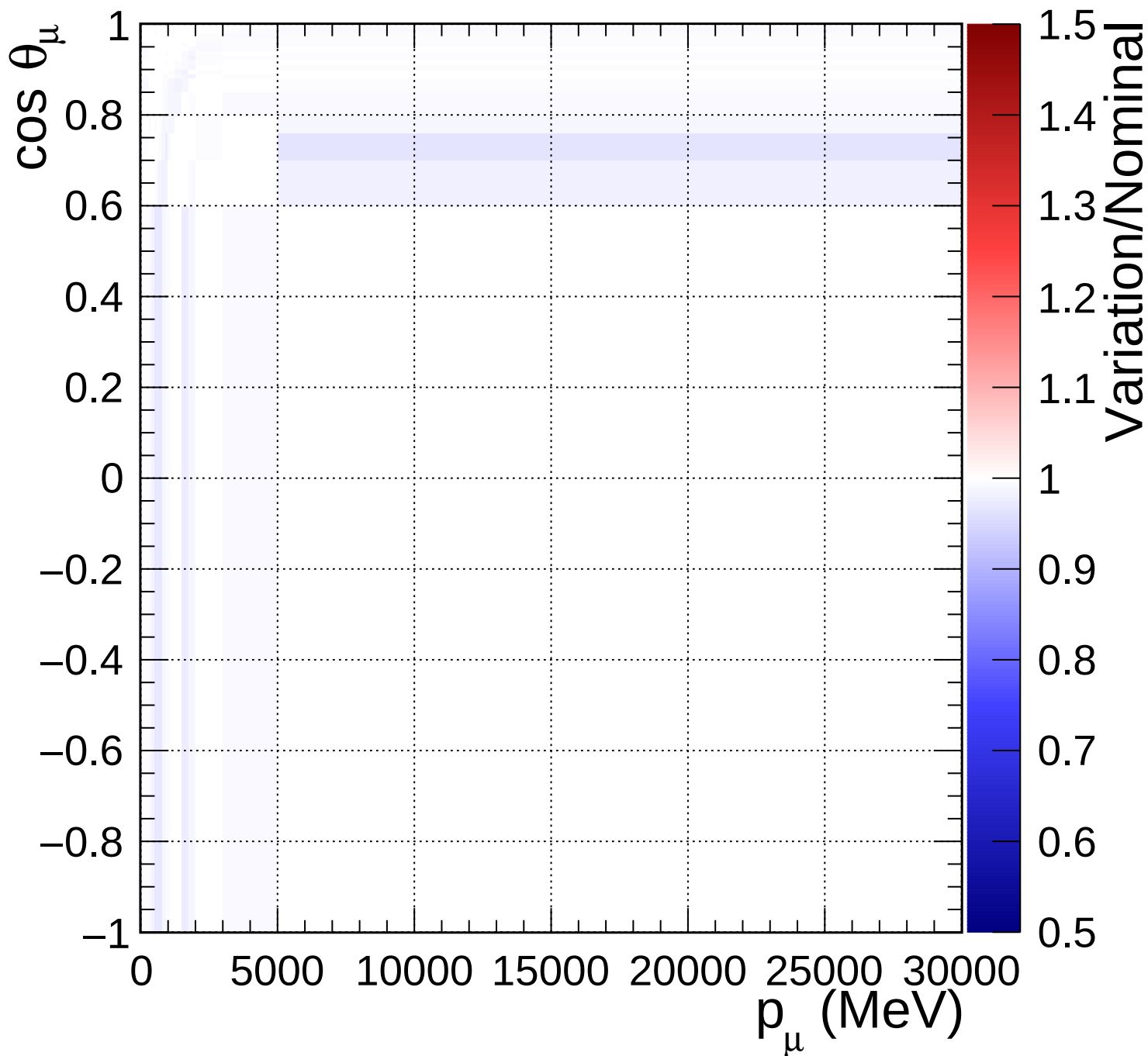
FGD1_numuCC_other_Q2_norm_6_0.46
