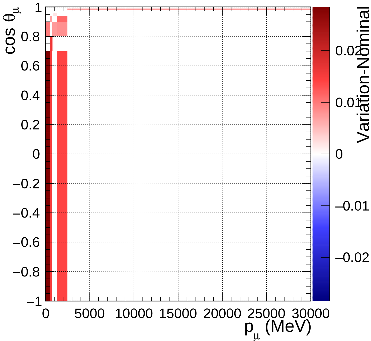
FGD1_anti-numuCC_1pi_Q2_norm_5_1.11
