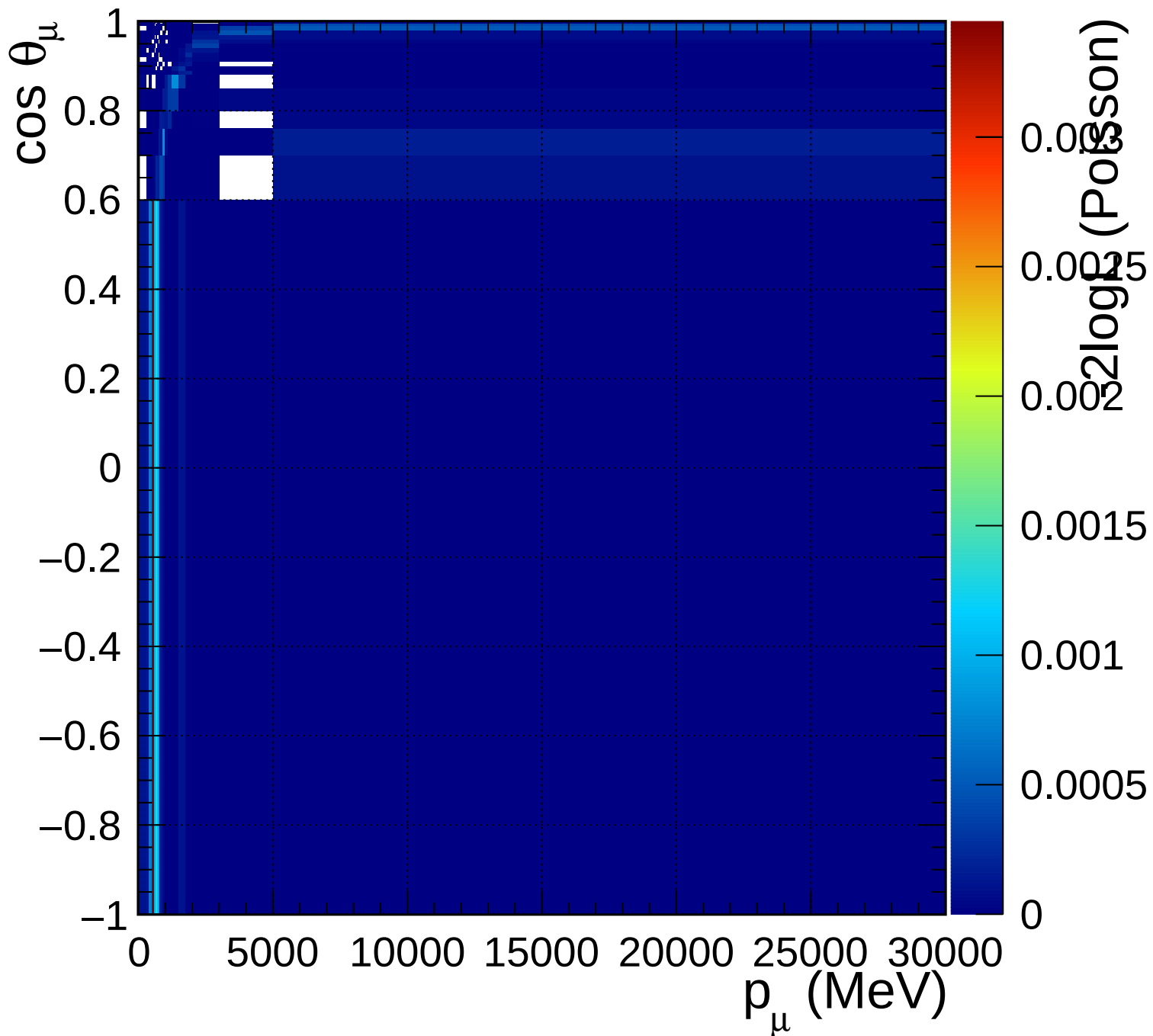
FGD1_numuCC_other_Q2_norm_6_1.18
