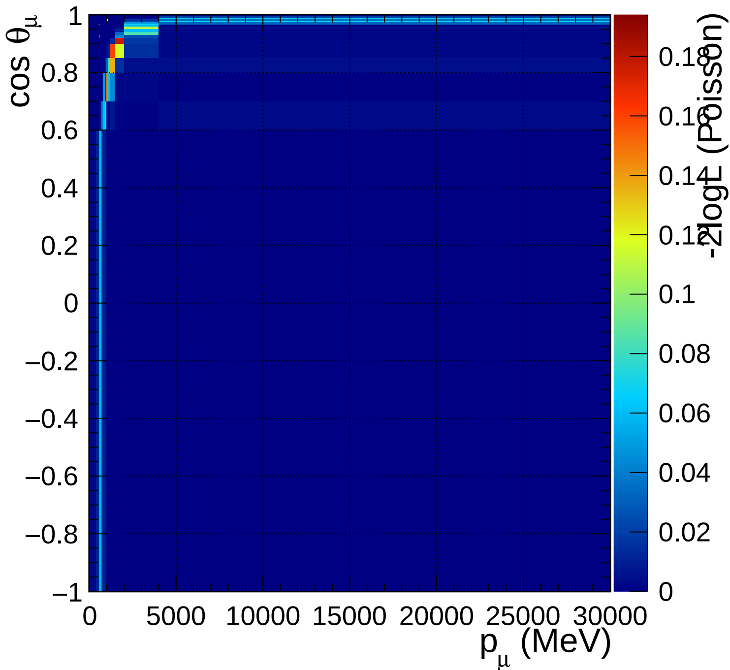
FGD2_anti-numuCC_0pi_Q2_norm_6_0.46
