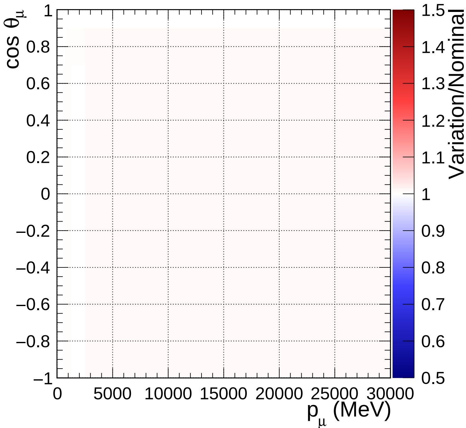
FGD2_anti-numuCC_1pi_Q2_norm_6_1.18
