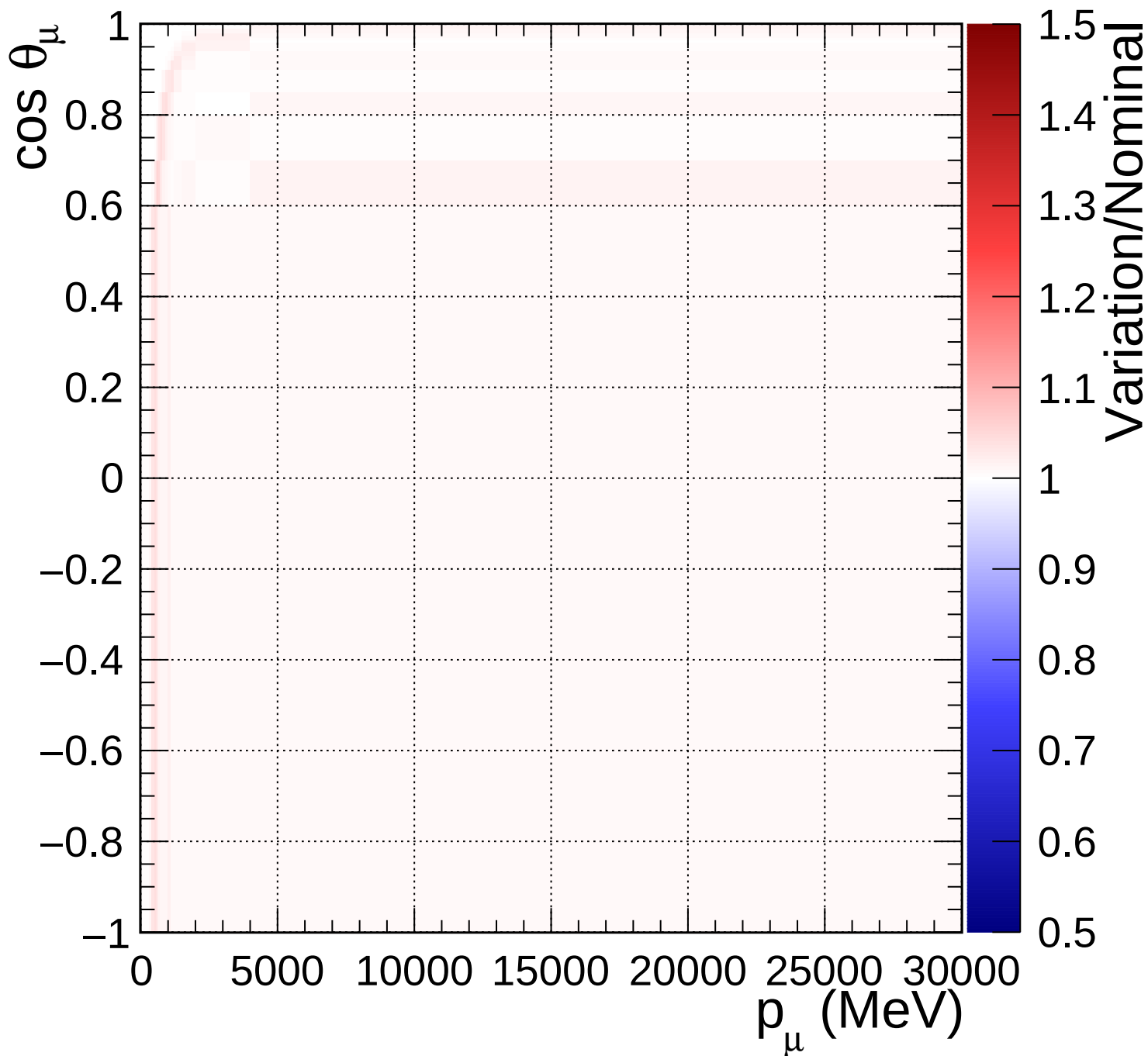
FGD2_anti-numuCC_0pi_Q2_norm_5_1.11
