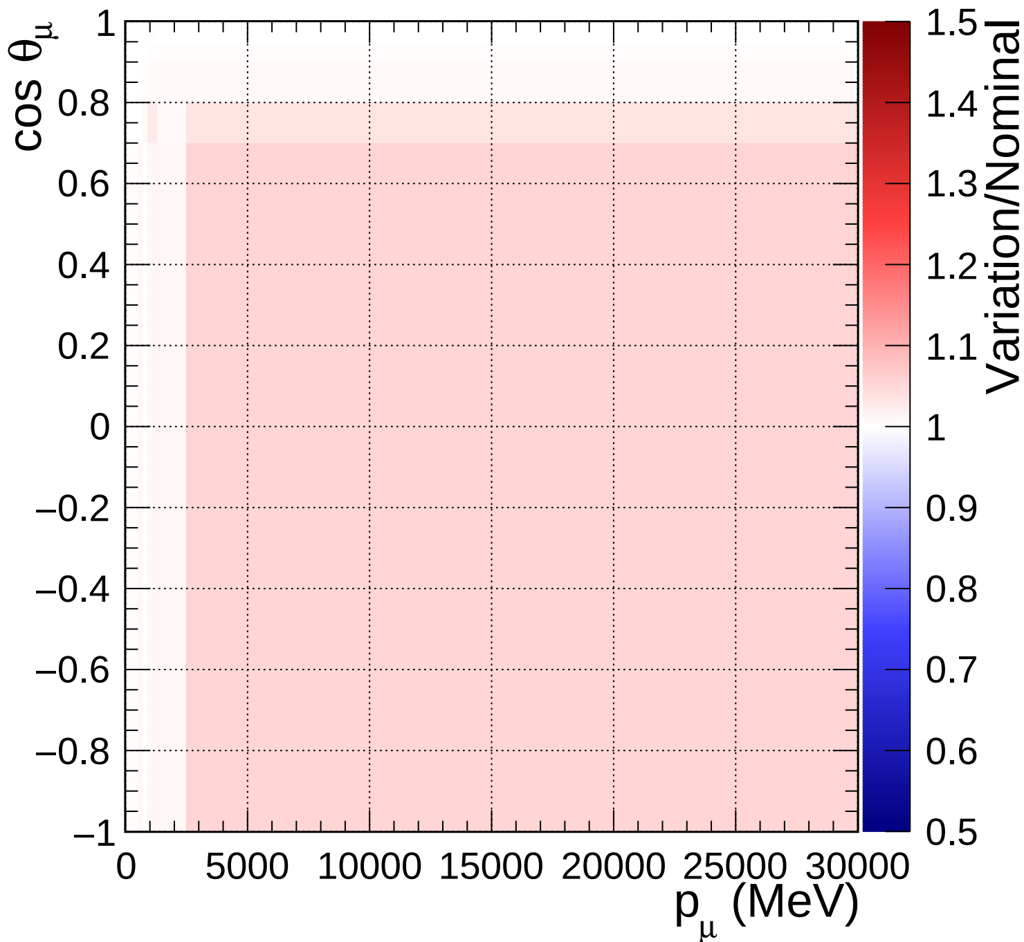
FGD1_anti-numuCC_1pi_Q2_norm_6_1.54
