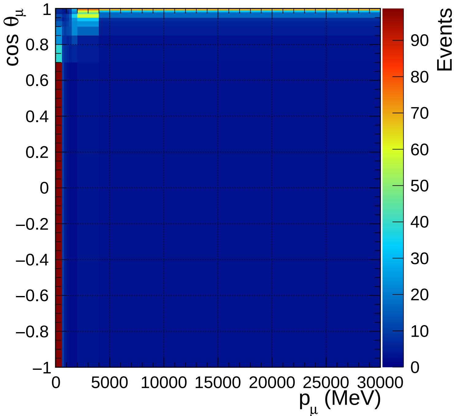
FGD1_anti-numuCC_other_Q2_norm_5_1
