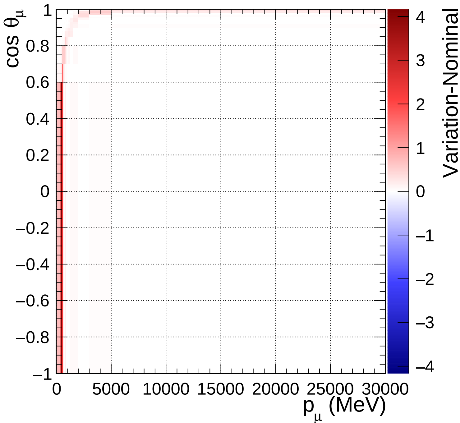
FGD1_numuCC_1pi_Q2_norm_5_1.33
