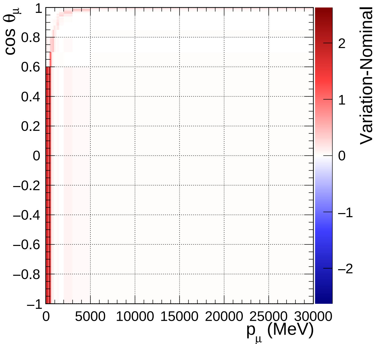
FGD2_numuCC_1pi_Q2_norm_5_1.33
