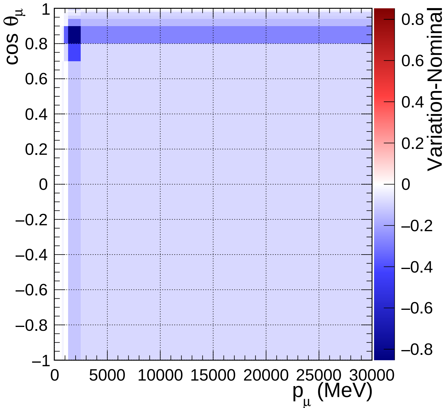
FGD2_anti-numuCC_1pi_Q2_norm_7_0.6
