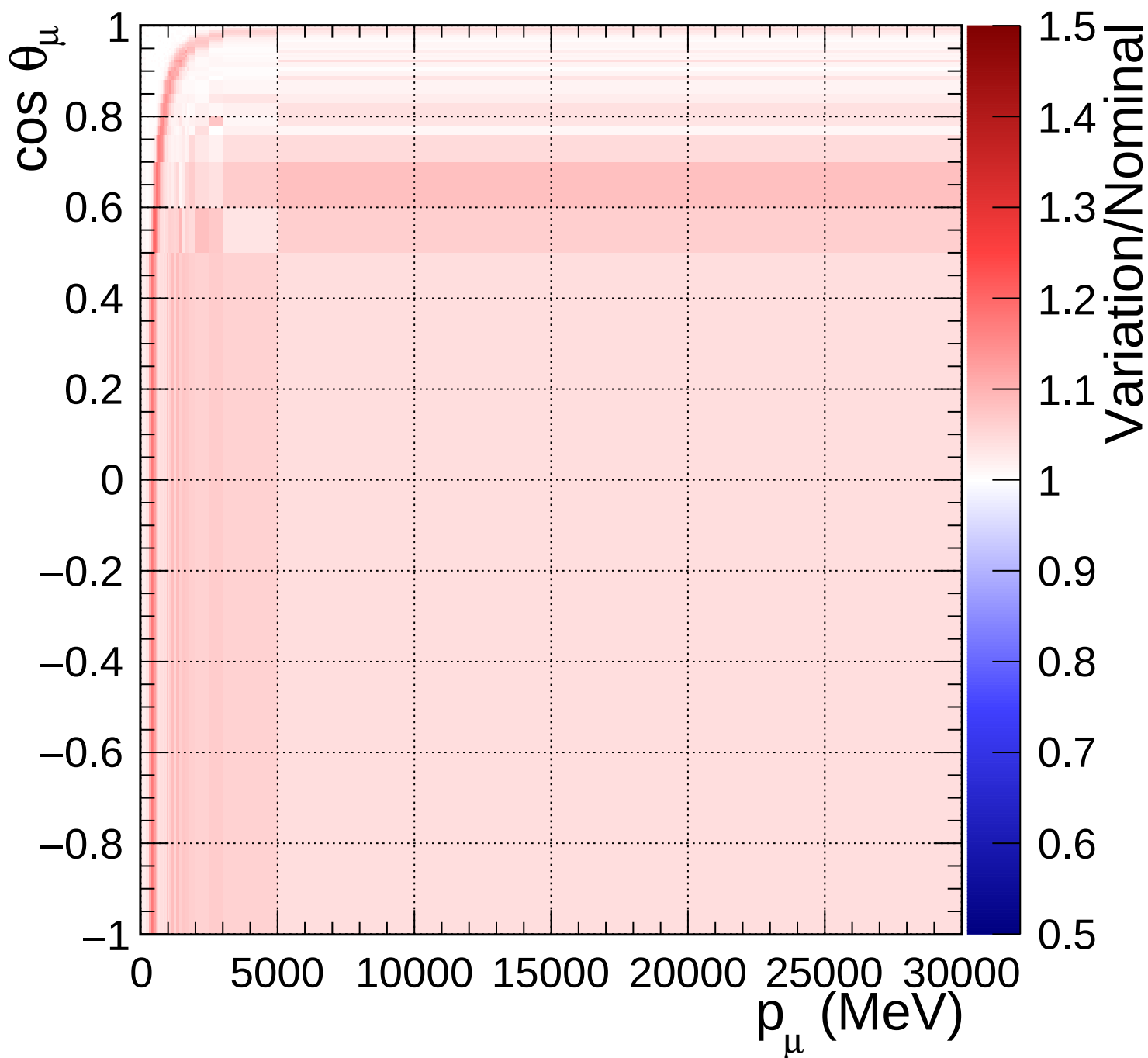
FGD1_numuCC_0pi_Q2_norm_5_1.33
