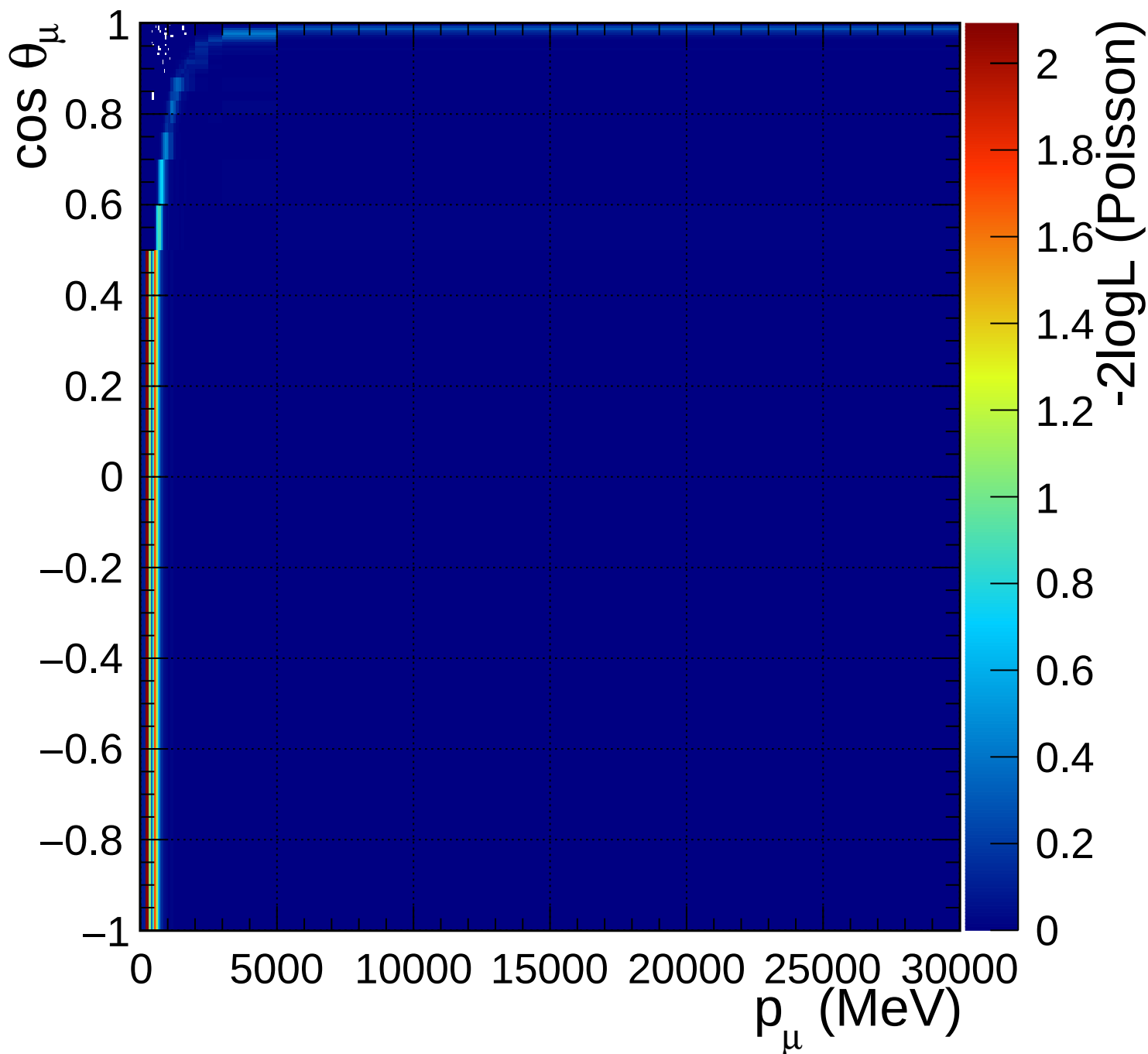
FGD2_numuCC_0pi_Q2_norm_6_1.54
