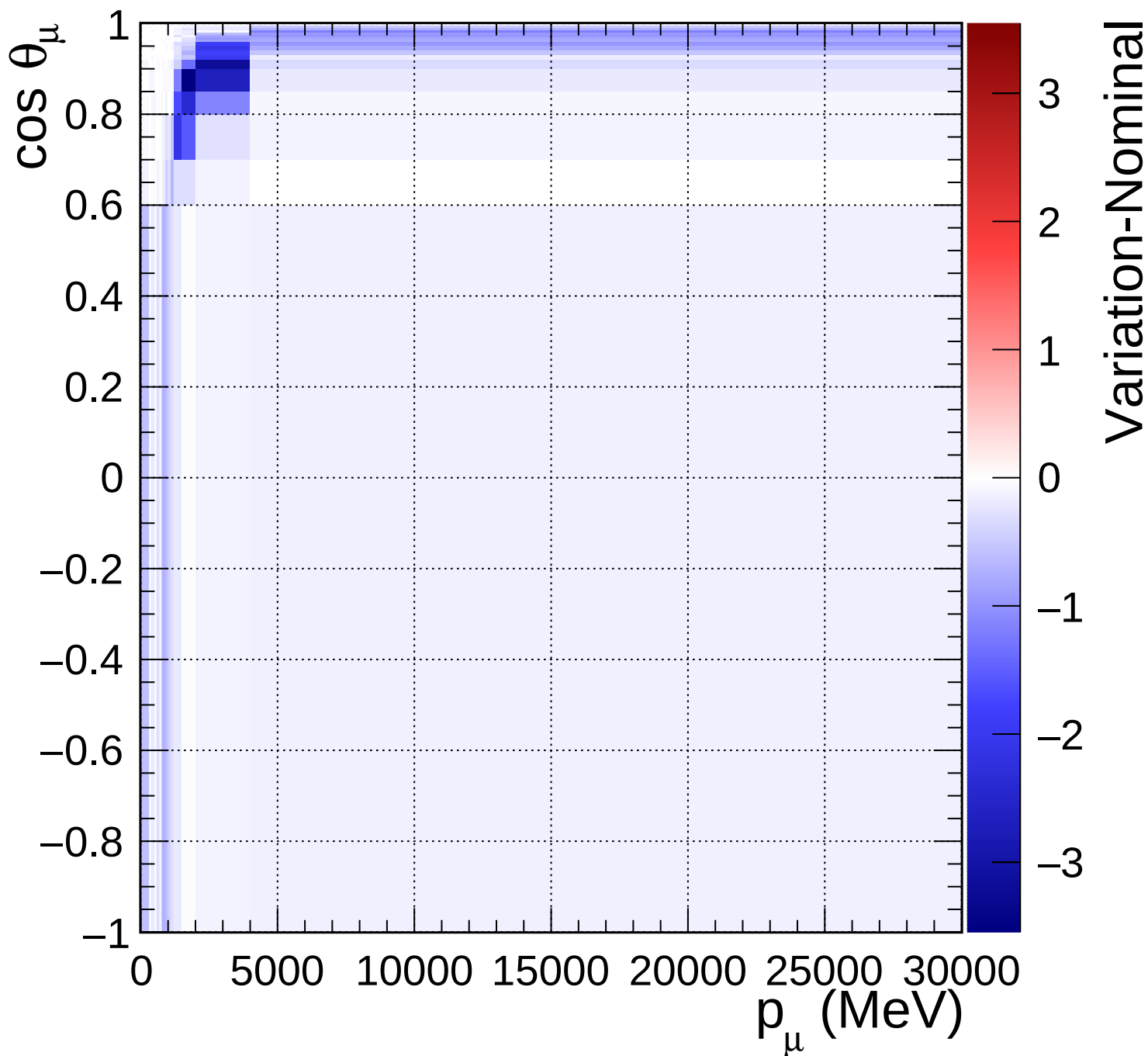
FGD1_anti-numuCC_0pi_Q2_norm_7_-0.2
