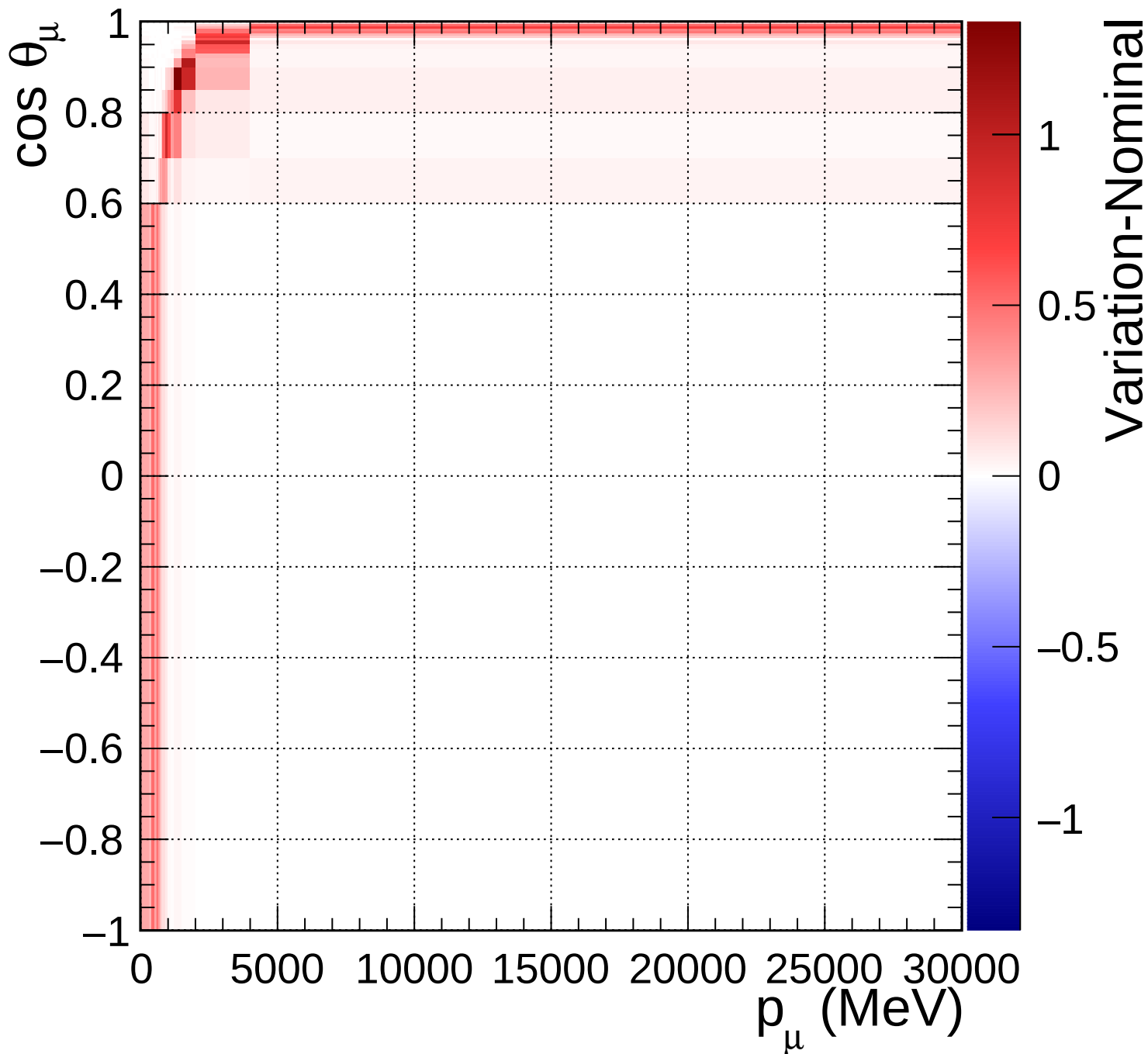
FGD2_anti-numuCC_0pi_Q2_norm_6_1.18
