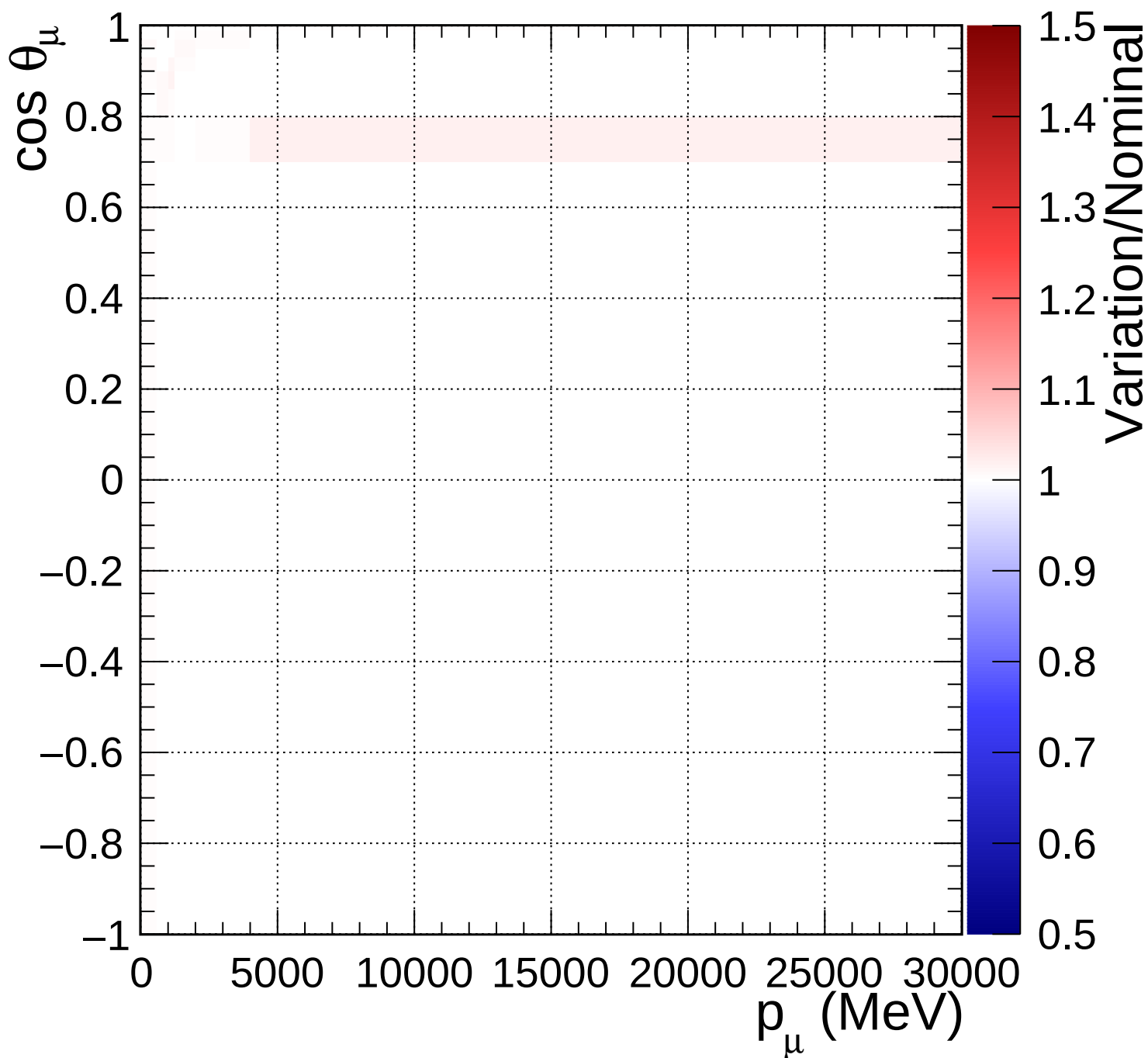
FGD1_NuMuBkg_CCother_in_AntiNu_Mode_Q2_norm_5_1.33
