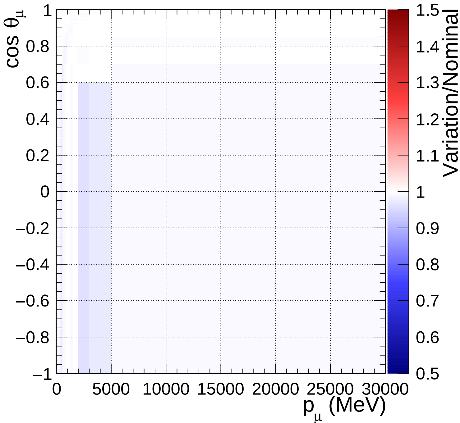
FGD2_numuCC_1pi_Q2_norm_5_0.67
