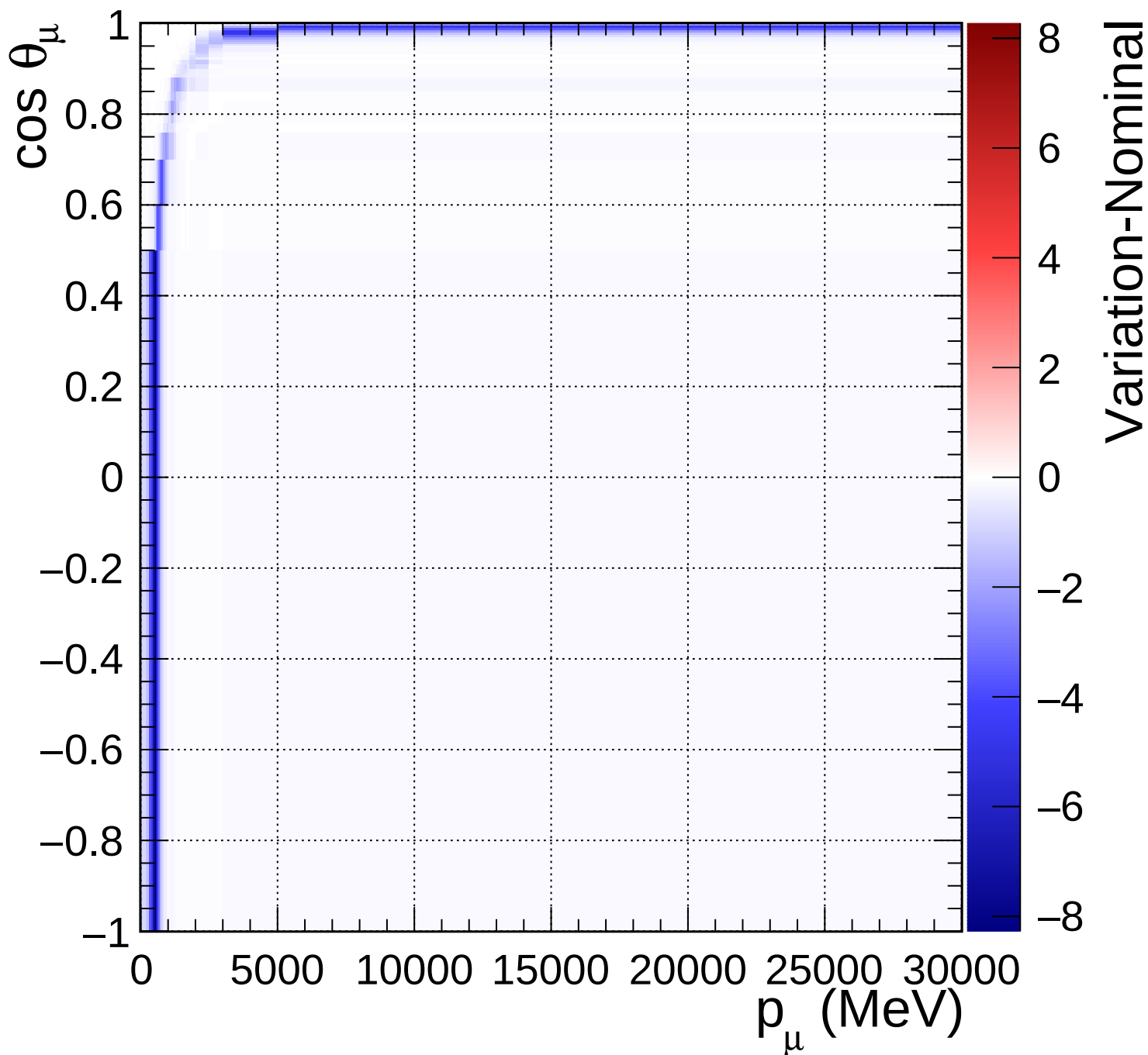
FGD1_numuCC_0pi_Q2_norm_6_0.82
