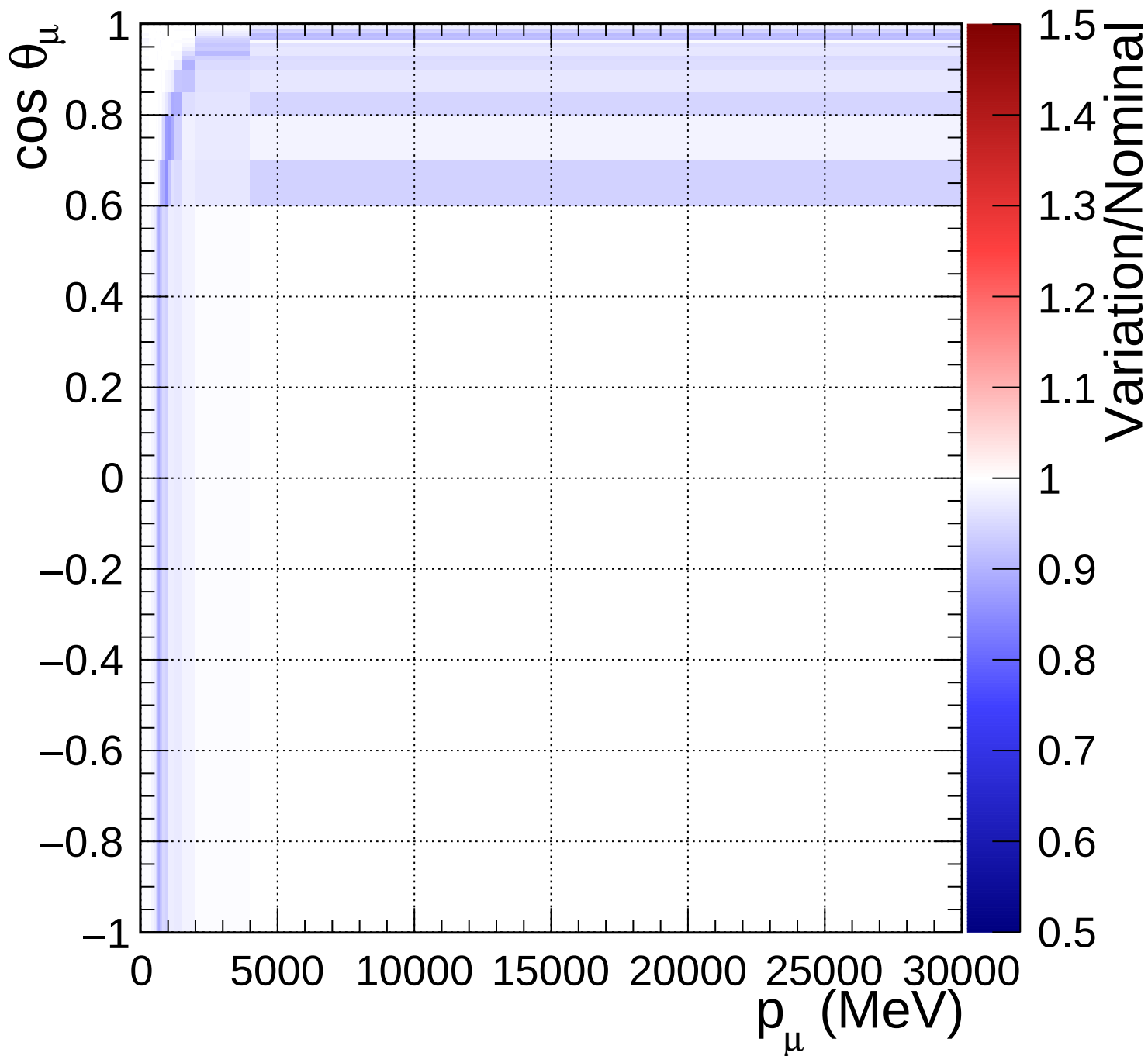
FGD2_anti-numuCC_0pi_Q2_norm_6_0.46
