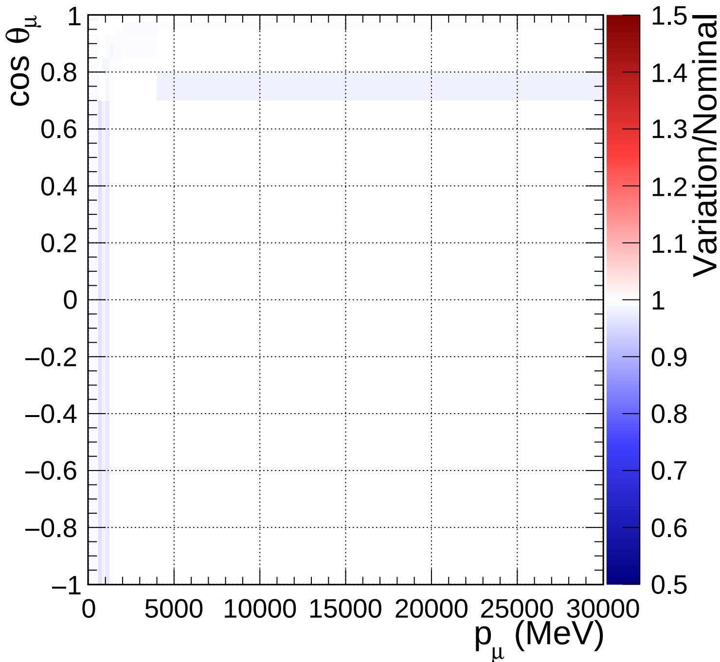
FGD2_anti-numuCC_other_Q2_norm_6_0.46
