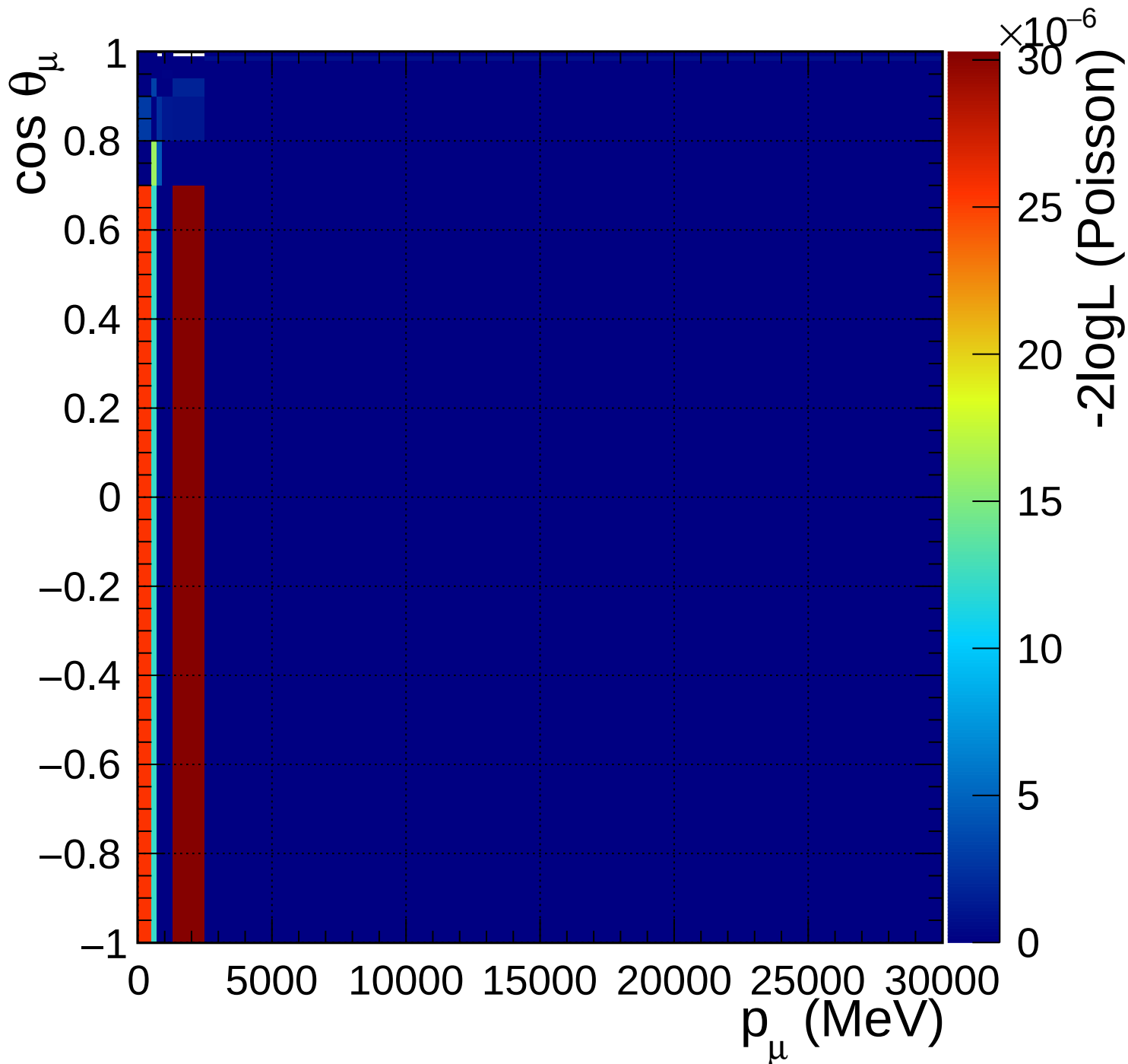
FGD1_anti-numuCC_1pi_Q2_norm_5_0.89
