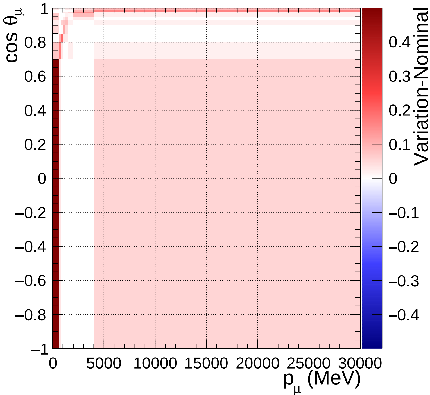
FGD2_anti-numuCC_other_Q2_norm_5_1.33
