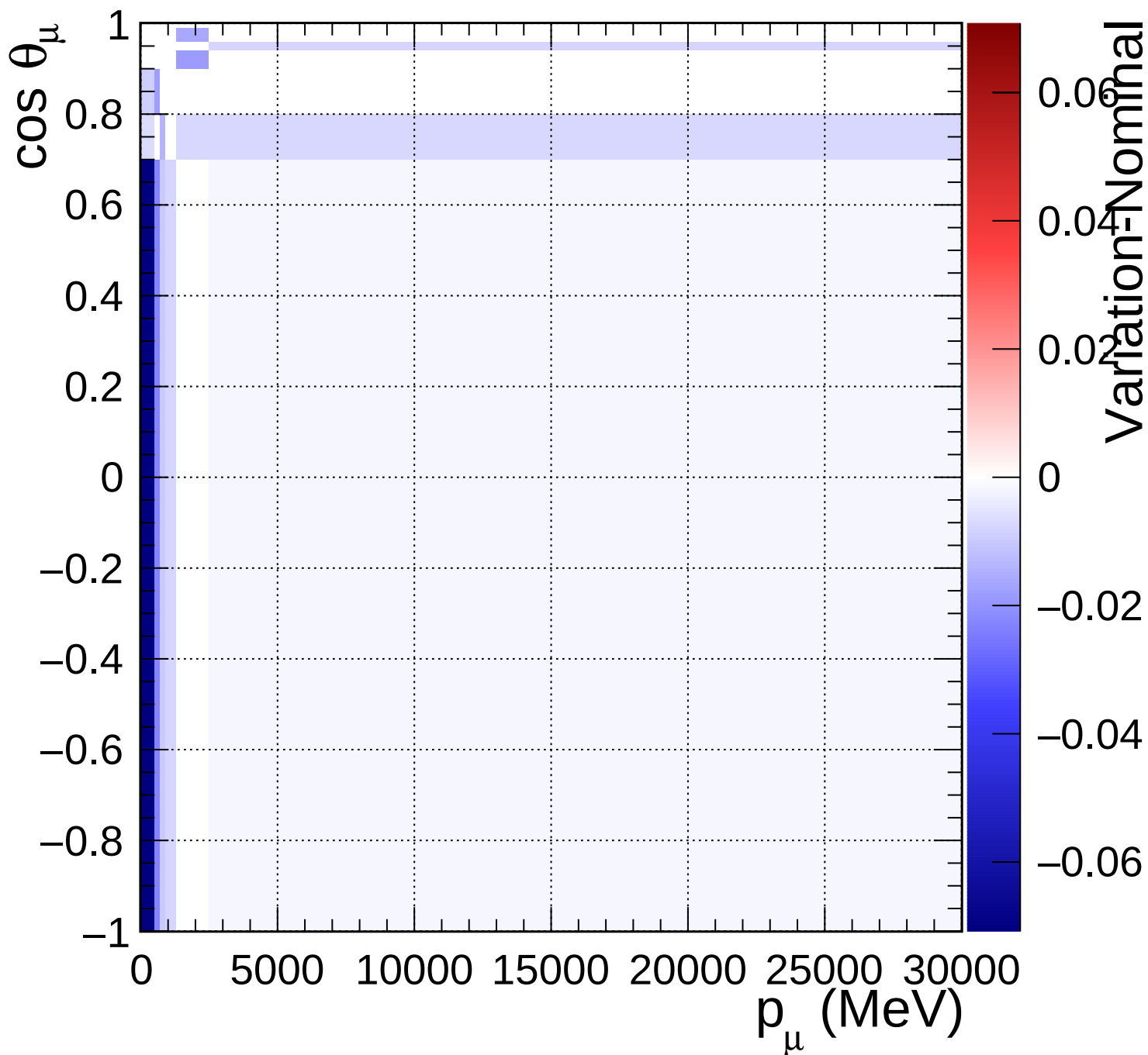
FGD2_anti-numuCC_1pi_Q2_norm_5_0.89
