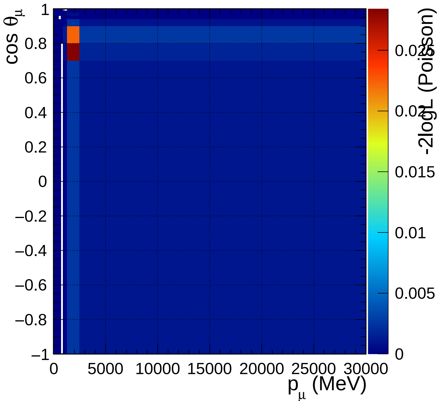
FGD1_anti-numuCC_1pi_Q2_norm_7_1.4
