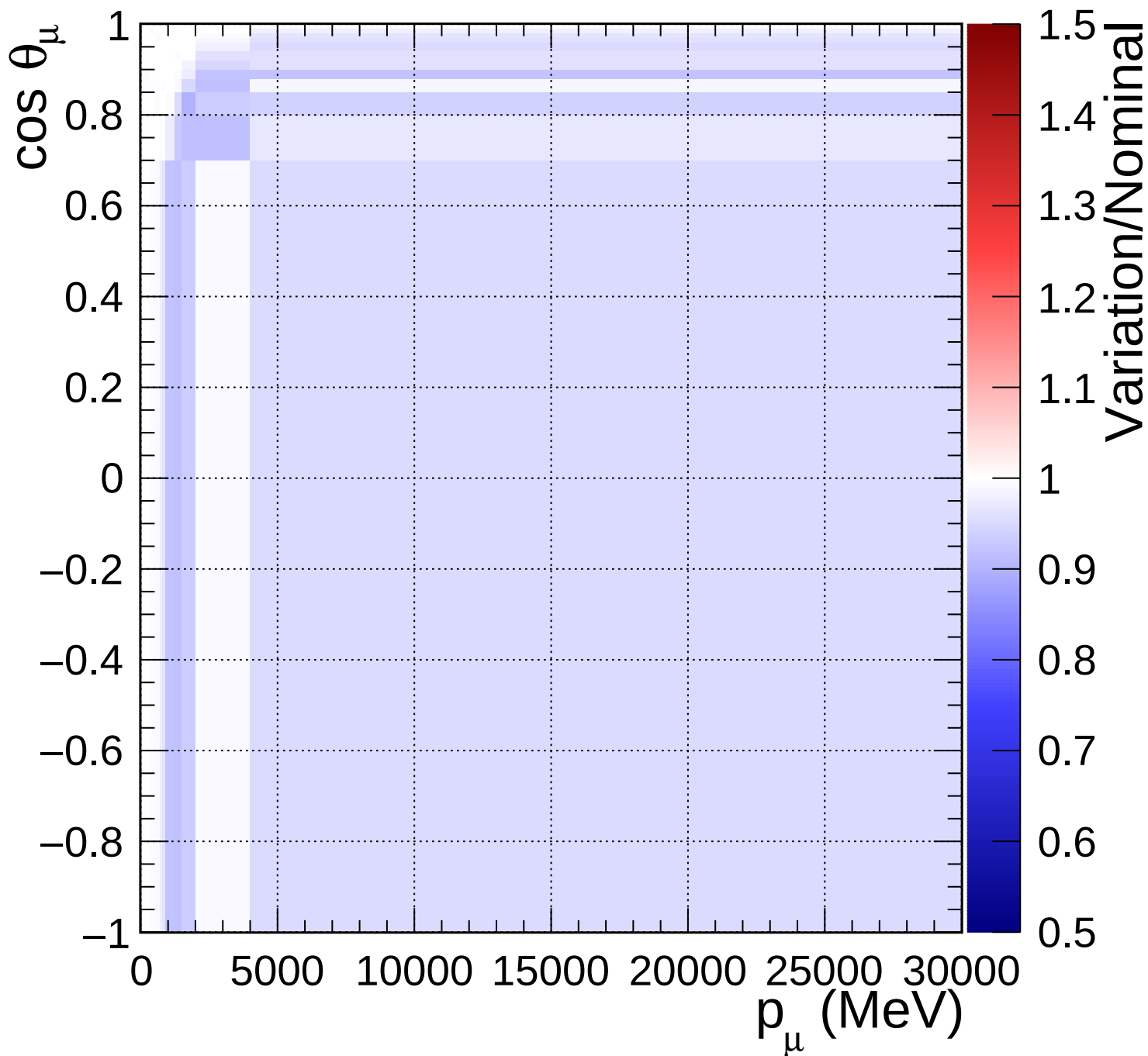
FGD2_NuMuBkg_CC0pi_in_AntiNu_Mode_Q2_norm_7_0.6
