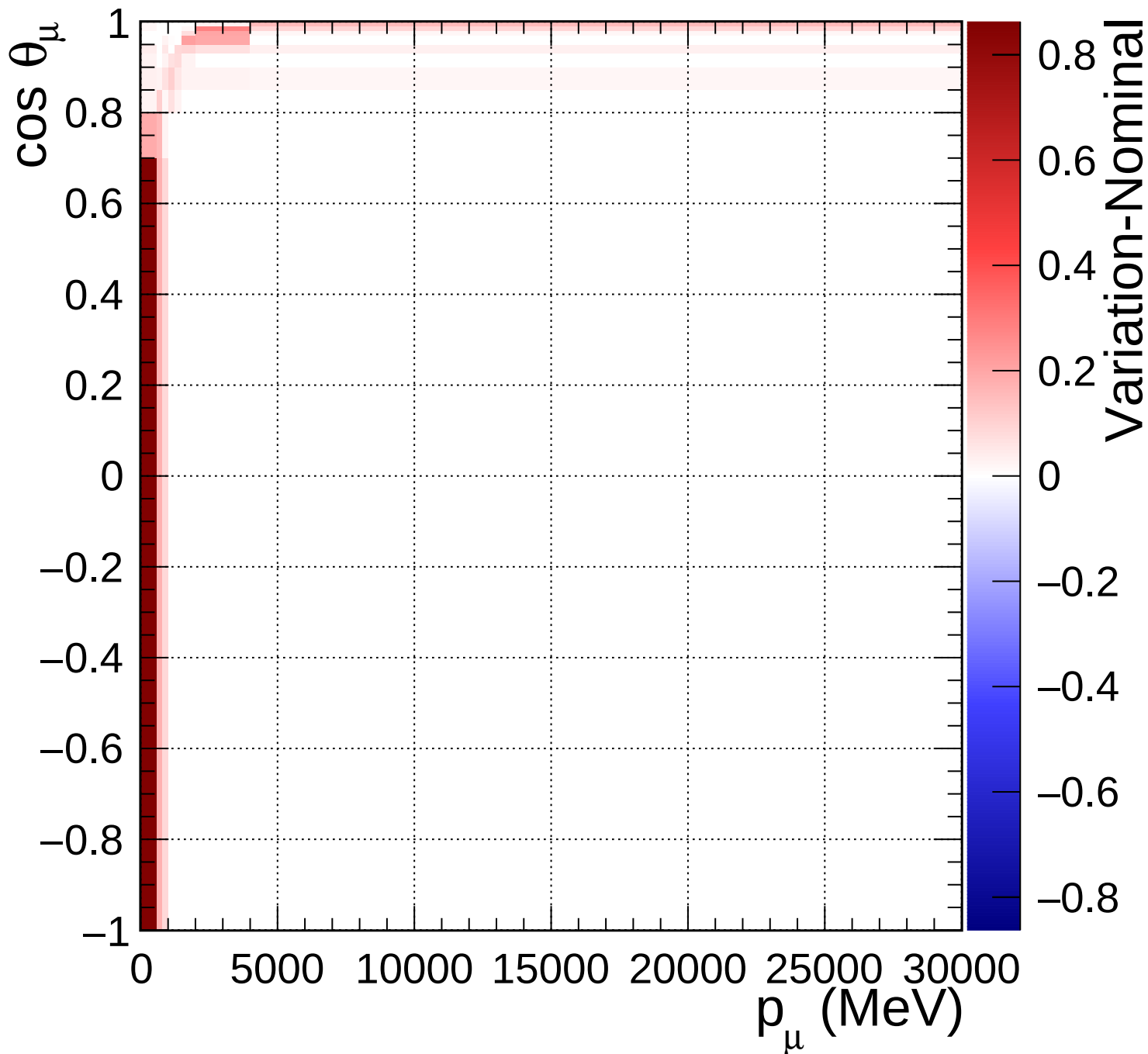
FGD1_anti-numuCC_other_Q2_norm_5_1.33
