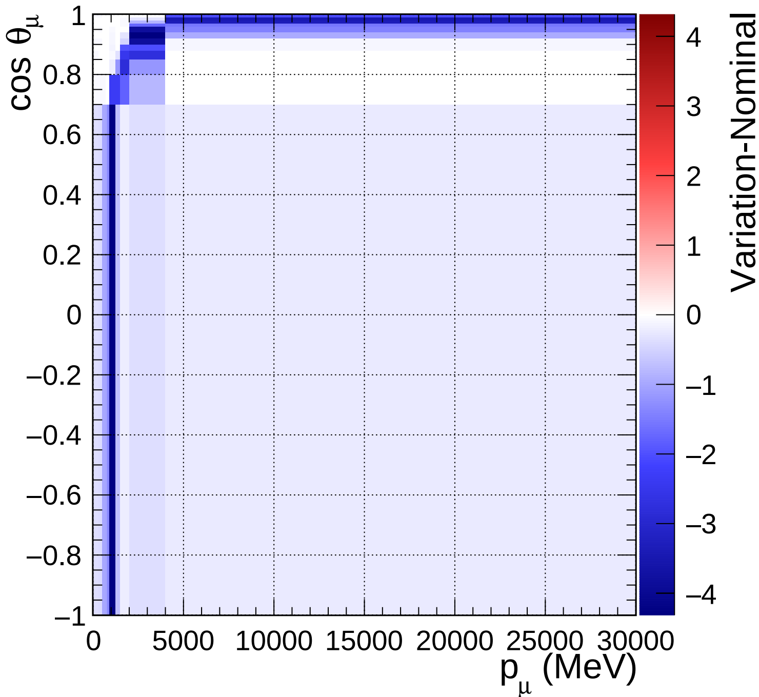
FGD1_NuMuBkg_CC0pi_in_AntiNu_Mode_Q2_norm_7_-0.2
