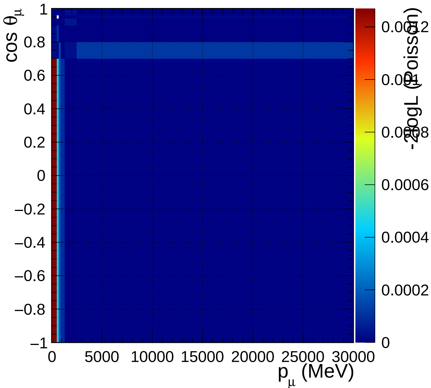
FGD2_anti-numuCC_1pi_Q2_norm_5_0.67
