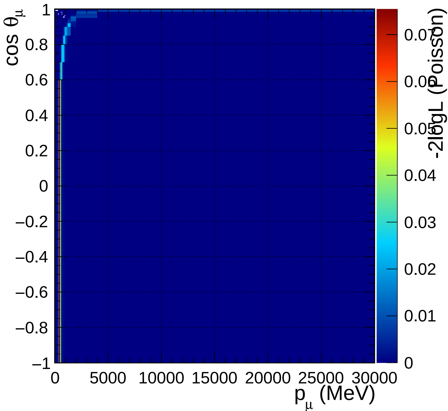
FGD1_anti-numuCC_0pi_Q2_norm_5_0.89
