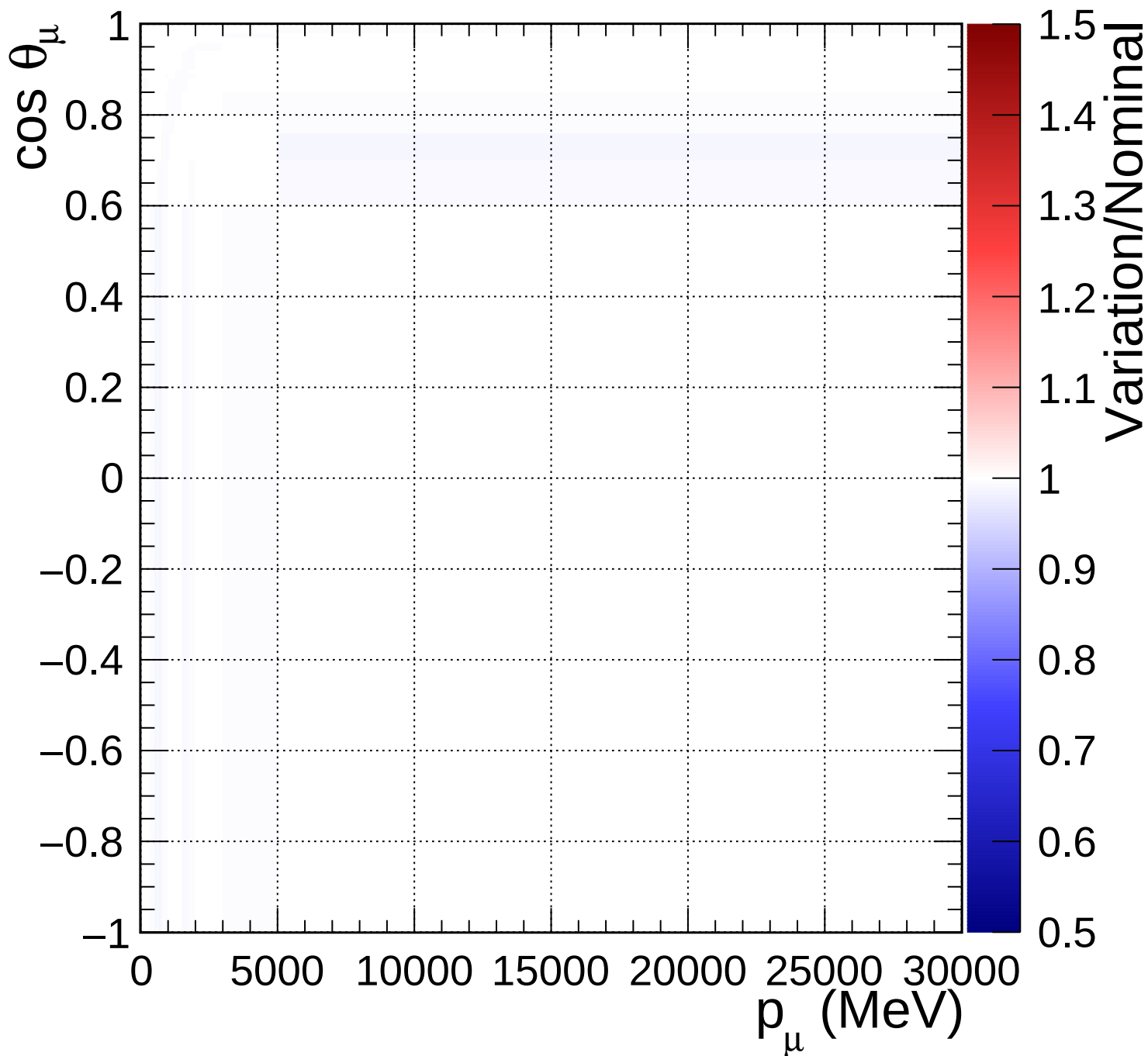
FGD1_numuCC_other_Q2_norm_6_0.82
