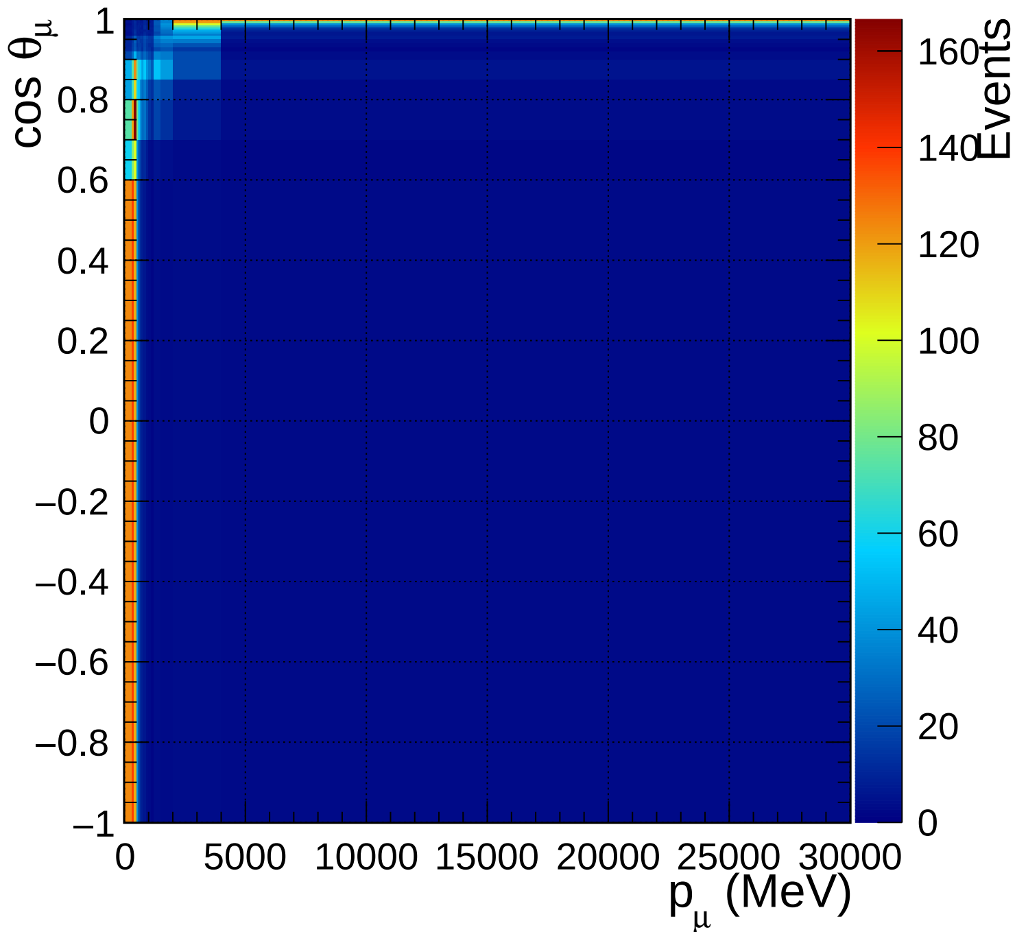
FGD1_anti-numuCC_0pi_Q2_norm_6_1
