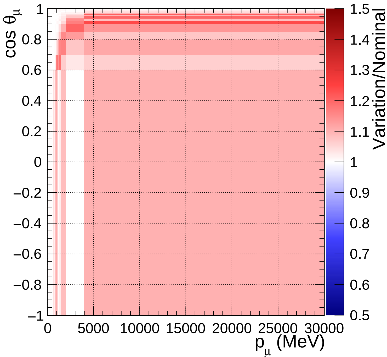
FGD2_anti-numuCC_0pi_Q2_norm_7_2.2
