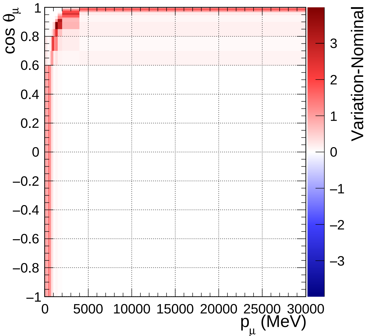
FGD2_anti-numuCC_0pi_Q2_norm_6_1.54
