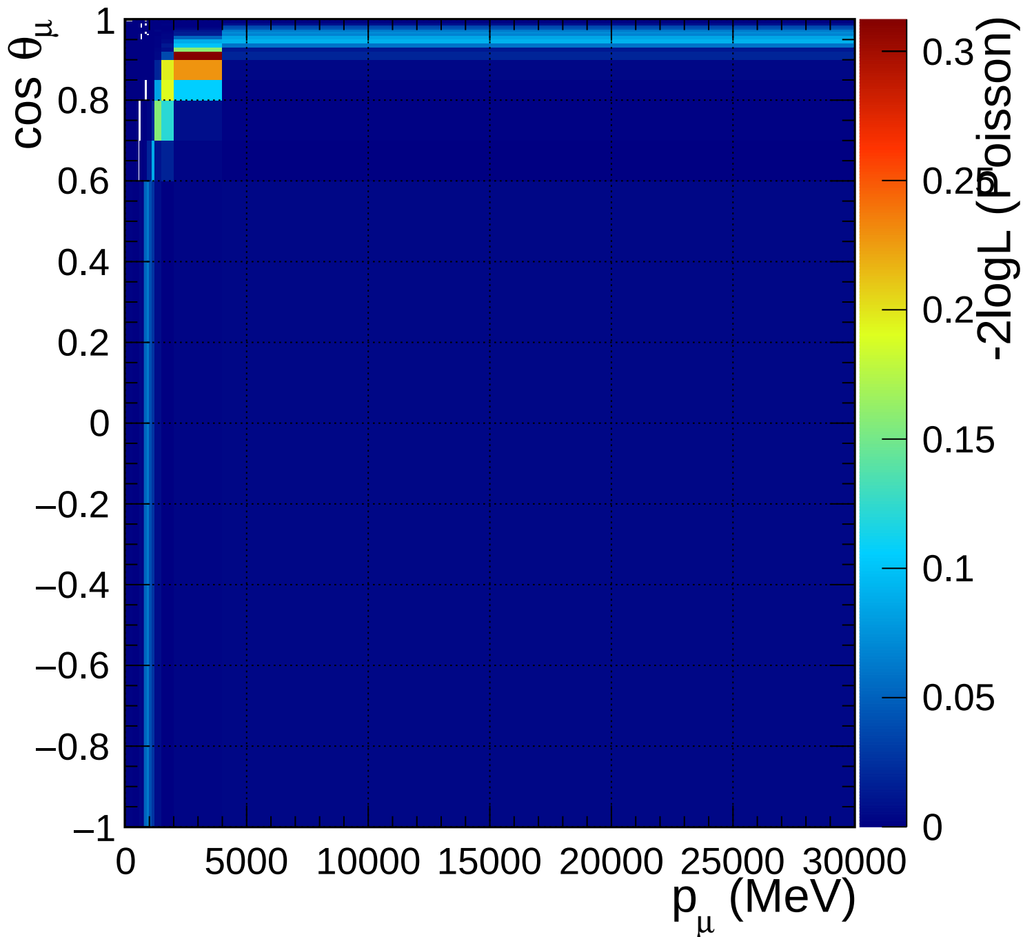
FGD1_anti-numuCC_0pi_Q2_norm_7_2.2
