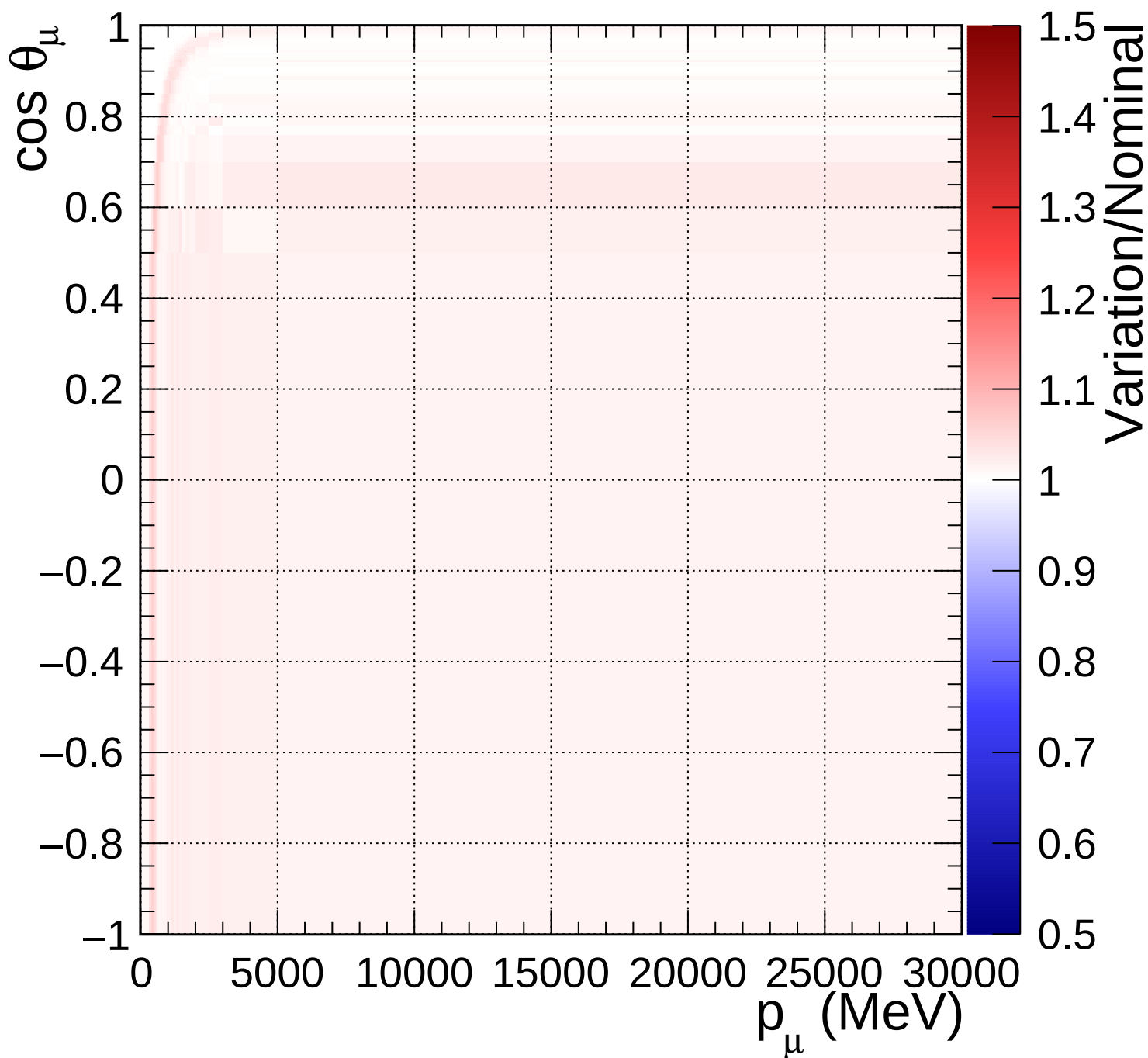
FGD1_numuCC_0pi_Q2_norm_5_1.11
