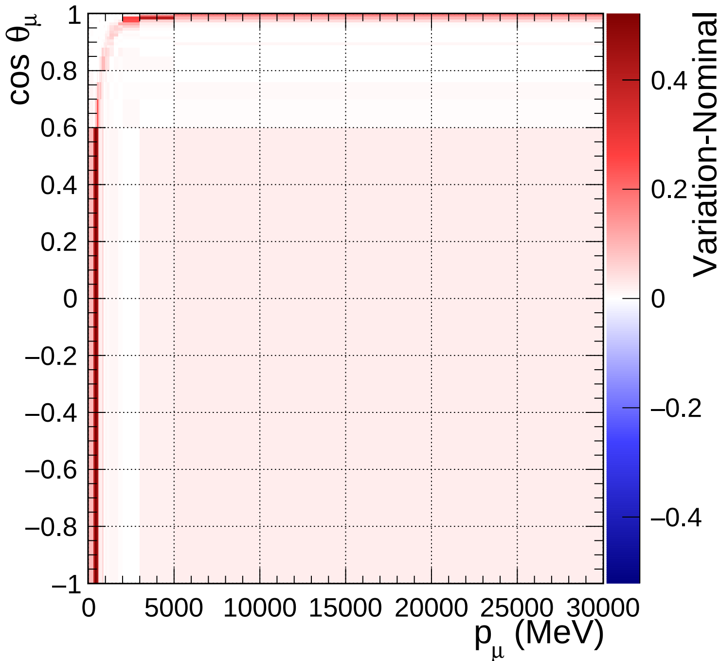
FGD1_numuCC_other_Q2_norm_5_1.11
