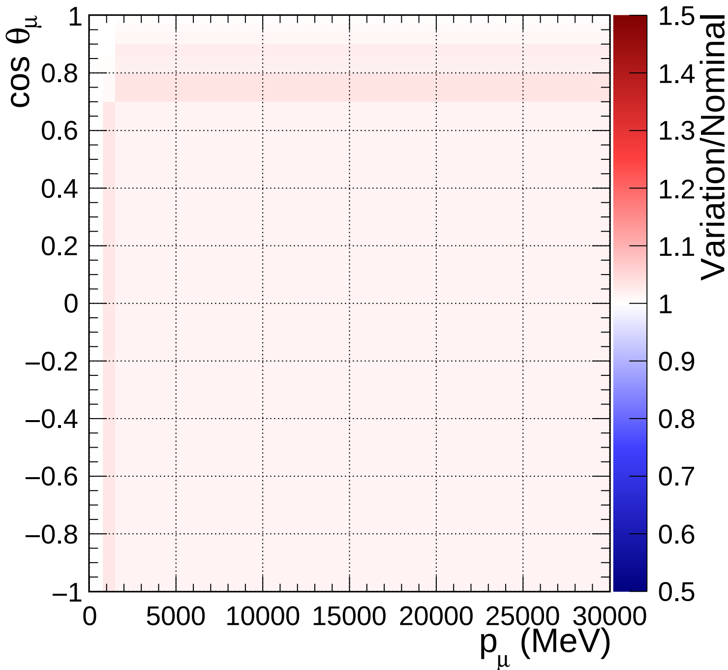
FGD1_NuMuBkg_CC1pi_in_AntiNu_Mode_Q2_norm_7_1.4
