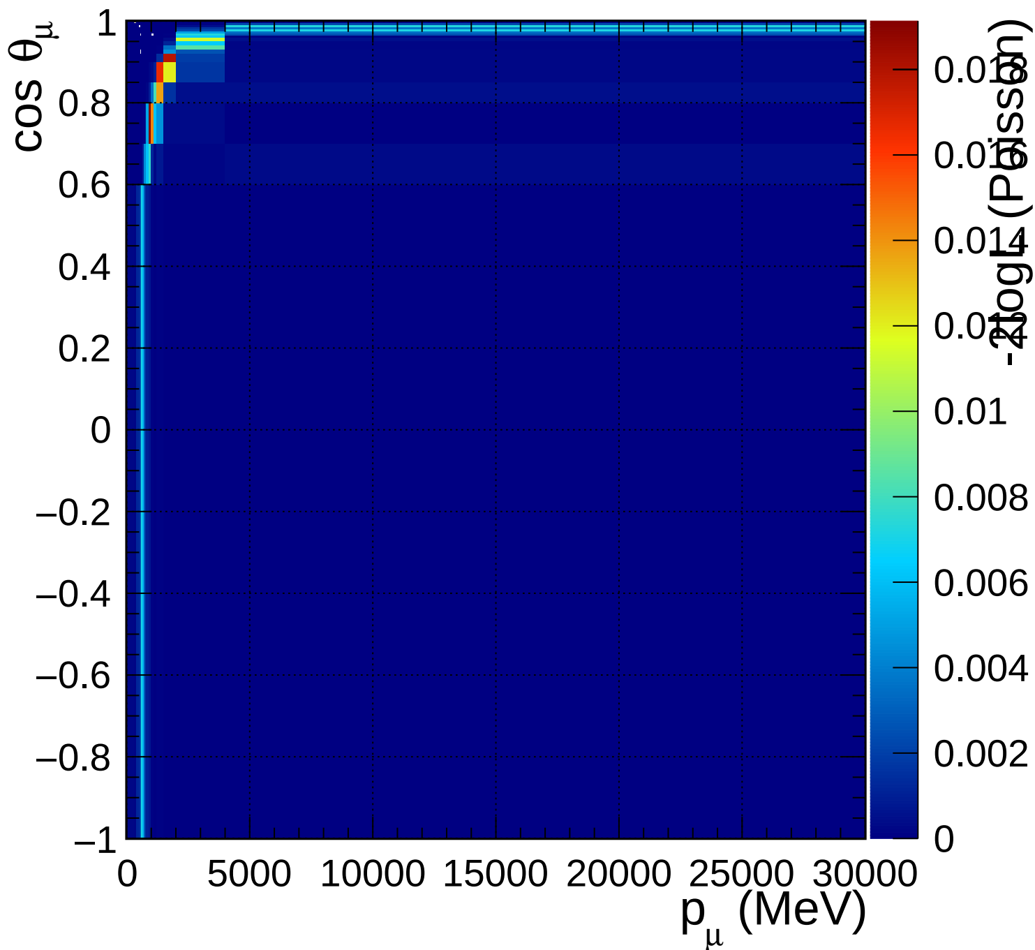
FGD2_anti-numuCC_0pi_Q2_norm_6_1.18
