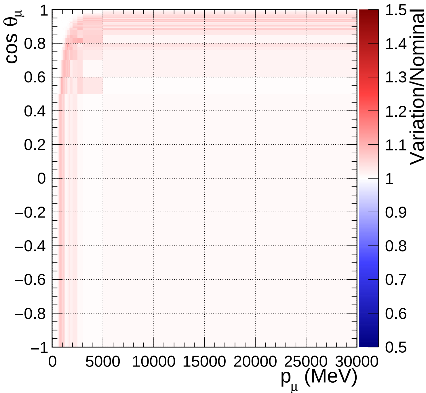
FGD2_numuCC_0pi_Q2_norm_7_1.4
