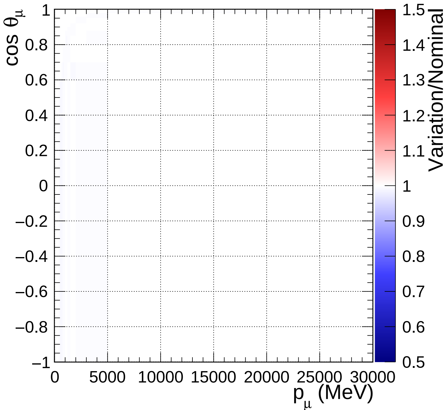
FGD1_numuCC_1pi_Q2_norm_6_0.82
