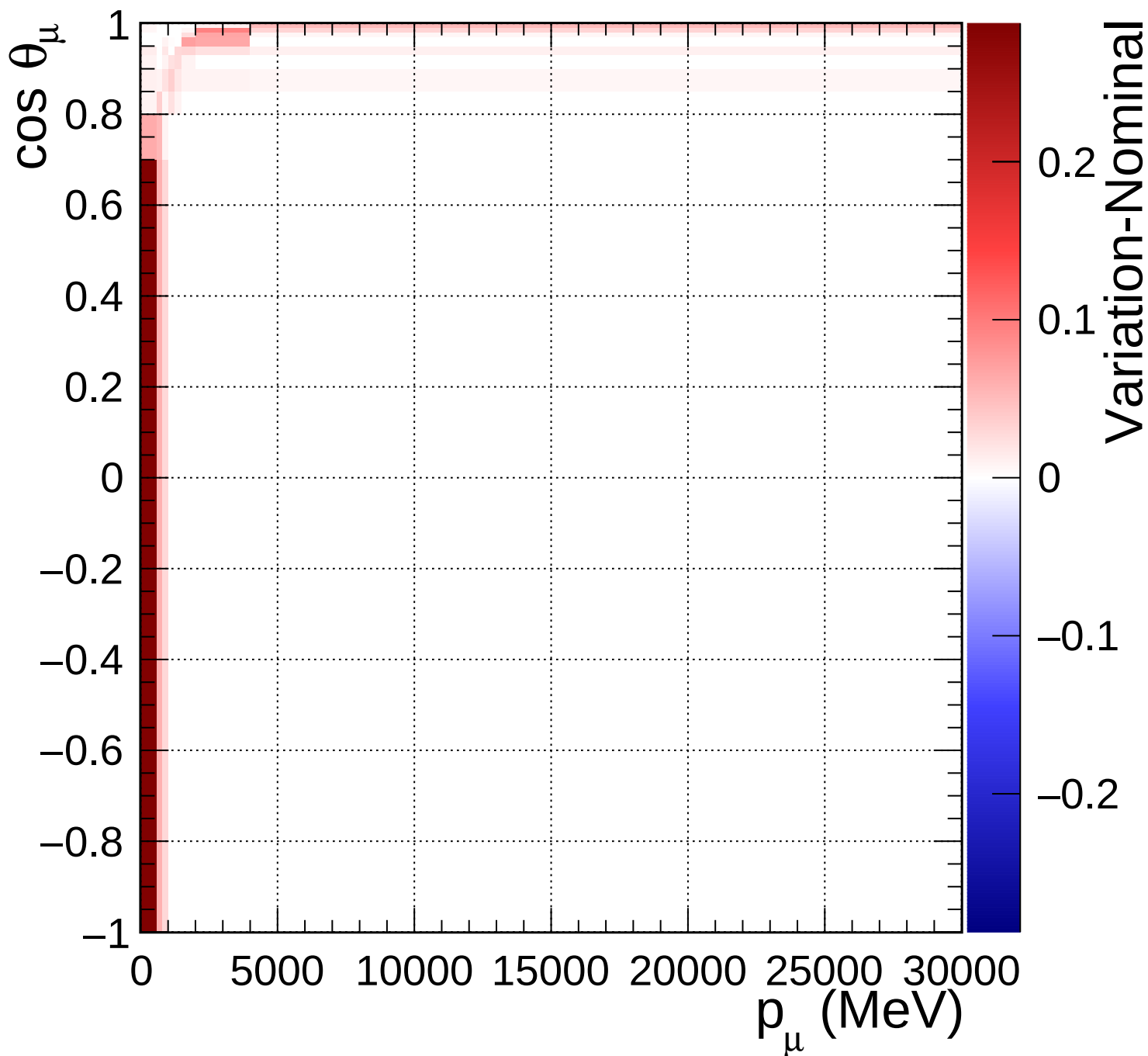
FGD1_anti-numuCC_other_Q2_norm_5_1.11
