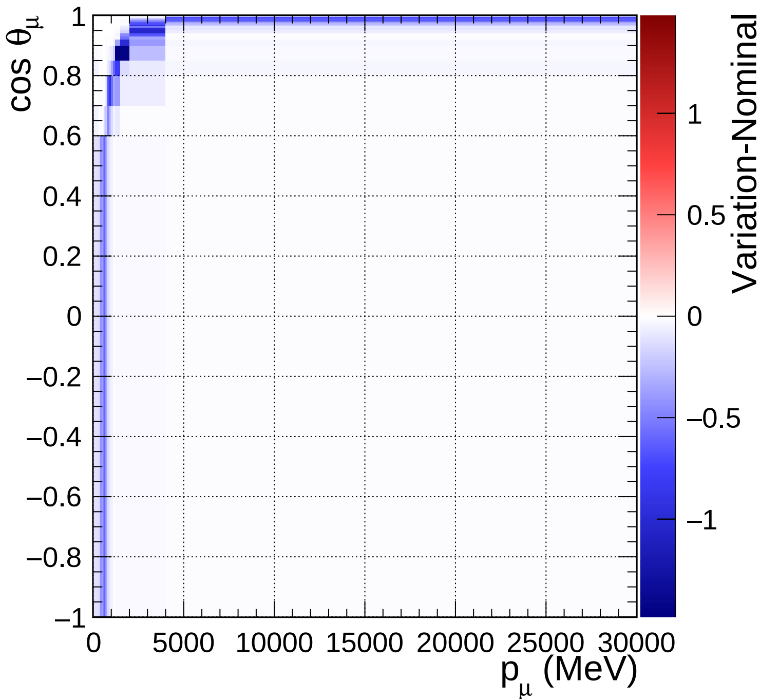
FGD1_anti-numuCC_0pi_Q2_norm_6_0.82
