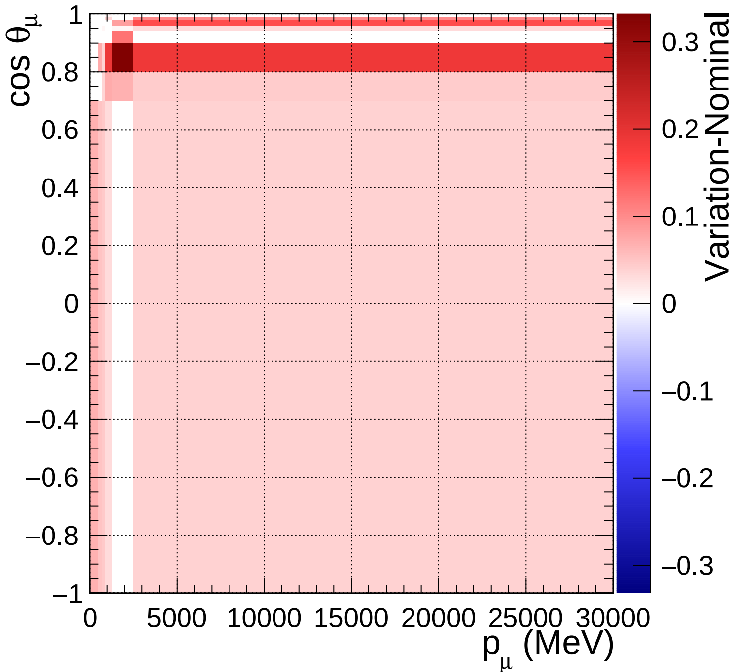
FGD2_anti-numuCC_1pi_Q2_norm_6_1.54
