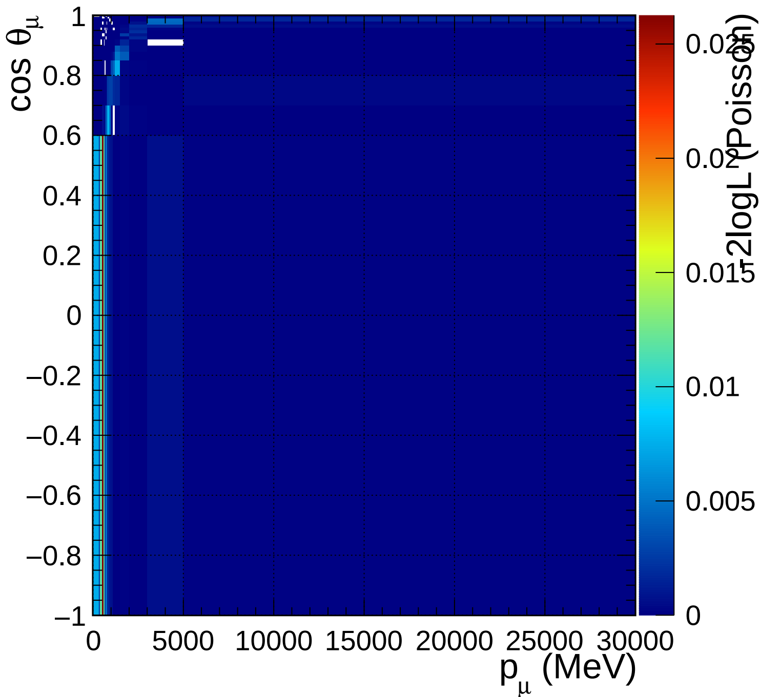
FGD2_numuCC_1pi_Q2_norm_6_1.54
