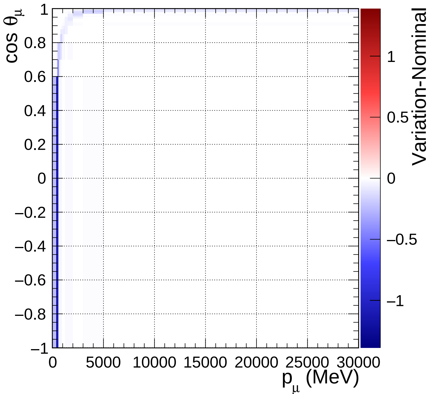
FGD1_numuCC_1pi_Q2_norm_5_0.89
