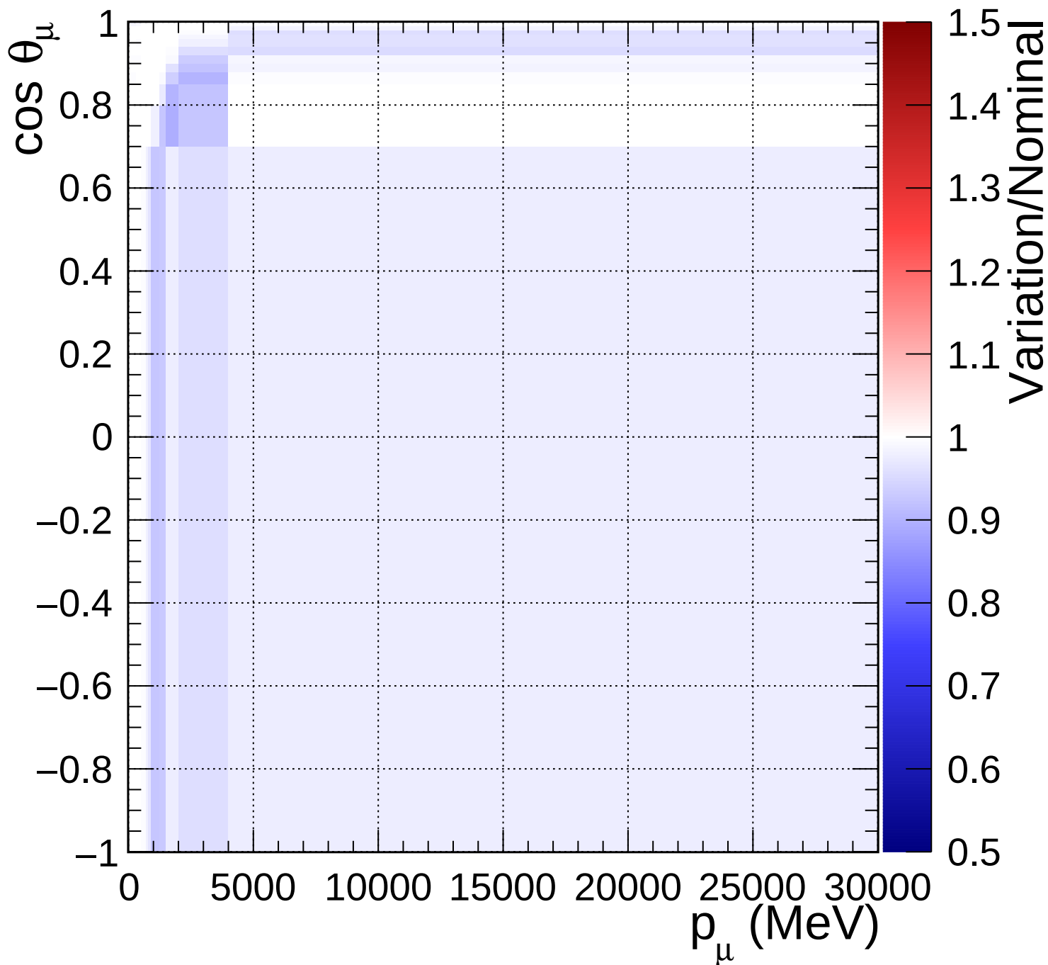
FGD1_NuMuBkg_CC0pi_in_AntiNu_Mode_Q2_norm_7_0.6
