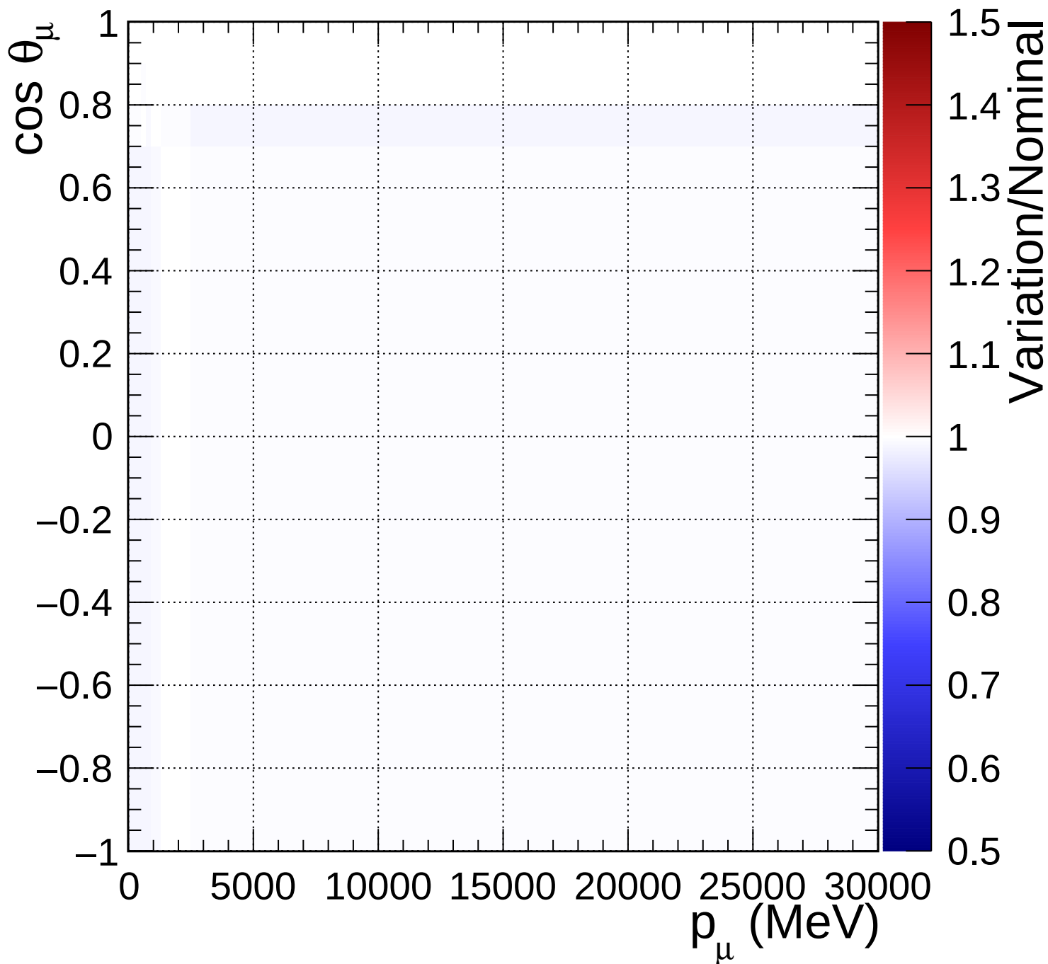
FGD2_anti-numuCC_1pi_Q2_norm_5_0.67
