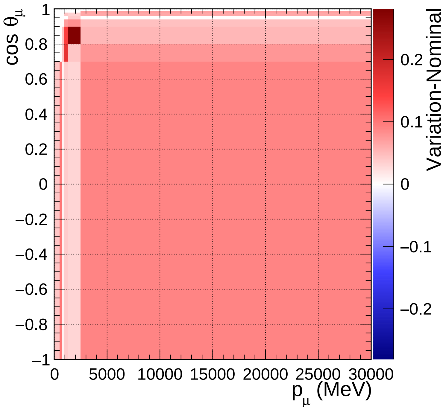
FGD1_anti-numuCC_1pi_Q2_norm_6_1.54
