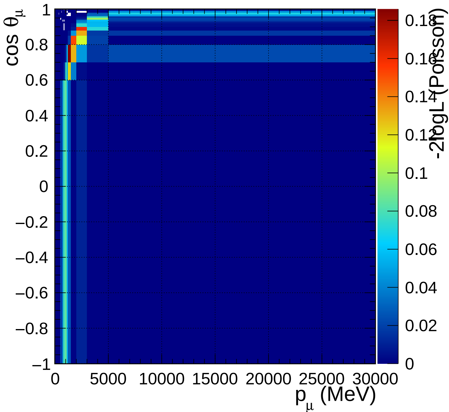
FGD1_numuCC_1pi_Q2_norm_7_2.2
