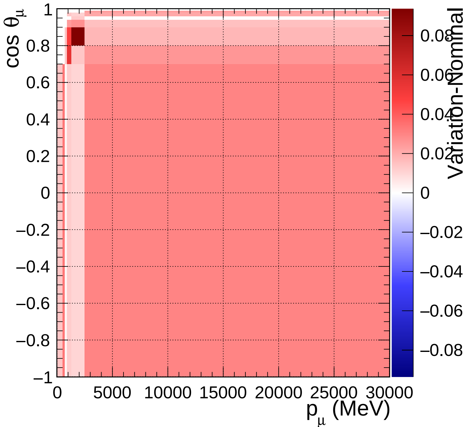
FGD1_anti-numuCC_1pi_Q2_norm_6_1.18
