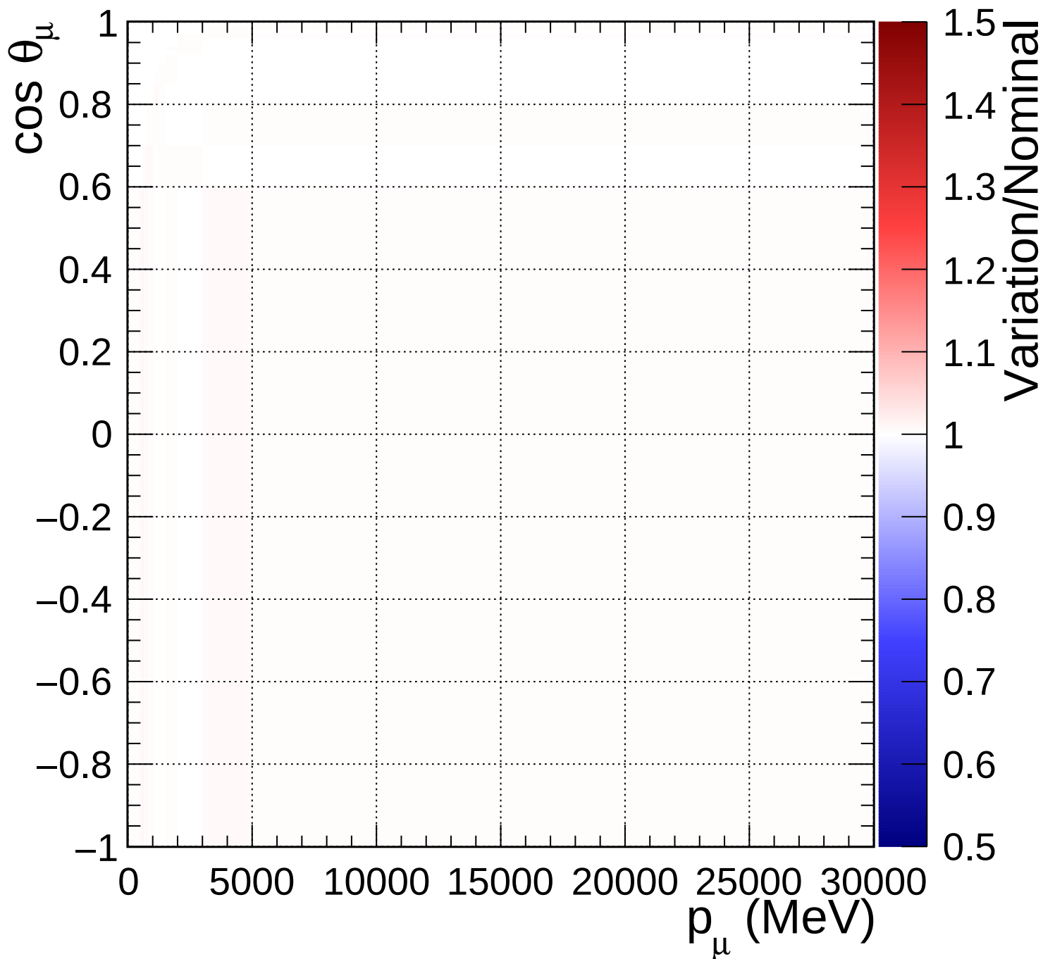
FGD2_numuCC_1pi_Q2_norm_6_1.18
