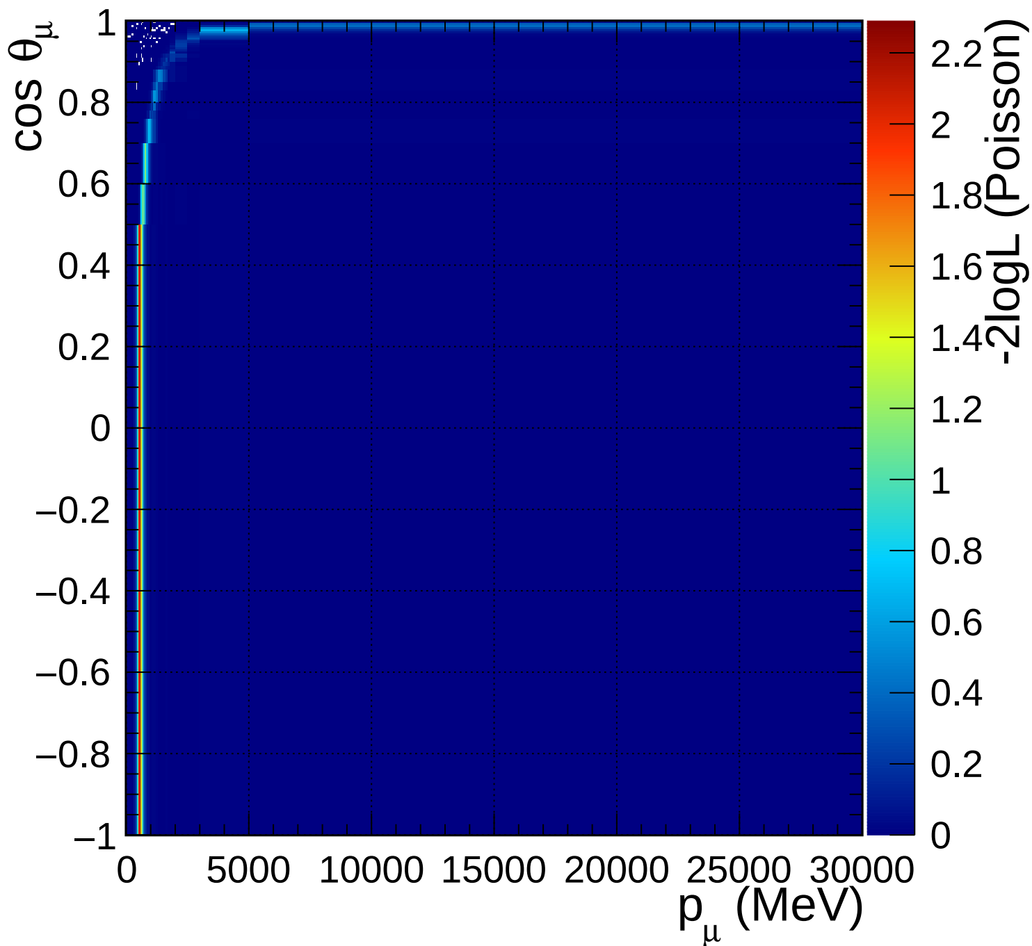
FGD1_numuCC_0pi_Q2_norm_6_0.46
