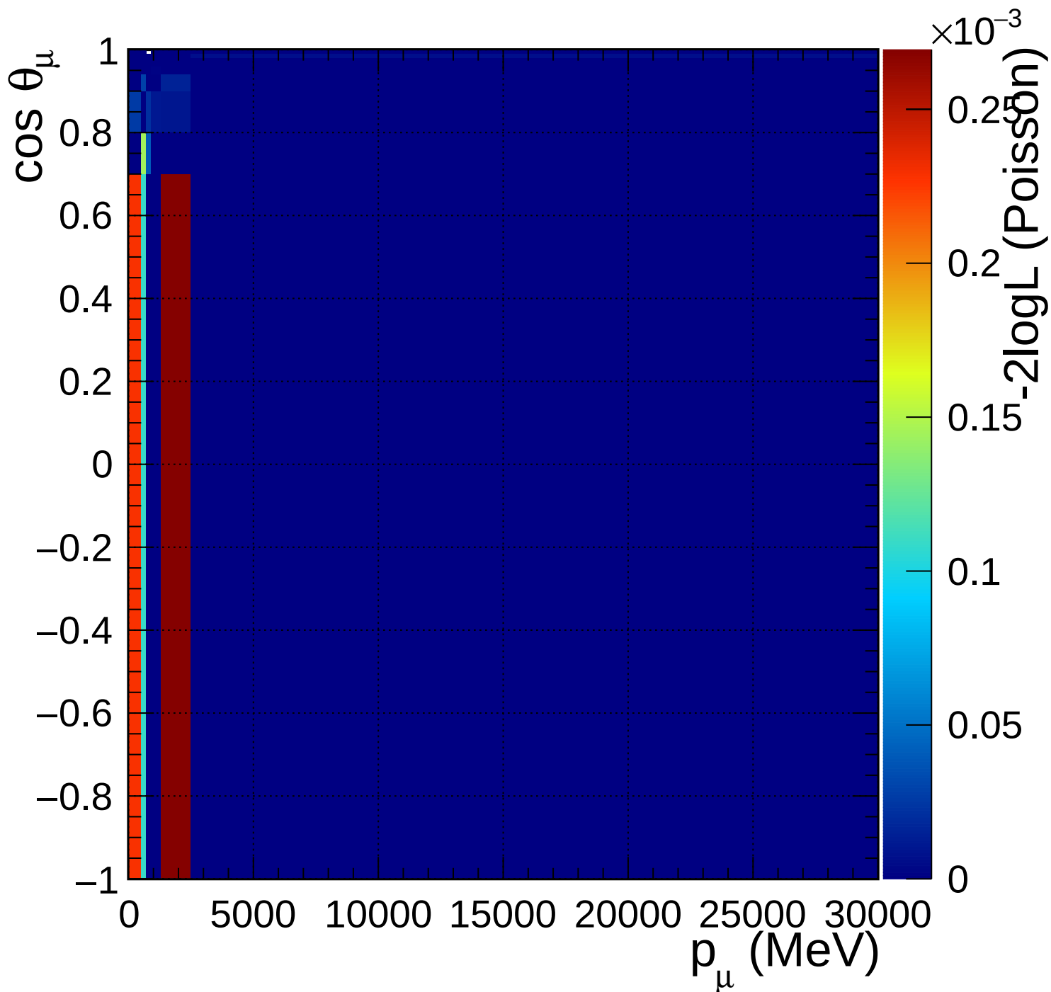
FGD1_anti-numuCC_1pi_Q2_norm_5_1.33
