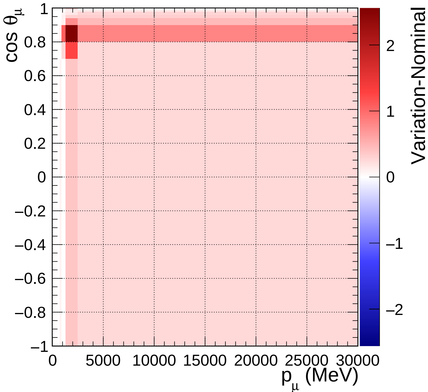
FGD2_anti-numuCC_1pi_Q2_norm_7_2.2
