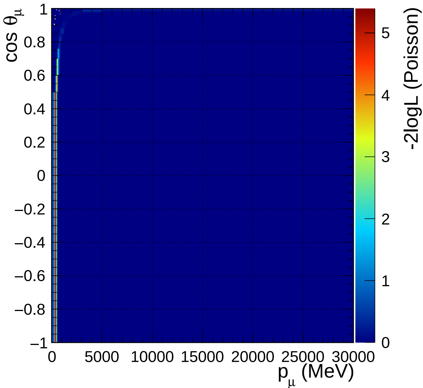
FGD2_numuCC_0pi_Q2_norm_5_0.67
