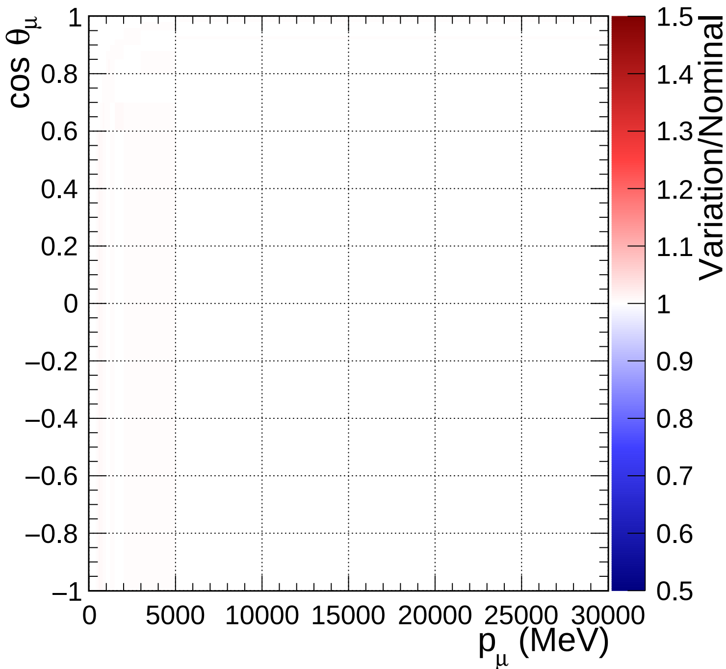
FGD1_numuCC_1pi_Q2_norm_6_1.18
