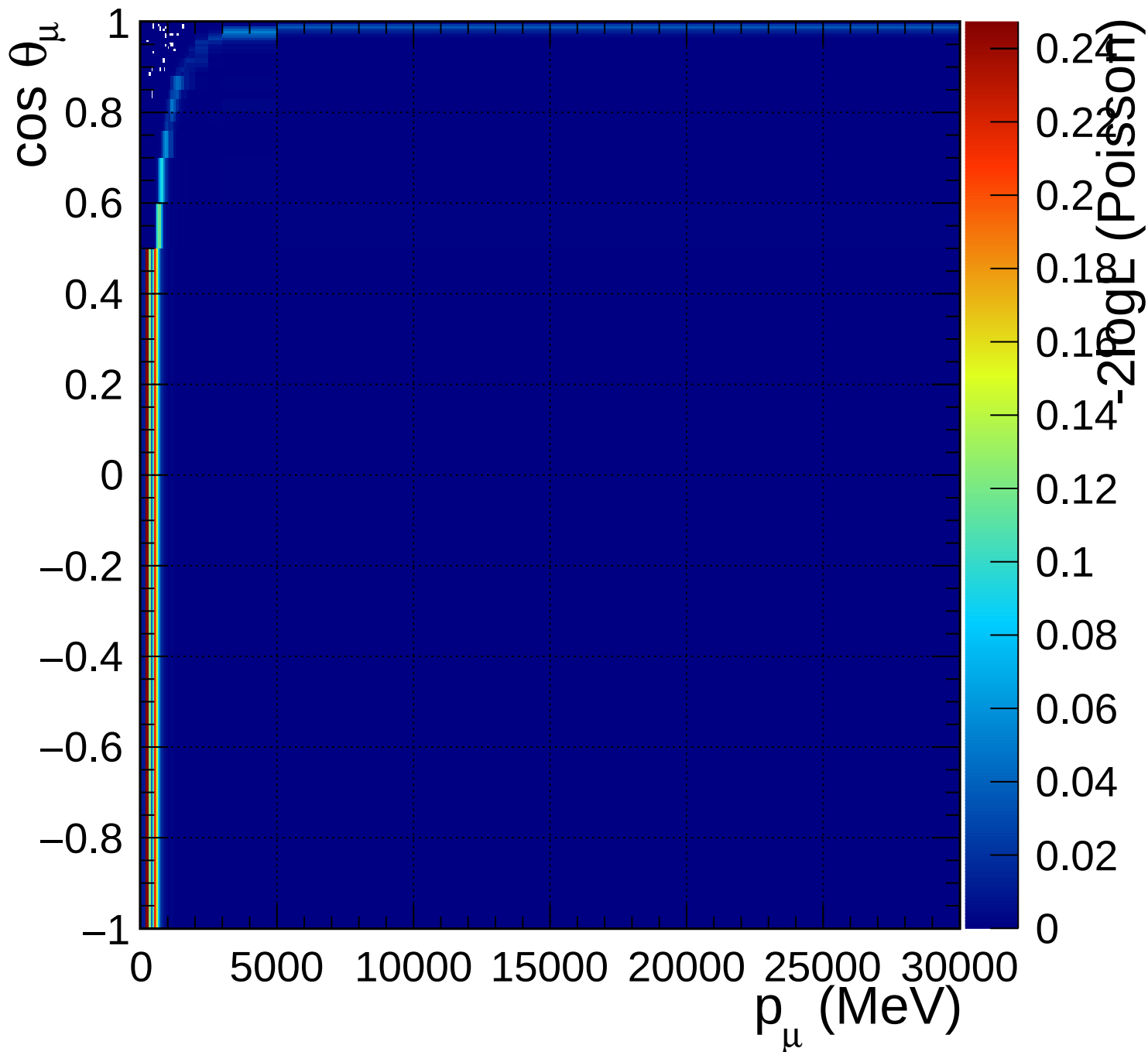
FGD2_numuCC_0pi_Q2_norm_6_0.82
