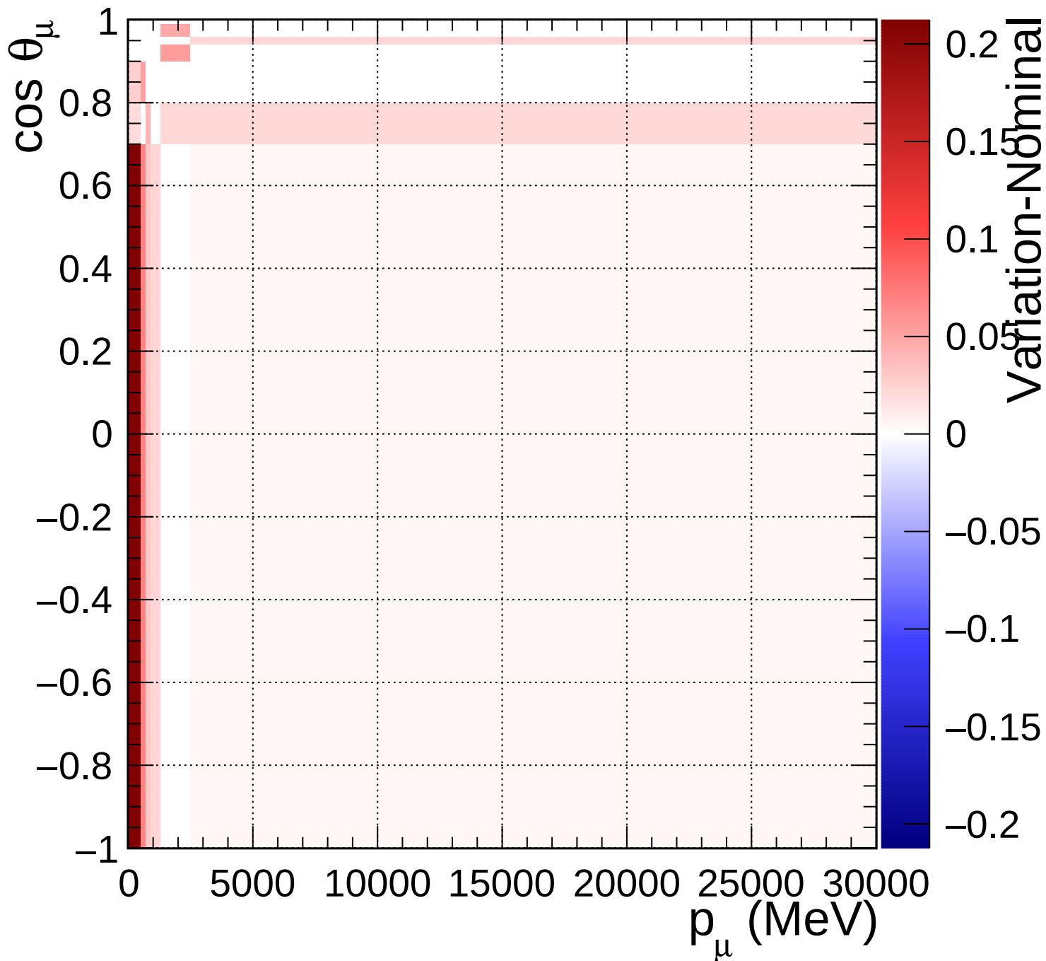
FGD2_anti-numuCC_1pi_Q2_norm_5_1.33
