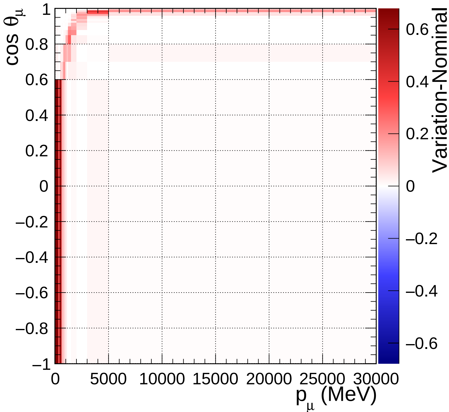
FGD2_numuCC_1pi_Q2_norm_6_1.18
