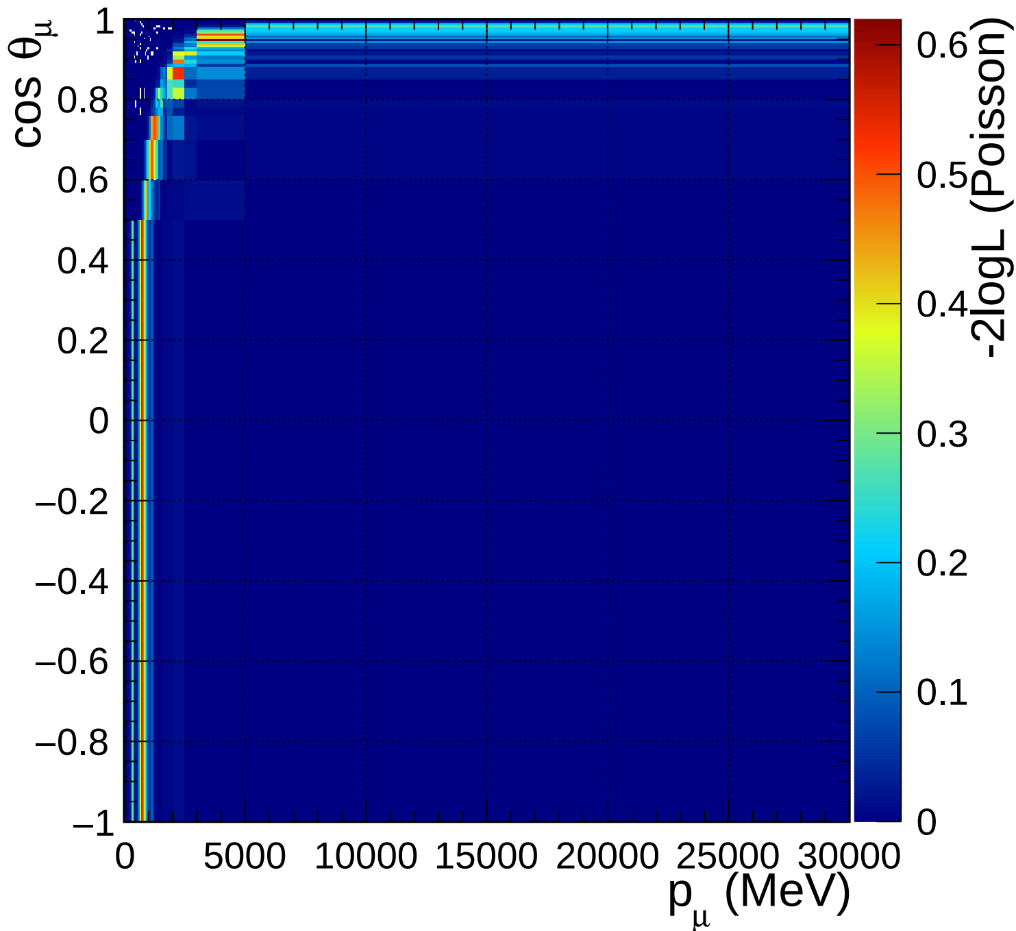
FGD2_numuCC_0pi_Q2_norm_7_2.2
