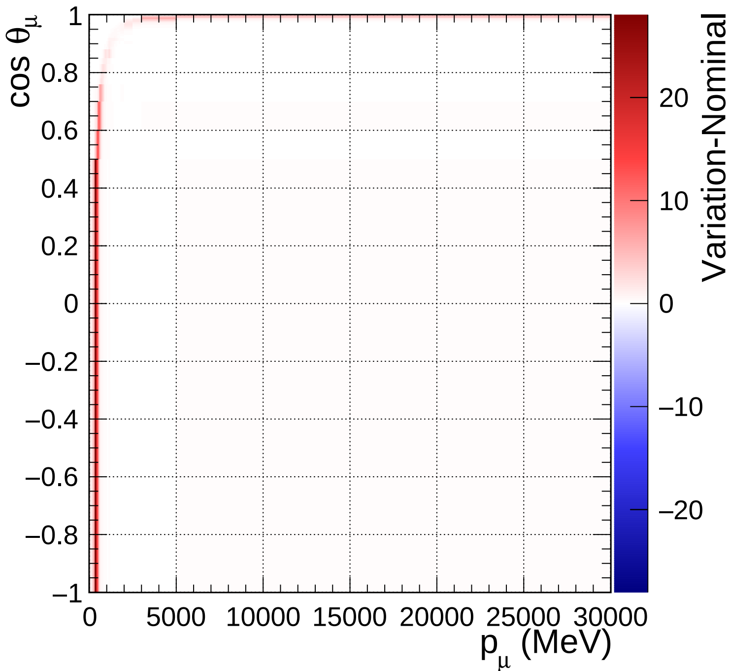
FGD1_numuCC_0pi_Q2_norm_5_1.11
