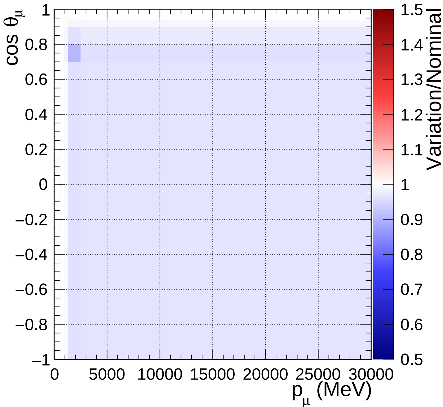
FGD1_anti-numuCC_1pi_Q2_norm_7_0.6
