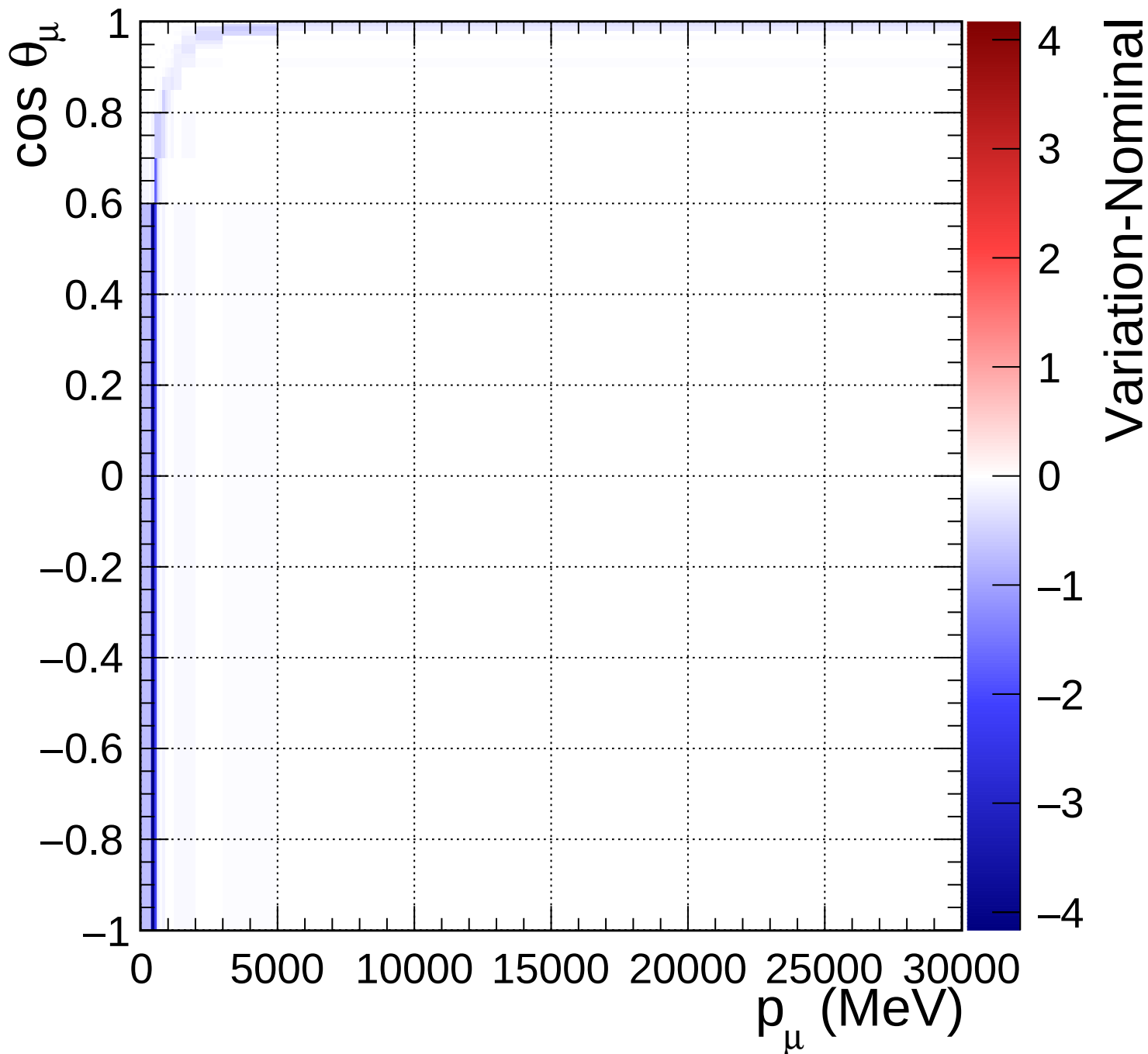
FGD1_numuCC_1pi_Q2_norm_5_0.67
