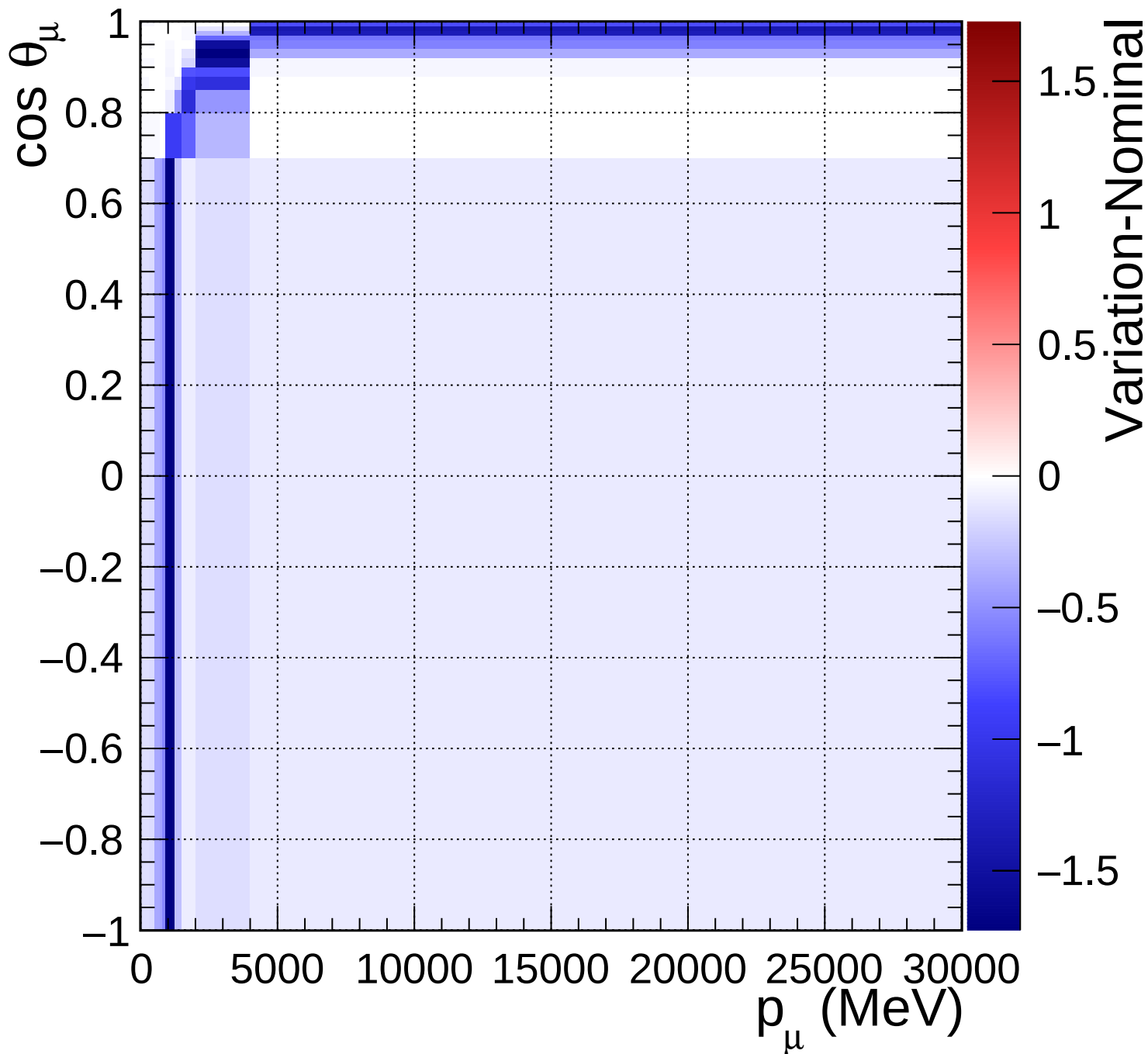
FGD1_NuMuBkg_CC0pi_in_AntiNu_Mode_Q2_norm_7_0.6
