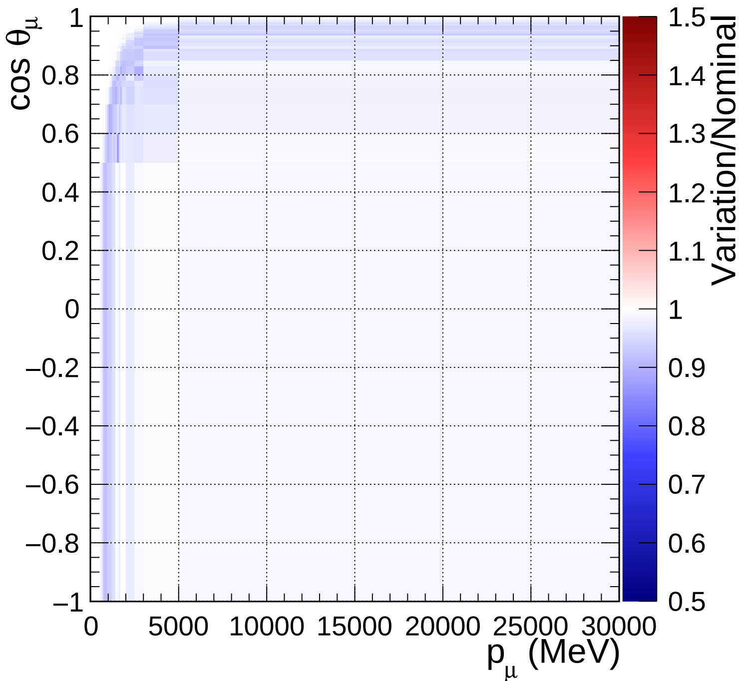
FGD1_numuCC_0pi_Q2_norm_7_0.6
