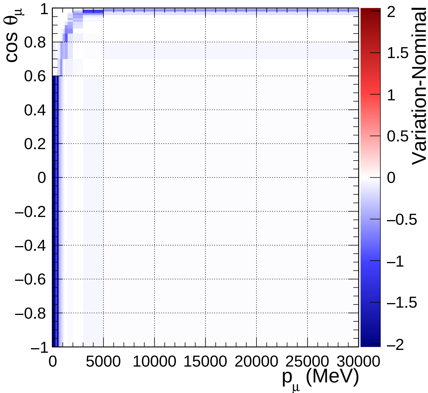
FGD2_numuCC_1pi_Q2_norm_6_0.46
