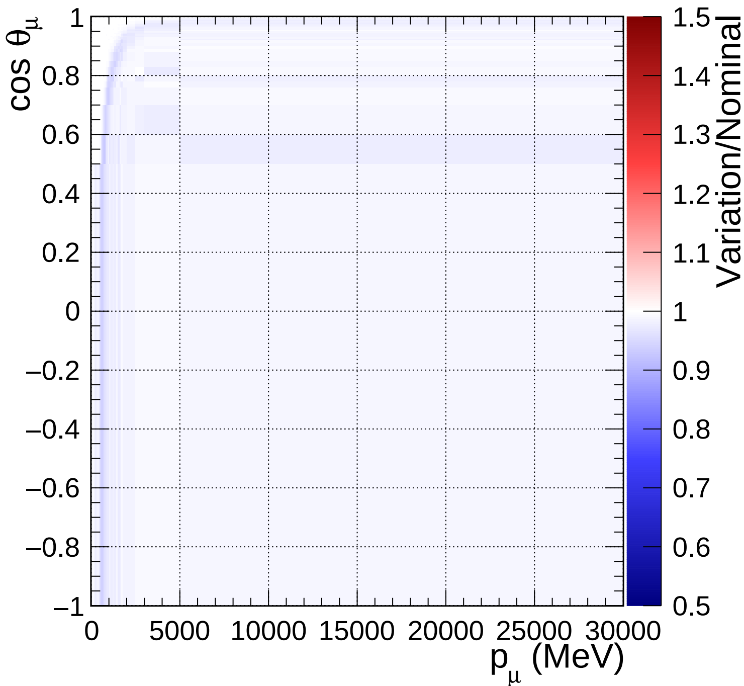
FGD2_numuCC_0pi_Q2_norm_6_0.82
