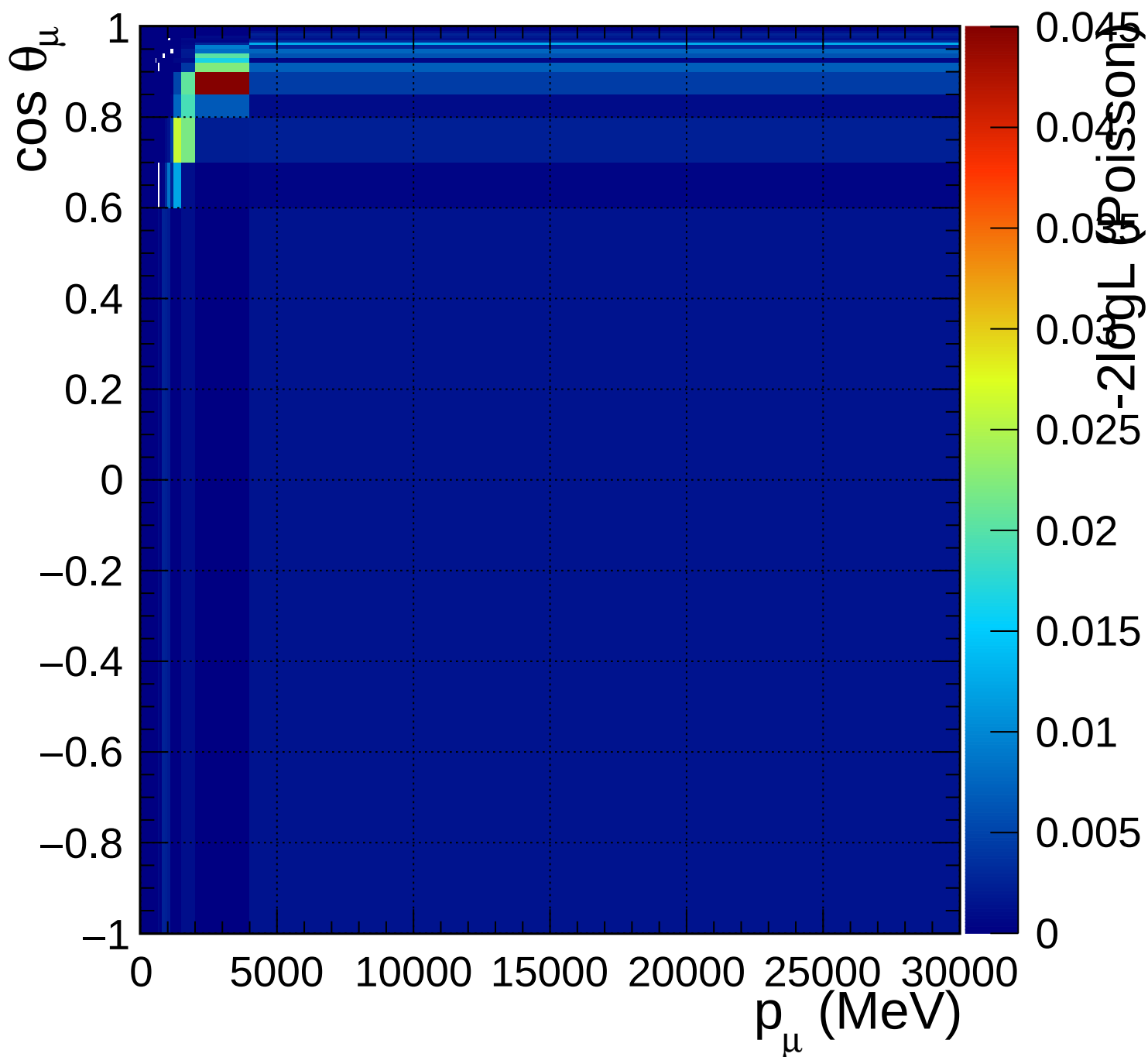
FGD2_anti-numuCC_0pi_Q2_norm_7_1.4
