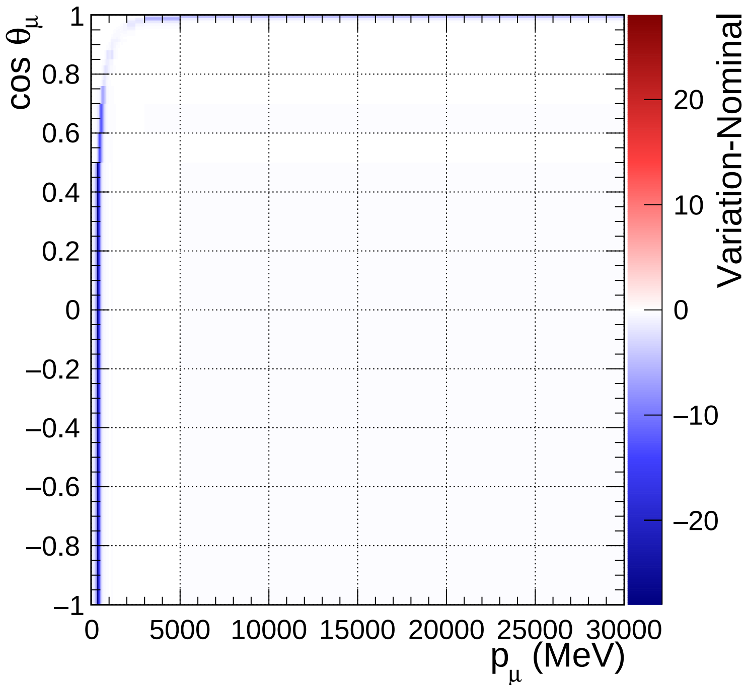
FGD1_numuCC_0pi_Q2_norm_5_0.89
