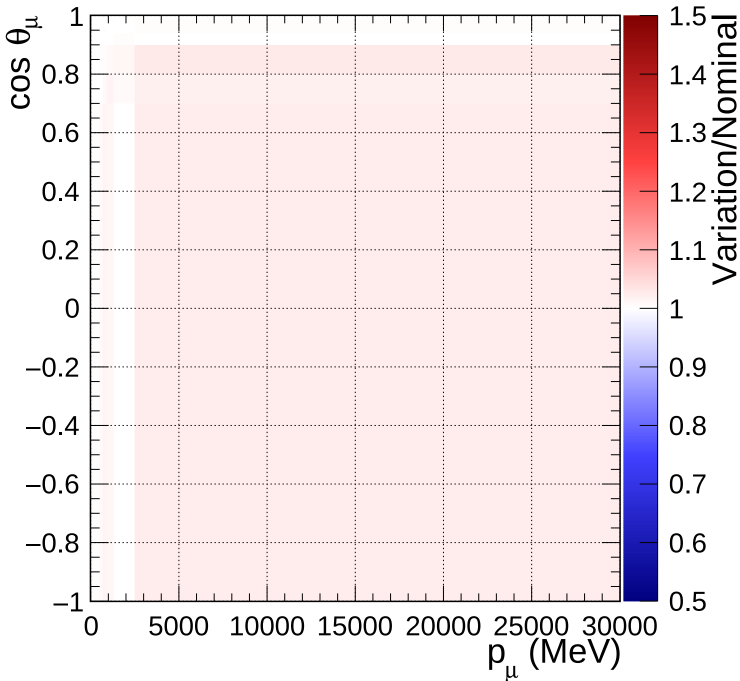
FGD2_anti-numuCC_1pi_Q2_norm_6_1.54
