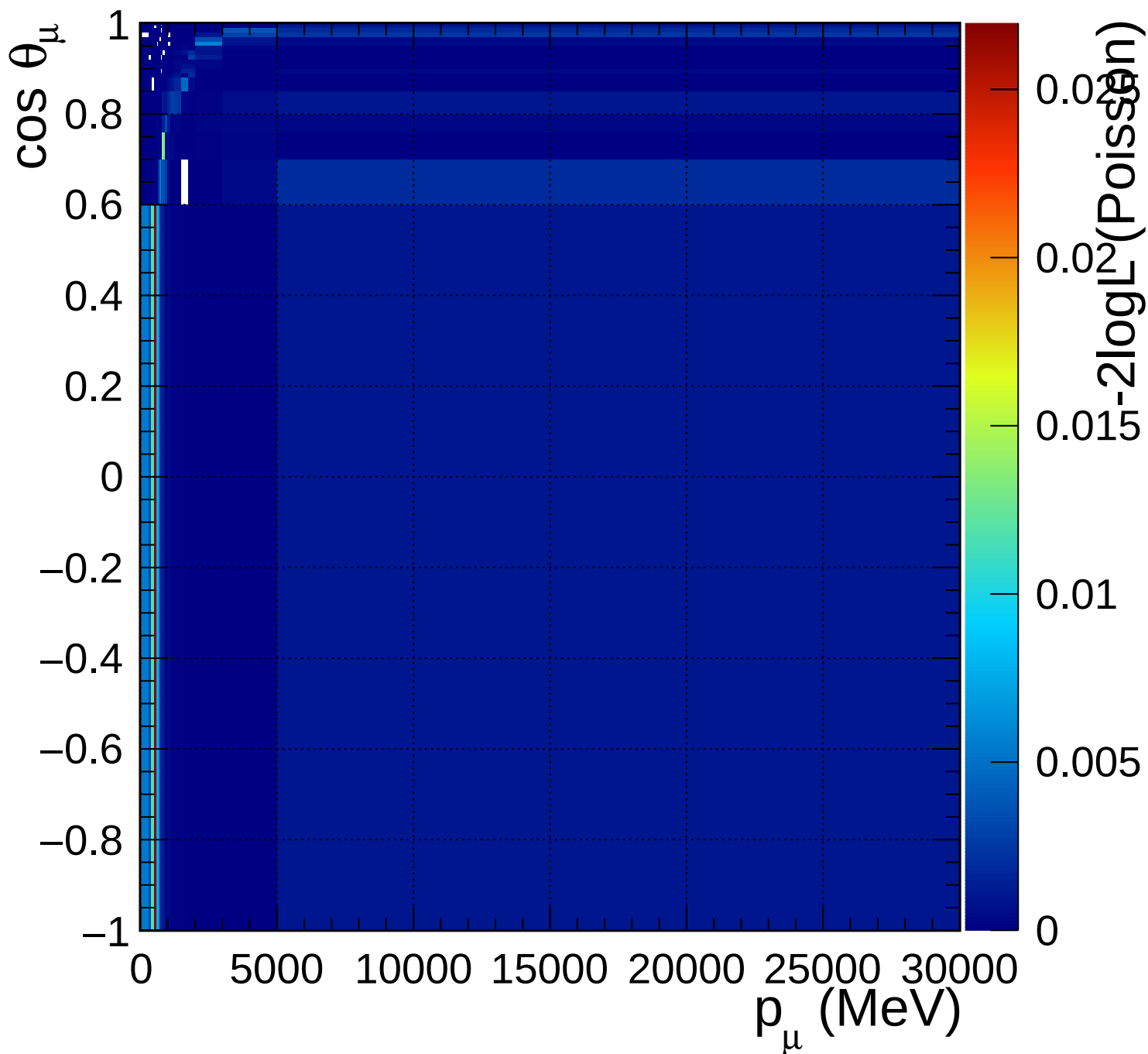
FGD2_numuCC_other_Q2_norm_6_0.46
