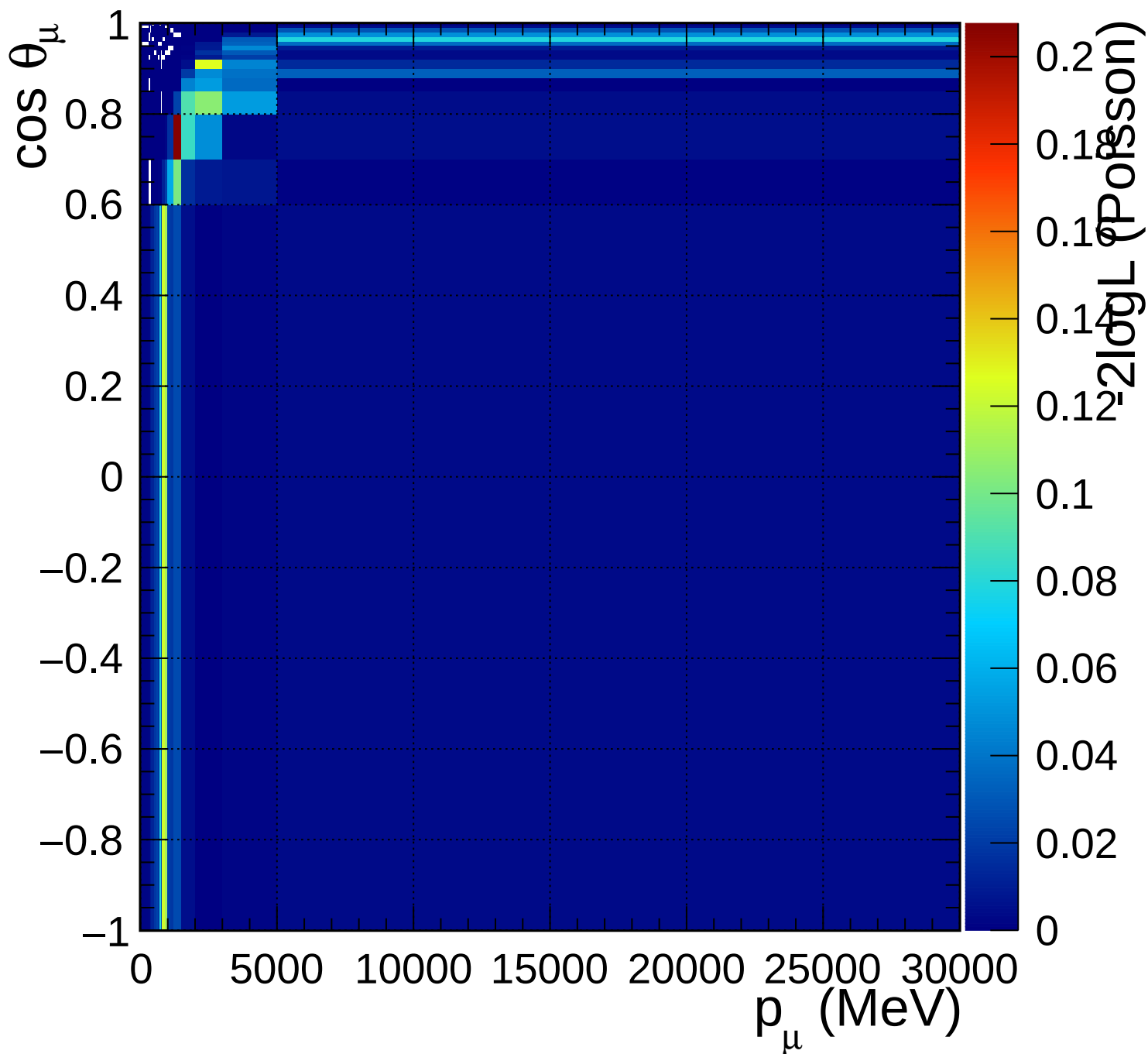
FGD2_numuCC_1pi_Q2_norm_7_2.2
