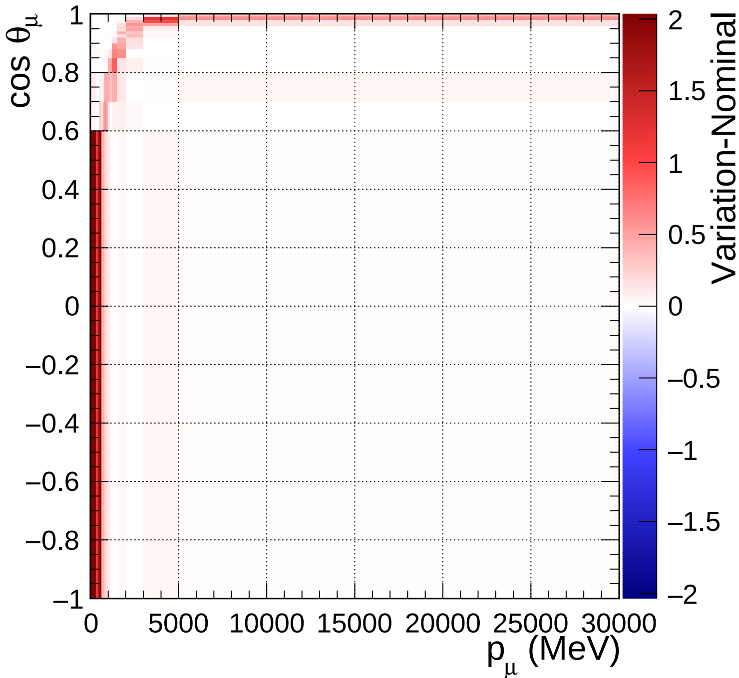
FGD2_numuCC_1pi_Q2_norm_6_1.54
