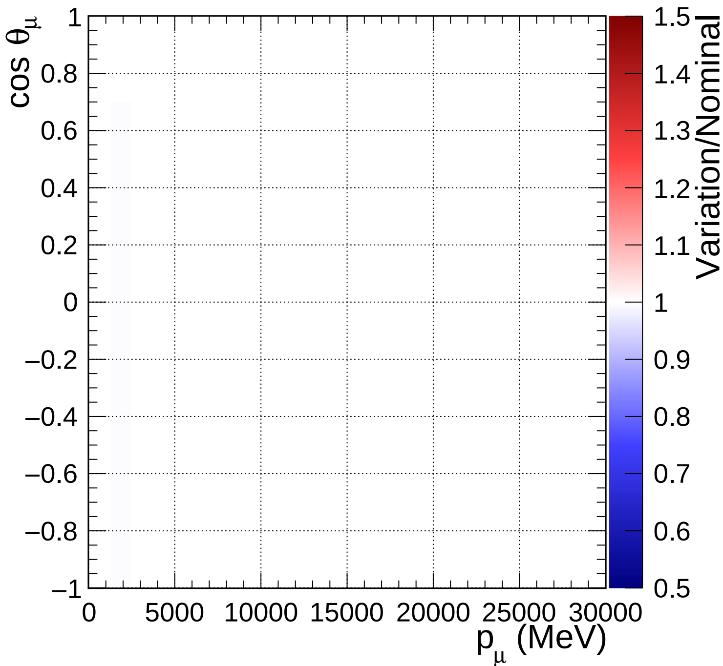
FGD1_anti-numuCC_1pi_Q2_norm_5_0.89
