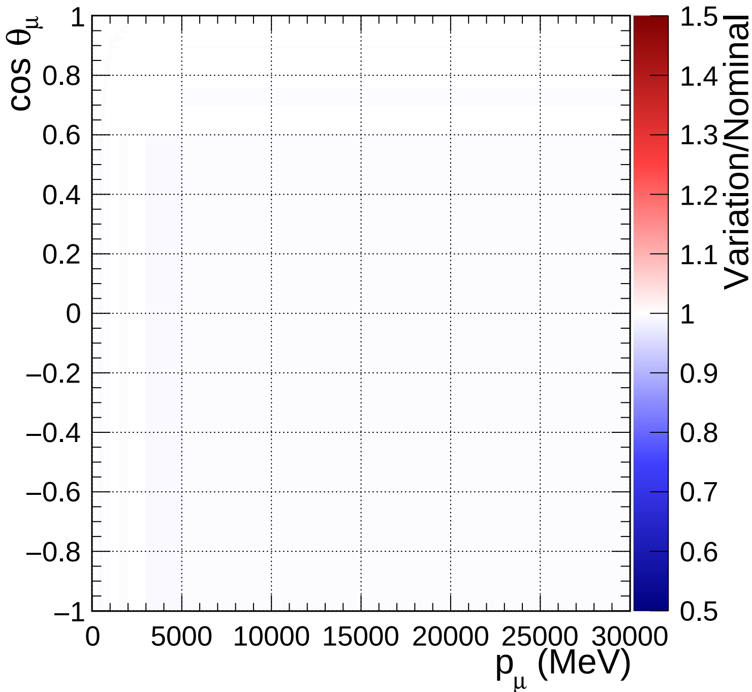
FGD1_numuCC_other_Q2_norm_5_0.89
