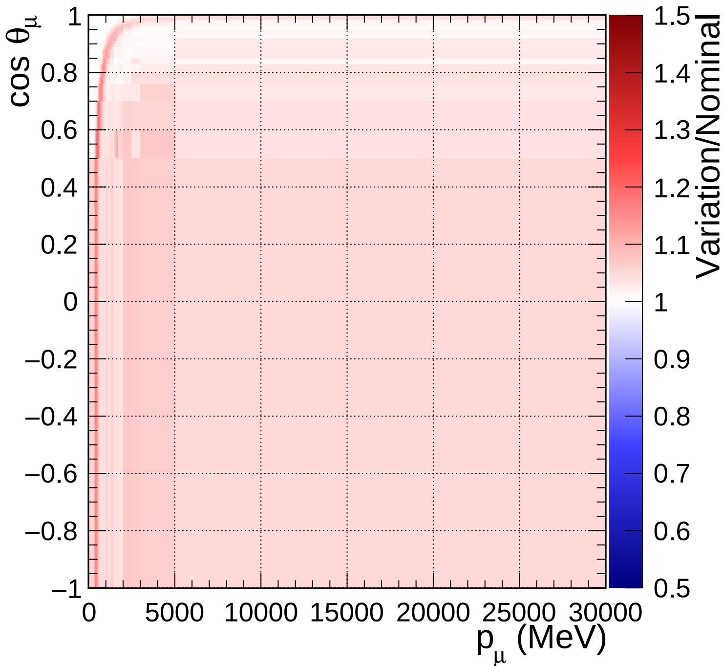
FGD2_numuCC_0pi_Q2_norm_5_1.33
