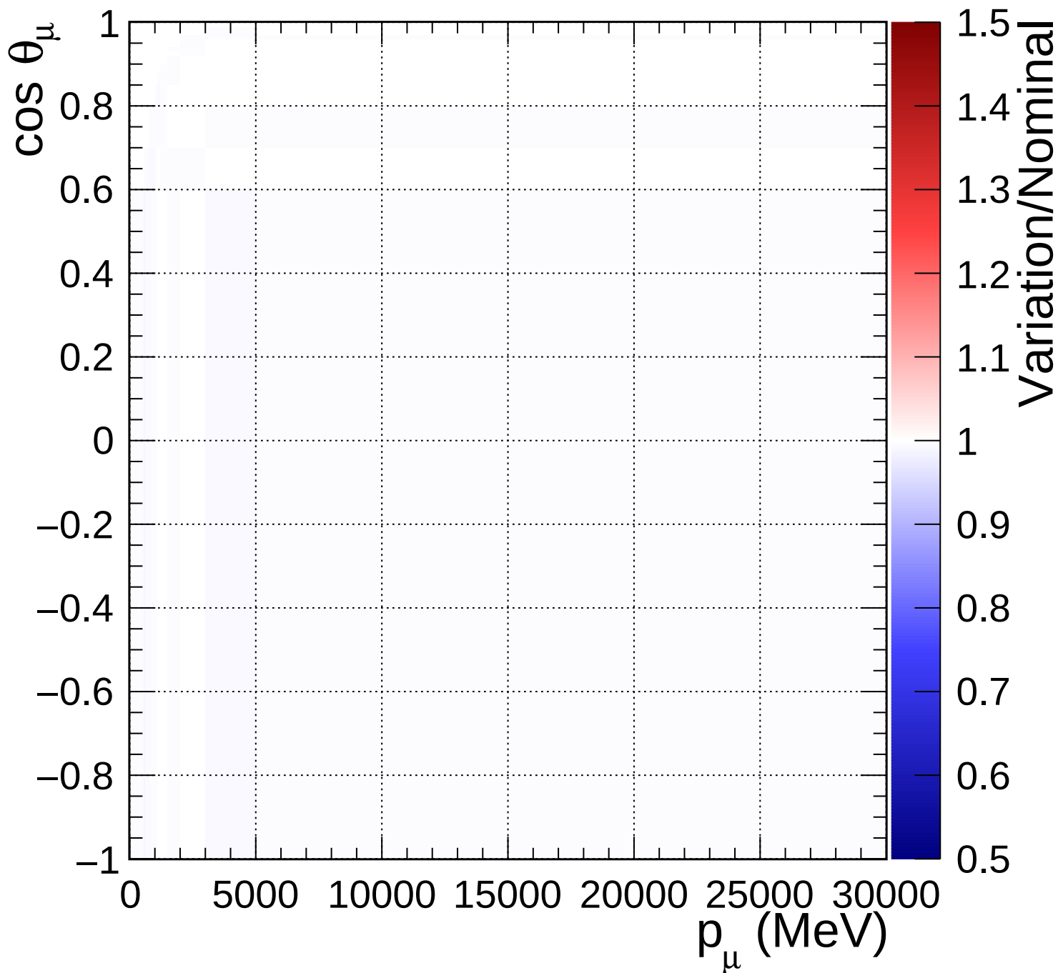
FGD2_numuCC_1pi_Q2_norm_6_0.82
