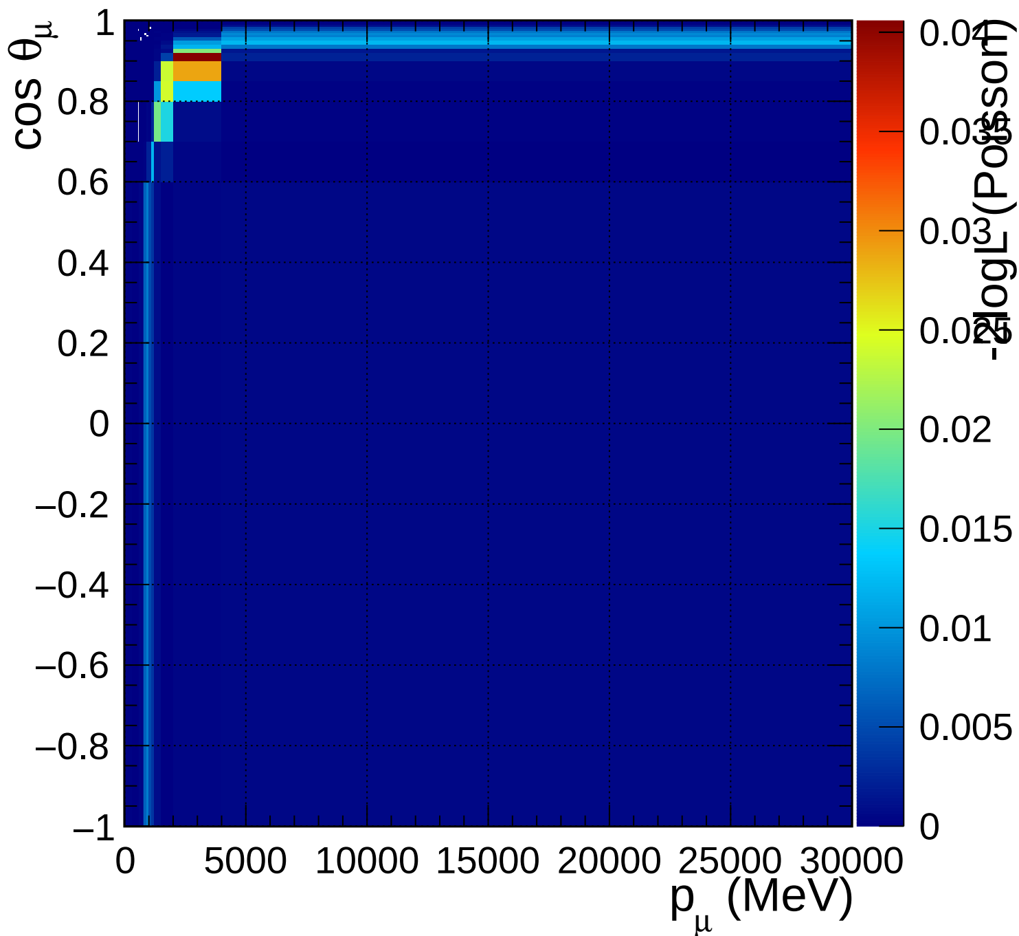
FGD1_anti-numuCC_0pi_Q2_norm_7_0.6
