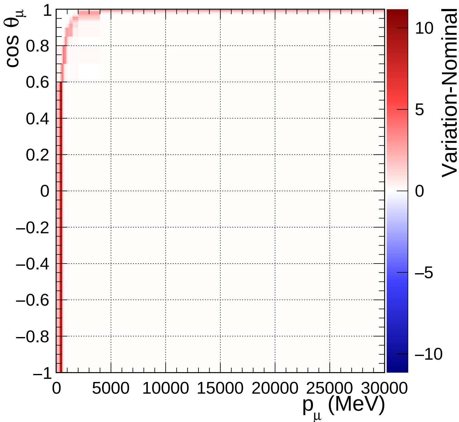
FGD2_anti-numuCC_0pi_Q2_norm_5_1.33
