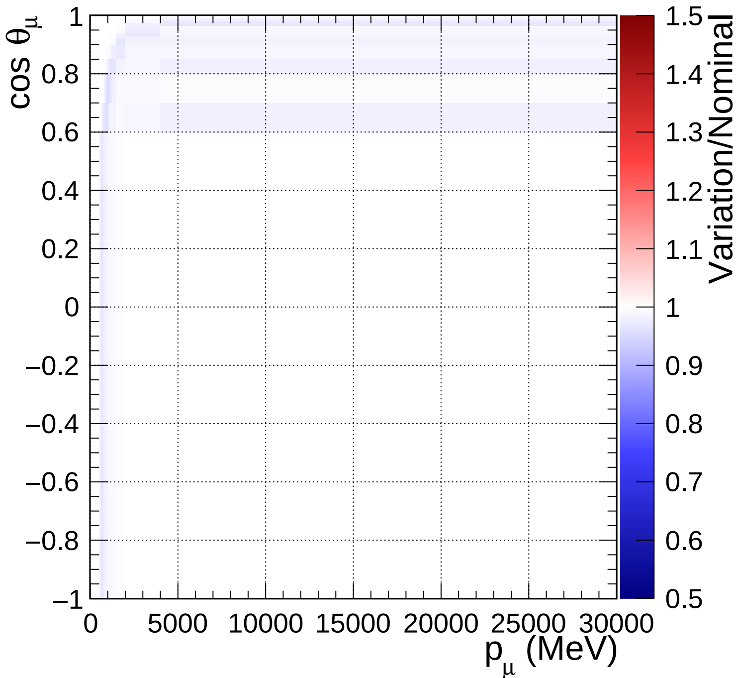
FGD2_anti-numuCC_0pi_Q2_norm_6_0.82
