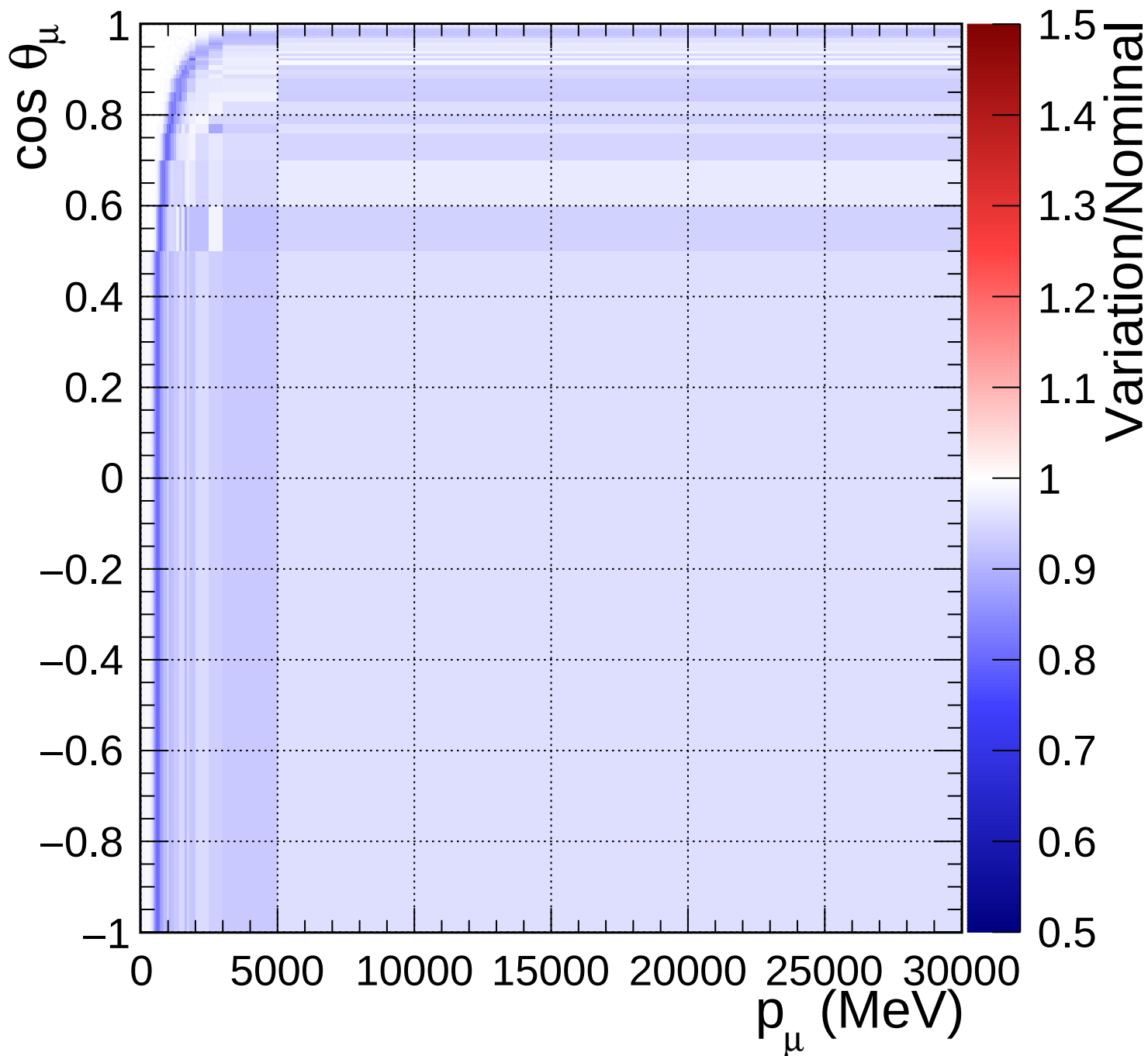
FGD1_numuCC_0pi_Q2_norm_6_0.46
