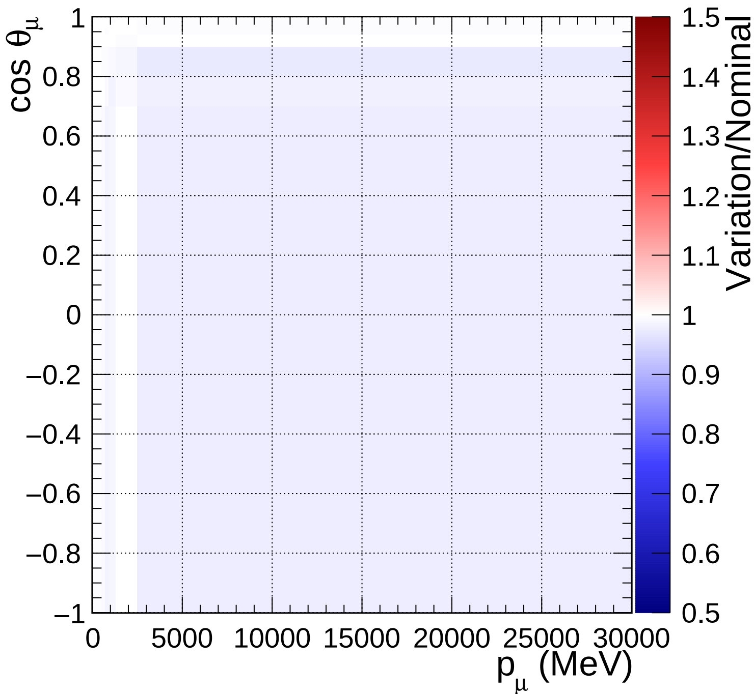
FGD2_anti-numuCC_1pi_Q2_norm_6_0.46
