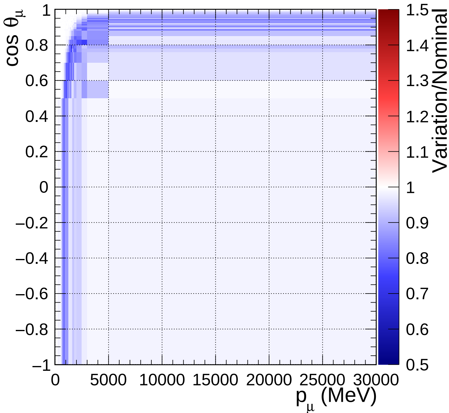
FGD2_numuCC_0pi_Q2_norm_7_-0.2
