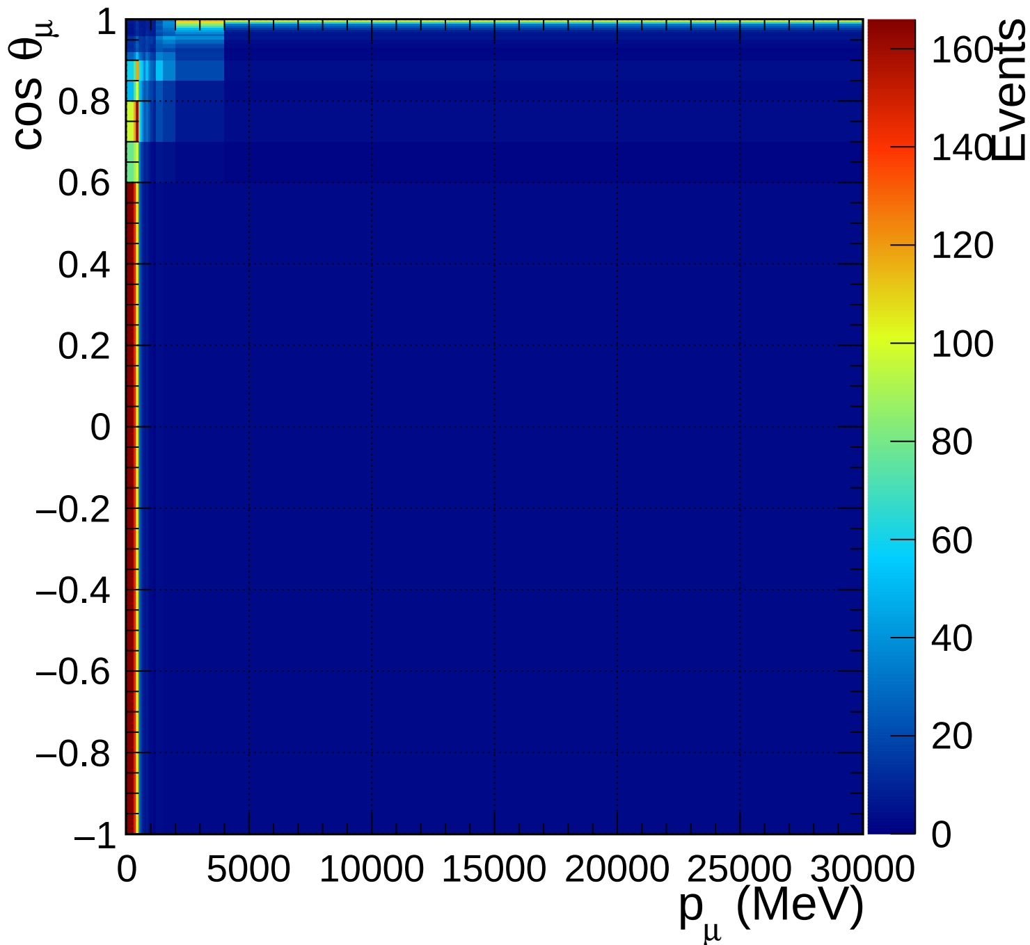
FGD2_anti-numuCC_0pi_Q2_norm_6_1
