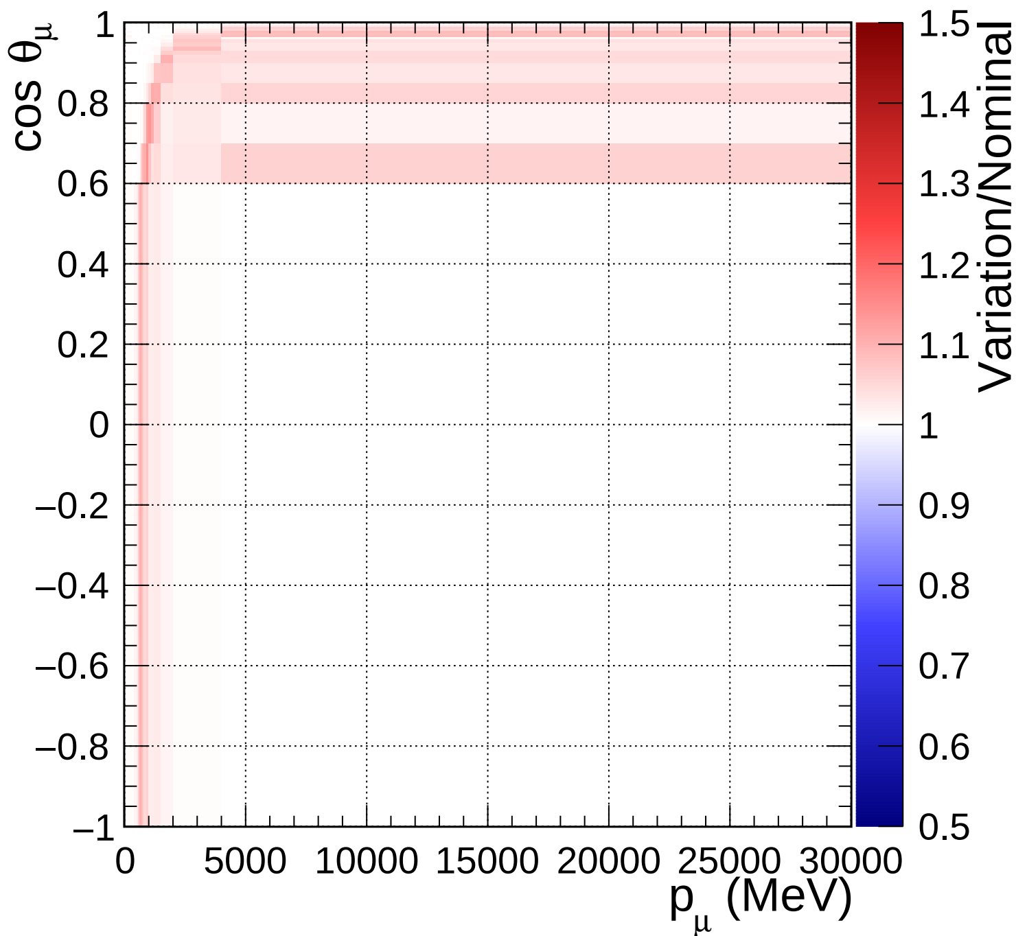
FGD2_anti-numuCC_0pi_Q2_norm_6_1.54
