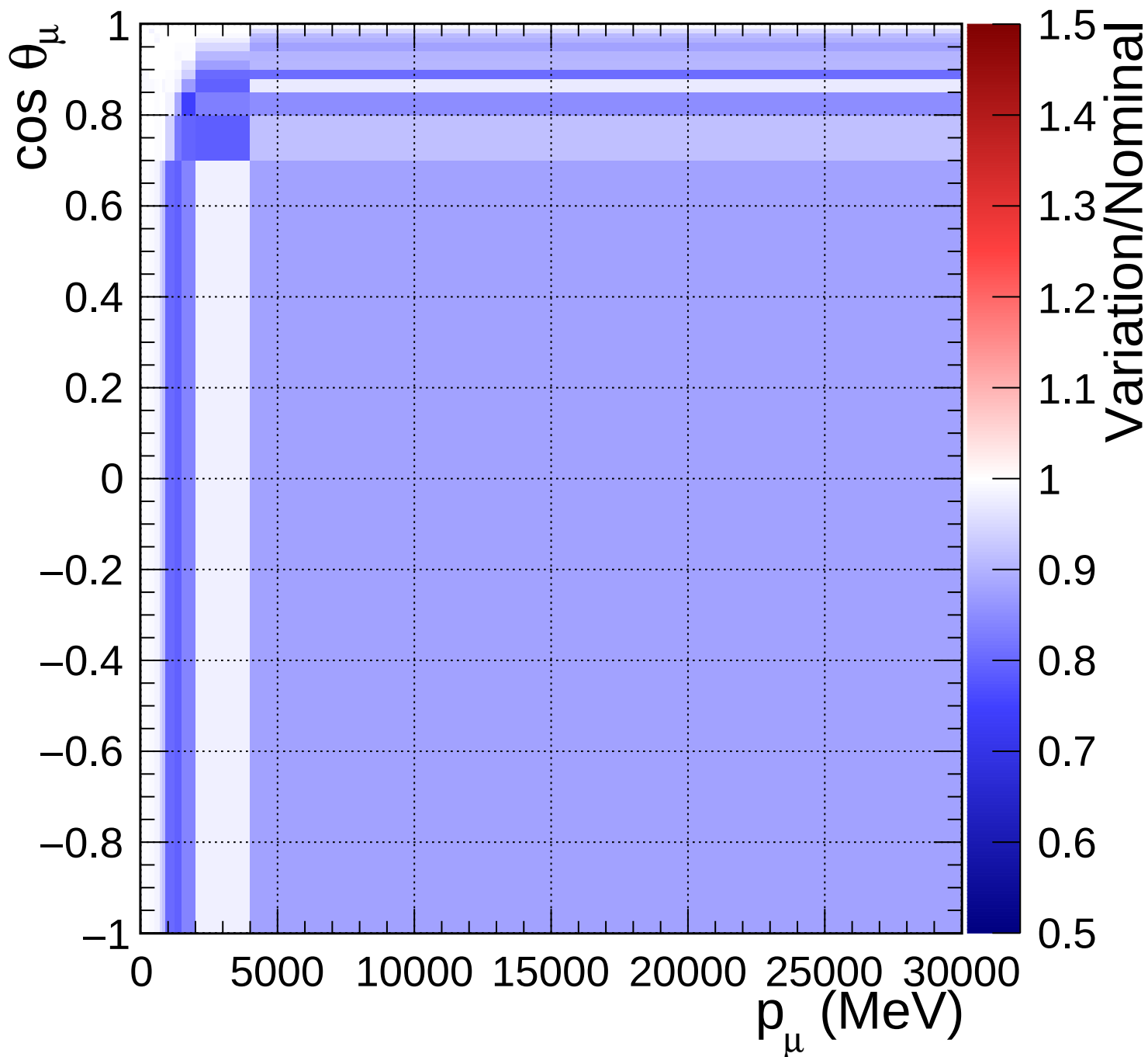
FGD2_NuMuBkg_CC0pi_in_AntiNu_Mode_Q2_norm_7_-0.2
