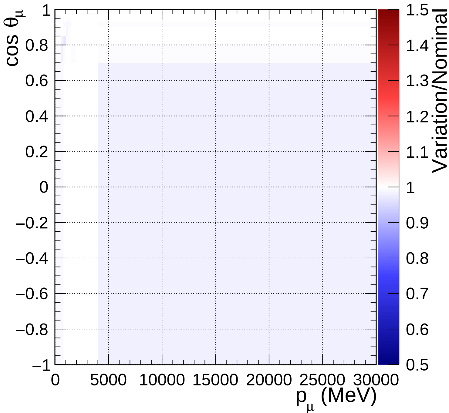
FGD2_anti-numuCC_other_Q2_norm_5_0.67
