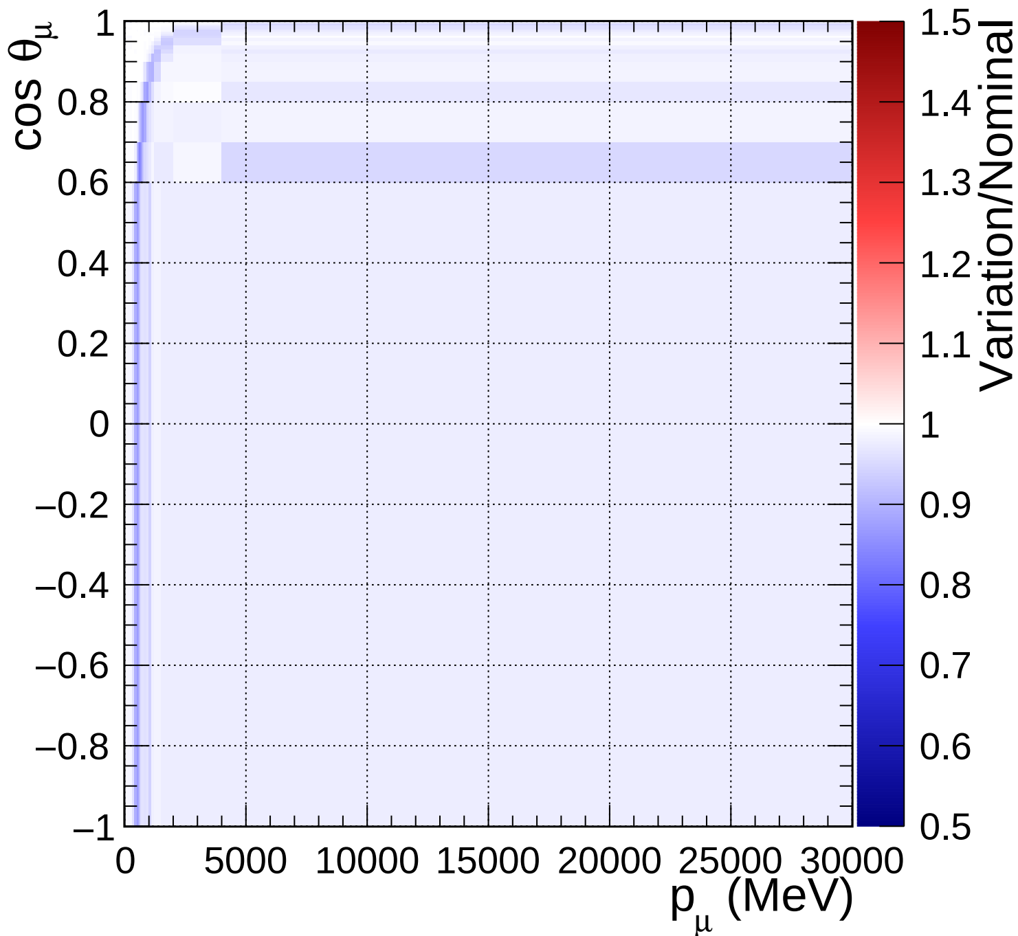
FGD2_anti-numuCC_0pi_Q2_norm_5_0.67
