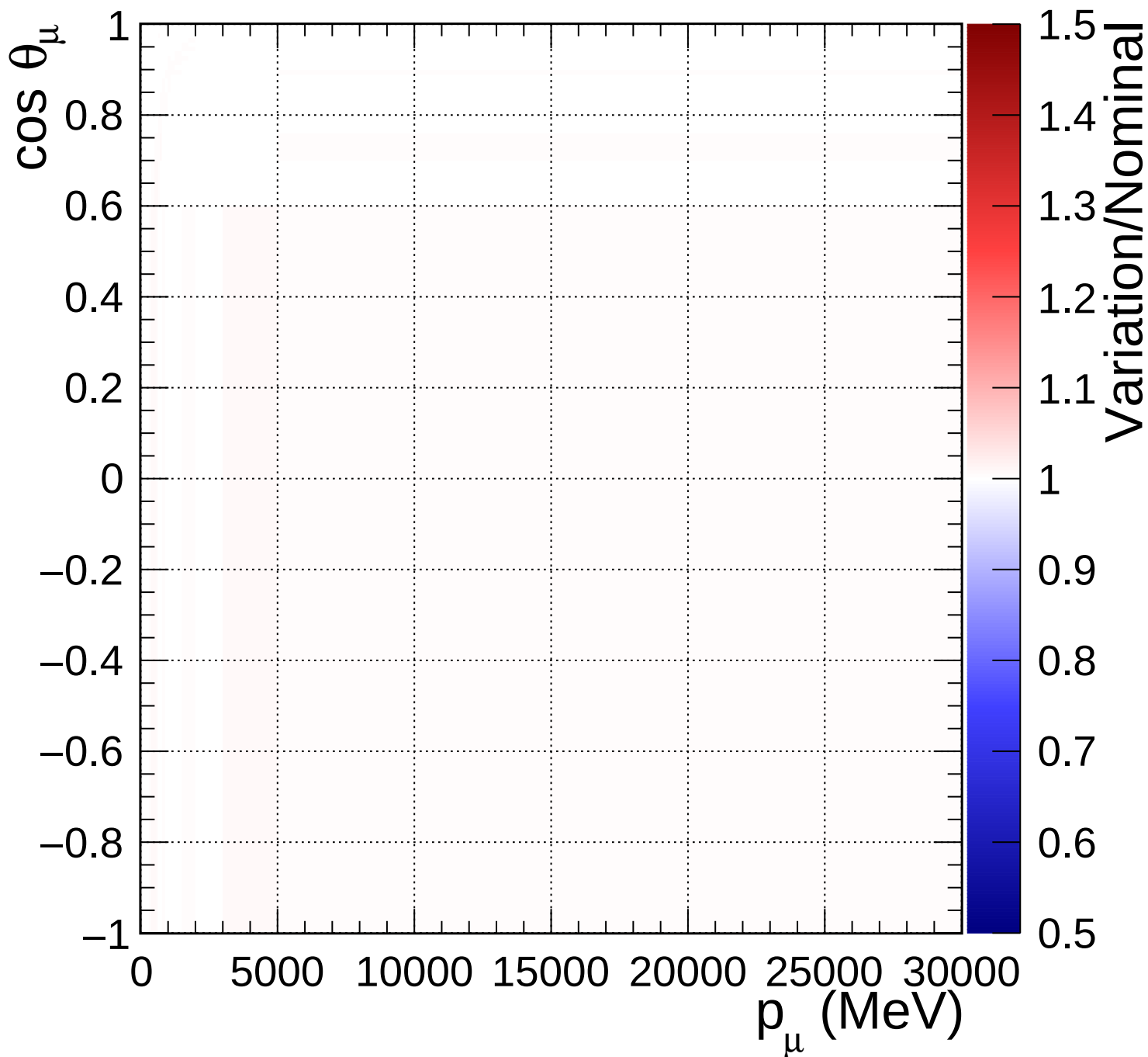
FGD1_numuCC_other_Q2_norm_5_1.11
