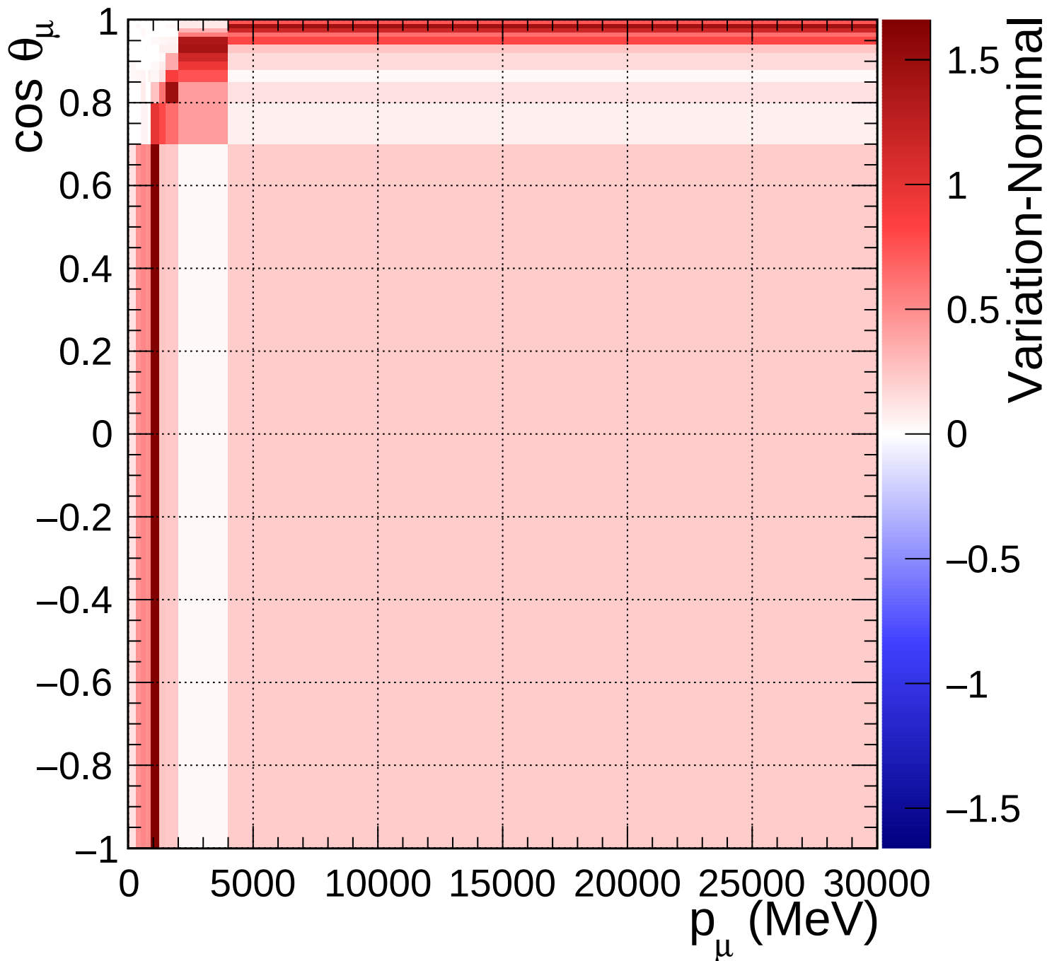
FGD2_NuMuBkg_CC0pi_in_AntiNu_Mode_Q2_norm_7_1.4
