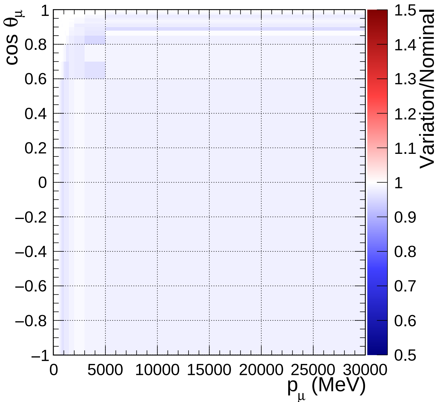
FGD2_numuCC_1pi_Q2_norm_7_0.6
