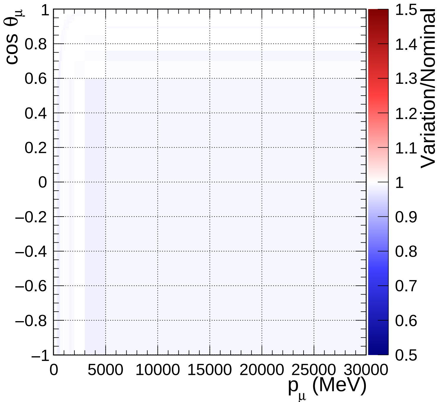
FGD1_numuCC_other_Q2_norm_5_0.67
