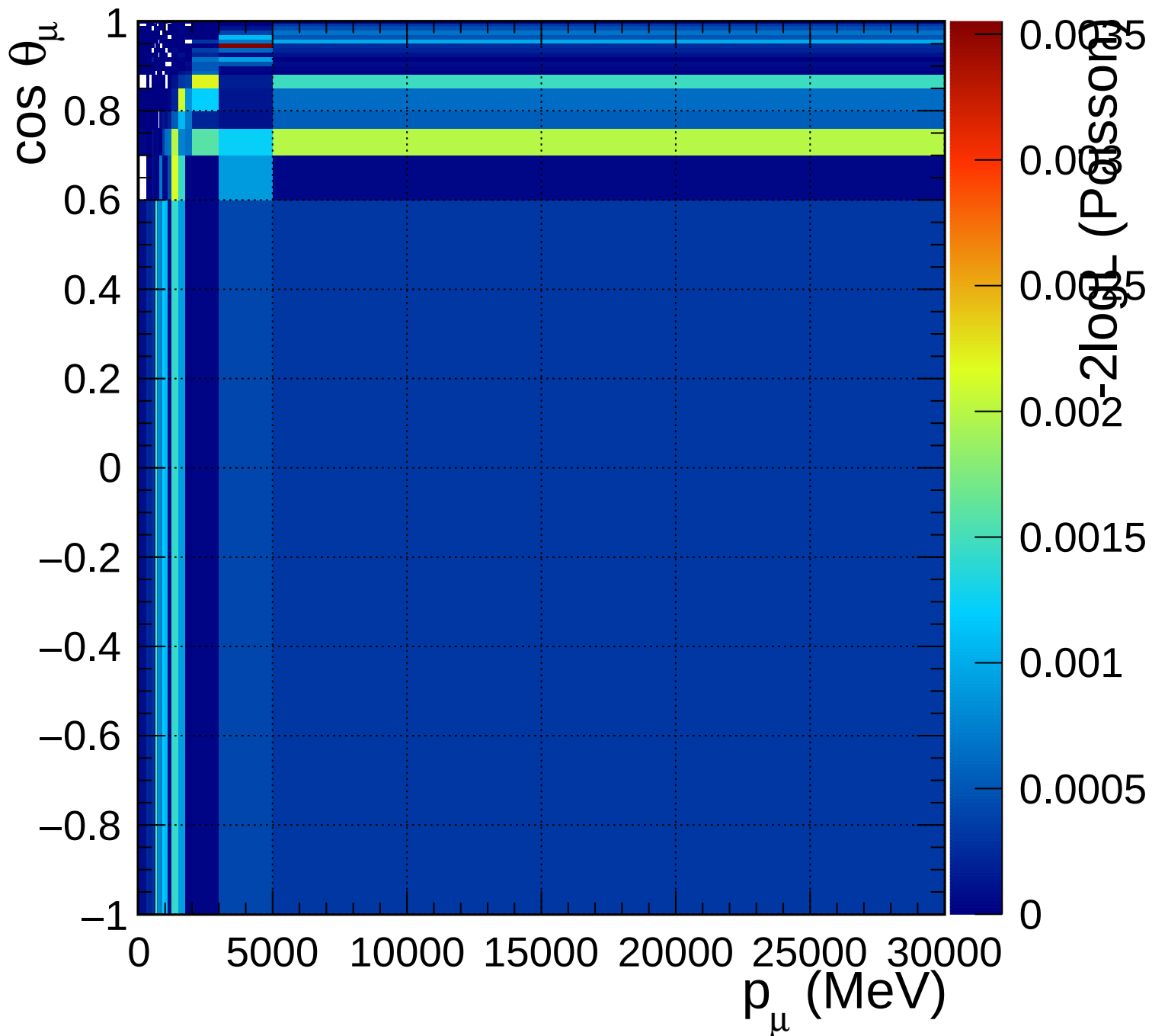
FGD2_numuCC_other_Q2_norm_7_0.6
