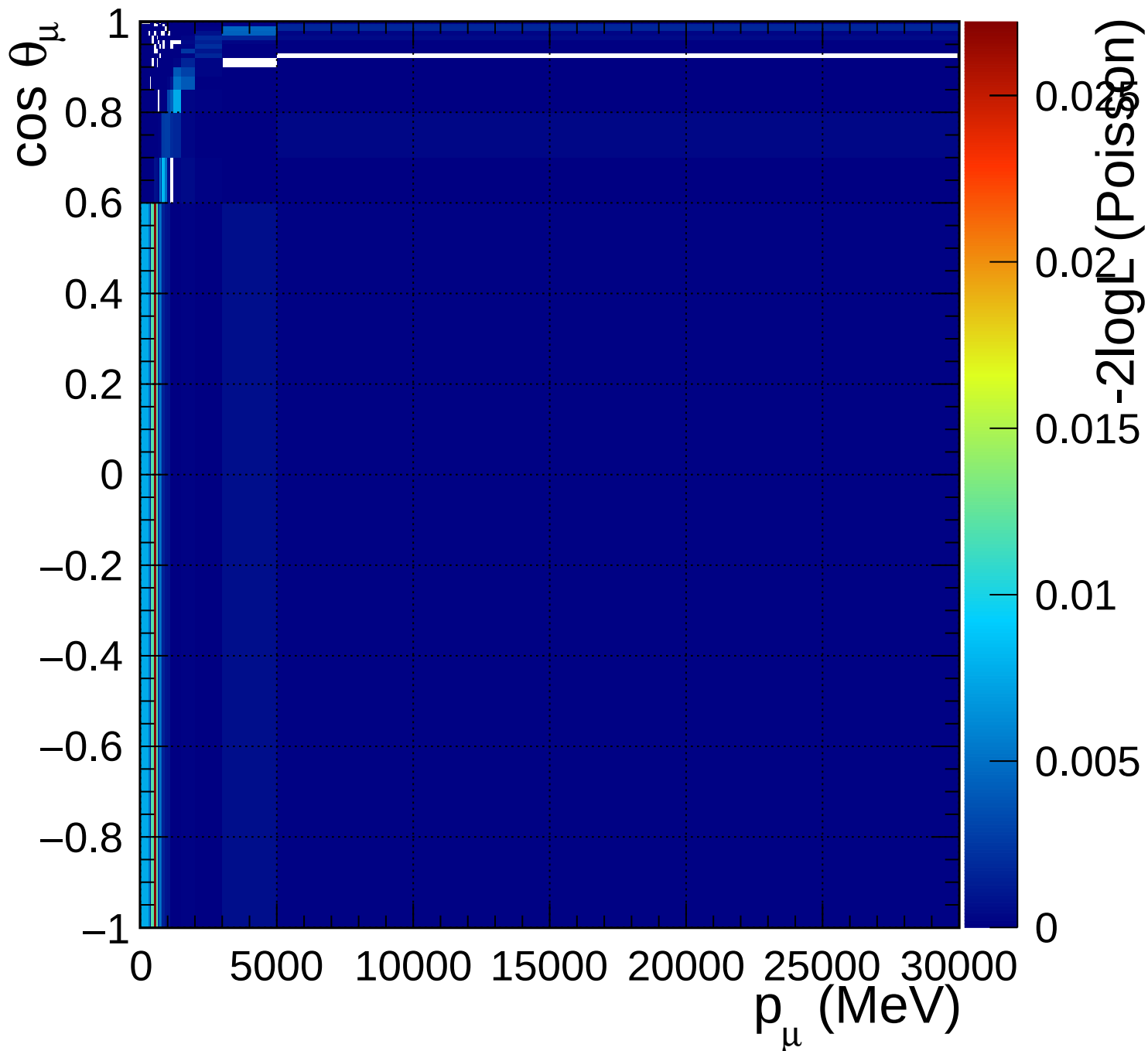
FGD2_numuCC_1pi_Q2_norm_6_0.46
