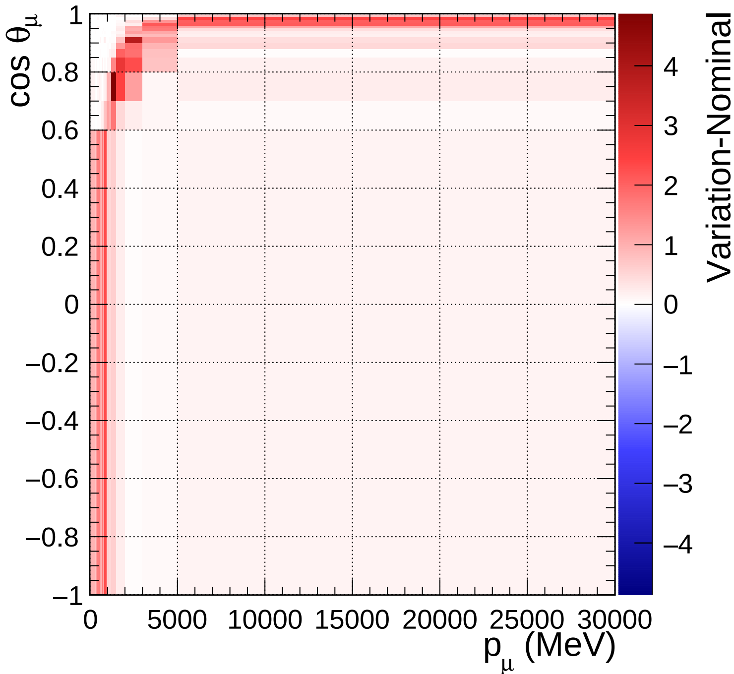
FGD2_numuCC_1pi_Q2_norm_7_2.2
