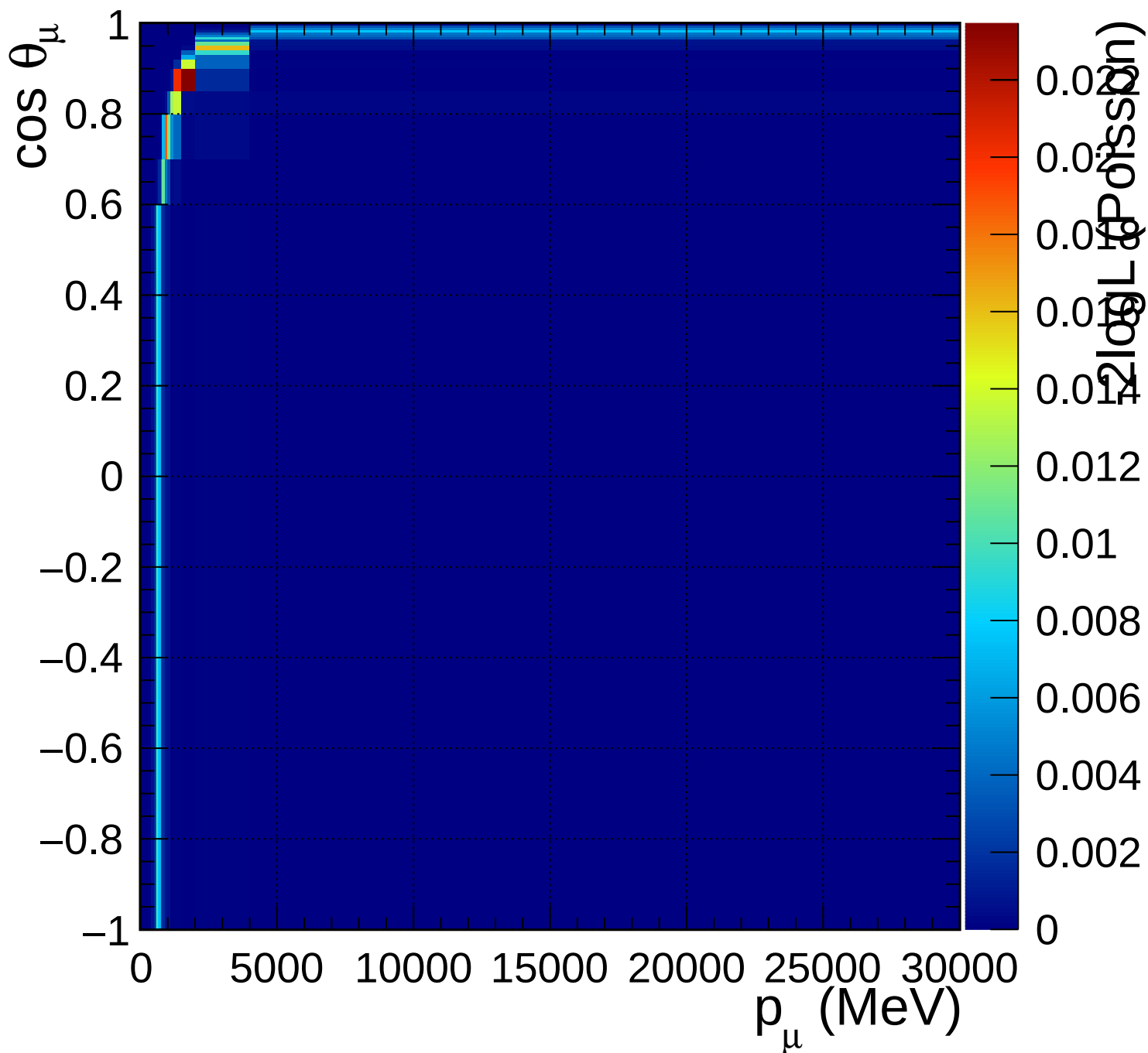
FGD1_anti-numuCC_0pi_Q2_norm_6_1.18
