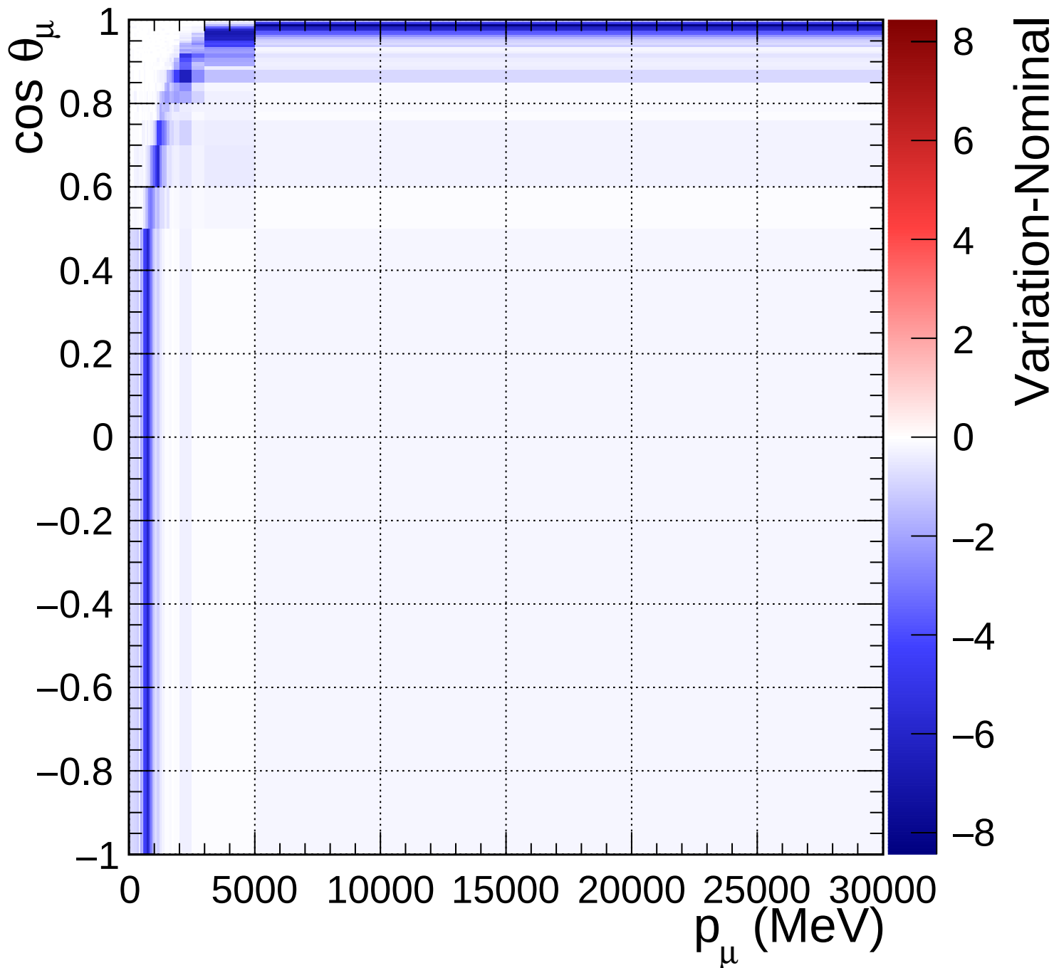
FGD1_numuCC_0pi_Q2_norm_7_-0.2
