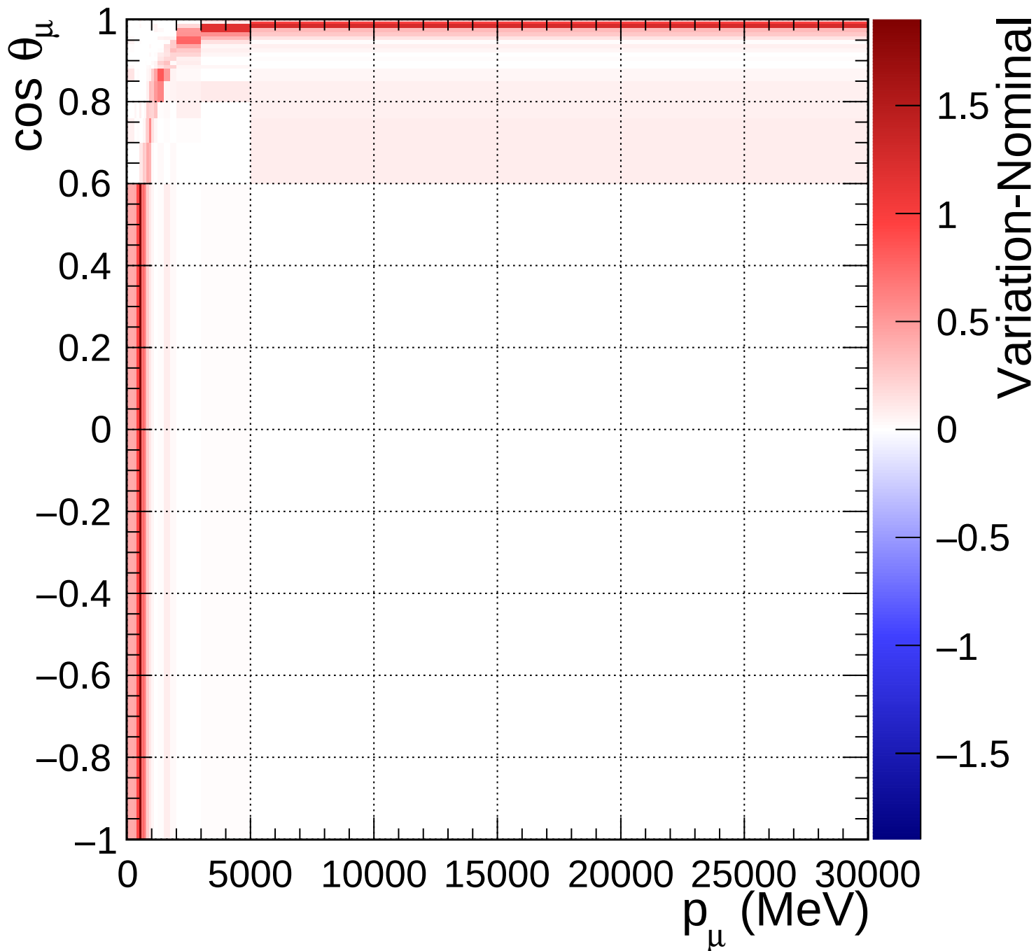
FGD1_numuCC_other_Q2_norm_6_1.54
