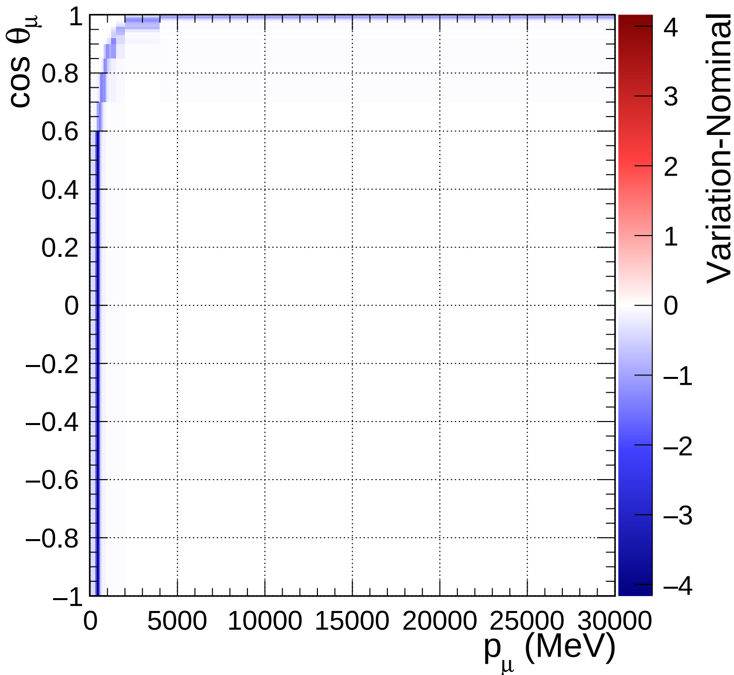
FGD1_anti-numuCC_0pi_Q2_norm_5_0.89
