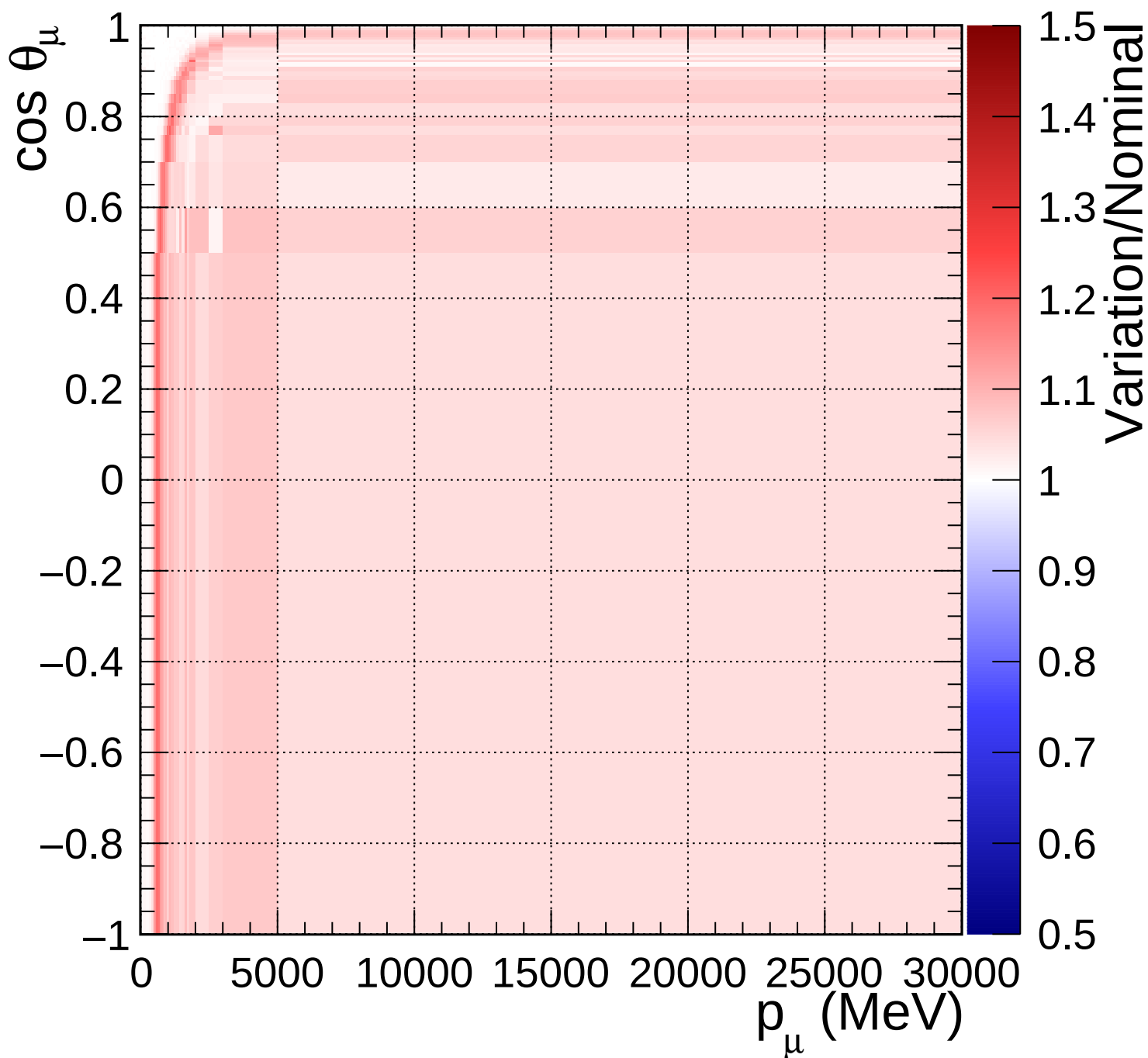
FGD1_numuCC_0pi_Q2_norm_6_1.54
