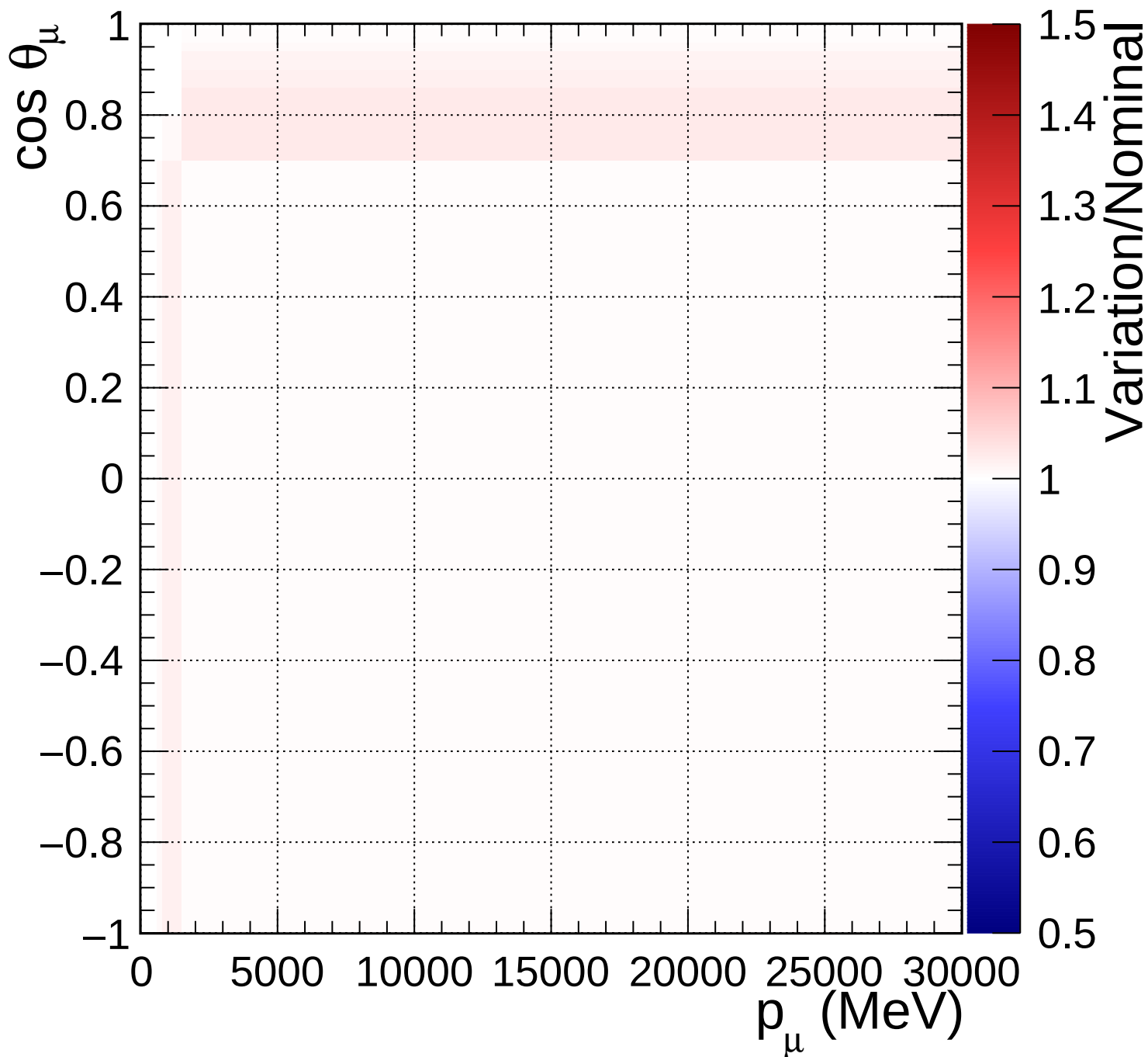
FGD2_NuMuBkg_CC1pi_in_AntiNu_Mode_Q2_norm_7_1.4
