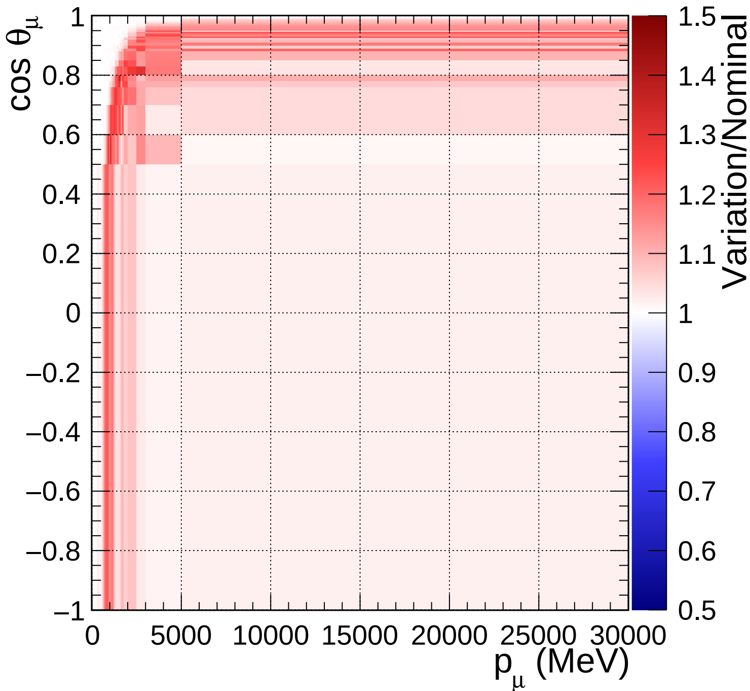
FGD2_numuCC_0pi_Q2_norm_7_2.2
