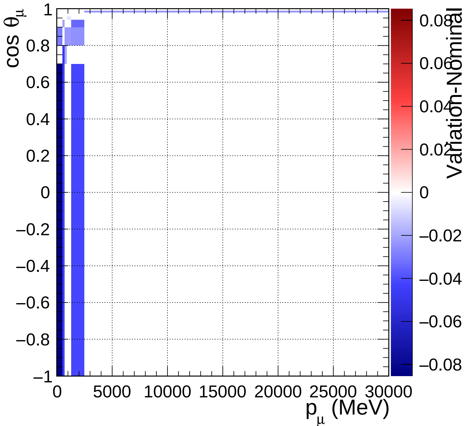
FGD1_anti-numuCC_1pi_Q2_norm_5_0.67
