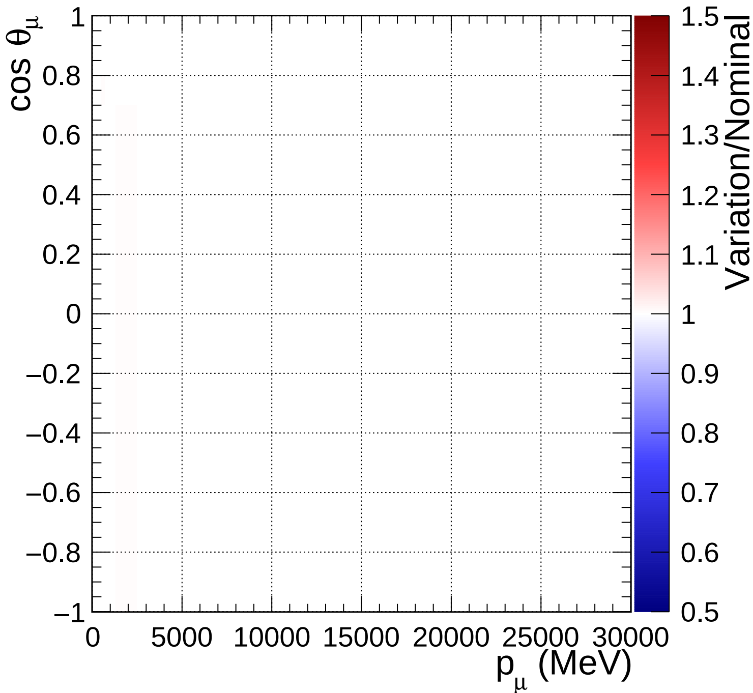
FGD1_anti-numuCC_1pi_Q2_norm_5_1.11
