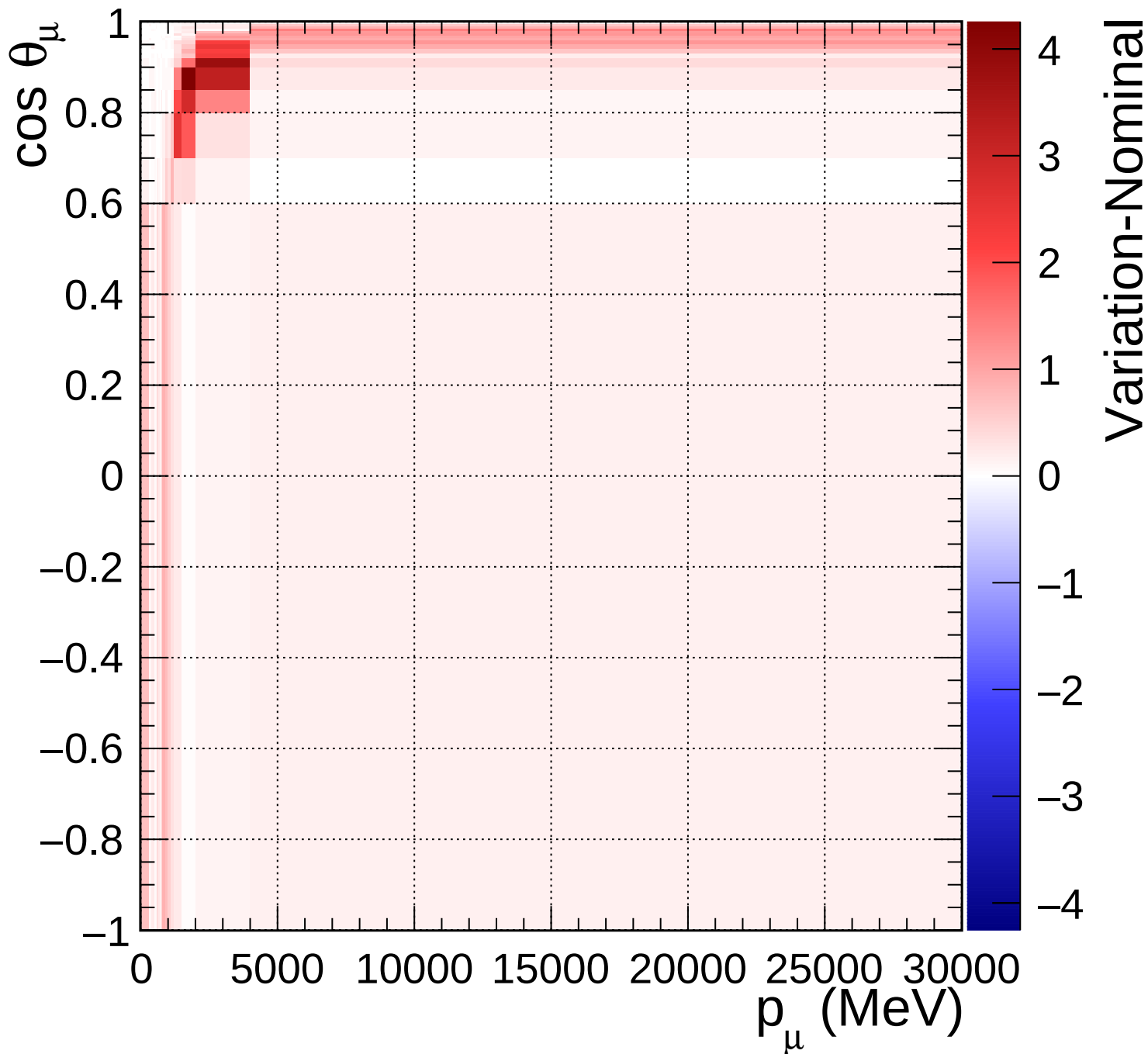
FGD1_anti-numuCC_0pi_Q2_norm_7_2.2
