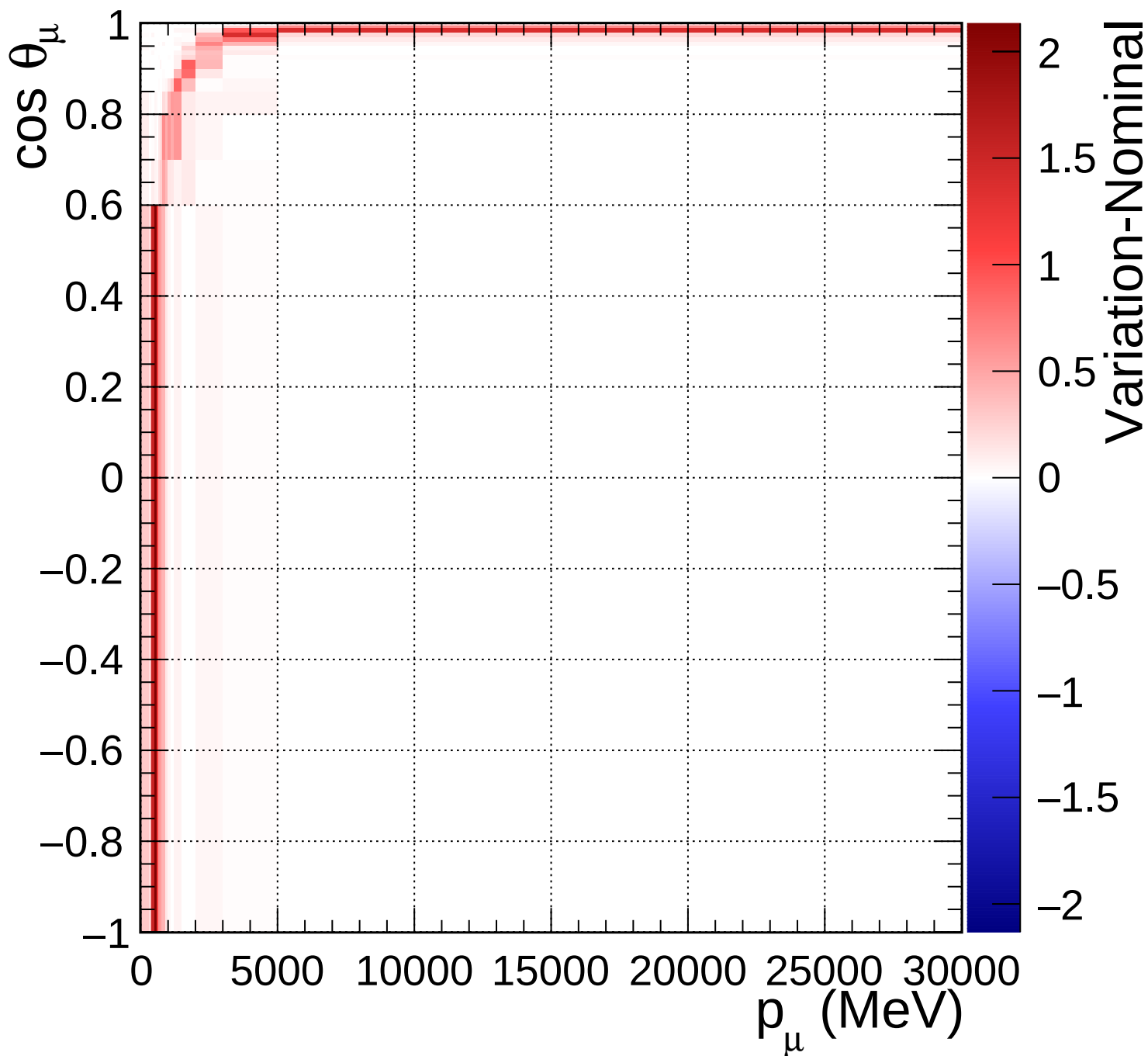
FGD1_numuCC_1pi_Q2_norm_6_1.54
