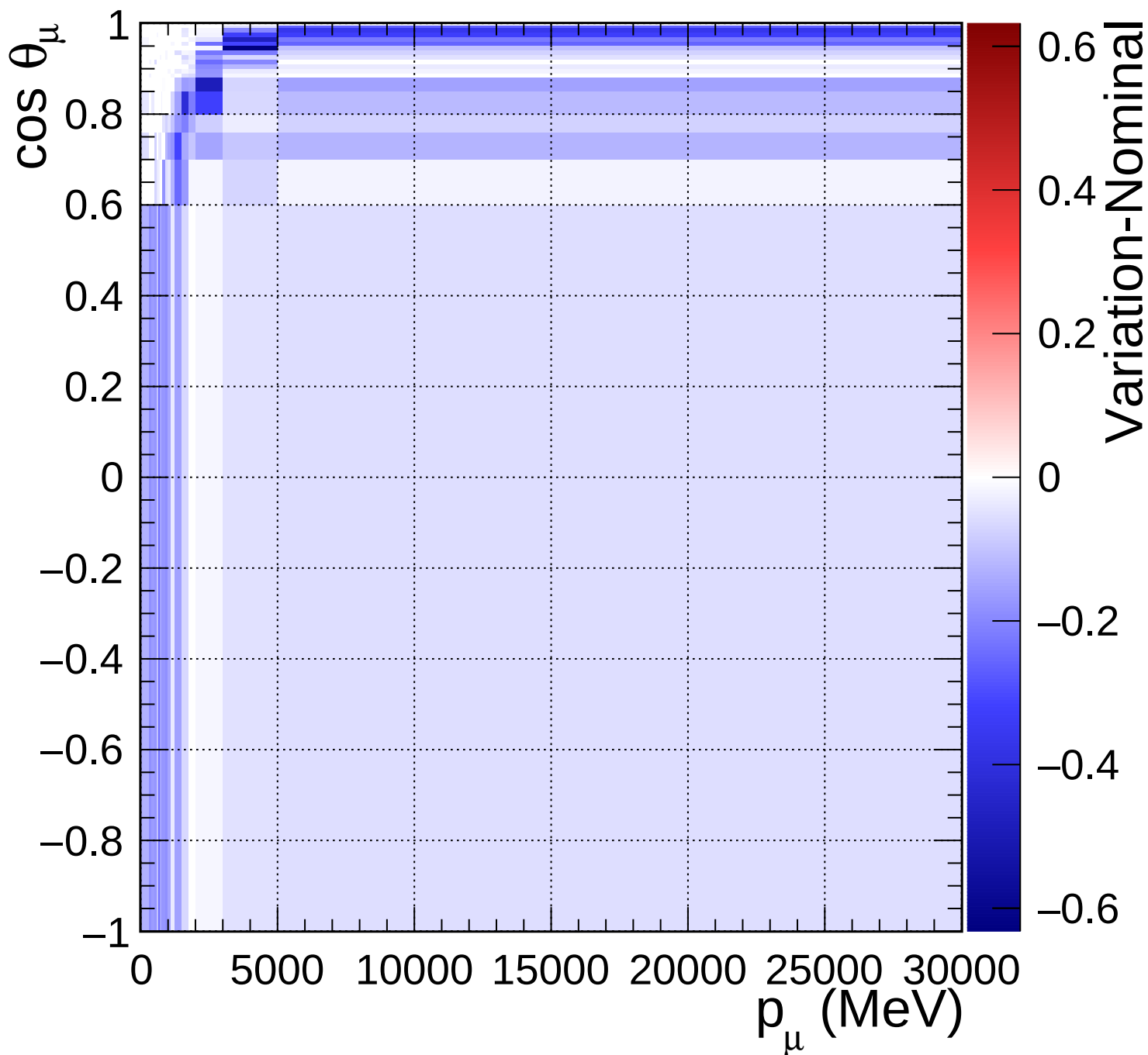
FGD2_numuCC_other_Q2_norm_7_0.6
