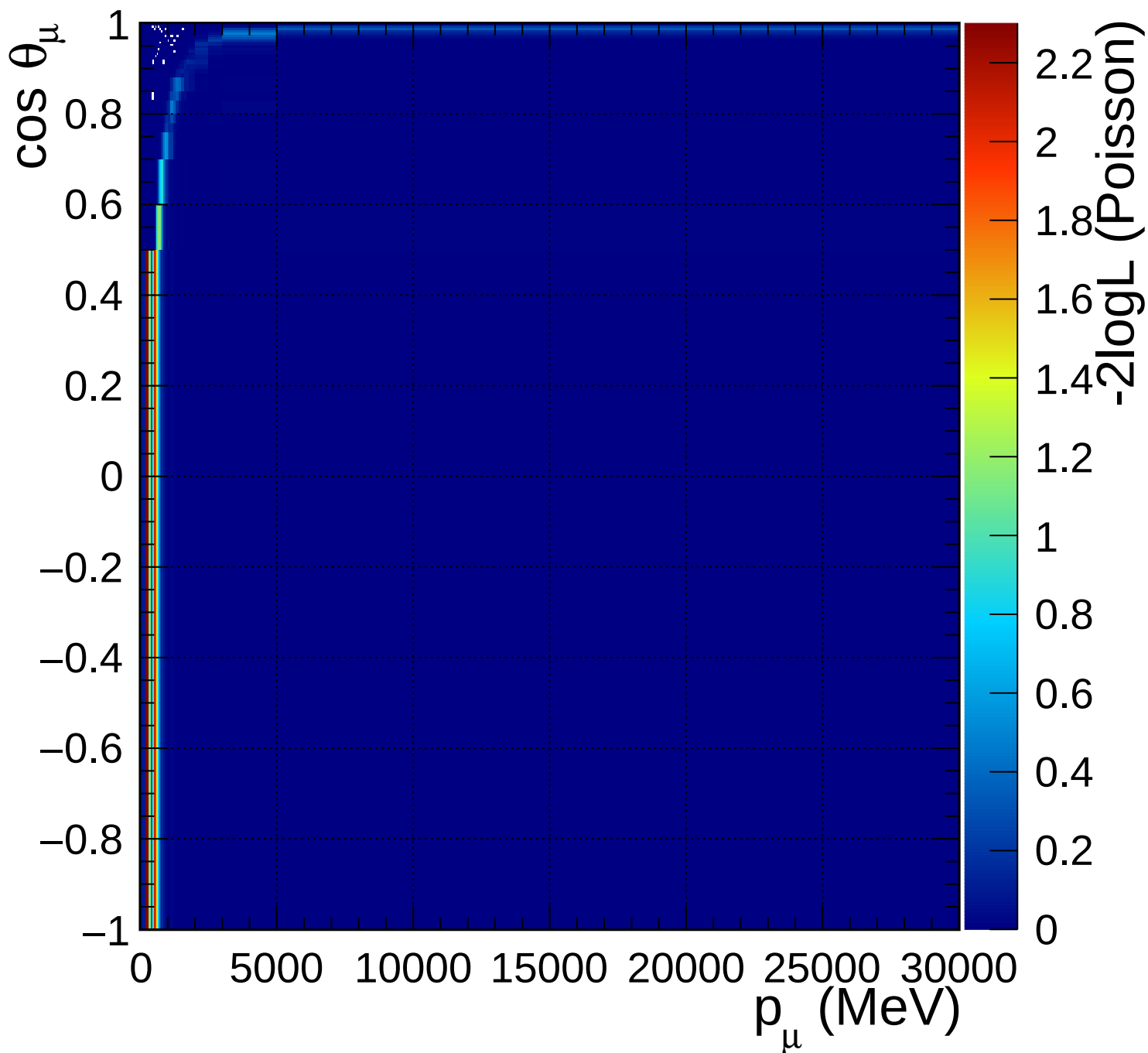
FGD2_numuCC_0pi_Q2_norm_6_0.46
