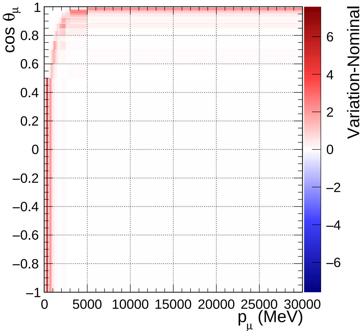
FGD2_numuCC_0pi_Q2_norm_7_1.4
