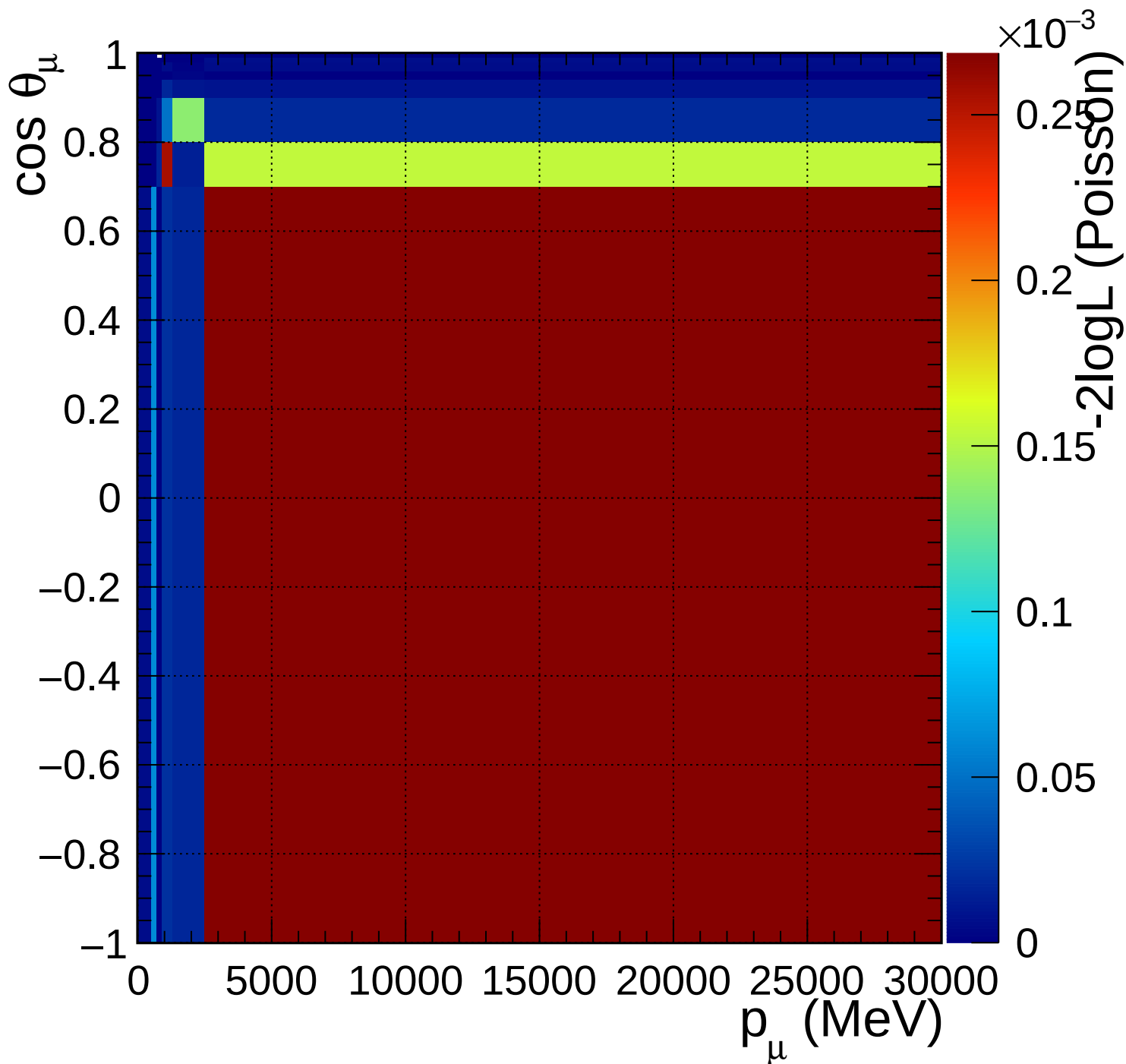
FGD1_anti-numuCC_1pi_Q2_norm_6_1.18
