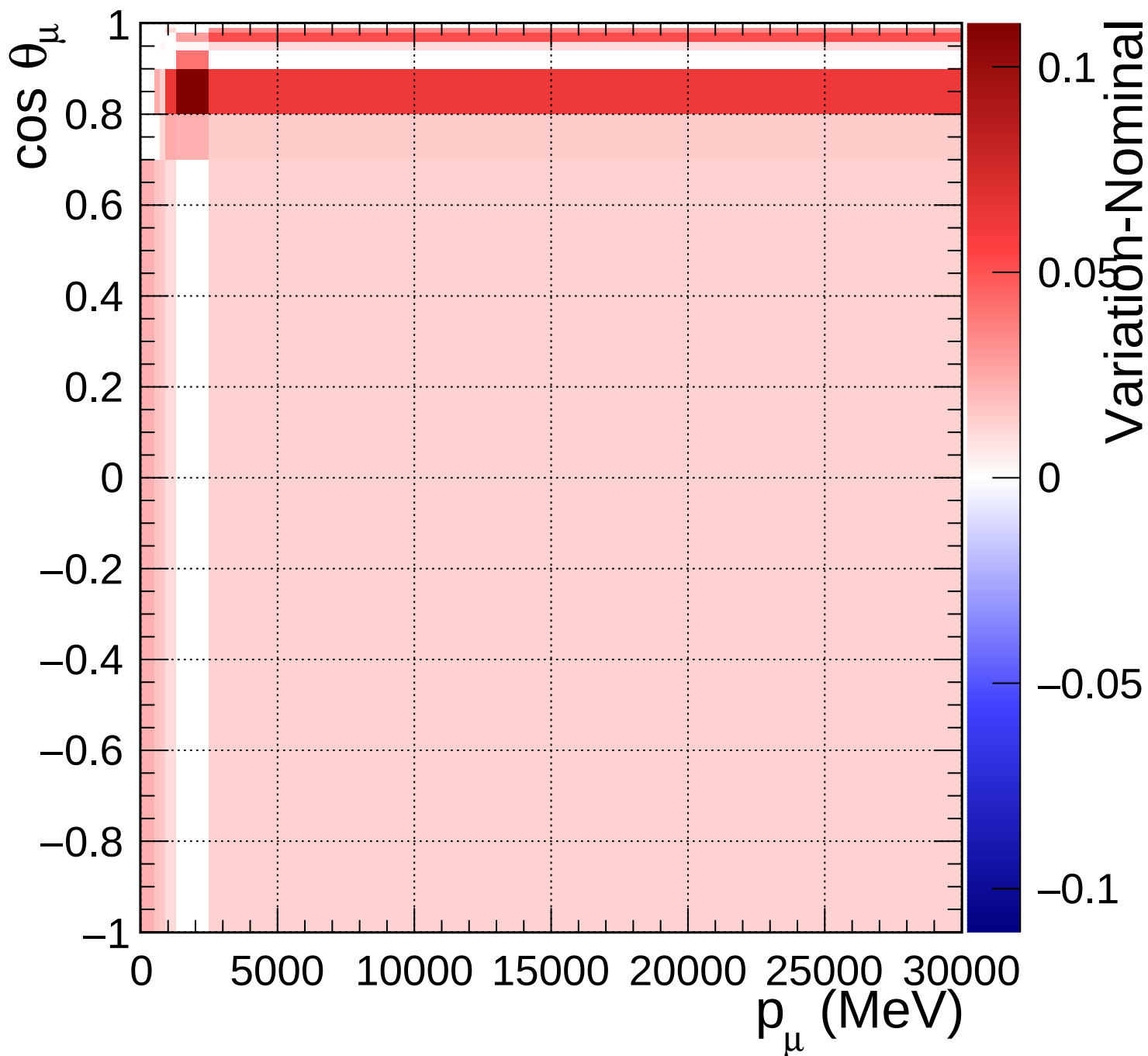
FGD2_anti-numuCC_1pi_Q2_norm_6_1.18
