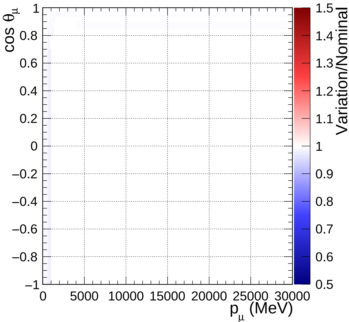
FGD1_anti-numuCC_other_Q2_norm_5_0.67
