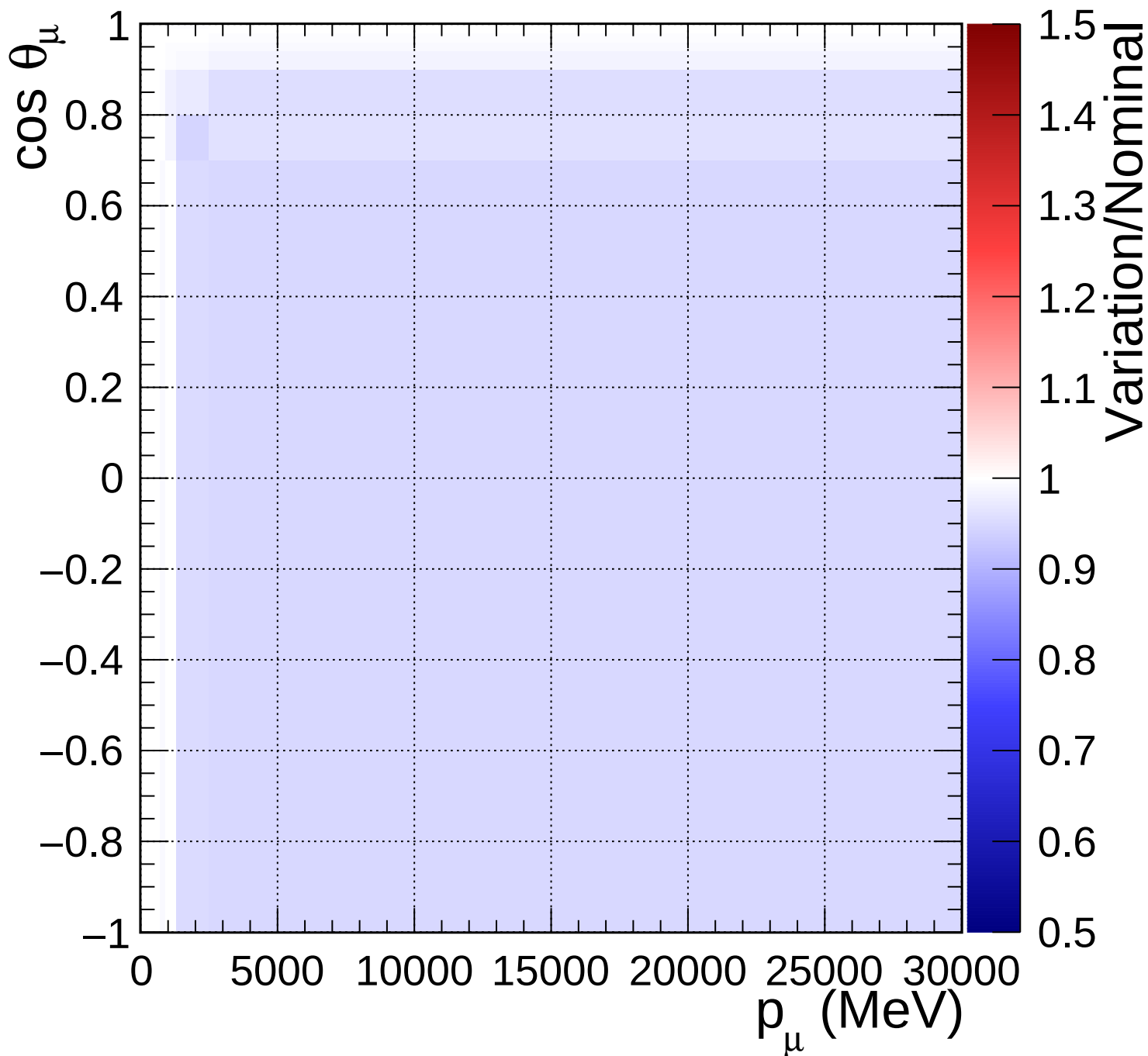
FGD2_anti-numuCC_1pi_Q2_norm_7_0.6
