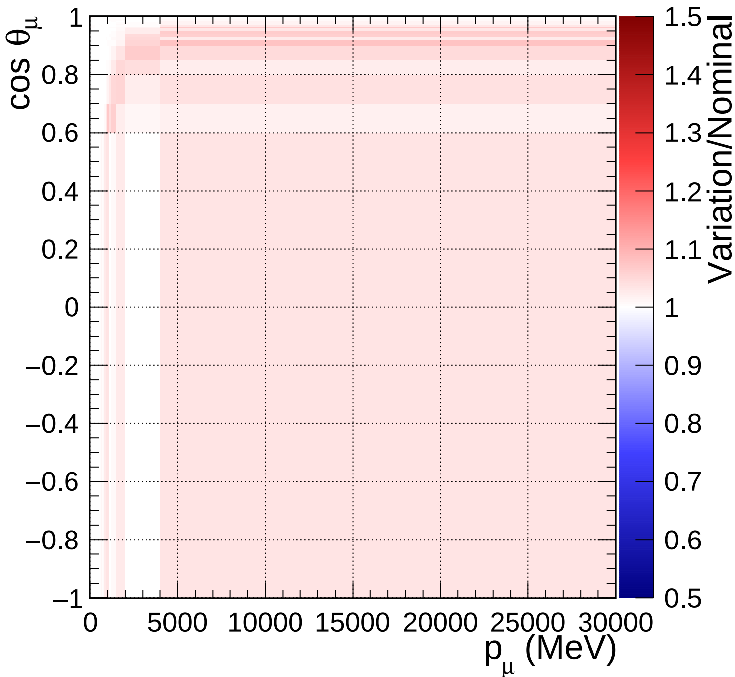
FGD2_anti-numuCC_0pi_Q2_norm_7_1.4
