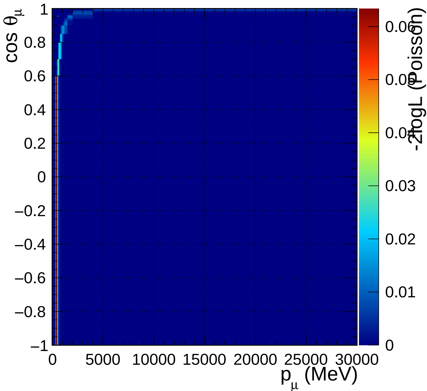
FGD2_anti-numuCC_0pi_Q2_norm_5_1.11
