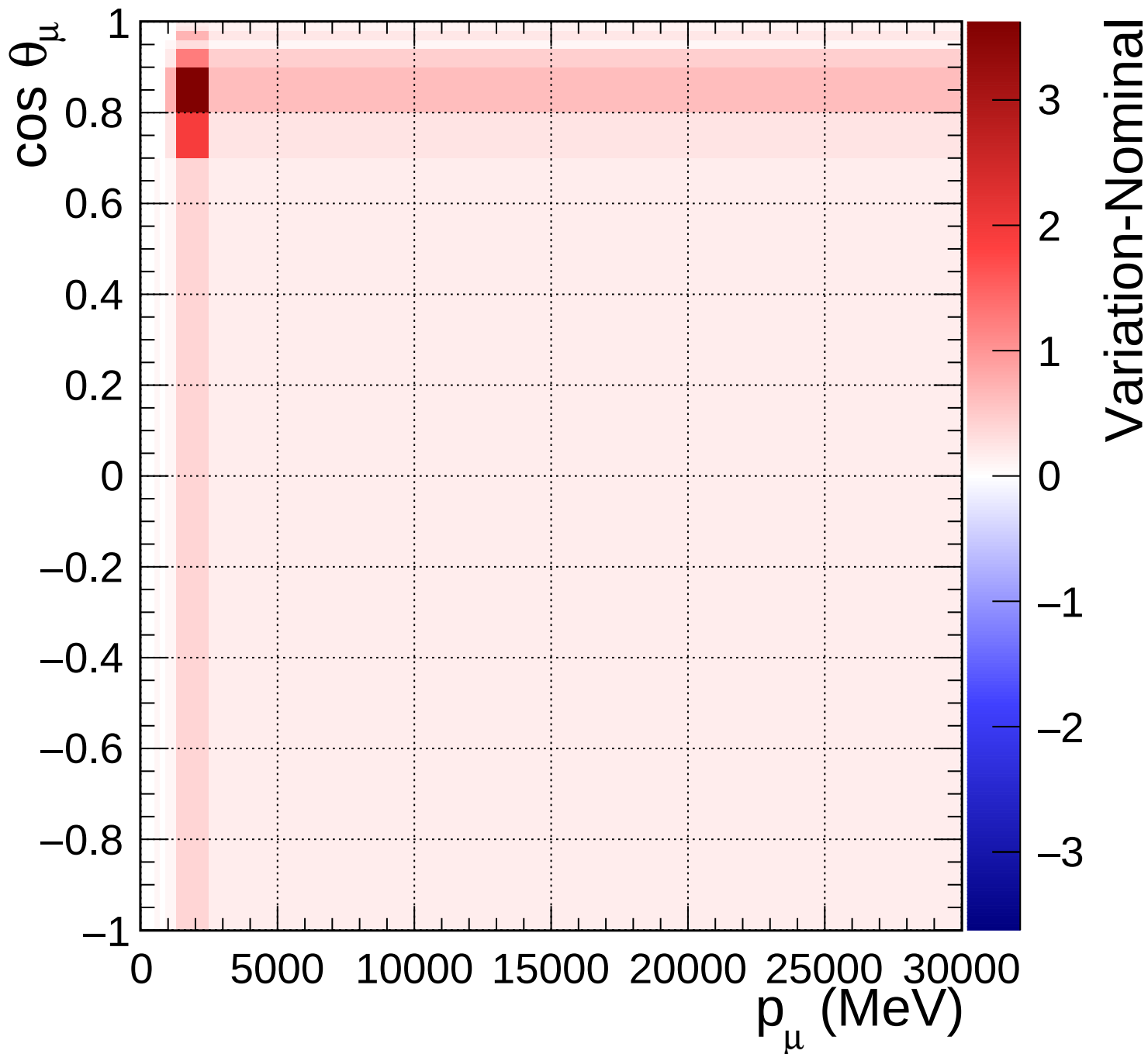
FGD1_anti-numuCC_1pi_Q2_norm_7_2.2
