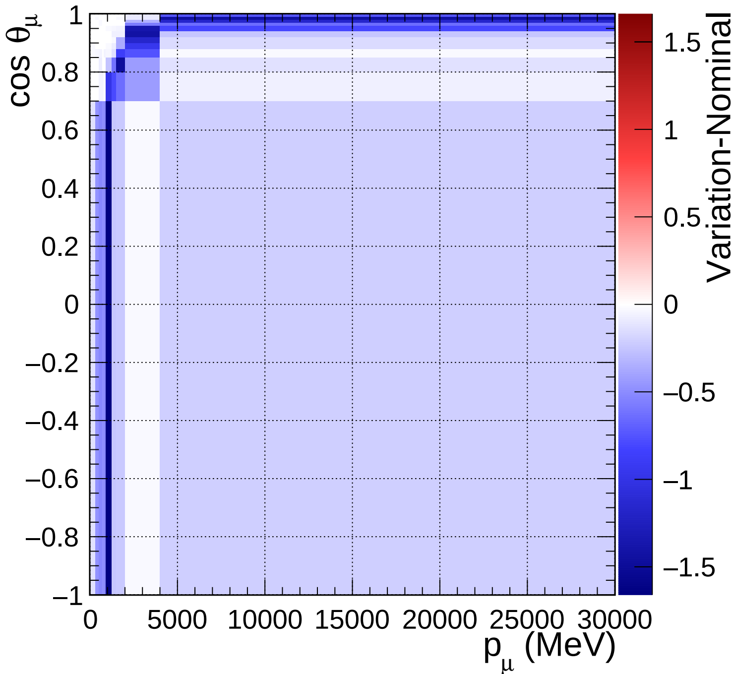
FGD2_NuMuBkg_CC0pi_in_AntiNu_Mode_Q2_norm_7_0.6
