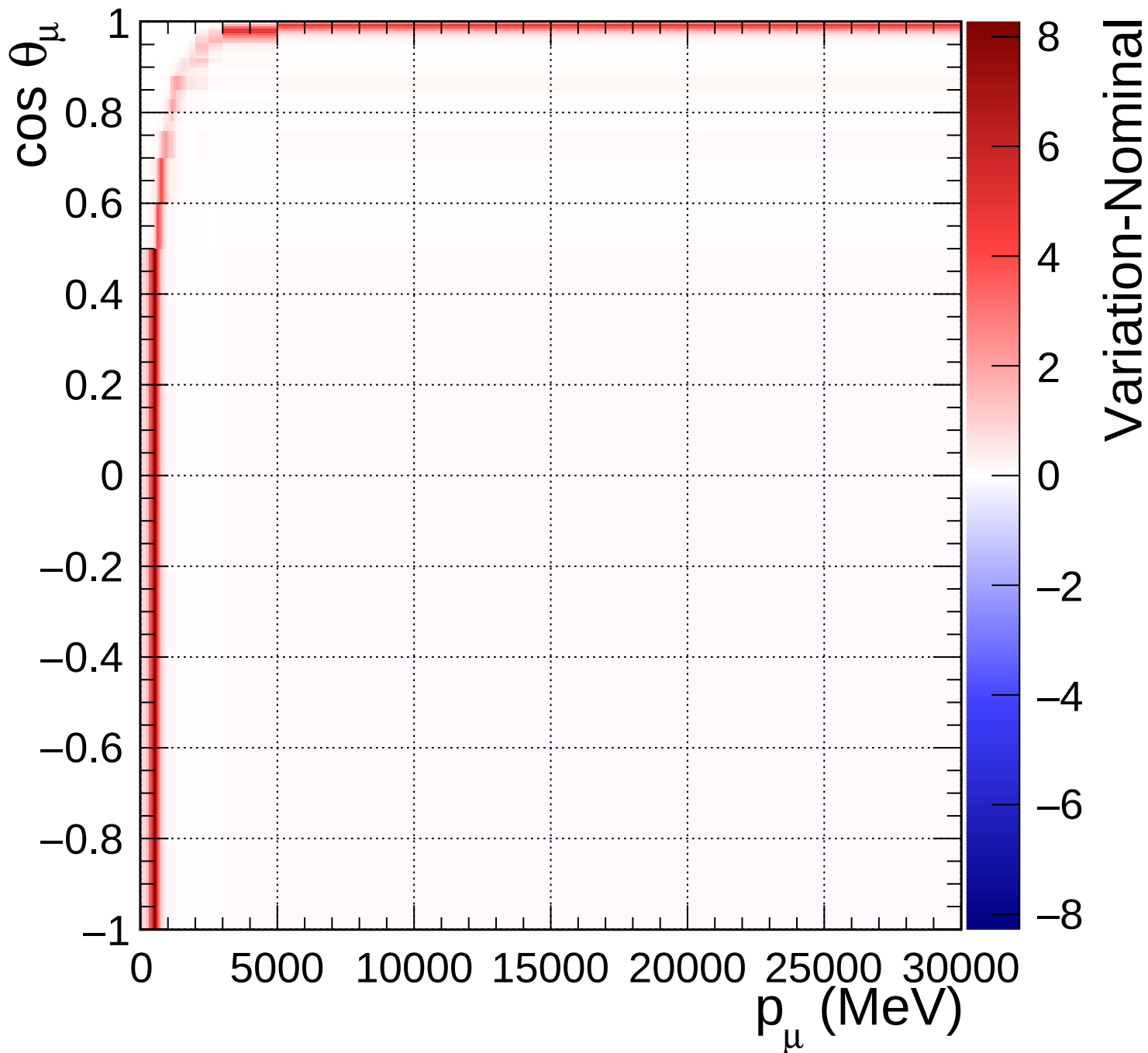
FGD1_numuCC_0pi_Q2_norm_6_1.18
