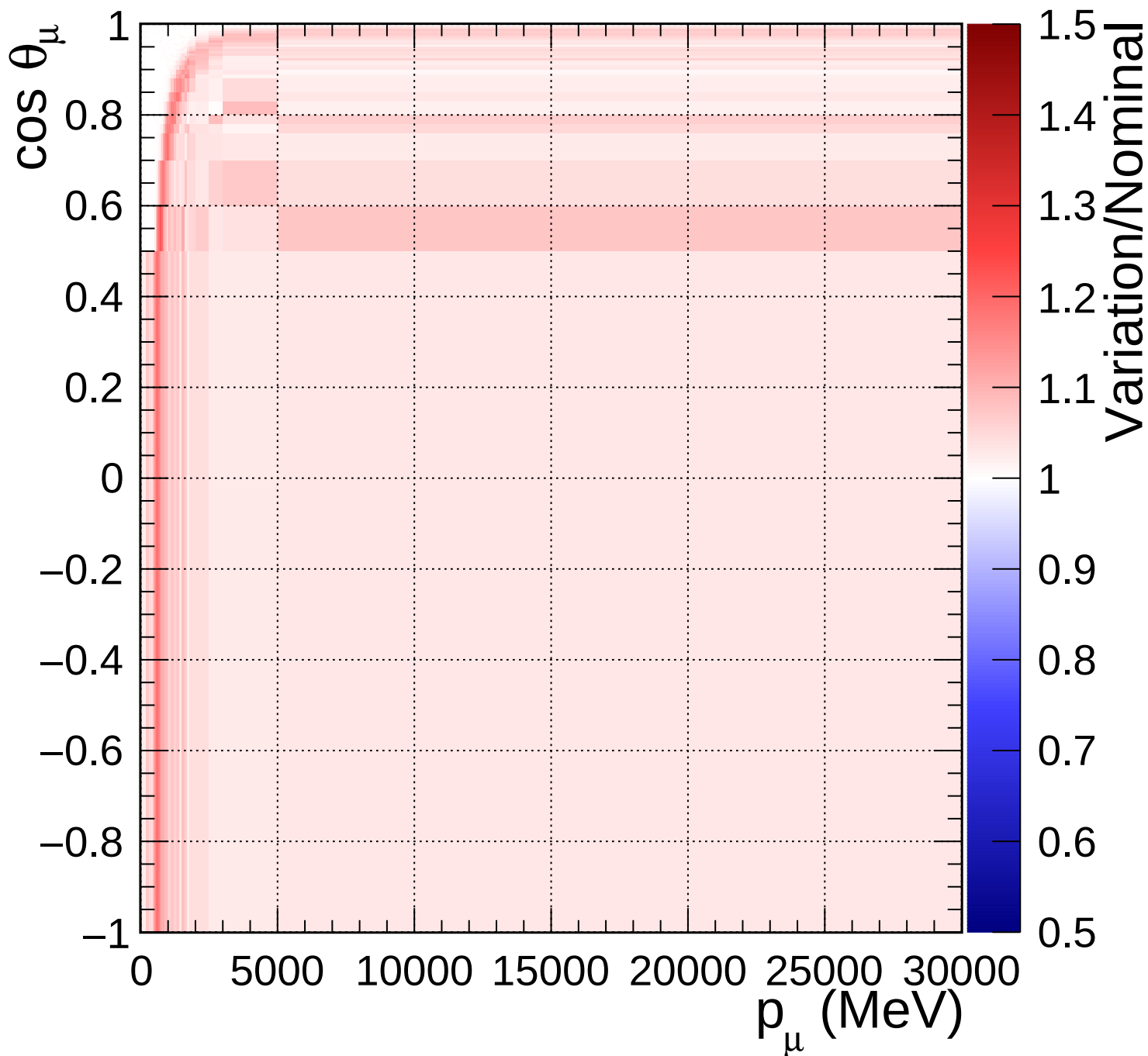
FGD2_numuCC_0pi_Q2_norm_6_1.54
