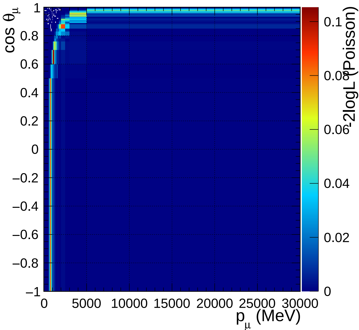
FGD1_numuCC_0pi_Q2_norm_7_1.4
