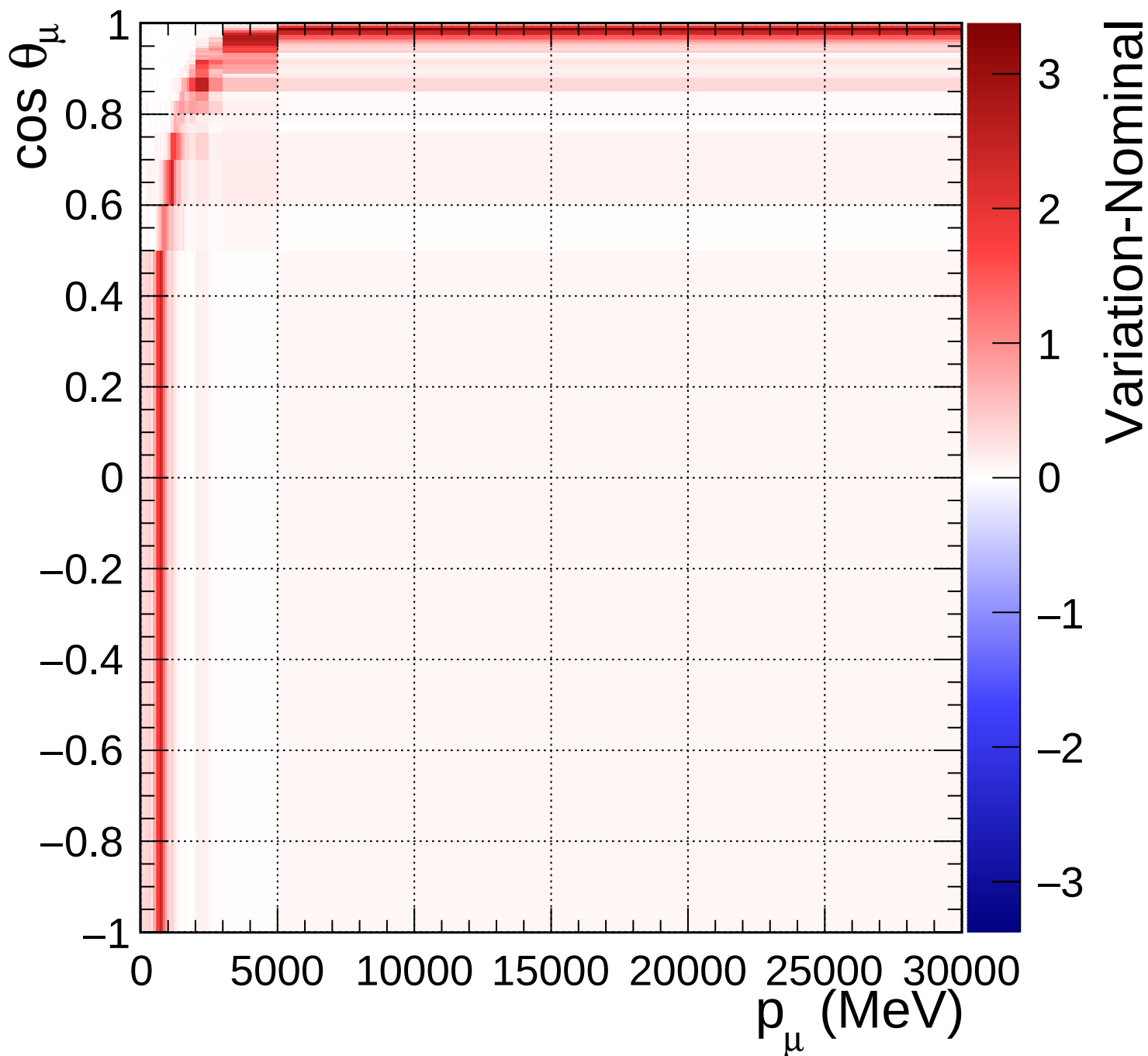
FGD1_numuCC_0pi_Q2_norm_7_1.4
