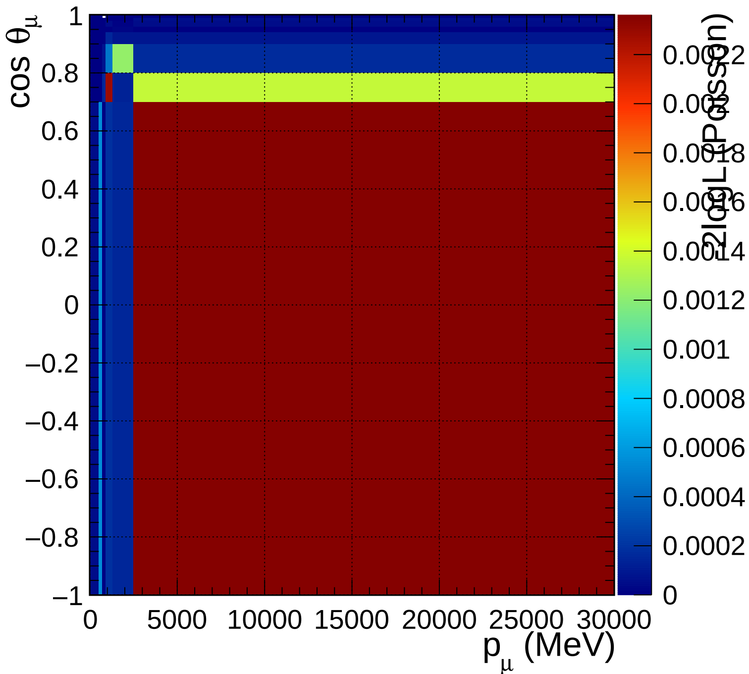
FGD1_anti-numuCC_1pi_Q2_norm_6_1.54
