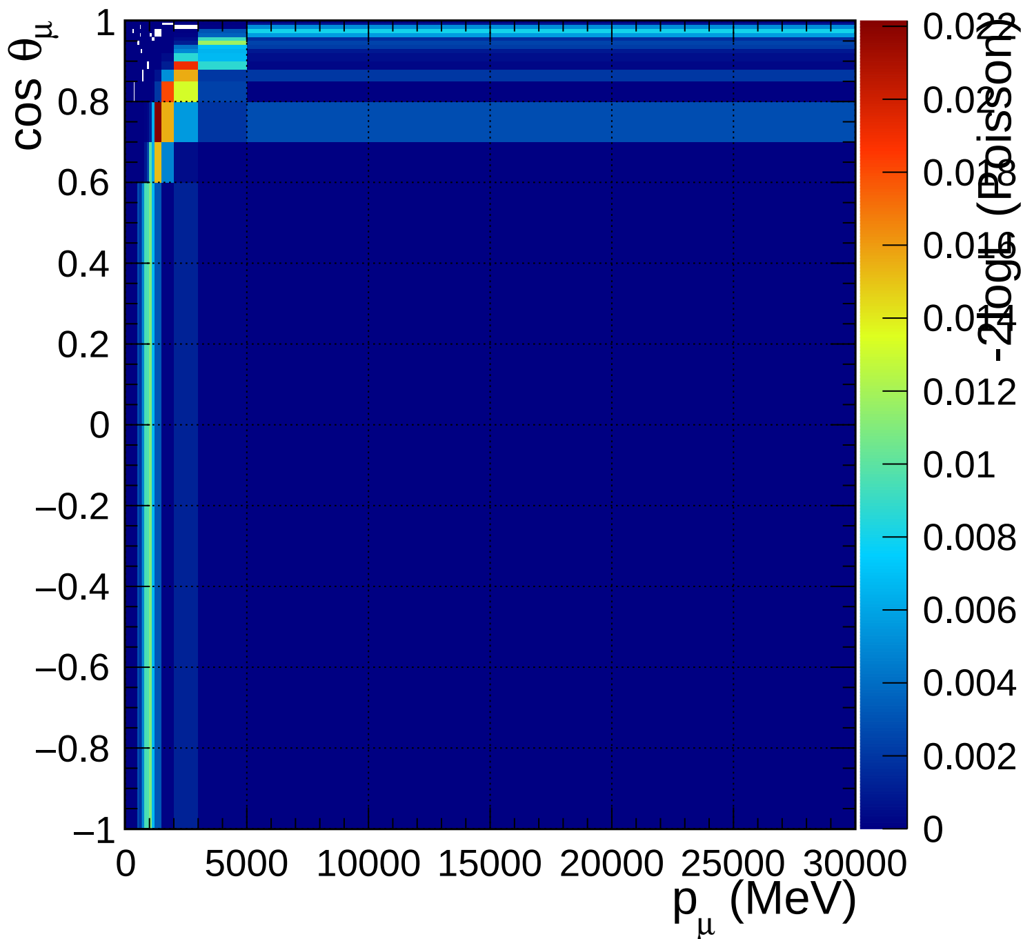
FGD1_numuCC_1pi_Q2_norm_7_0.6
