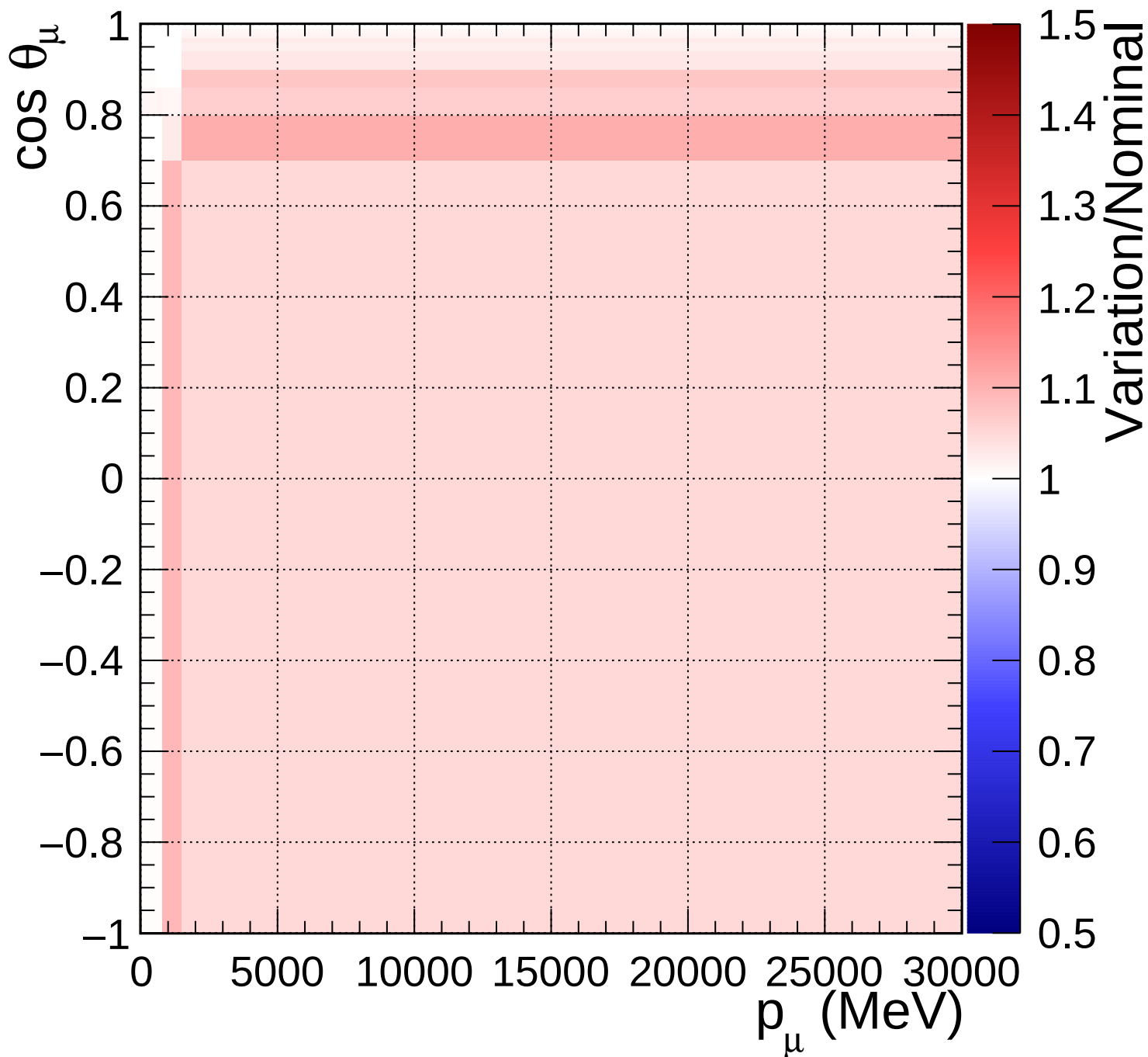
FGD1_NuMuBkg_CC1pi_in_AntiNu_Mode_Q2_norm_7_2.2
