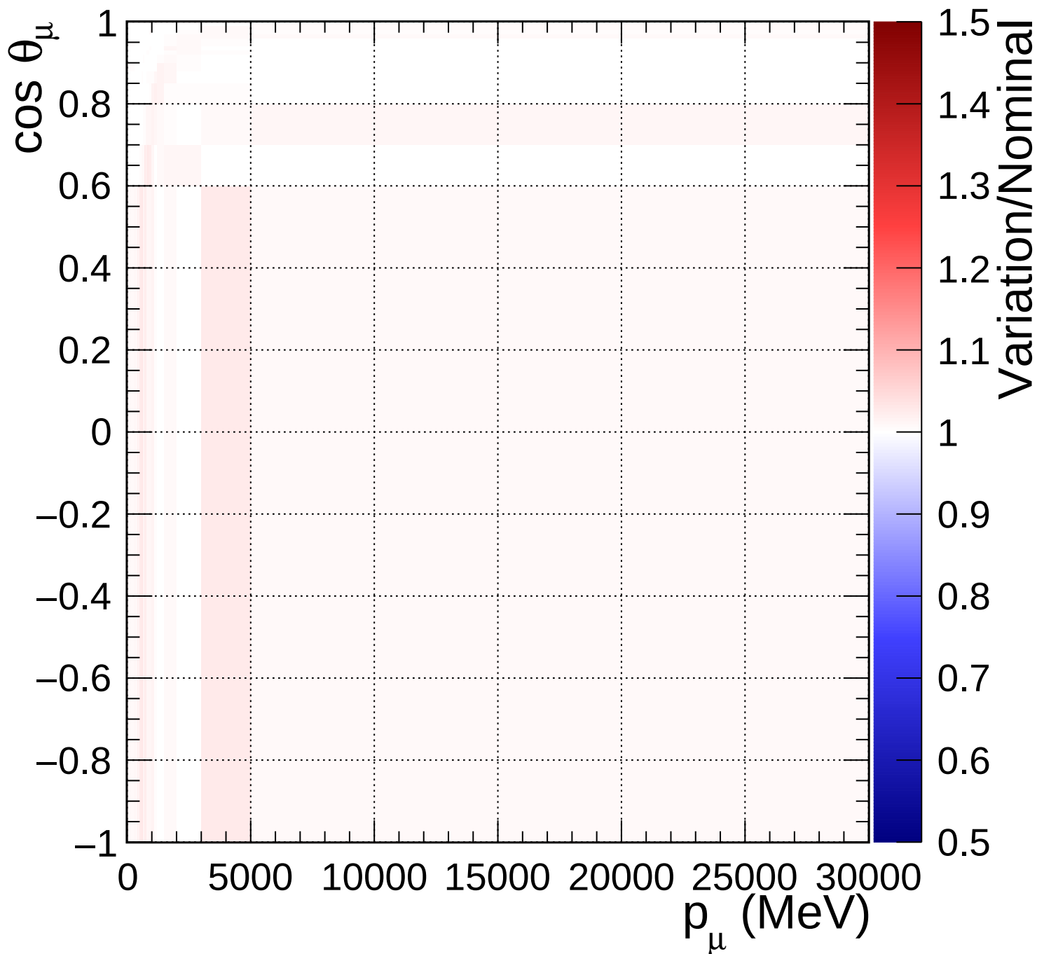
FGD2_numuCC_1pi_Q2_norm_6_1.54
