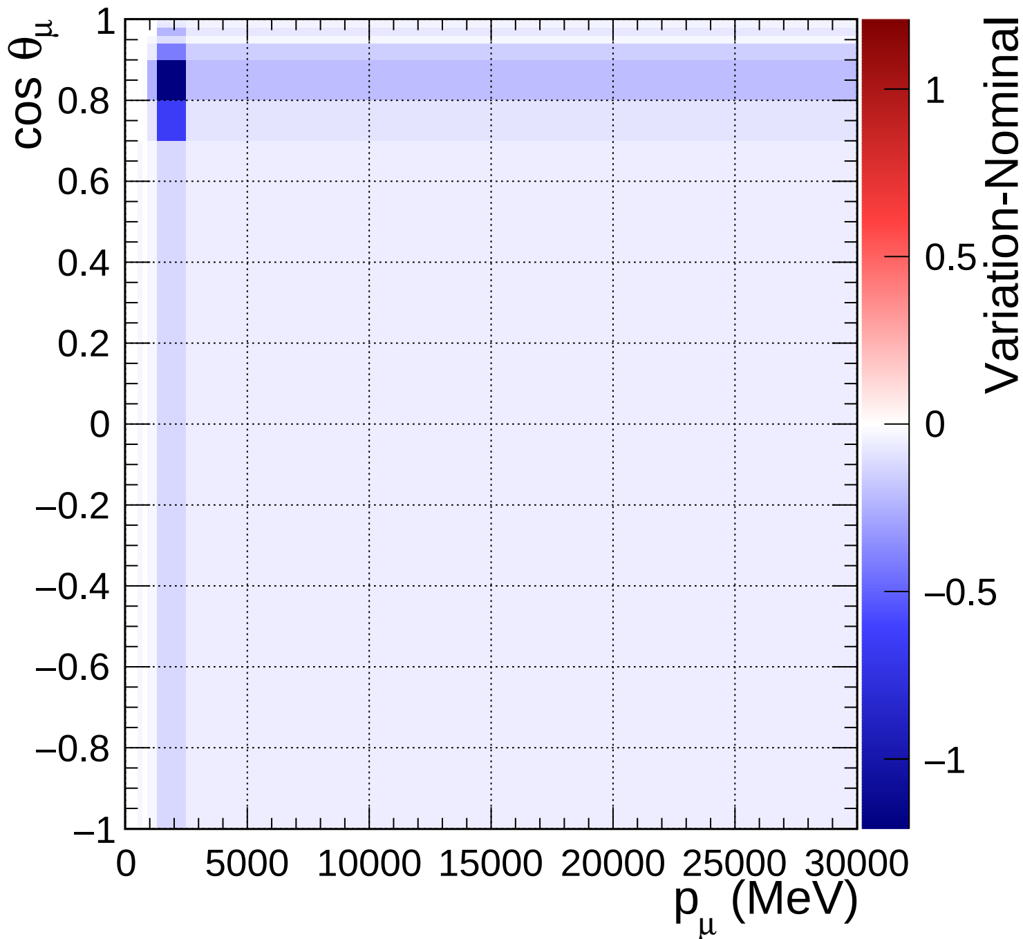
FGD1_anti-numuCC_1pi_Q2_norm_7_0.6
