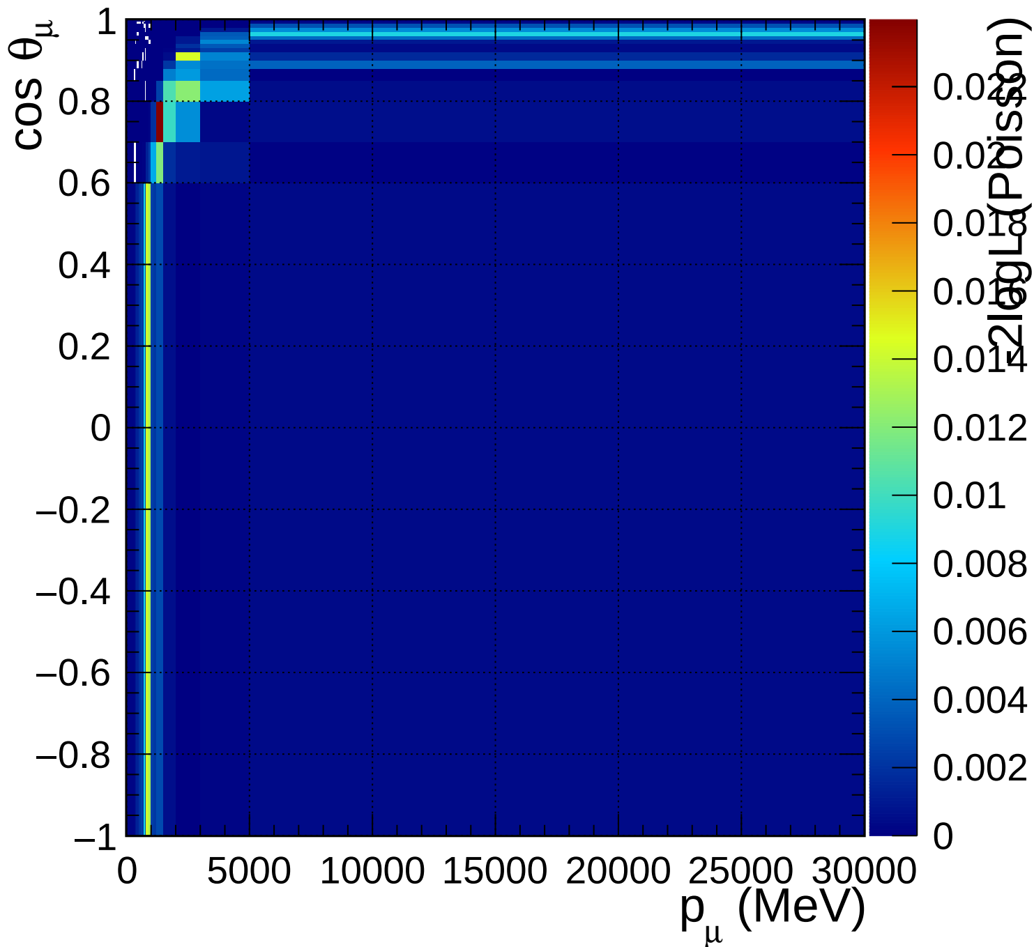
FGD2_numuCC_1pi_Q2_norm_7_1.4
