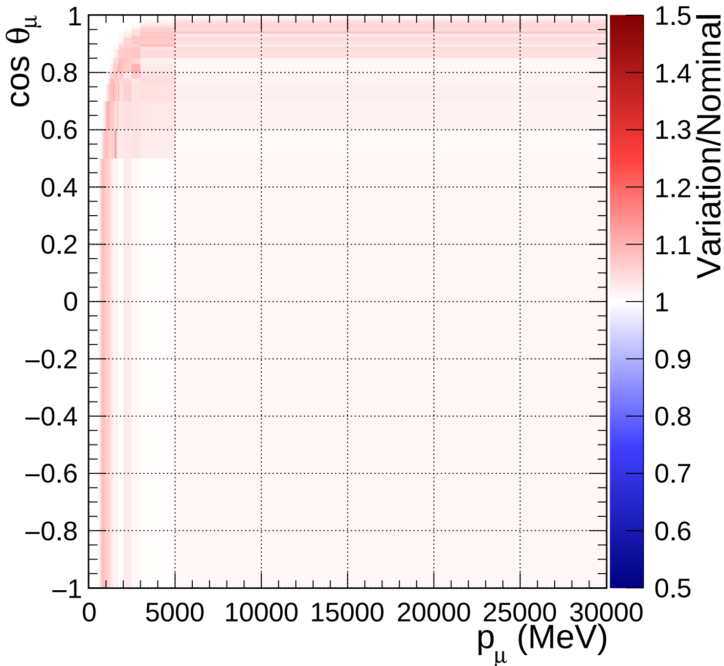
FGD1_numuCC_0pi_Q2_norm_7_1.4
