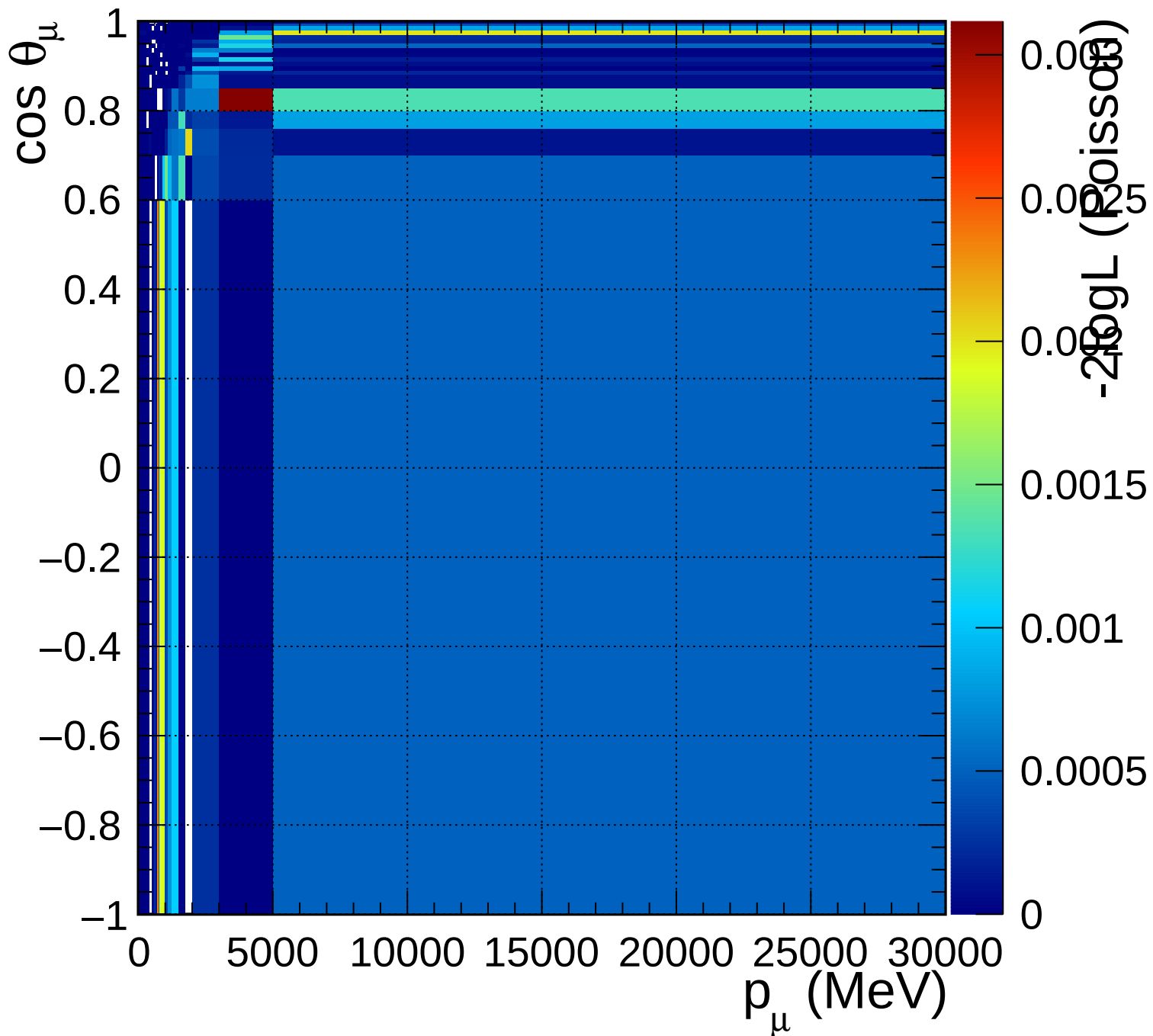
FGD1_numuCC_other_Q2_norm_7_0.6
