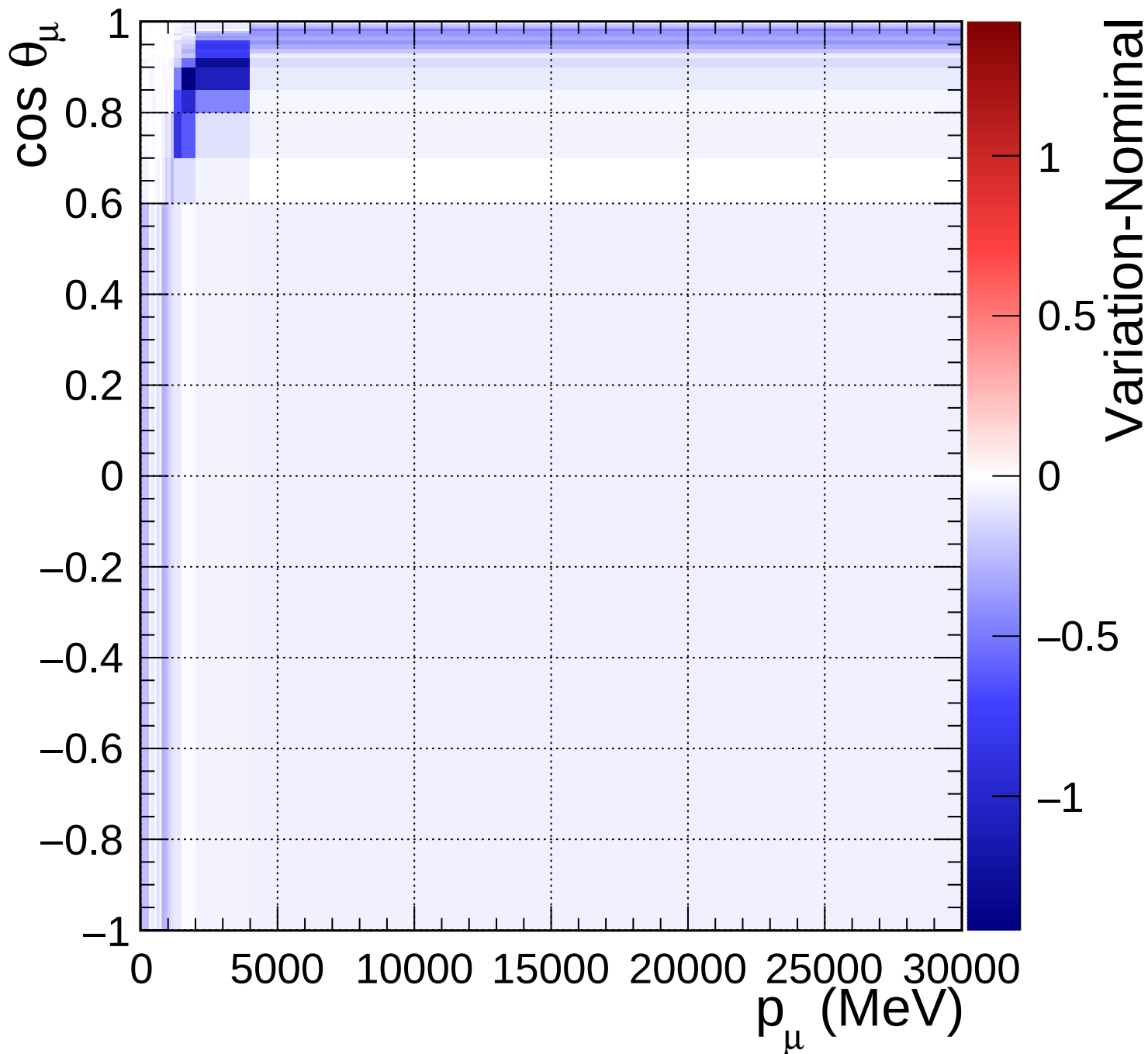
FGD1_anti-numuCC_0pi_Q2_norm_7_0.6
