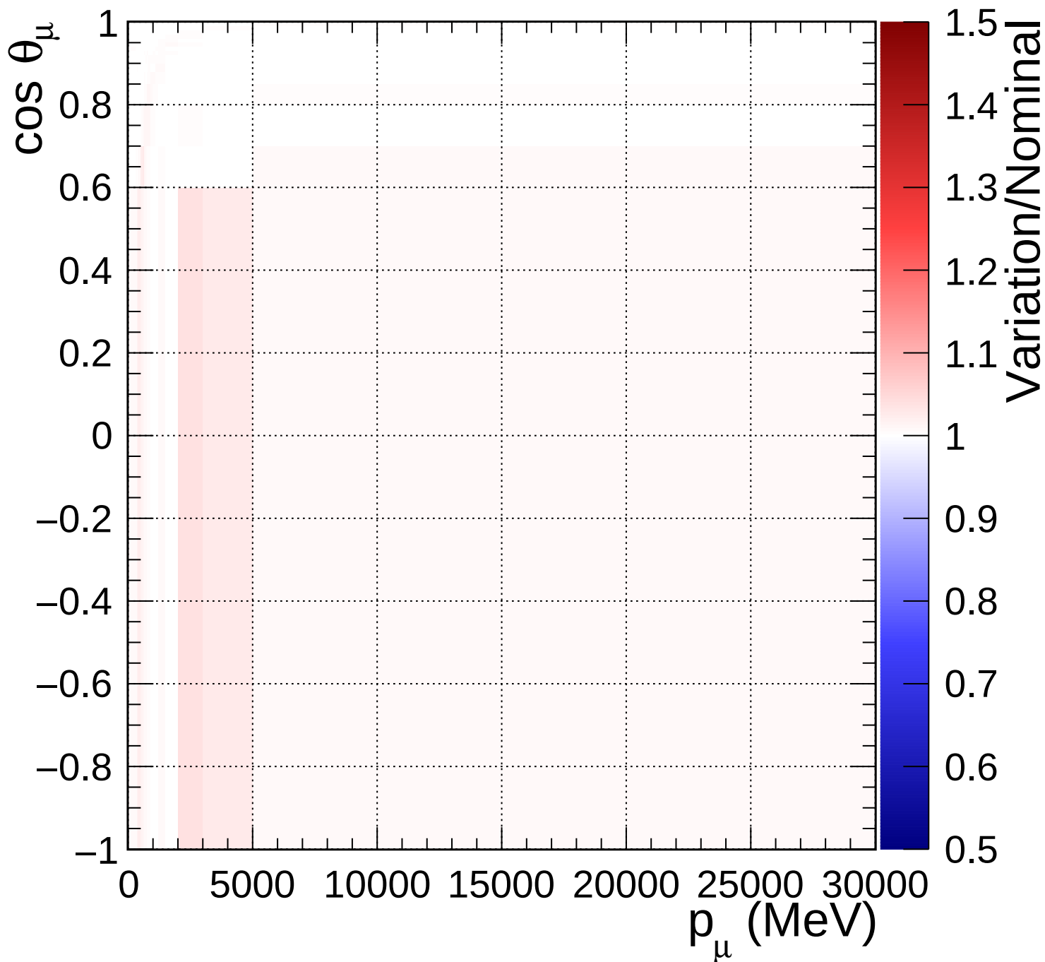
FGD2_numuCC_1pi_Q2_norm_5_1.33
