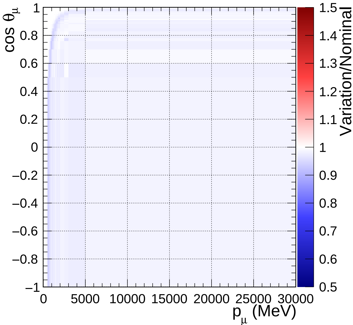
FGD1_numuCC_0pi_Q2_norm_6_0.82
