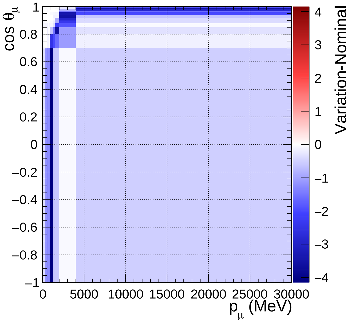
FGD2_NuMuBkg_CC0pi_in_AntiNu_Mode_Q2_norm_7_-0.2
