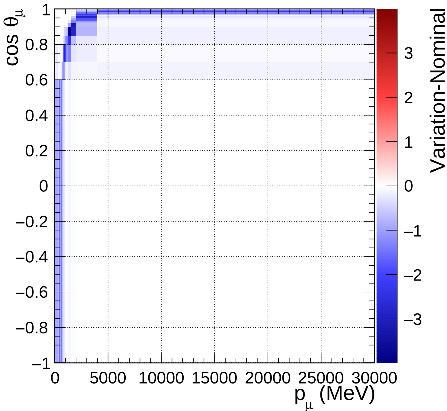
FGD2_anti-numuCC_0pi_Q2_norm_6_0.46
