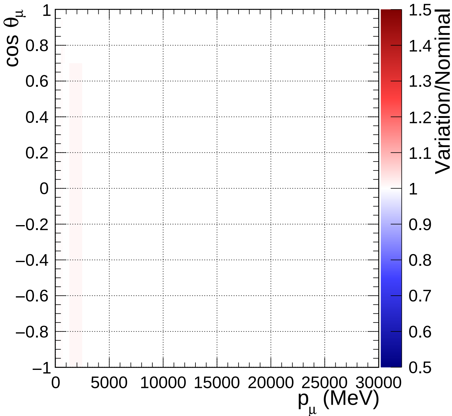
FGD1_anti-numuCC_1pi_Q2_norm_5_1.33
