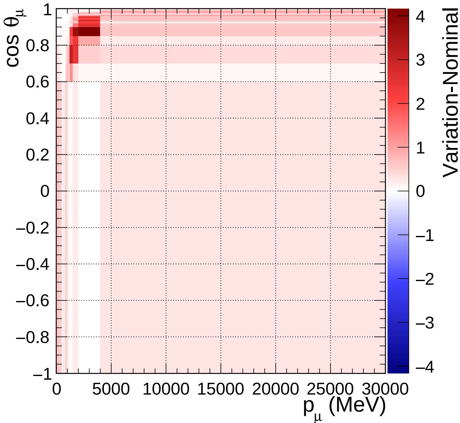
FGD2_anti-numuCC_0pi_Q2_norm_7_2.2
