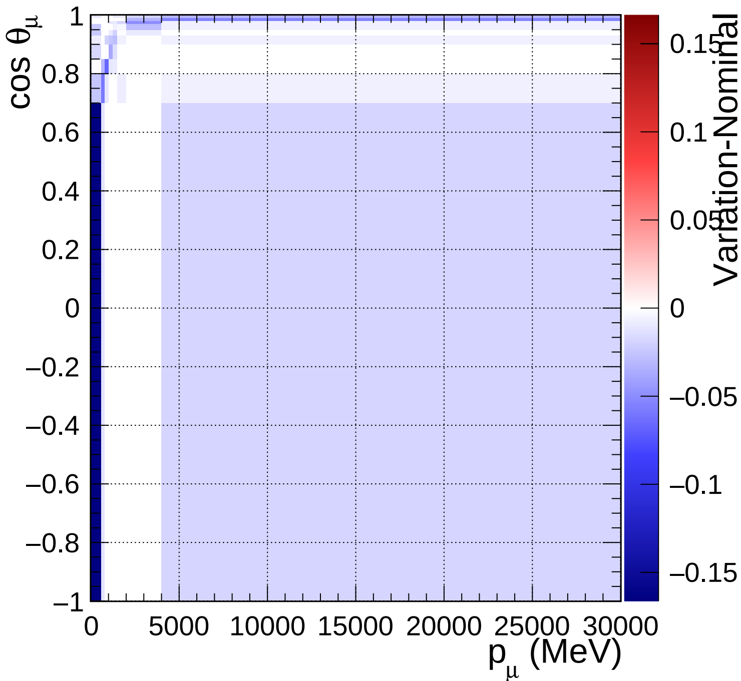
FGD2_anti-numuCC_other_Q2_norm_5_0.89
