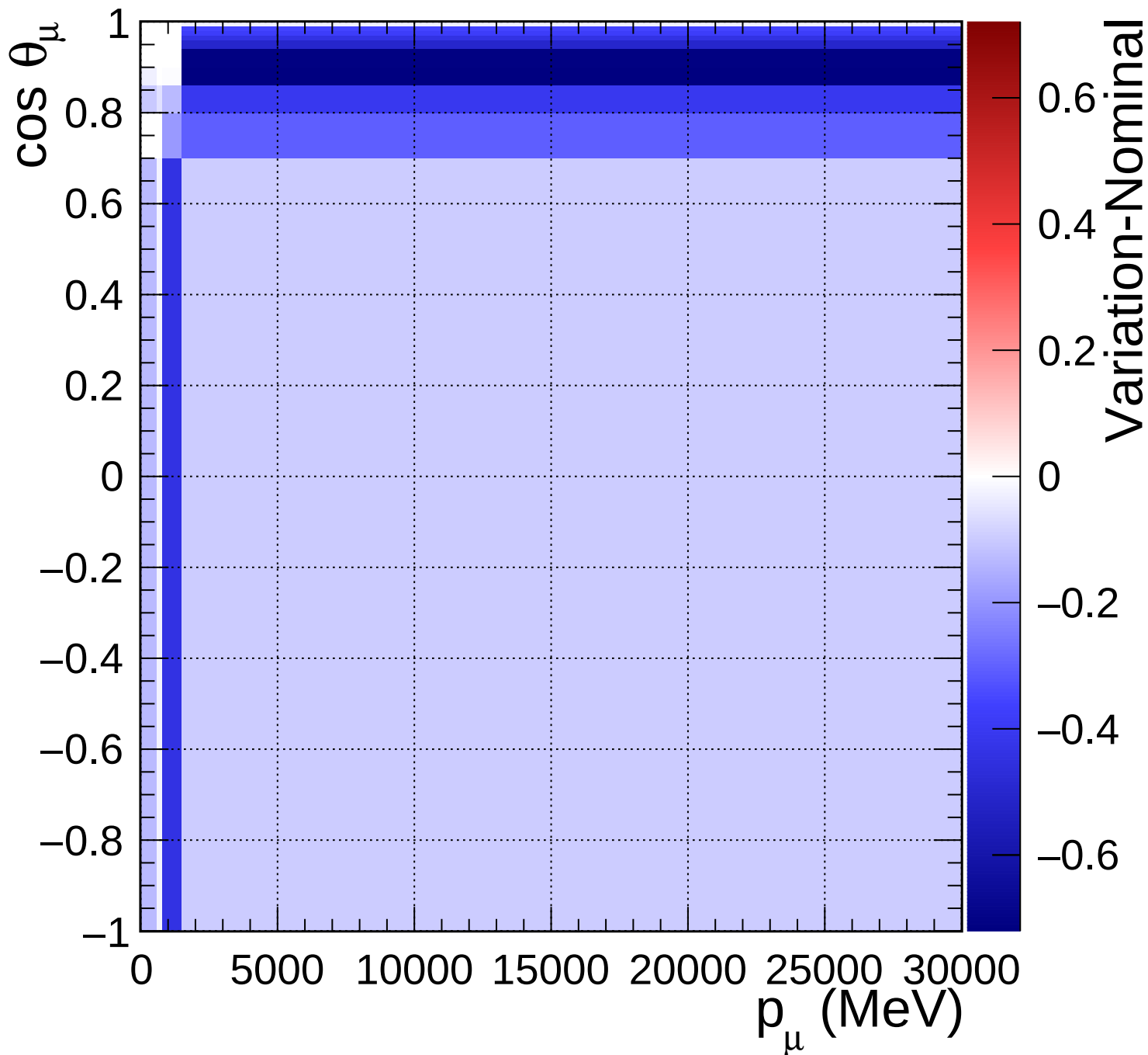
FGD1_NuMuBkg_CC1pi_in_AntiNu_Mode_Q2_norm_7_0.6
