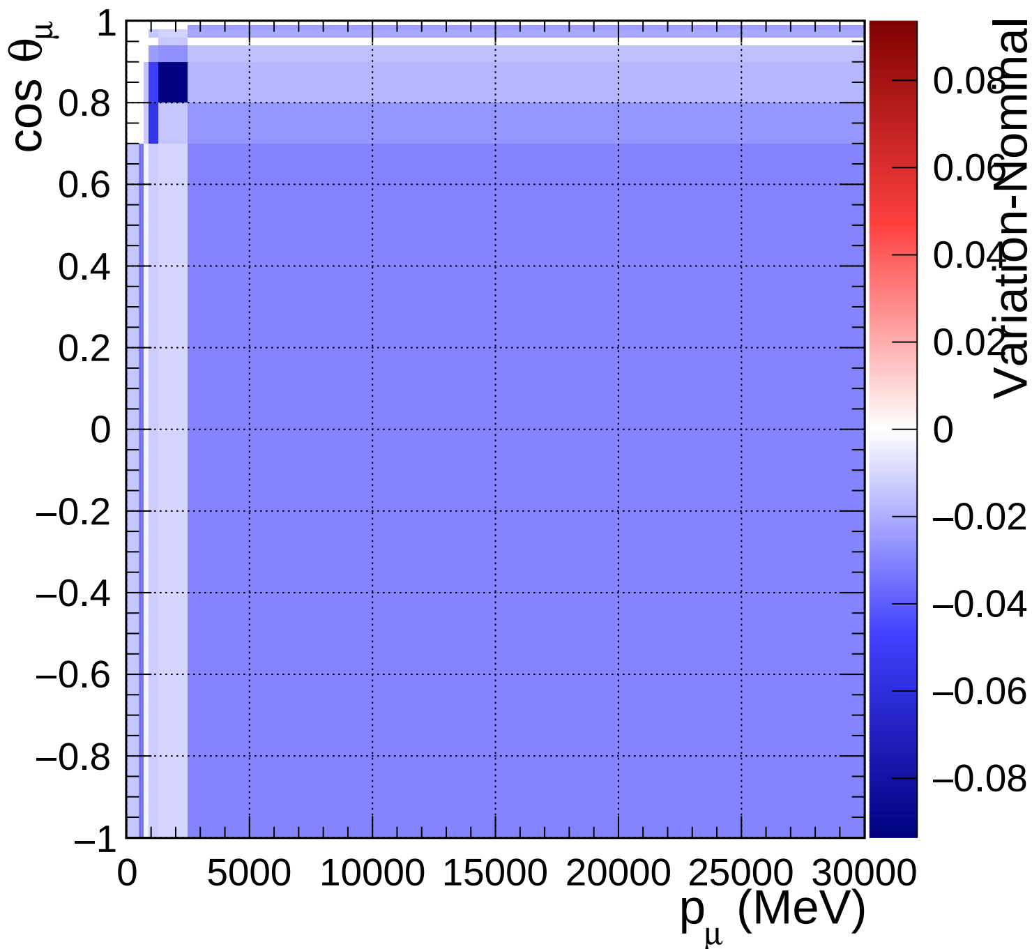
FGD1_anti-numuCC_1pi_Q2_norm_6_0.82
