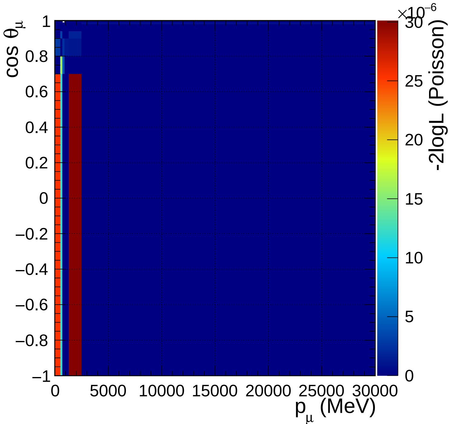
FGD1_anti-numuCC_1pi_Q2_norm_5_1.11
