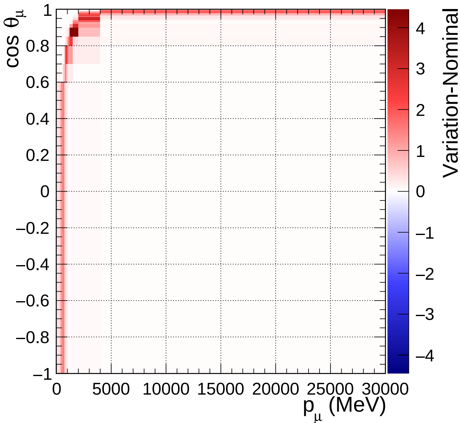
FGD1_anti-numuCC_0pi_Q2_norm_6_1.54
