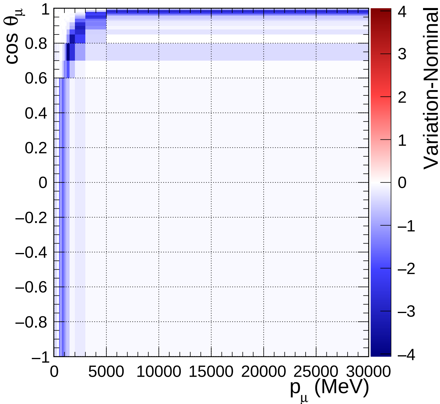
FGD1_numuCC_1pi_Q2_norm_7_-0.2
