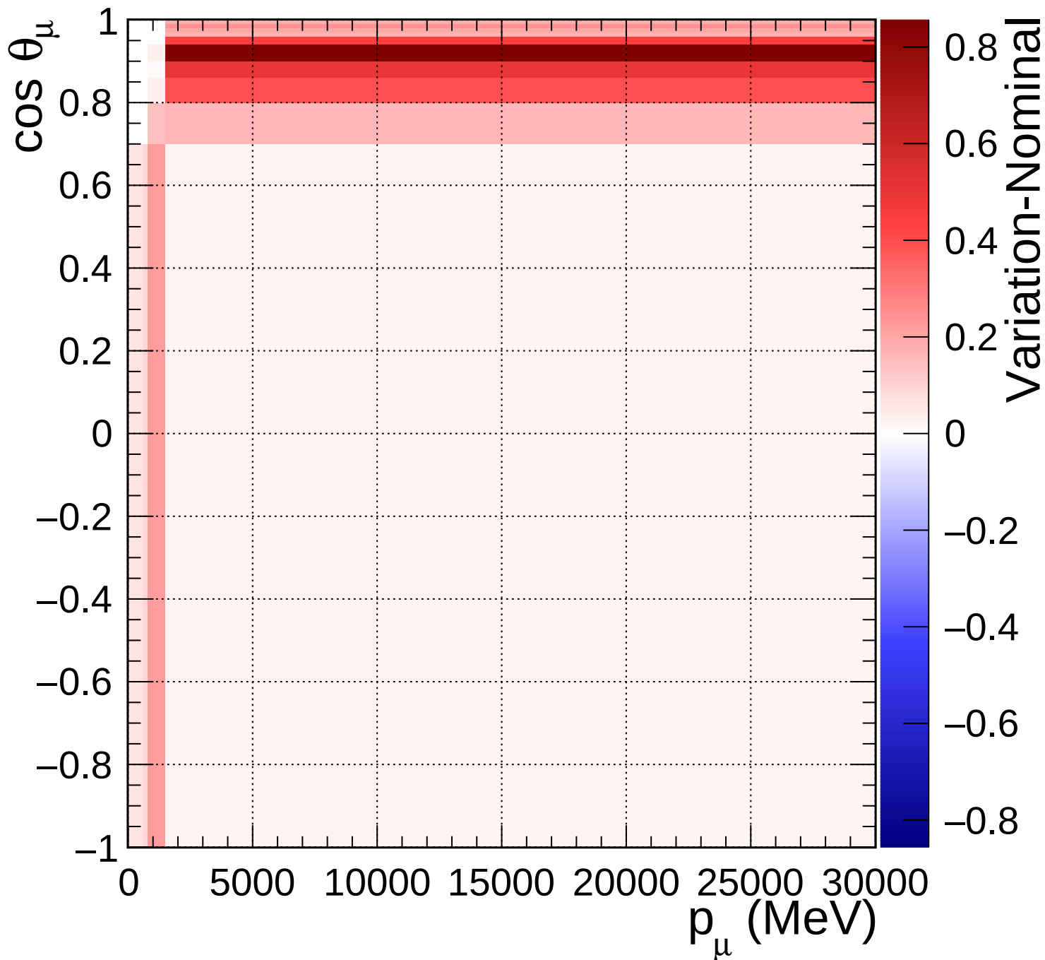
FGD2_NuMuBkg_CC1pi_in_AntiNu_Mode_Q2_norm_7_1.4
