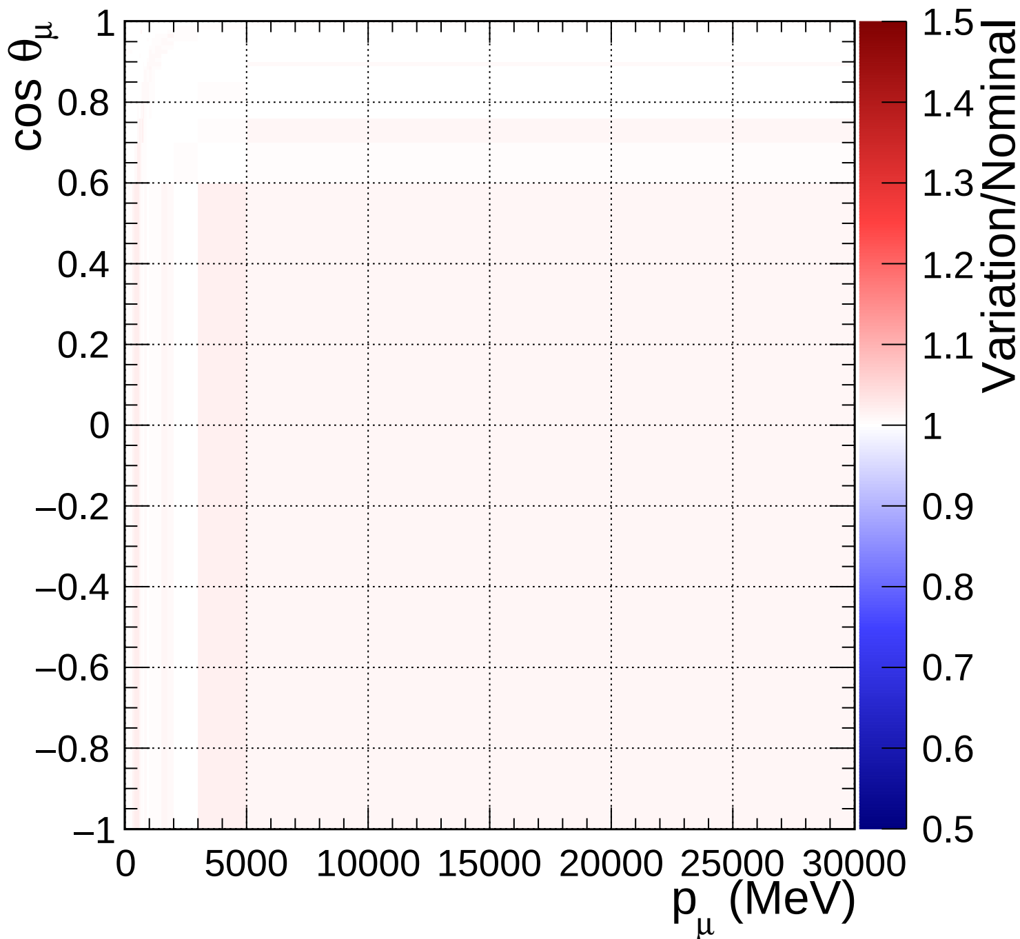
FGD1_numuCC_other_Q2_norm_5_1.33
