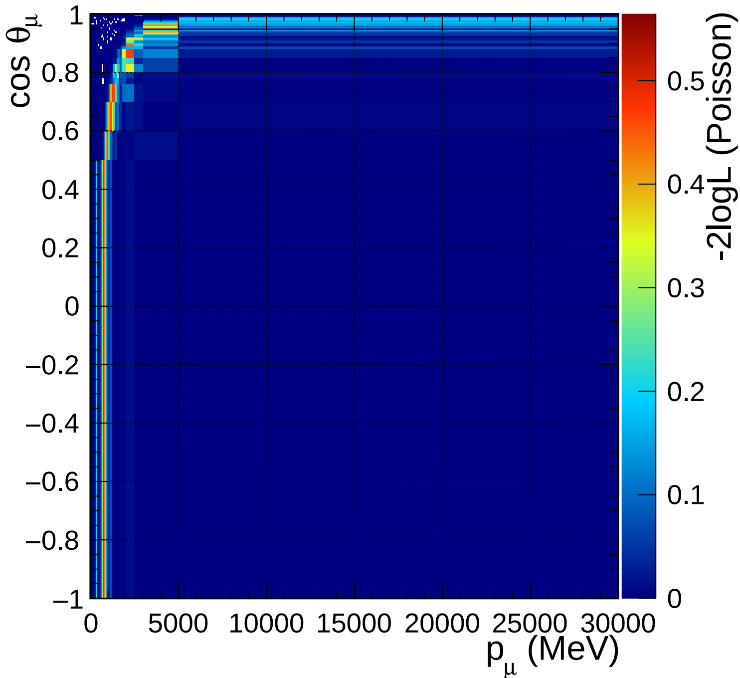
FGD2_numuCC_0pi_Q2_norm_7_-0.2
