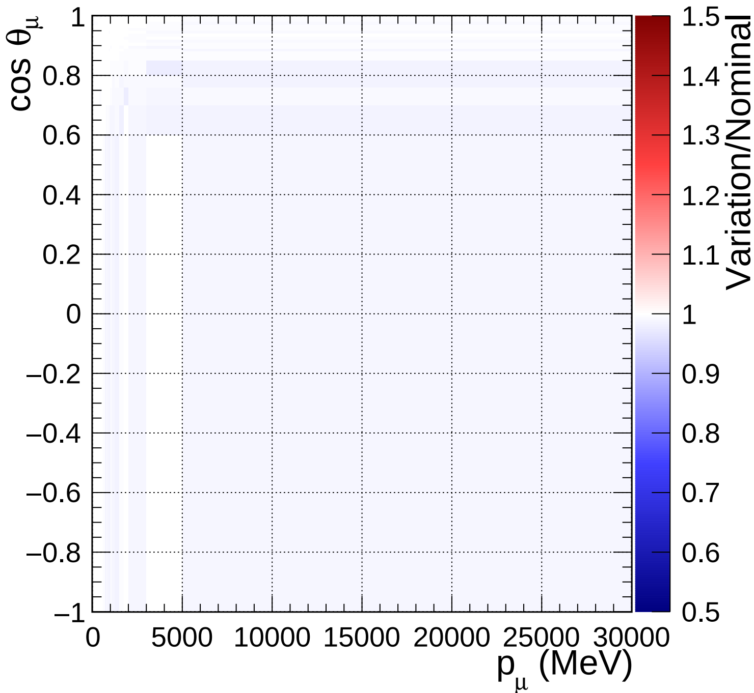
FGD1_numuCC_other_Q2_norm_7_0.6
