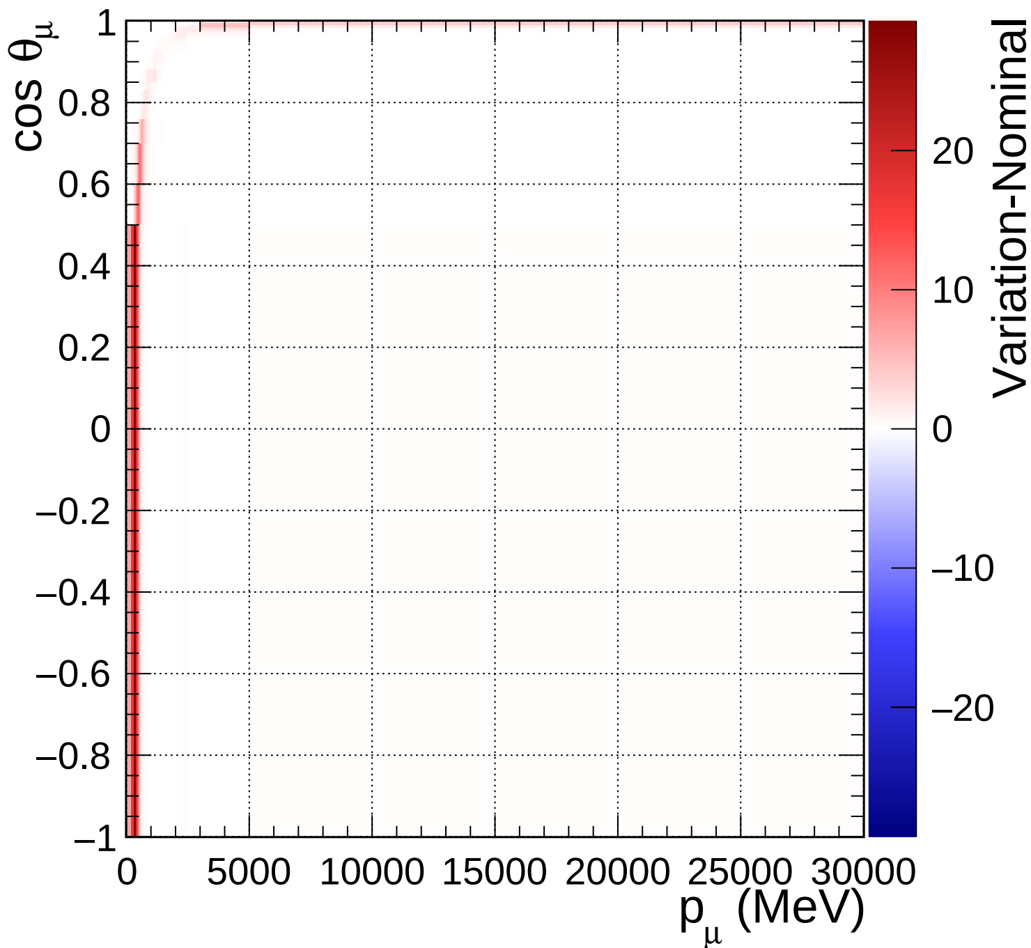
FGD2_numuCC_0pi_Q2_norm_5_1.11
