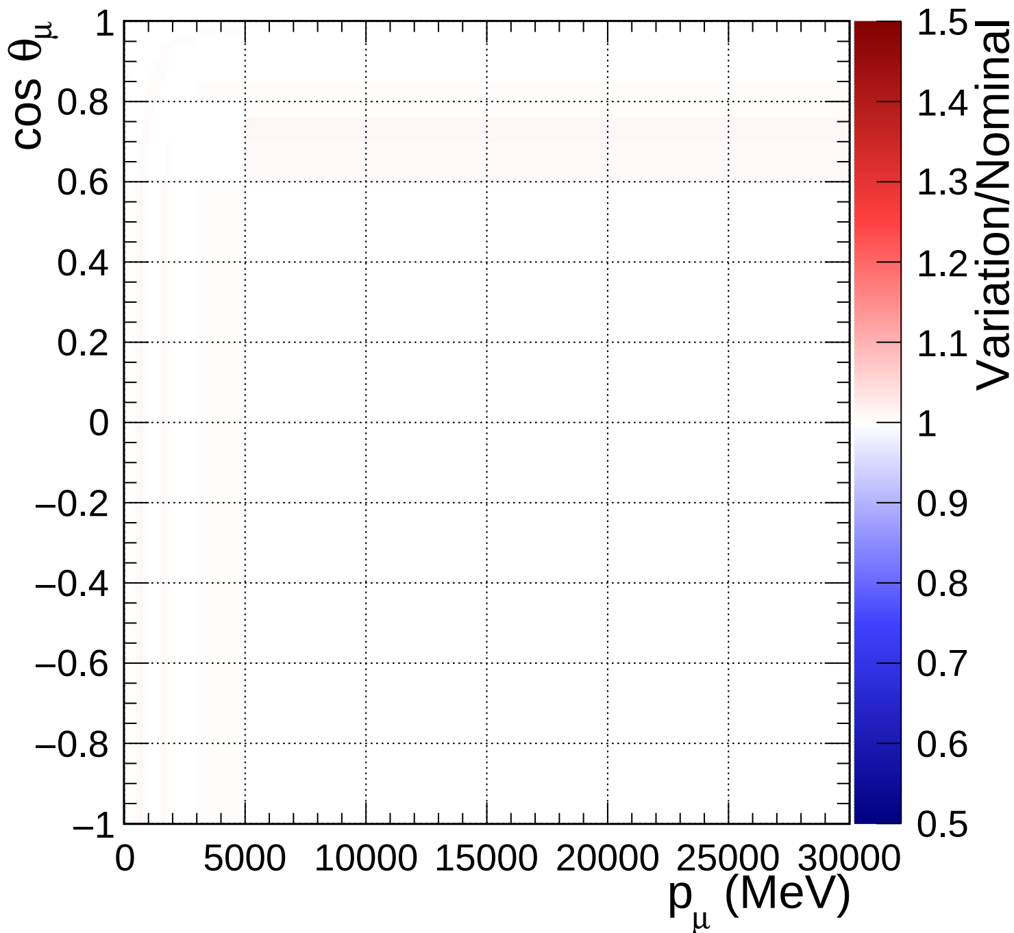
FGD1_numuCC_other_Q2_norm_6_1.18
