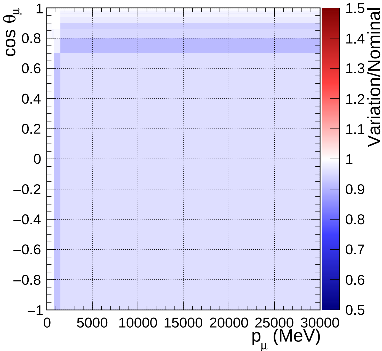
FGD1_NuMuBkg_CC1pi_in_AntiNu_Mode_Q2_norm_7_-0.2
