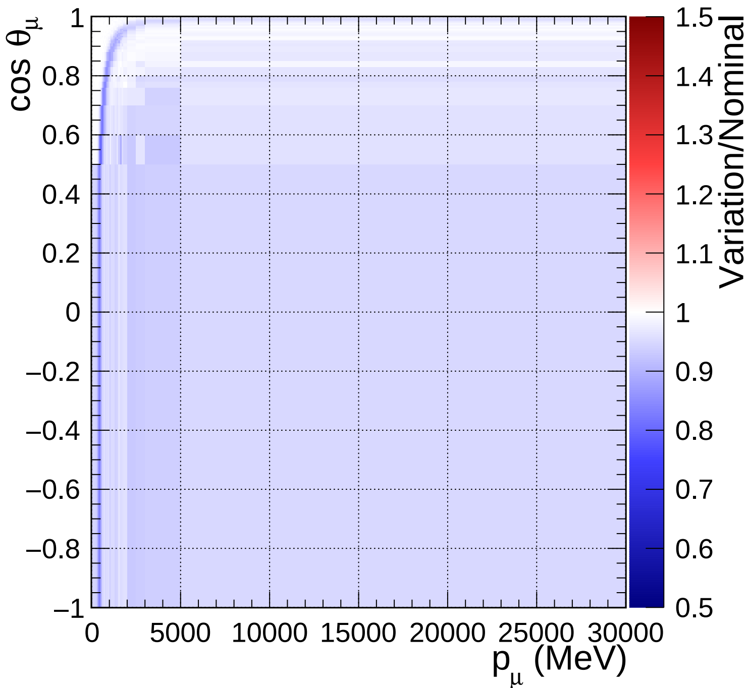
FGD2_numuCC_0pi_Q2_norm_5_0.67
