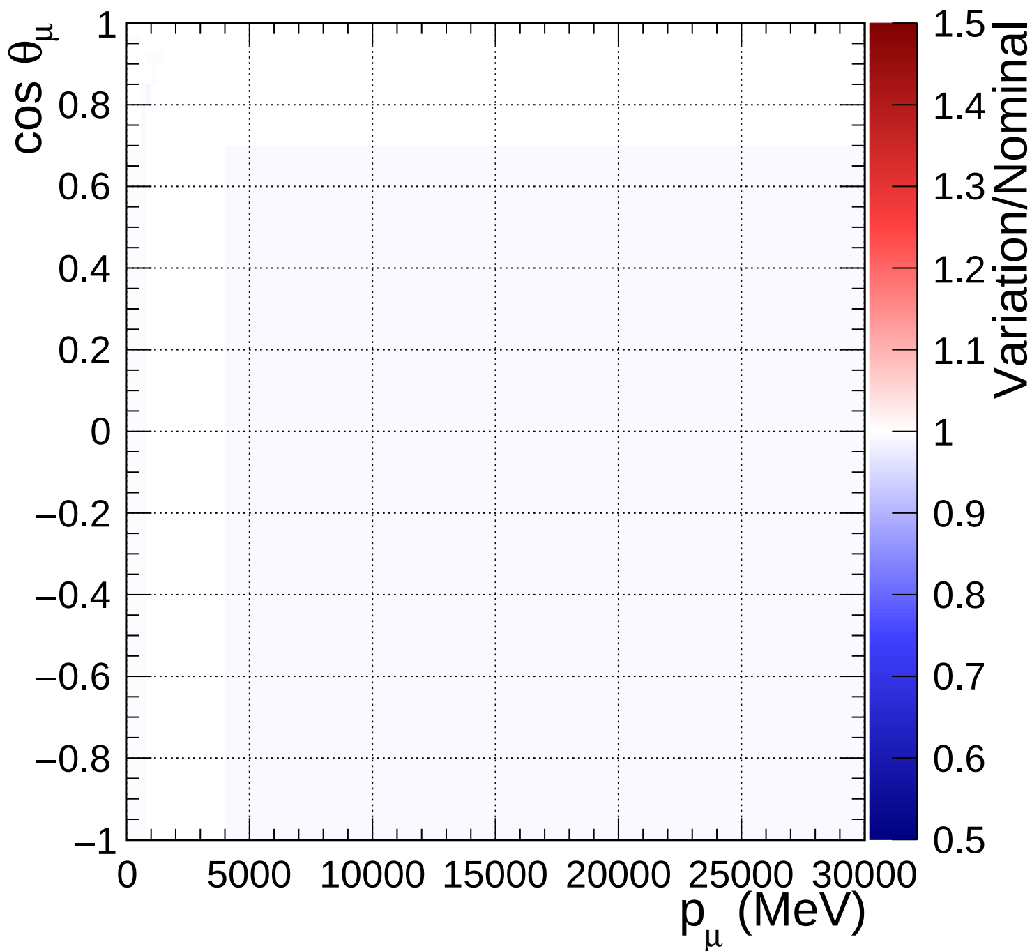
FGD2_anti-numuCC_other_Q2_norm_5_0.89
