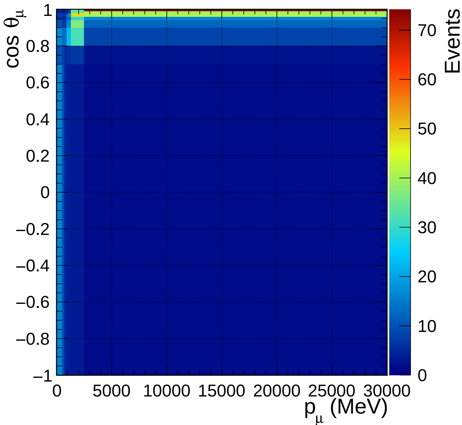
FGD1_anti-numuCC_1pi_Q2_norm_6_1
