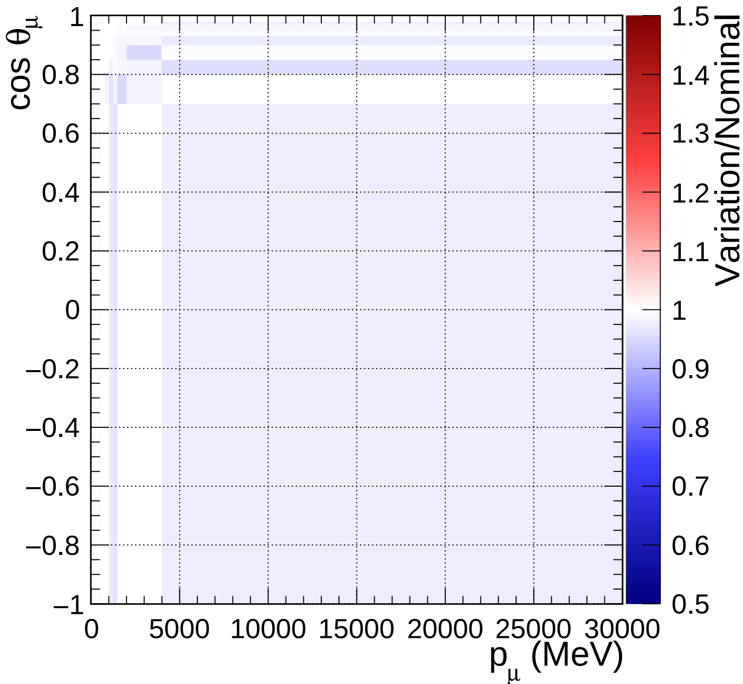
FGD2_anti-numuCC_other_Q2_norm_7_-0.2
