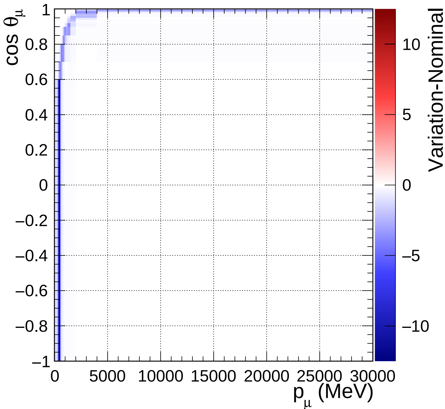
FGD1_anti-numuCC_0pi_Q2_norm_5_0.67
