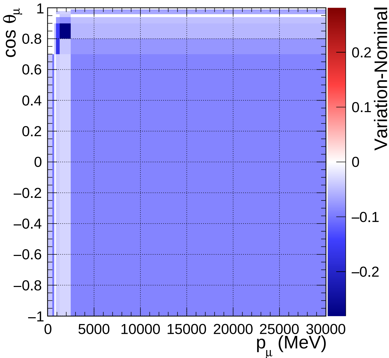
FGD1_anti-numuCC_1pi_Q2_norm_6_0.46
