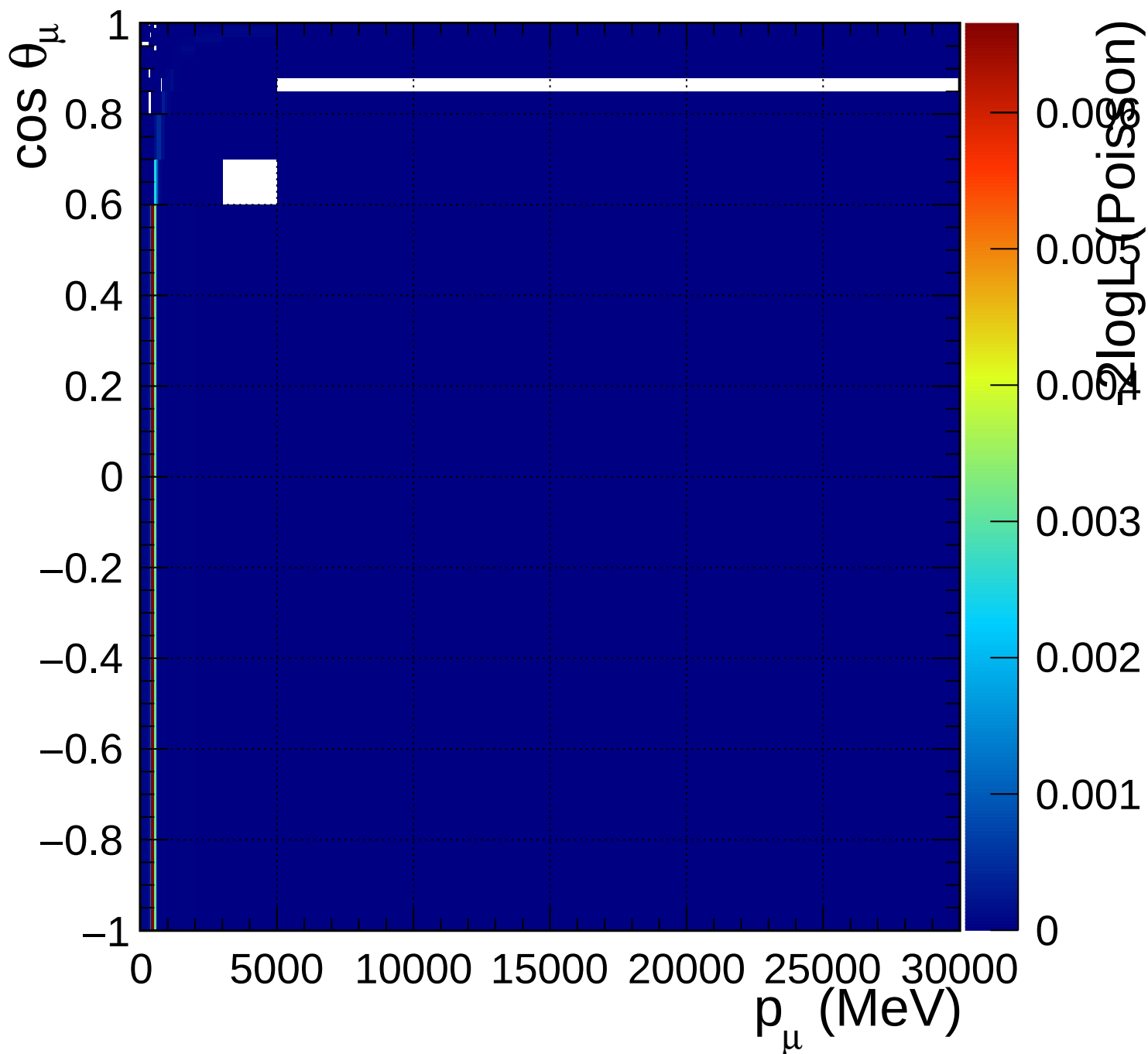
FGD1_numuCC_1pi_Q2_norm_5_0.89
