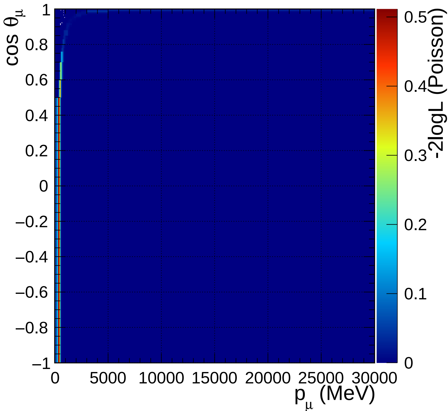
FGD2_numuCC_0pi_Q2_norm_5_1.11
