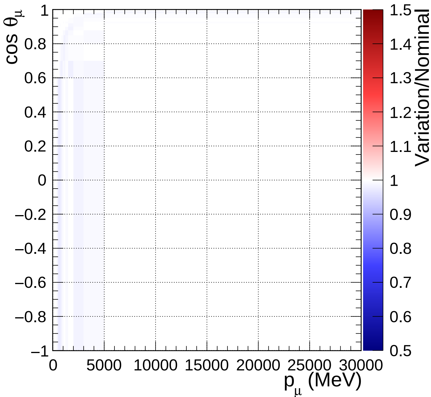
FGD1_numuCC_1pi_Q2_norm_6_0.46
