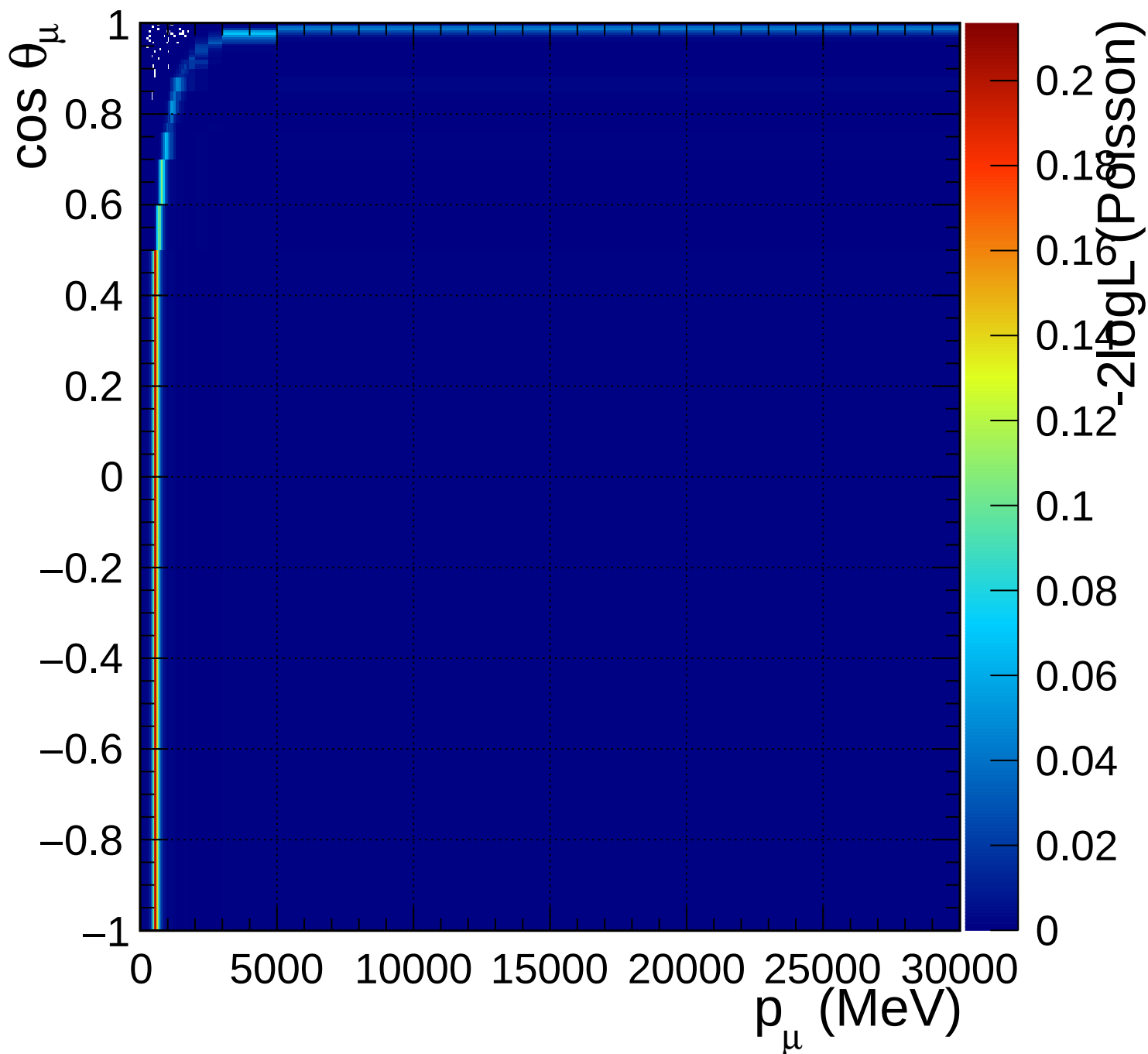
FGD1_numuCC_0pi_Q2_norm_6_1.18
