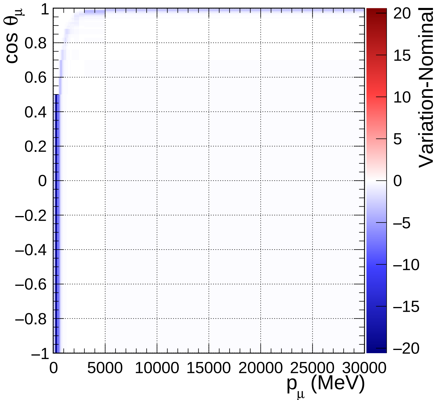
FGD2_numuCC_0pi_Q2_norm_6_0.82
