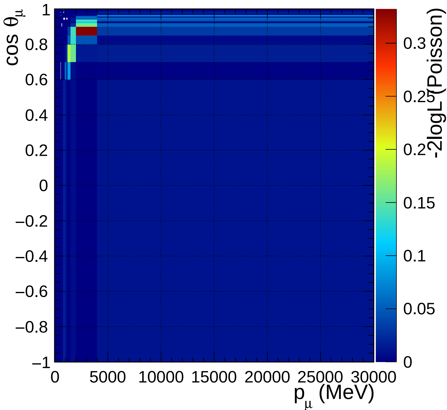
FGD2_anti-numuCC_0pi_Q2_norm_7_-0.2
