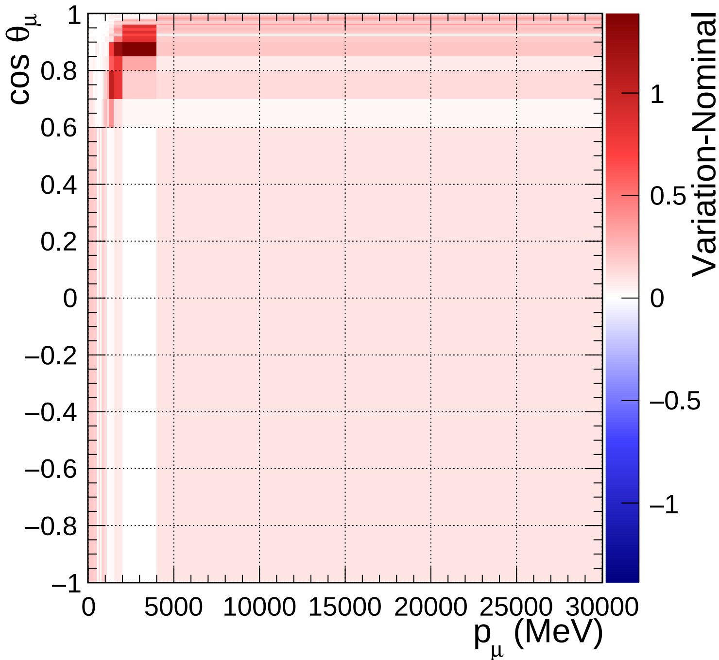
FGD2_anti-numuCC_0pi_Q2_norm_7_1.4
