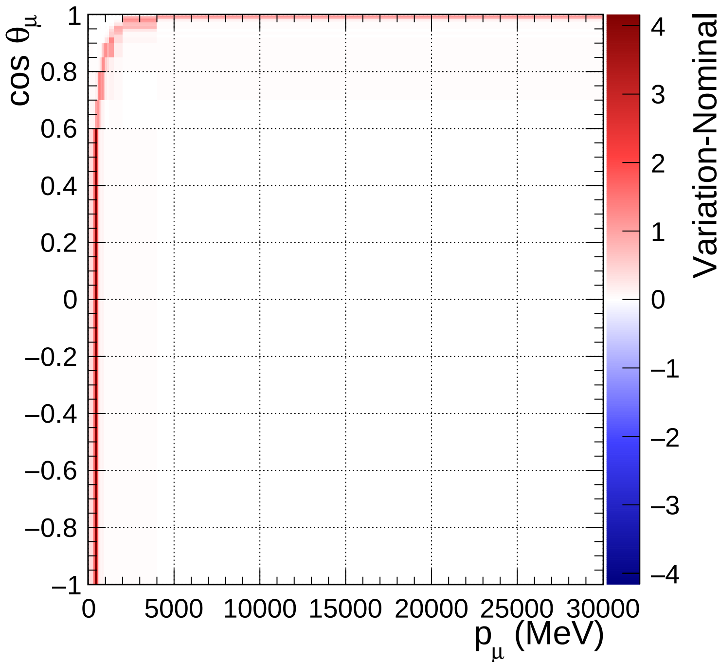
FGD1_anti-numuCC_0pi_Q2_norm_5_1.11
