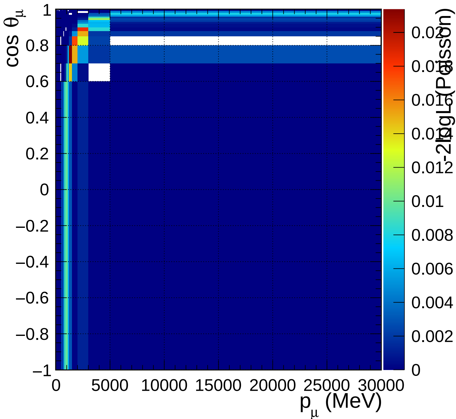
FGD1_numuCC_1pi_Q2_norm_7_1.4
