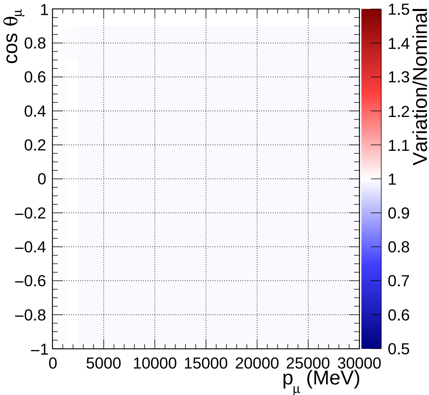
FGD2_anti-numuCC_1pi_Q2_norm_6_0.82
