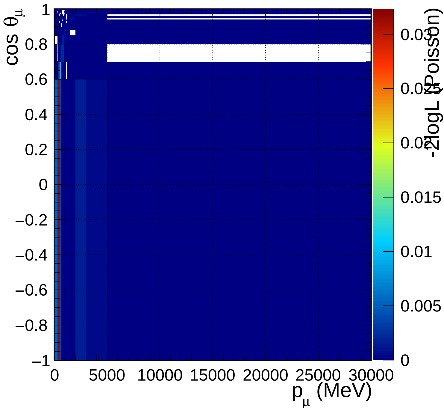
FGD2_numuCC_1pi_Q2_norm_5_0.67
