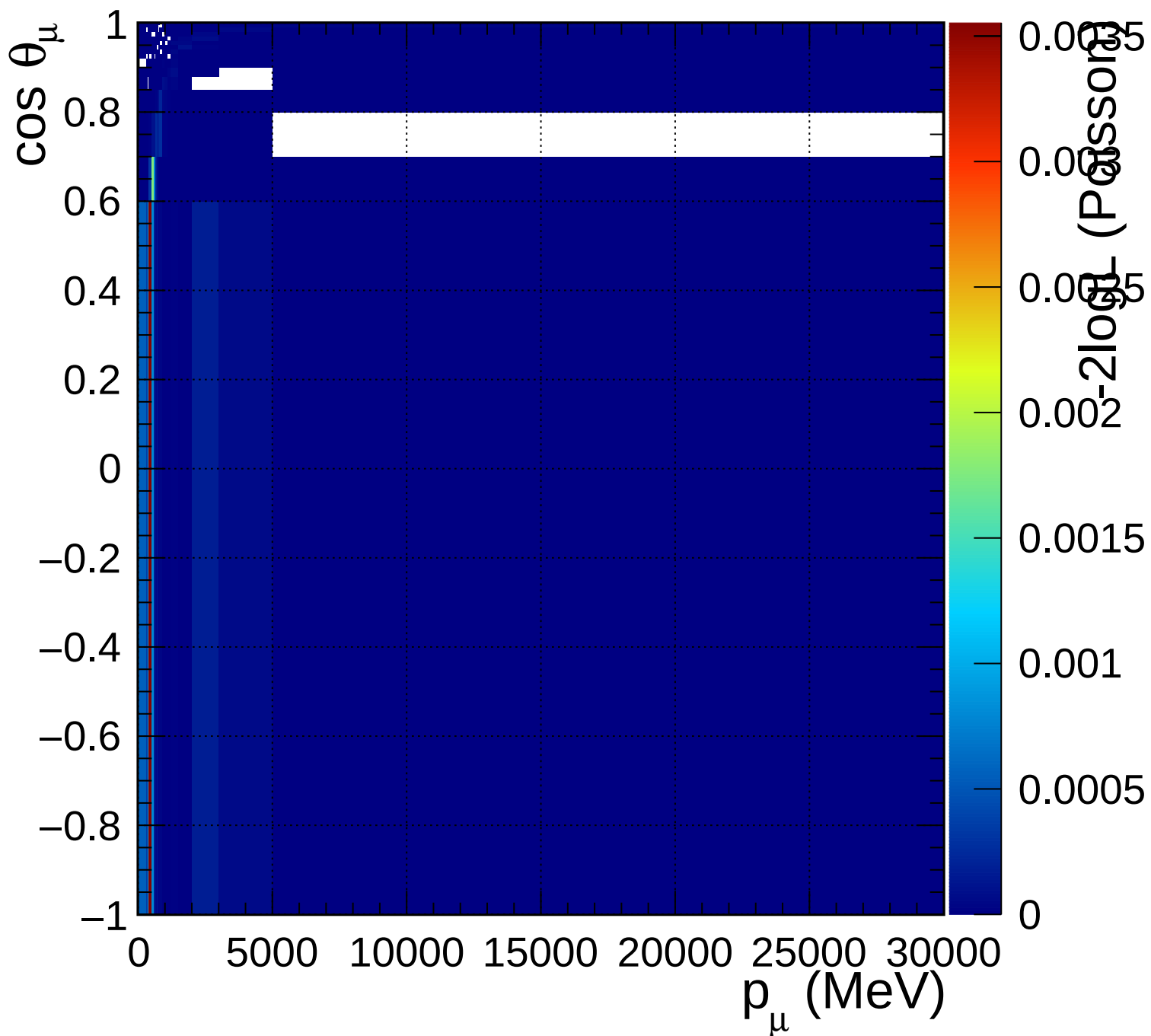
FGD2_numuCC_1pi_Q2_norm_5_0.89
