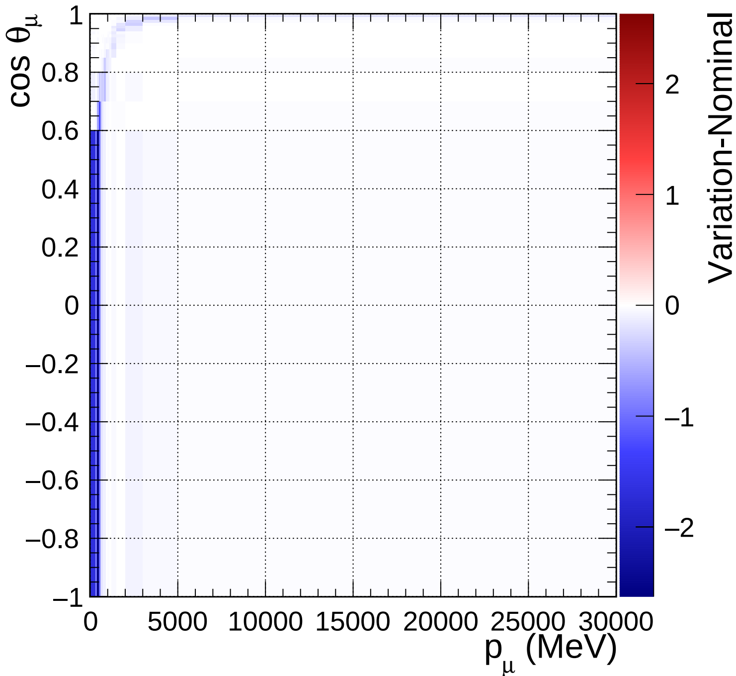
FGD2_numuCC_1pi_Q2_norm_5_0.67
