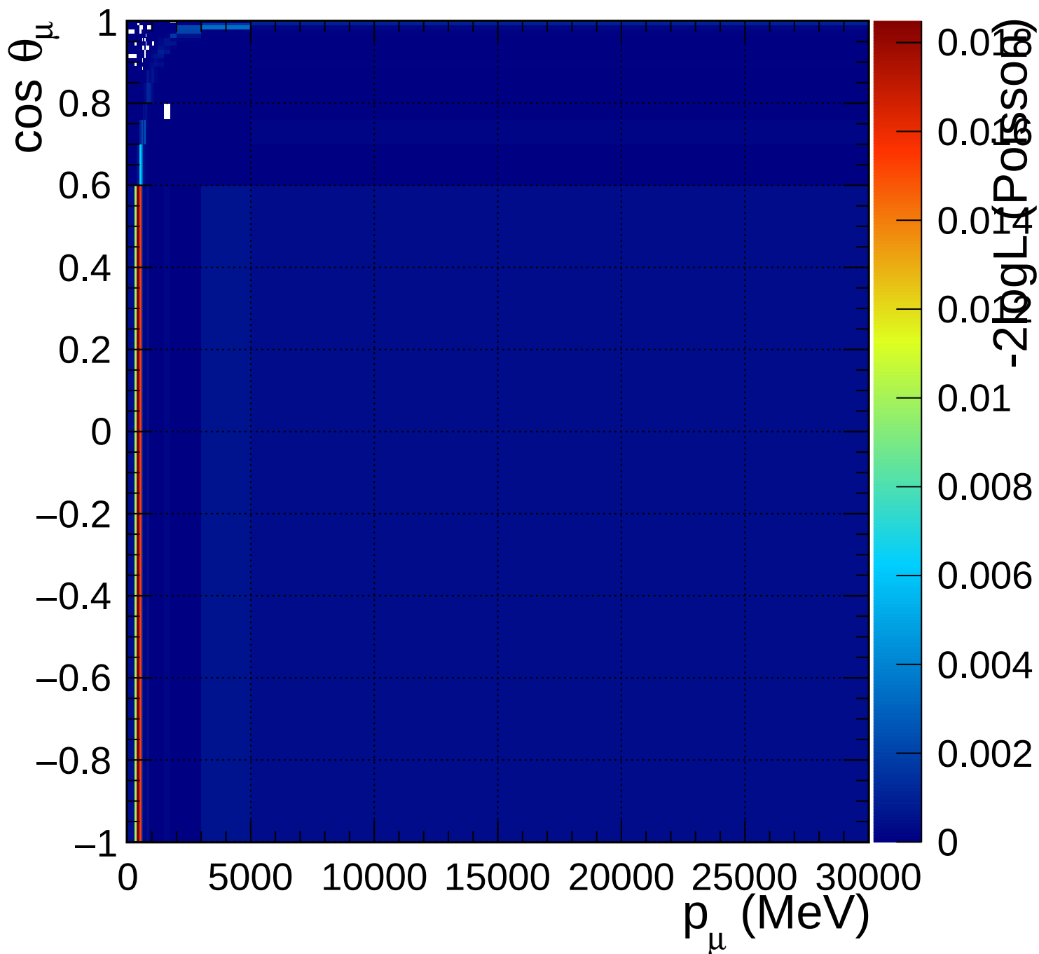
FGD1_numuCC_other_Q2_norm_5_0.67
