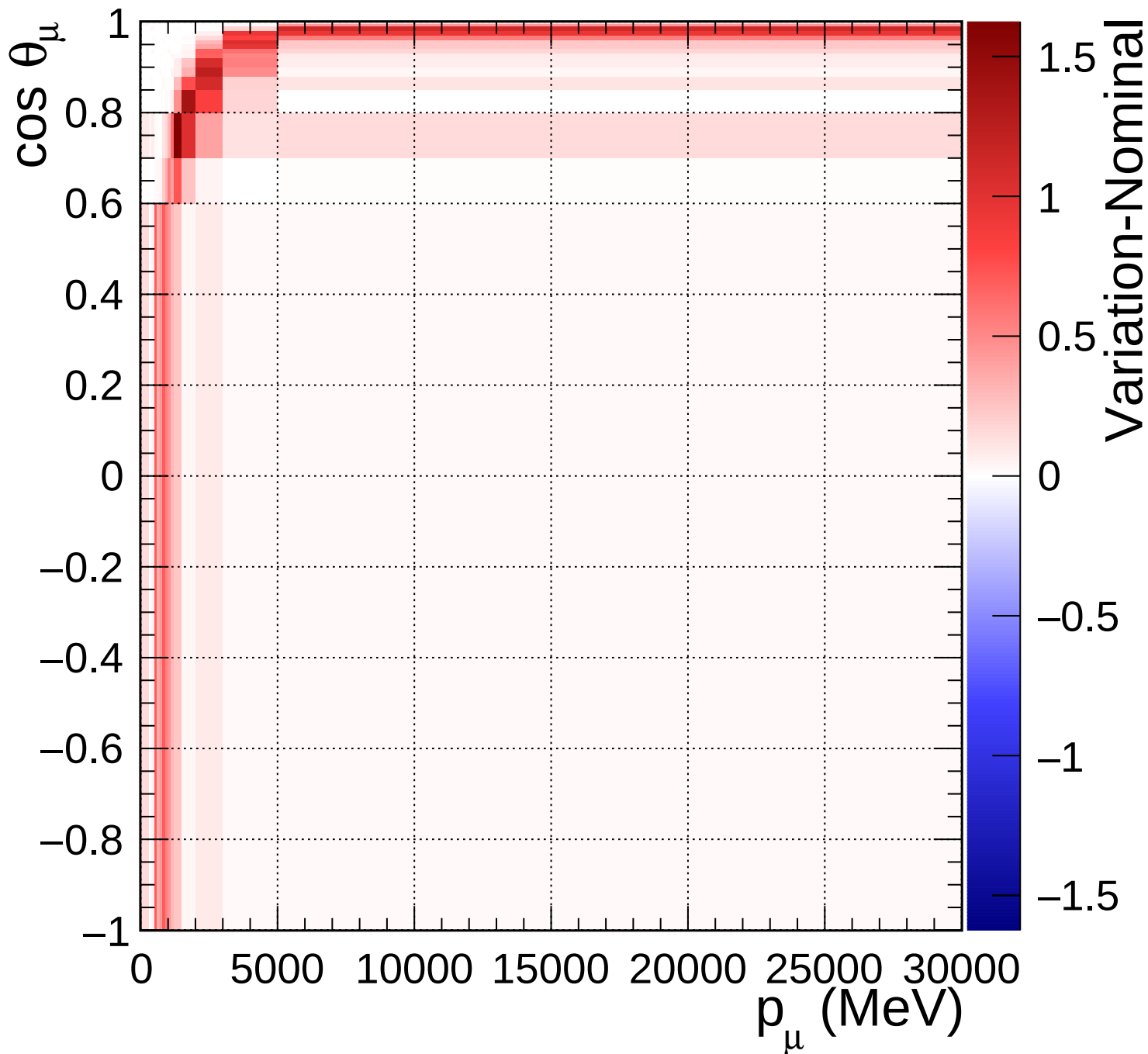
FGD1_numuCC_1pi_Q2_norm_7_1.4
