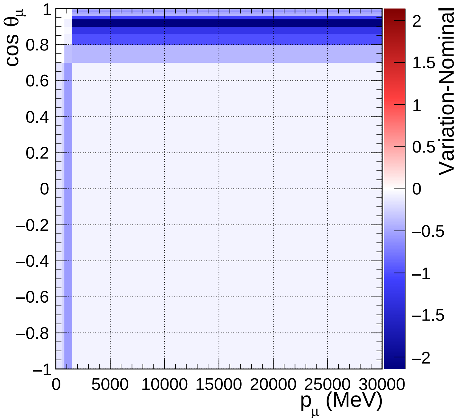
FGD2_NuMuBkg_CC1pi_in_AntiNu_Mode_Q2_norm_7_-0.2
