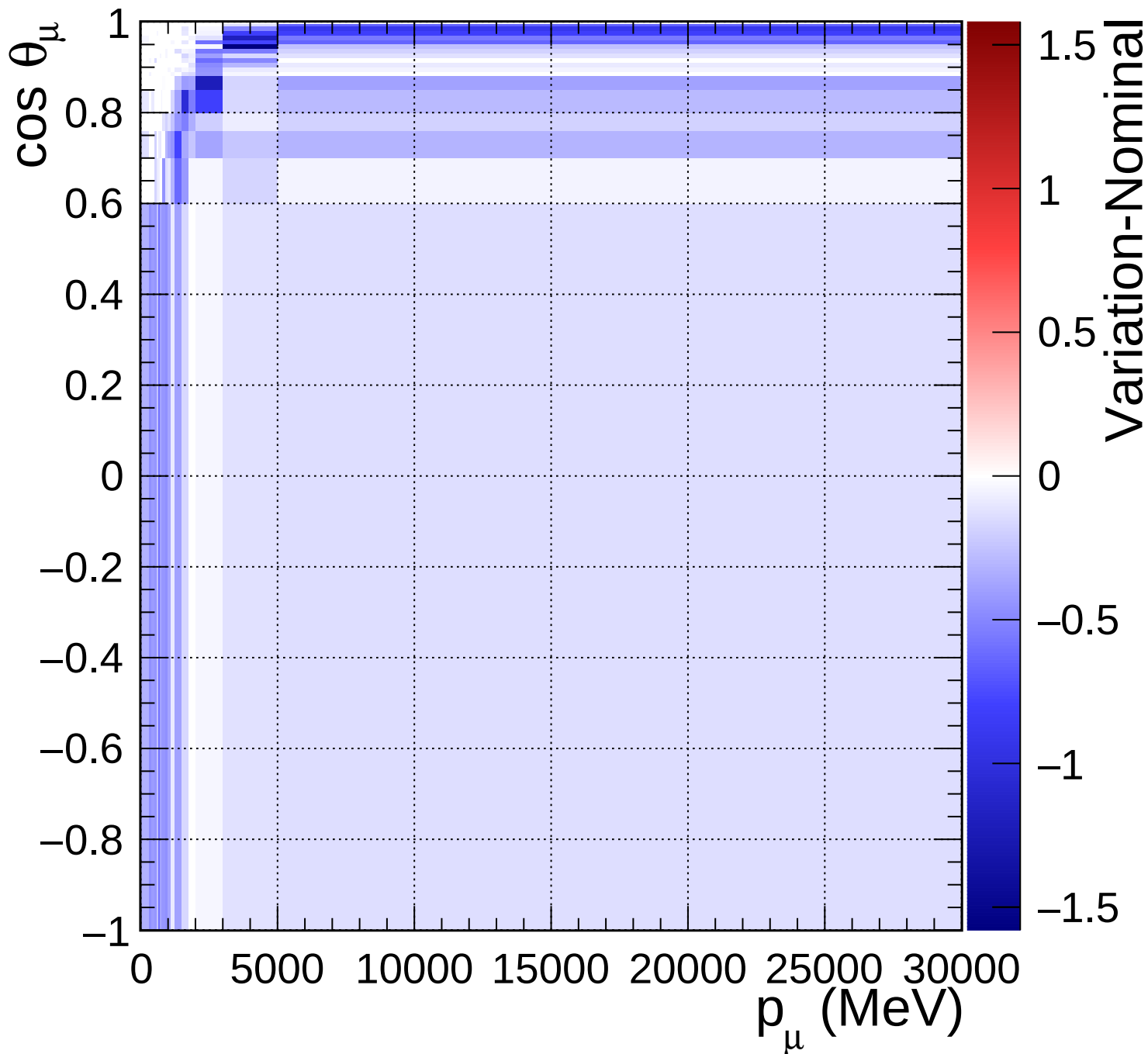
FGD2_numuCC_other_Q2_norm_7_-0.2
