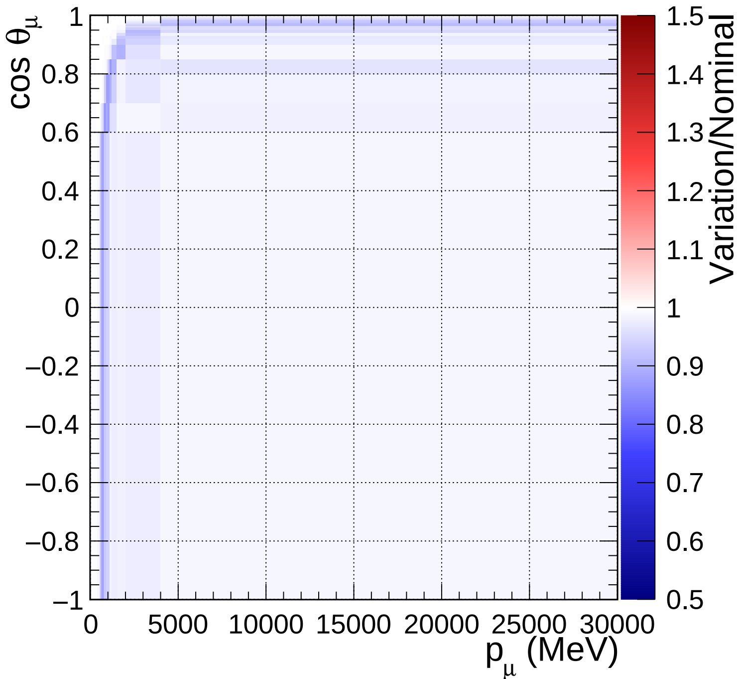
FGD1_anti-numuCC_0pi_Q2_norm_6_0.46
