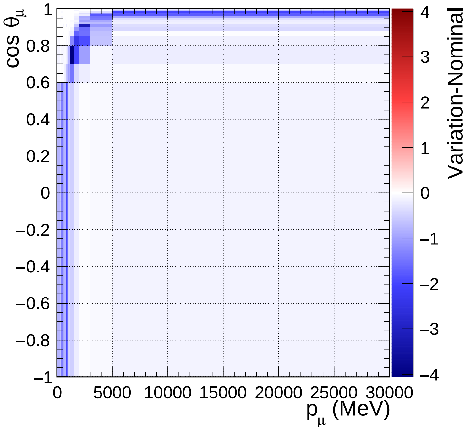
FGD2_numuCC_1pi_Q2_norm_7_-0.2
