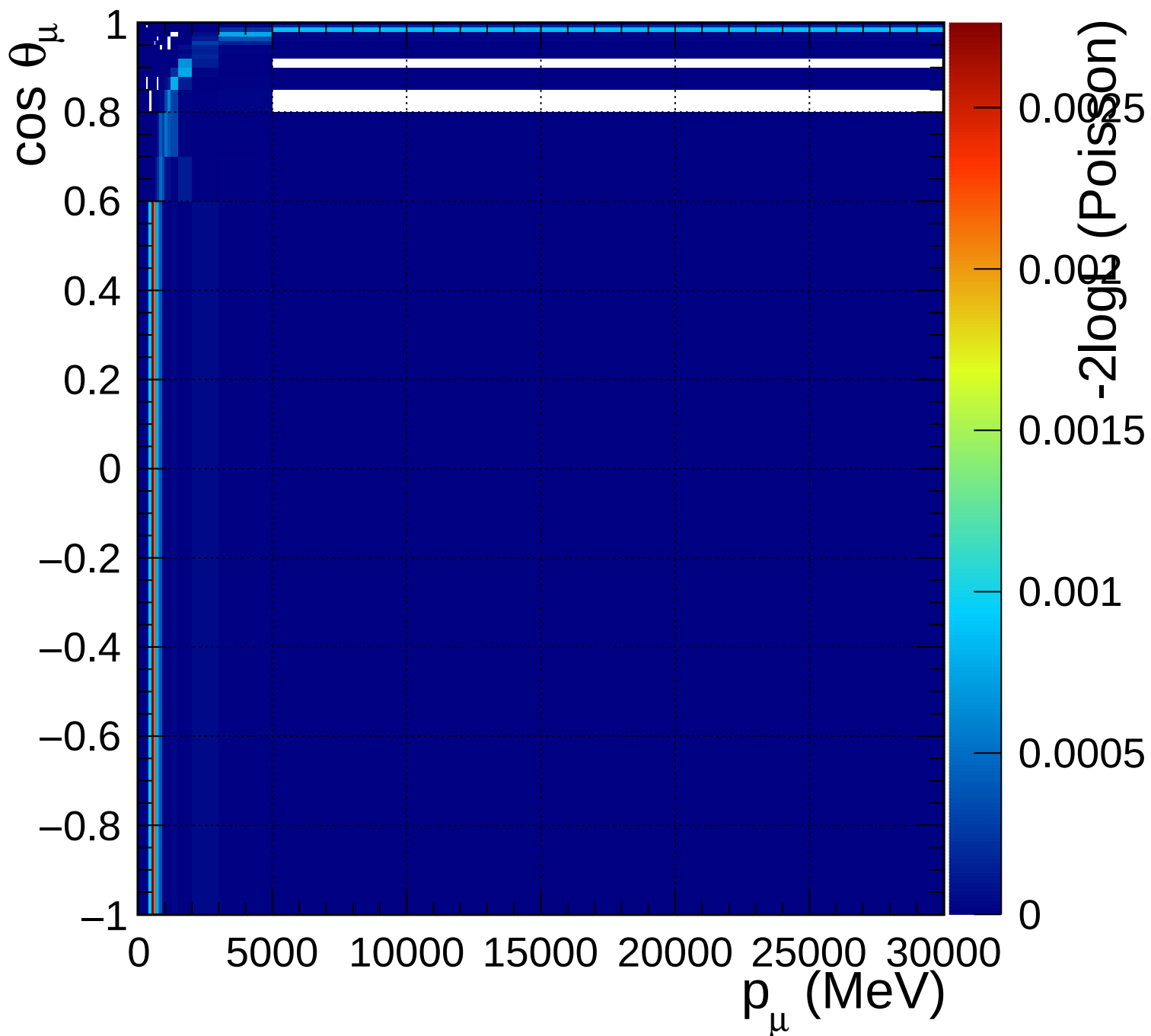
FGD1_numuCC_1pi_Q2_norm_6_1.18
