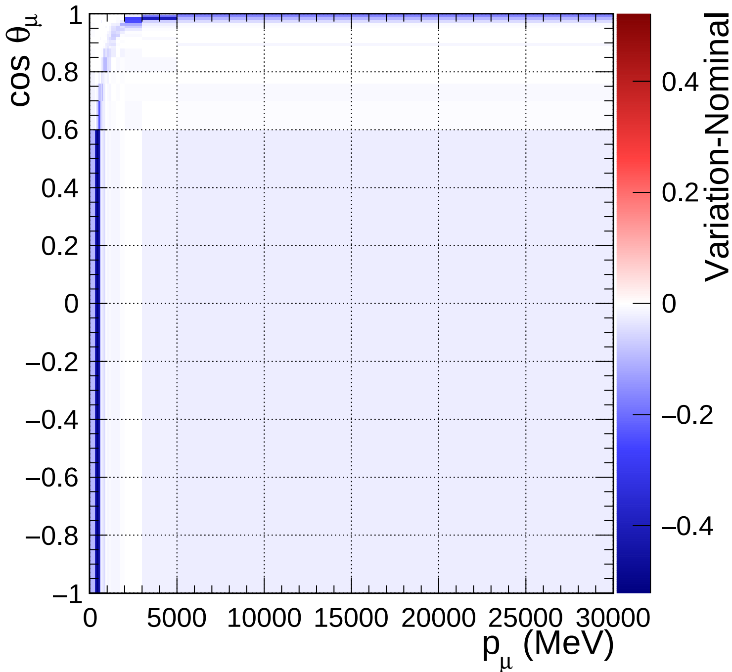
FGD1_numuCC_other_Q2_norm_5_0.89
