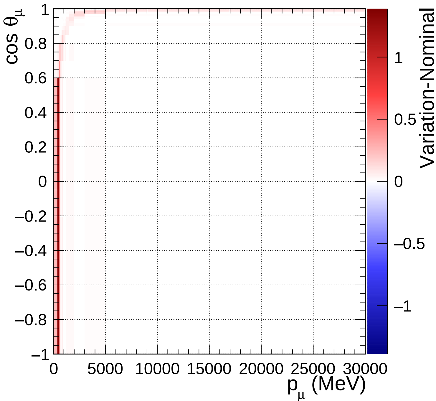
FGD1_numuCC_1pi_Q2_norm_5_1.11
