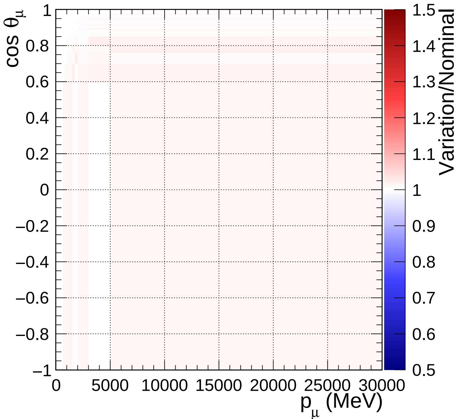
FGD1_numuCC_other_Q2_norm_7_1.4
