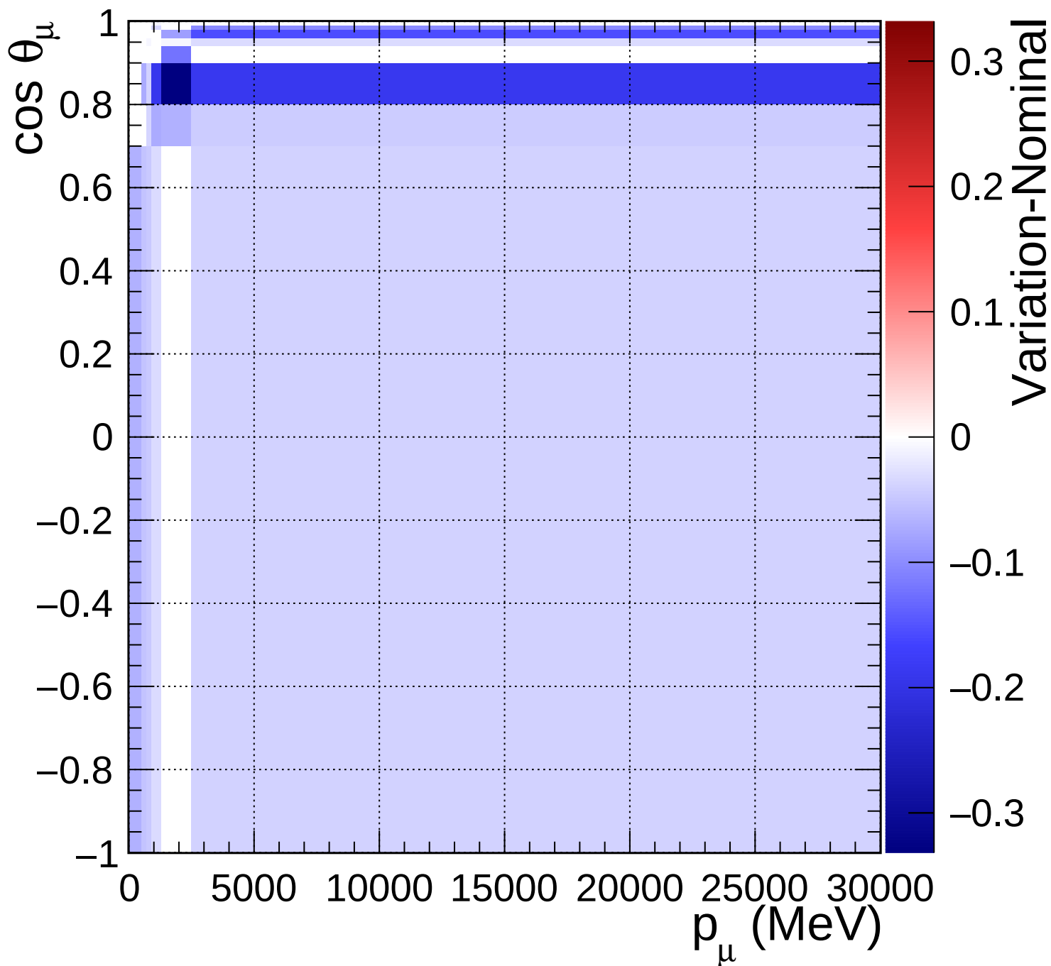
FGD2_anti-numuCC_1pi_Q2_norm_6_0.46
