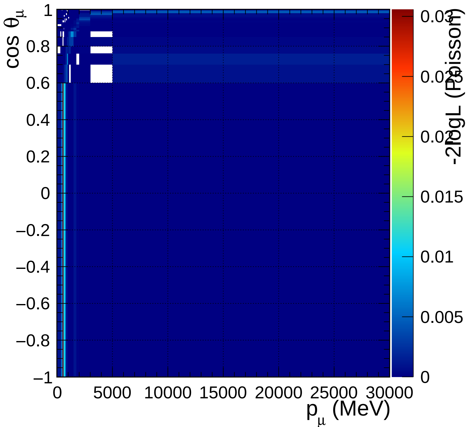
FGD1_numuCC_other_Q2_norm_6_1.54
