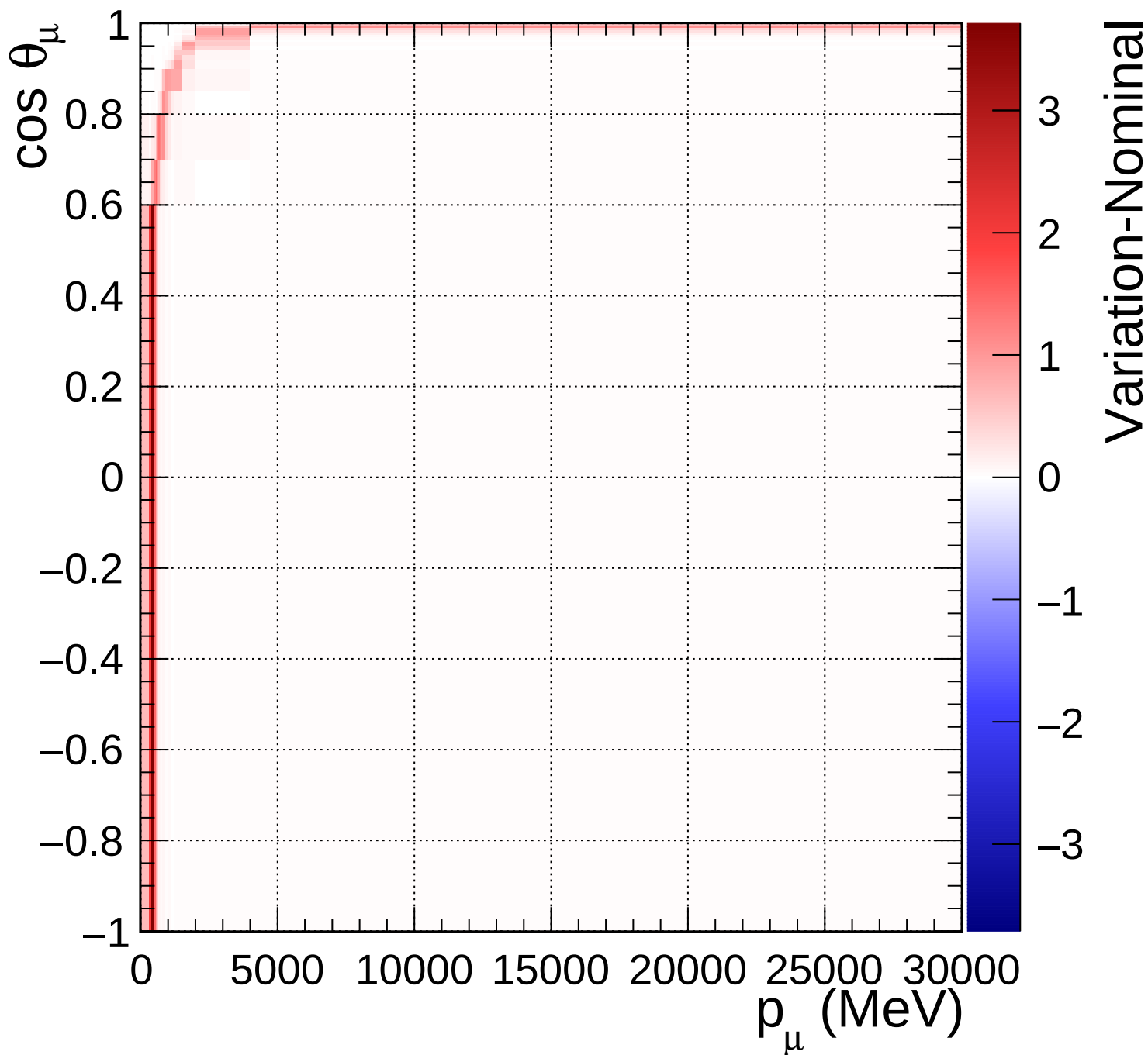
FGD2_anti-numuCC_0pi_Q2_norm_5_1.11
