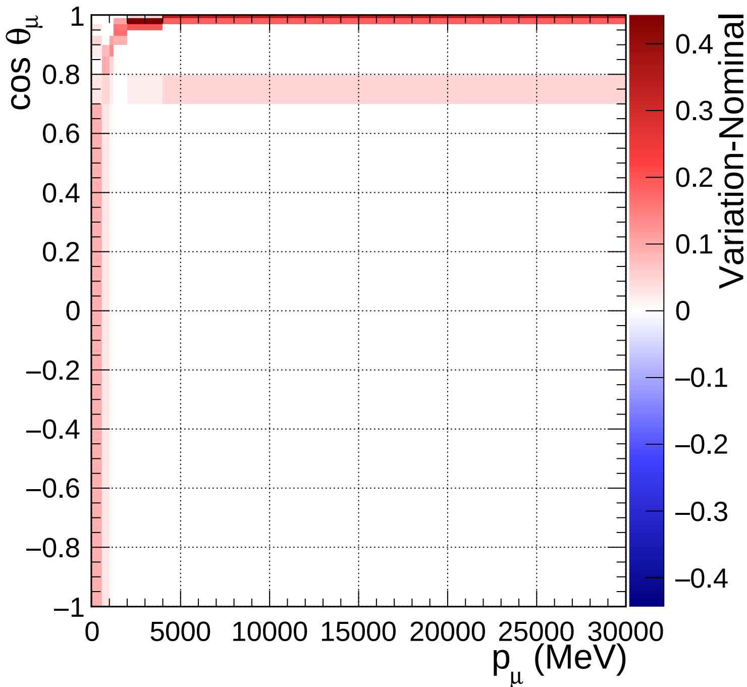
FGD1_NuMuBkg_CCother_in_AntiNu_Mode_Q2_norm_5_1.33
