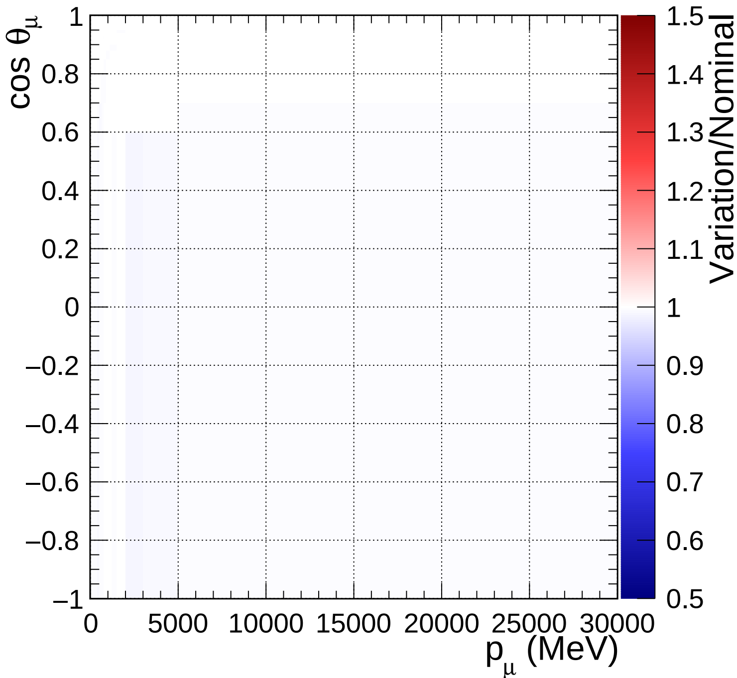
FGD2_numuCC_1pi_Q2_norm_5_0.89
