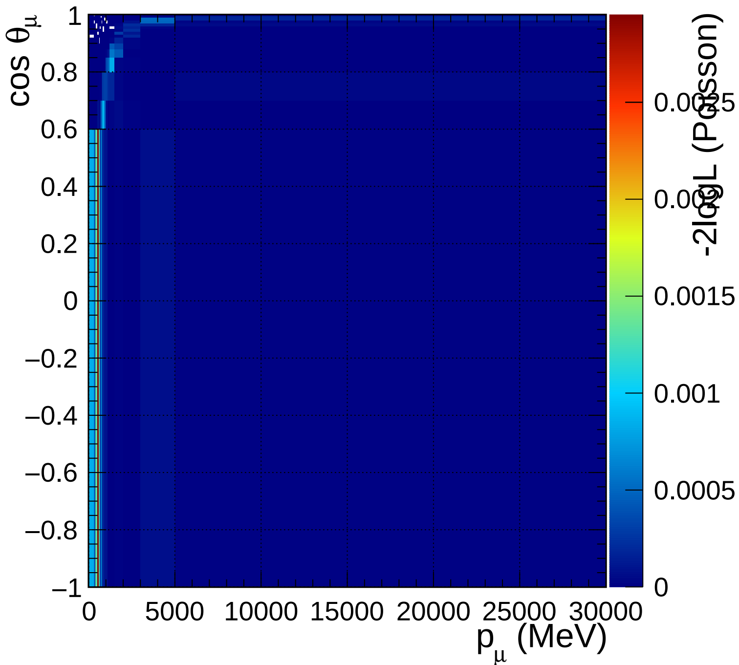
FGD2_numuCC_1pi_Q2_norm_6_1.18
