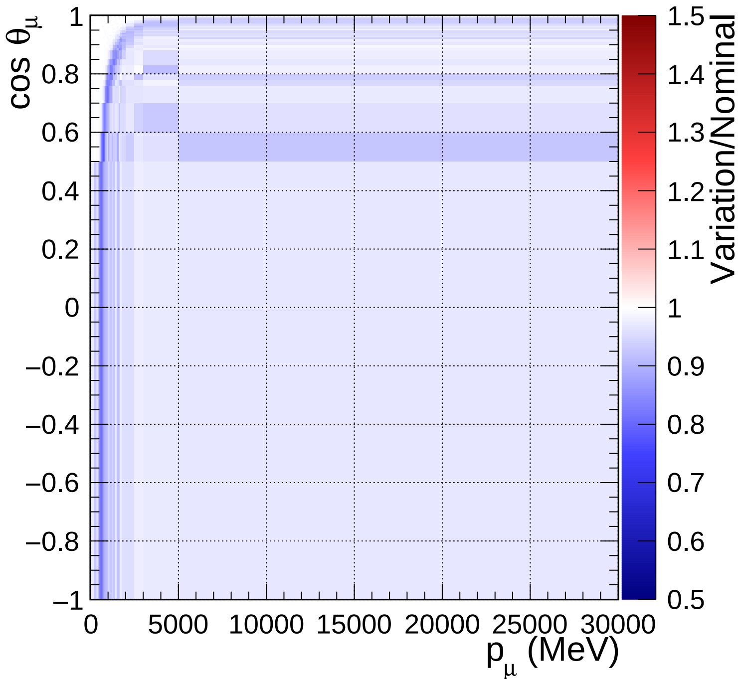
FGD2_numuCC_0pi_Q2_norm_6_0.46
