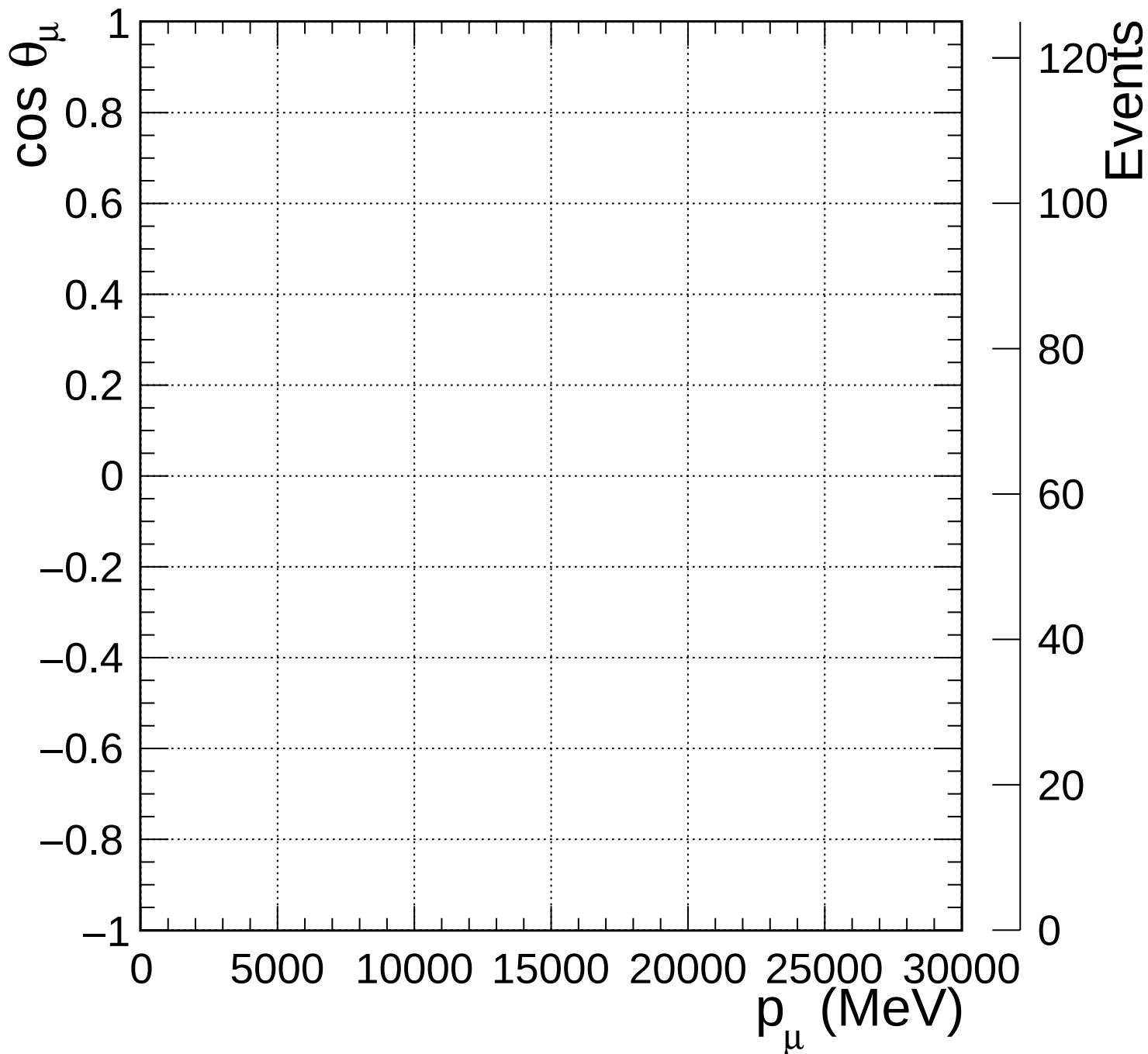
FGD2_NuMuBkg_CC1pi_in_AntiNu_Mode_Q2_norm_6_1
