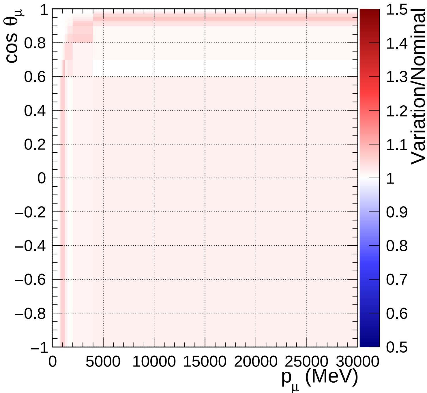
FGD1_anti-numuCC_0pi_Q2_norm_7_1.4
