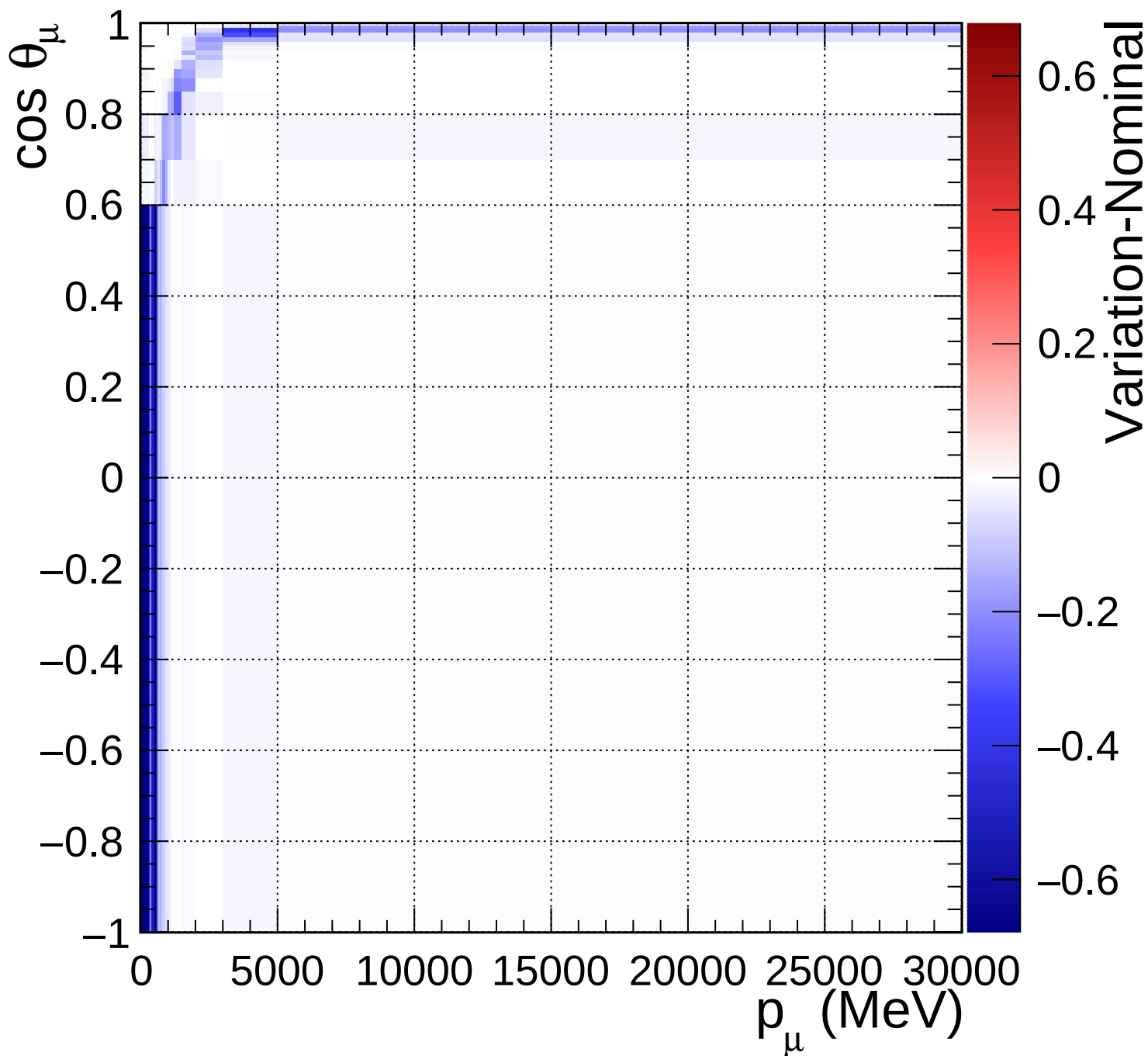
FGD2_numuCC_1pi_Q2_norm_6_0.82
