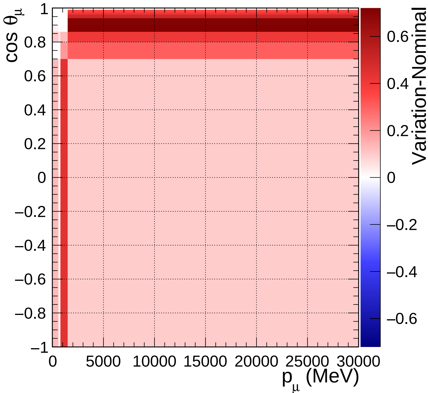
FGD1_NuMuBkg_CC1pi_in_AntiNu_Mode_Q2_norm_7_1.4
