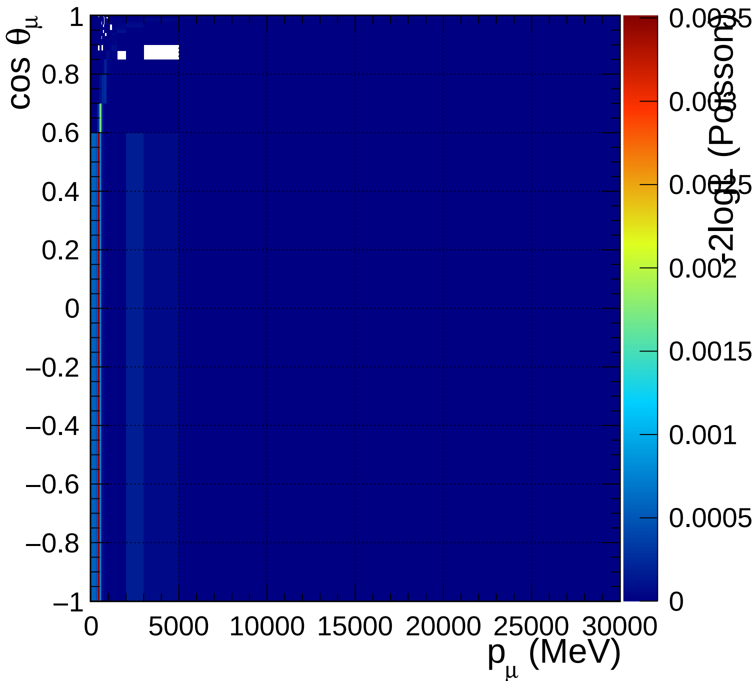
FGD2_numuCC_1pi_Q2_norm_5_1.11
