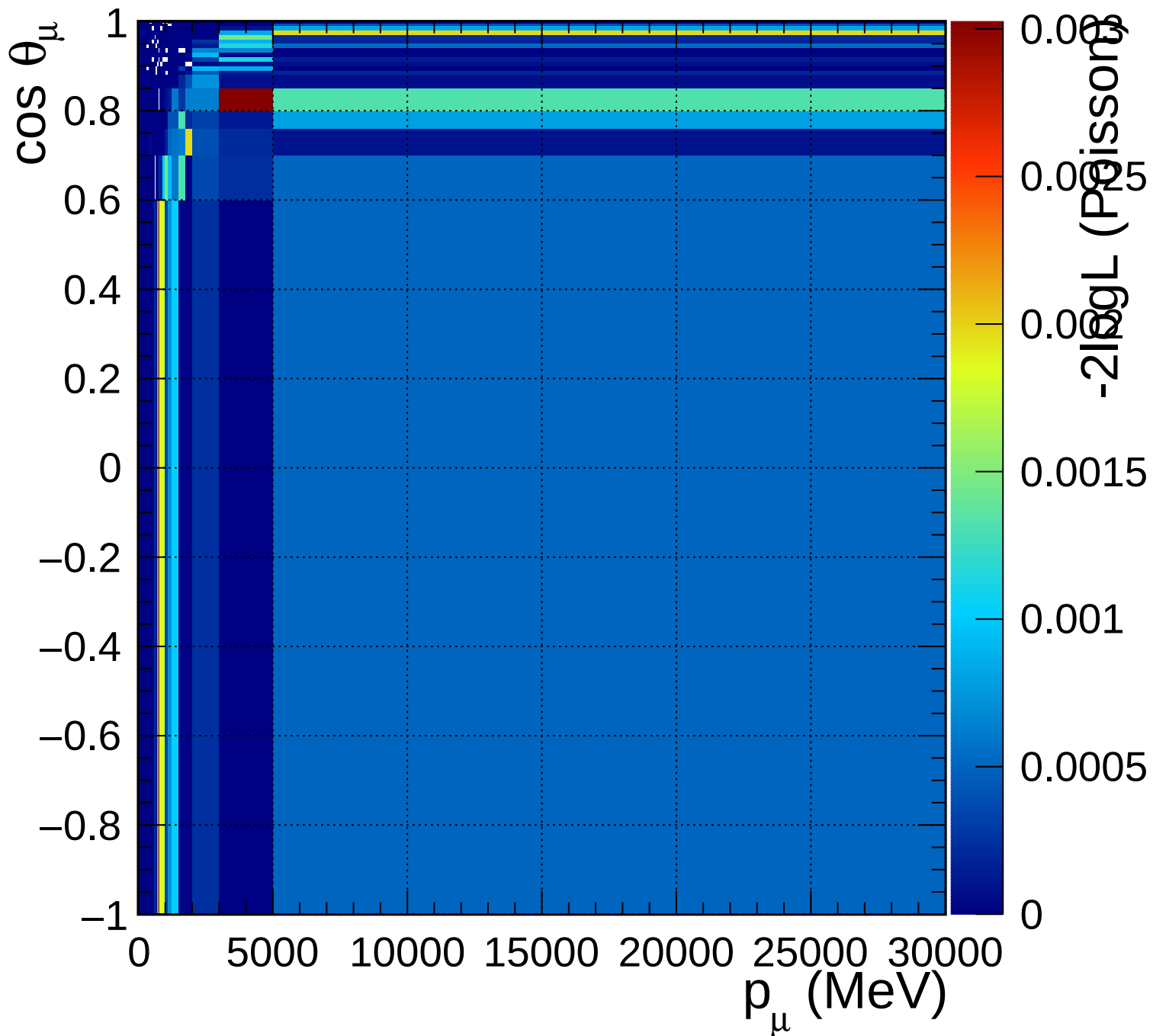
FGD1_numuCC_other_Q2_norm_7_1.4
