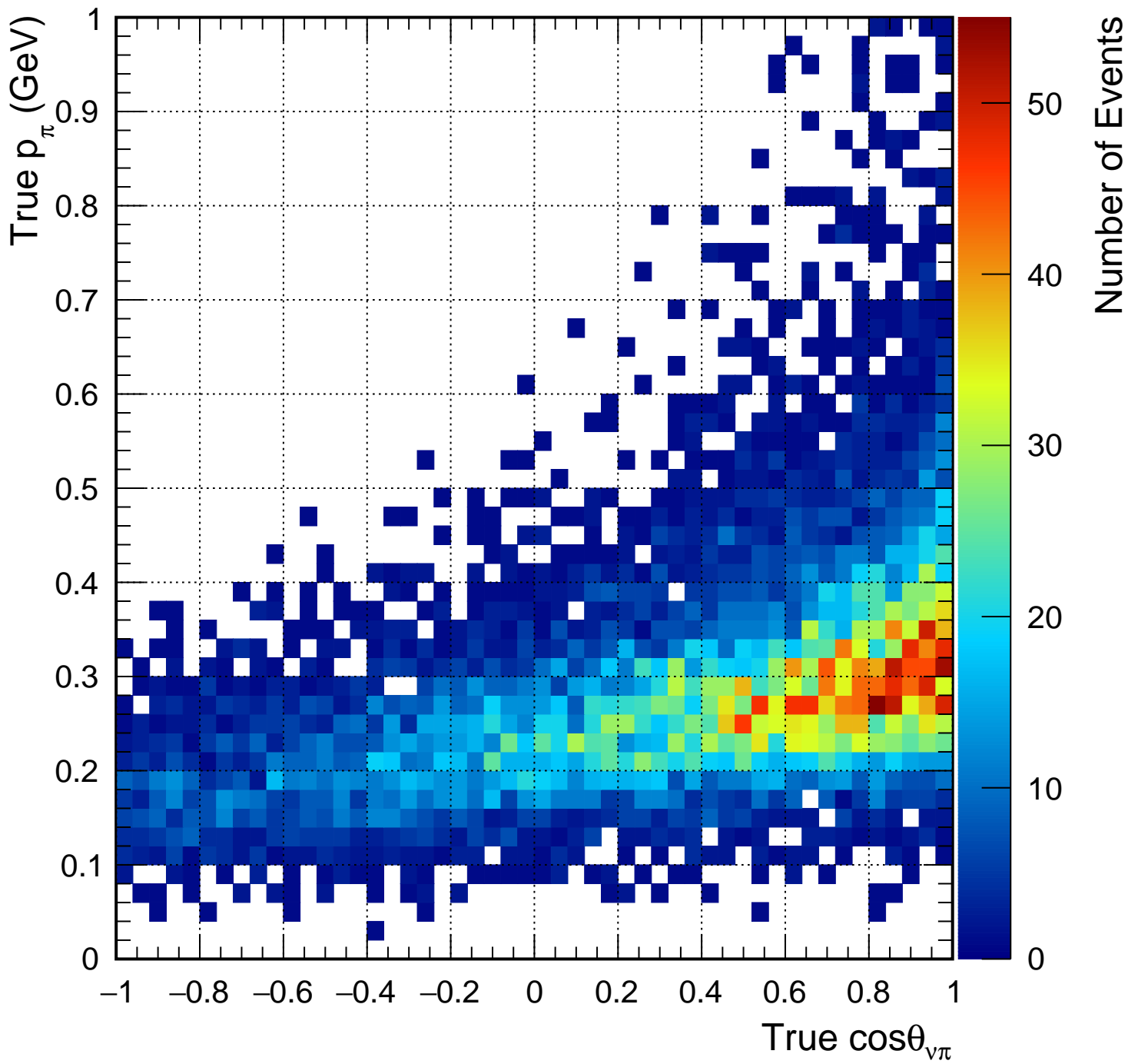
True CC1 \pi^+1e && Selected not as \nu_e CC1 \pi
