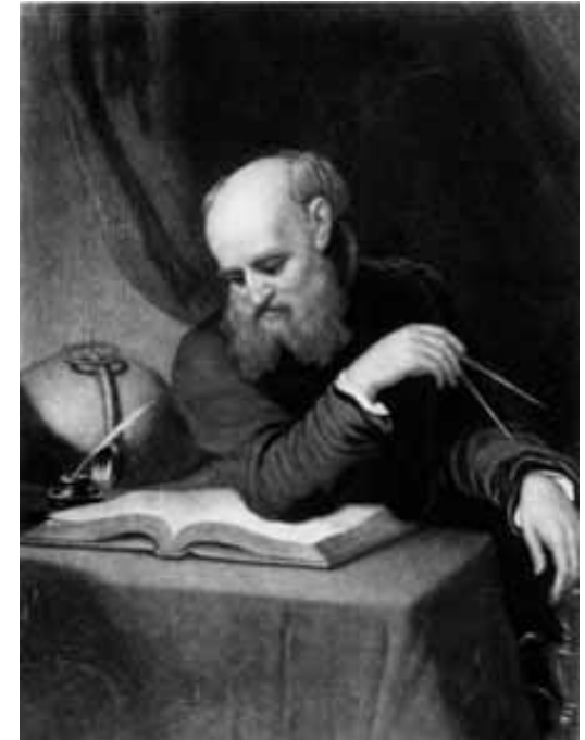
Galileo Galilei
