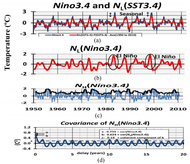
Figure 2. Plots based upon index Nino3.4 : (a) Nino3.4 (blue) and Index N_L(SST3.4) (red); (b) N_L(Nino3.4) , the low frequency component of Nino3.4 ; (c) N_H(Nino3.4) (blue), the high frequency component of Nino3.4 and its amplitude A_H(Nino3.4) (black); (d) Covariance of N_H(nino3.4) vs. lag \tau . The variance of 0.624 (C^2) at \tau = 0 is indicated.
