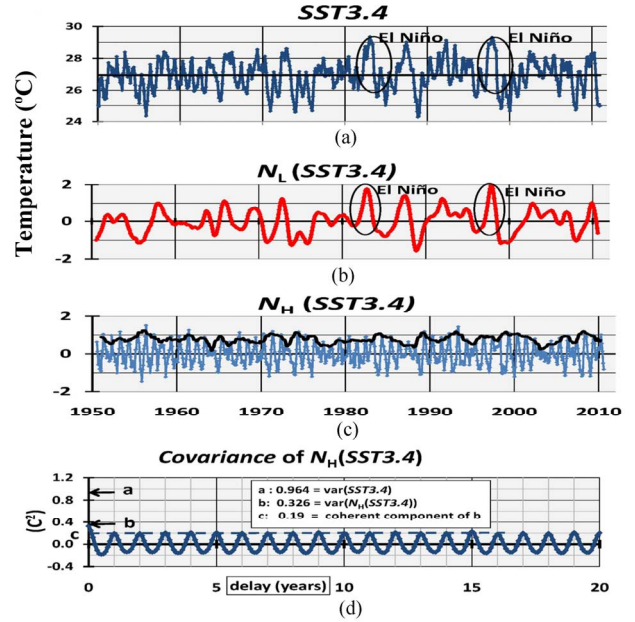
Figure 1. Plots based upon SST3.4 : (a) SST3.4 , Black line is the average; (b) N_L(SST3.4) , the low frequency component of SST3.4 ; Two El Niños are indicated; (c) N_H(SST3.4) (blue), the high frequency component of SST3.4 and its amplitude A_H(SST3.4) (black); (d) Covariance of N_H(SST3.4) vs. lag \tau . The variance of 0.326 (C^2) at \tau = 0 is indicated.
