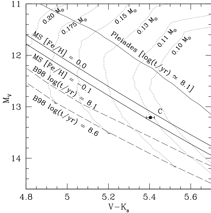
Fig. 4.— Color-magnitude ( V-K vs. M_V ) for Fomalhaut C (LP 876-10). The empirical main sequences for [\text{Fe}/\text{H}] = 0.0 and -0.1 from Johnson & Apps (2009) are plotted as thick solid lines , along with the color-magnitude sequence for the \sim 125 Myr-old Pleiades cluster from Stauffer et al. (2007, adopting d = 133.5 pc from Soderblom et al. 2005) ( thin solid line ). The theoretical evolutionary tracks from Baraffe et al. (1998) are plotted as dotted lines , and the isochrones for the approximate age of the Pleiades ( \log(t/\text{yr}) = 8.1 ) and Fomalhaut A & B ( \log(t/\text{yr}) = 8.6 ) are plotted as long dashed lines . The evolutionary tracks do not accurately predict the solar composition main sequence nor Pleiades sequence for this color-magnitude combination. Note that the Pleiades has a well-determined Lithium depletion boundary and main sequence turn-off age consistent with \sim 125 Myr (Ventura et al. 1998; Stauffer et al. 1998; Barrado y Navascués et al. 2004), and the main sequence “turn-on” appears to be consistent with this age as well (Barenfeld et al. 2013). Fomalhaut C appears to lie on the empirical main sequence of Johnson & Apps (2009) with [\text{Fe}/\text{H}] \simeq -0.07 .
