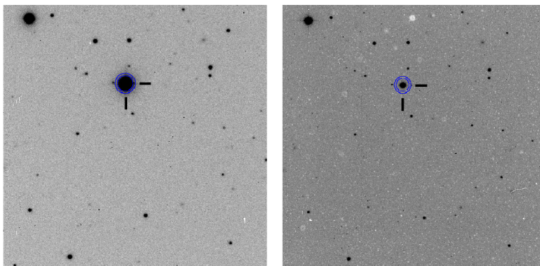
Fig. 1.— Left : Kron-Cousins I-band image of LP 876-10 taken with SMARTS 0.9-m telescope in 2004. Right : Johnson V-band image of LP 876-10 taken with SMARTS 0.9-m telescope in 2012. Star is circled in blue and is near 22:48:04.5 -24:22:08 (J2000). Field of view for both images is 6.8 arcminutes square. North is up and east is left. Fomalhaut A and B are not in the field of view.
