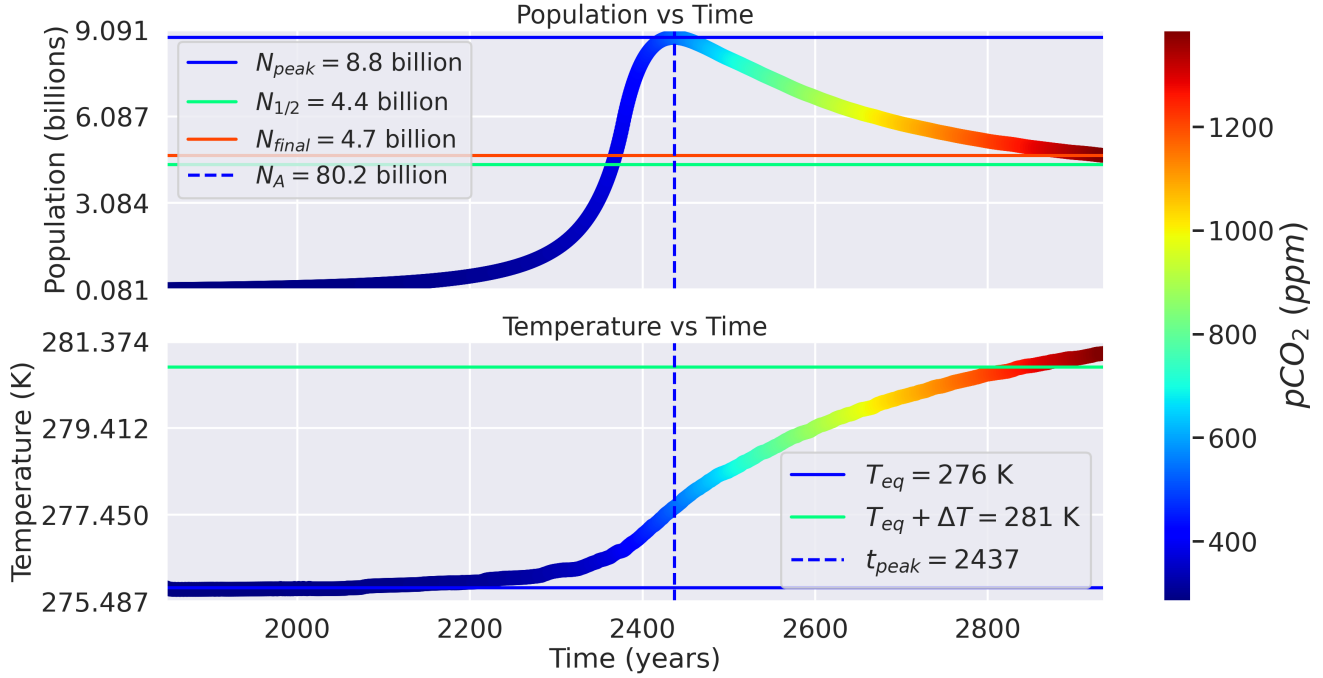
Figure 3: (3) Soft Anthropocene (green line close to red line)
