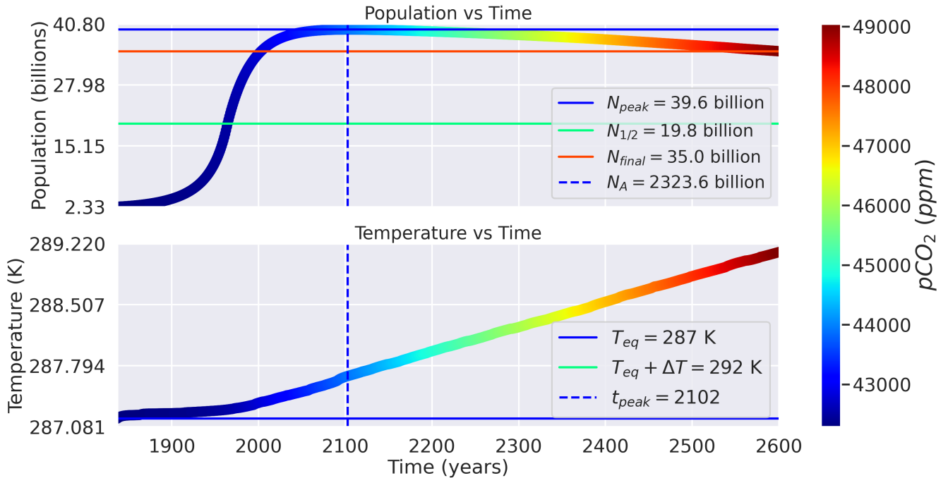
Figure 4: (4) Overpopulation (carrying cap reached)
