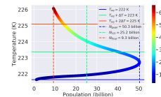
Distance: 1.06 AU, Carrying Capacity: 70 billion ppl, \Lambda : 3.771
