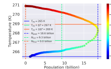
Distance: 1.03 AU, Carrying Capacity: 70 billion ppl, \Lambda : 0.126
