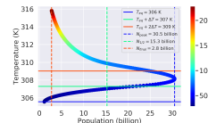
Distance: 0.97 AU, Carrying Capacity: 100 billion ppl, \Lambda : 0.35
