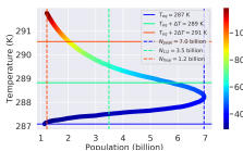
Distance: 1.0 AU, Carrying Capacity: 40 billion ppl, \Lambda : 1.28
