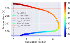
Distance: 1.03 AU, Carrying Capacity: 40 billion ppl, \Lambda : 0.221
