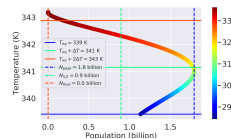
Distance: 0.94 AU, Carrying Capacity: 70 billion ppl, \Lambda : 0.031
