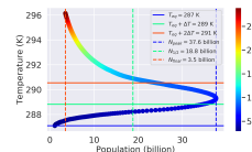
Distance: 1.0 AU, Carrying Capacity: 100 billion ppl, \Lambda : 0.512
