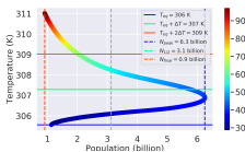
Distance: 0.97 AU, Carrying Capacity: 40 billion ppl, \Lambda : 0.876
