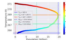
Distance: 1.03 AU, Carrying Capacity: 100 billion ppl, \Lambda : 0.088
