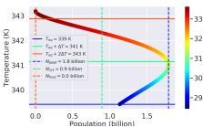
Distance: 0.94 AU, Carrying Capacity: 40 billion ppl, \Lambda : 0.054
