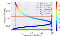
Distance: 1.0 AU, Carrying Capacity: 40 billion ppl, \Lambda : 1.28
