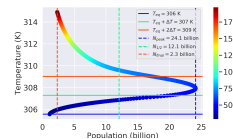
Distance: 0.97 AU, Carrying Capacity: 70 billion ppl, \Lambda : 0.5
