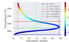
Distance: 1.0 AU, Carrying Capacity: 70 billion ppl, \Lambda : 0.732
