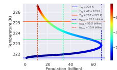
Distance: 1.06 AU, Carrying Capacity: 100 billion ppl, \Lambda : 2.64
