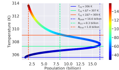
Distance: 0.97 AU, Carrying Capacity: 40 billion ppl, \Lambda : 0.876
