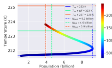
Distance: 1.06 AU, Carrying Capacity: 40 billion ppl, \Lambda : 6.599
