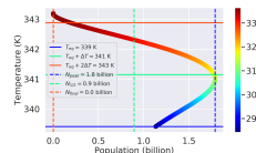
Distance: 0.94 AU, Carrying Capacity: 100 billion ppl, \Lambda : 0.022
