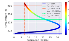
Distance: 1.06 AU, Carrying Capacity: 40 billion ppl, \Lambda : 6.599
