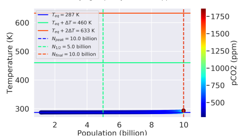
Distance: 1.0 AU, Carrying Capacity: 10 billion ppl, \Lambda : 512.137
