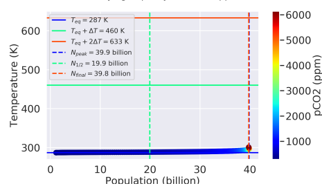
Distance: 1.0 AU, Carrying Capacity: 40 billion ppl, \Lambda : 128.034
