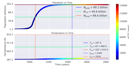
Distance: 1.0 AU, Carrying Capacity: 100 billion ppl, \Lambda : 51.214
