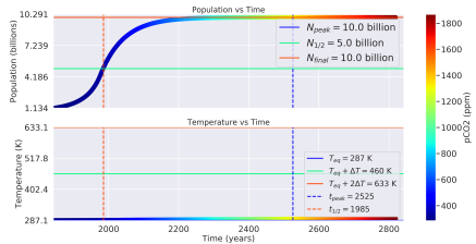
Distance: 1.0 AU, Carrying Capacity: 10 billion ppl, \Lambda : 512.137
