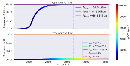
Distance: 1.0 AU, Carrying Capacity: 70 billion ppl, \Lambda : 73.162
