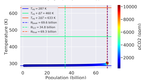
Distance: 1.0 AU, Carrying Capacity: 70 billion ppl, \Lambda : 73.162
