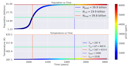
Distance: 1.0 AU, Carrying Capacity: 40 billion ppl, \Lambda : 128.034
