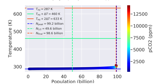
Distance: 1.0 AU, Carrying Capacity: 100 billion ppl, \Lambda : 51.214
