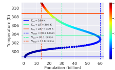
Distance: 0.98 AU, Carrying Capacity: 100 billion ppl, \Gamma : 1.435
