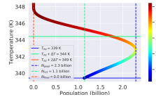
Distance: 0.94 AU, Carrying Capacity: 40 billion ppl, \Gamma : 0.849
