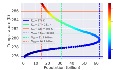
Distance: 1.02 AU, Carrying Capacity: 100 billion ppl, \Gamma : 1.247
