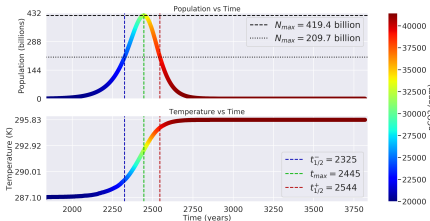
Distance: 1.05 AU, p\text{CO}_2 : 19,984ppm, T_{\text{eq}} : 287.102K
