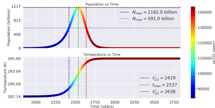
Distance: 1.1 AU, p\text{CO}_2 : 83,684ppm, T_{\text{eq}} : 287.137K
