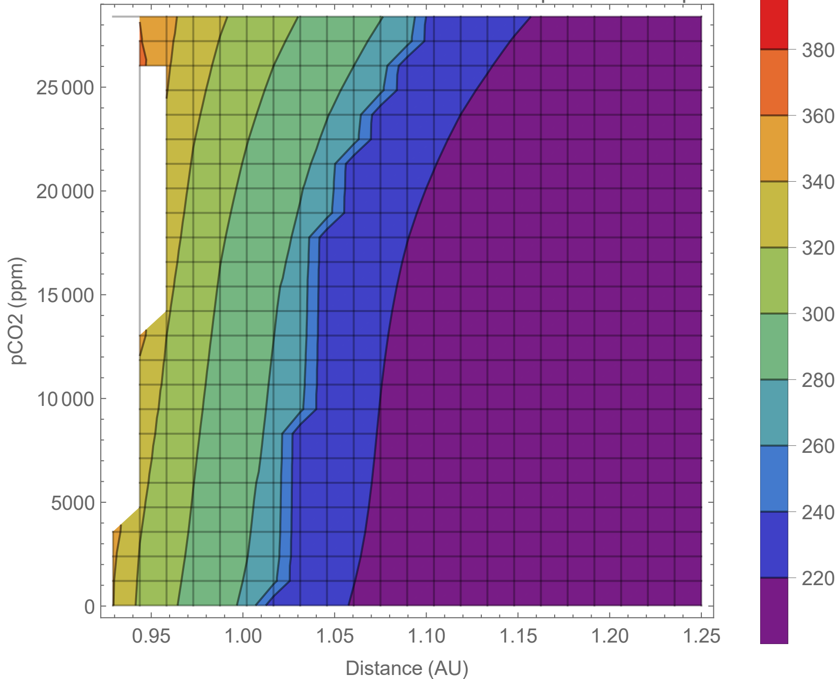
Distance Vs Partial CO2 Pressure vs Equilibrium temp
