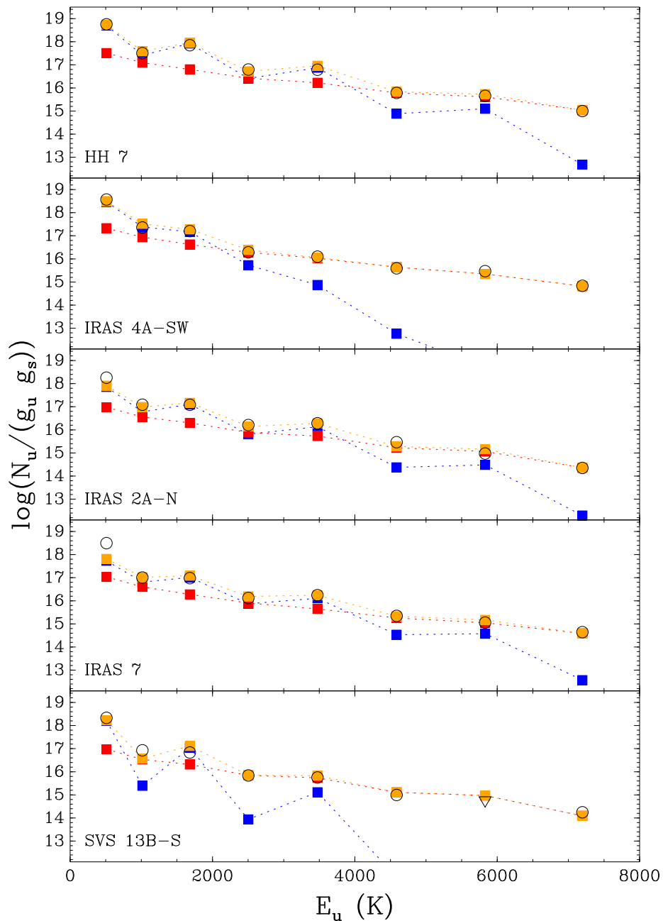
Fig. 9.— Same as in Fig. 5, but with the two velocity components shock model predictions over plotted (see § 5.1). The blue and red squares connected by dotted lines show the emission from the slow and fast shock components, respectively. The orange squares connected by dotted lines show the total emission from these two components. Note that some of the blue squares (at low energies), as well as some of the red squares (at high energies) are masked by the orange squares.
