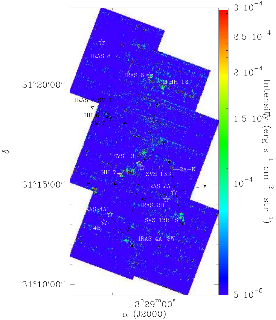
Fig. 4 h.— H 2 S(6) map obtained with the SL module. Contours show the 3\sigma noise level.
