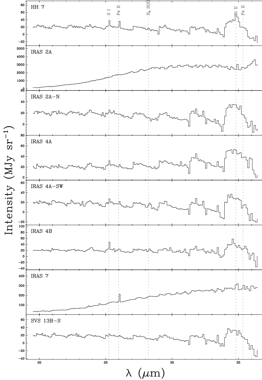
Fig. 3.— Same as Fig. 1 for the LH module. For clarity the spectral resolution has been degraded by a factor 4. The steps seen in some of these spectra are caused by offsets in response of the different orders of the module.
