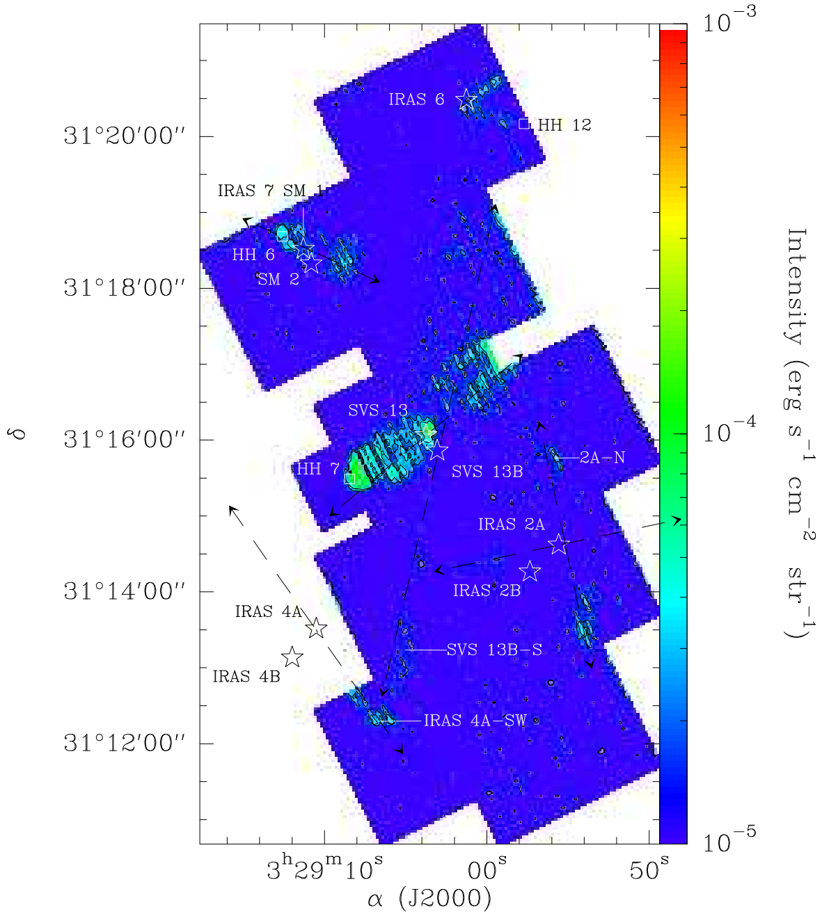
Fig. 4 e.— H 2 S(2) map obtained with the SH module. Contours show the 3 and 5 \sigma noise levels.
