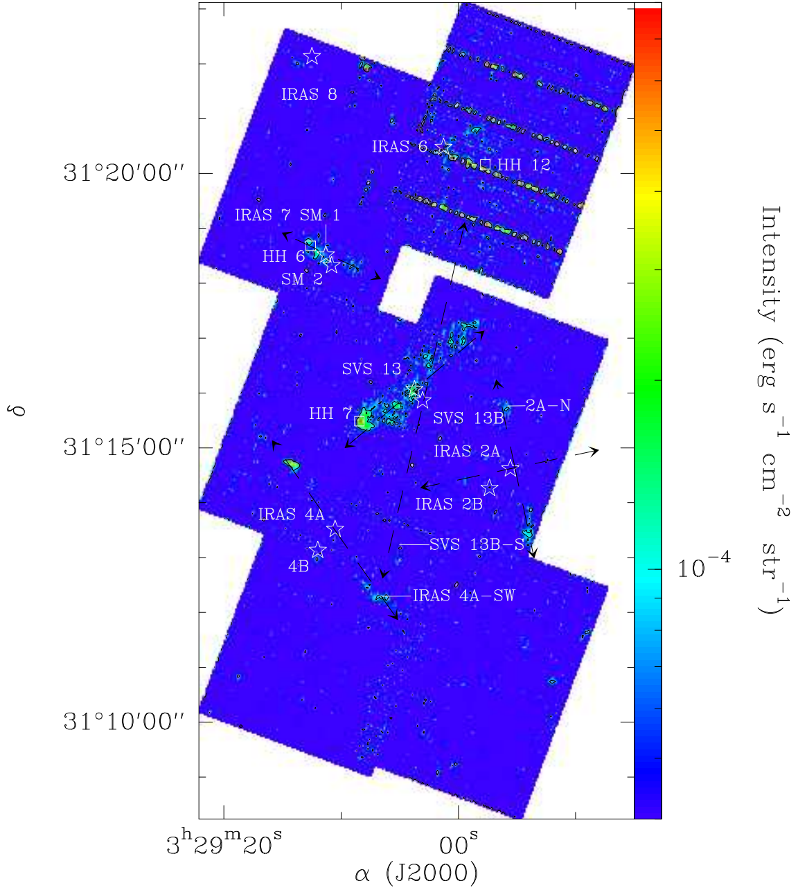
Fig. 4 f.— H 2 S(4) map obtained with the SL module. Contours show the 3 \sigma noise level.
