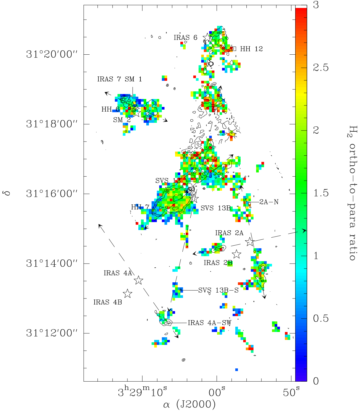
Fig. 8.— Same as Fig. 6 for the H 2 ortho-to-para ratio.
