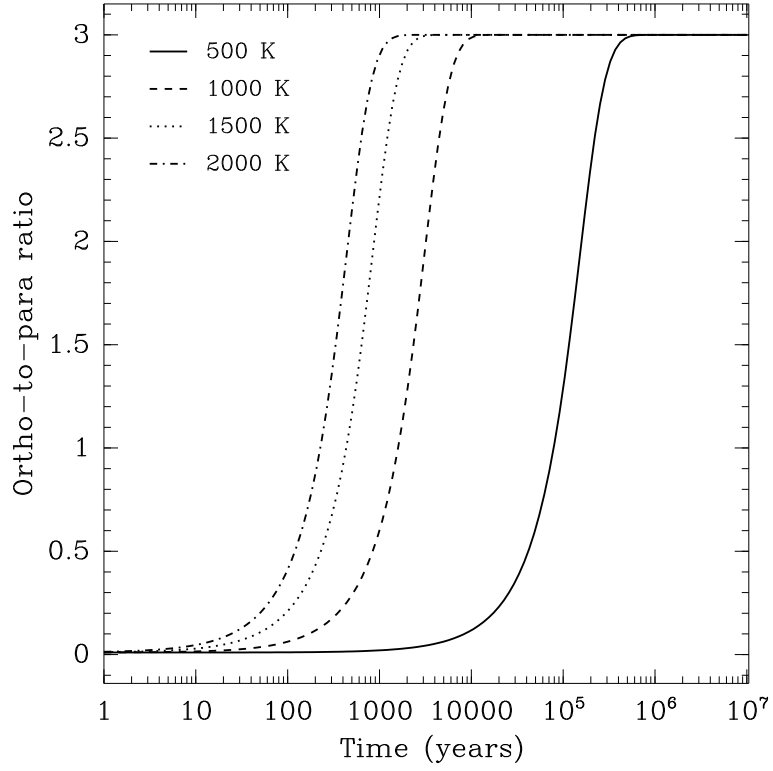
Fig. 10.— \text{H}_2 ortho-to-para ratio as a function of time for different gas temperatures. An initial opr of 0.01 and H density of 10 \text{ cm}^{-3} are assumed for all curves.
