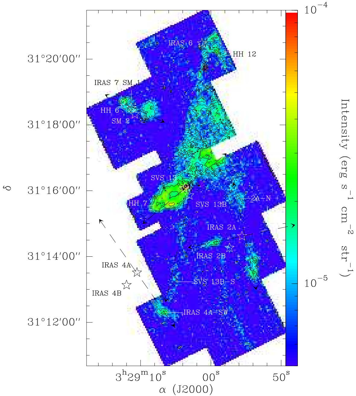
Fig. 4 a.— H 2 S(1) continuum subtracted map obtained with the SH module. YSOs are indicated by open stars, while several HH objects are indicated by open squares. The outflows discussed in the text are indicated by dashed arrows. The two positions along the IRAS 2 and IRAS 4A outflows that are discussed in the text, IRAS 2A-N and IRAS 4A-SW, are also shown. Contours show the 3, 5 and 10 \sigma noise levels. See the electronic edition of the Journal for panels d-i.
