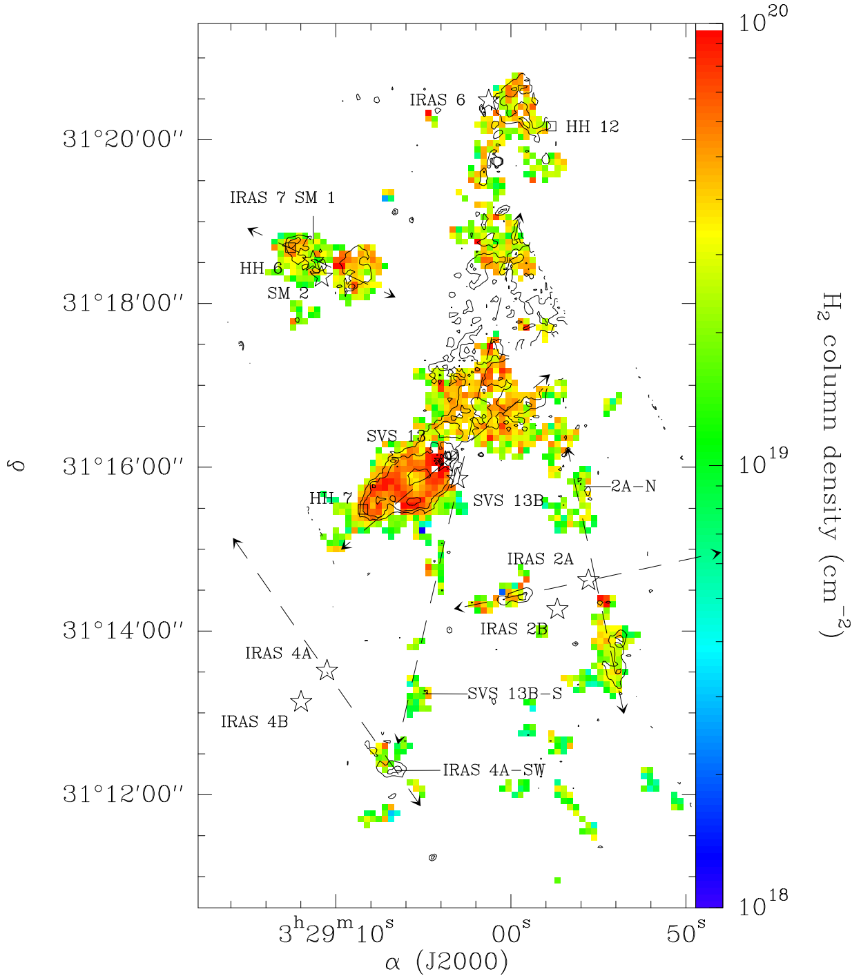
Fig. 6.— H 2 column density map (color points) on top of the H 2 S(1) emission (black contours). Regions of the map that appear in white correspond to points where a rotational diagram could not be constructed because of missing data or insufficient signal-to-noise ratio. Contour levels are those of the S(1) emission taken from Fig. 4 a.. Pixel size is 5".
