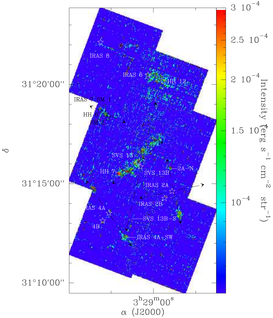
Fig. 4 i.— H 2 S(7) map obtained with the SL module. Contours show the 3 σ noise level.
