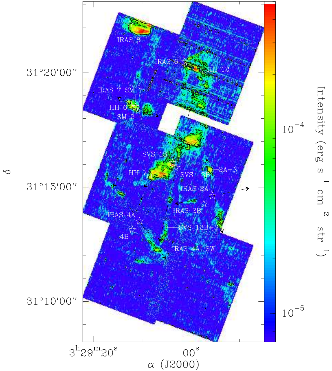
Fig. 4 c.— H 2 S(3) map obtained with the SL module. Contours show the 3 and 5 \sigma noise level.
