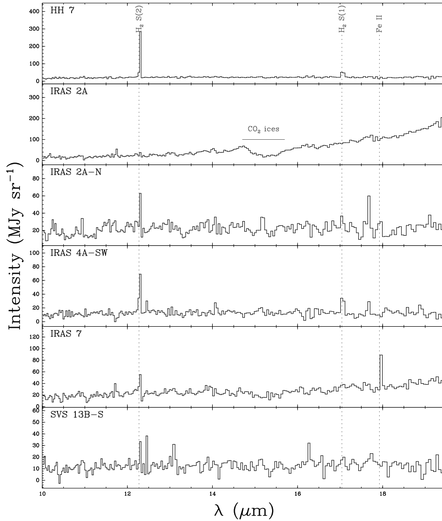
Fig. 2.— Same as Fig. 1 for the SH module. The position of the 15.2 \mu CO 2 ice feature is indicated. For clarity the spectral resolution has been degraded by a factor 4.
