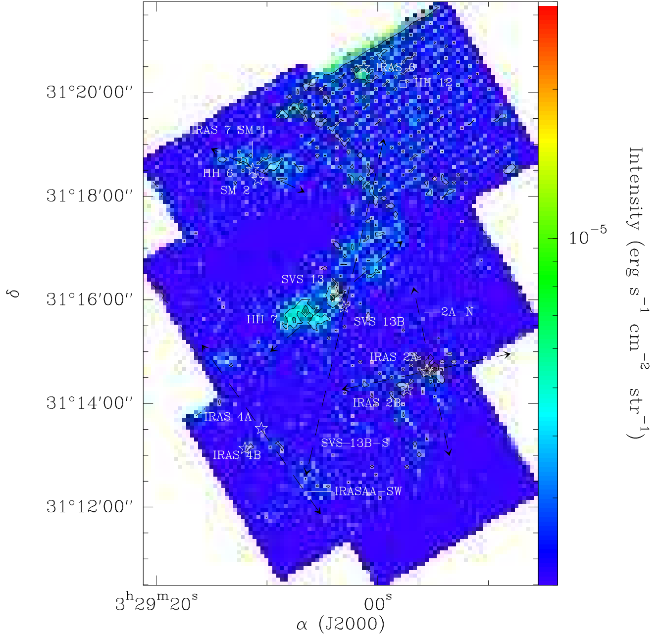
Fig. 4 d.— H 2 S(0) map obtained with the LH module. Contour levels are drawn at 3\sigma .
