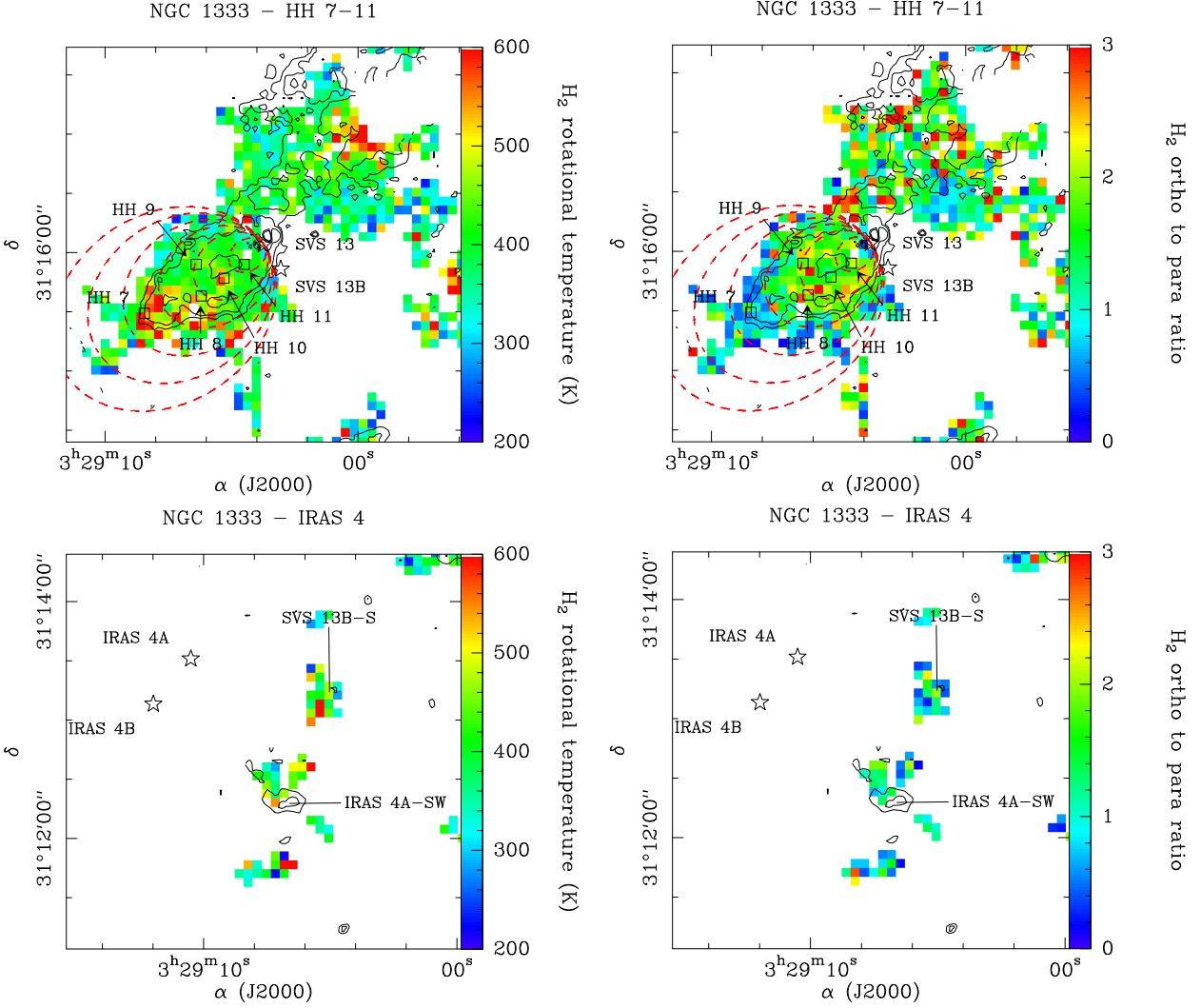
Fig. 11.— Side-by-side comparison between the rotational temperature and opr around SVS 13 (upper panels) and IRAS 4 (lower panels). The position of several HH objects around SVS 13, from Walawender et al. (2005), are indicated. The ellipses that were used to average the opr and the rotational temperature (see § A) are shown.
