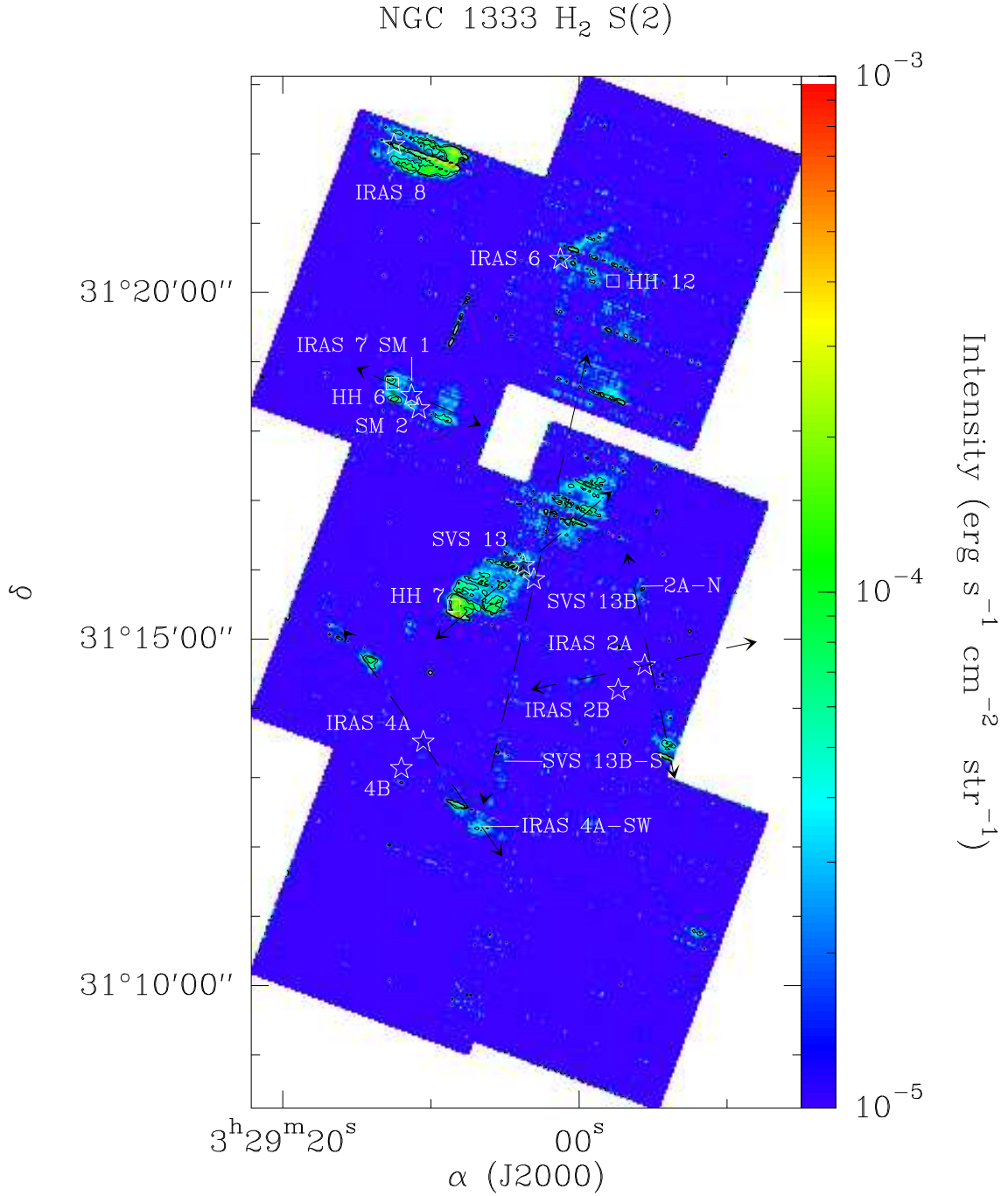
Fig. 4 b.— H 2 S(2) map obtained with the SL module. Contours show the 3 and 5 \sigma noise level.
