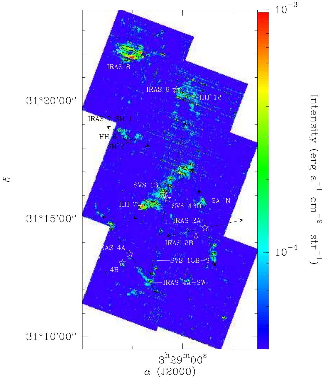
Fig. 4 g.— H 2 S(5) map obtained with the SL module. Contours show the 3 \sigma noise level.
