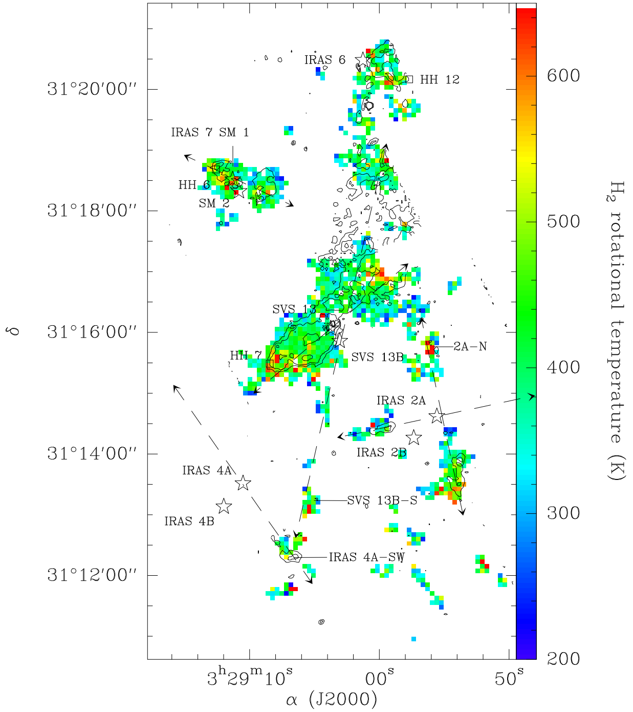
Fig. 7.— Same as Fig. 6 for the H 2 rotational temperature.
