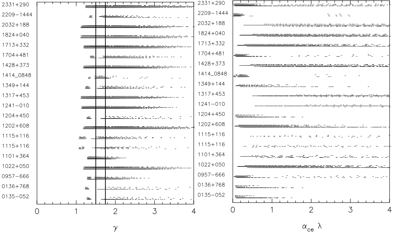
Figure 5. Left: reconstructed \gamma values for the last phase of mass transfer in the formation of double white dwarfs (see Table 1). Right: reconstructed \alpha\lambda values for the same.
