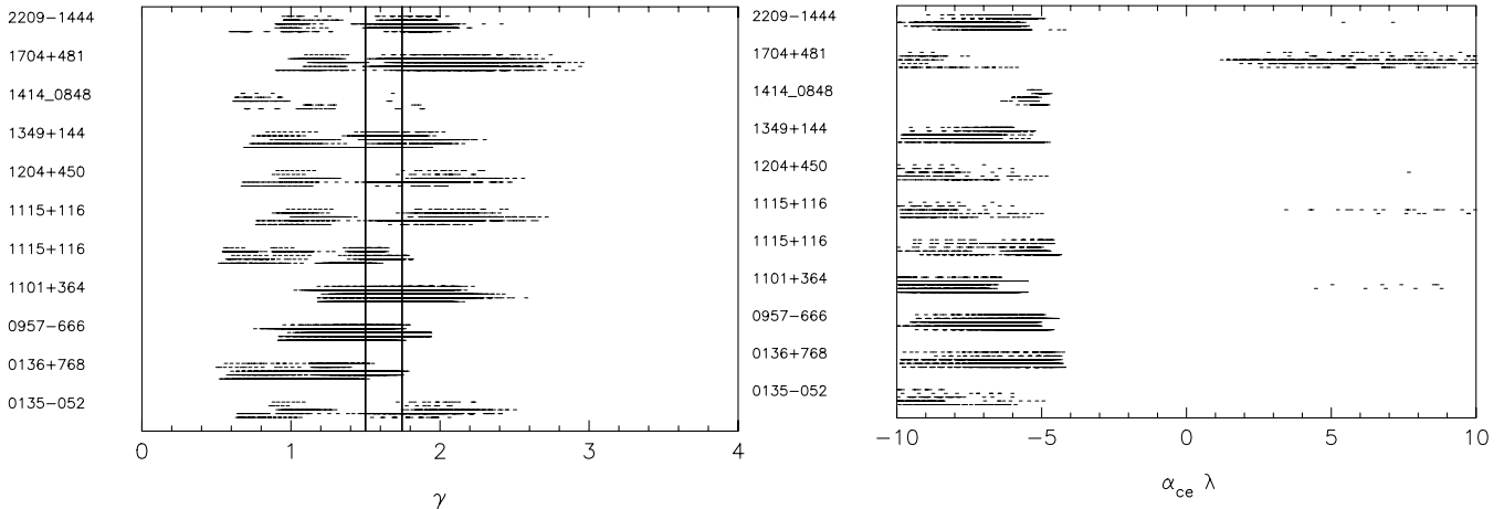
Figure 1. Left: reconstructed \gamma values for the first phase of mass transfer in the formation of double white dwarfs. Right: reconstructed \alpha\lambda values for the same. The horizontal lines are made up of small dashes representing the reconstructed values of \gamma and \alpha\lambda for different values of the mass of the progenitor of the white dwarf and the companion. The different lines for each object represent different values of the white dwarf mass (within 0.05 M_{\odot} of the value in Table 1).
