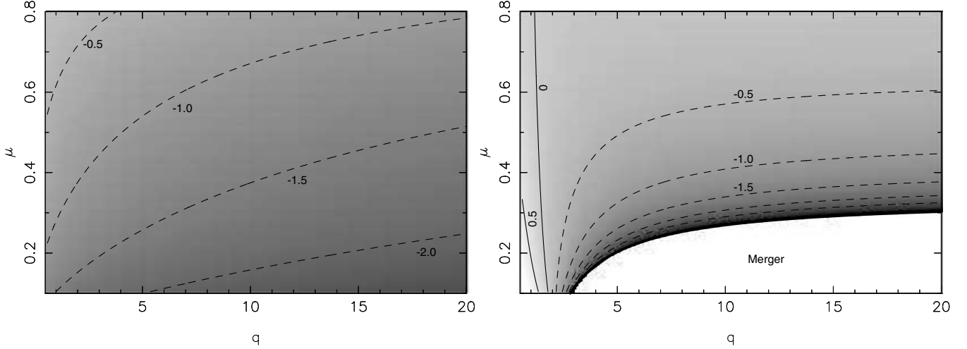
Figure 3. Relative change in separation for dynamical mass transfer described by the standard \alpha -formalism (left-hand panel) and the \gamma -algorithm (right-hand panel) as a function of mass ratio q and core mass fraction \mu . The logarithm of (a_f/a_i) is shown as the grey scale and the contours.
