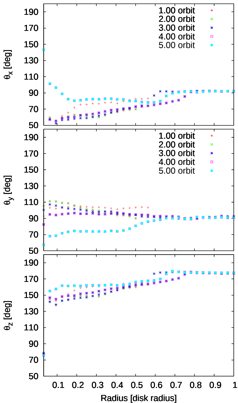
Projected angular momentum vs r_{\text{disk}} and time
