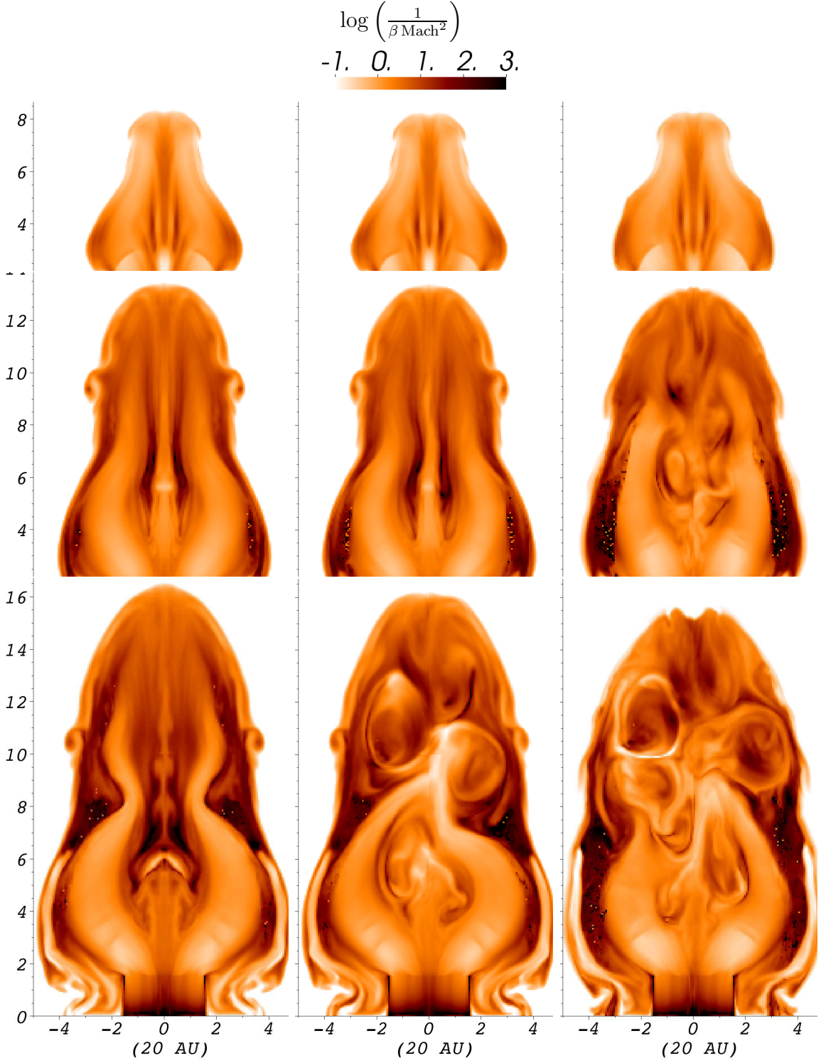
Fig. 9.— Evolution of the ratio of Poynting to kinetic flux, 1/(\beta \text{Mach}^2) . These logarithmic greyscale maps show the magnetic towers in the adiabatic (left), the rotating (middle) and the cooling (right) cases. From top to bottom time is equal to 42, 84 and 118 yr.
