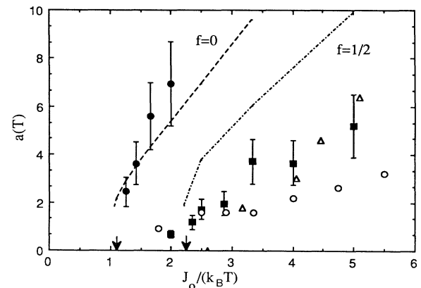
FIG. 2. Exponent a(T) of the current-voltage relation V \sim I^{1+a} vs J_0/T . For the unfrustrated case: solid circles are results from fits to the data of Fig. 1(a); dashed line is the theoretical prediction (5). For the fully frustrated case: squares are results from fits to the data of Fig. 1(b); dot-dashed line is from Eq. (5); triangles are experimental results of van Wees, van der Zant, and Mooij [Ref. 7(a)]; open circles are experimental results of Carini [Ref. 7(b)]. Arrows indicate transition temperatures T_c(f=0) and T_c(f=1/2) . Estimated errors of 25% are shown as error bars on our numerical results.
