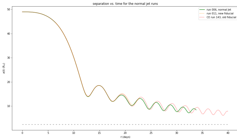
Figure 2. Separation for the normal jet runs
