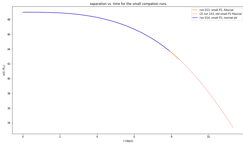
Figure 4. Separation for the small companion runs - initial speeds corrected
