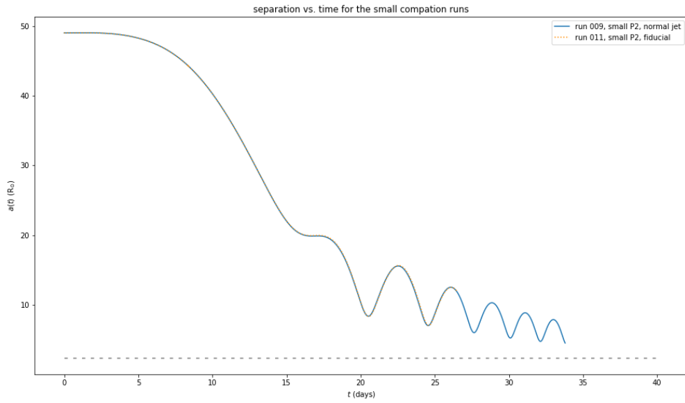
Figure 3. Separation for the small companion runs
