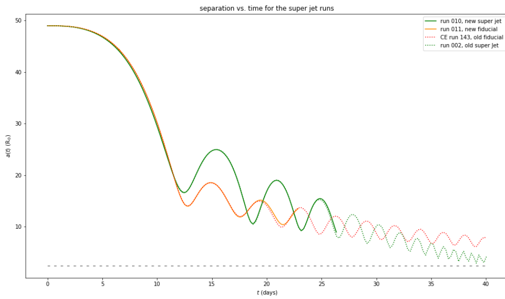
Figure 1. Separation for the super jet runs
