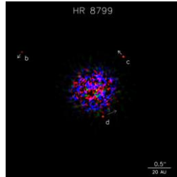
C. Marois and B. Macintosh, Keck Observatory
