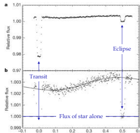
HD 189733 at \lambda = 8 \mu\text{m} ; Knutson et al. 2007 .
