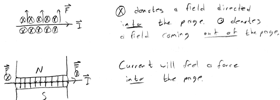
Figure 8.7: Force on current due to magnet
