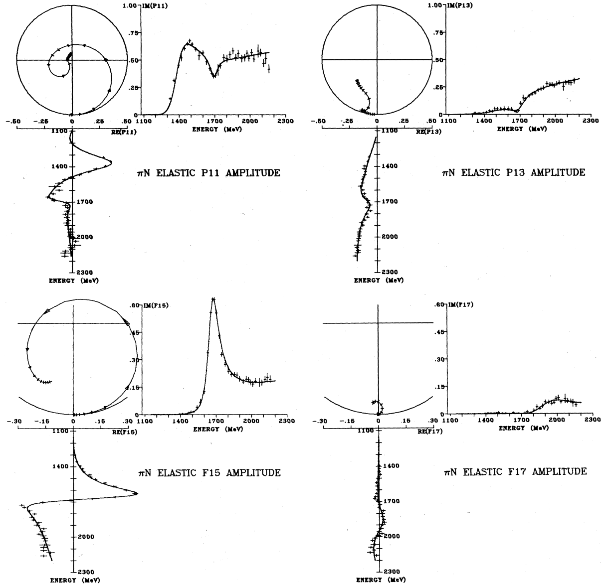
FIG. 4. Even-parity I = \frac{1}{2} partial-wave amplitudes for J \leq \frac{7}{2} . See also the caption to Fig. 2.
