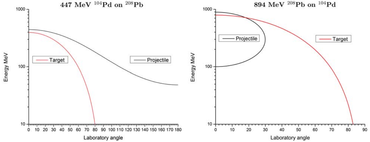
Figure 5.4: Recoil energies, in MeV , versus laboratory scattering angle. (Left) Scattering of 447 MeV ^{104}Pd by ^{208}Pb for Q = -5.0 MeV . (Right) Scattering of 894 MeV ^{208}Pb on ^{104}Pd for Q = -5.0 MeV .
