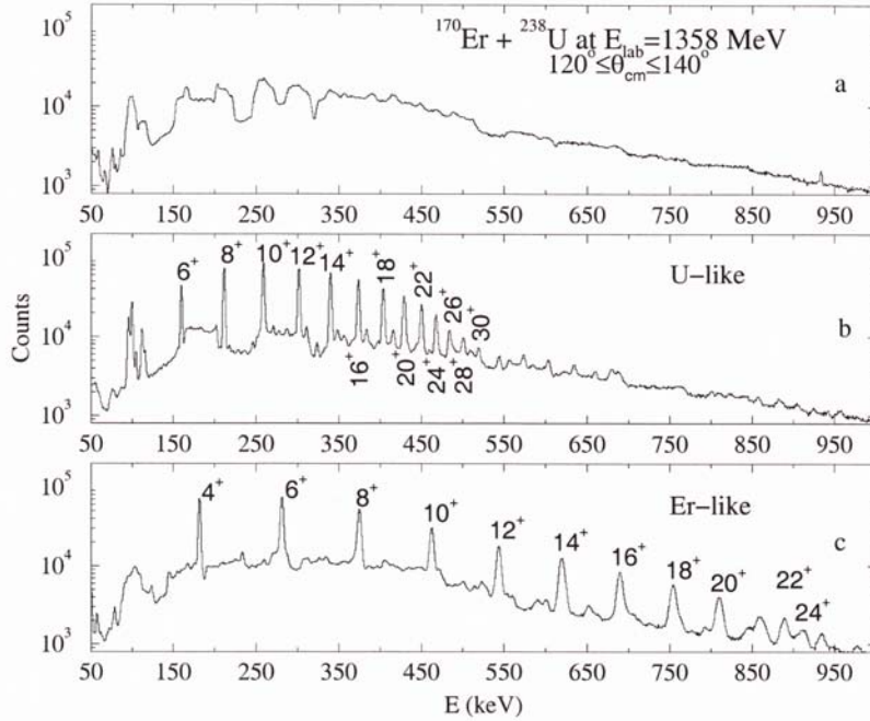
Figure 2.5: Typical \gamma -ray spectra for 1358 \text{ MeV} ^{238}\text{U} beam on a 0.5 \text{ mg/cm}^2 ^{170}\text{Er} target detected using Gammasphere in coincidence recoil ions detected by CHICO. (a) shows the raw coincident \gamma ray spectrum, (b) shows the coincident \gamma ray spectrum Doppler-corrected for U recoils, (c) shows the coincident \gamma ray spectrum Doppler-corrected for Er recoils. [WU00]
