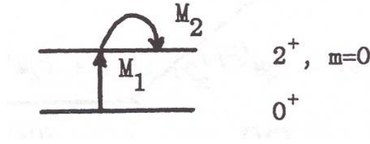
Figure 6.4: Reorientation effect for the two-level system.
