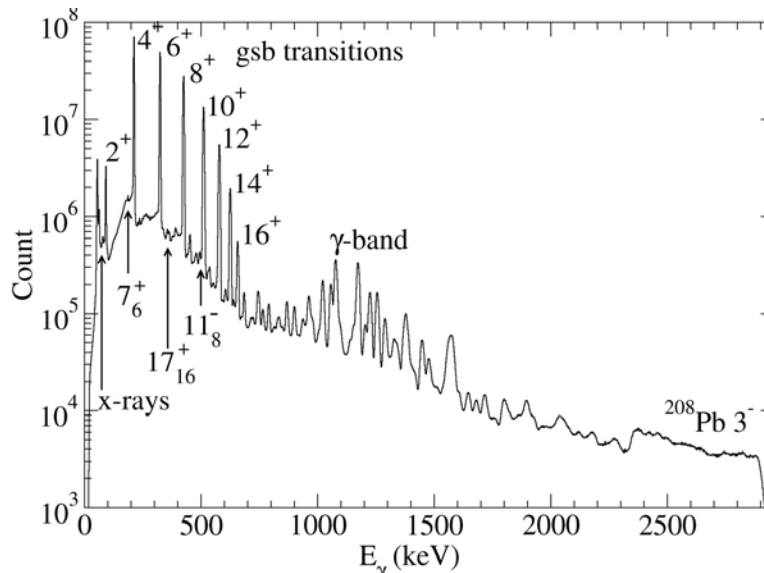
Figure 2.6: A recoil- \gamma -ray coincidence spectrum for projectile scattering angle range 35^\circ \leq \theta \leq 50^\circ obtained using a 985\text{ MeV } ^{178}\text{Hf} beam bombarding a 0.5\text{ mg/cm}^2 ^{208}\text{Pb} target. The \gamma -ray spectrum is Doppler corrected for ^{178}\text{Hf} . In-band transitions in the ground band, and \gamma -band to ground band transitions are cleanly resolved. The 3^- \rightarrow 0_{gsb} in ^{208}\text{Pb} has been broadened due to use of the wrong Doppler correction. [HAY10b]
