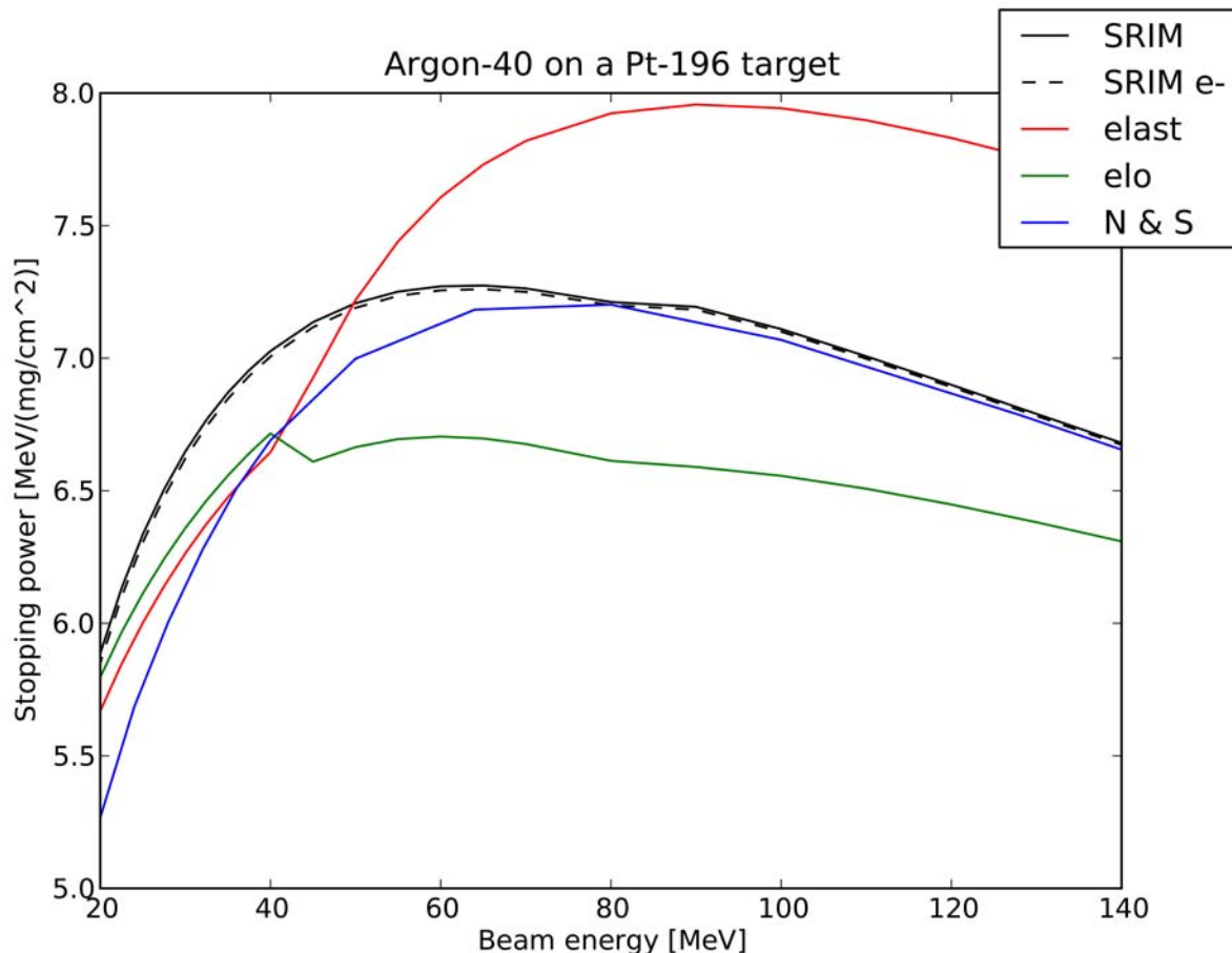
Figure 5.6: The calculated stopping power for an ^{40}\text{Ar} beam in ^{196}\text{Pt} is shown as a function of beam energy given by the 2011 version of the Ziegler code SRIM[ZIE08], Northcliffe and Schilling[NOR70], and the utility computer codes ELO and ELAST.
