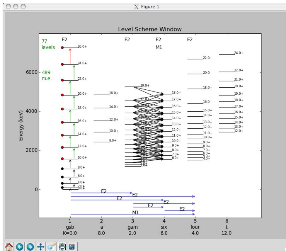
Figure 8.1: The RACHEL level scheme display shows the couplings between bands (blue arrows labeled with the multipolarity), in-band couplings (“E2” and “M1” at the tops of bands), fixed matrix elements (not variable in fits) shown as black arrows between levels, selected master (fit parameter) matrix elements shown as green arrows between levels, and matrix elements dependent on the masters displayed as red arrows.
