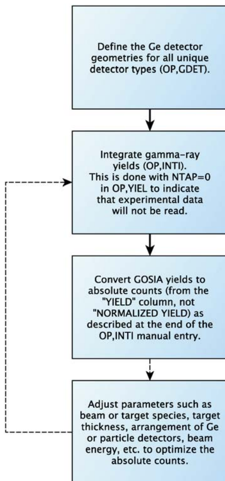
Figure 14.2: Overall flow diagram for use of Gosia.
