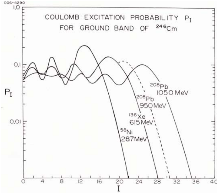
Figure 2.7: The calculated probability for Coulomb excitation of the ground band of ^{246}\text{Cm} by backscattered ions. The E2 matrix elements were assumed to be related by the spheroidal rotor relation. [CLI86]
