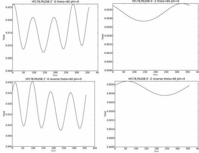
Figure 4.2: Upper row: Target excitation of ^{208}\text{Pb} by a 890\text{MeV } ^{178}\text{Hf} beam scattered at \theta_{proj} = 60^\circ . Lower row: Projectile excitation of a 890\text{MeV } ^{178}\text{Hf} beam scattered at \theta_{proj} = 60^\circ by a ^{208}\text{Pb} target. Left column: shows a 2^+ state at 1.175\text{MeV} decaying to the 0^+ ground state. Right column: shows a 1.0\text{MeV } 0^+ state decaying to the ground-band 2^+ state. The calculated yields are plotted versus \theta_\gamma which is measured with respect to the incident beam direction. The deorientation effect has been switched off.
