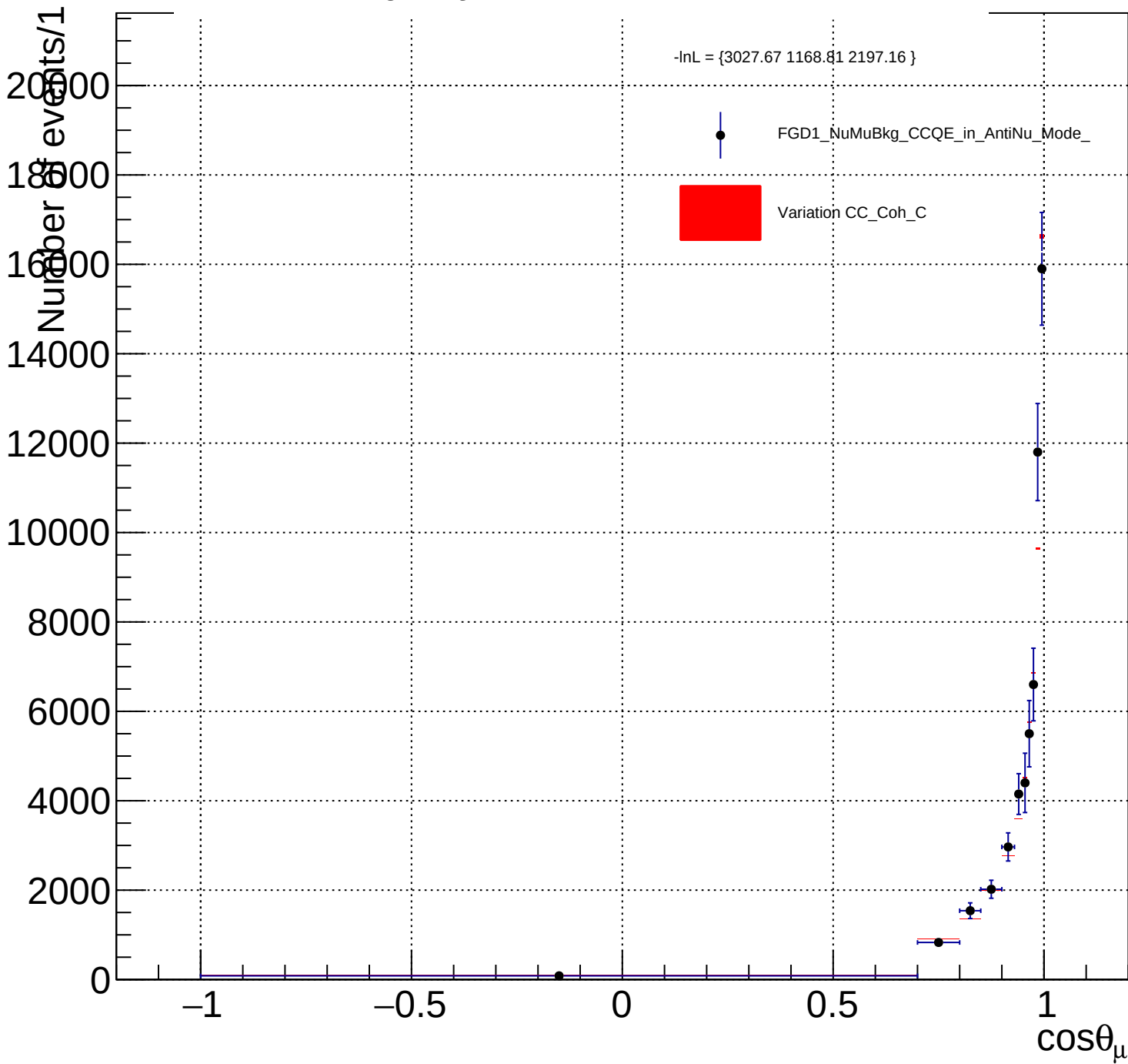
FGD1_NuMuBkg_CCQE_in_AntiNu_Mode__CC_Coh_C_Y_norm
