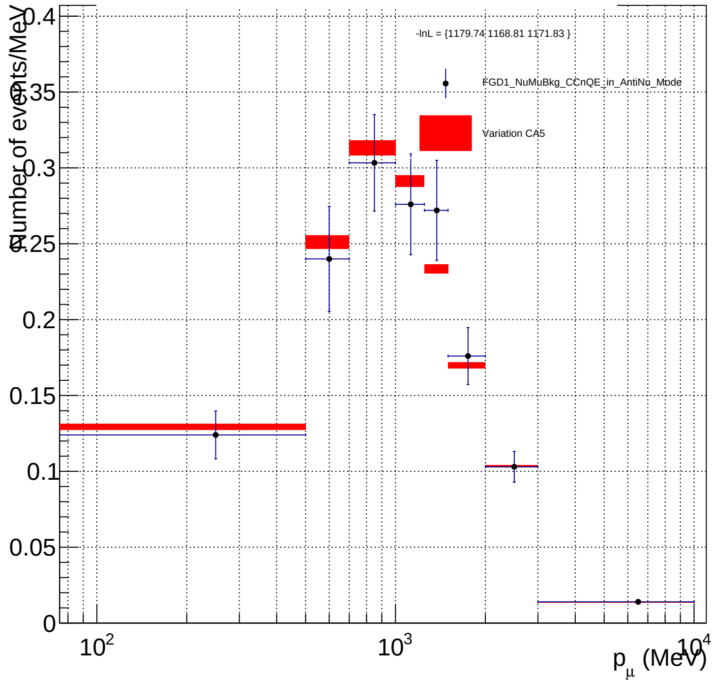
FGD1_NuMuBkg_CCnQE_in_AntiNu_Mode_CA5_X_norm
