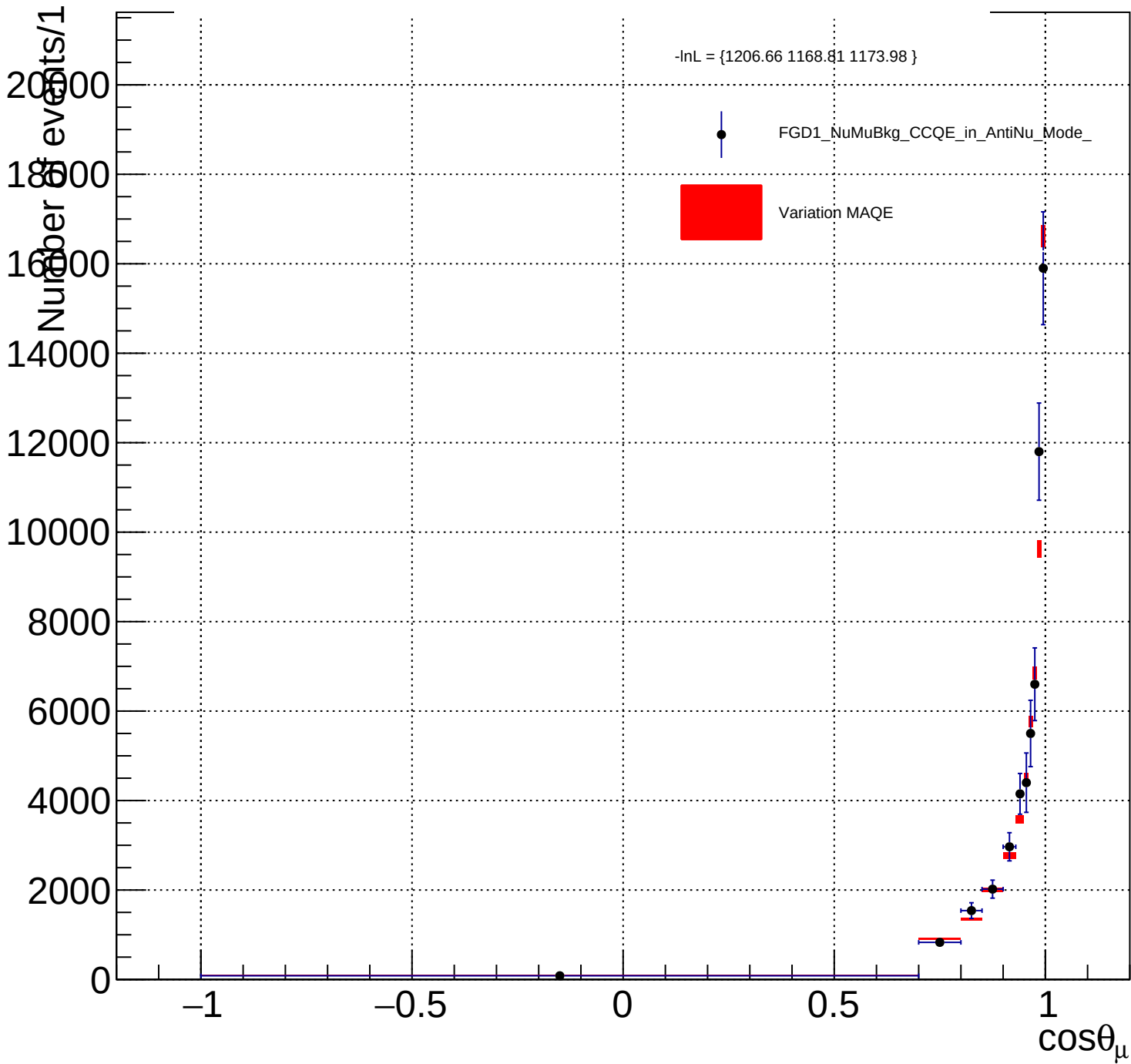
FGD1_NuMuBkg_CCQE_in_AntiNu_Mode__MAQE_Y_norm
