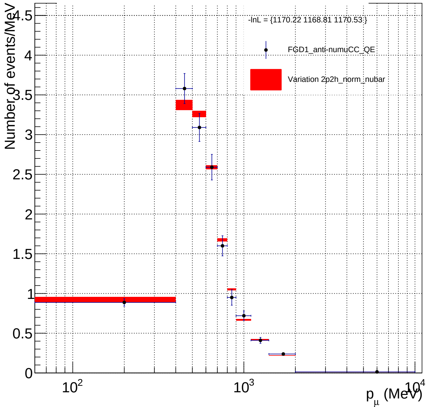
FGD1_anti-numuCC_QE_2p2h_norm_nubar_X_norm
