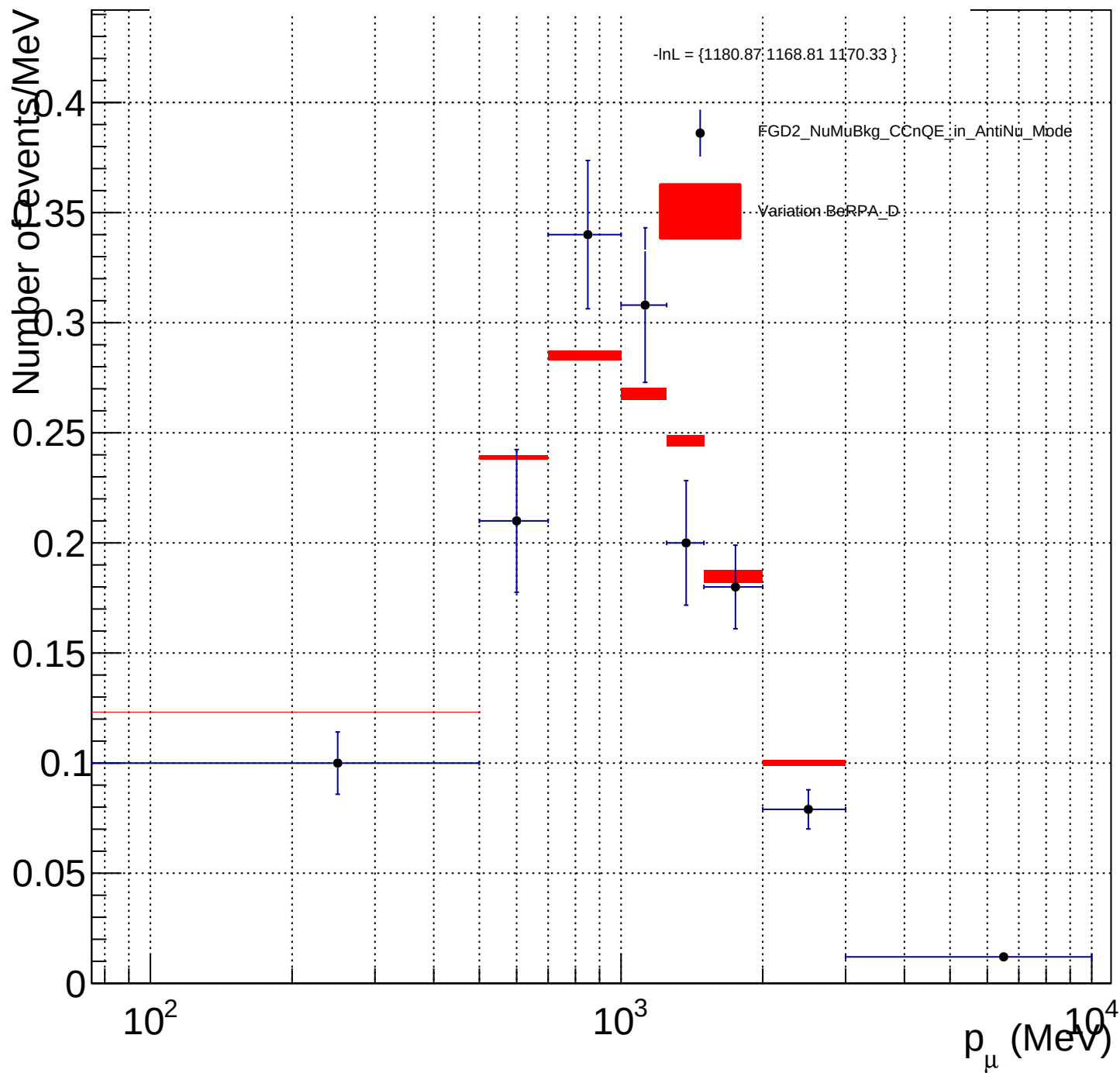
FGD2_NuMuBkg_CCnQE_in_AntiNu_Mode_BeRPA_D_X_norm
