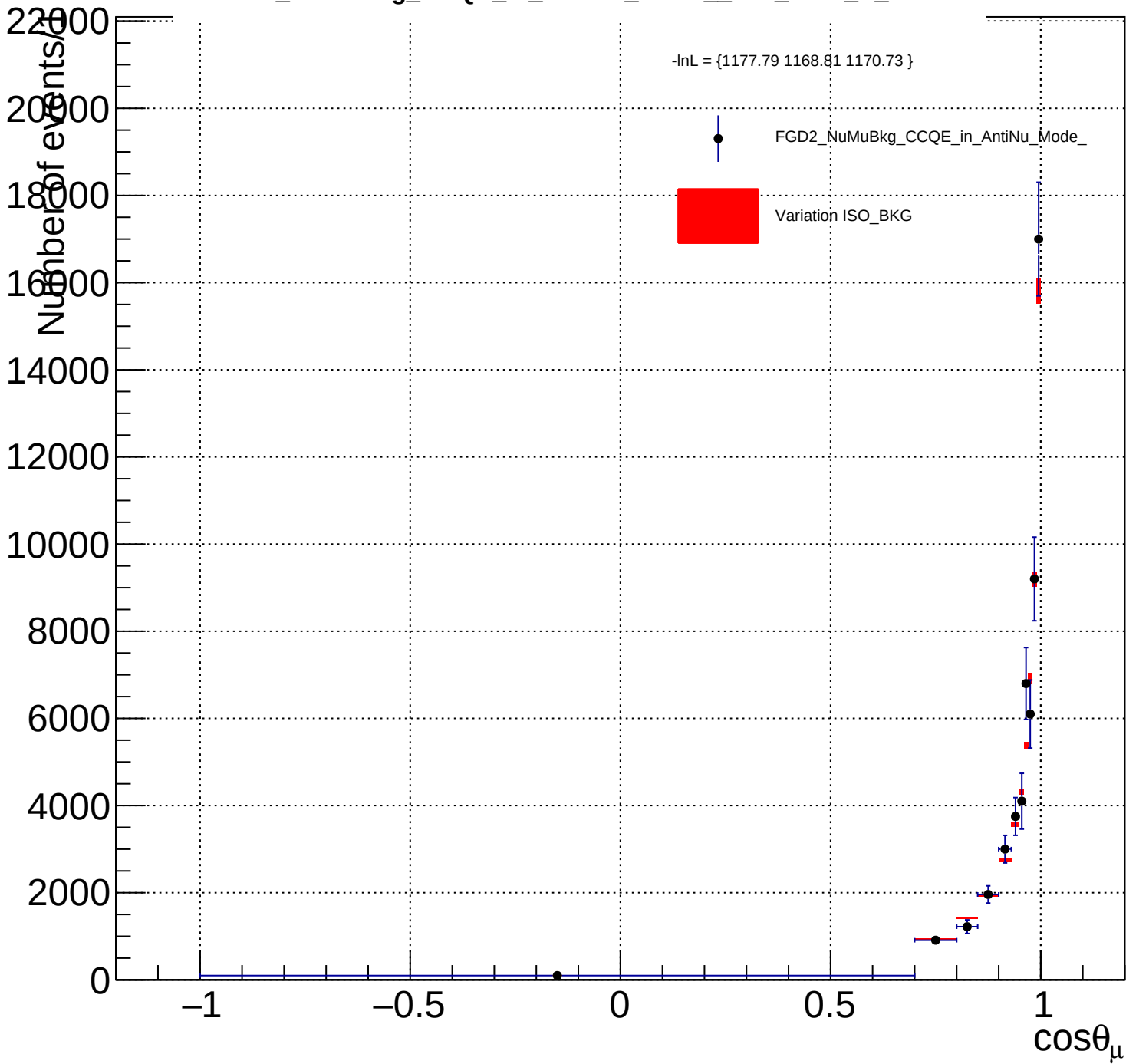
FGD2_NuMuBkg_CCQE_in_AntiNu_Mode_ISO_BKG_Y_norm
