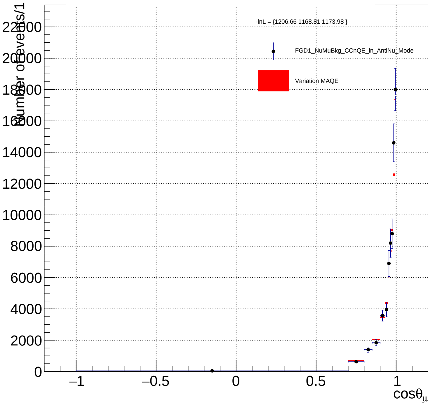
FGD1_NuMuBkg_CCnQE_in_AntiNu_Mode_MAZE_Y_norm
