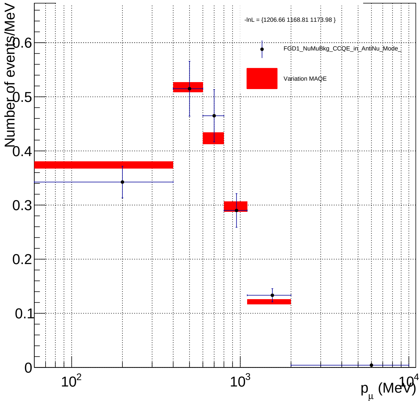
FGD1_NuMuBkg_CCQE_in_AntiNu_Mode__MAQE_X_norm
