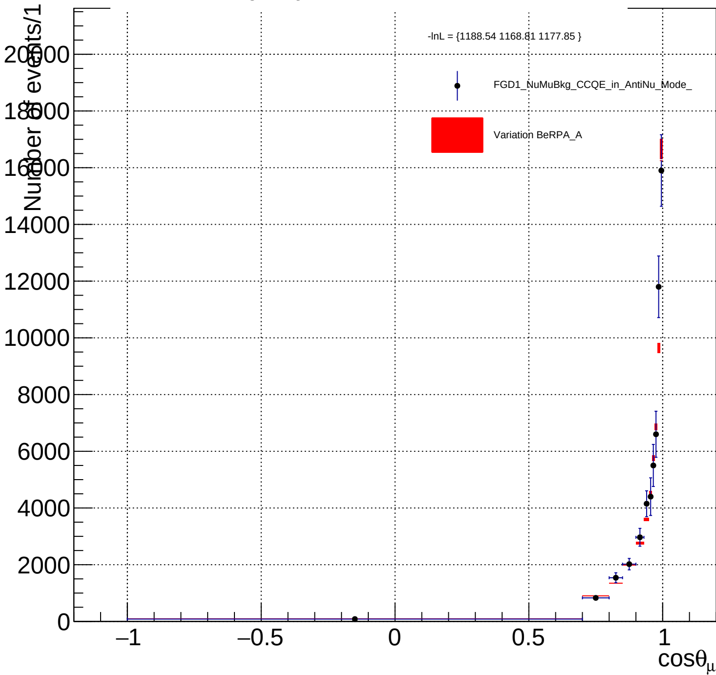
FGD1_NuMuBkg_CCQE_in_AntiNu_Mode__BeRPA_A_Y_norm
