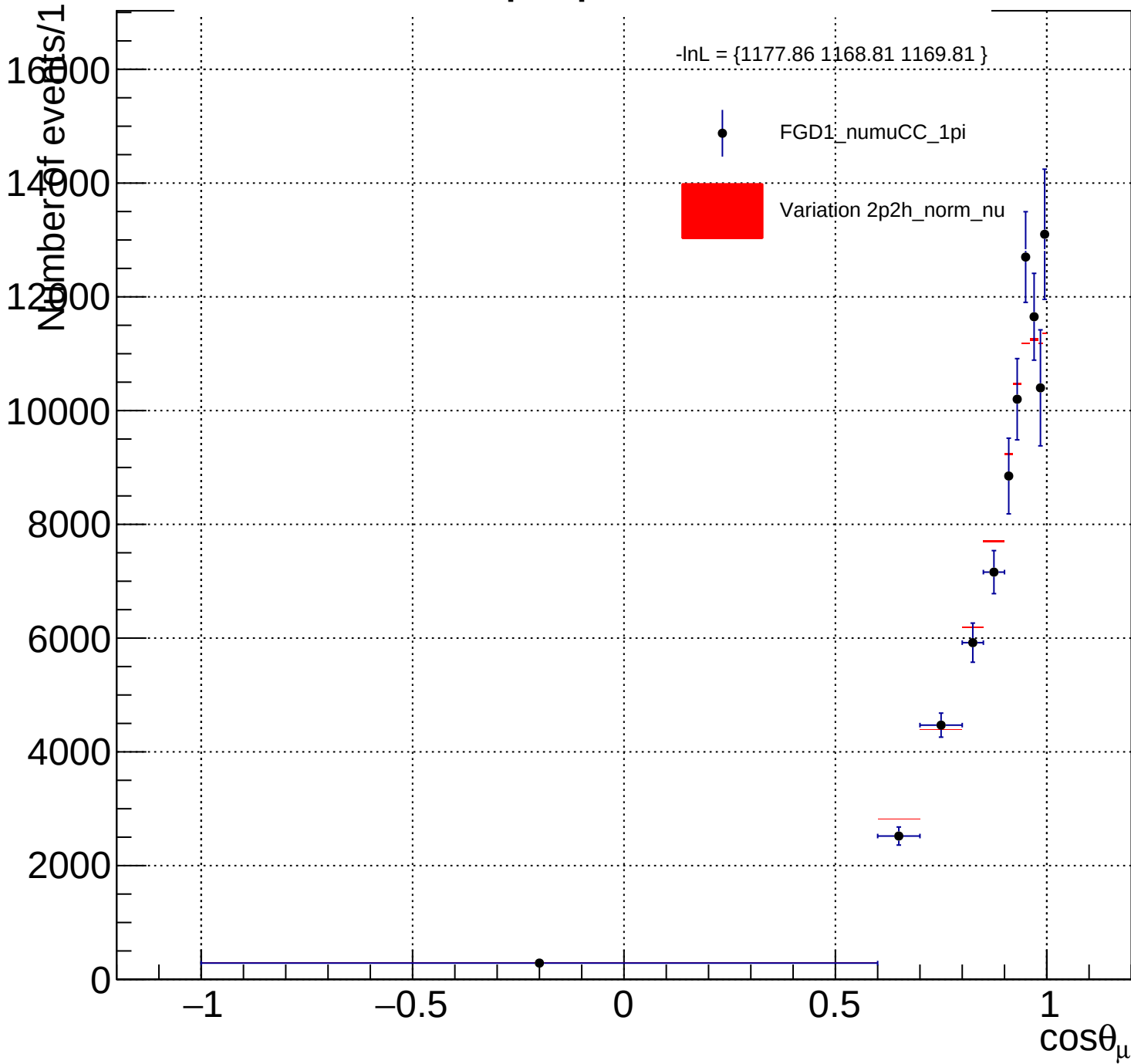
FGD1_numuCC_1pi_2p2h_norm_nu_Y_norm
