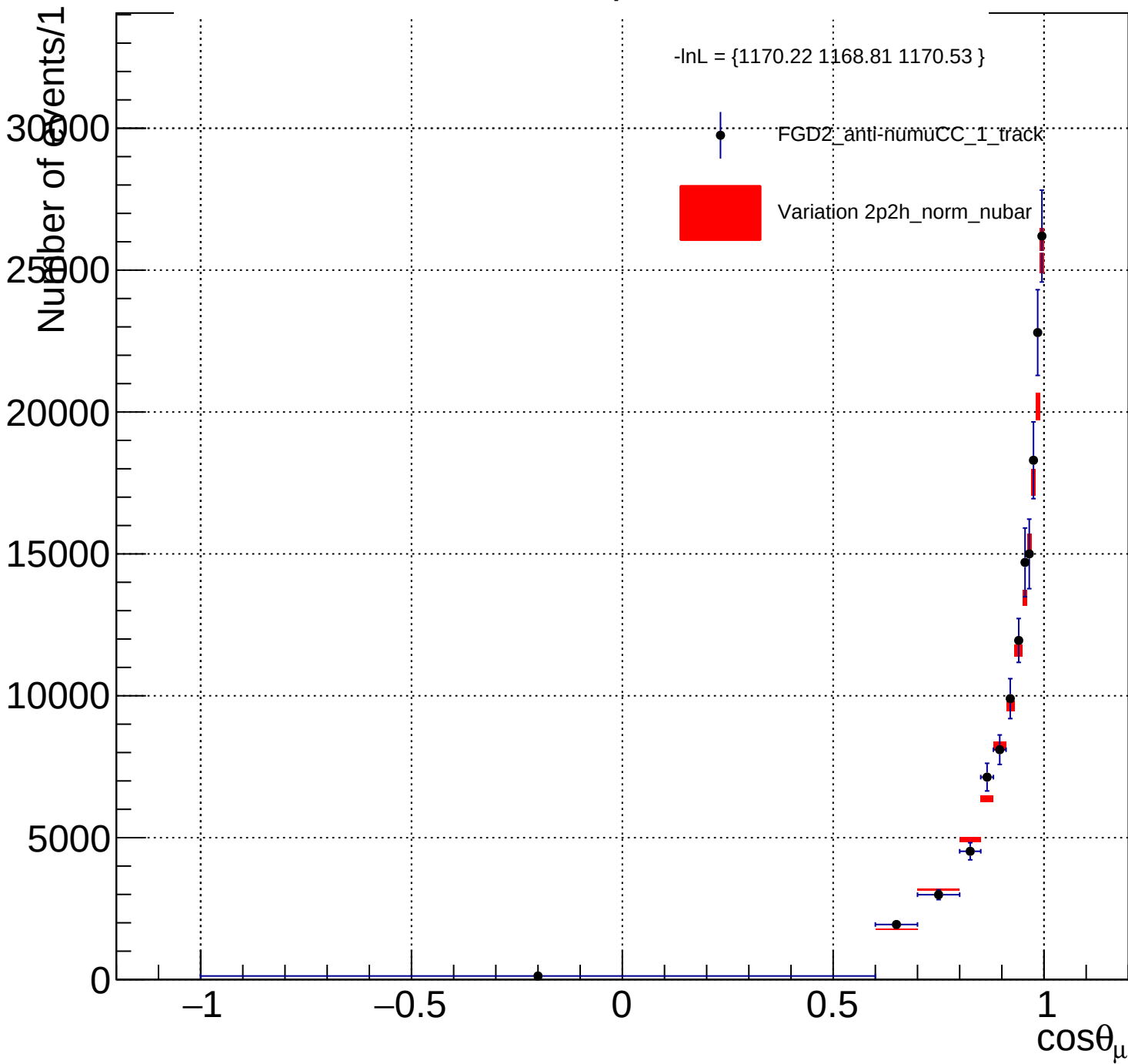
FGD2_anti-numuCC_1_track_2p2h_norm_nubar_Y_norm
