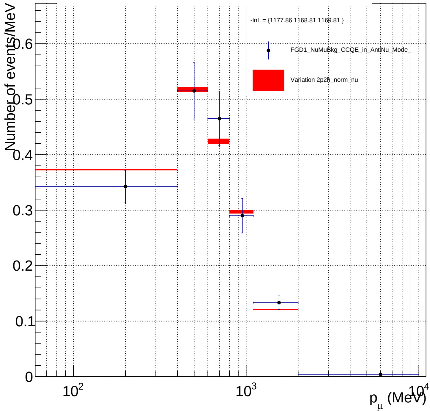
FGD1_NuMuBkg_CCQE_in_AntiNu_Mode_2p2h_norm_nu_X_norm
