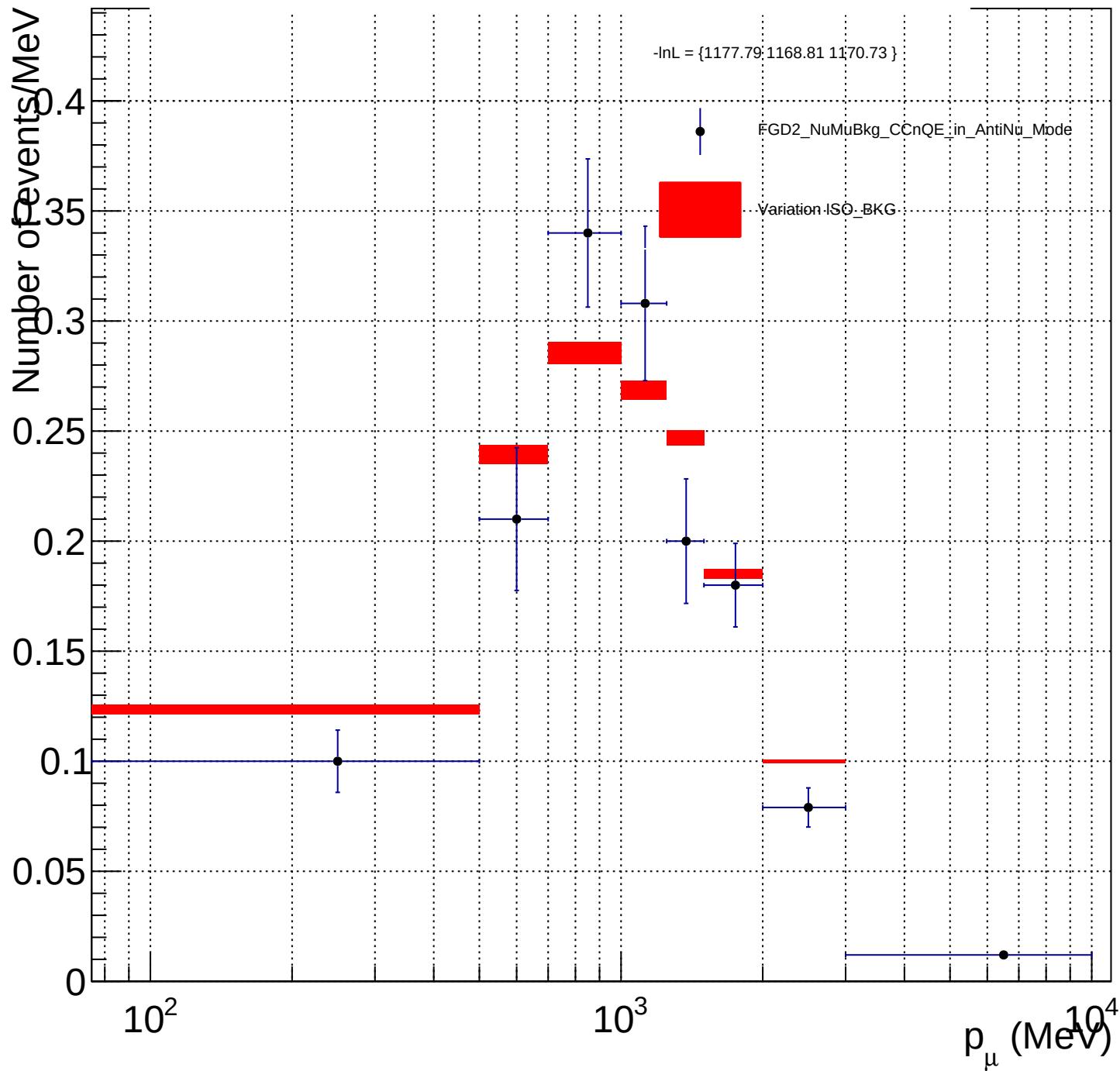
FGD2_NuMuBkg_CCnQE_in_AntiNu_Mode_ISO_BKG_X_norm
