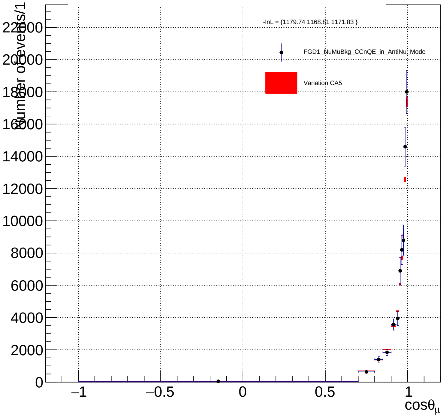
FGD1_NuMuBkg_CCnQE_in_AntiNu_Mode_CA5_Y_norm
