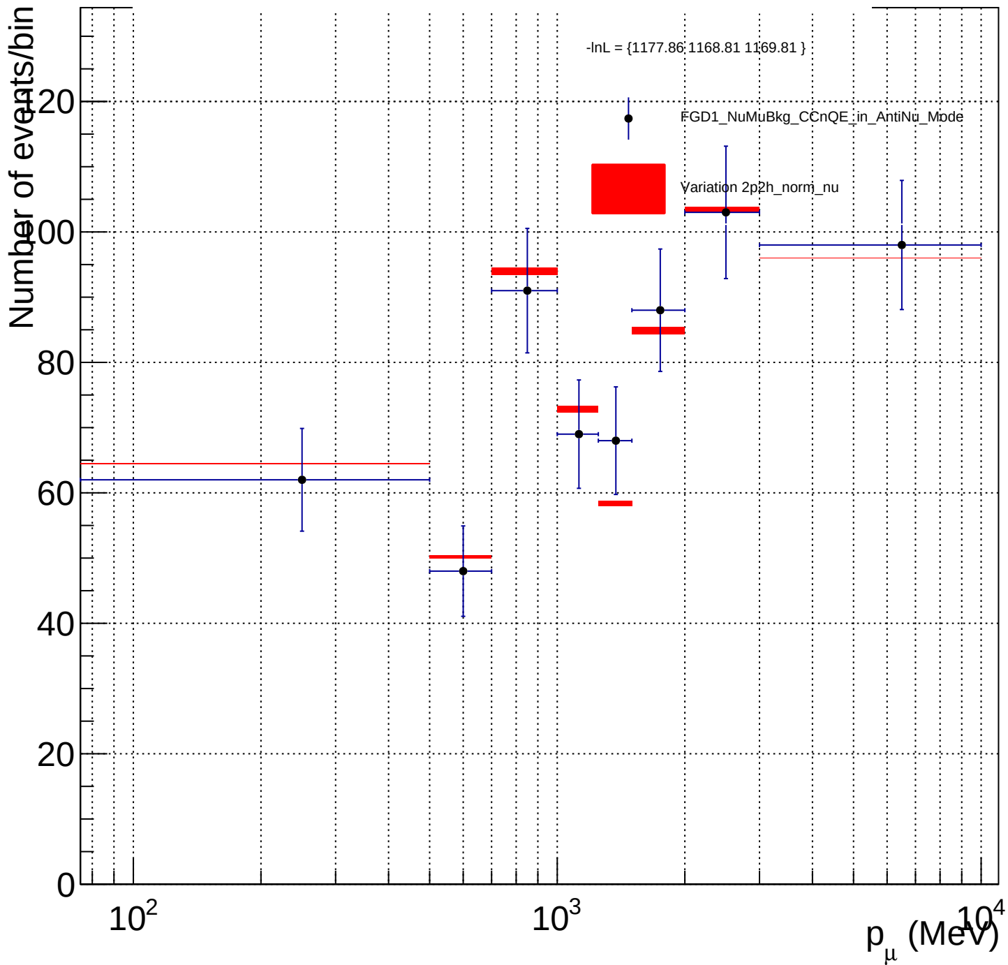
FGD1_NuMuBkg_CCnQE_in_AntiNu_Mode_2p2h_norm_nu_X
