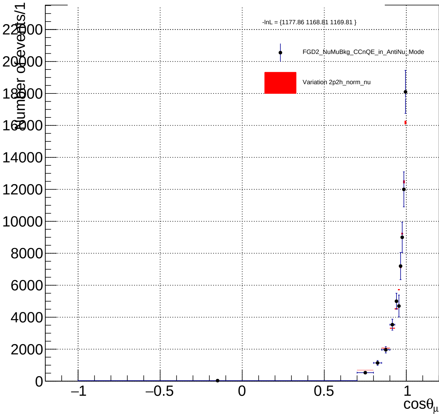
FGD2_NuMuBkg_CCnQE_in_AntiNu_Mode_2p2h_norm_nu_Y_norm
