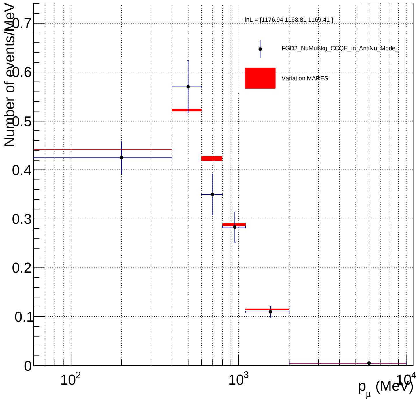
FGD2_NuMuBkg_CCQE_in_AntiNu_Mode__MARES_X_norm
