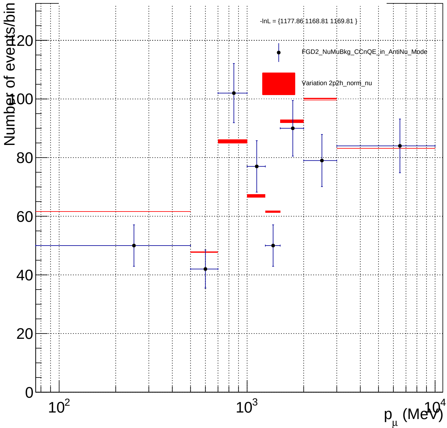
FGD2_NuMuBkg_CCnQE_in_AntiNu_Mode_2p2h_norm_nu_X
