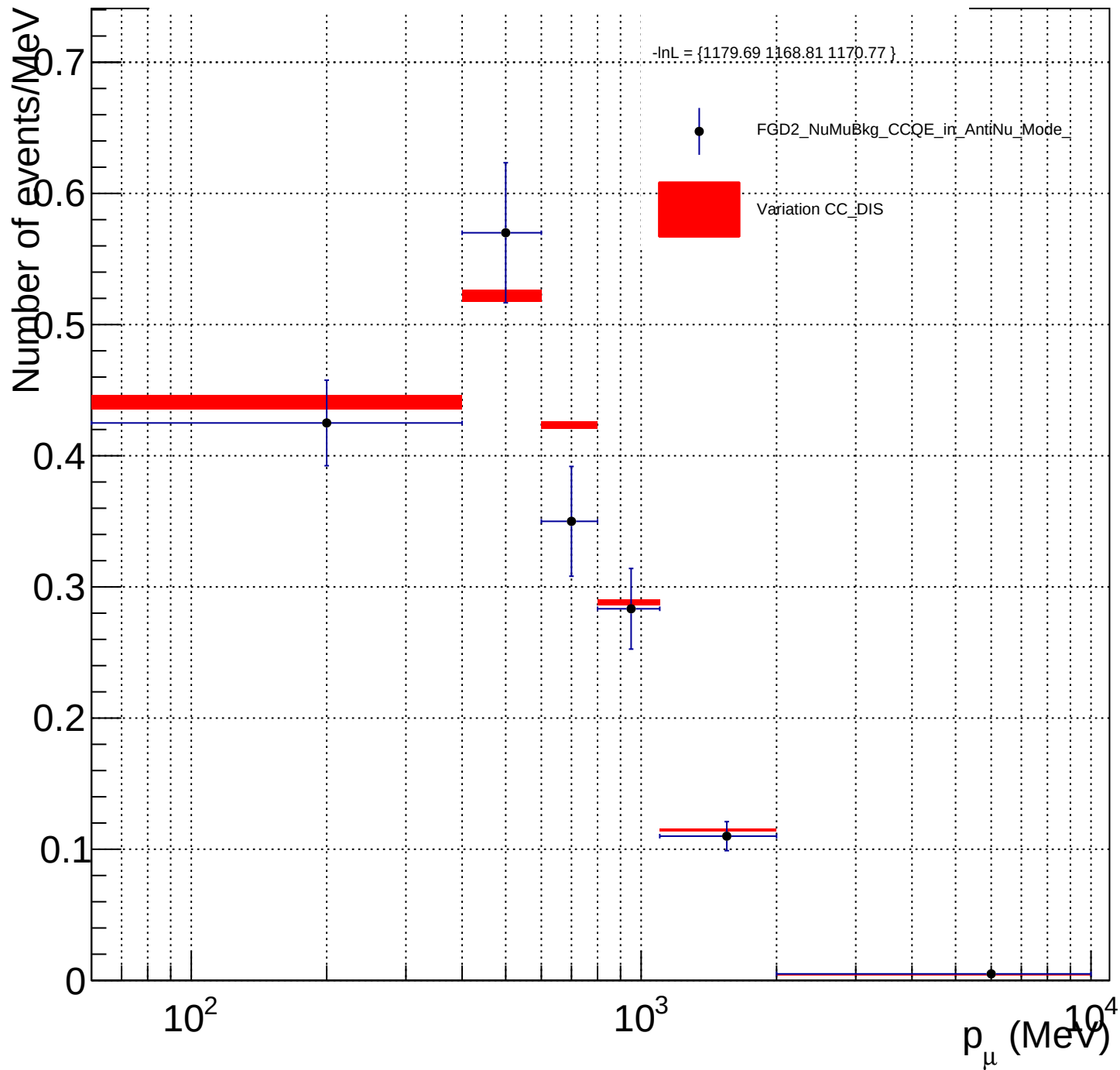
FGD2_NuMuBkg_CCQE_in_AntiNu_Mode_CC_DIS_X_norm
