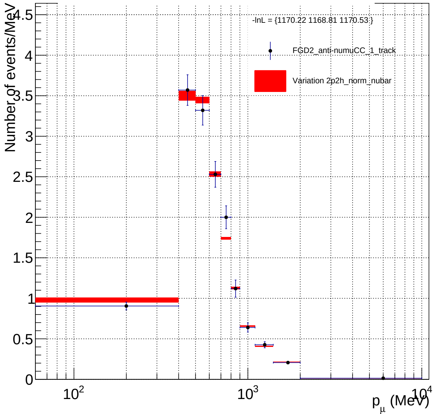
FGD2_anti-numuCC_1_track_2p2h_norm_nubar_X_norm
