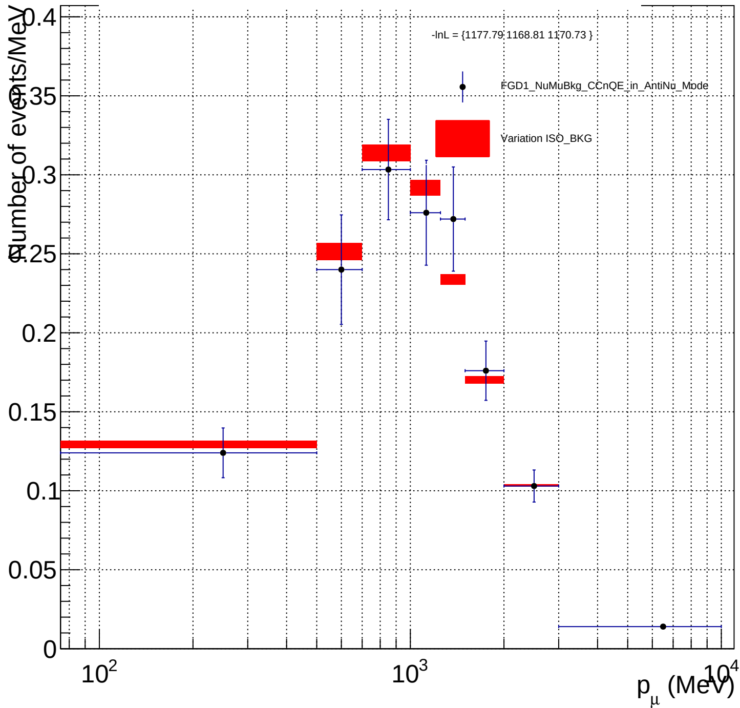
FGD1_NuMuBkg_CCnQE_in_AntiNu_Mode_ISO_BKG_X_norm
