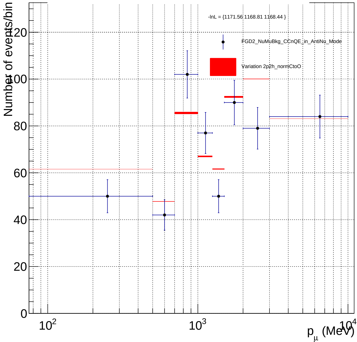
FGD2_NuMuBkg_CCnQE_in_AntiNu_Mode_2p2h_normCtoO_X
