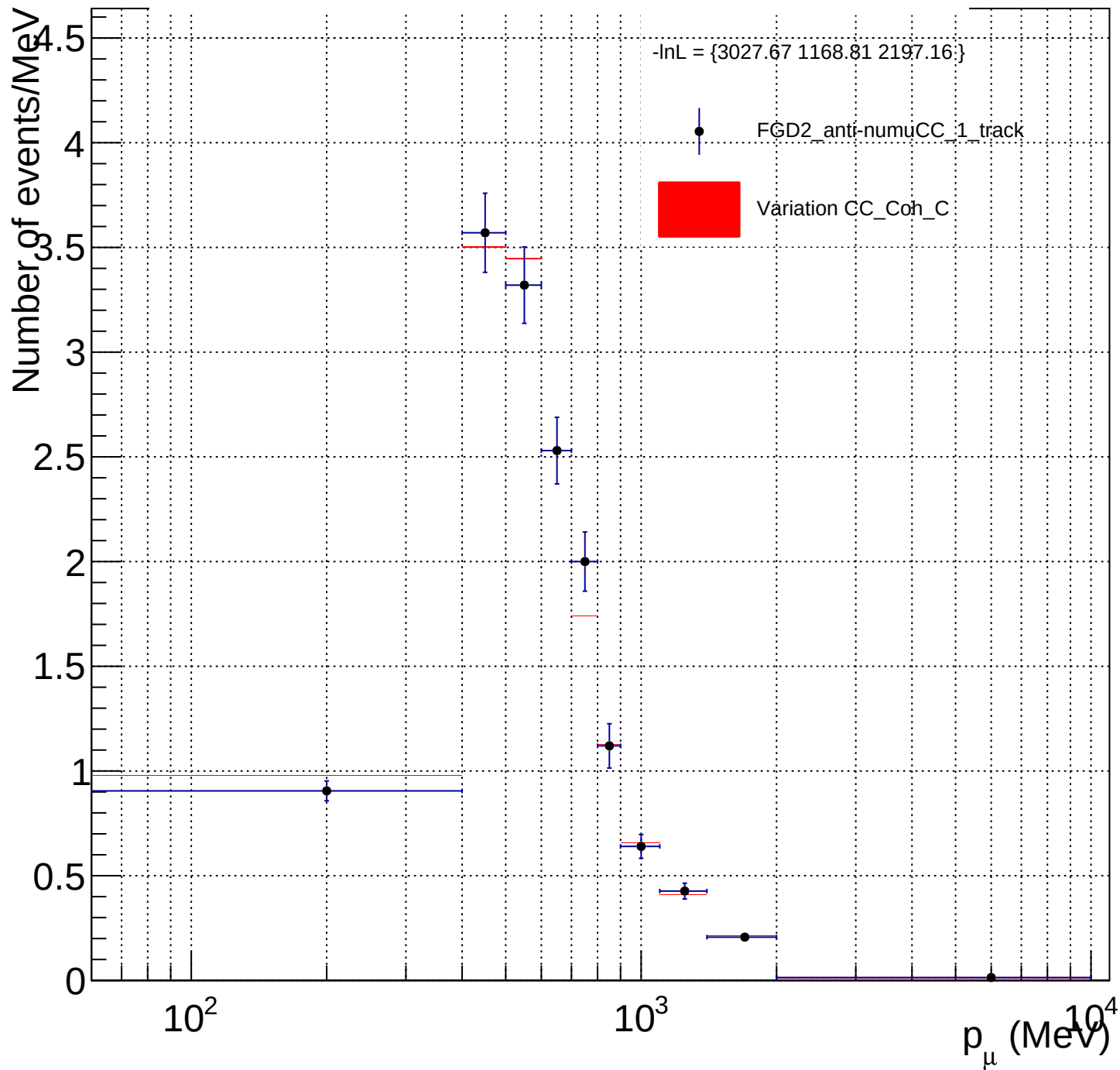
FGD2_anti-numuCC_1_track_CC_Coh_C_X_norm
