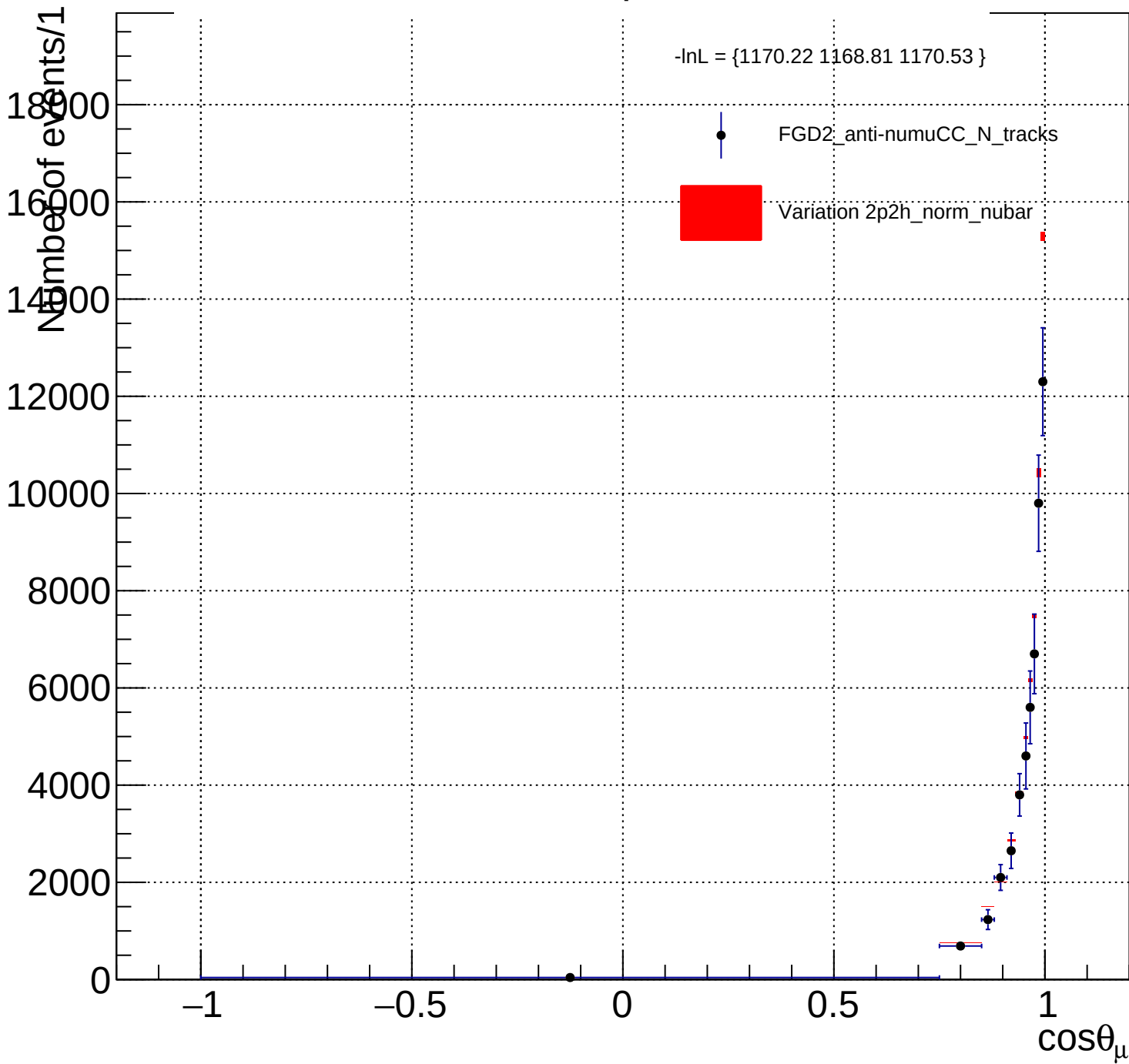
FGD2_anti-numuCC_N_tracks_2p2h_norm_nubar_Y_norm
