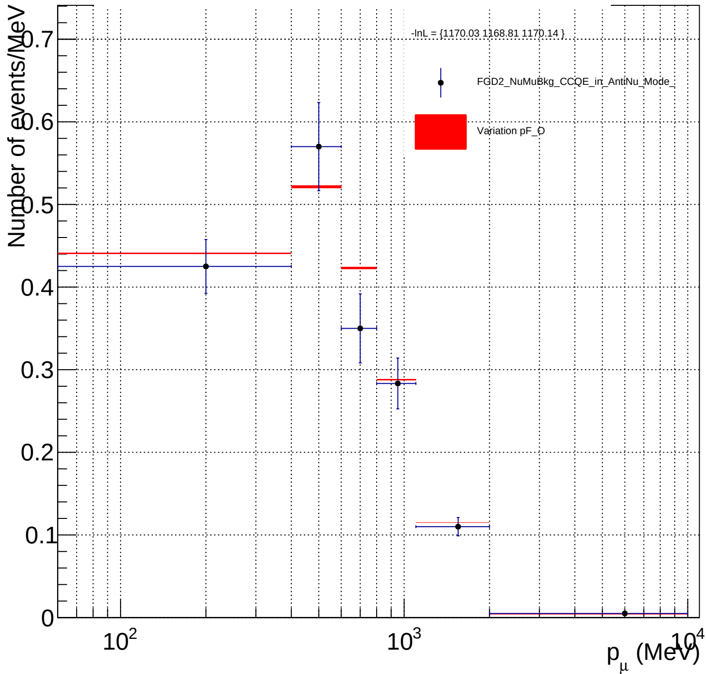
FGD2_NuMuBkg_CCQE_in_AntiNu_Mode_pF_O_X_norm
