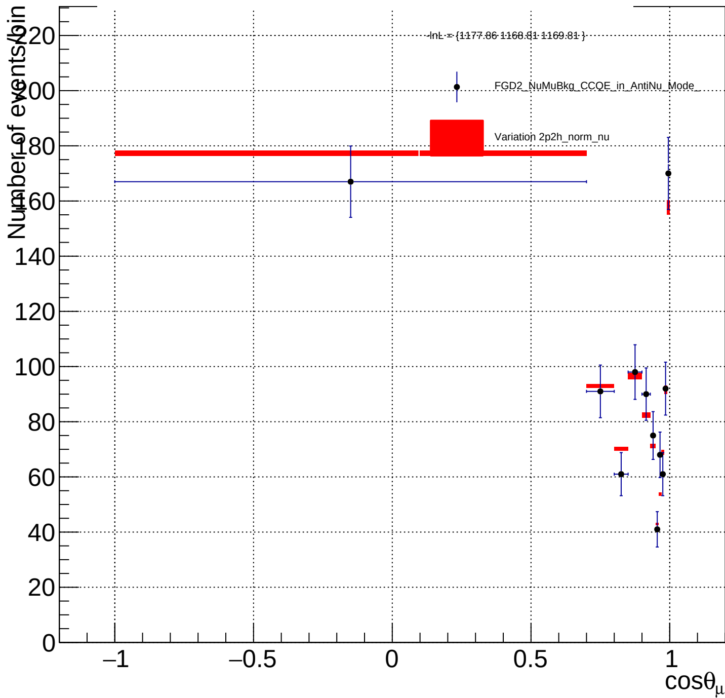
FGD2_NuMuBkg_CCQE_in_AntiNu_Mode_2p2h_norm_nu_Y
