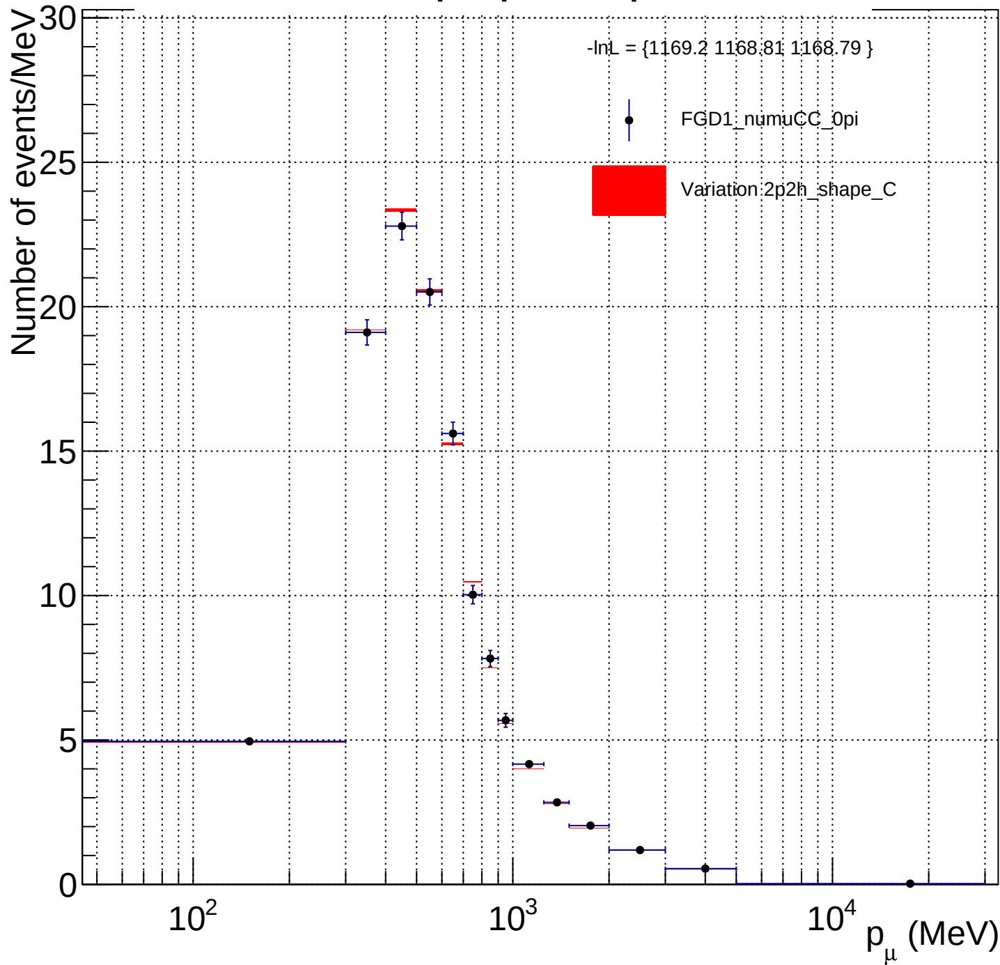
FGD1_numuCC_0pi_2p2h_shape_C_X_norm
