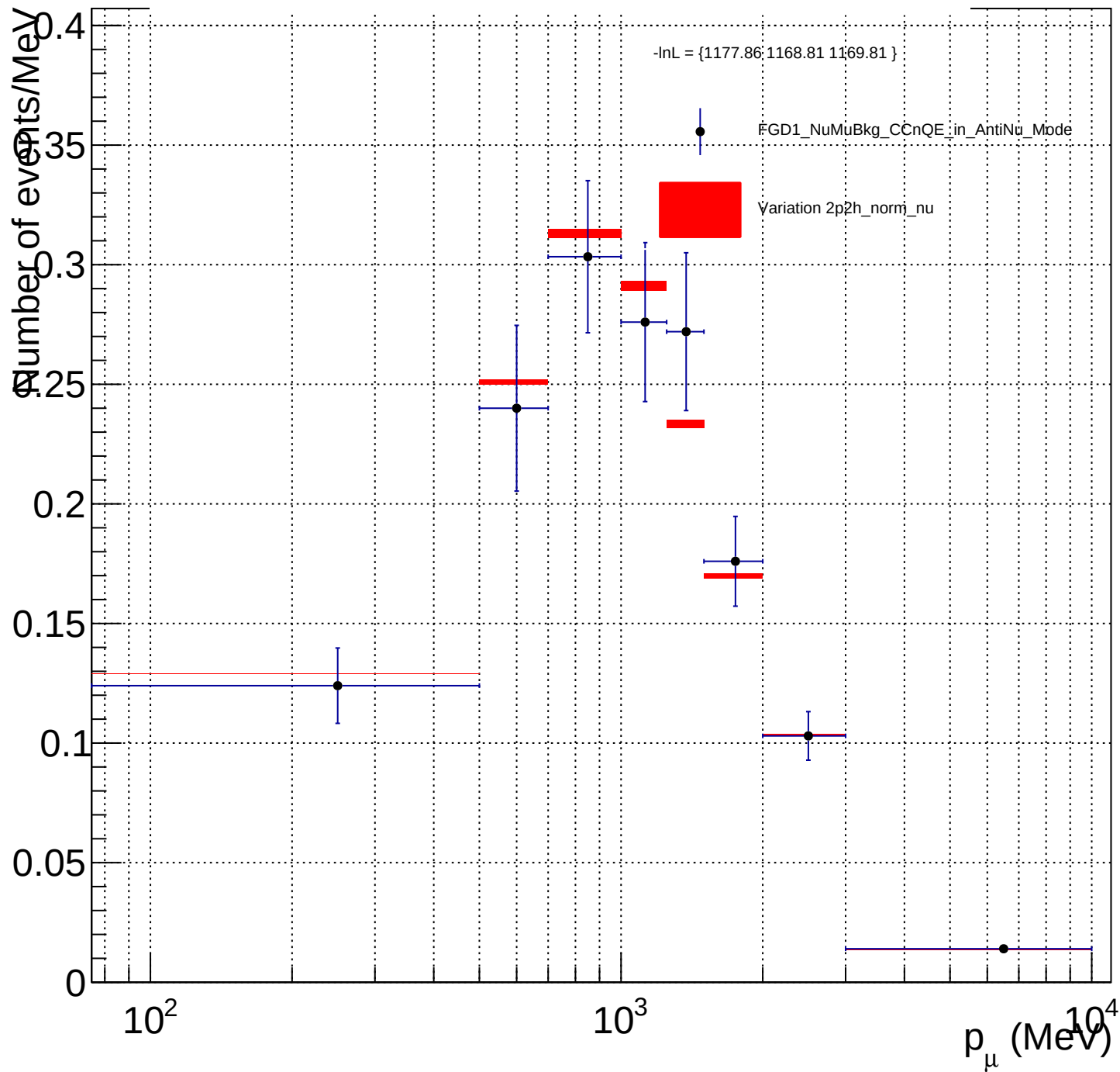
FGD1_NuMuBkg_CCnQE_in_AntiNu_Mode_2p2h_norm_nu_X_norm
