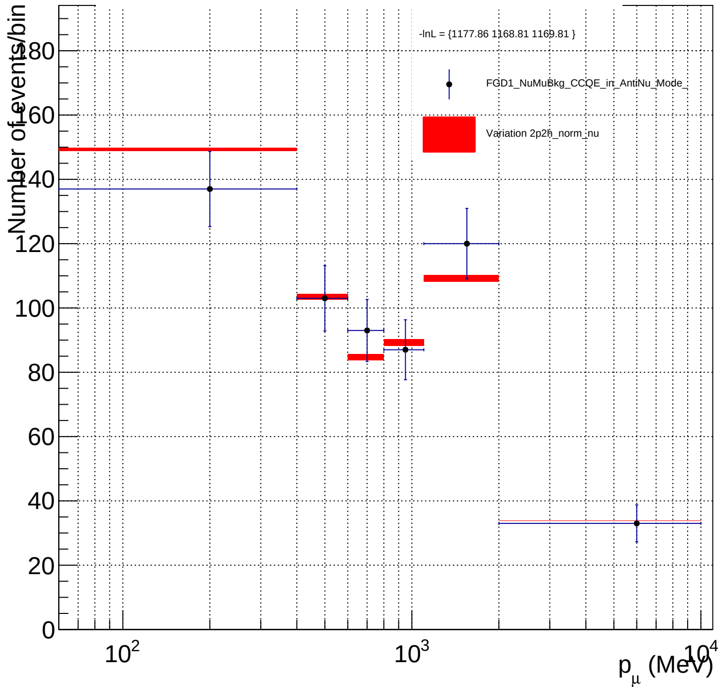
FGD1_NuMuBkg_CCQE_in_AntiNu_Mode_2p2h_norm_nu_X
