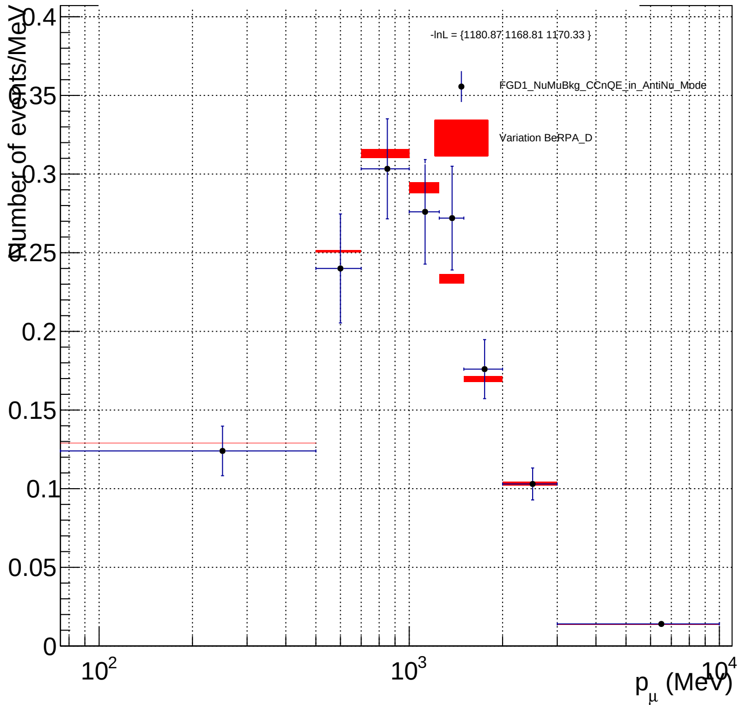
FGD1_NuMuBkg_CCnQE_in_AntiNu_Mode_BeRPA_D_X_norm
