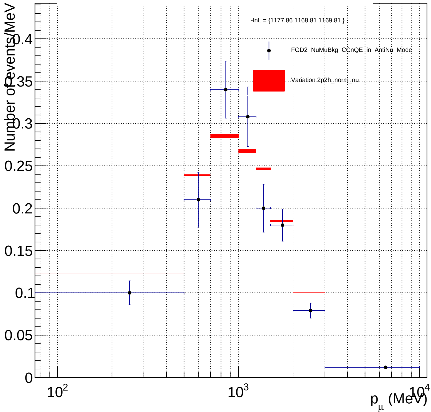
FGD2_NuMuBkg_CCnQE_in_AntiNu_Mode_2p2h_norm_nu_X_norm
