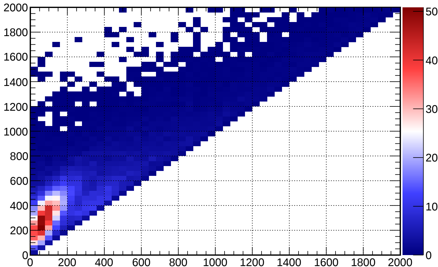
FGD2_anti-numuCC_1_track_2p2h_shape_O_nubar_0
