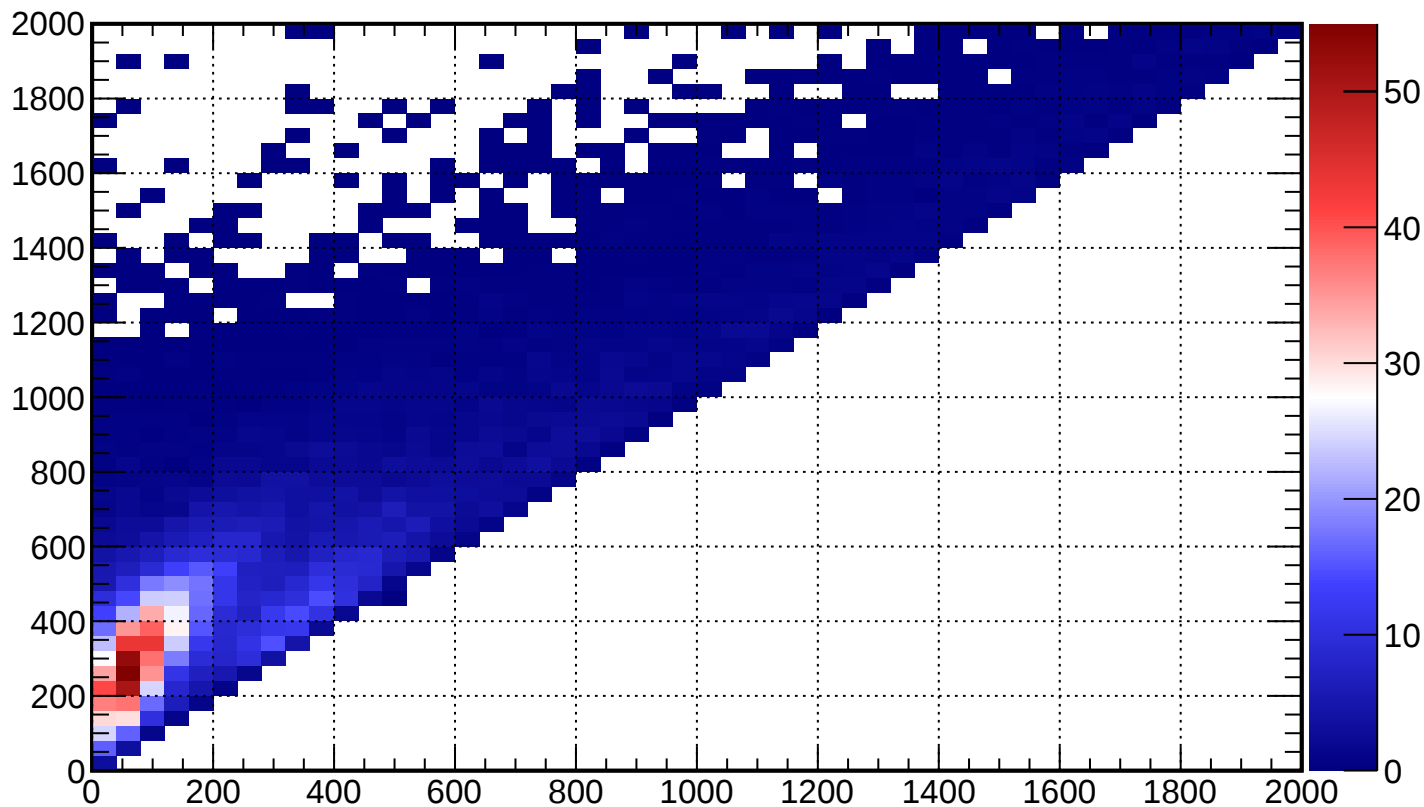
FGD1_anti-numuCC_QE_2p2h_shape_C_nubar_1
