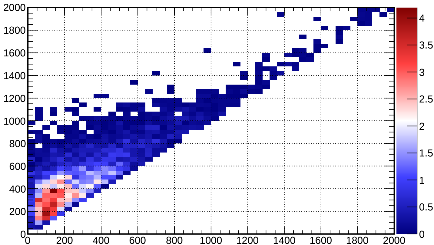
FGD1_anti-numuCC_QE_2p2h_shape_C_nubar_0_2p2h
