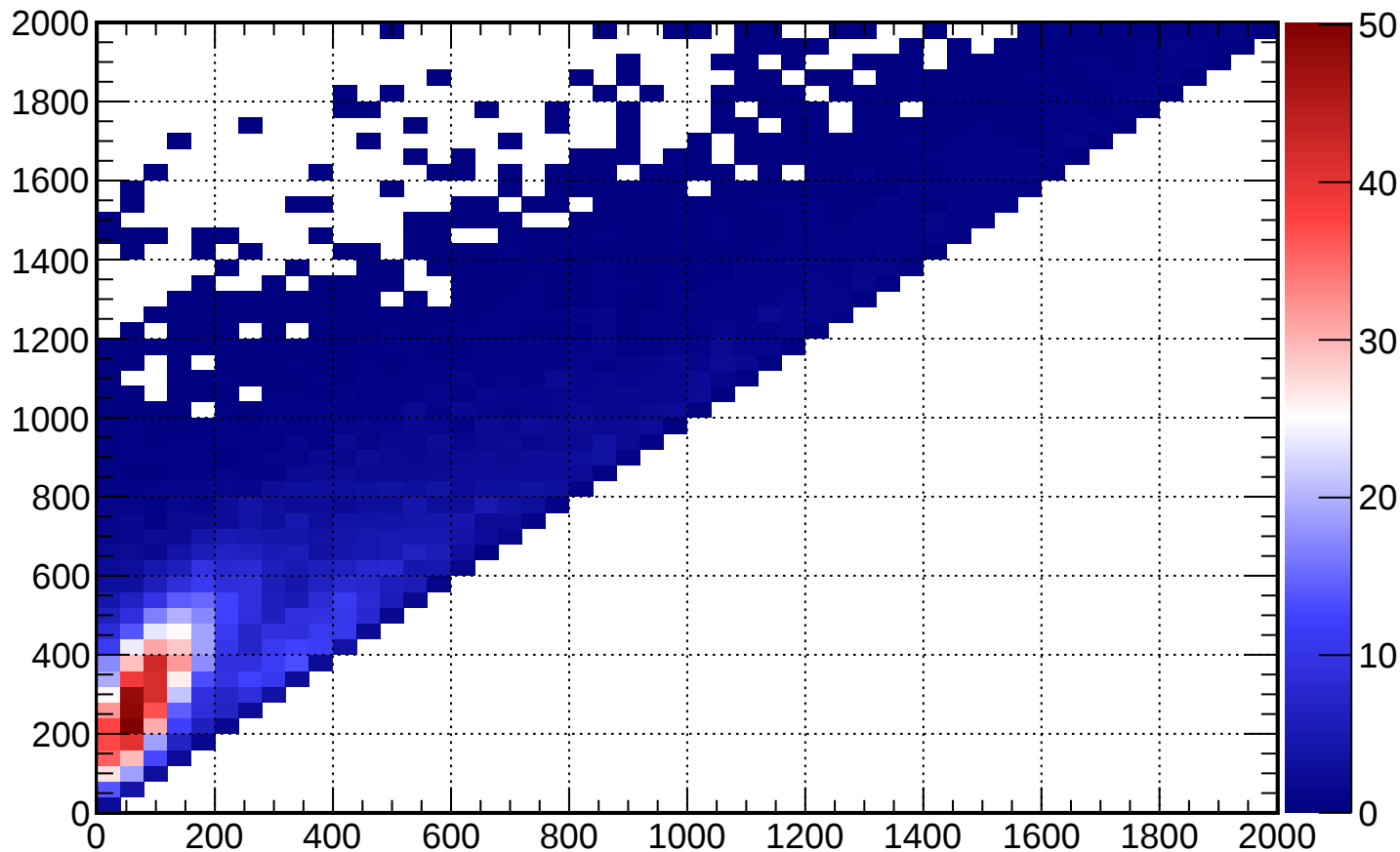
FGD2_anti-numuCC_1_track_2p2h_shape_O_nubar_1
