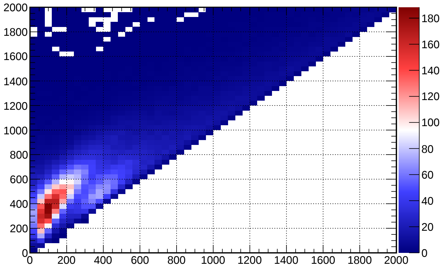
FGD2_numuCC_0pi_2p2h_shape_O_nu_0
