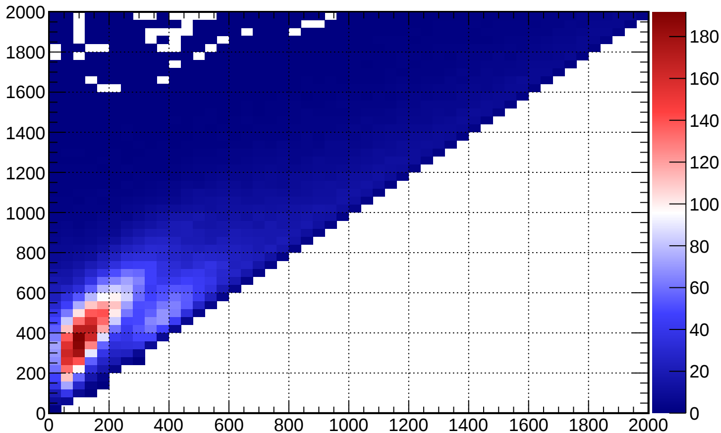
FGD2_numuCC_0pi_2p2h_shape_O_nu_-1
