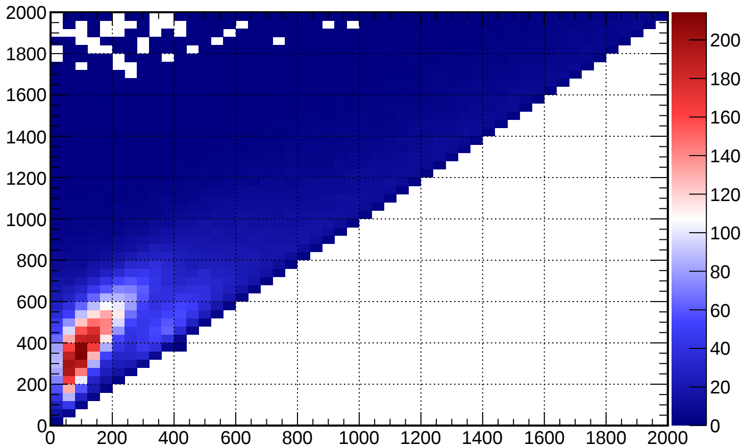
FGD1_numuCC_0pi_2p2h_shape_C_nu_-1
