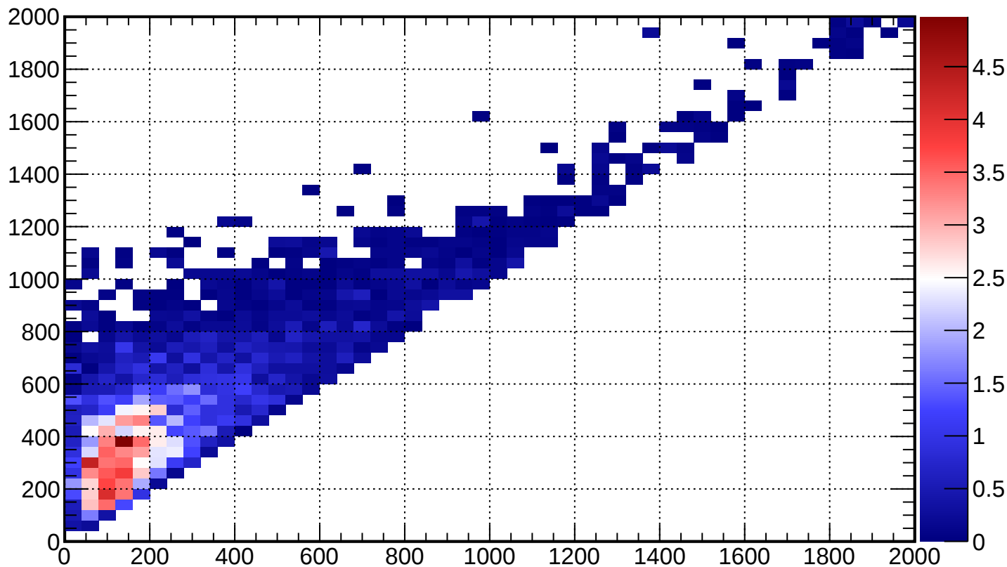
FGD1_anti-numuCC_QE_2p2h_shape_C_nubar_-1_2p2h
