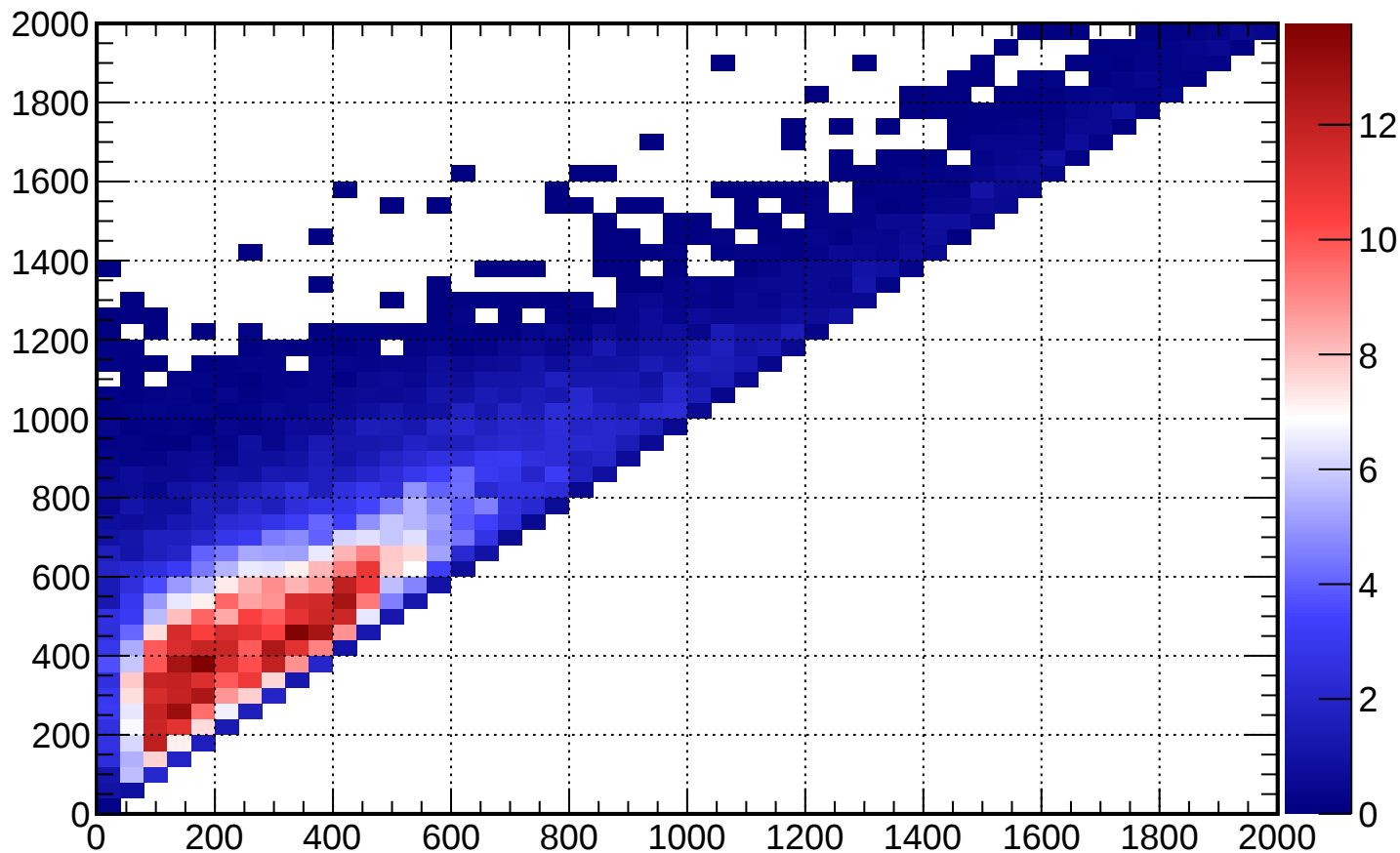
FGD2_numuCC_0pi_2p2h_shape_O_nu_0_2p2h
