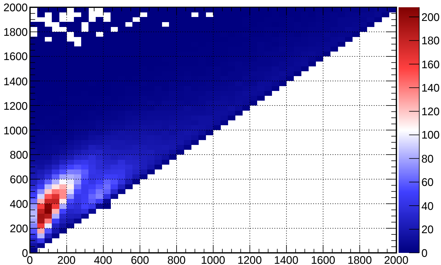
FGD1_numuCC_0pi_2p2h_shape_C_nu_0
