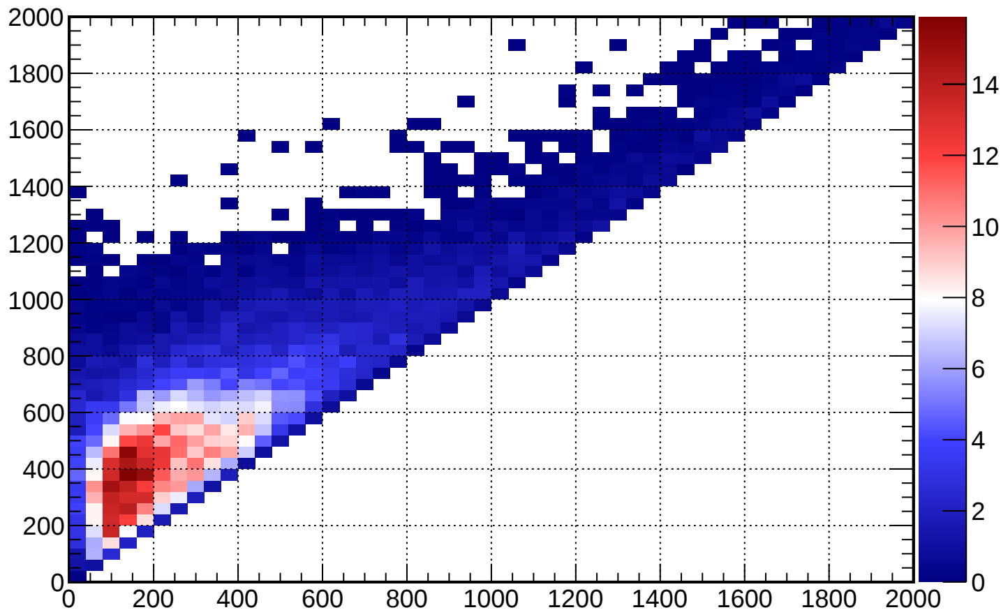
FGD2_numuCC_0pi_2p2h_shape_O_nu_-1_2p2h
