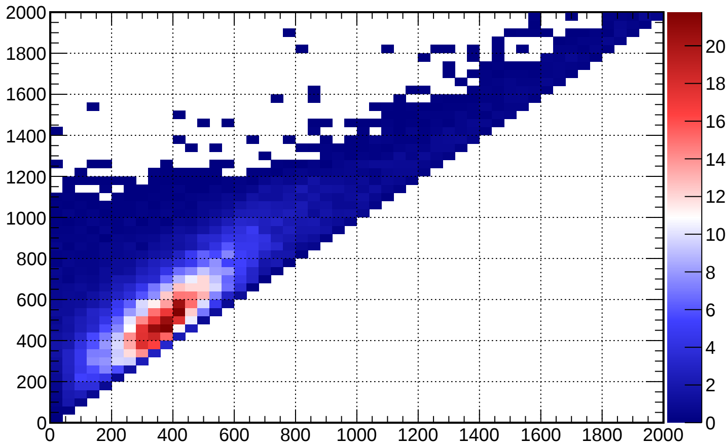
FGD1_numuCC_0pi_2p2h_shape_C_nu_1_2p2h
