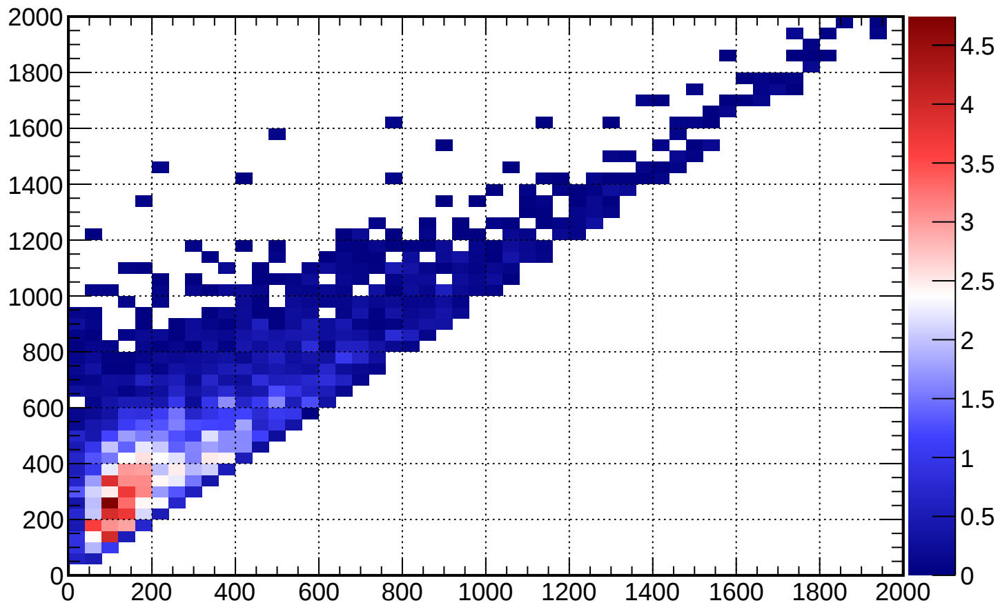
FGD2_anti-numuCC_1_track_2p2h_shape_O_nubar_0_2p2h
