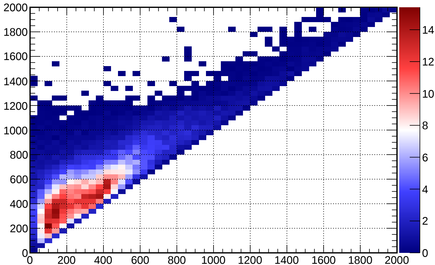
FGD1_numuCC_0pi_2p2h_shape_C_nu_0_2p2h
