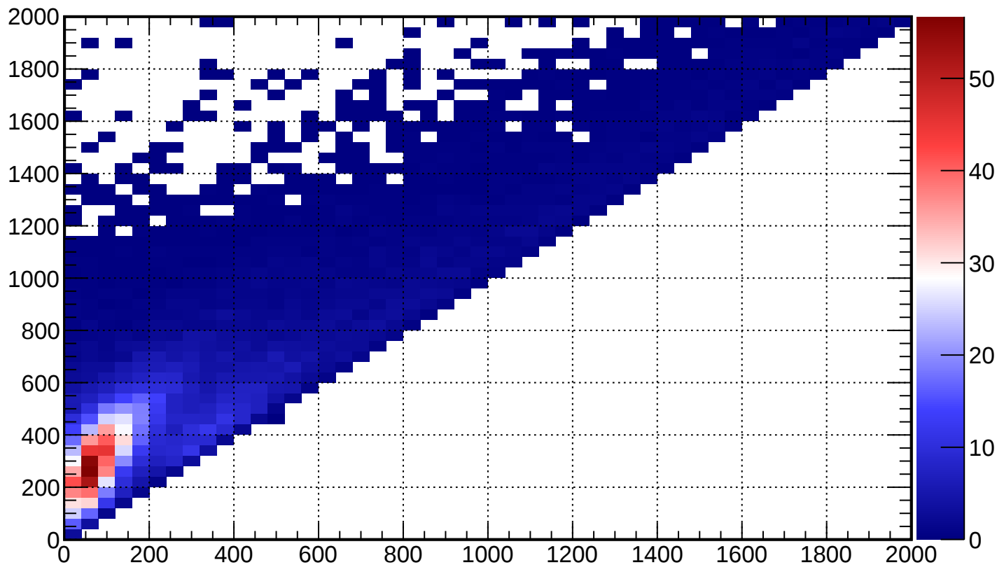
FGD1_anti-numuCC_QE_2p2h_shape_C_nubar_0
