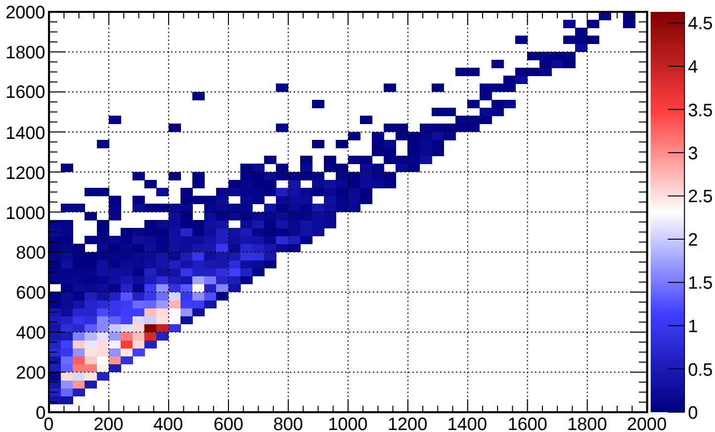
FGD2_anti-numuCC_1_track_2p2h_shape_O_nubar_1_2p2h
