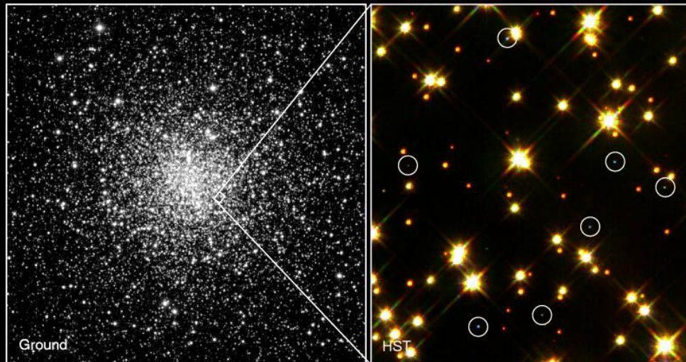
Seven white dwarfs (circled) in a small section of globular cluster M4 (By H. Richer and M. Bolte . Left: Kitt Peak National Observatory 36"; right: Hubble Space Telescope).
