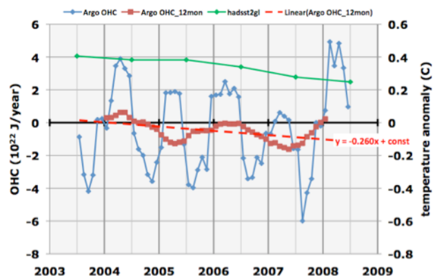
Figure 1. Ocean heat content from Argo (left scale: blue, original data; red, filtered) and ocean surface temperatures (right scale, green). Conversion of the OHC slope to \text{W/m}^2 is made by multiplying by 0.62, yielding -0.161 \text{ W/m}^2 .
