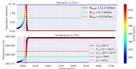
Distance: 1.03 AU, Carrying Capacity: 70 billion ppl, \Lambda : 0.063
