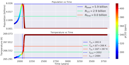
Distance: 1.03 AU, Carrying Capacity: 40 billion ppl, \Lambda : 0.11
