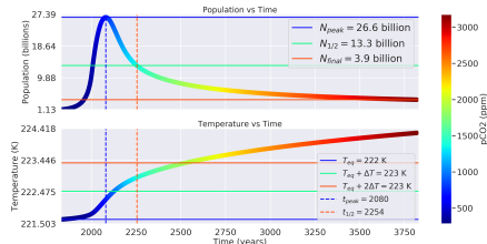
Distance: 1.06 AU, Carrying Capacity: 40 billion ppl, \Lambda : 3.3
