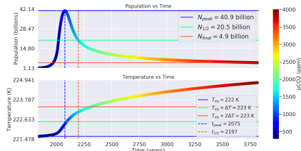
Distance: 1.06 AU, Carrying Capacity: 70 billion ppl, \Lambda : 1.885
