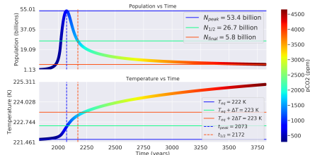
Distance: 1.06 AU, Carrying Capacity : 100 billion ppl, \Lambda : 1.32
