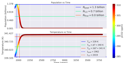
Distance: 0.94 AU, Carrying Capacity : 70 billion ppl, \Lambda : 0.016
