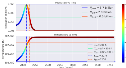
Distance: 0.97 AU, Carrying Capacity: 70 billion ppl, \Lambda : 0.25
