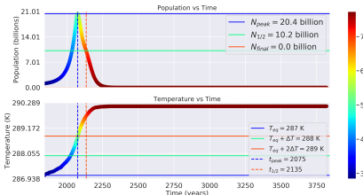
Distance: 1.0 AU, Carrying Capacity: 100 billion ppl, \Lambda : 0.256
