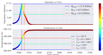
Distance: 1.0 AU, Carrying Capacity: 70 billion ppl, \Lambda : 0.366
