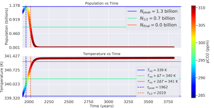
Distance: 0.94 AU, Carrying Capacity: 40 billion ppl, \Lambda : 0.027
