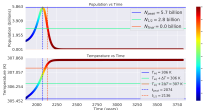
Distance: 0.97 AU, Carrying Capacity: 100 billion ppl, \Lambda : 0.175
