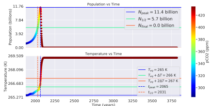
Distance: 1.03 AU, Carrying Capacity : 100 billion ppl, \Lambda : 0.044
