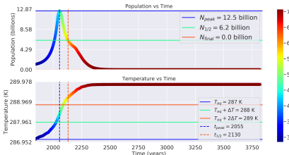
Distance: 1.0 AU, Carrying Capacity : 40 billion ppl, \Lambda : 0.64
