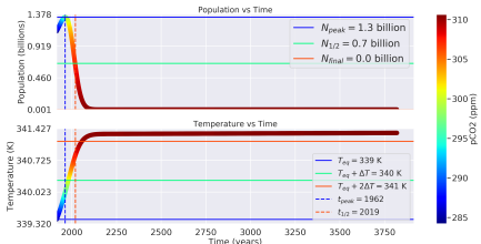
Distance: 0.94 AU, Carrying Capacity : 100 billion ppl, \Lambda : 0.011
