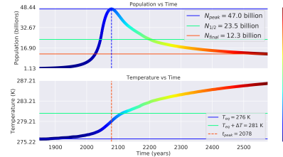
Distance: 1.02 AU, Carrying Capacity: 70 billion ppl, \Gamma : 0.873
