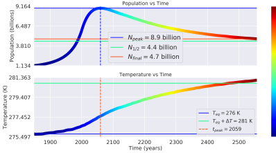
Distance: 1.02 AU, Carrying Capacity: 40 billion ppl, \Gamma : 0.499
