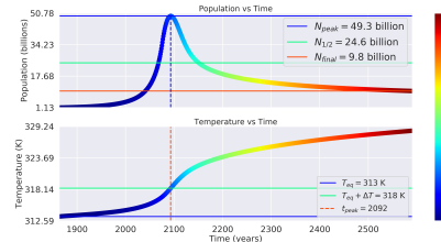
Distance: 0.96 AU, Carrying Capacity: 100 billion ppl, \Gamma : 2.276
