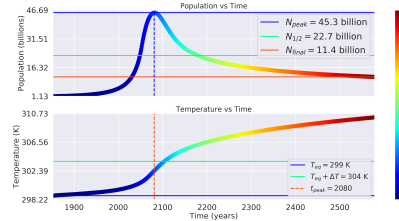
Distance: 0.98 AU, Carrying Capacity: 70 billion ppl, \Gamma : 1.005
