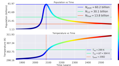
Distance: 0.98 AU, Carrying Capacity: 100 billion ppl, \Gamma : 1.435
