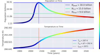
Distance: 1.0 AU, Carrying Capacity: 40 billion ppl, \Gamma : 0.486
