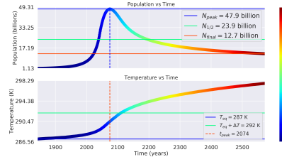
Distance: 1.0 AU, Carrying Capacity: 70 billion ppl, \Gamma : 0.851
