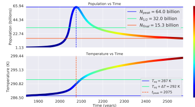
Distance: 1.0 AU, Carrying Capacity: 100 billion ppl, \Gamma : 1.215
