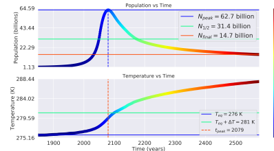
Distance: 1.02 AU, Carrying Capacity: 100 billion ppl, \Gamma : 1.247
