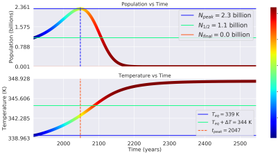
Distance: 0.94 AU, Carrying Capacity: 70 billion ppl, \Gamma : 3.398
