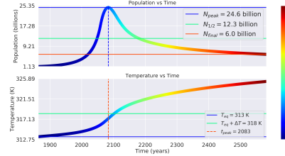
Distance: 0.96 AU, Carrying Capacity: 40 billion ppl, \Gamma : 0.91
