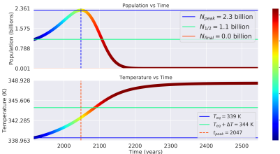
Distance: 0.94 AU, Carrying Capacity: 100 billion ppl, \Gamma : 5.946
