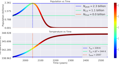
Distance: 0.94 AU, Carrying Capacity: 40 billion ppl, \Gamma : 0.849
