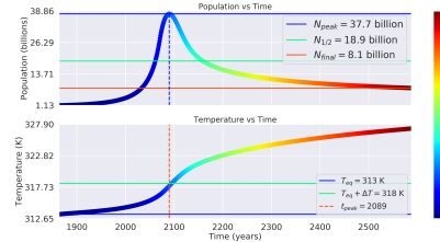
Distance: 0.96 AU, Carrying Capacity: 70 billion ppl, \Gamma : 1.593
