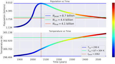
Distance: 0.98 AU, Carrying Capacity: 40 billion ppl, \Gamma : 0.574
