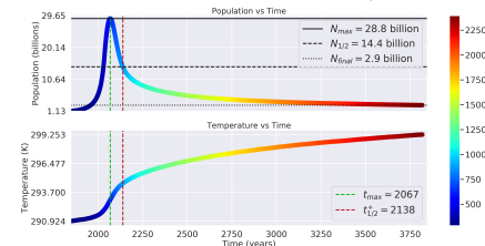
Distance: 0.993 AU, Carrying Capacity: 70 billion ppl, T_{eq} : 290.924K
