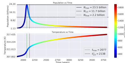
Distance: 0.967 AU, Carrying Capacity: 70 billion ppl, T_{eq} : 307.802K
