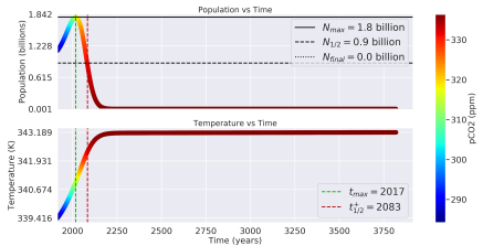
Distance: 0.94 AU, Carrying Capacity: 40 billion ppl, T_{eq} : 339.416K
