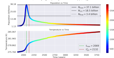
Distance: 1.02 AU, Carrying Capacity: 100 billion ppl, T_{eq} : 275.796K
