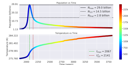
Distance: 1.02 AU, Carrying Capacity: 70 billion ppl, T_{eq} : 275.796K
