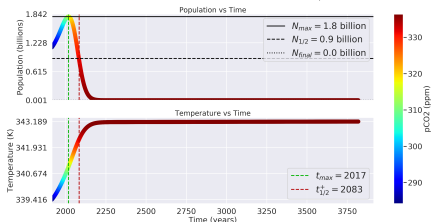
Distance: 0.94 AU, Carrying Capacity: 70 billion ppl, T_{eq} : 339.416K
