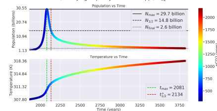
Distance: 0.967 AU, Carrying Capacity: 100 billion ppl, T_{eq} : 307.802K
