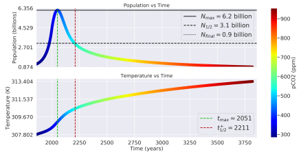
Distance: 0.967 AU, Carrying Capacity: 40 billion ppl, T_{eq} : 307.802K
