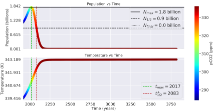
Distance: 0.94 AU, Carrying Capacity: 40 billion ppl, T_{eq} : 339.416K
