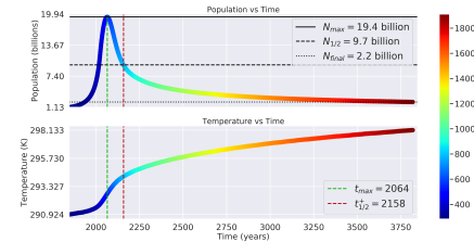
Distance: 0.993 AU, Carrying Capacity: 40 billion ppl, T_{eq} : 290.924K
