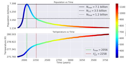
Distance: 1.02 AU, Carrying Capacity: 40 billion ppl, T_{eq} : 275.796K
