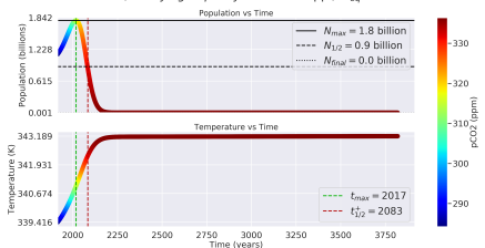
Distance: 0.94 AU, Carrying Capacity: 100 billion ppl, T_{eq} : 339.416K
