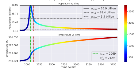
Distance: 0.993 AU, Carrying Capacity: 100 billion ppl, T_{eq} : 290.924K
