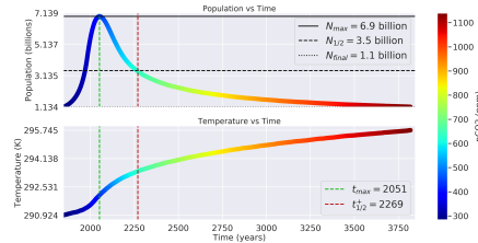
Distance: 0.993 AU, Carrying Capacity: 40 billion ppl, T_{eq} : 290.924K
