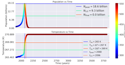
Distance: 1.03 AU, Carrying Capacity: 70 billion ppl, \Lambda : 0.126
