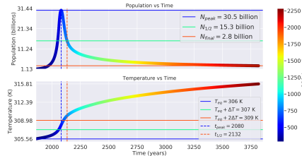
Distance: 0.97 AU, Carrying Capacity: 100 billion ppl, \Lambda : 0.35
