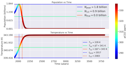
Distance: 0.94 AU, Carrying Capacity: 100 billion ppl, \Lambda : 0.032
