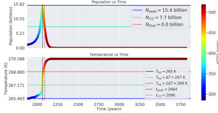
Distance: 1.03 AU, Carrying Capacity: 40 billion ppl, \Lambda : 0.221
