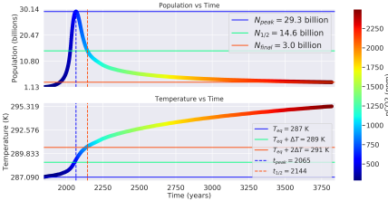
Distance: 1.0 AU, Carrying Capacity: 70 billion ppl, \Lambda : 0.732
