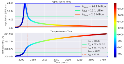
Distance: 0.97 AU, Carrying Capacity: 70 billion ppl, \Lambda : 0.5
