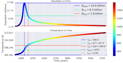
Distance: 0.97 AU, Carrying Capacity: 40 billion ppl, \Lambda : 0.876
