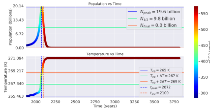
Distance: 1.03 AU, Carrying Capacity: 100 billion ppl, \Lambda : 0.088
