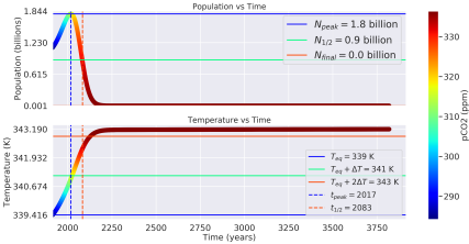
Distance: 0.94 AU, Carrying Capacity: 70 billion ppl, \Lambda : 0.056
