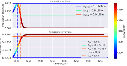
Distance: 0.94 AU, Carrying Capacity: 40 billion ppl, \Lambda : 0.225
