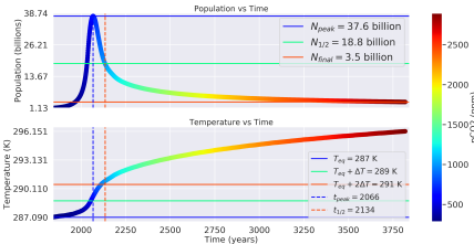
Distance: 1.0 AU, Carrying Capacity: 100 billion ppl, \Lambda : 0.512
