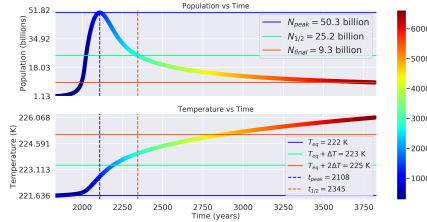
Distance: 1.06 AU, Carrying Capacity: 70 billion ppl, \Lambda : 3.771
