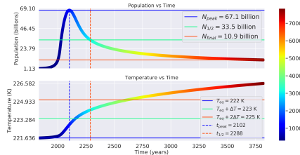
Distance: 1.06 AU, Carrying Capacity: 100 billion ppl, \Lambda : 2.64
