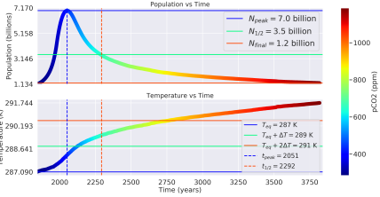
Distance: 1.0 AU, Carrying Capacity: 40 billion ppl, \Lambda : 1.28
