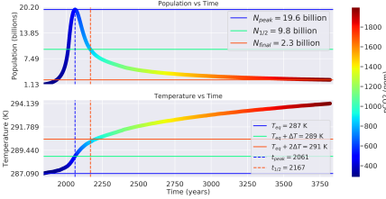
Distance: 1.0 AU, Carrying Capacity: 40 billion ppl, \Lambda : 1.28
