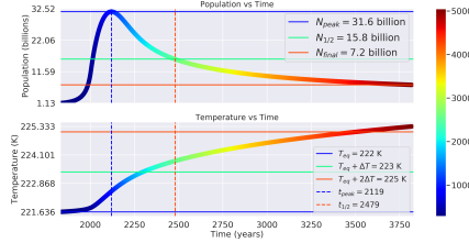
Distance: 1.06 AU, Carrying Capacity: 40 billion ppl, \Lambda : 6.599
