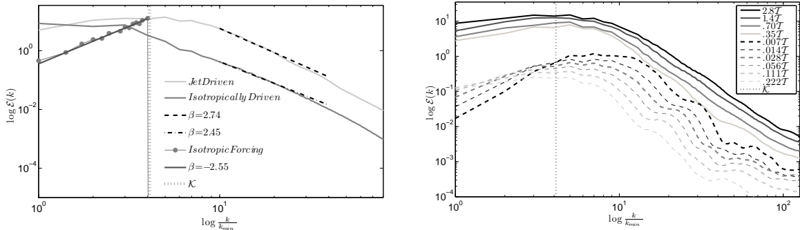
Fig. 3.— The left panel shows a comparison of the velocity power spectrum for the outflow driven turbulence and the isotropically forced turbulence at 3\mathcal{T} . The right panel shows the development of the power spectra for both single and multiple outflow runs. The characteristic wave number for the outflows \mathcal{K} = \frac{2\pi}{\mathcal{L}} is shown for reference.
