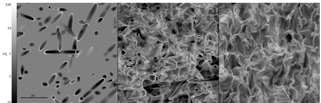
Fig. 1.— Cross cuts of log density for the outflow driven turbulence at .5\mathcal{T} (Left), and at 2.6\mathcal{T} (Center) as well as for the isotropically forced turbulence (Right). Note the interaction of outflow shells at early times (Left) and the presence of distinct “holes” in the turbulent density distribution at later times (Center).
