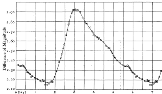
FIG. 1.—Light-Curve of \delta Cephei.
