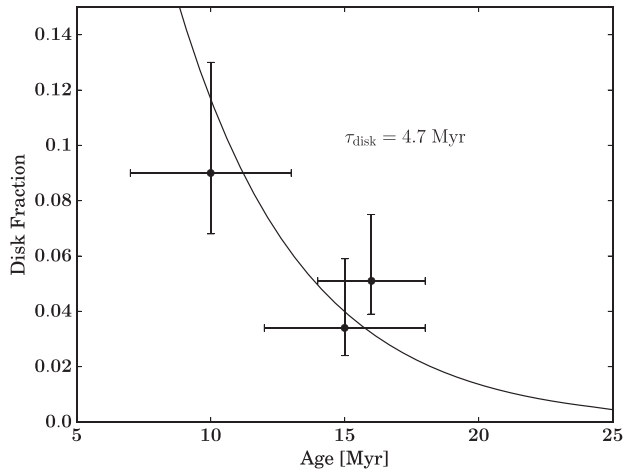
Figure 16. Mean subgroup age versus disc fraction (‘Full Disc’; see Table 13) for K-type stars, \sim 0.7\text{--}1.3\ M_{\odot} , from the three subgroups of Sco–Cen. The best-fitting exponential decay curve f_{\text{disc}} = e^{-t/\tau_{\text{disc}}} has \tau_{\text{disc}} = 4.7\ \text{Myr} .
