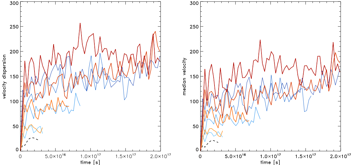
Figure 3. The evolution of the velocity dispersion (left panel) and median velocity within the central 100 kpc (all in \text{km s}^{-1} ). Blue (red) lines are for 100 (200) galaxies respectively, for equally spaced masses ranging from 3 \times 10^{11} M_{\odot} to 1.2 \times 10^{12} M_{\odot} . The galaxy mass increases gradually from the lightest to the darkest color. The black dashed line is for the pure HBI case, where there is no stirring. The run is halted at early times if a cooling catastrophe occurs.
