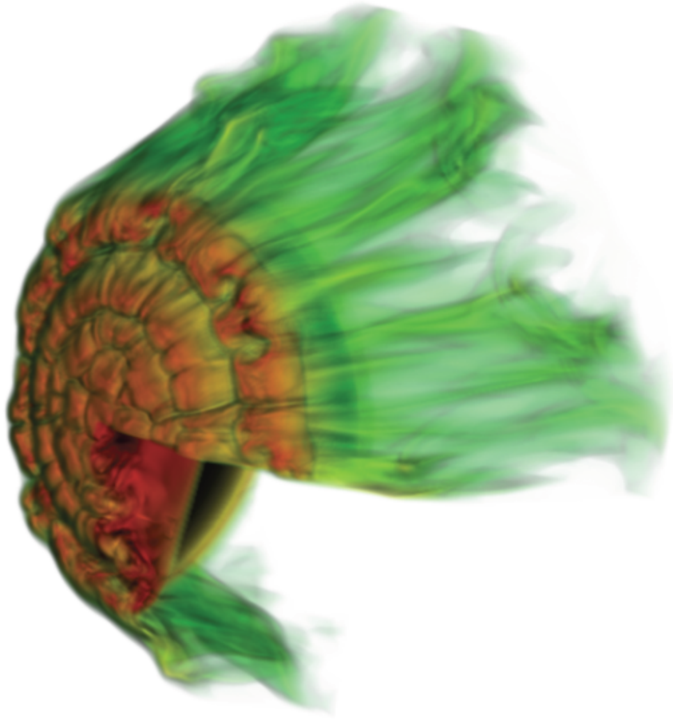
3D radiative shocked clump (1 quadrant, reflected)
